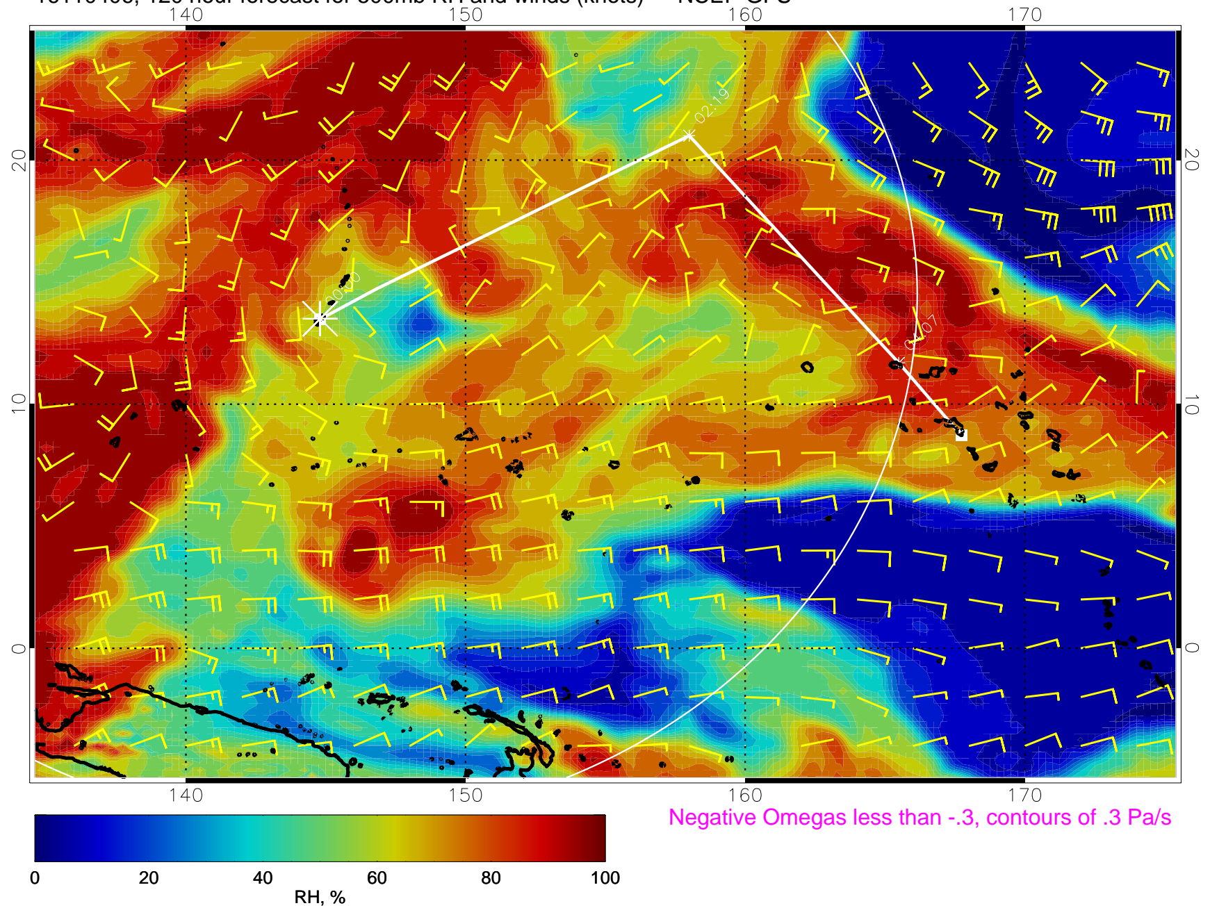
16110406, 120 hour forecast for 500mb RH and winds (knots) -- NCEP GFS
