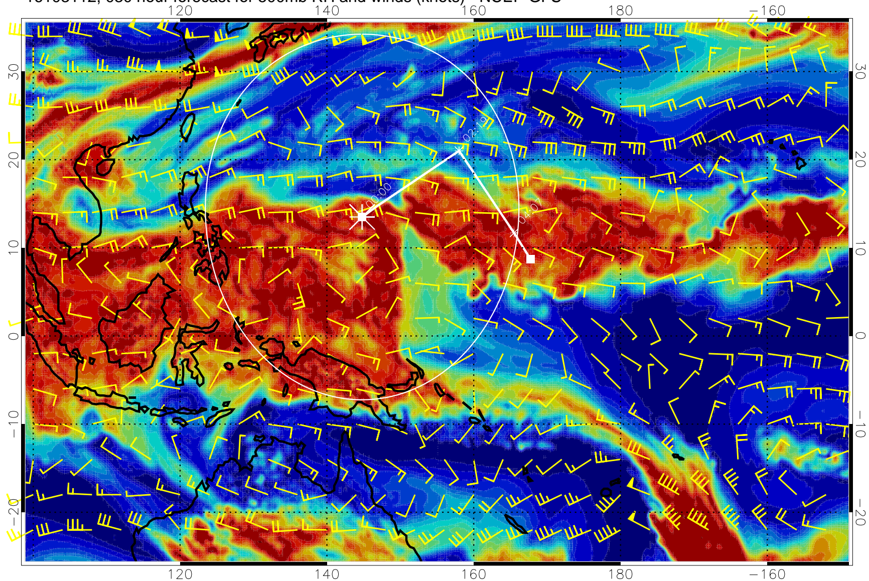
16103112, 030 hour forecast for 500mb RH and winds (knots) - NCEP GFS
