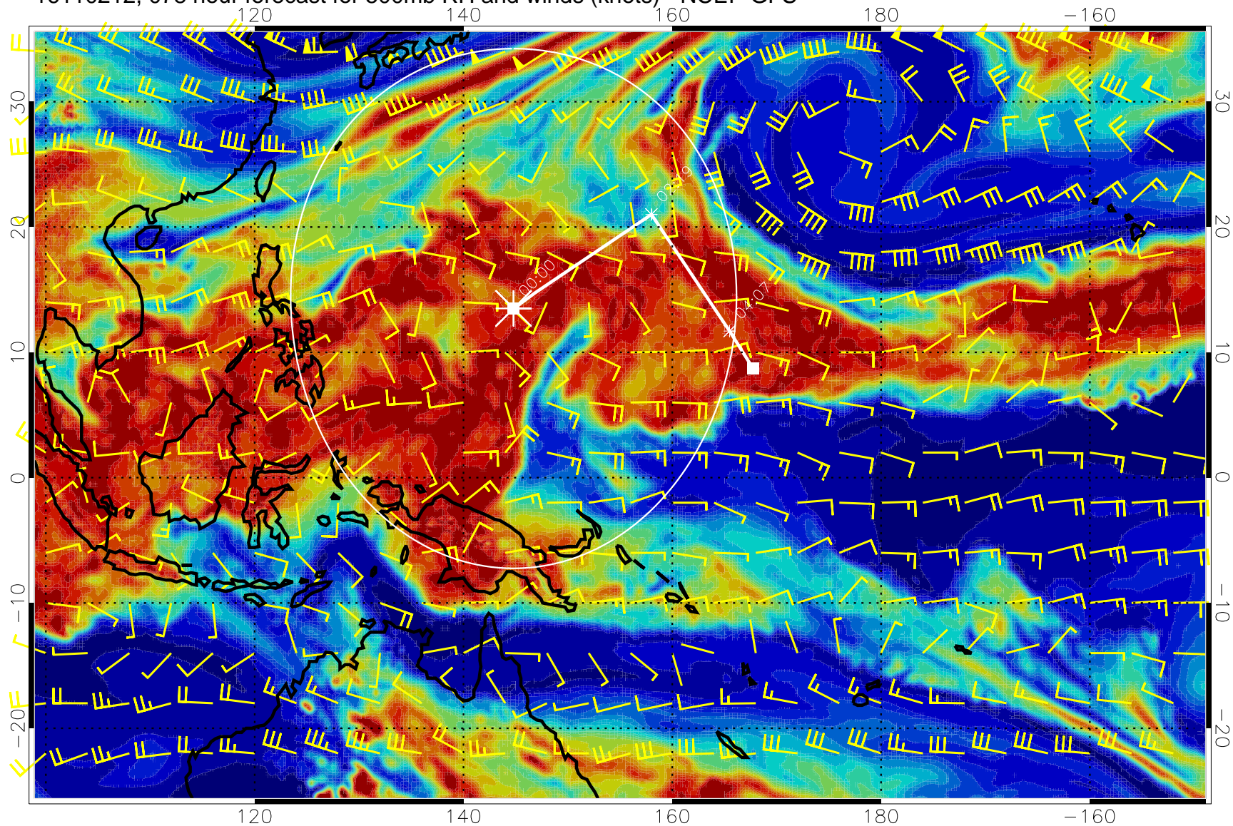
16110212, 078 hour forecast for 500mb RH and winds (knots) - NCEP GFS
