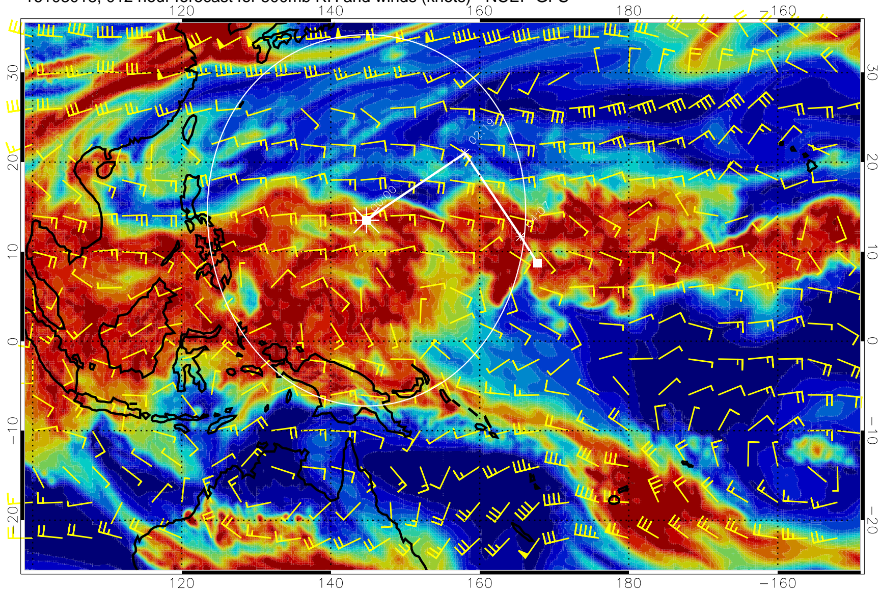
16103018, 012 hour forecast for 500mb RH and winds (knots) - NCEP GFS
