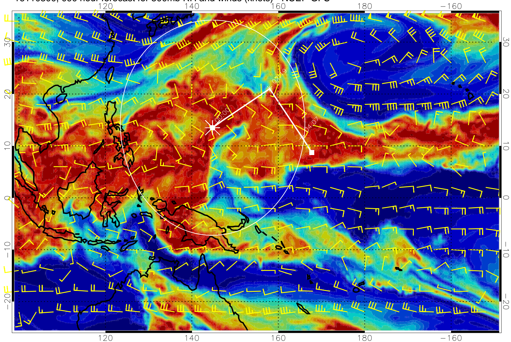
16110300, 090 hour forecast for 500mb RH and winds (knots) - NCEP GFS
