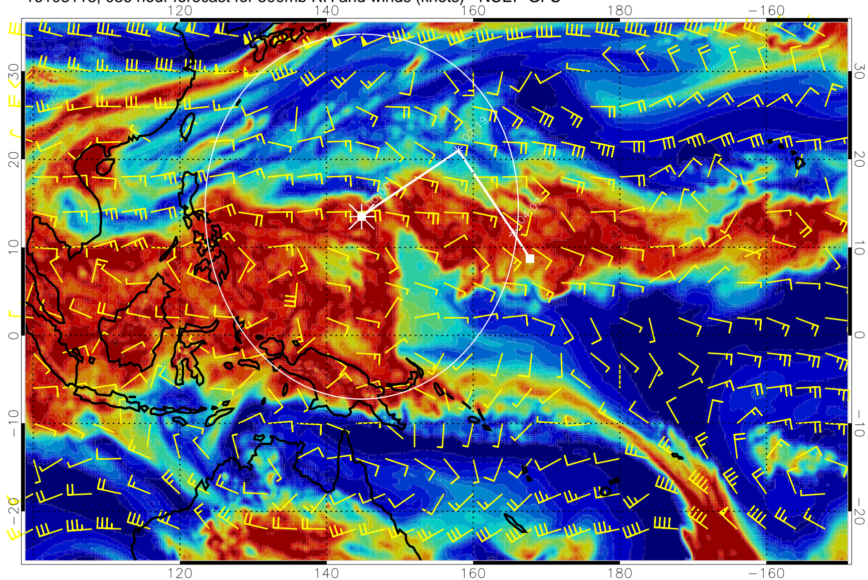
16103118, 036 hour forecast for 500mb RH and winds (knots) - NCEP GFS
