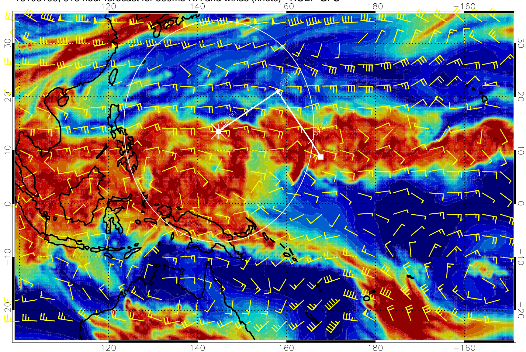
16103100, 018 hour forecast for 500mb RH and winds (knots) - NCEP GFS
