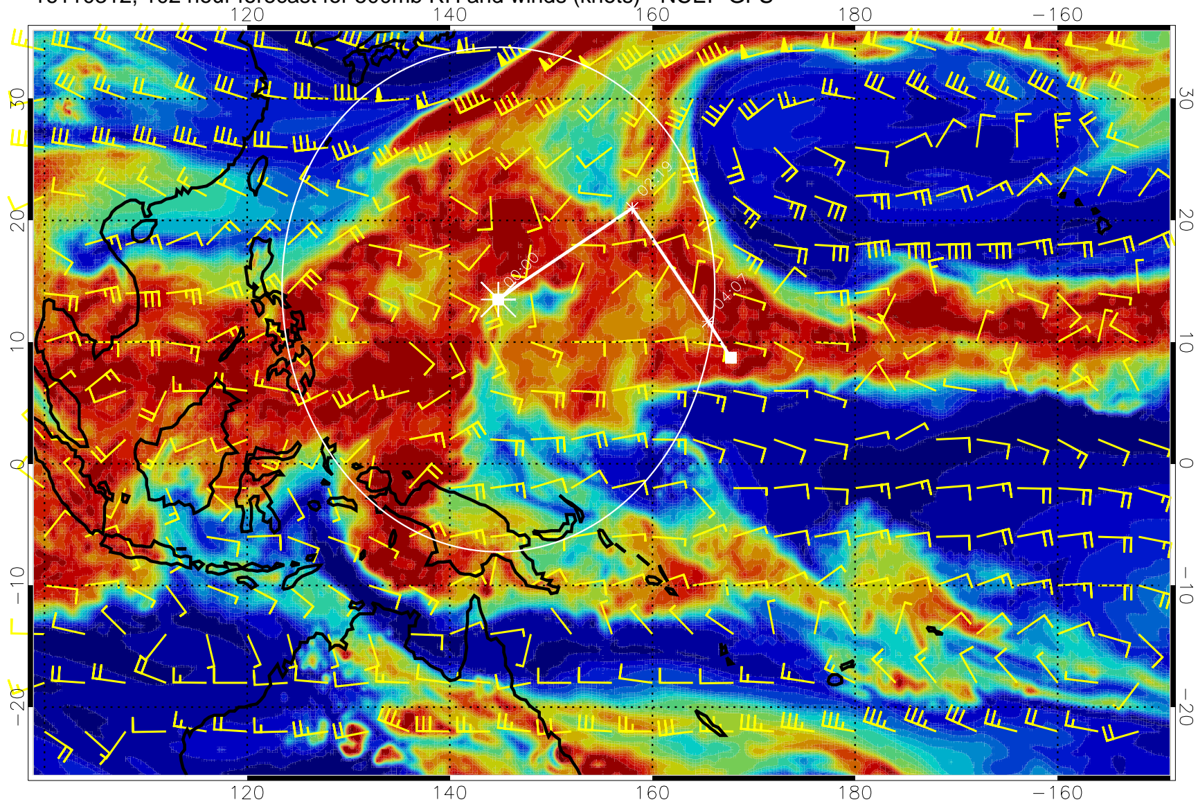
16110312, 102 hour forecast for 500mb RH and winds (knots) - NCEP GFS
