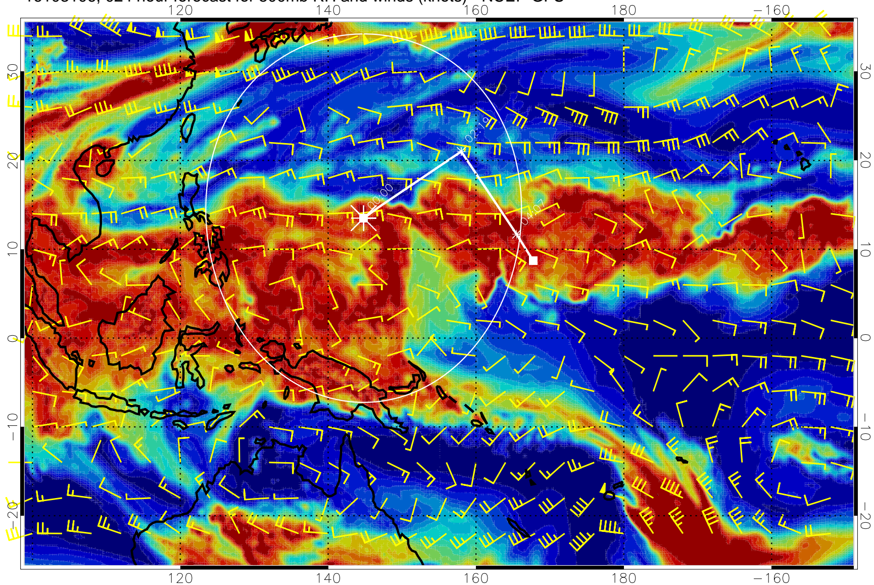
16103106, 024 hour forecast for 500mb RH and winds (knots) - NCEP GFS
