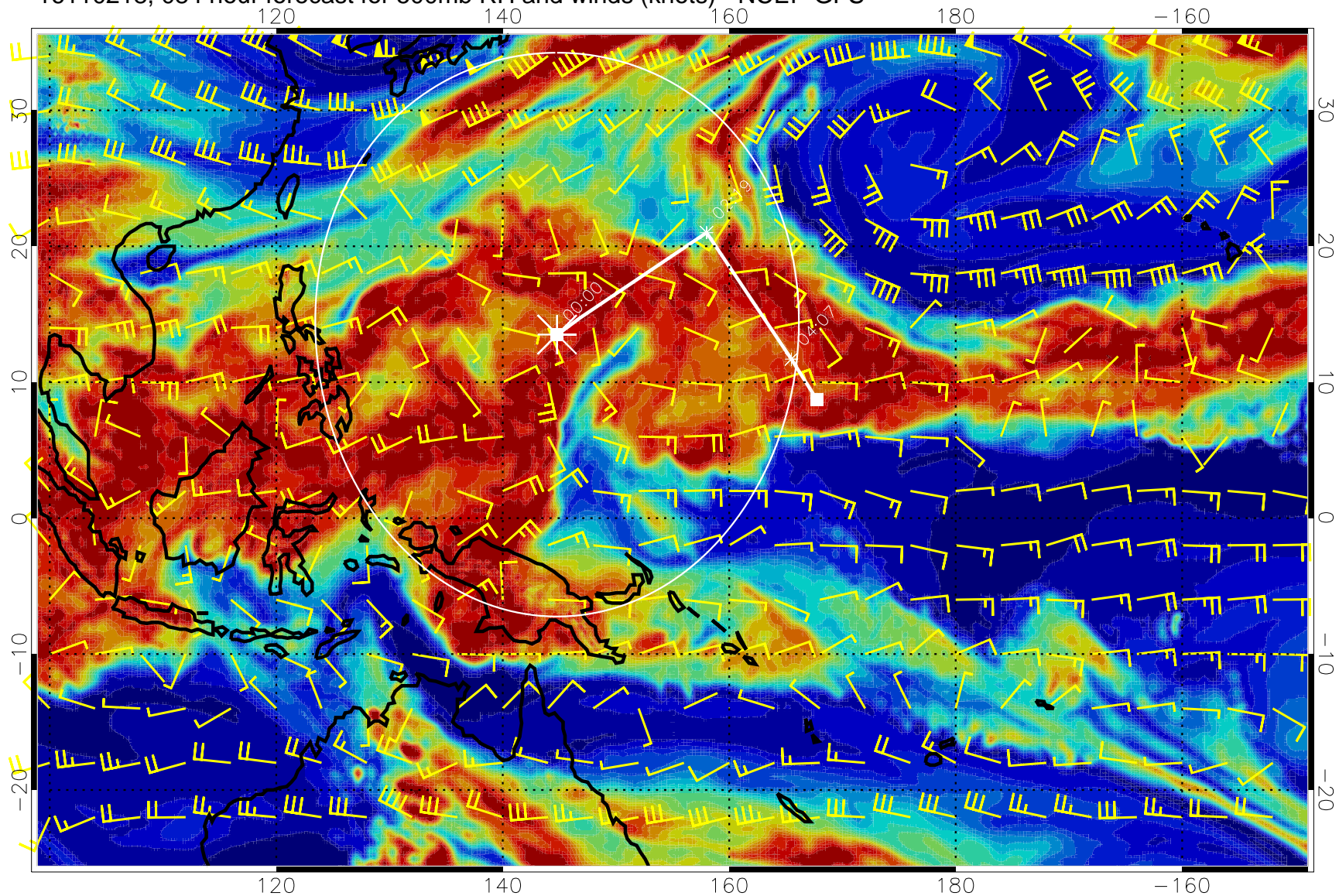
16110218, 084 hour forecast for 500mb RH and winds (knots) - NCEP GFS
