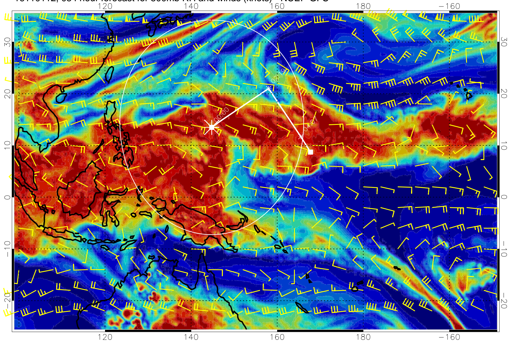
16110112, 054 hour forecast for 500mb RH and winds (knots) - NCEP GFS
