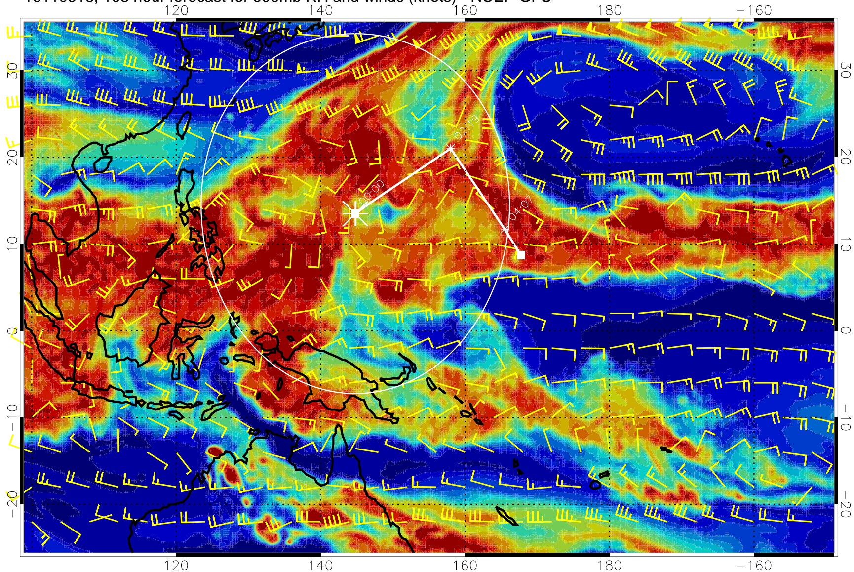
16110318, 108 hour forecast for 500mb RH and winds (knots) - NCEP GFS
