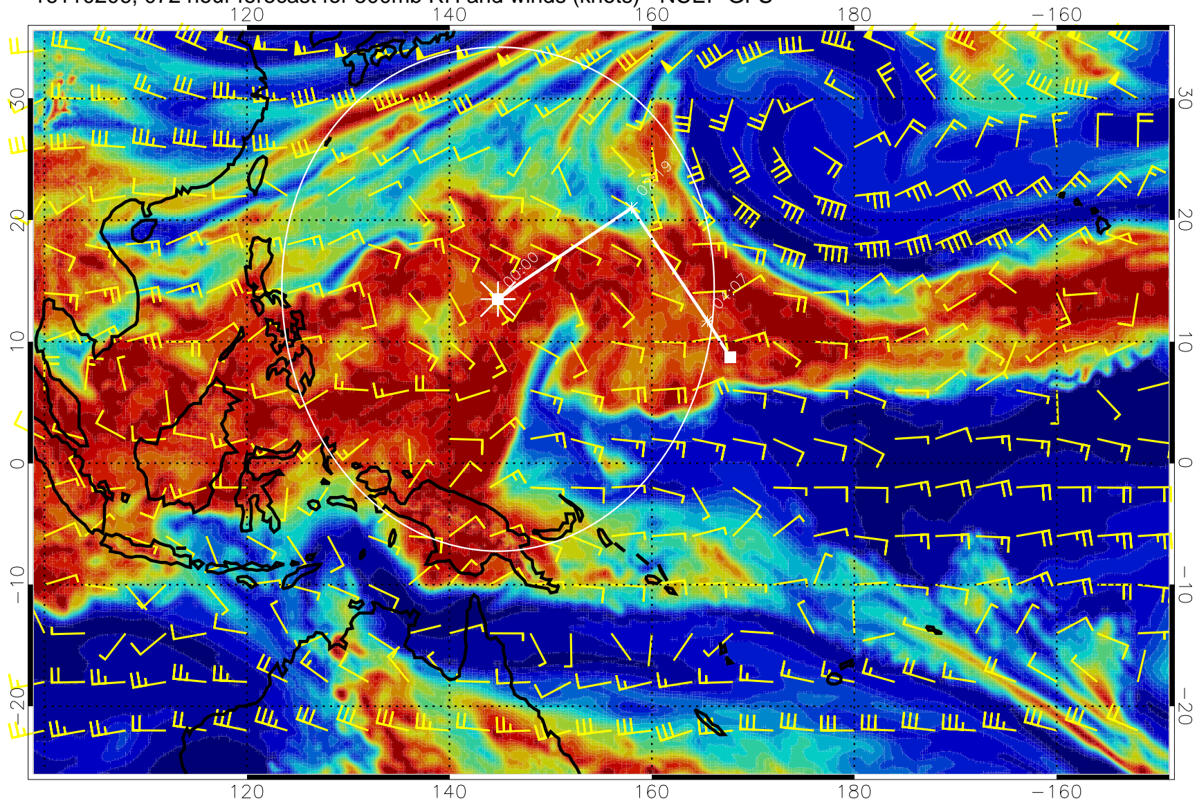
16110206, 072 hour forecast for 500mb RH and winds (knots) - NCEP GFS
