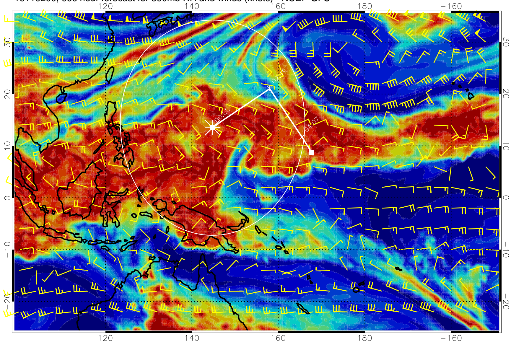
16110200, 066 hour forecast for 500mb RH and winds (knots) - NCEP GFS
