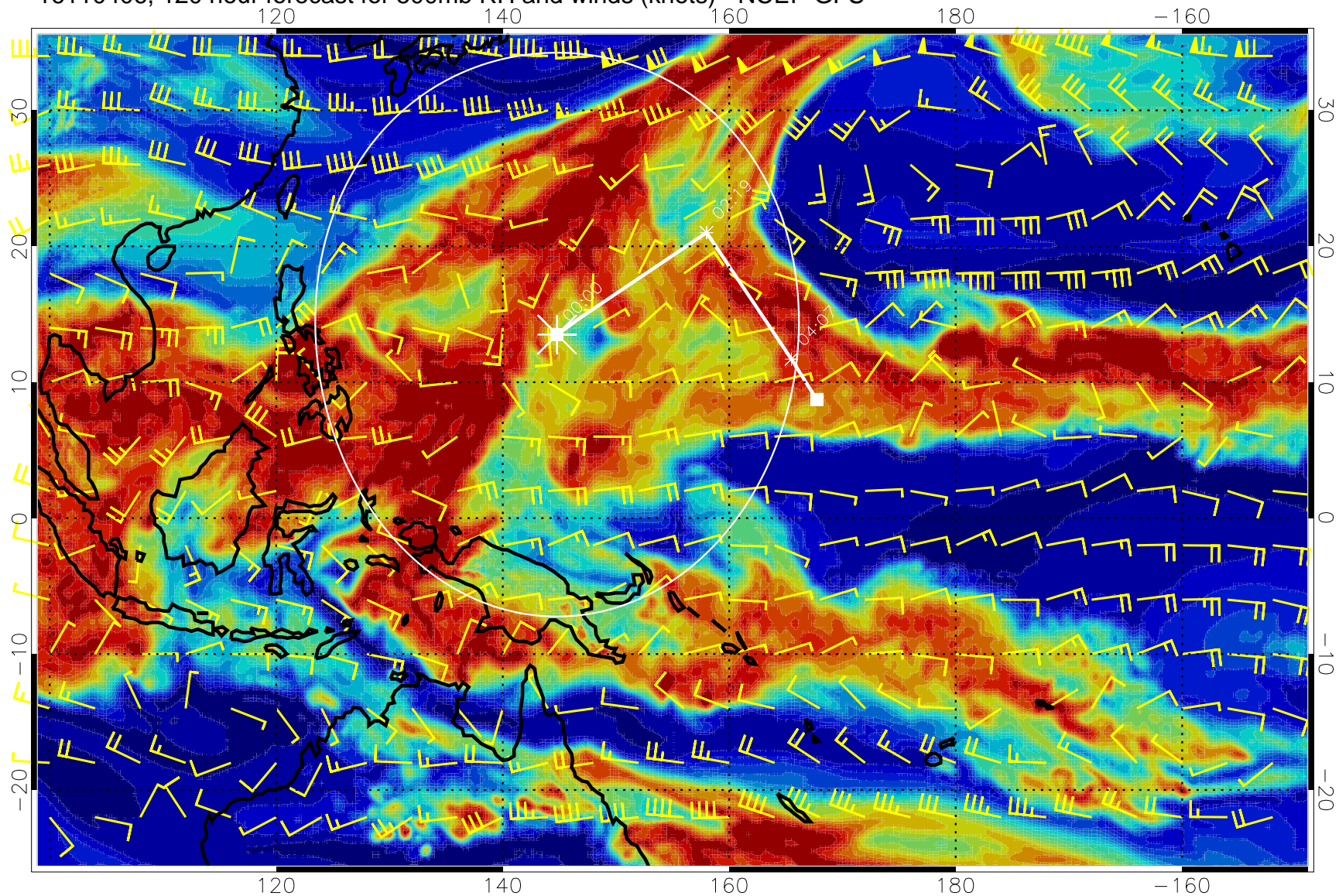
16110406, 120 hour forecast for 500mb RH and winds (knots) - NCEP GFS
