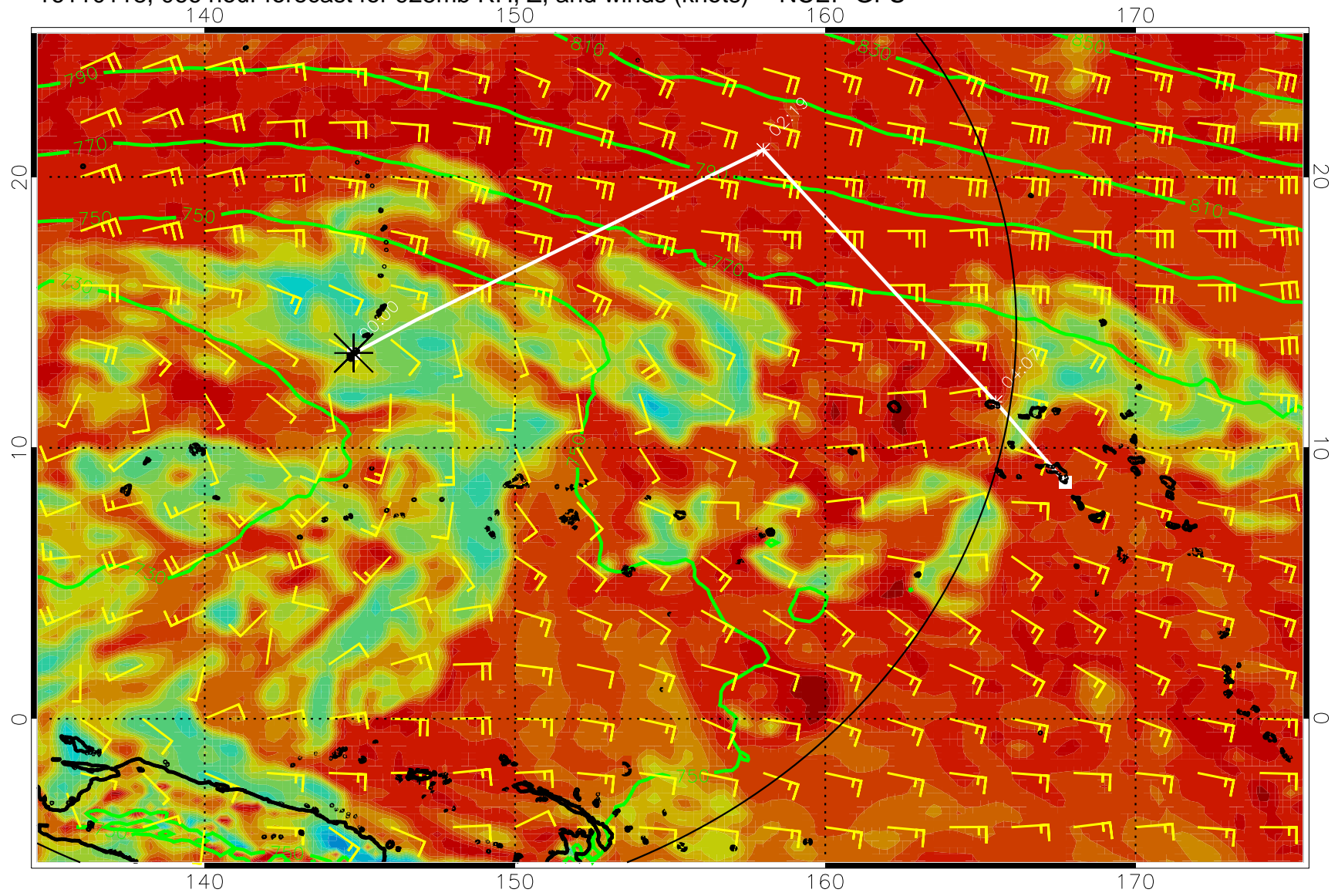
16110118, 066 hour forecast for 925mb RH, Z, and winds (knots) -- NCEP GFS
