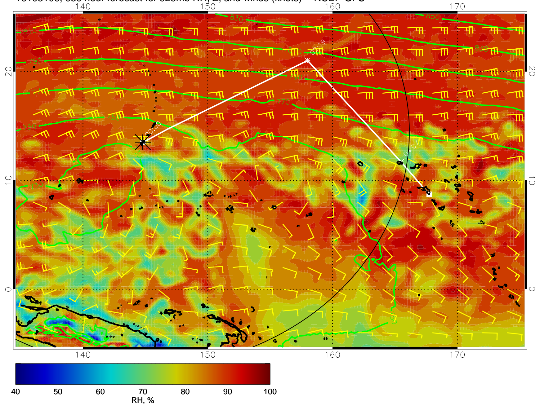
16103106, 030 hour forecast for 925mb RH, Z, and winds (knots) -- NCEP GFS
