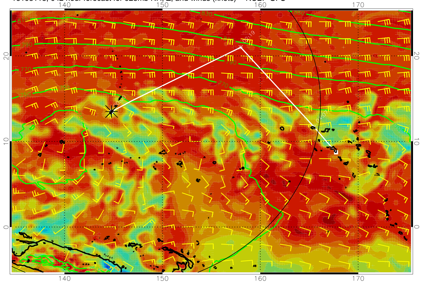
16103118, 042 hour forecast for 925mb RH, Z, and winds (knots) -- NCEP GFS
