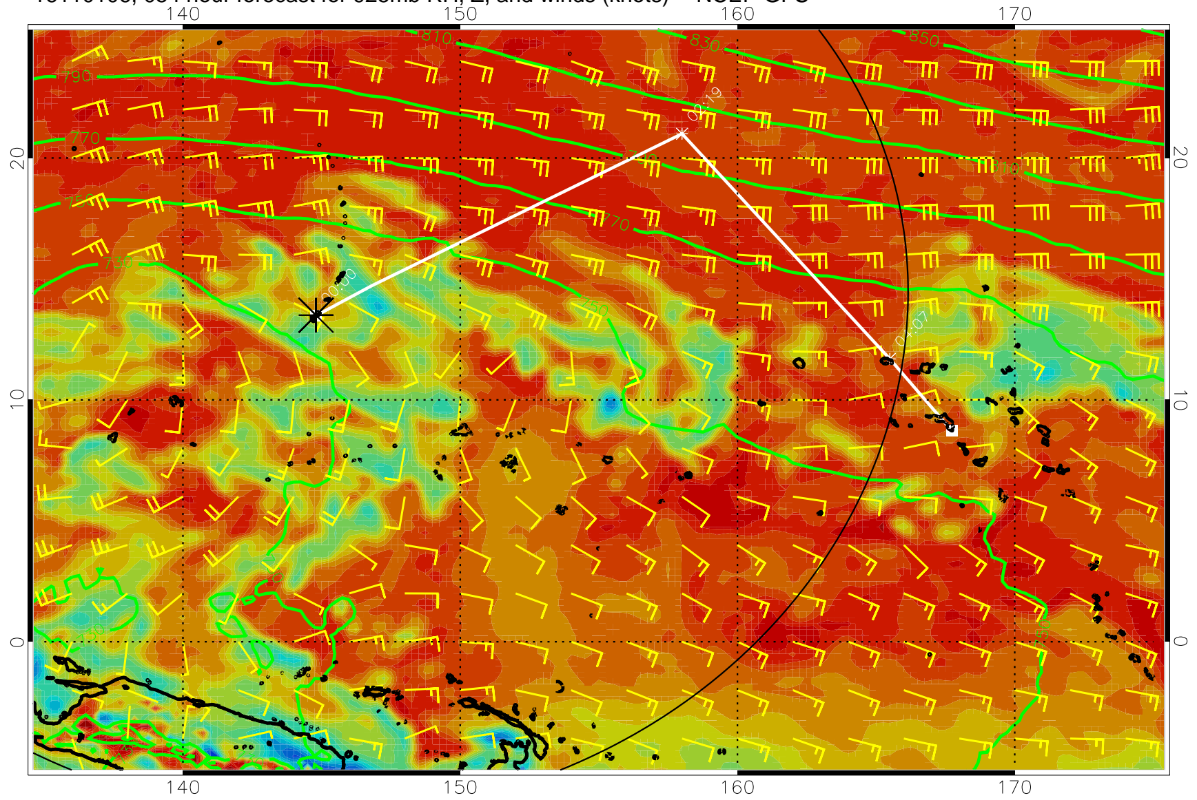
16110106, 054 hour forecast for 925mb RH, Z, and winds (knots) -- NCEP GFS
