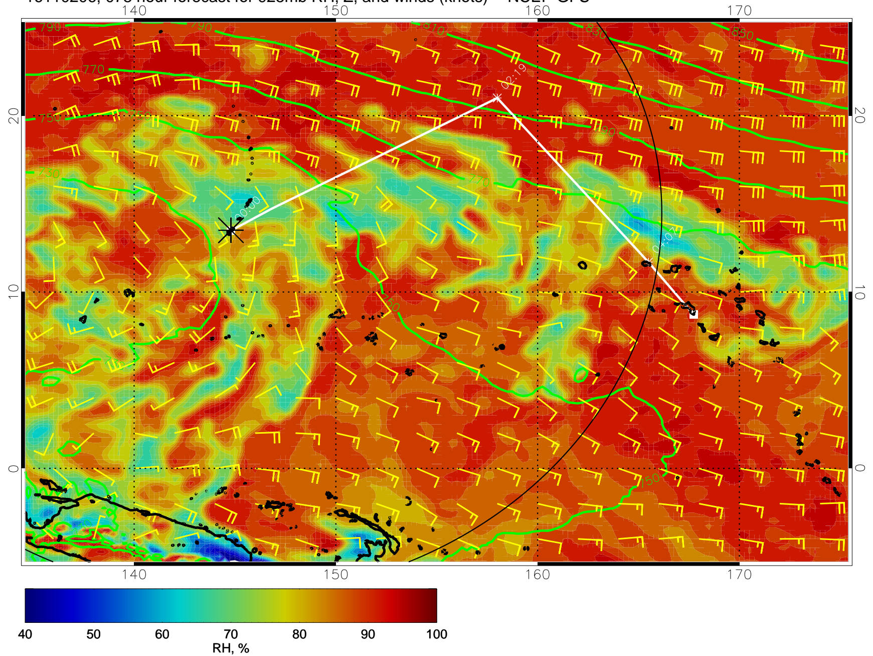
16110206, 078 hour forecast for 925mb RH, Z, and winds (knots) -- NCEP GFS
