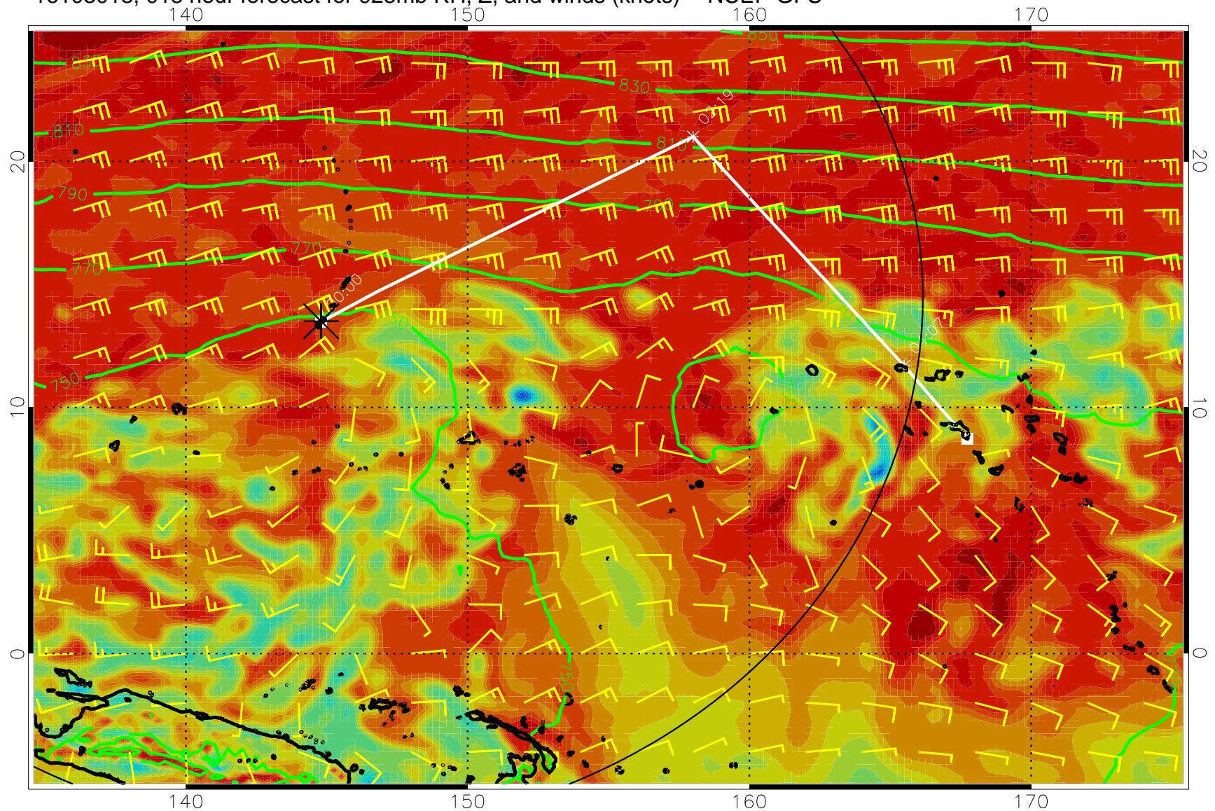
16103018, 018 hour forecast for 925mb RH, Z, and winds (knots) -- NCEP GFS
