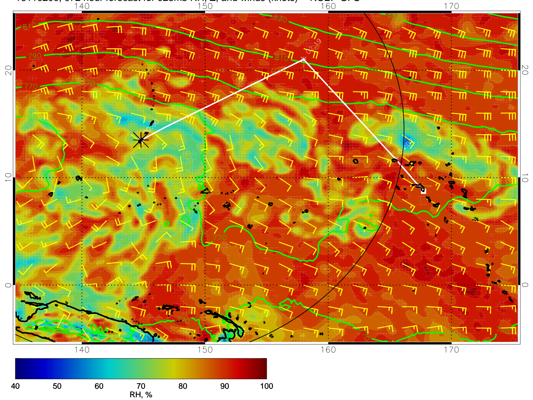
16110200, 072 hour forecast for 925mb RH, Z, and winds (knots) -- NCEP GFS
