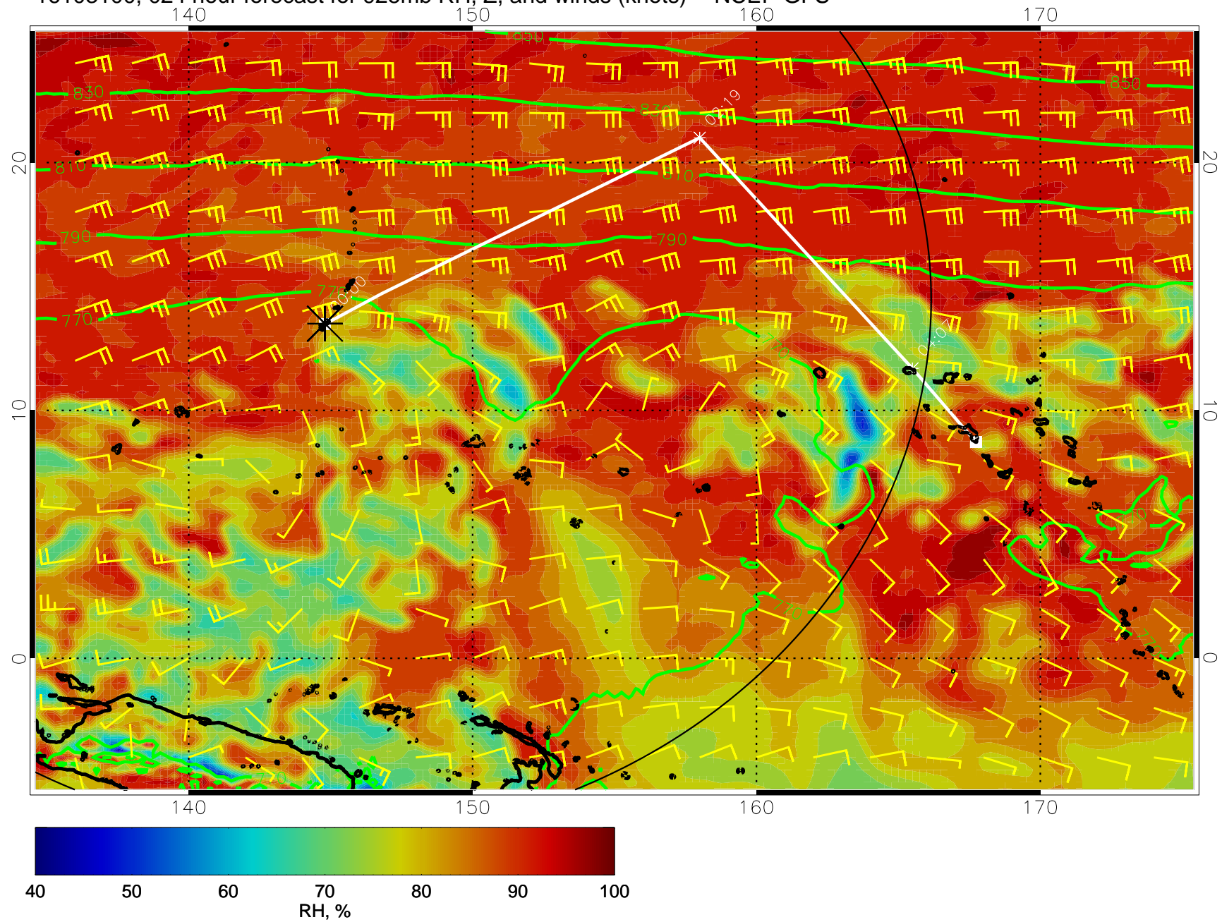
16103100, 024 hour forecast for 925mb RH, Z, and winds (knots) -- NCEP GFS
