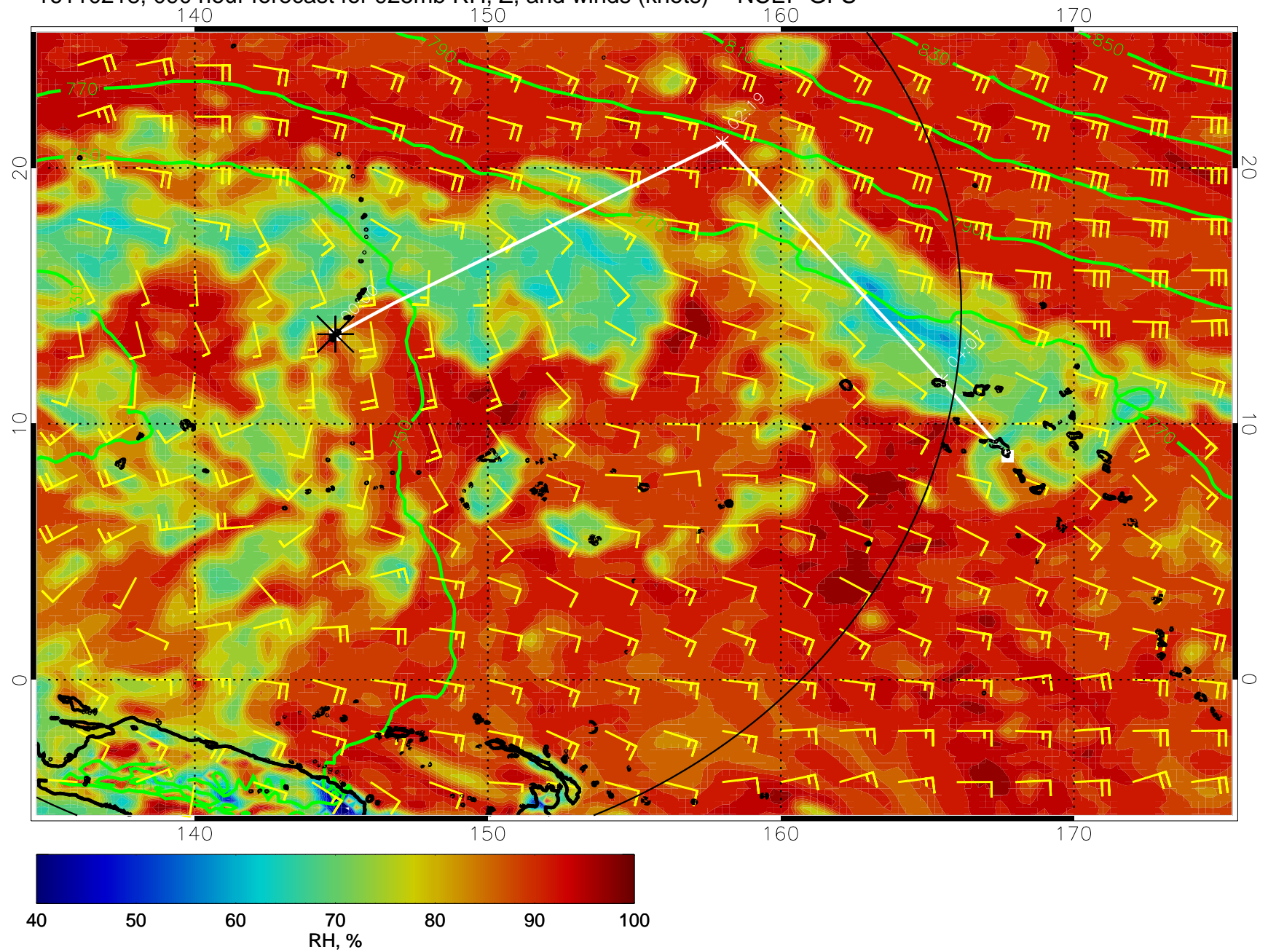
16110218, 090 hour forecast for 925mb RH, Z, and winds (knots) -- NCEP GFS
