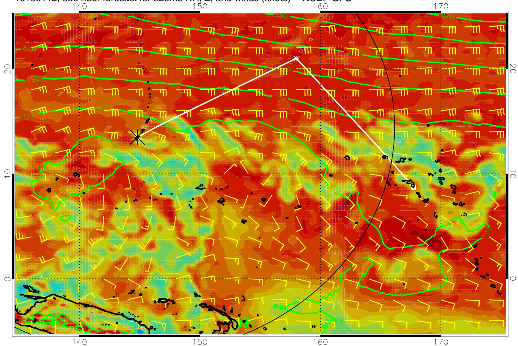
16103112, 036 hour forecast for 925mb RH, Z, and winds (knots) -- NCEP GFS
