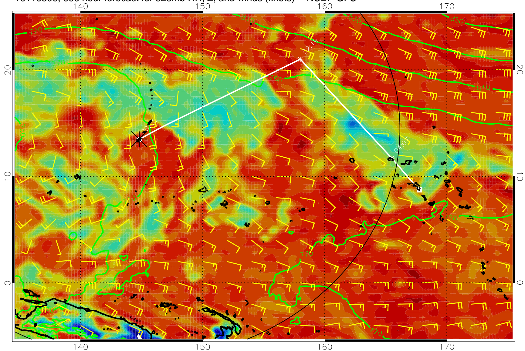
16110300, 096 hour forecast for 925mb RH, Z, and winds (knots) -- NCEP GFS
