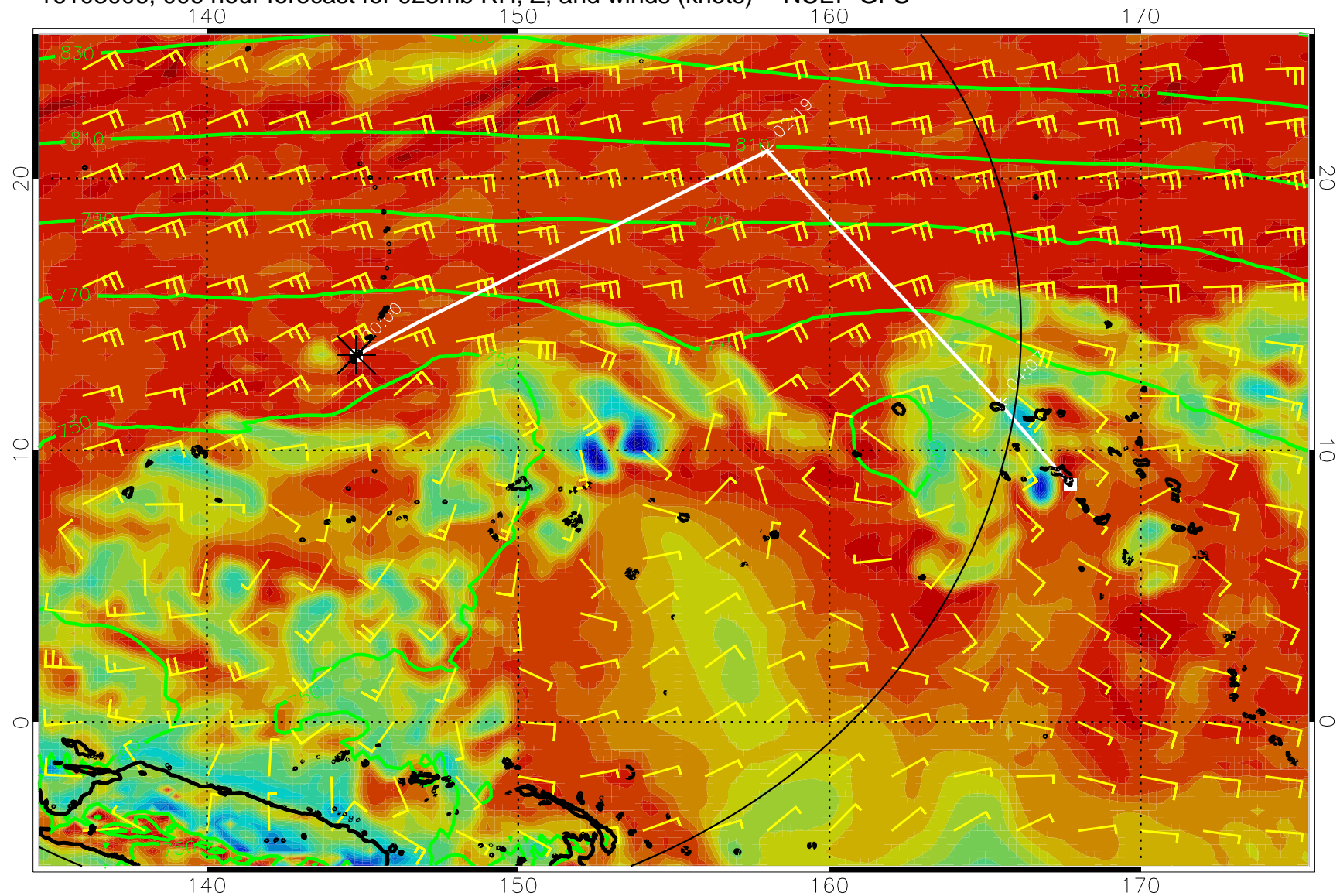
16103006, 006 hour forecast for 925mb RH, Z, and winds (knots) -- NCEP GFS
