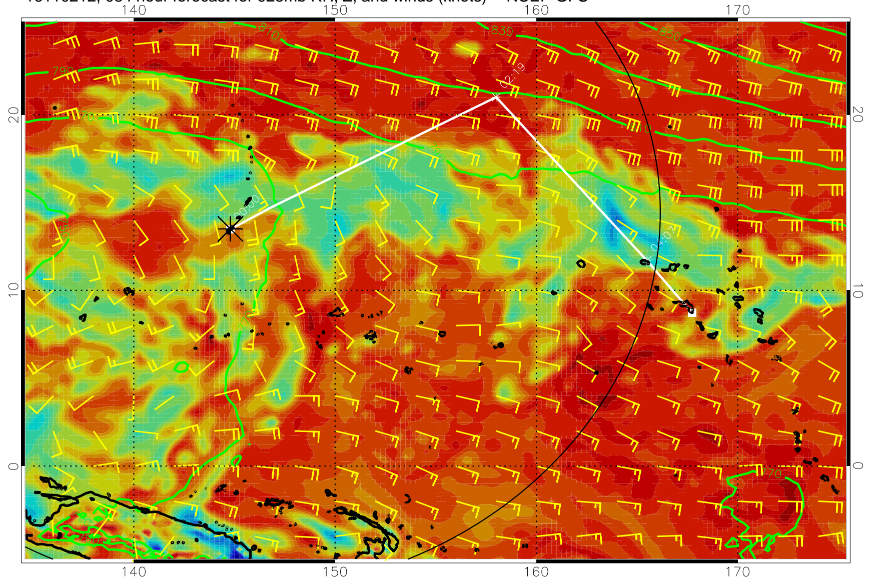
16110212, 084 hour forecast for 925mb RH, Z, and winds (knots) -- NCEP GFS
