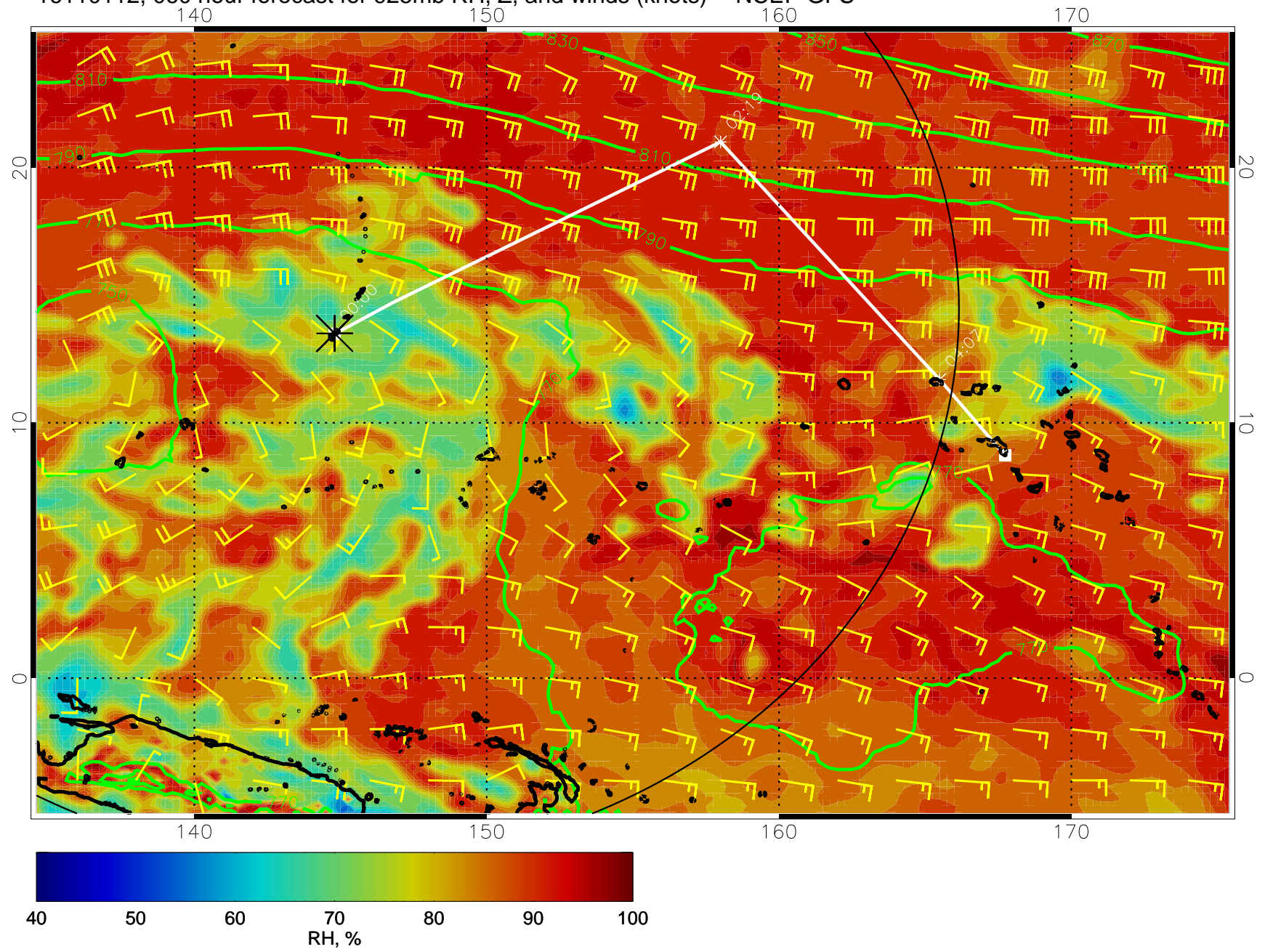
16110112, 060 hour forecast for 925mb RH, Z, and winds (knots) -- NCEP GFS
