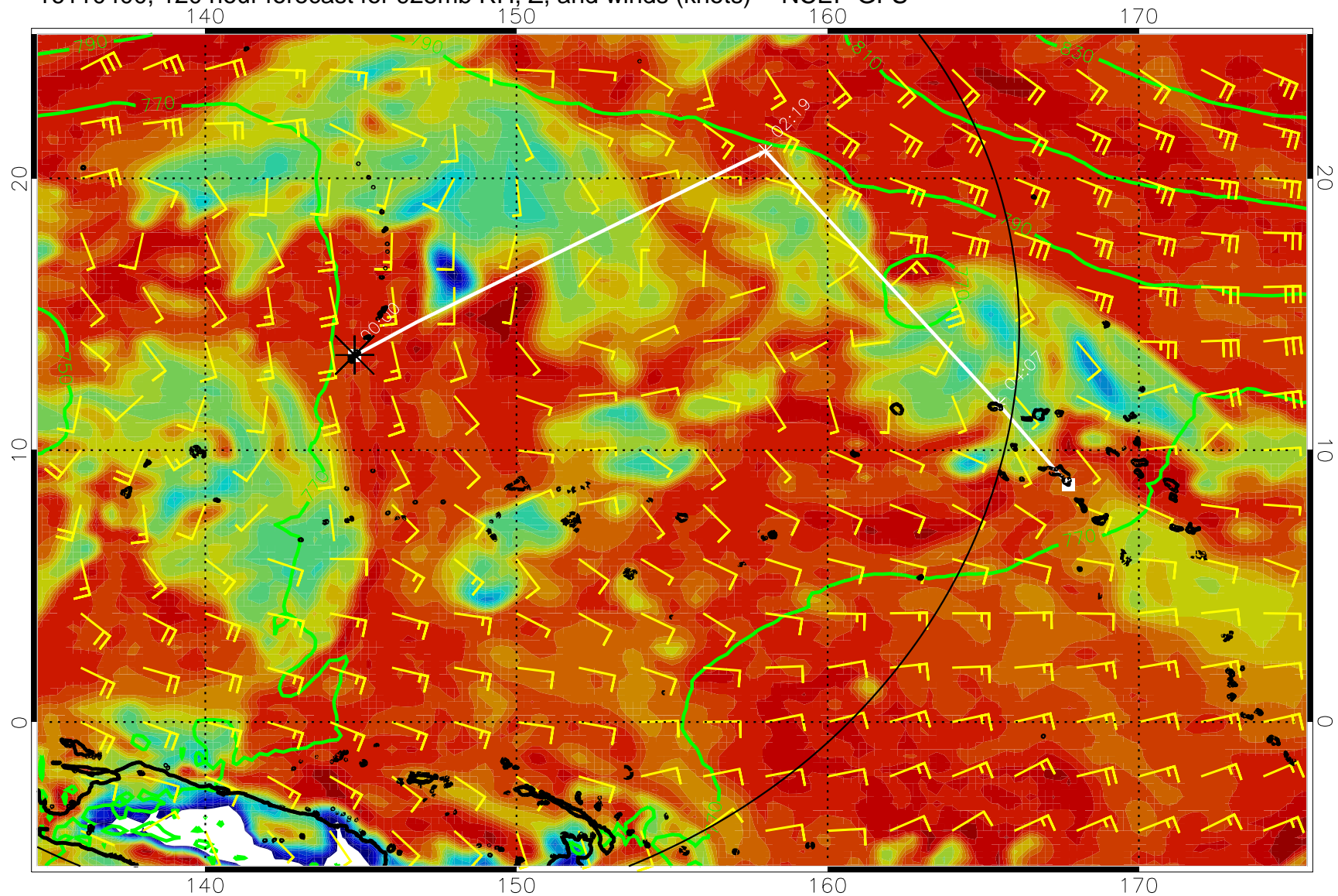
16110400, 120 hour forecast for 925mb RH, Z, and winds (knots) -- NCEP GFS
