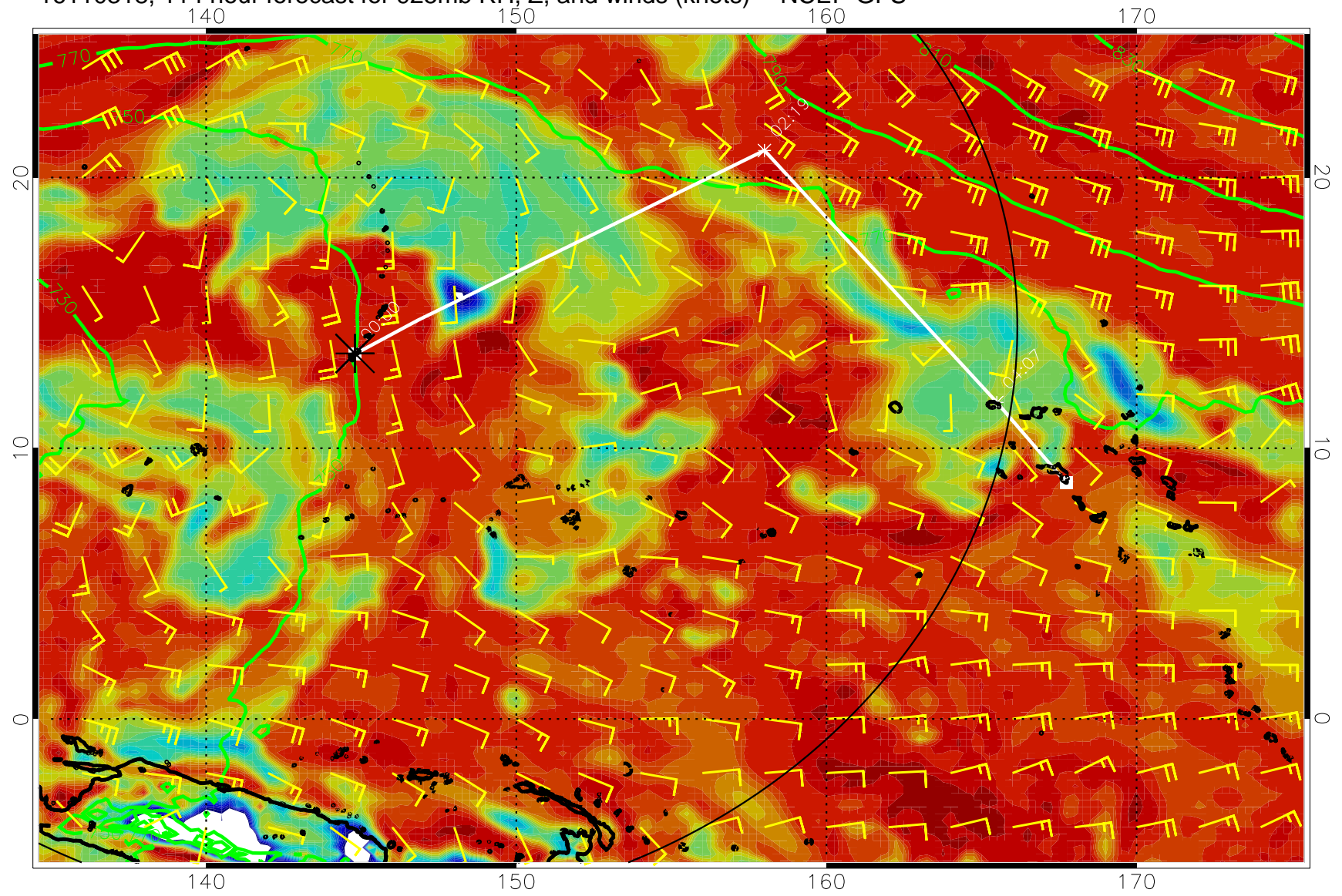
16110318, 114 hour forecast for 925mb RH, Z, and winds (knots) -- NCEP GFS
