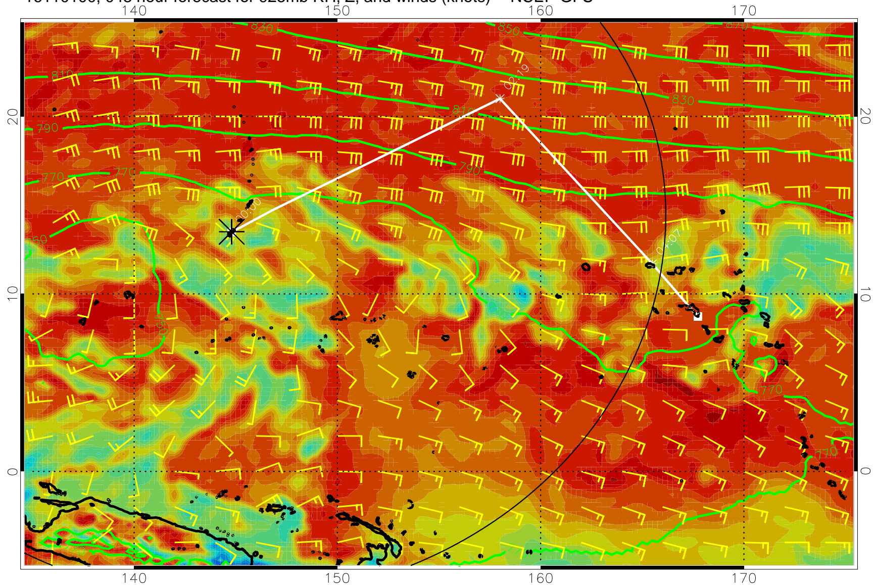
16110100, 048 hour forecast for 925mb RH, Z, and winds (knots) -- NCEP GFS
