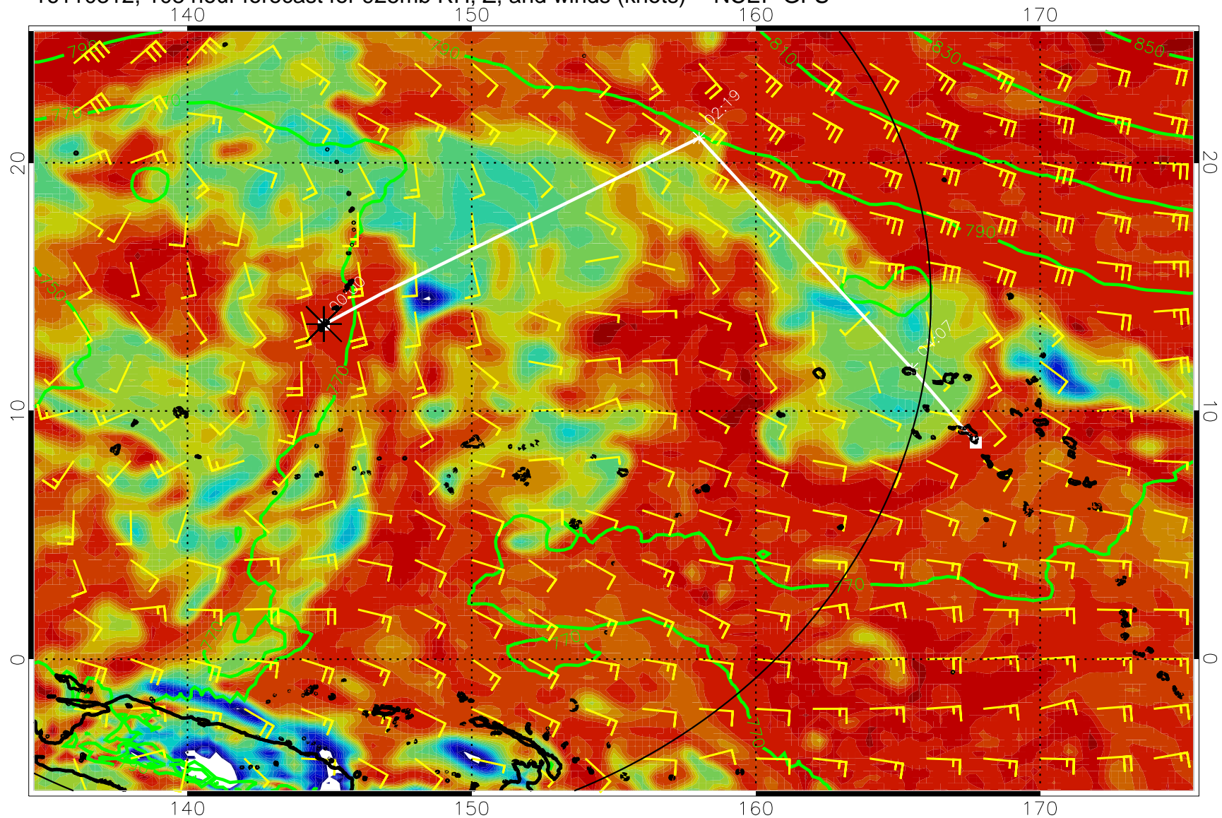
16110312, 108 hour forecast for 925mb RH, Z, and winds (knots) -- NCEP GFS
