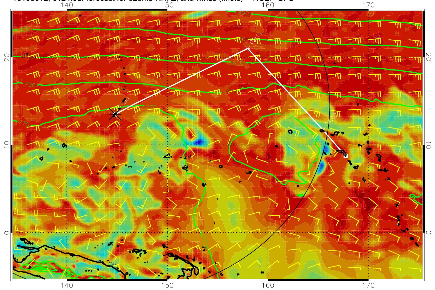
16103012, 012 hour forecast for 925mb RH, Z, and winds (knots) -- NCEP GFS
