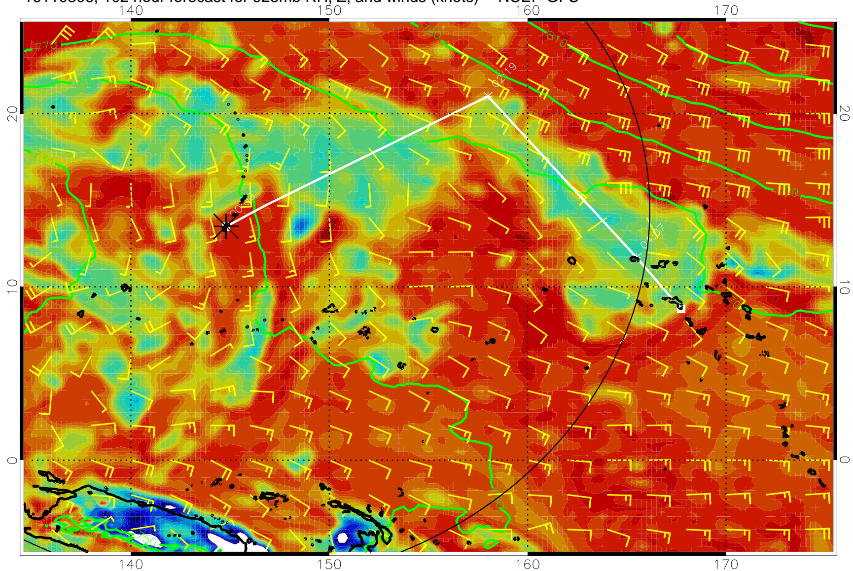
16110306, 102 hour forecast for 925mb RH, Z, and winds (knots) -- NCEP GFS
