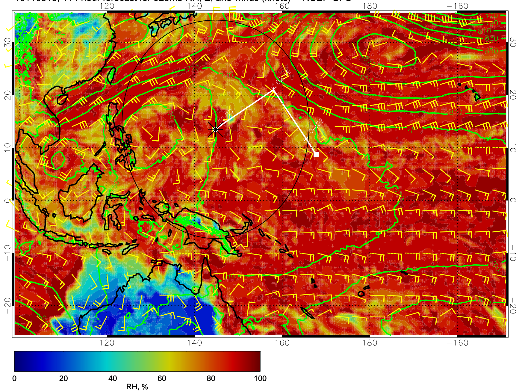
16110318, 114 hour forecast for 925mb RH, Z, and winds (knots) -- NCEP GFS
