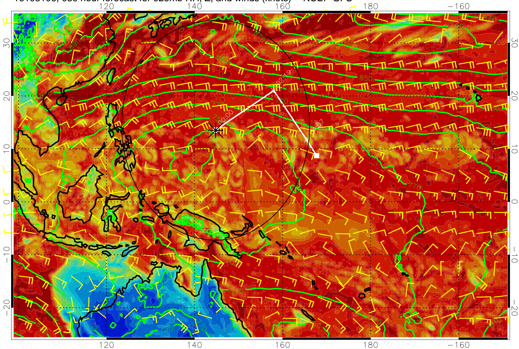
16103106, 030 hour forecast for 925mb RH, Z, and winds (knots) -- NCEP GFS
