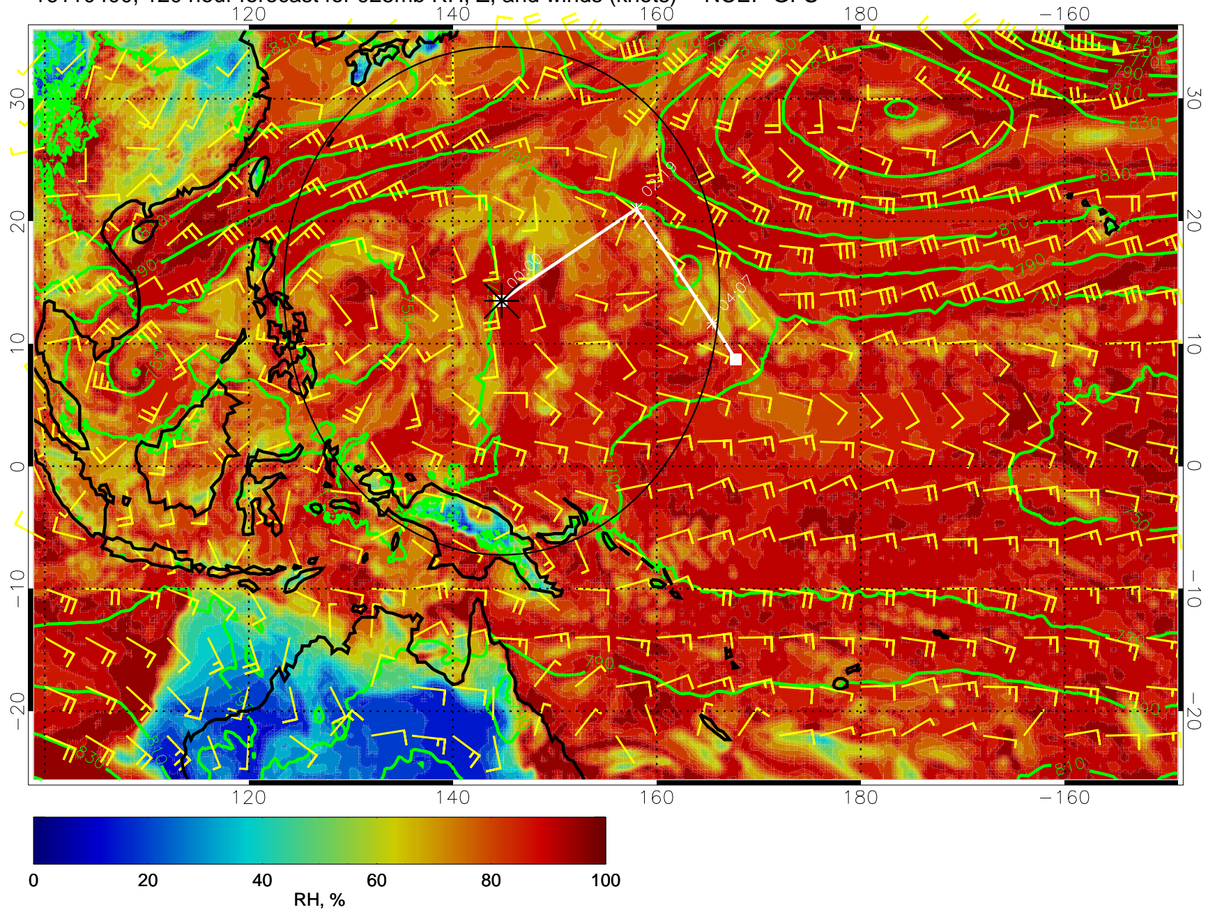
16110400, 120 hour forecast for 925mb RH, Z, and winds (knots) -- NCEP GFS
