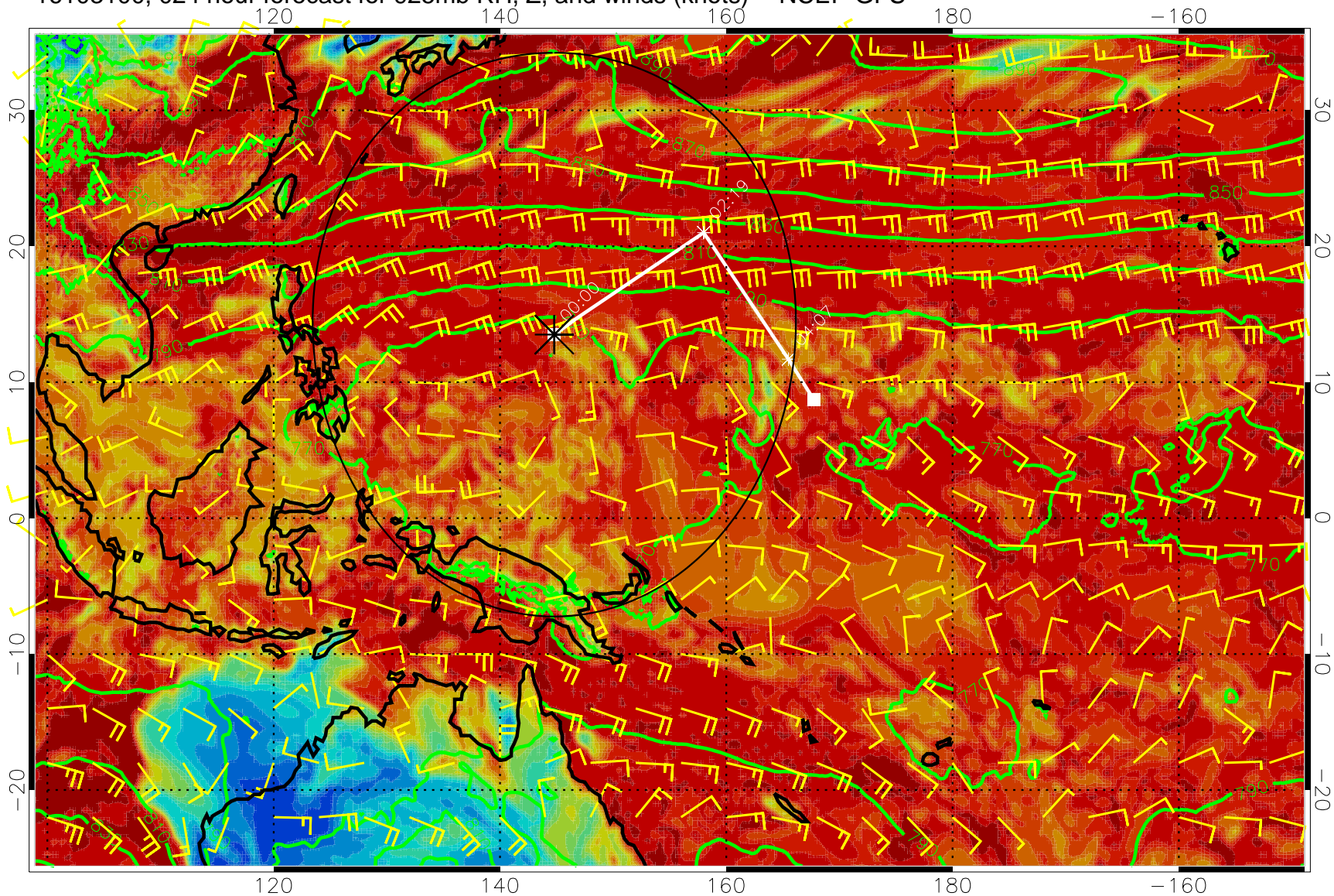
16103100, 024 hour forecast for 925mb RH, Z, and winds (knots) -- NCEP GFS
