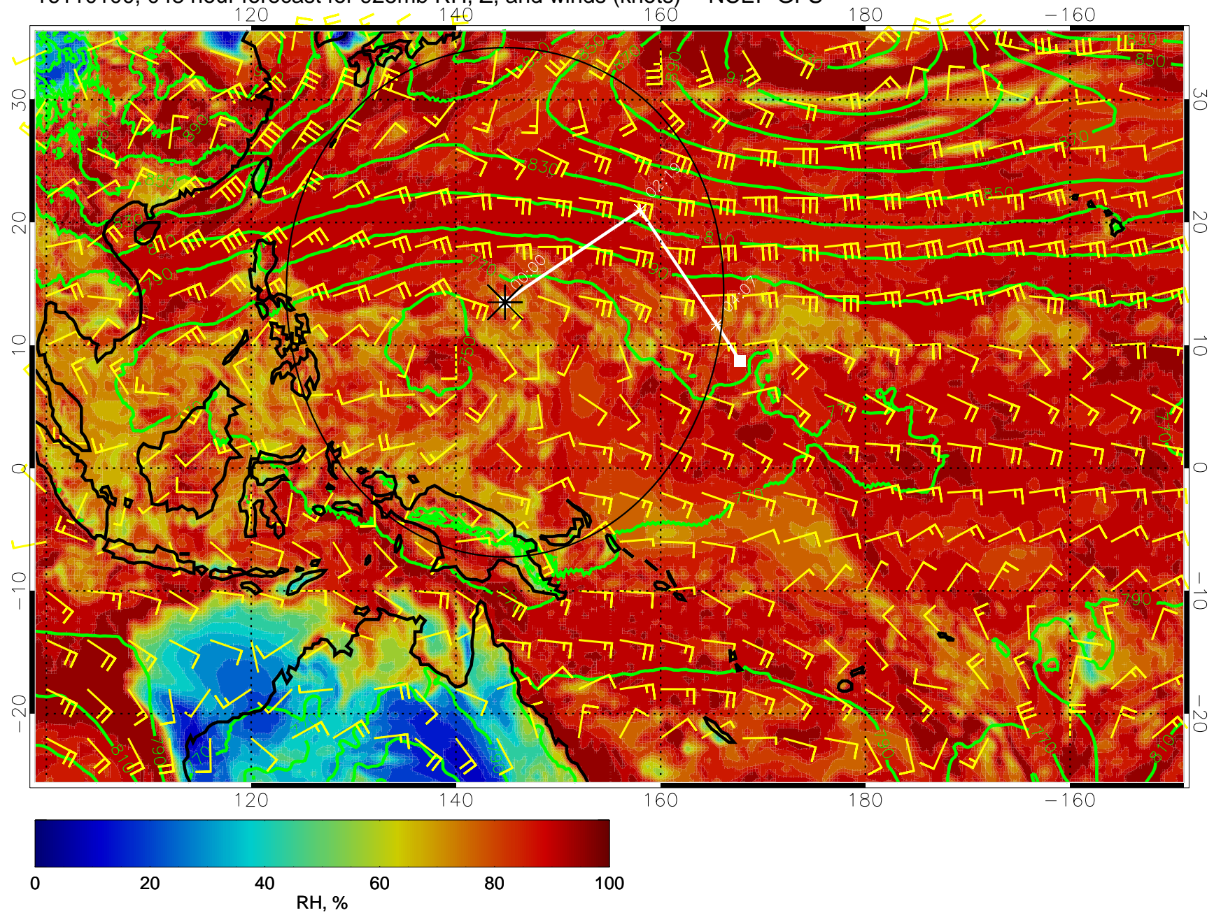
16110100, 048 hour forecast for 925mb RH, Z, and winds (knots) -- NCEP GFS
