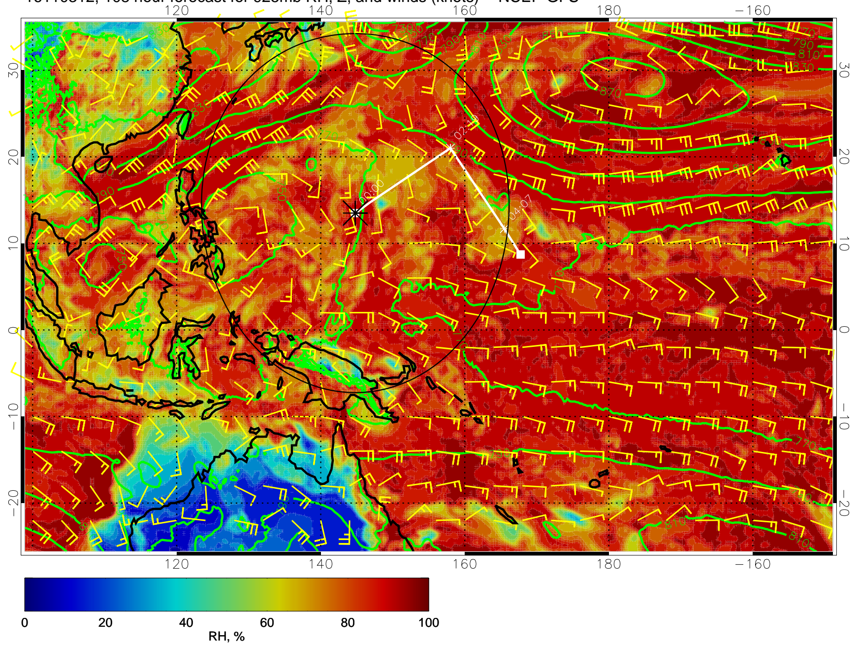
16110312, 108 hour forecast for 925mb RH, Z, and winds (knots) -- NCEP GFS
