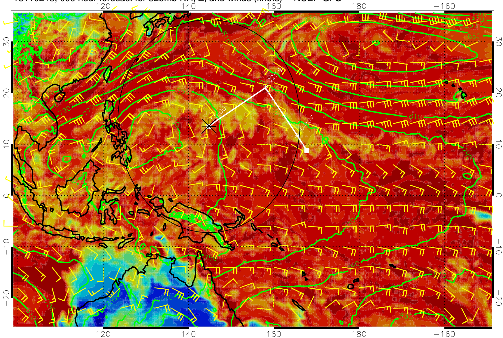
16110218, 090 hour forecast for 925mb RH, Z, and winds (knots) -- NCEP GFS
