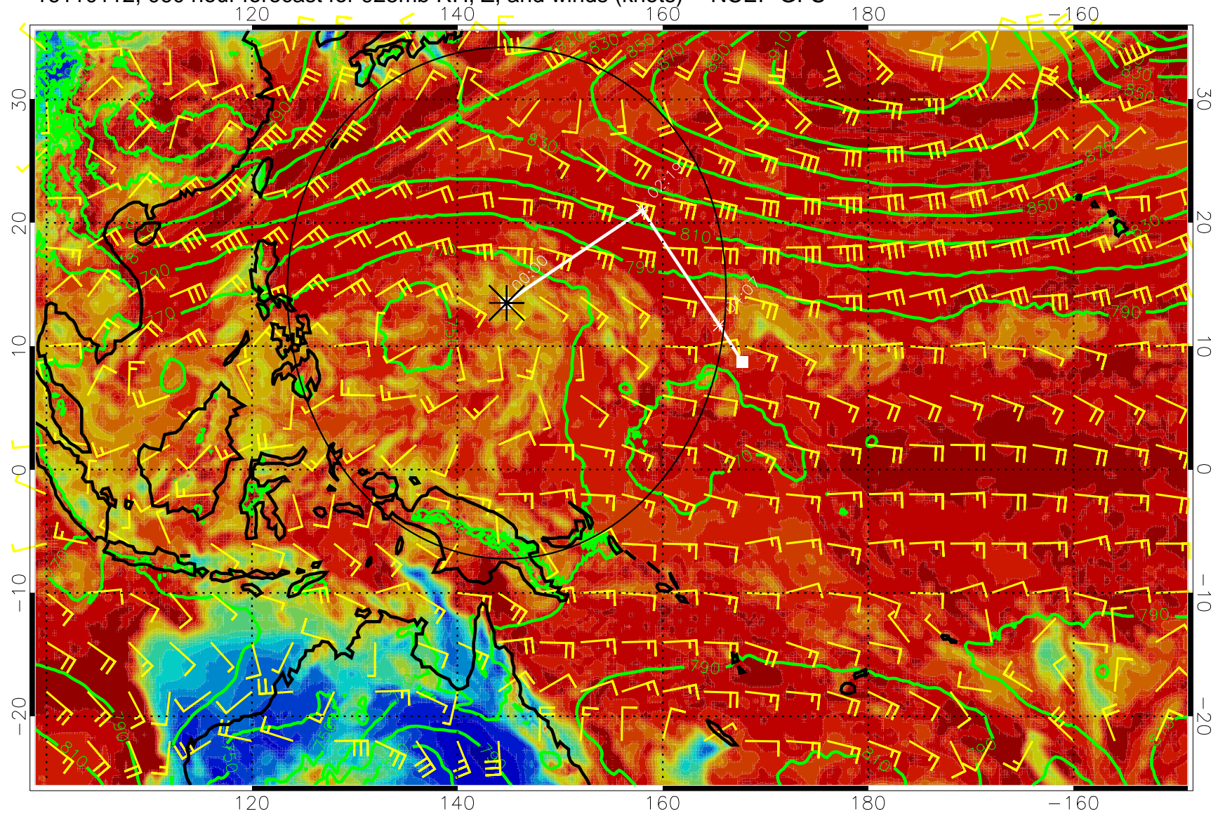
16110112, 060 hour forecast for 925mb RH, Z, and winds (knots) -- NCEP GFS
