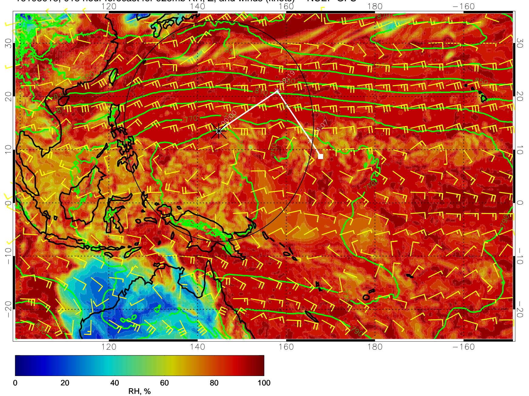
16103018, 018 hour forecast for 925mb RH, Z, and winds (knots) -- NCEP GFS
