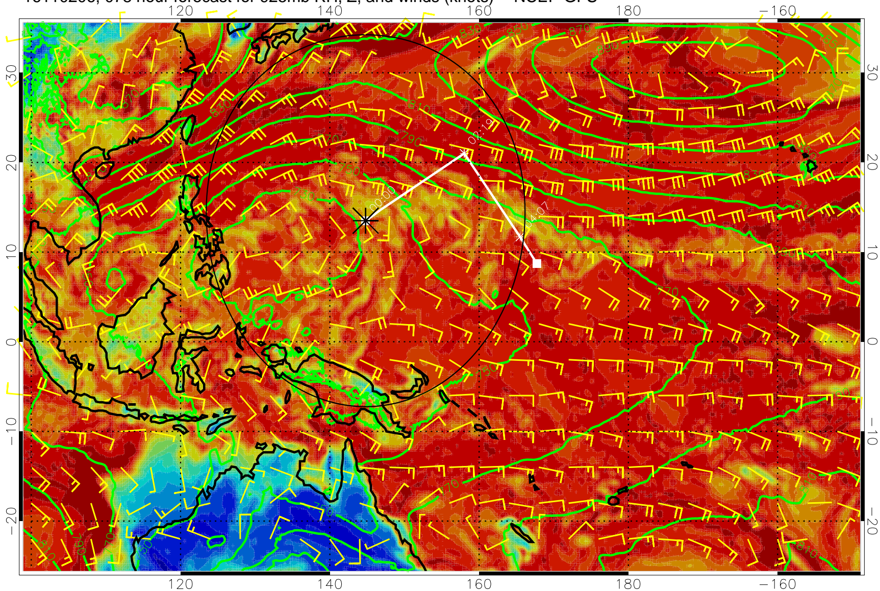
16110206, 078 hour forecast for 925mb RH, Z, and winds (knots) -- NCEP GFS
