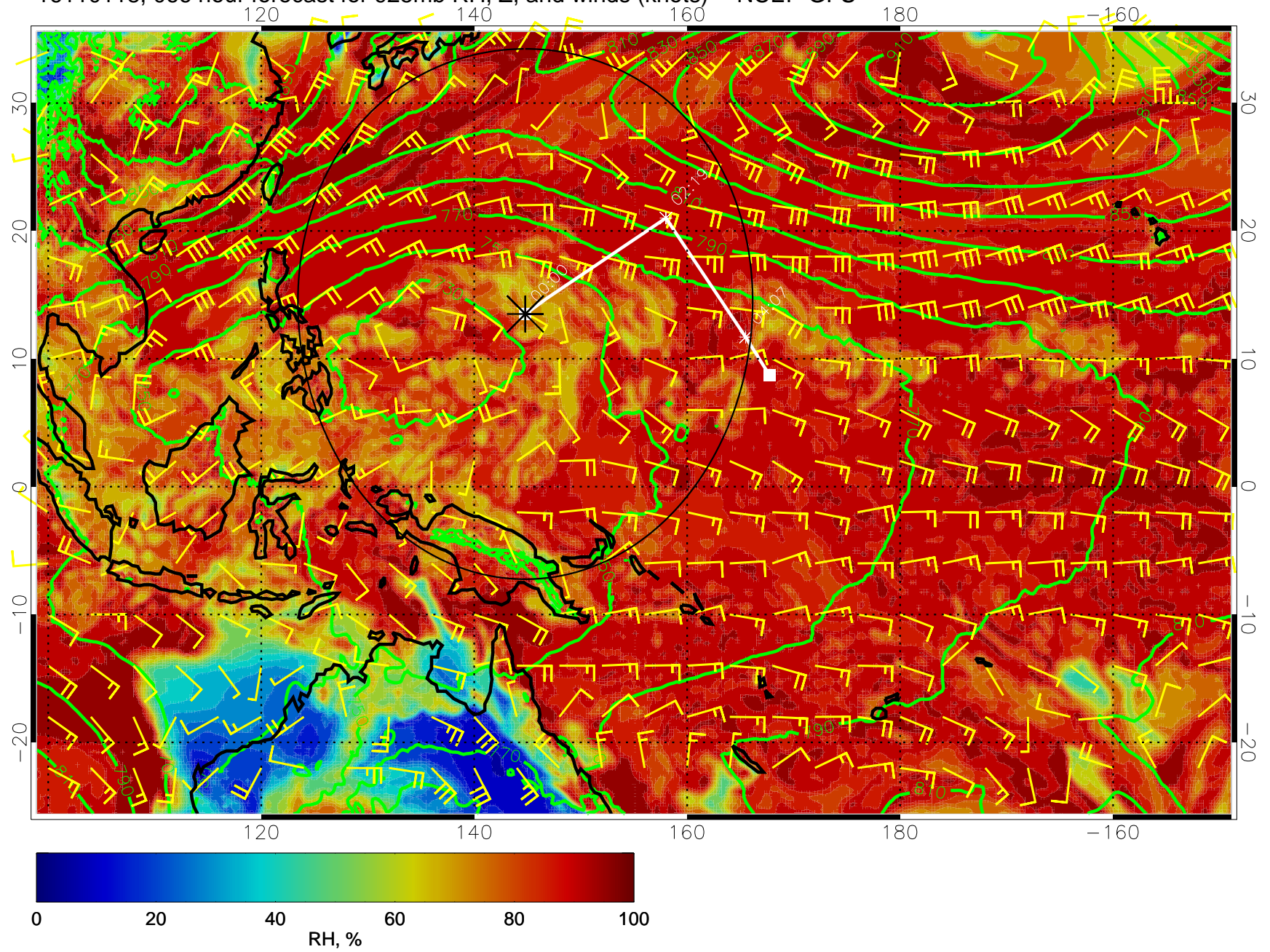
16110118, 066 hour forecast for 925mb RH, Z, and winds (knots) -- NCEP GFS
