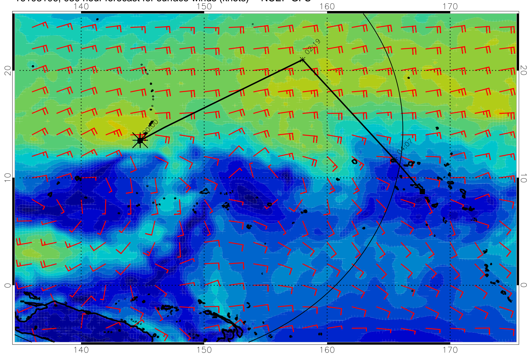
16103106, 030 hour forecast for surface winds (knots) -- NCEP GFS
