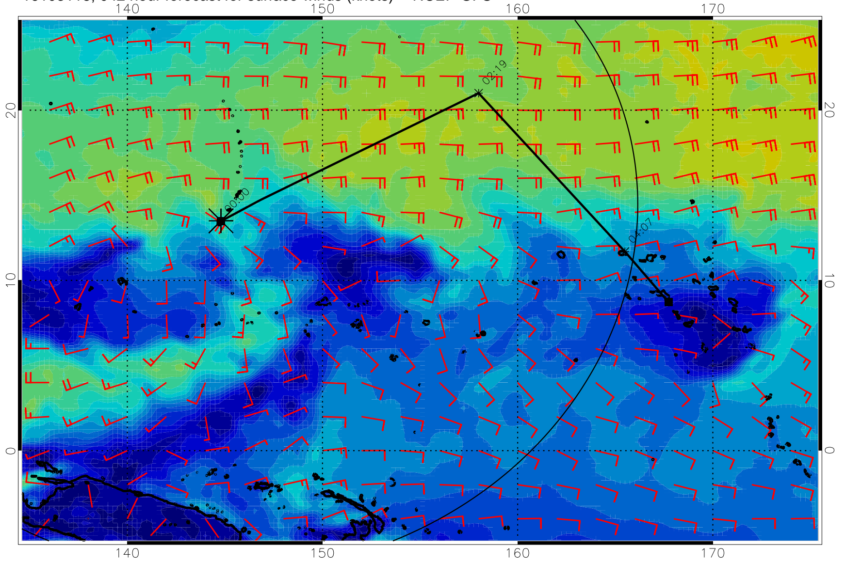
16103118, 042 hour forecast for surface winds (knots) -- NCEP GFS
