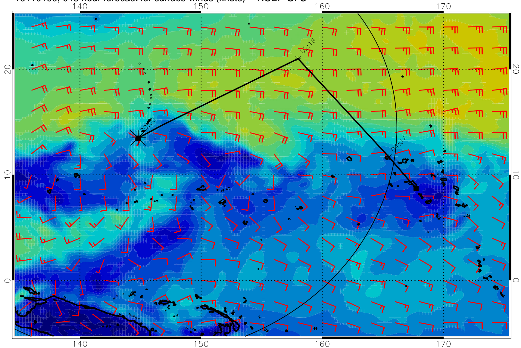
16110100, 048 hour forecast for surface winds (knots) -- NCEP GFS
