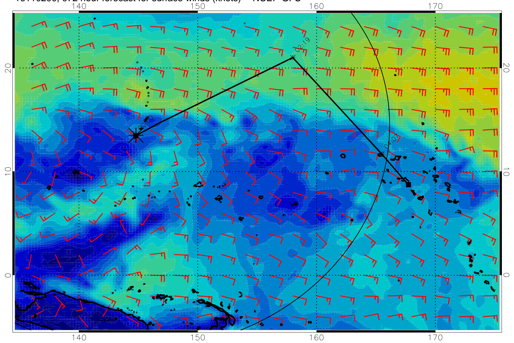
16110200, 072 hour forecast for surface winds (knots) -- NCEP GFS
