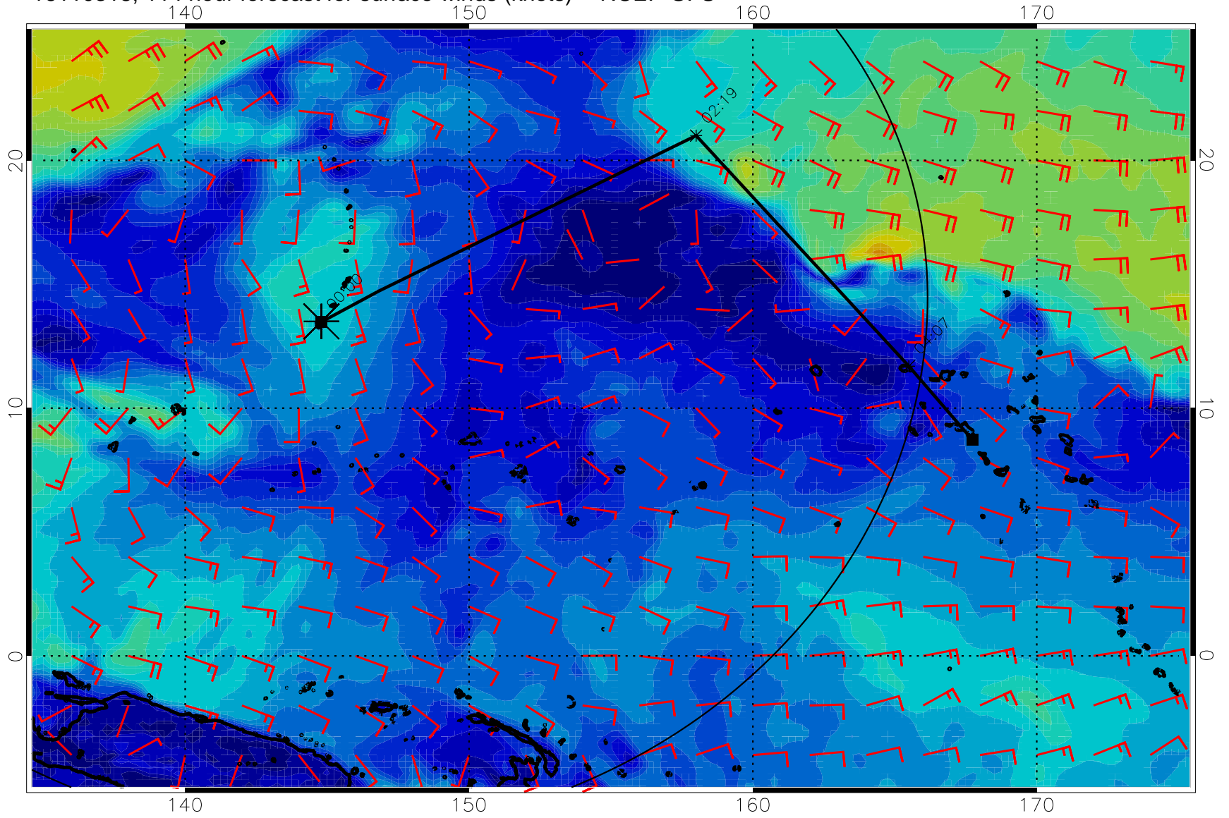
16110318, 114 hour forecast for surface winds (knots) -- NCEP GFS
