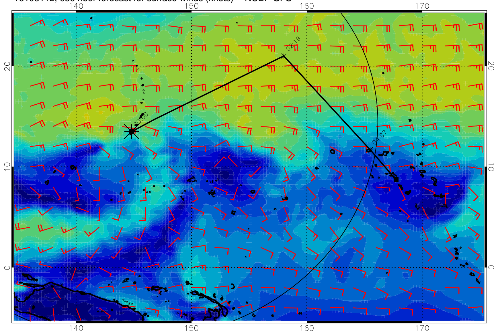
16103112, 036 hour forecast for surface winds (knots) -- NCEP GFS
