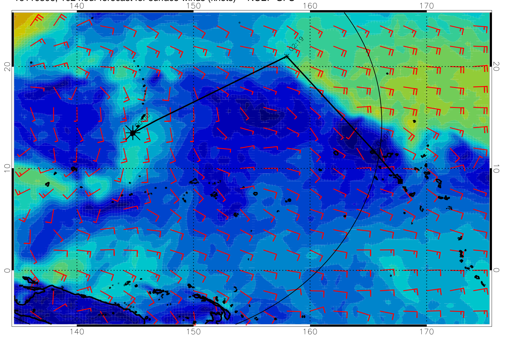
16110306, 102 hour forecast for surface winds (knots) -- NCEP GFS
