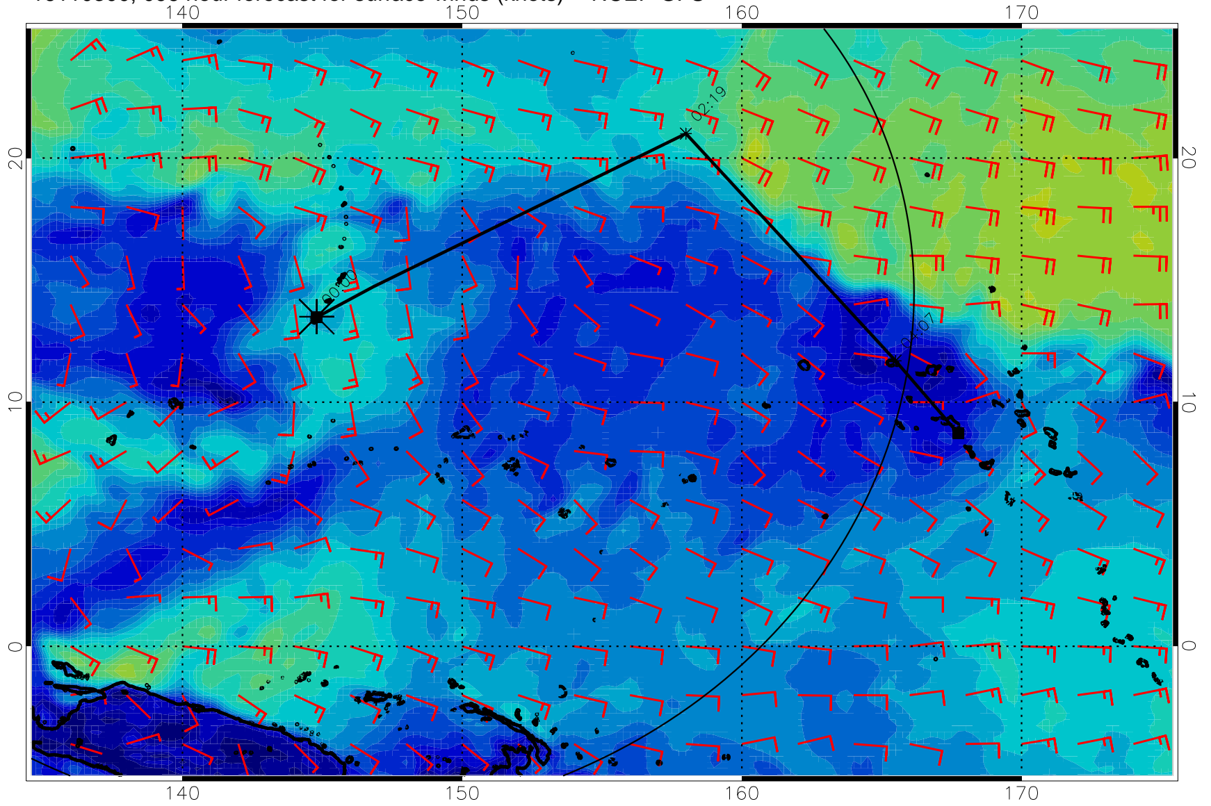
16110300, 096 hour forecast for surface winds (knots) -- NCEP GFS
