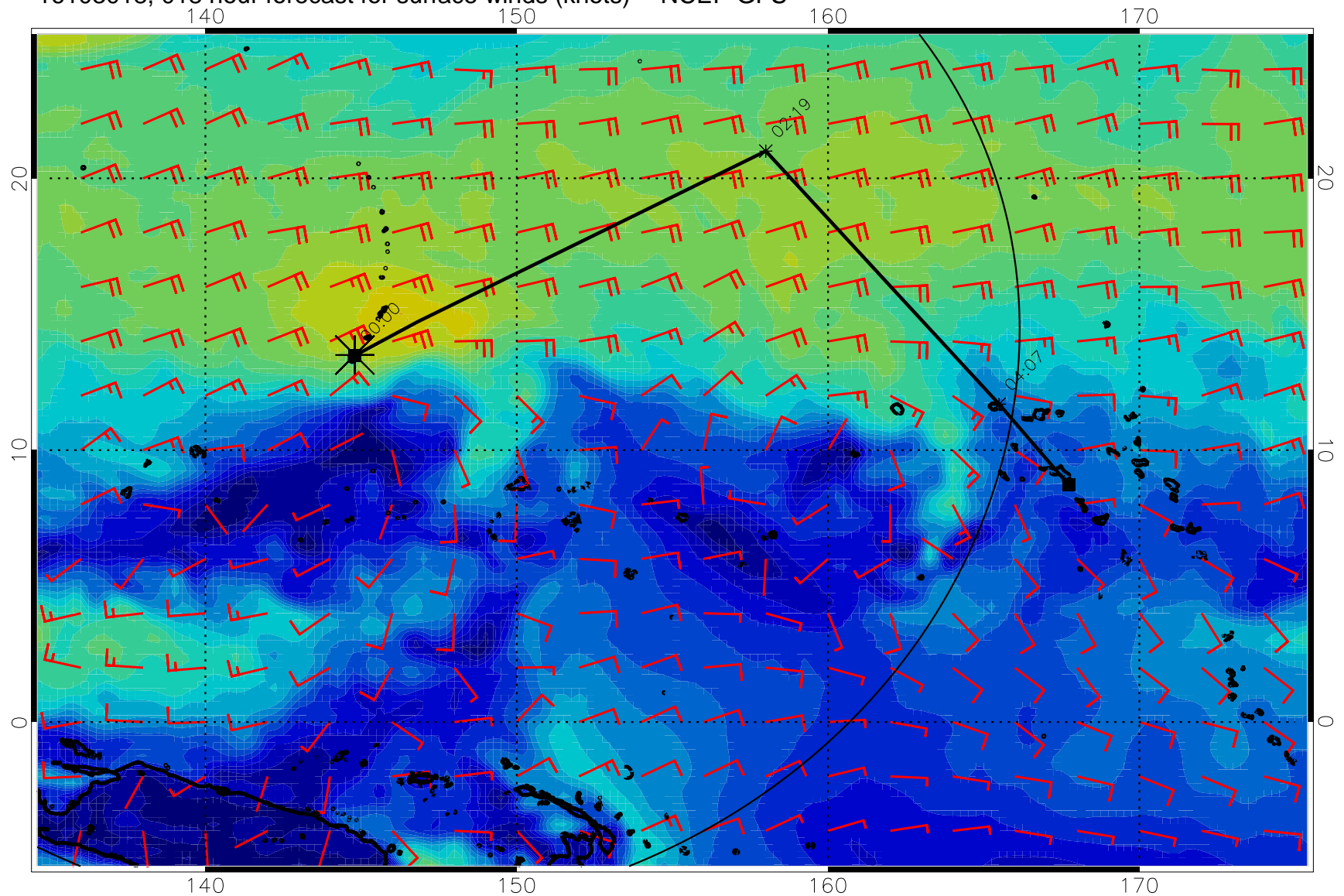
16103018, 018 hour forecast for surface winds (knots) -- NCEP GFS
