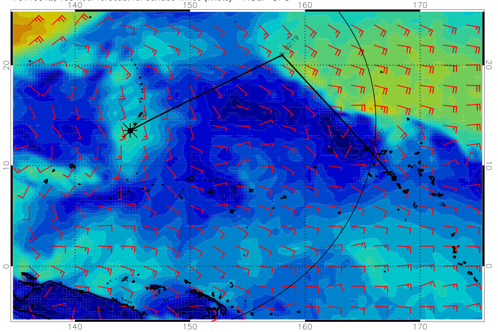
16110312, 108 hour forecast for surface winds (knots) -- NCEP GFS
