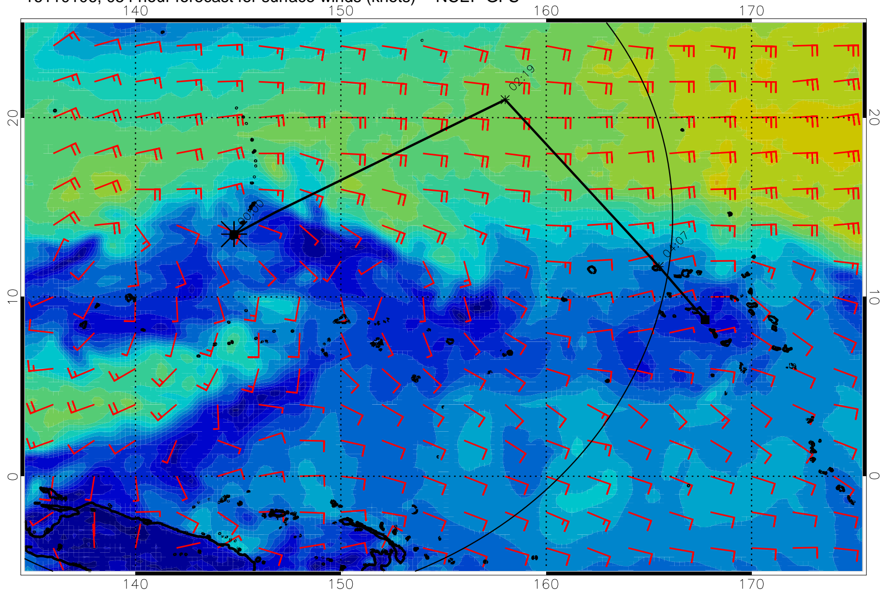
16110106, 054 hour forecast for surface winds (knots) -- NCEP GFS
