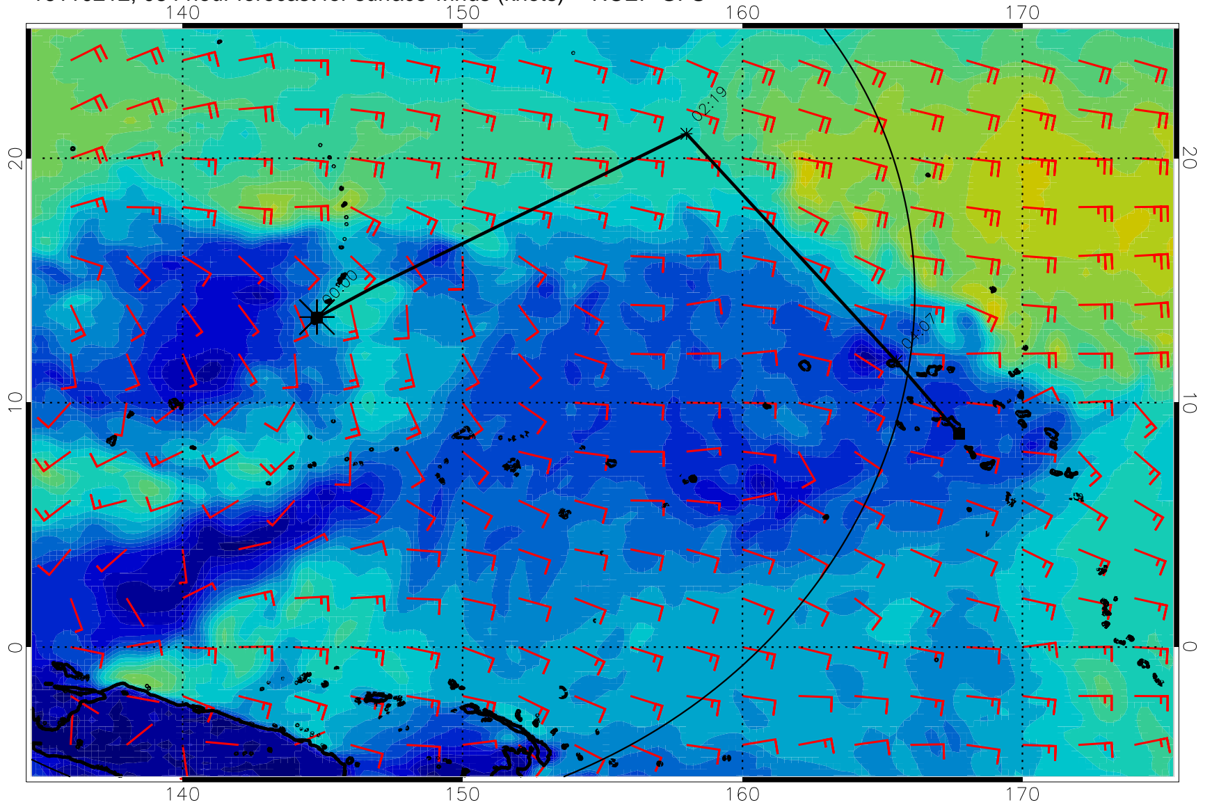
16110212, 084 hour forecast for surface winds (knots) -- NCEP GFS
