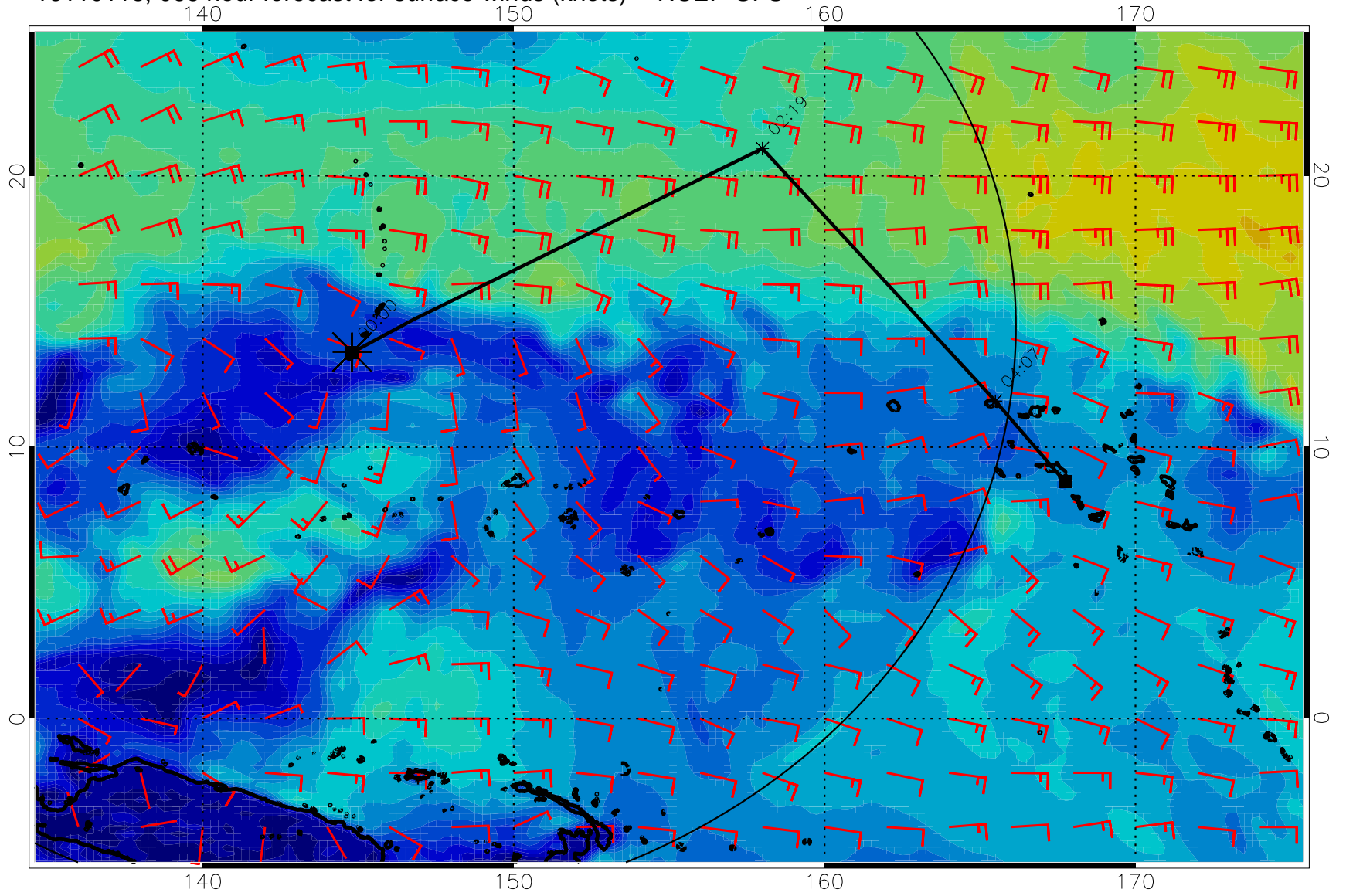
16110118, 066 hour forecast for surface winds (knots) -- NCEP GFS
