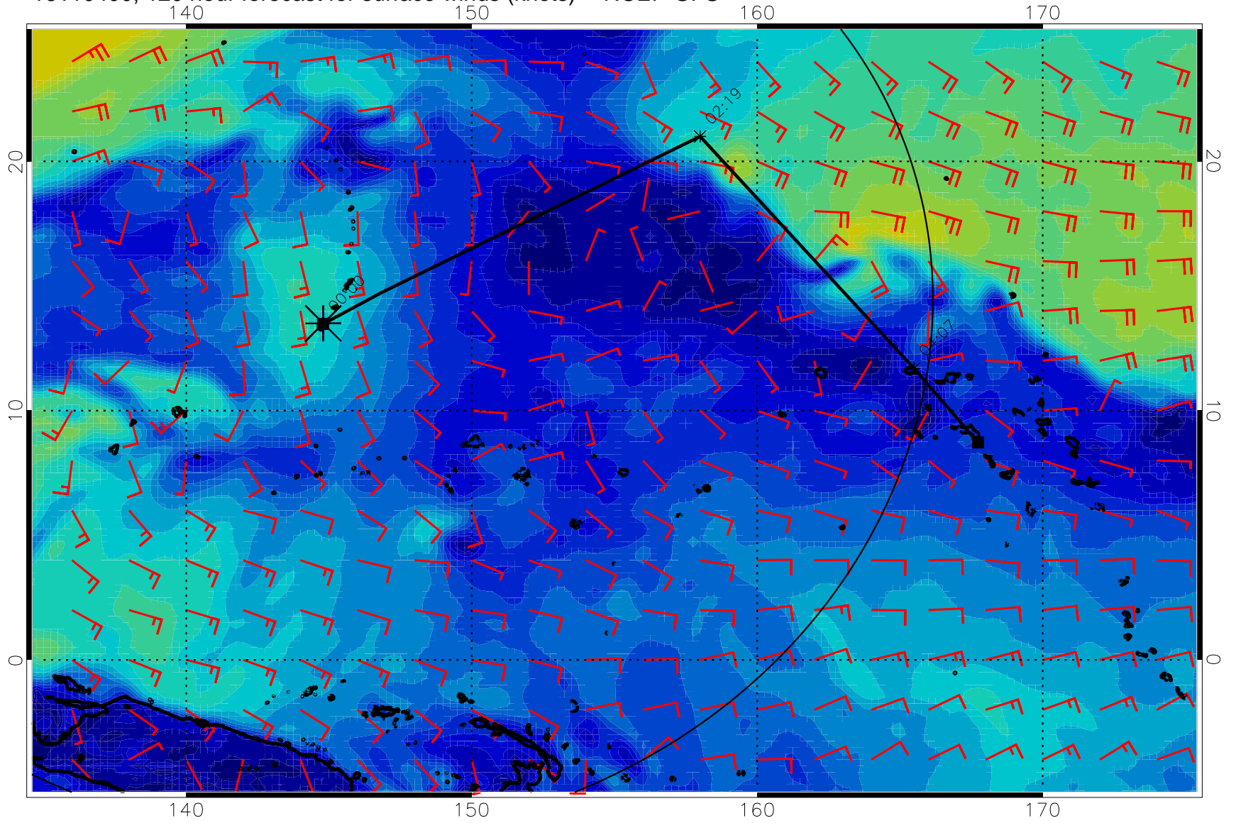
16110400, 120 hour forecast for surface winds (knots) -- NCEP GFS
