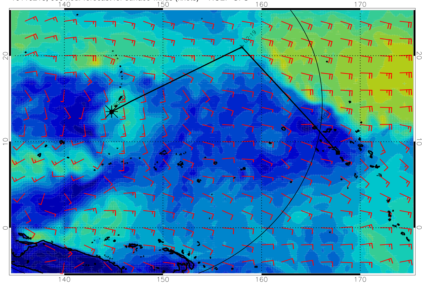
16110218, 090 hour forecast for surface winds (knots) -- NCEP GFS
