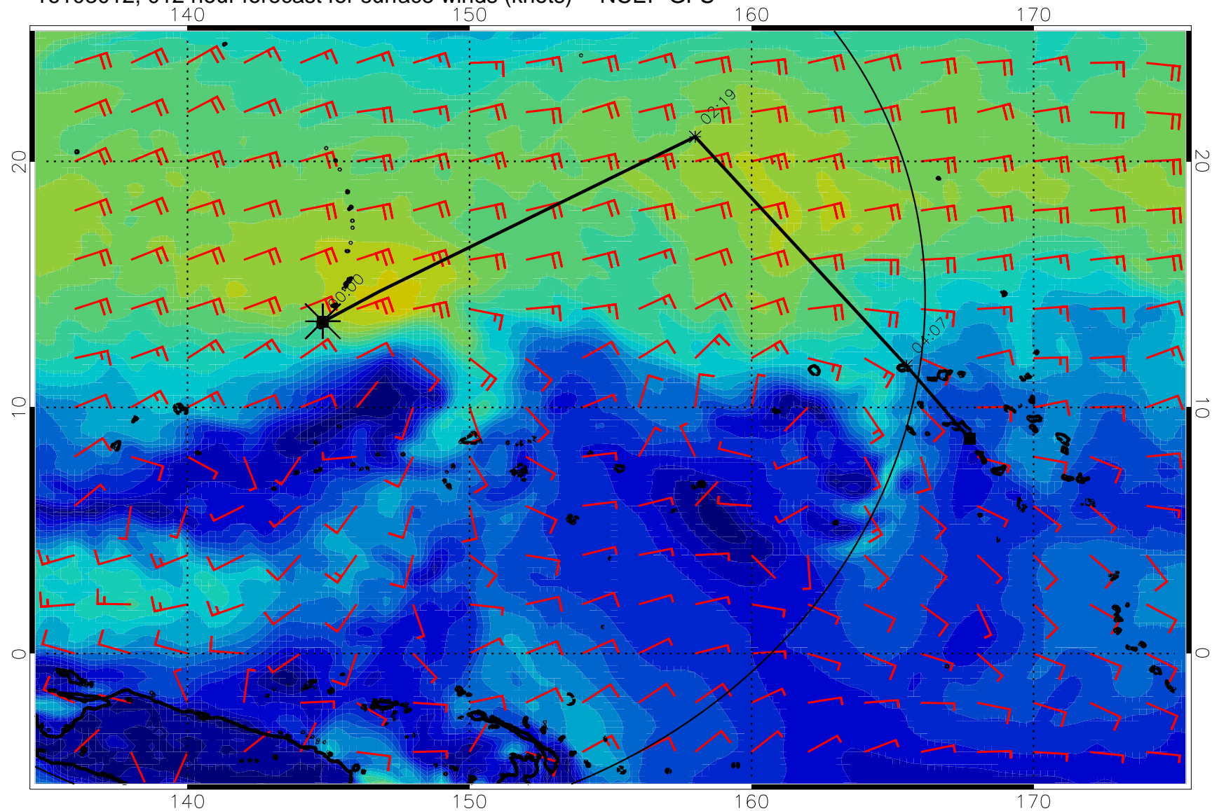
16103012, 012 hour forecast for surface winds (knots) -- NCEP GFS
