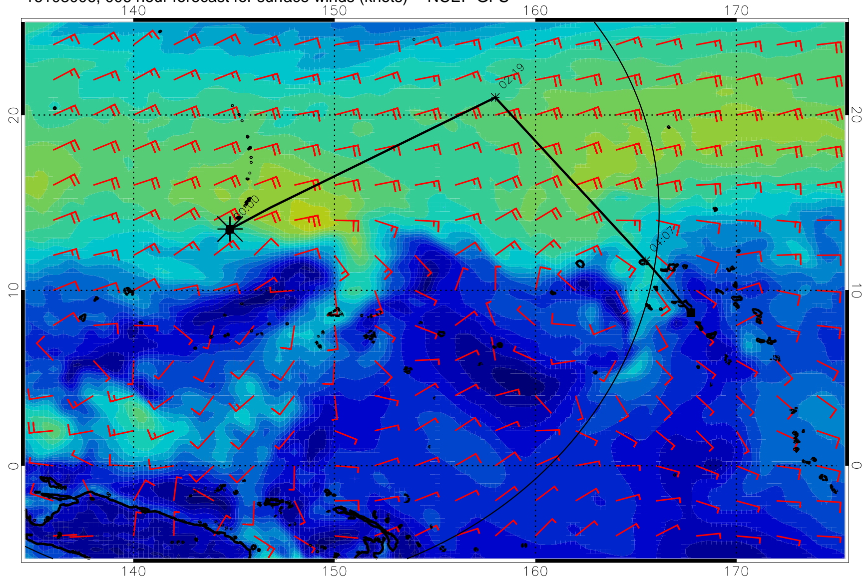
16103006, 006 hour forecast for surface winds (knots) -- NCEP GFS
