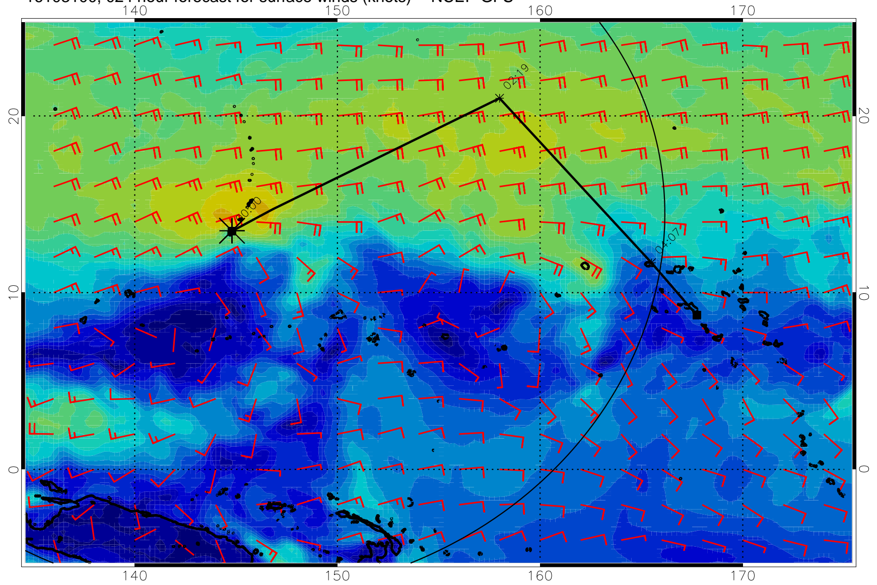
16103100, 024 hour forecast for surface winds (knots) -- NCEP GFS
