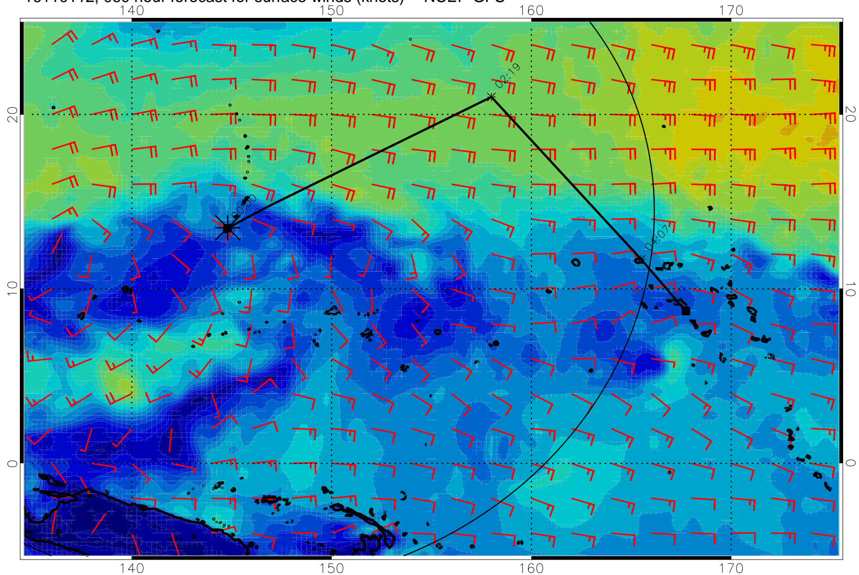
16110112, 060 hour forecast for surface winds (knots) -- NCEP GFS
