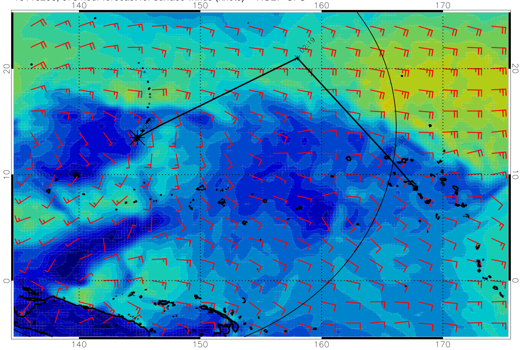
16110206, 078 hour forecast for surface winds (knots) -- NCEP GFS
