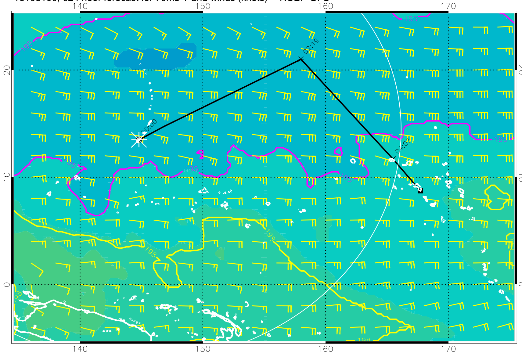
16103100, 024 hour forecast for 70mb T and winds (knots) -- NCEP GFS
