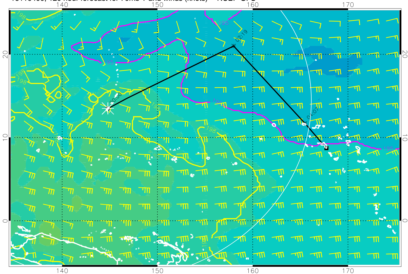
16110400, 120 hour forecast for 70mb T and winds (knots) -- NCEP GFS
