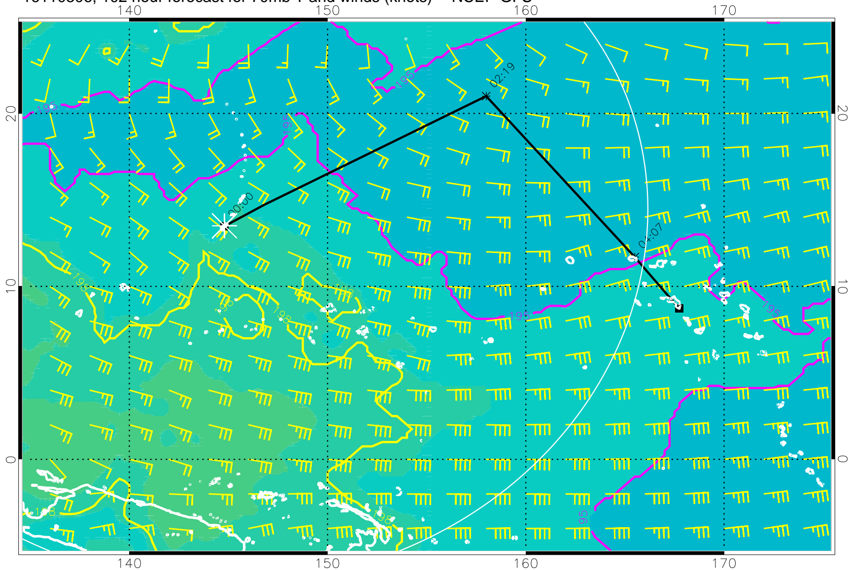
16110306, 102 hour forecast for 70mb T and winds (knots) -- NCEP GFS
