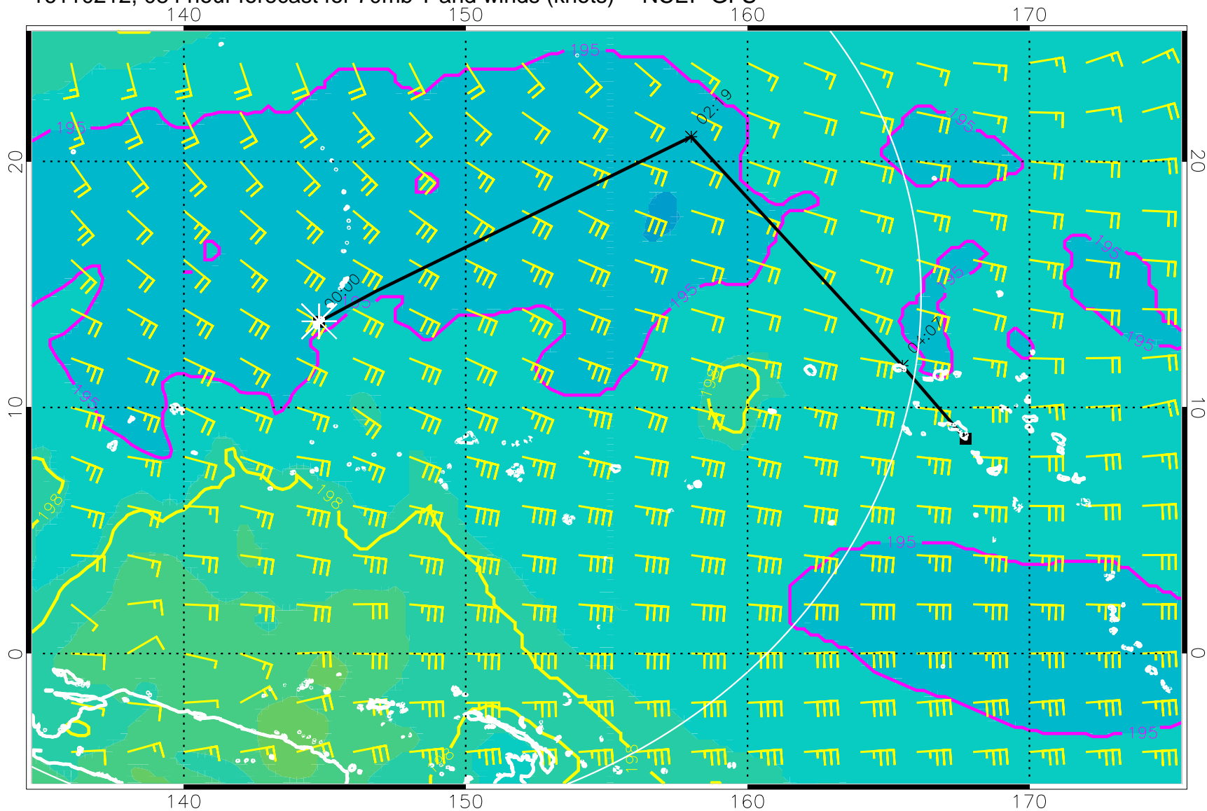
16110212, 084 hour forecast for 70mb T and winds (knots) -- NCEP GFS
