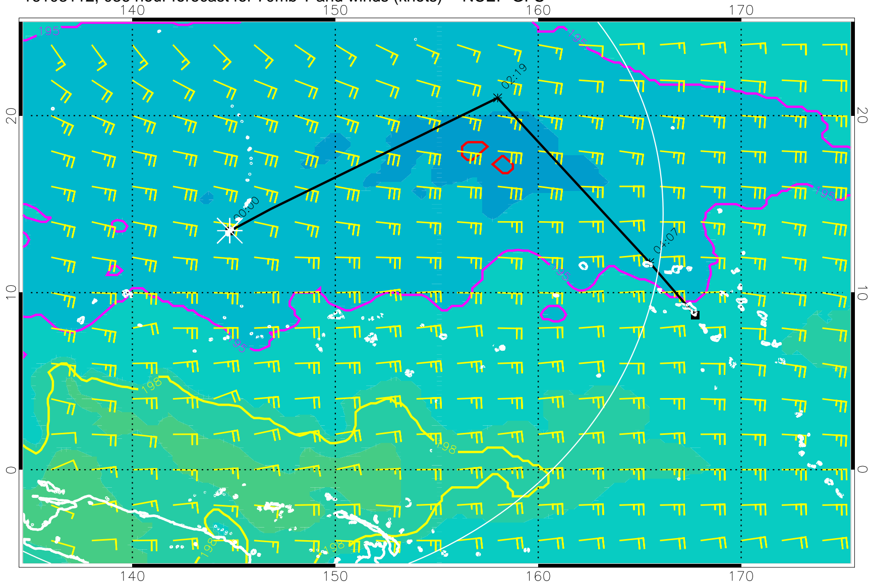
16103112, 036 hour forecast for 70mb T and winds (knots) -- NCEP GFS
