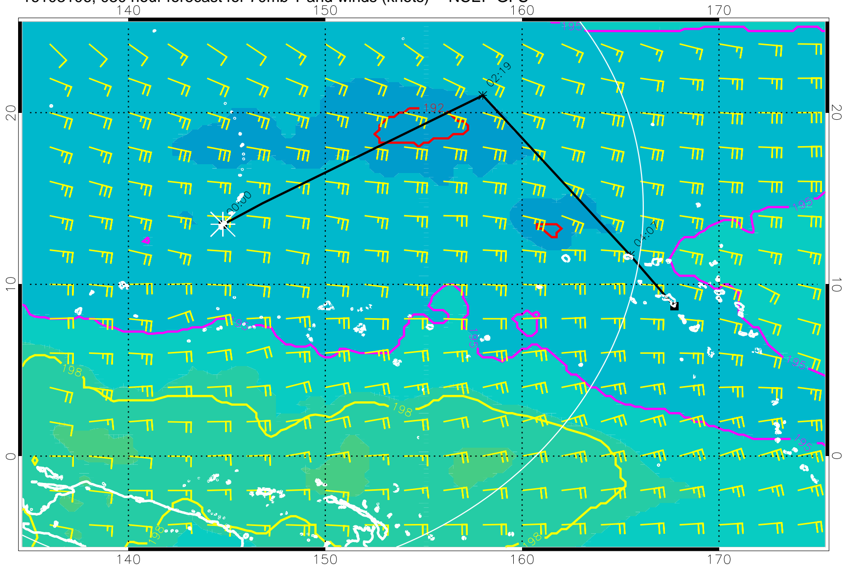
16103106, 030 hour forecast for 70mb T and winds (knots) -- NCEP GFS
