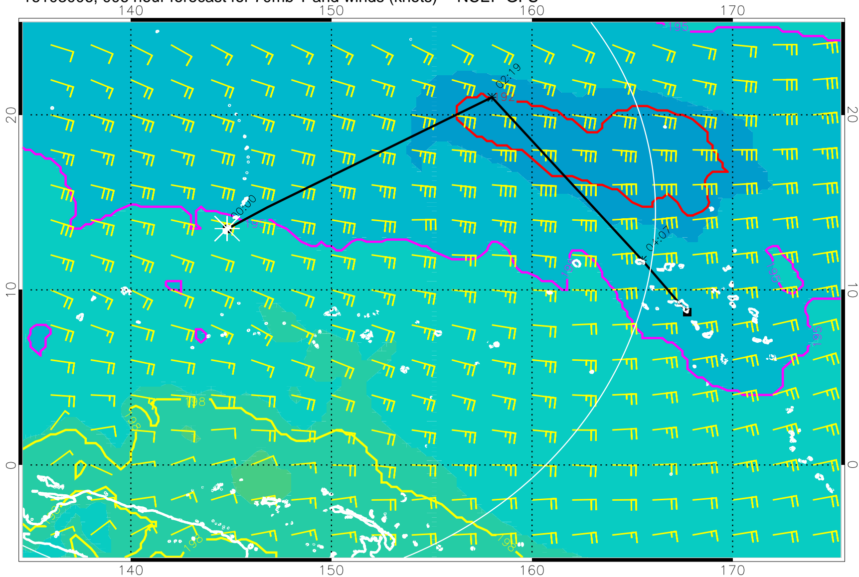
16103006, 006 hour forecast for 70mb T and winds (knots) -- NCEP GFS
