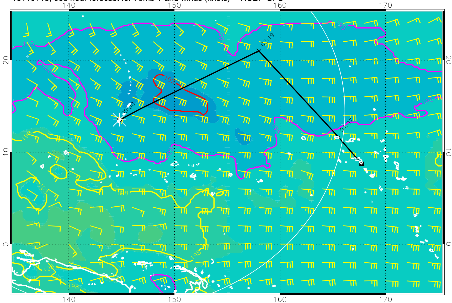
16110118, 066 hour forecast for 70mb T and winds (knots) -- NCEP GFS
