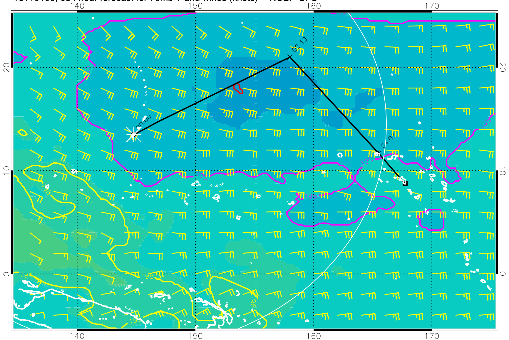
16110106, 054 hour forecast for 70mb T and winds (knots) -- NCEP GFS
