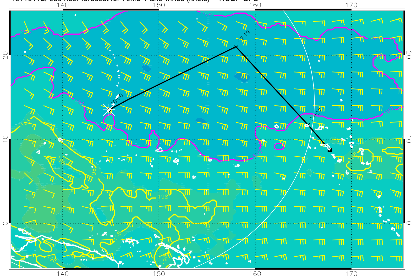
16110112, 060 hour forecast for 70mb T and winds (knots) -- NCEP GFS
