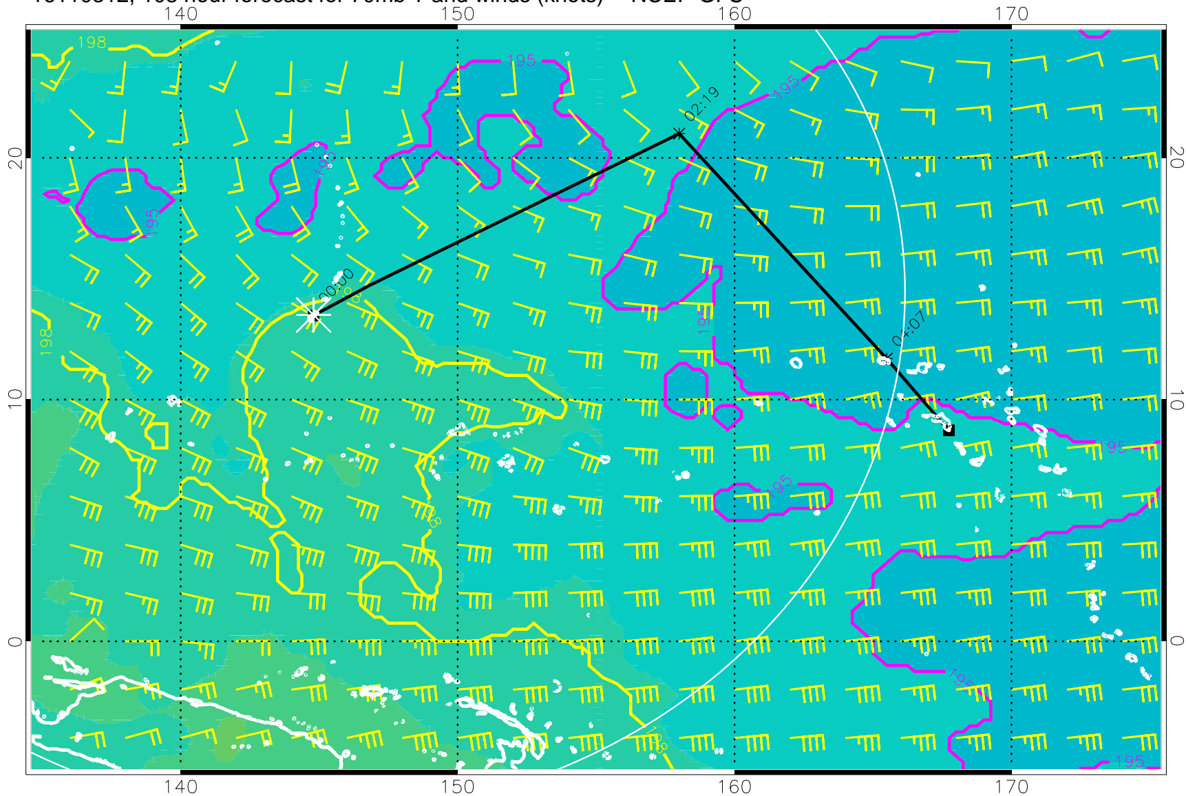
16110312, 108 hour forecast for 70mb T and winds (knots) -- NCEP GFS
