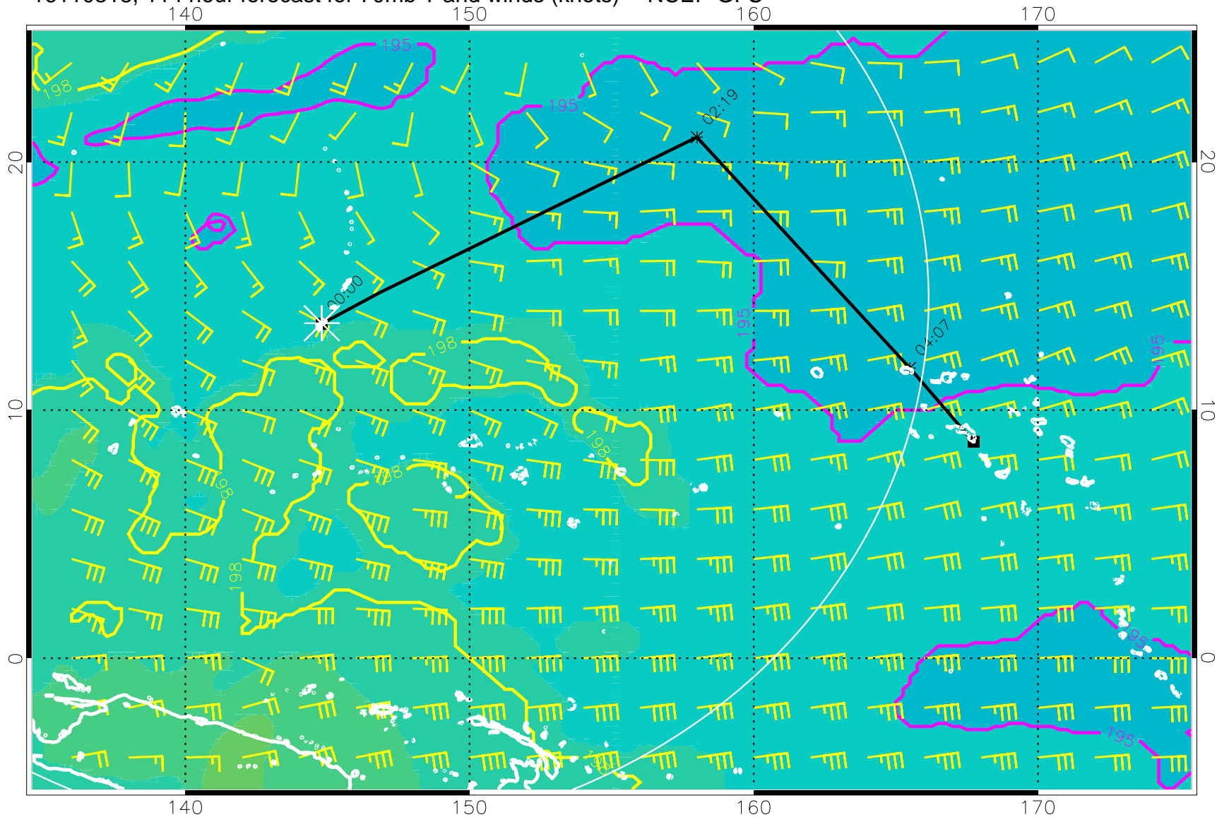
16110318, 114 hour forecast for 70mb T and winds (knots) -- NCEP GFS
