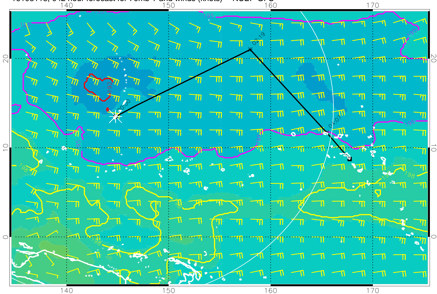
16103118, 042 hour forecast for 70mb T and winds (knots) -- NCEP GFS
