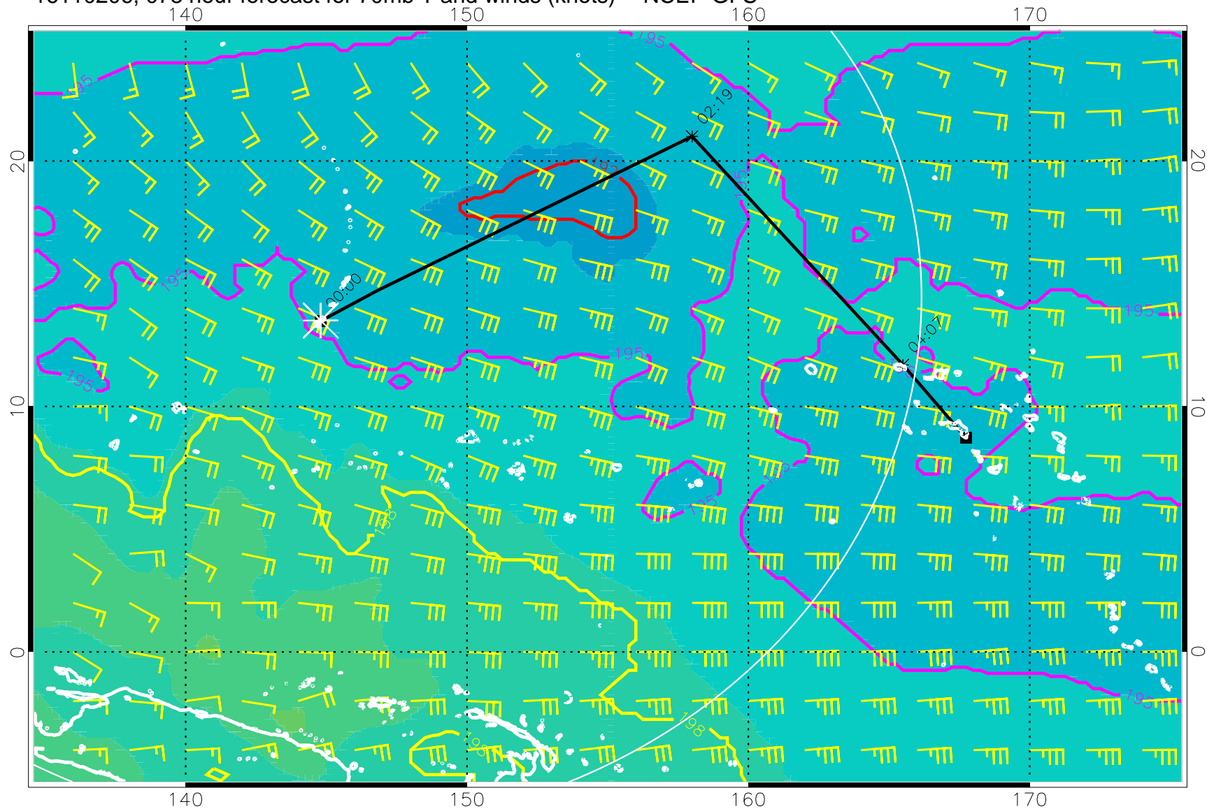
16110206, 078 hour forecast for 70mb T and winds (knots) -- NCEP GFS
