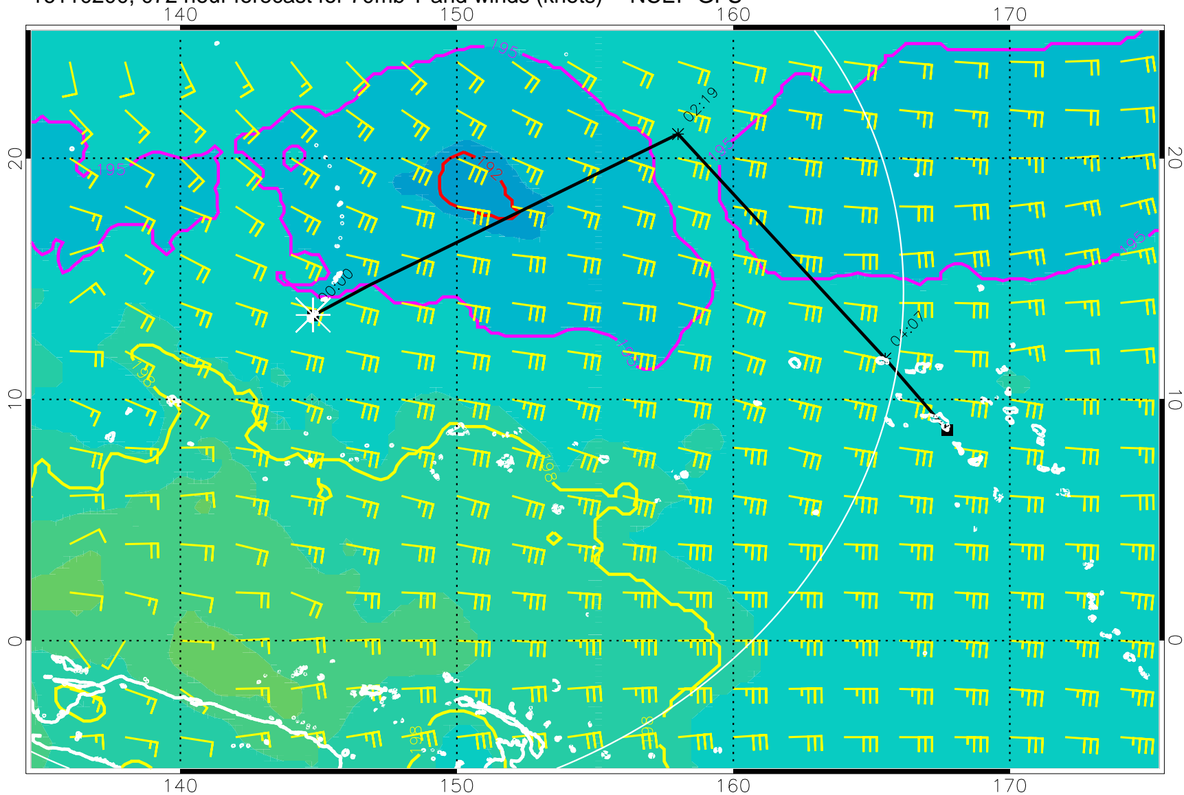
16110200, 072 hour forecast for 70mb T and winds (knots) -- NCEP GFS
