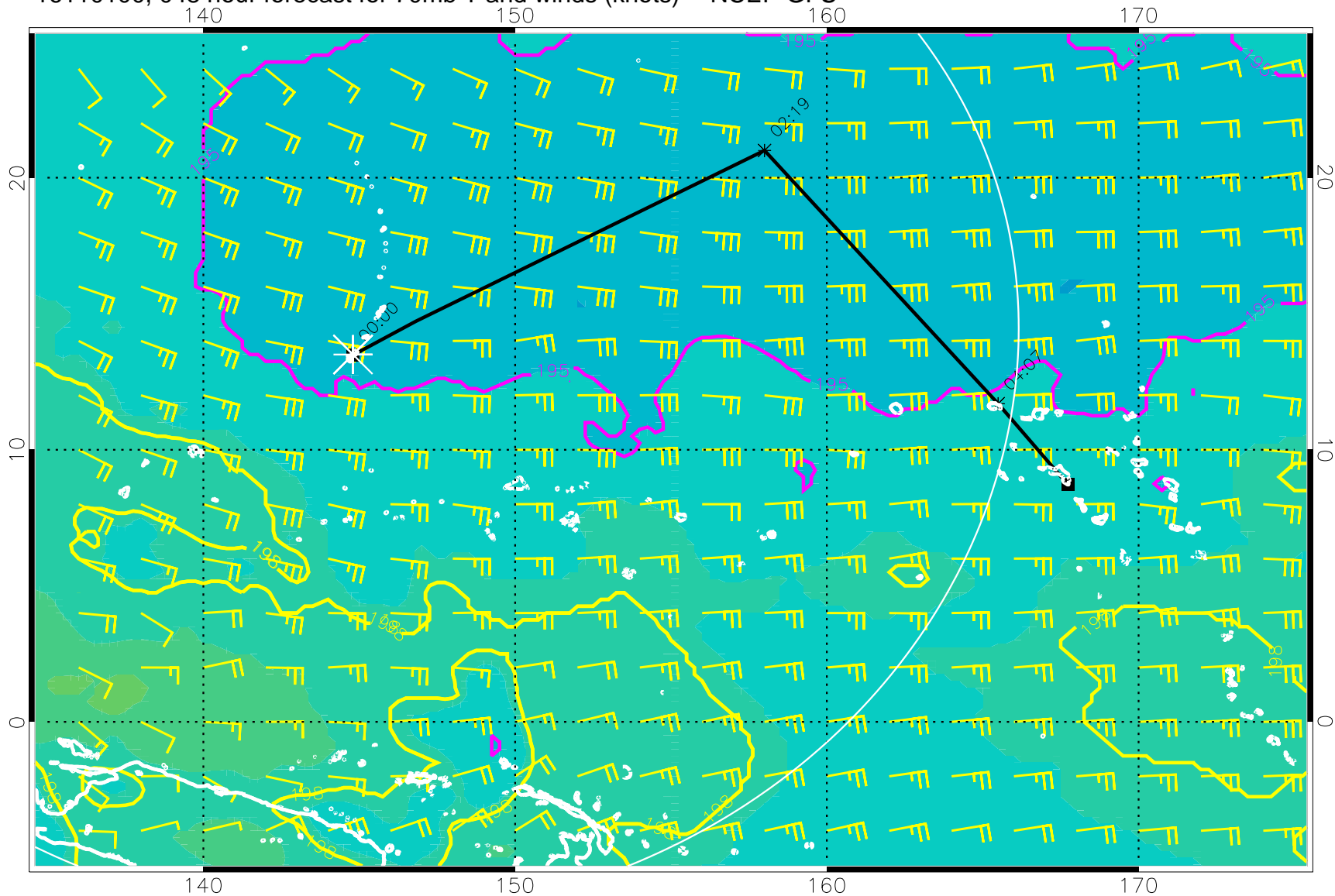
16110100, 048 hour forecast for 70mb T and winds (knots) -- NCEP GFS
