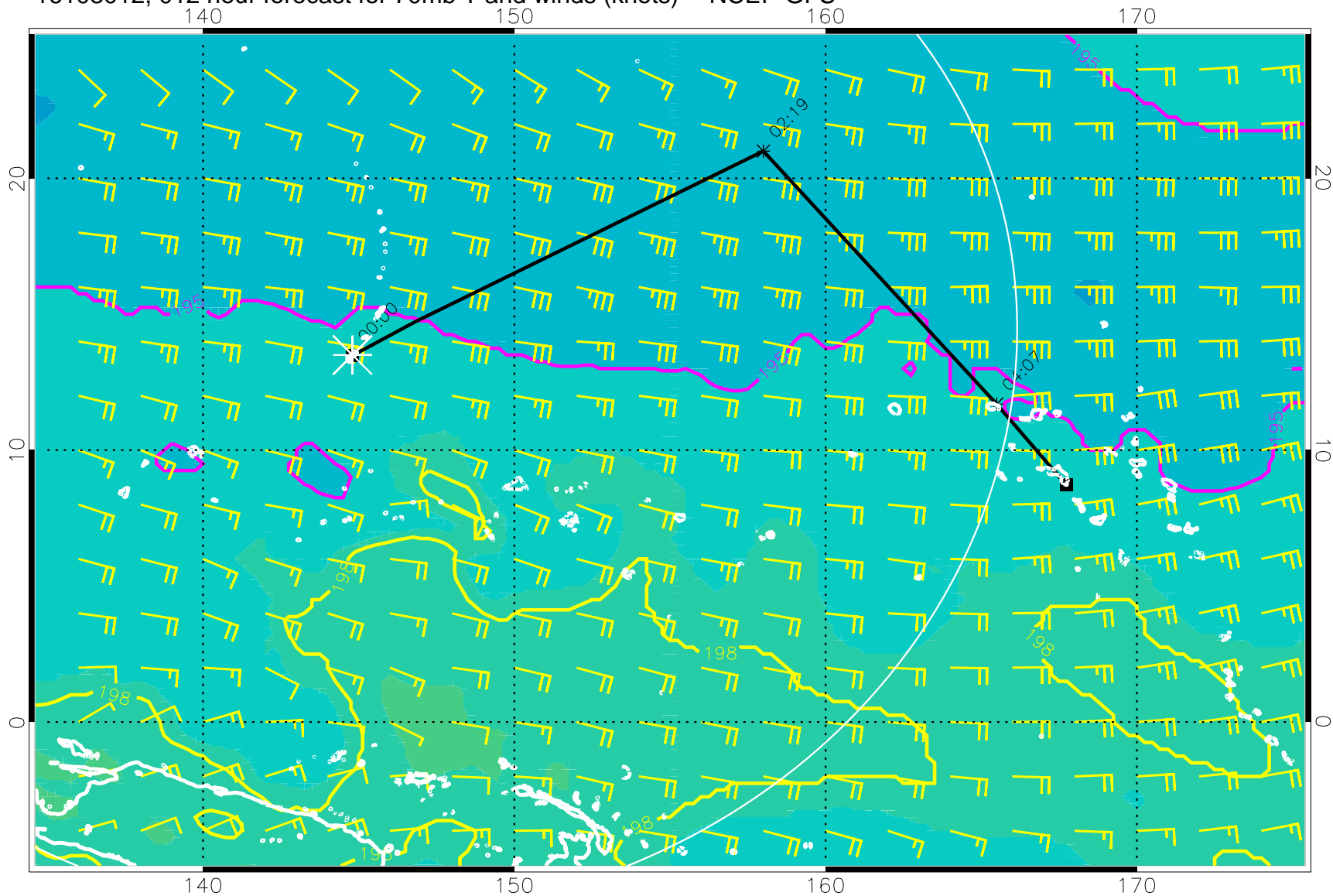
16103012, 012 hour forecast for 70mb T and winds (knots) -- NCEP GFS
