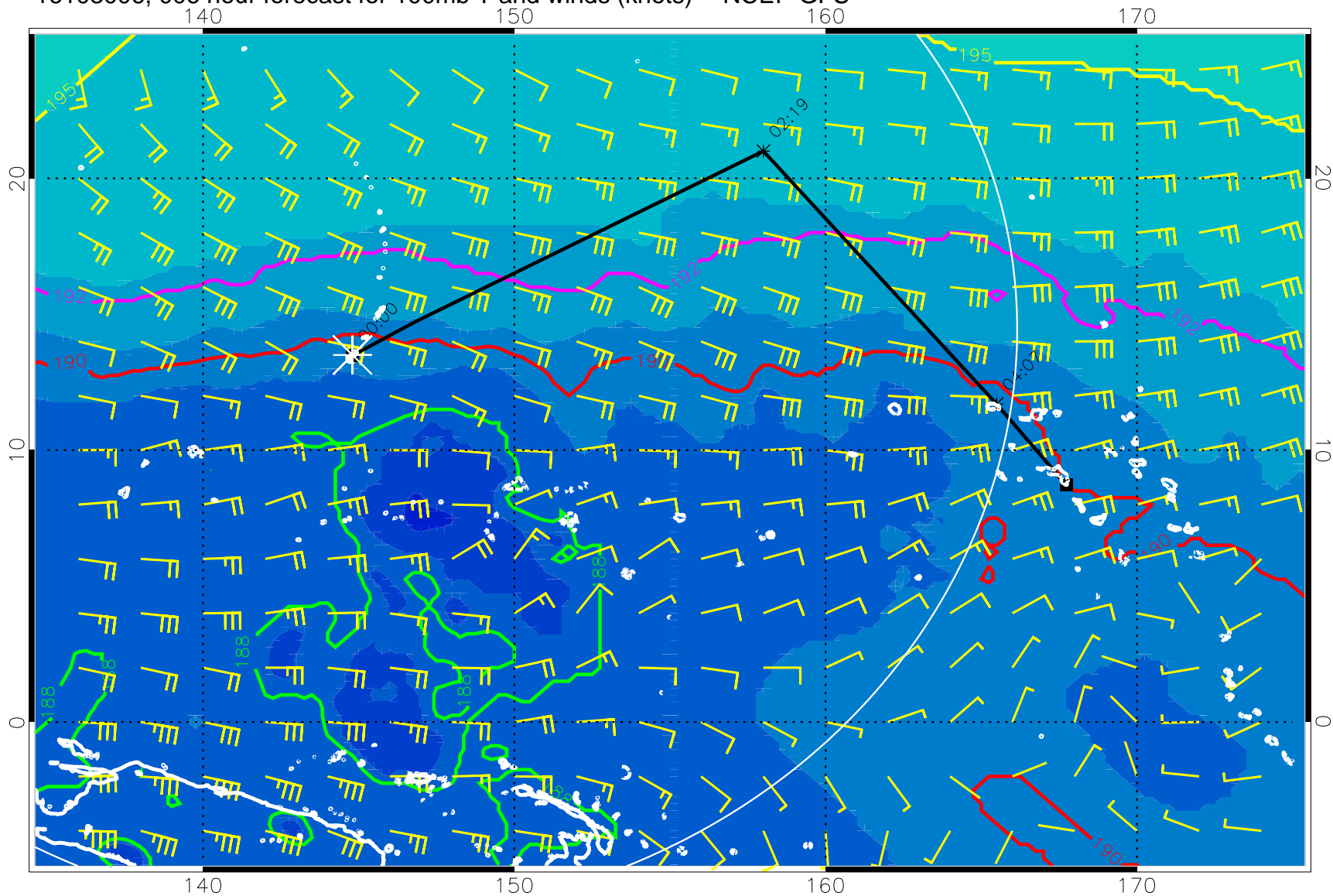
16103006, 006 hour forecast for 100mb T and winds (knots) -- NCEP GFS
