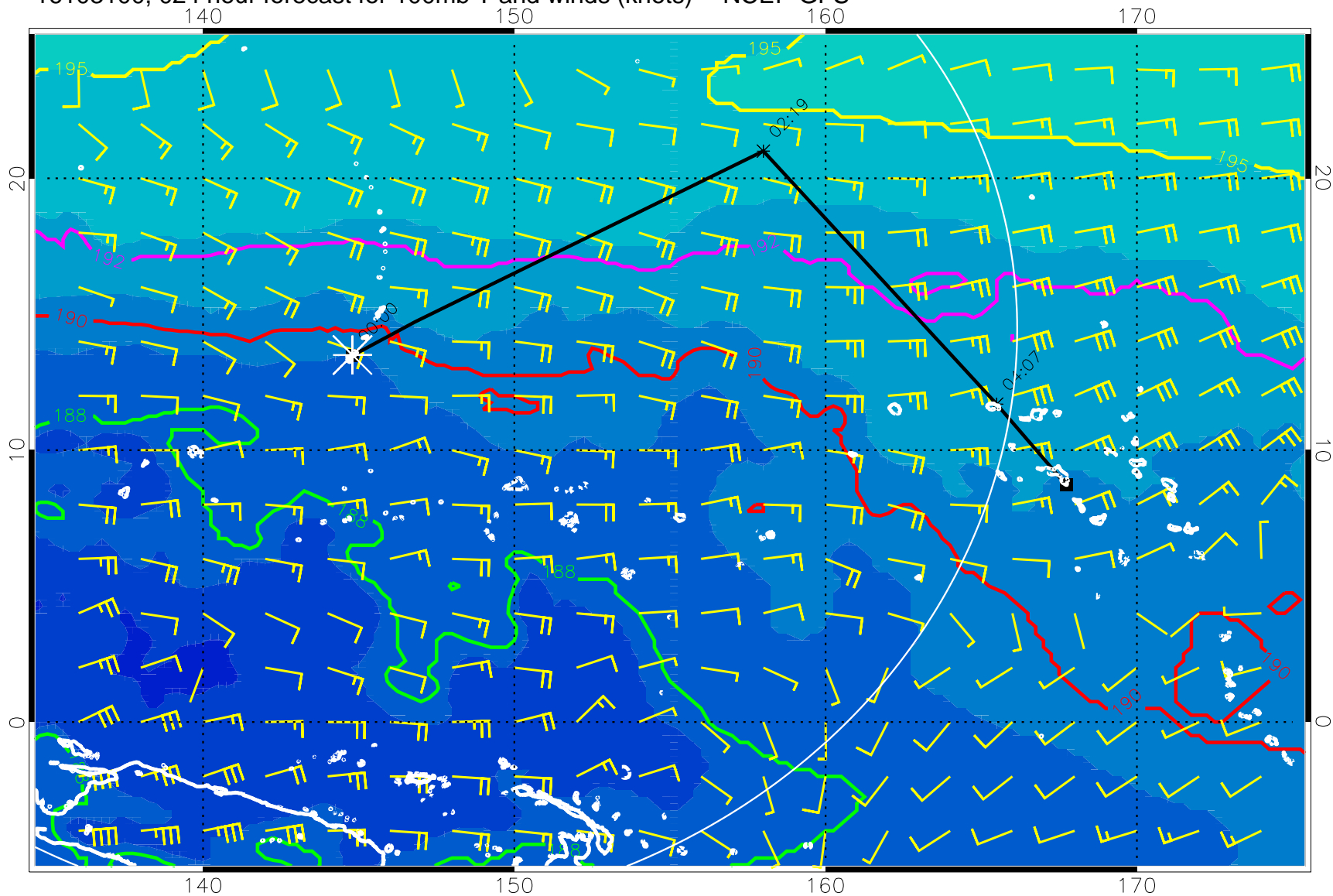
16103100, 024 hour forecast for 100mb T and winds (knots) -- NCEP GFS
