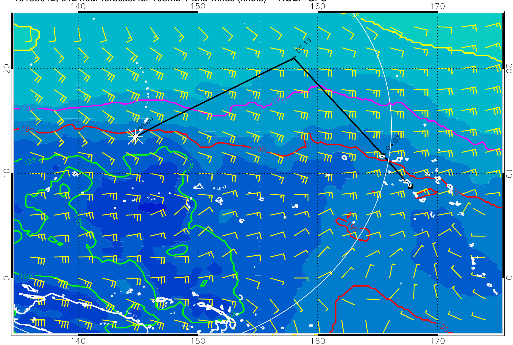
16103012, 012 hour forecast for 100mb T and winds (knots) -- NCEP GFS
