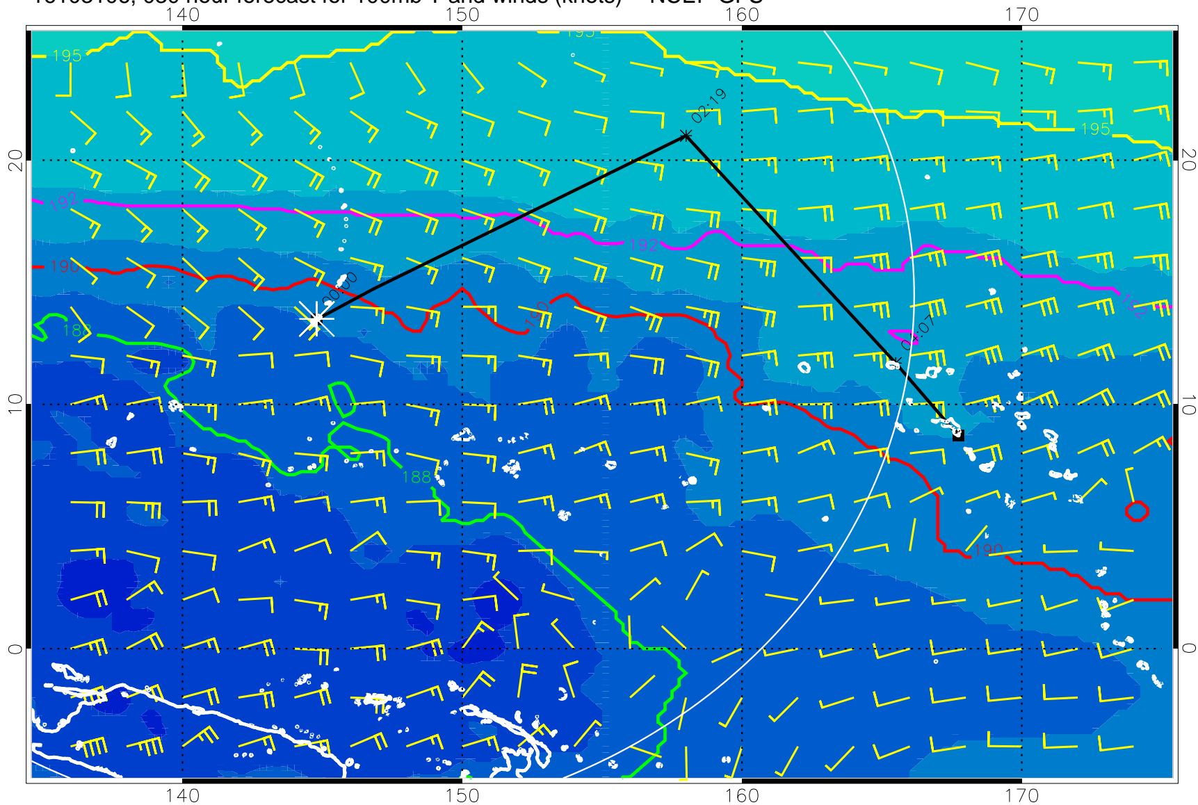
16103106, 030 hour forecast for 100mb T and winds (knots) -- NCEP GFS
