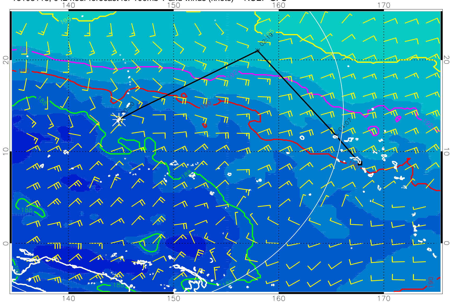
16103118, 042 hour forecast for 100mb T and winds (knots) -- NCEP GFS
