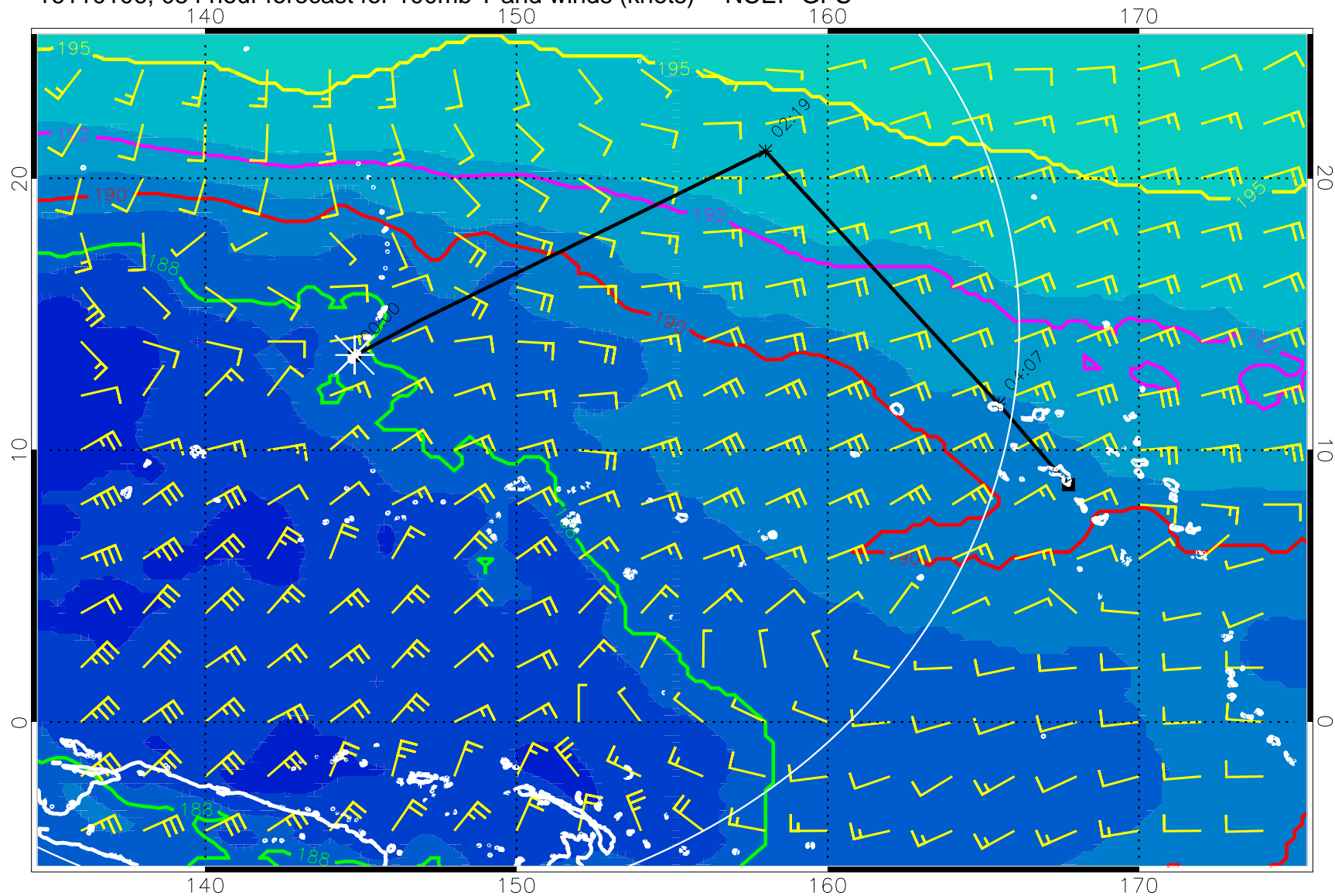
16110106, 054 hour forecast for 100mb T and winds (knots) -- NCEP GFS
