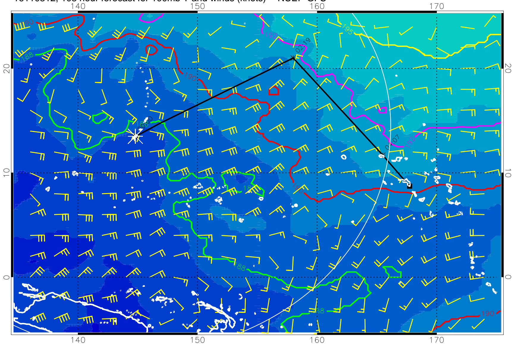
16110312, 108 hour forecast for 100mb T and winds (knots) -- NCEP GFS
