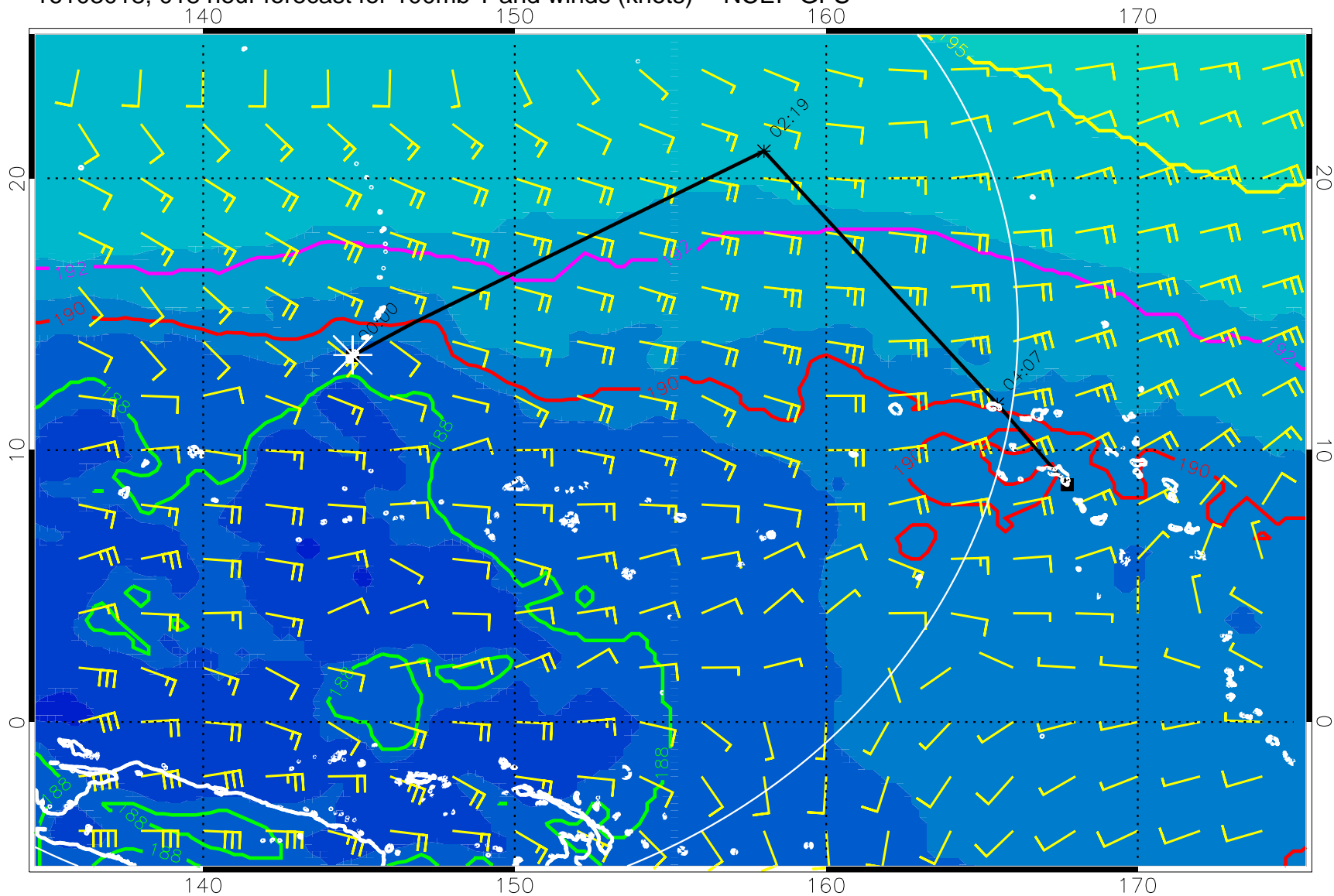
16103018, 018 hour forecast for 100mb T and winds (knots) -- NCEP GFS
