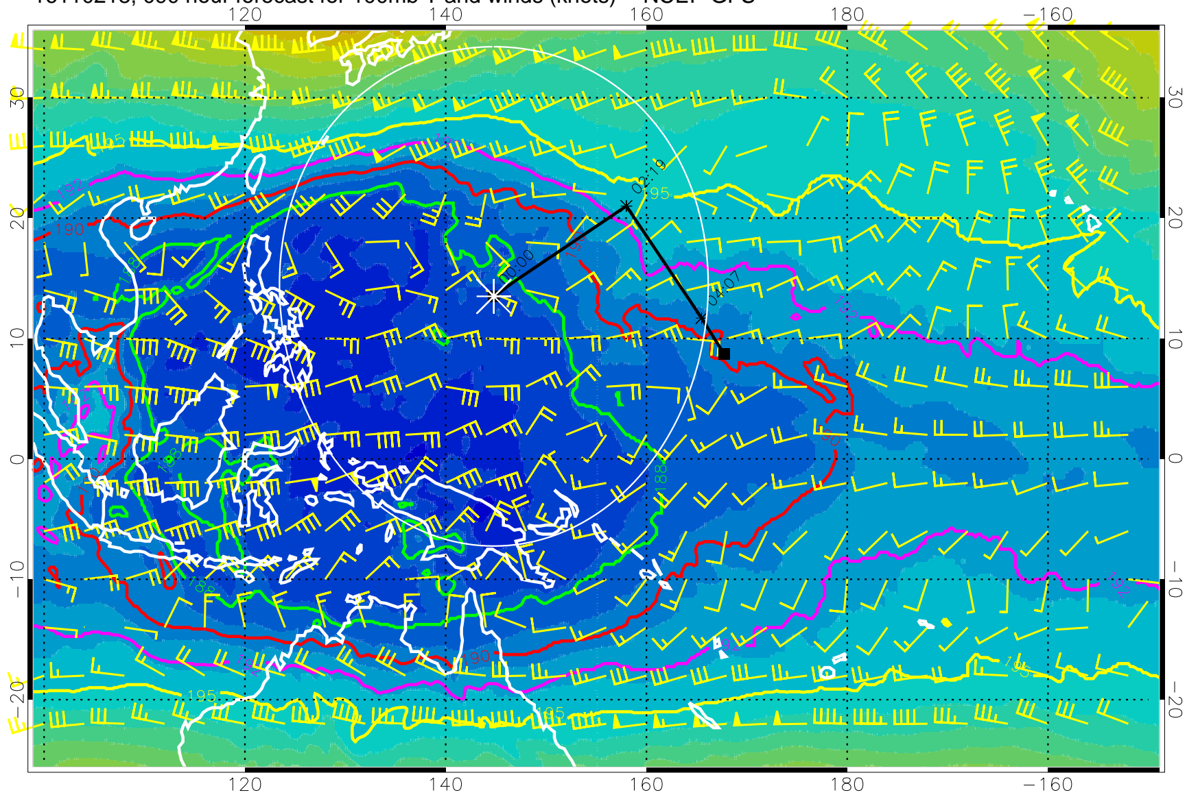
16110218, 090 hour forecast for 100mb T and winds (knots) -- NCEP GFS
