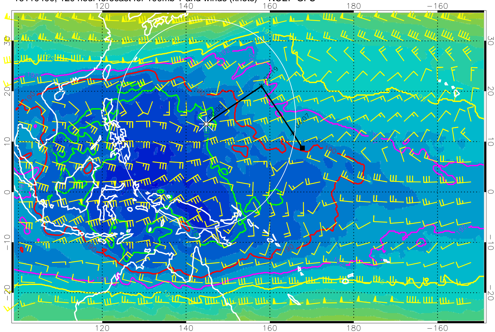
16110400, 120 hour forecast for 100mb T and winds (knots) -- NCEP GFS
