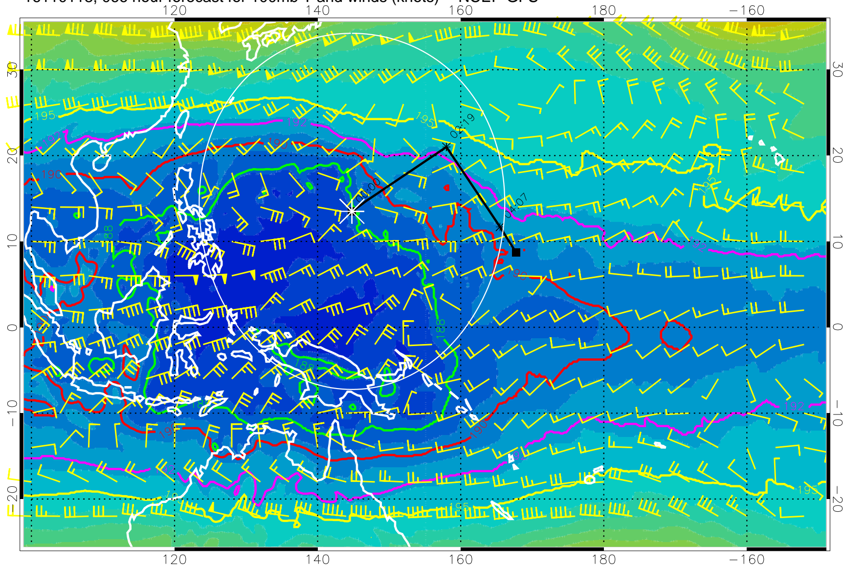
16110118, 066 hour forecast for 100mb T and winds (knots) -- NCEP GFS
