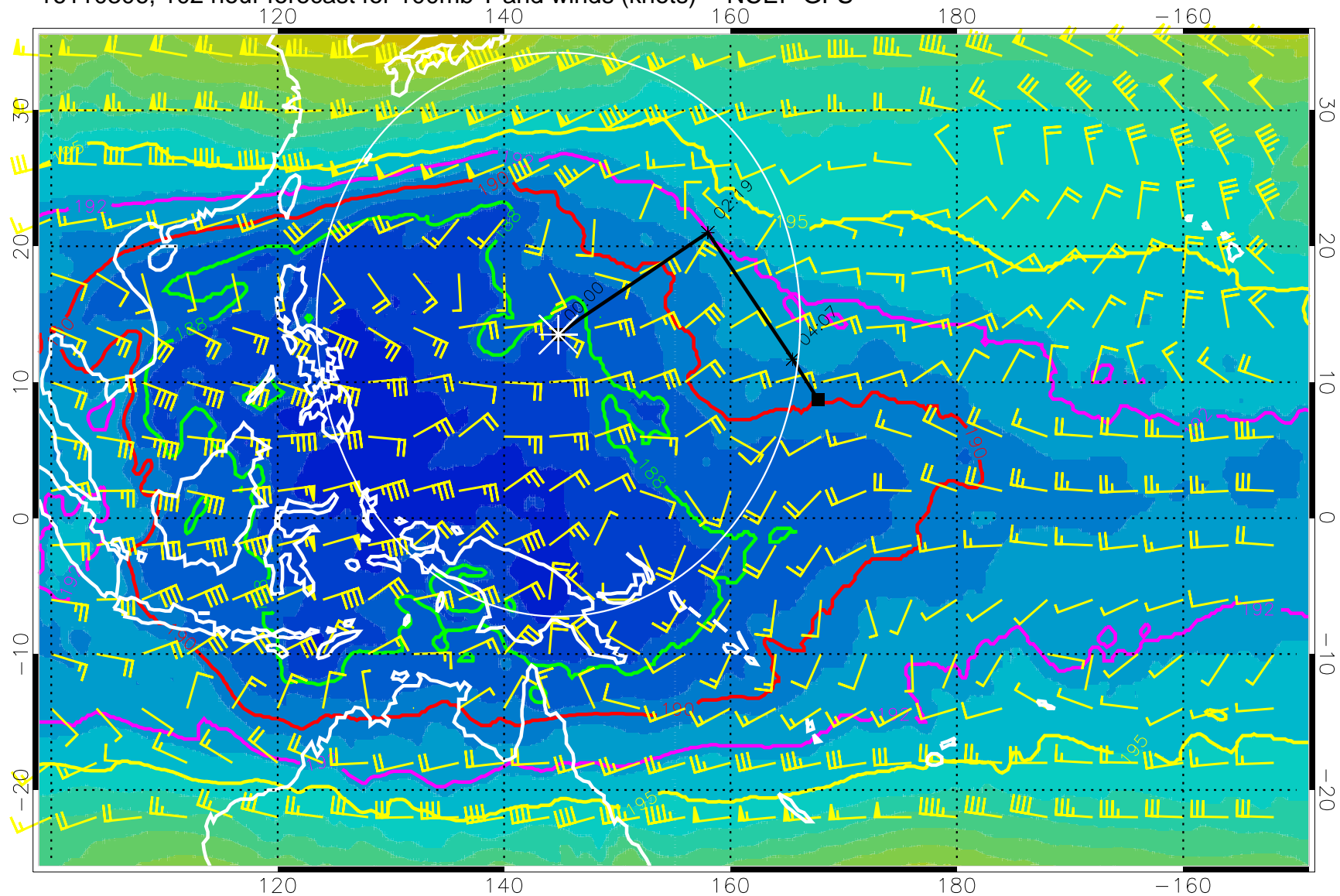
16110306, 102 hour forecast for 100mb T and winds (knots) -- NCEP GFS
