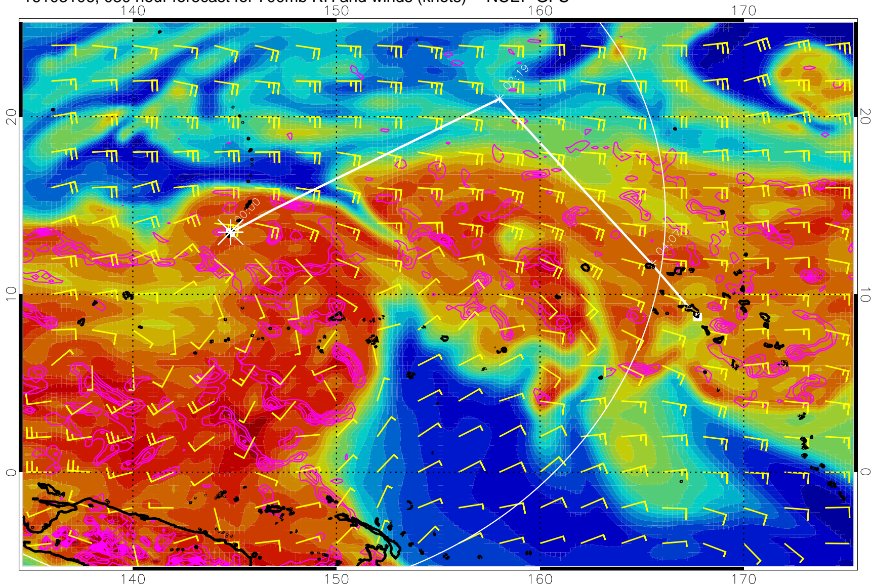
16103106, 030 hour forecast for 700mb RH and winds (knots) -- NCEP GFS
