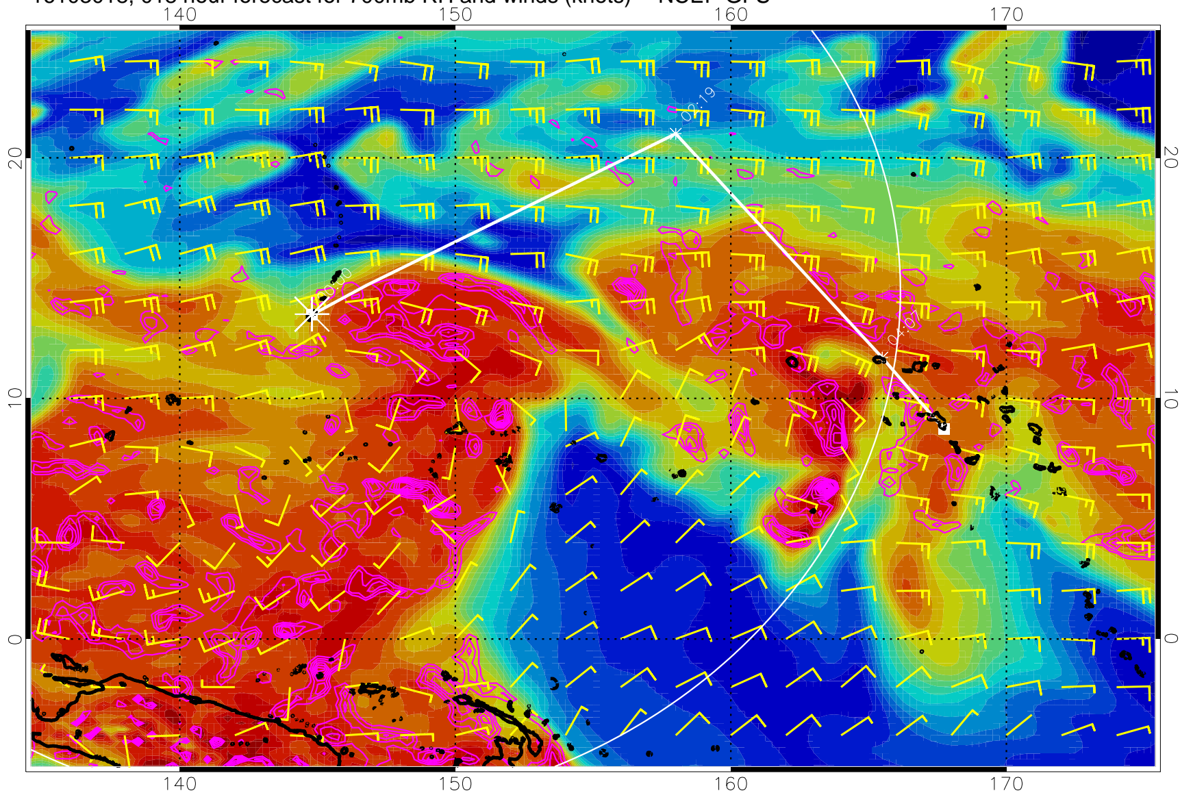
16103018, 018 hour forecast for 700mb RH and winds (knots) -- NCEP GFS
