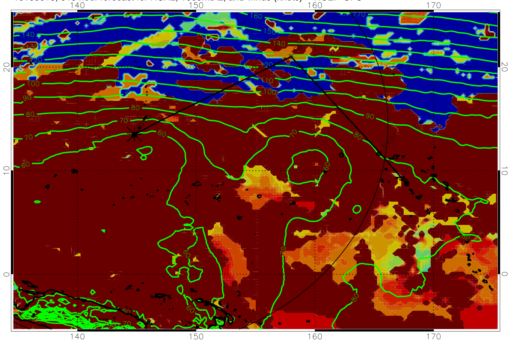
16103018, 018 hour forecast for HCAL, 1000mb Z, and winds (knots) -- NCEP GFS
