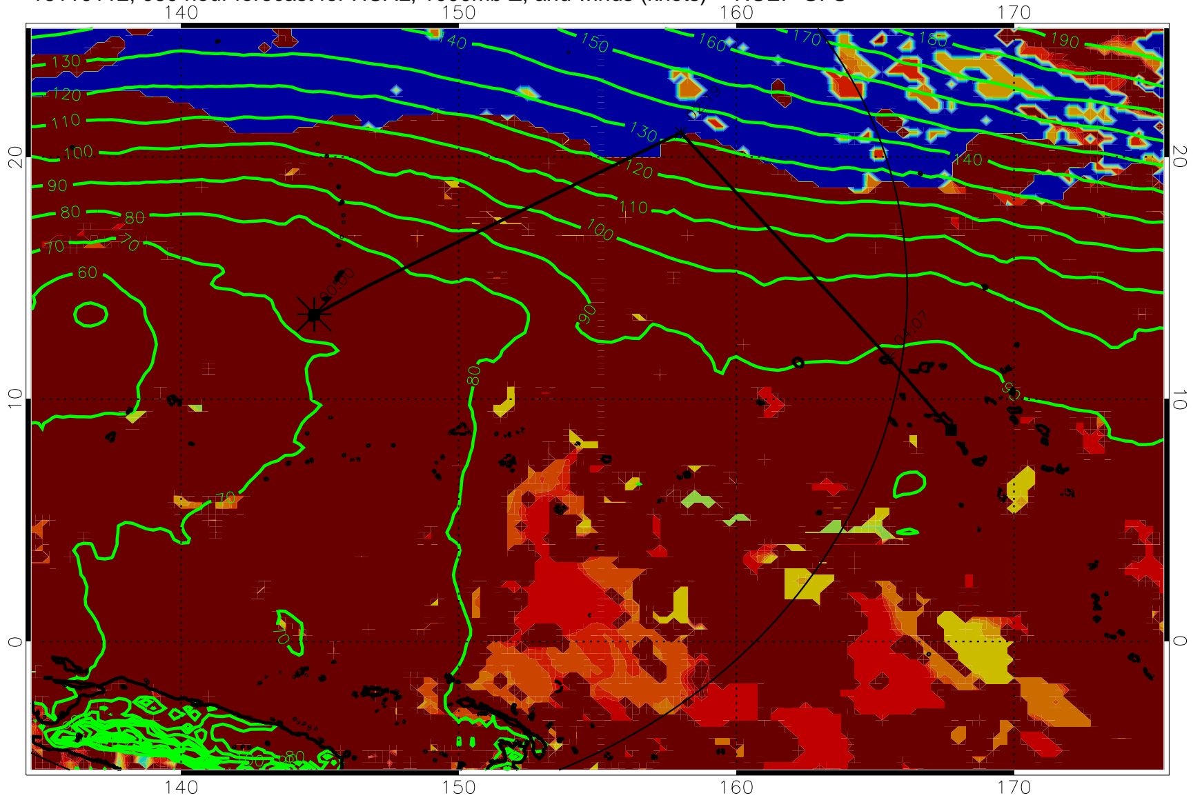
16110112, 060 hour forecast for HCAL, 1000mb Z, and winds (knots) -- NCEP GFS
