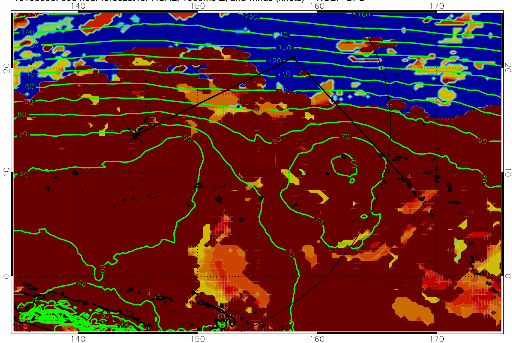
16103006, 006 hour forecast for HCAL, 1000mb Z, and winds (knots) -- NCEP GFS
