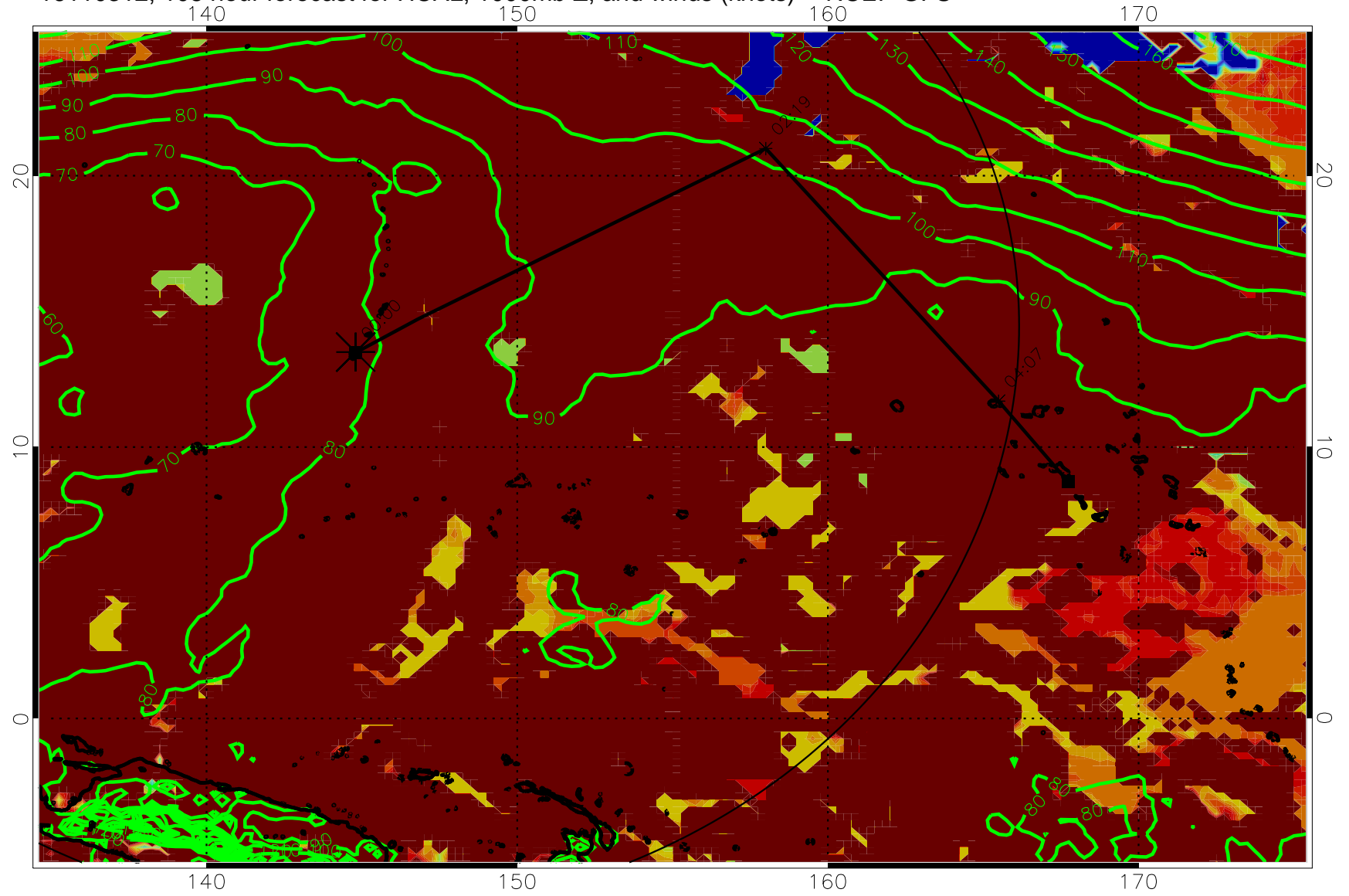
16110312, 108 hour forecast for HCAL, 1000mb Z, and winds (knots) -- NCEP GFS
