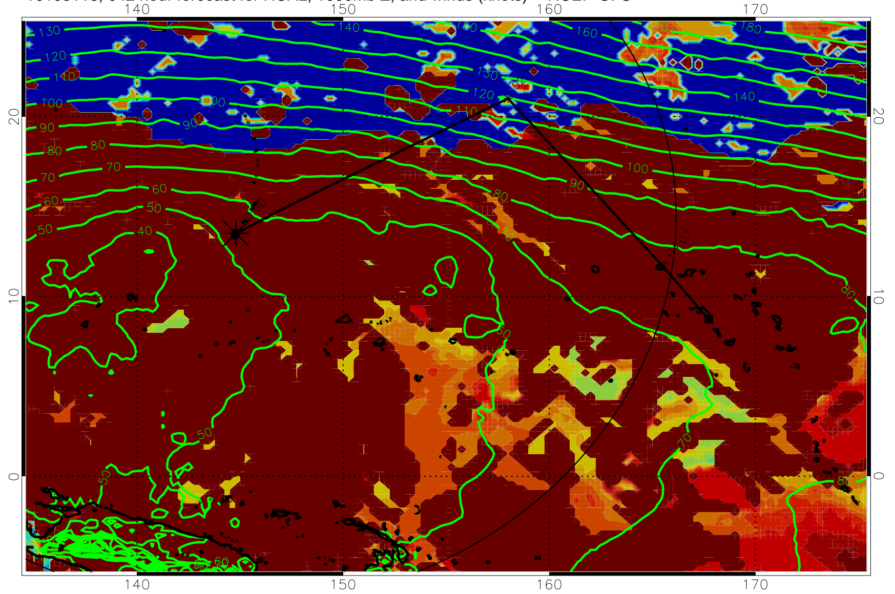
16103118, 042 hour forecast for HCAL, 1000mb Z, and winds (knots) -- NCEP GFS
