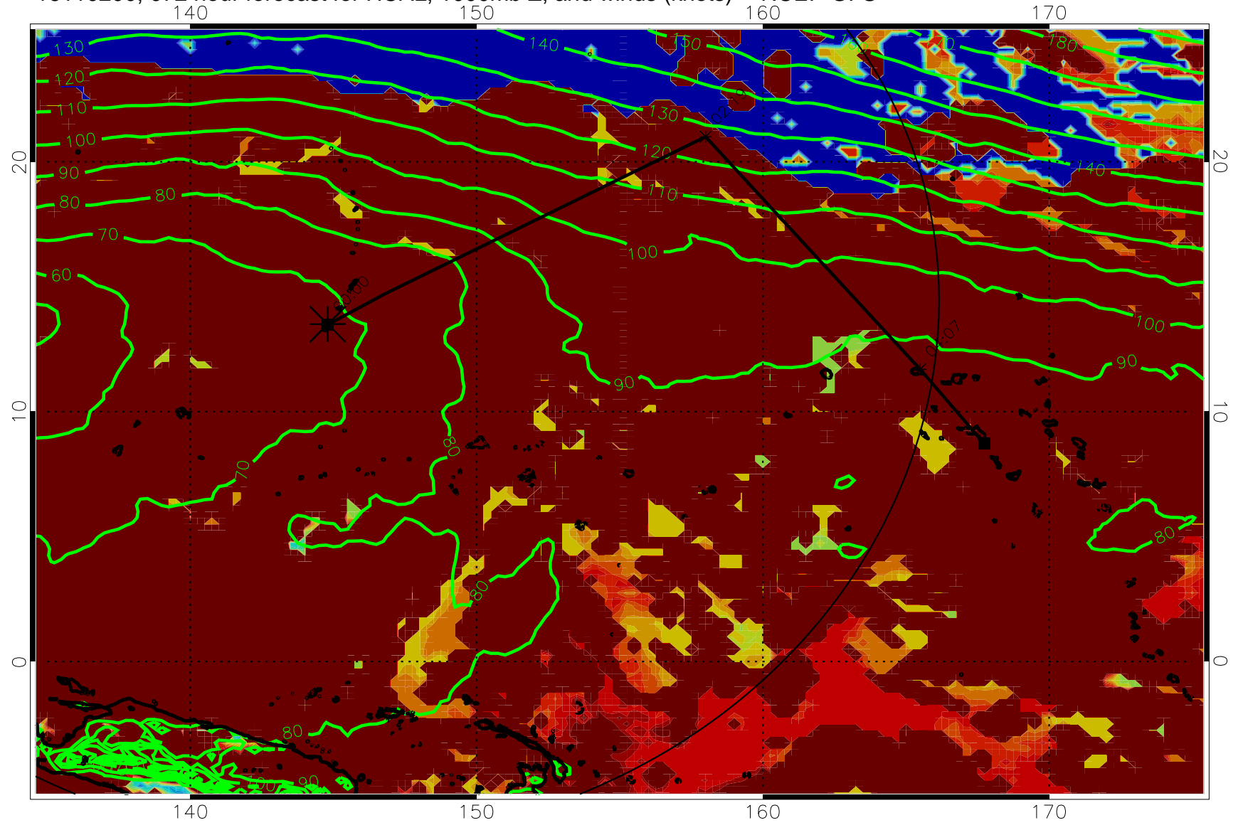
16110200, 072 hour forecast for HCAL, 1000mb Z, and winds (knots) -- NCEP GFS
