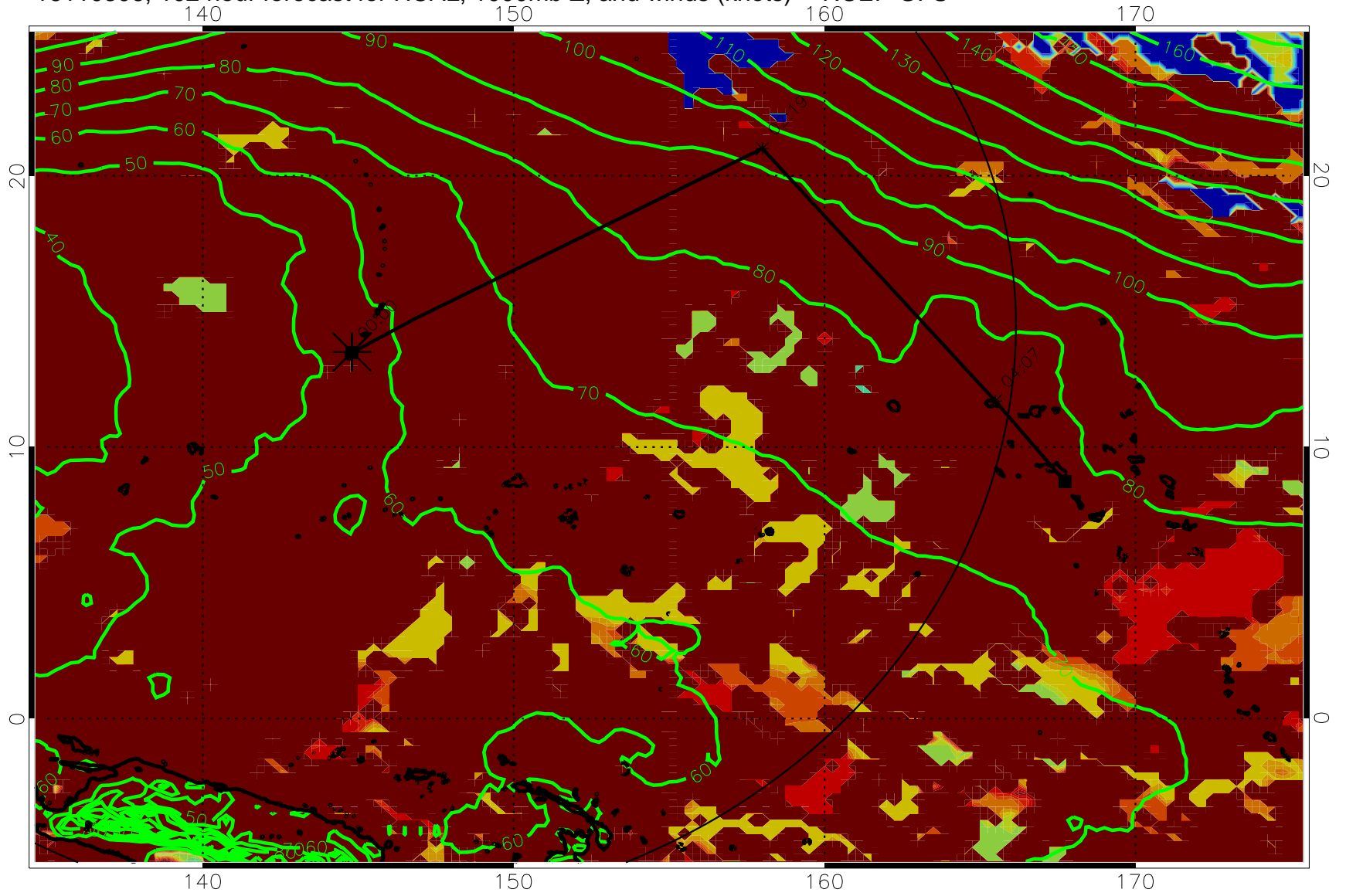
16110306, 102 hour forecast for HCAL, 1000mb Z, and winds (knots) -- NCEP GFS
