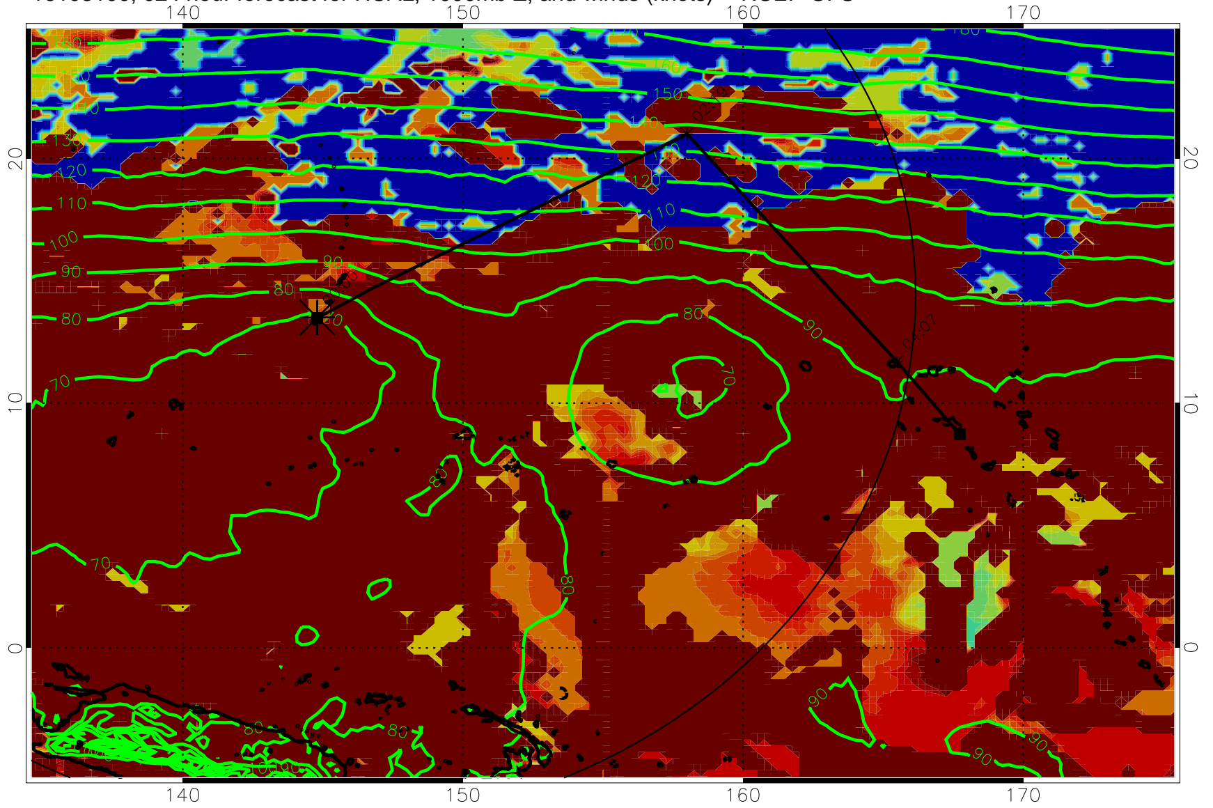
16103100, 024 hour forecast for HCAL, 1000mb Z, and winds (knots) -- NCEP GFS
