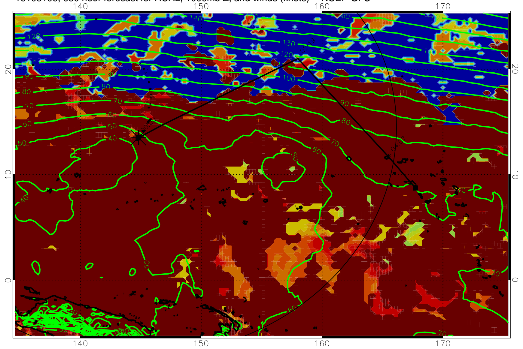
16103106, 030 hour forecast for HCAL, 1000mb Z, and winds (knots) -- NCEP GFS
