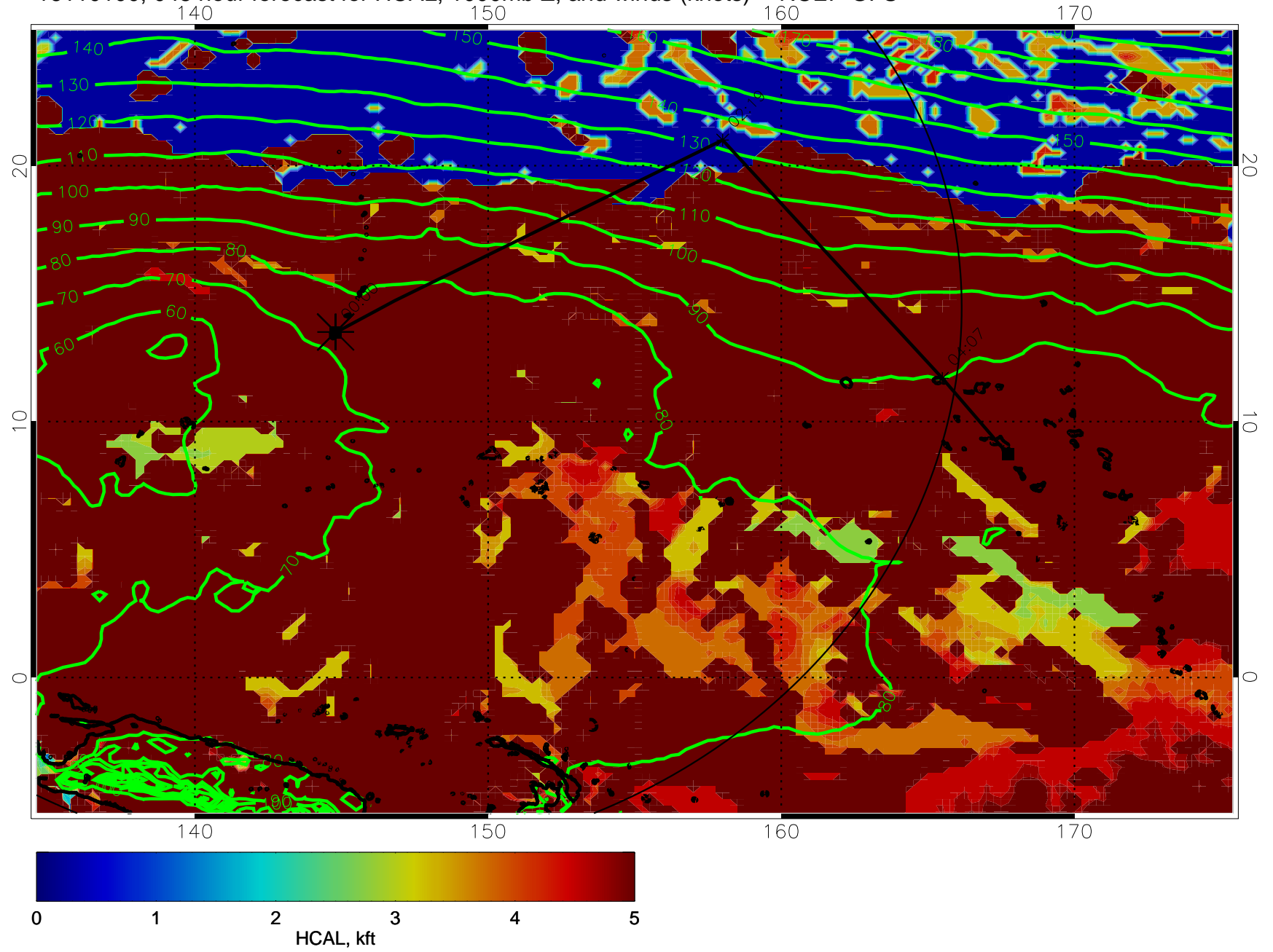
16110100, 048 hour forecast for HCAL, 1000mb Z, and winds (knots) -- NCEP GFS
