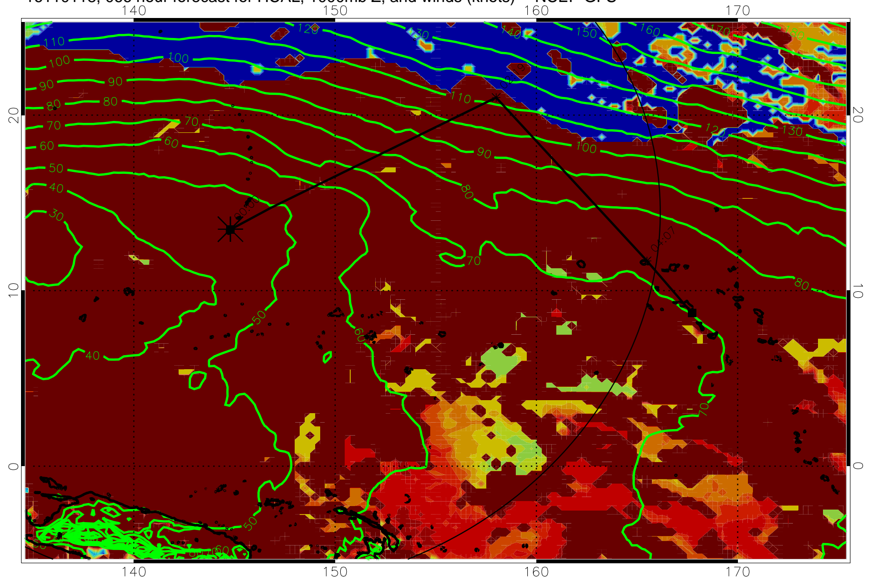
16110118, 066 hour forecast for HCAL, 1000mb Z, and winds (knots) -- NCEP GFS
