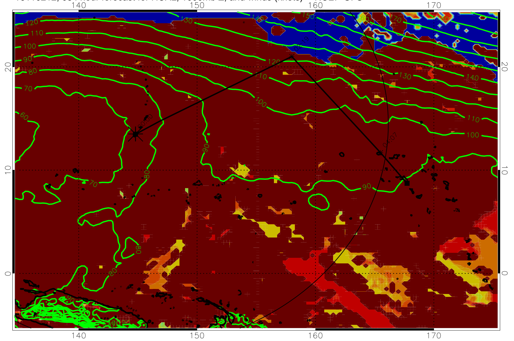
16110212, 084 hour forecast for HCAL, 1000mb Z, and winds (knots) -- NCEP GFS
