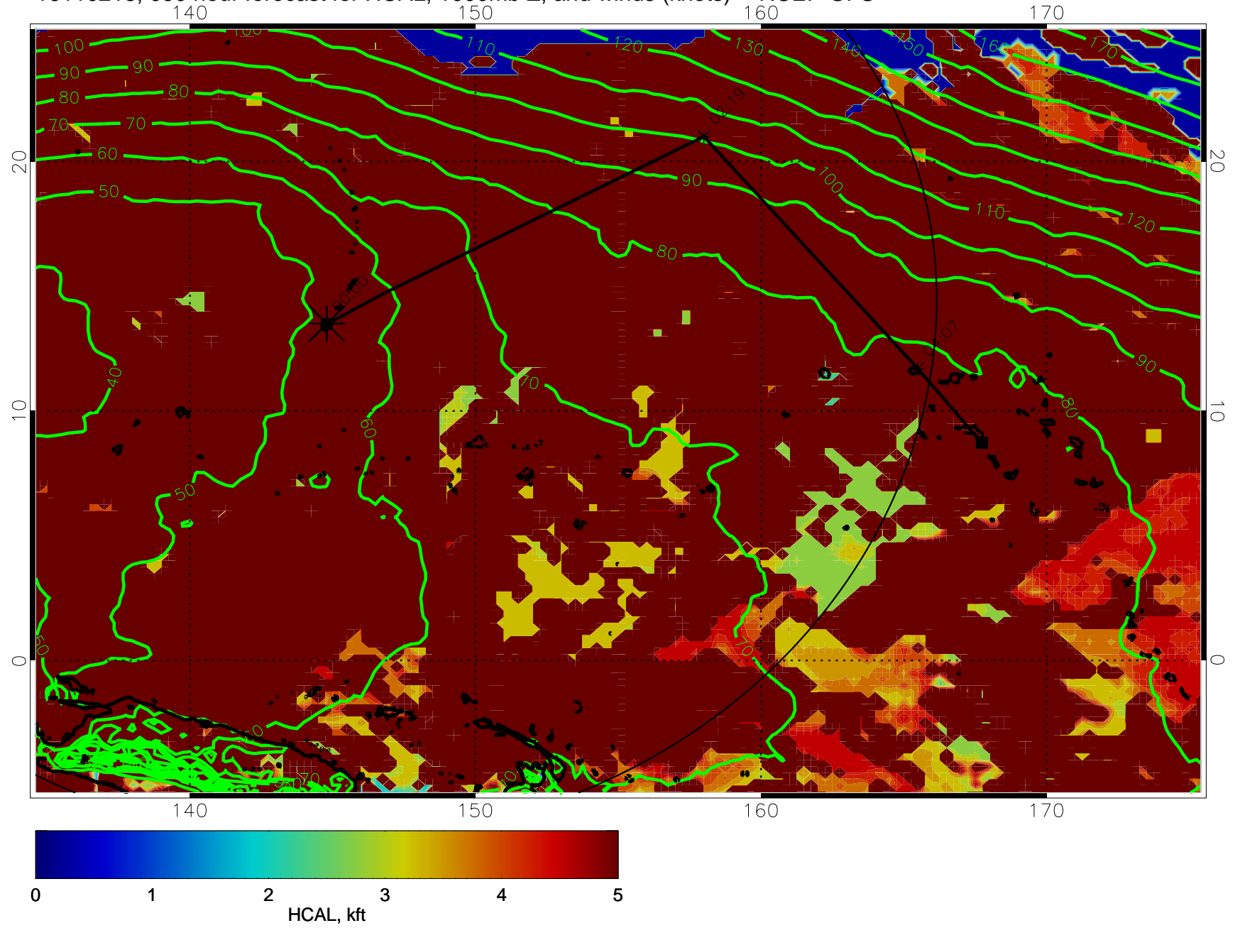
16110218, 090 hour forecast for HCAL, 1000mb Z, and winds (knots) -- NCEP GFS
