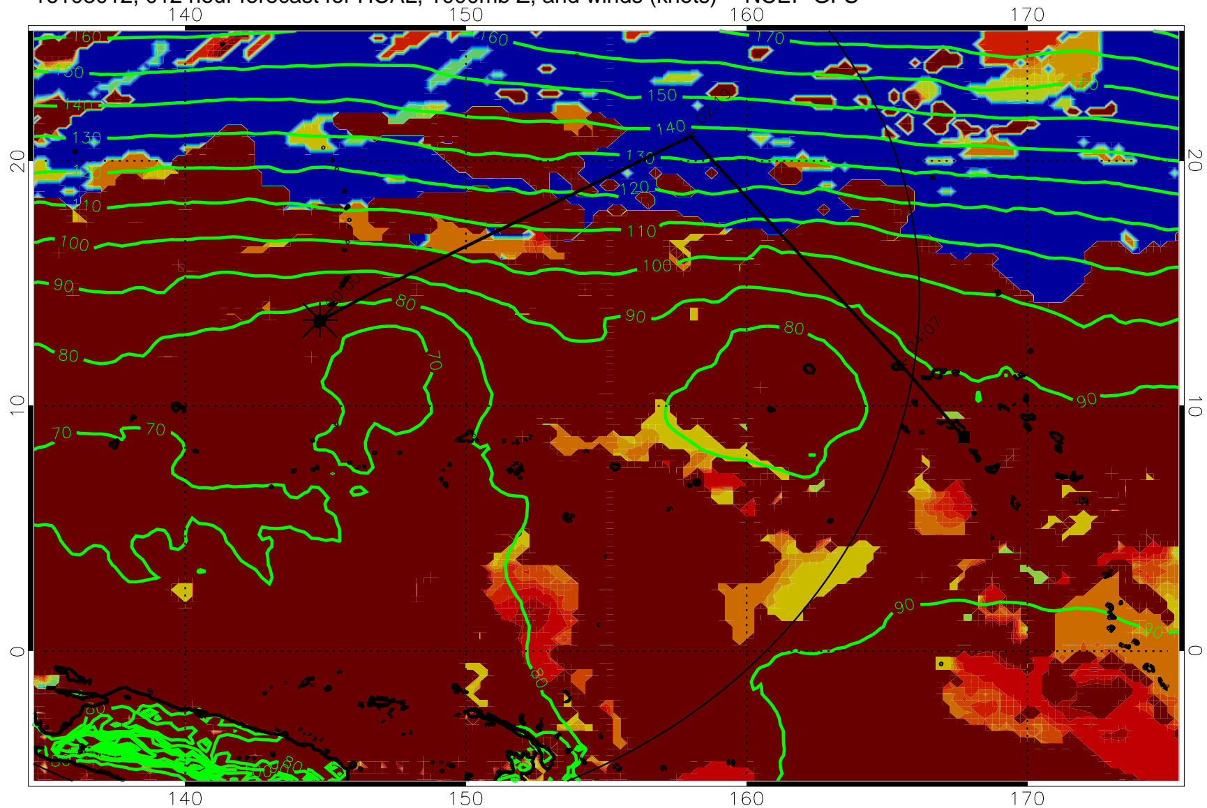
16103012, 012 hour forecast for HCAL, 1000mb Z, and winds (knots) -- NCEP GFS
