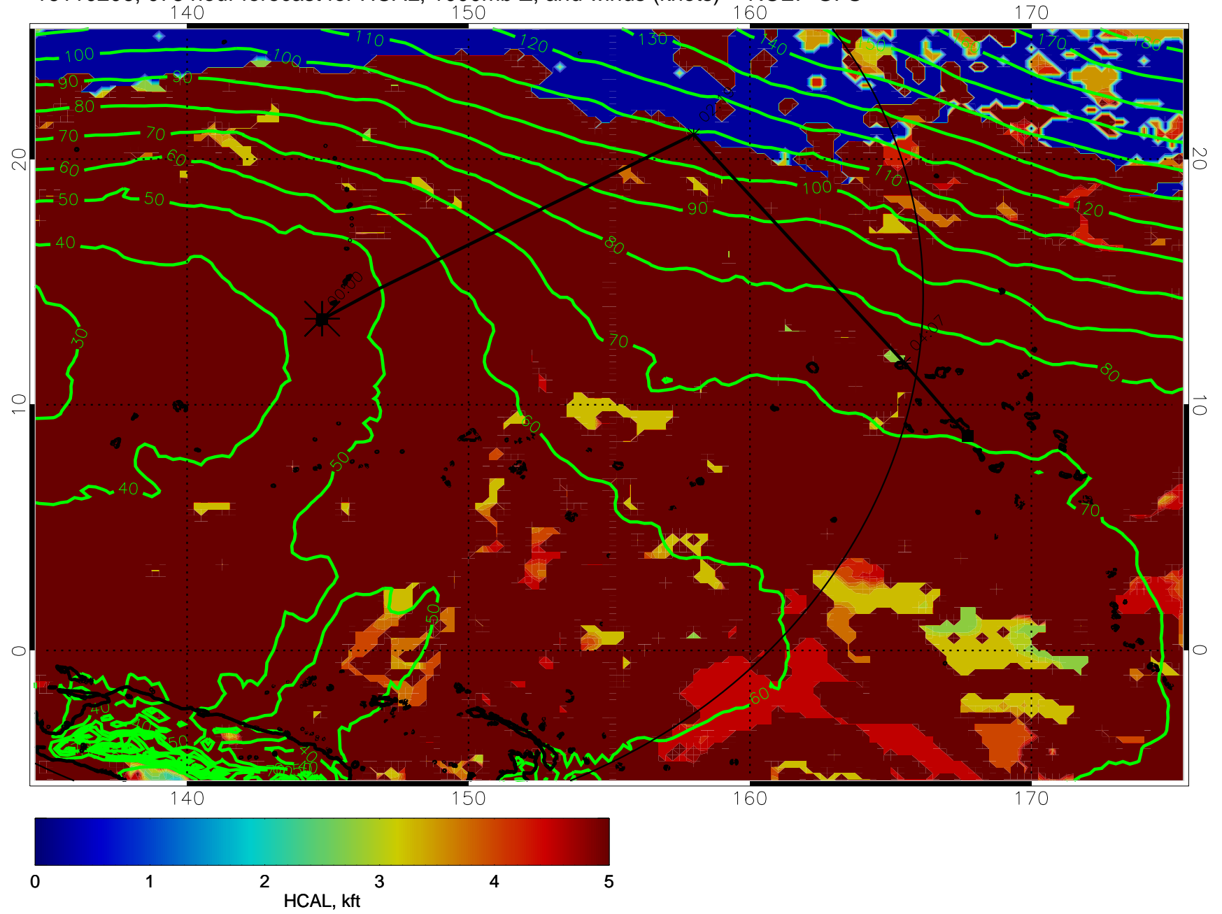
16110206, 078 hour forecast for HCAL, 1000mb Z, and winds (knots) -- NCEP GFS
