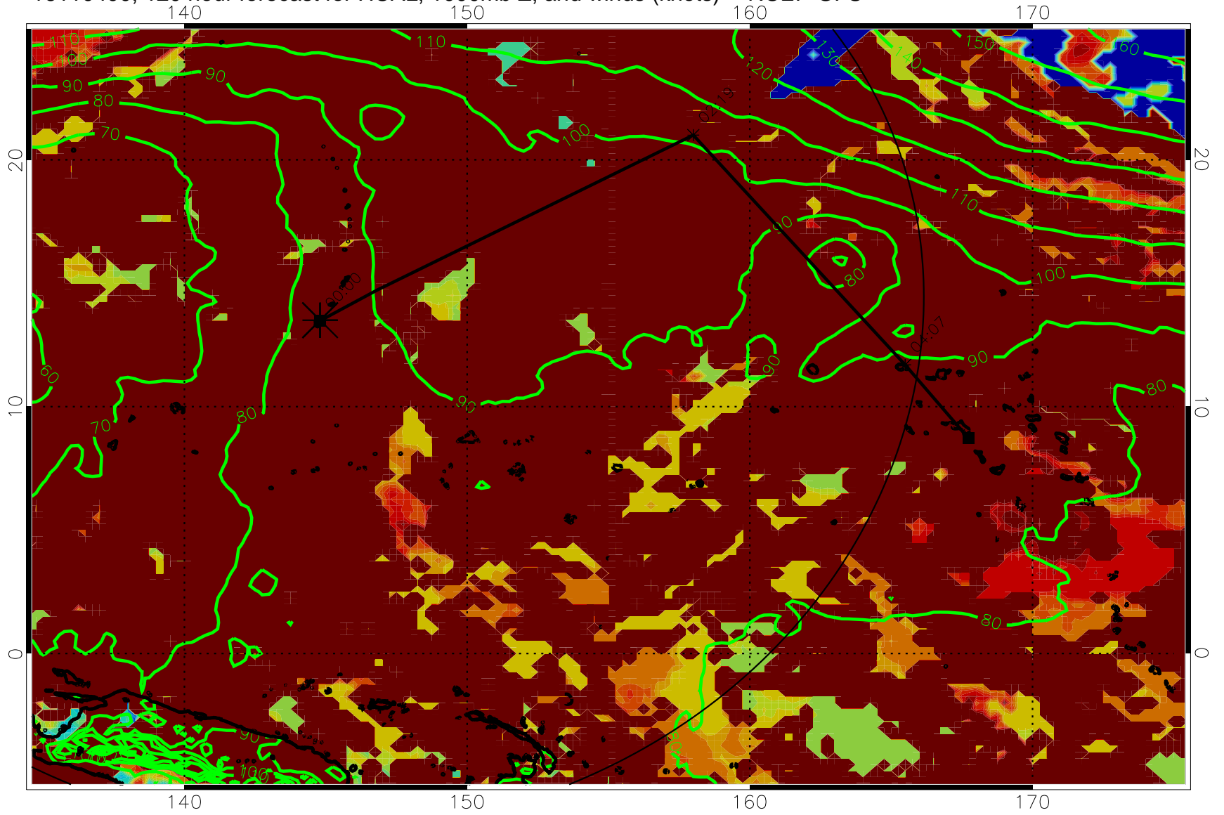
16110400, 120 hour forecast for HCAL, 1000mb Z, and winds (knots) -- NCEP GFS
