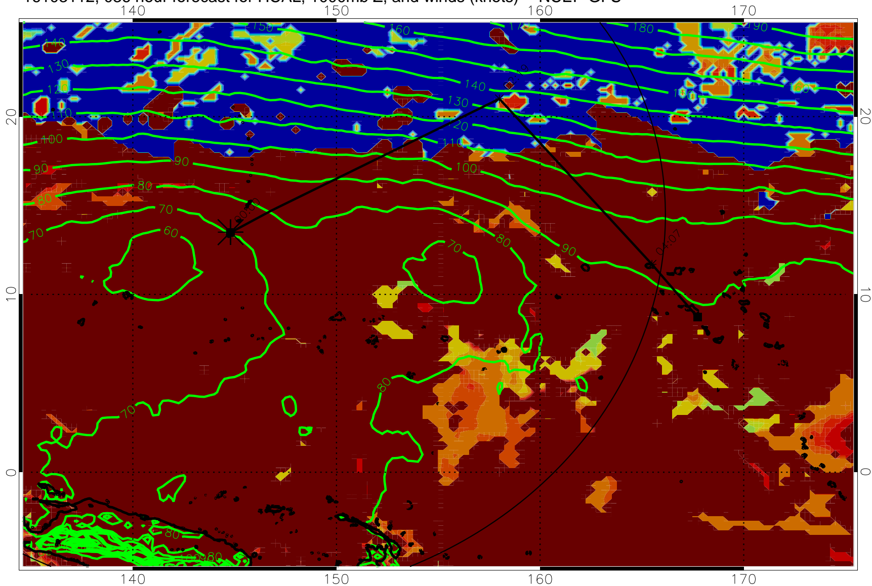
16103112, 036 hour forecast for HCAL, 1000mb Z, and winds (knots) -- NCEP GFS
