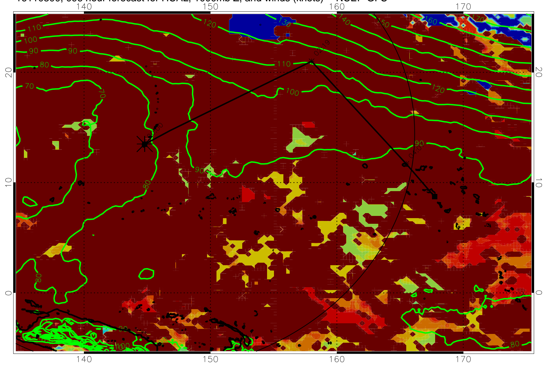
16110300, 096 hour forecast for HCAL, 1000mb Z, and winds (knots) -- NCEP GFS
