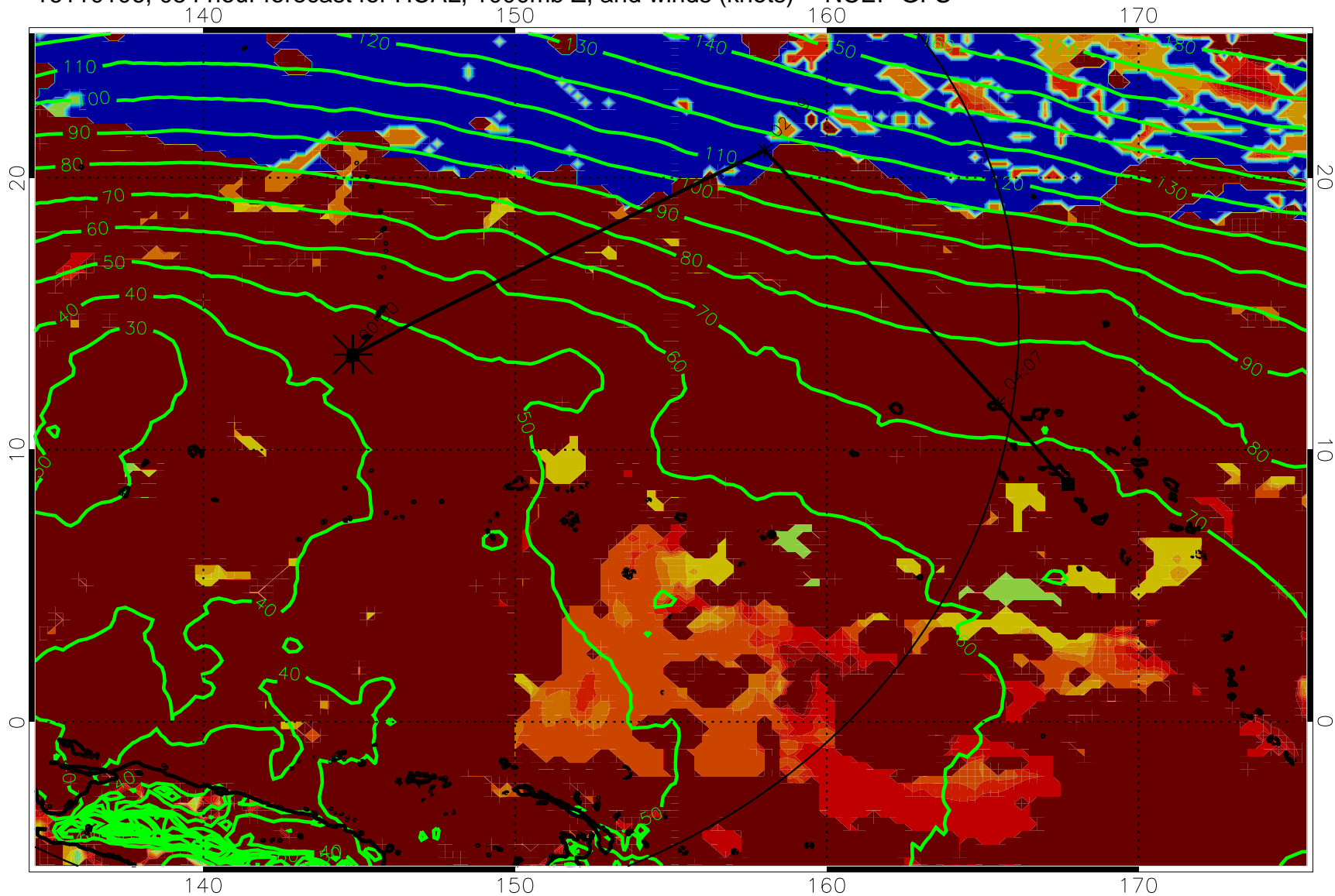
16110106, 054 hour forecast for HCAL, 1000mb Z, and winds (knots) -- NCEP GFS
