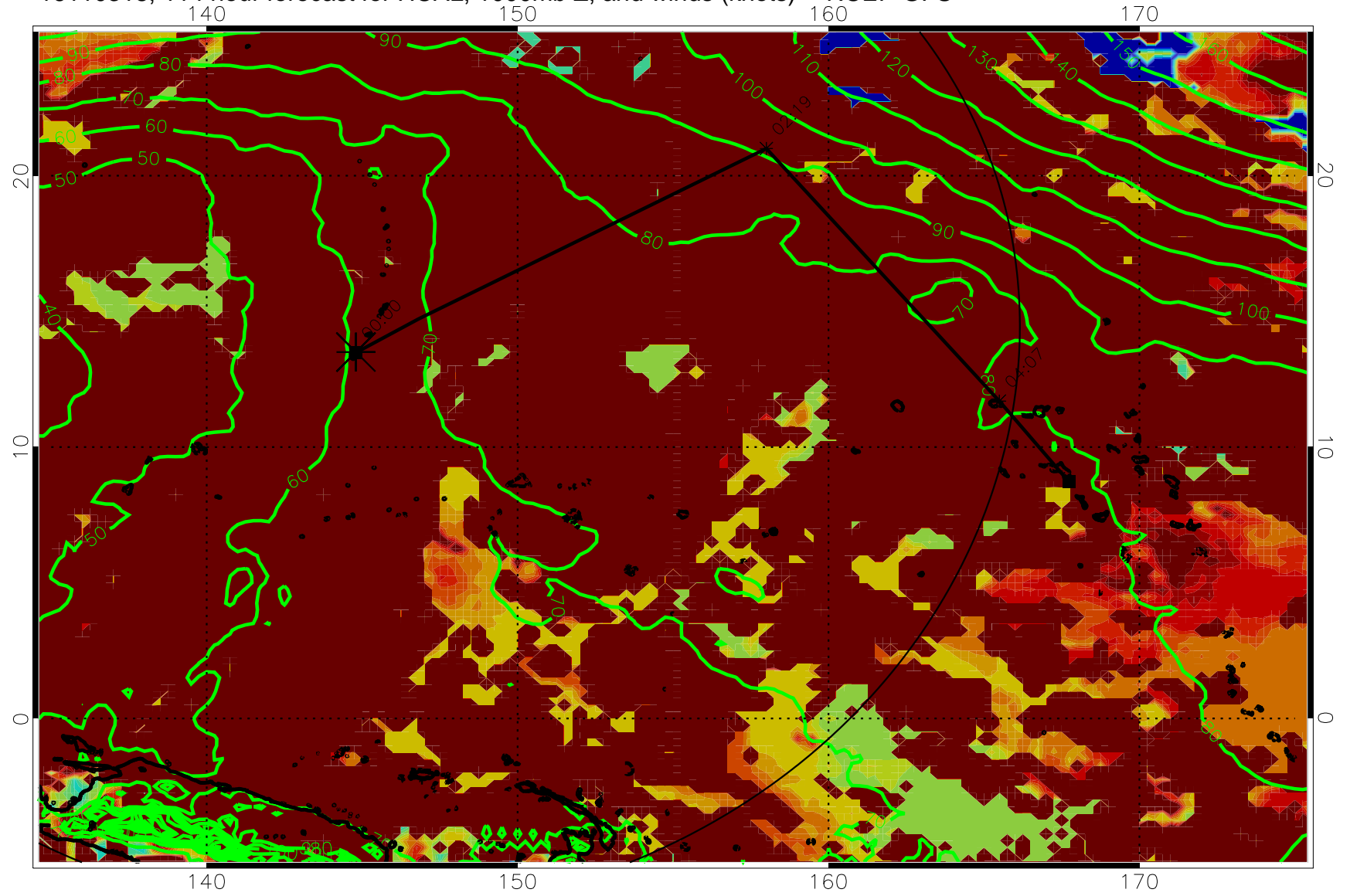
16110318, 114 hour forecast for HCAL, 1000mb Z, and winds (knots) -- NCEP GFS
