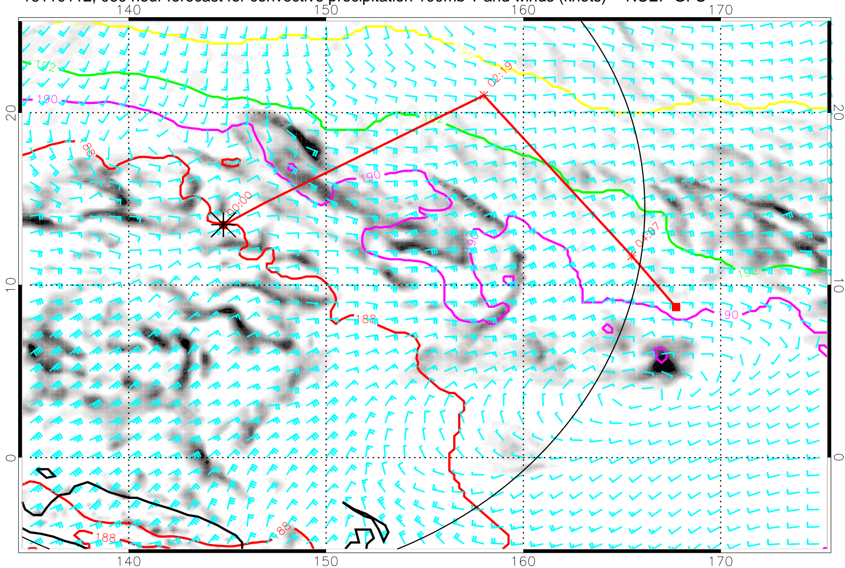
16110112, 060 hour forecast for convective precipitation 100mb T and winds (knots) -- NCEP GFS
