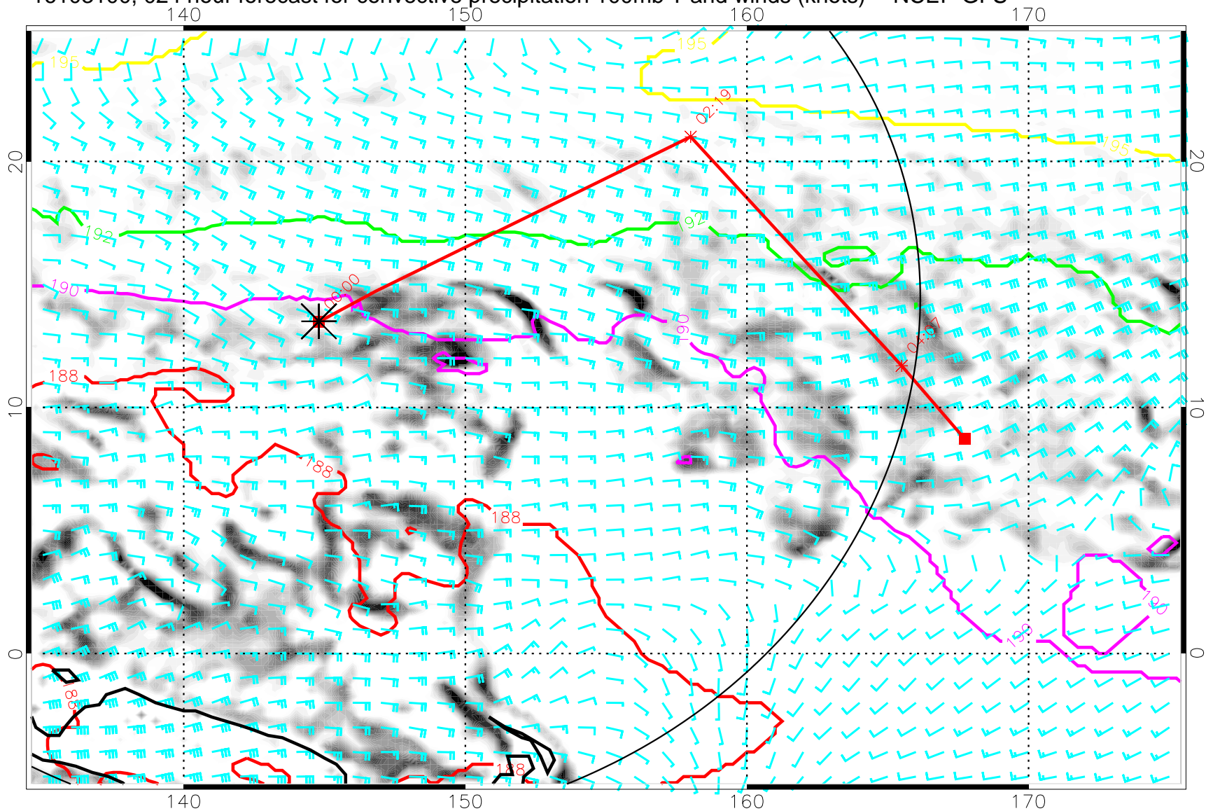
16103100, 024 hour forecast for convective precipitation 100mb T and winds (knots) -- NCEP GFS
