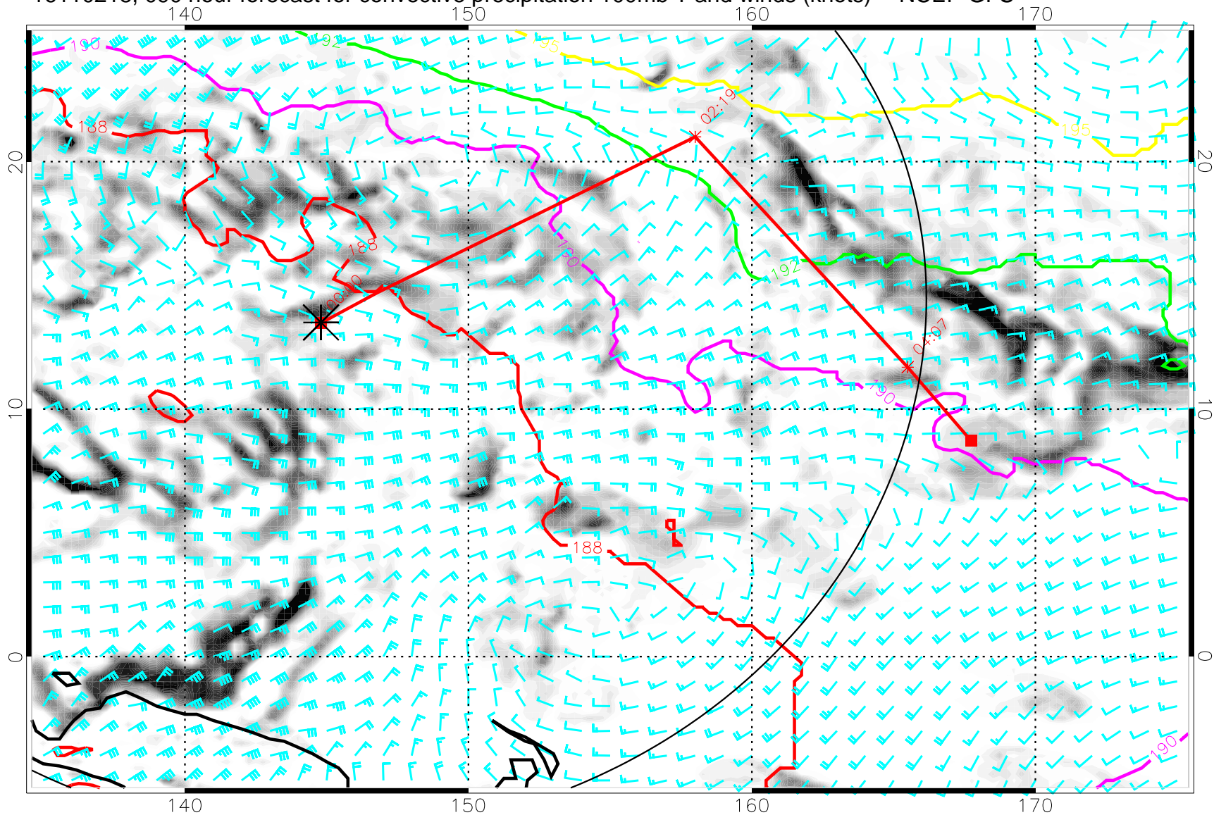
16110218, 090 hour forecast for convective precipitation 100mb T and winds (knots) -- NCEP GFS
