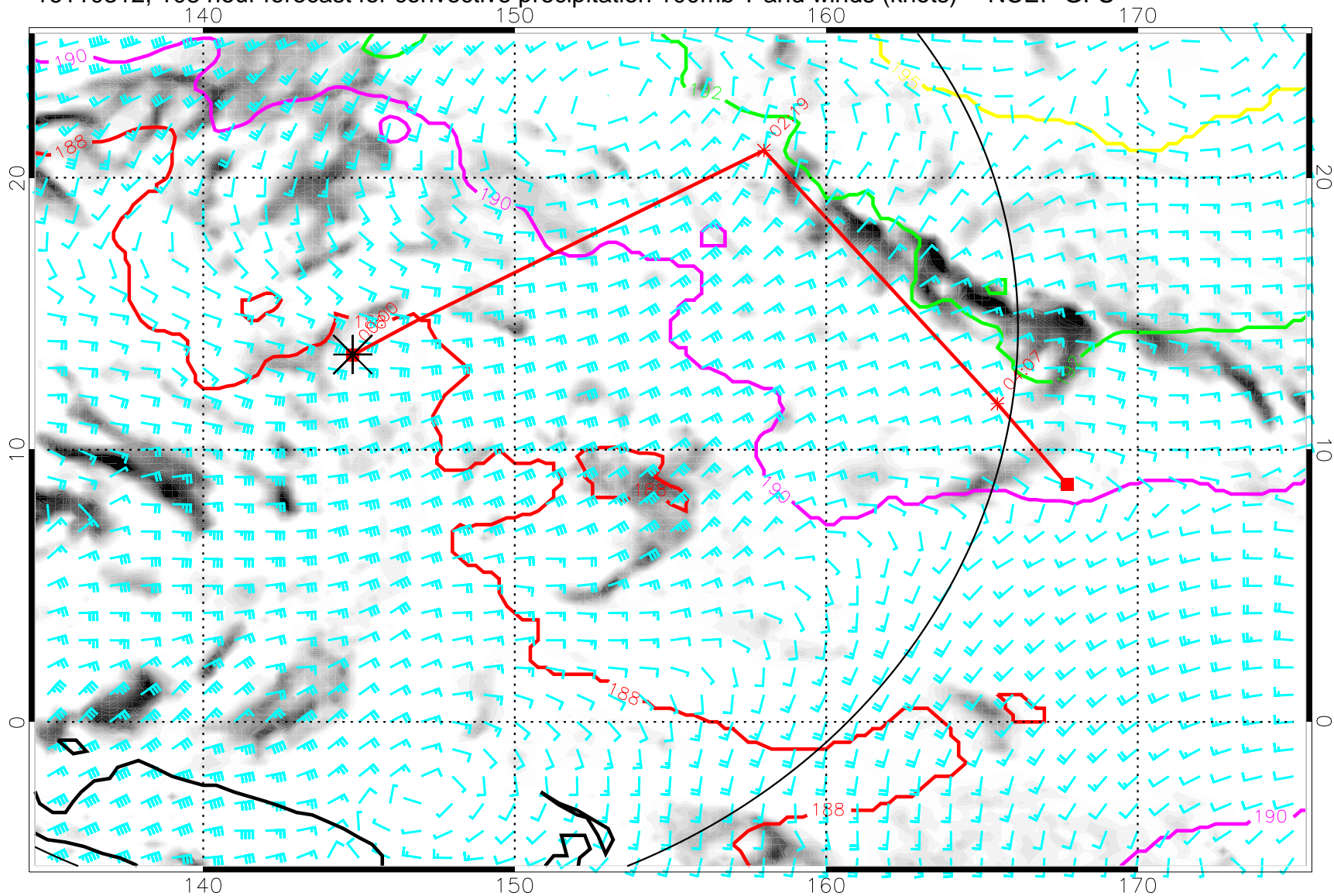
16110312, 108 hour forecast for convective precipitation 100mb T and winds (knots) -- NCEP GFS
