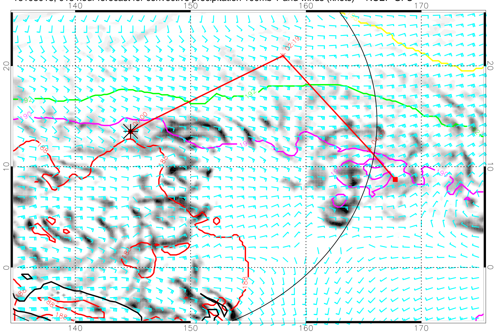
16103018, 018 hour forecast for convective precipitation 100mb T and winds (knots) -- NCEP GFS
