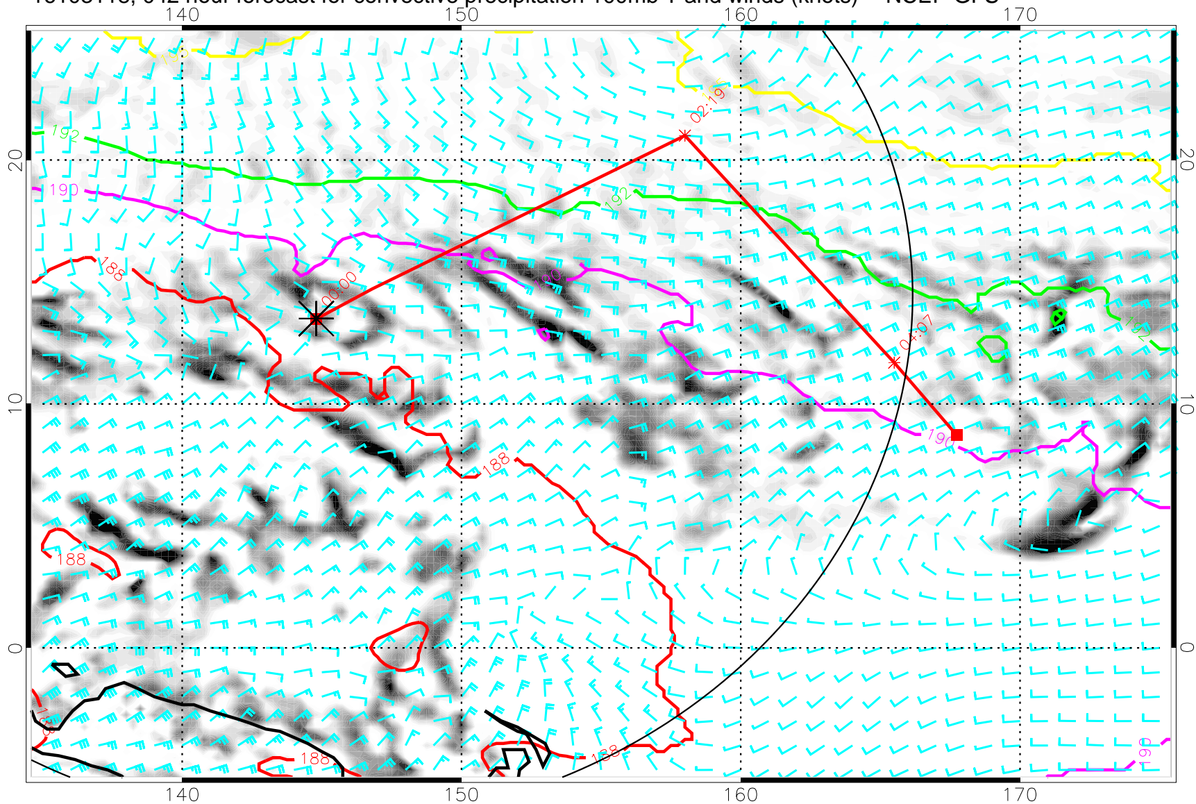
16103118, 042 hour forecast for convective precipitation 100mb T and winds (knots) -- NCEP GFS
