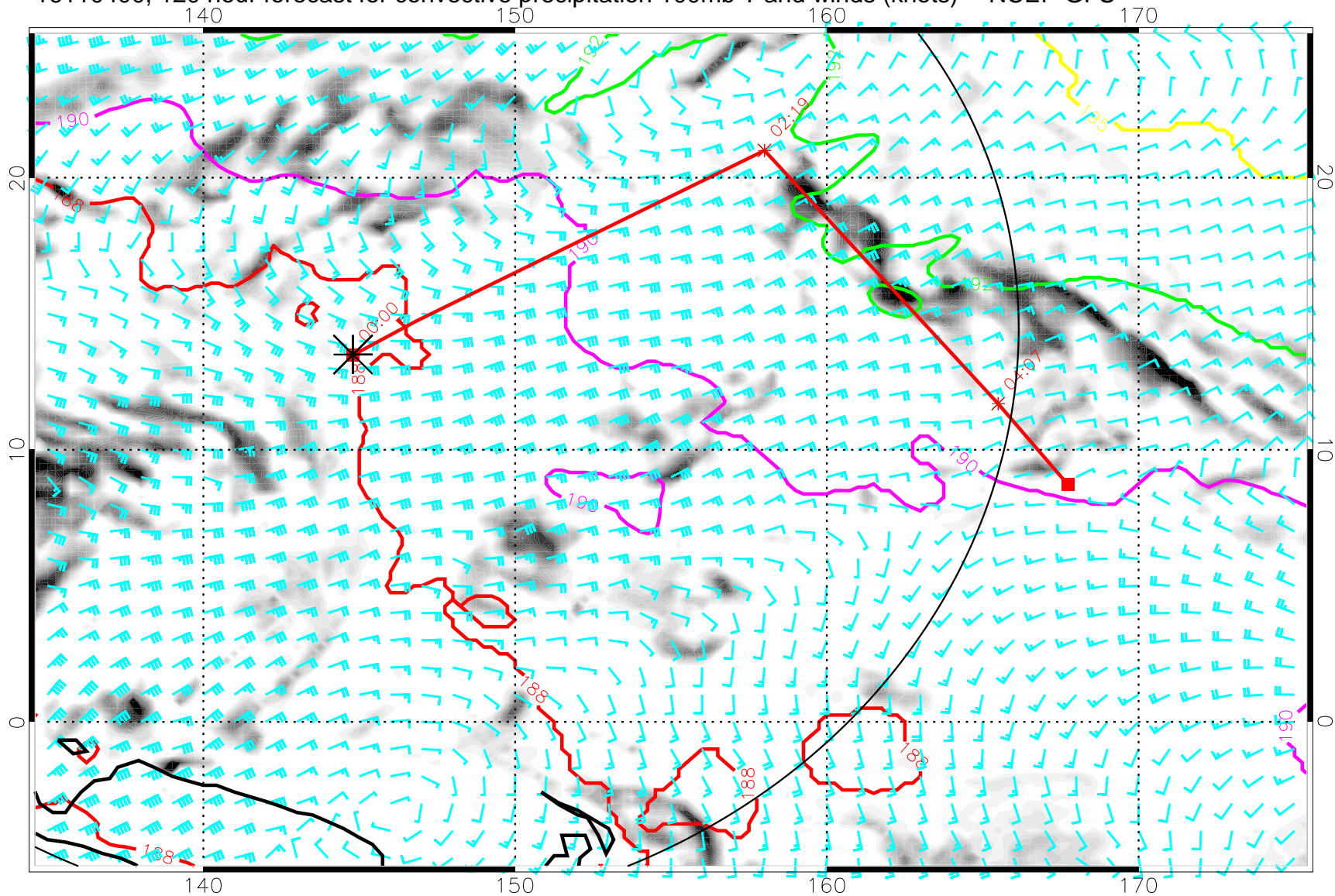
16110400, 120 hour forecast for convective precipitation 100mb T and winds (knots) -- NCEP GFS
