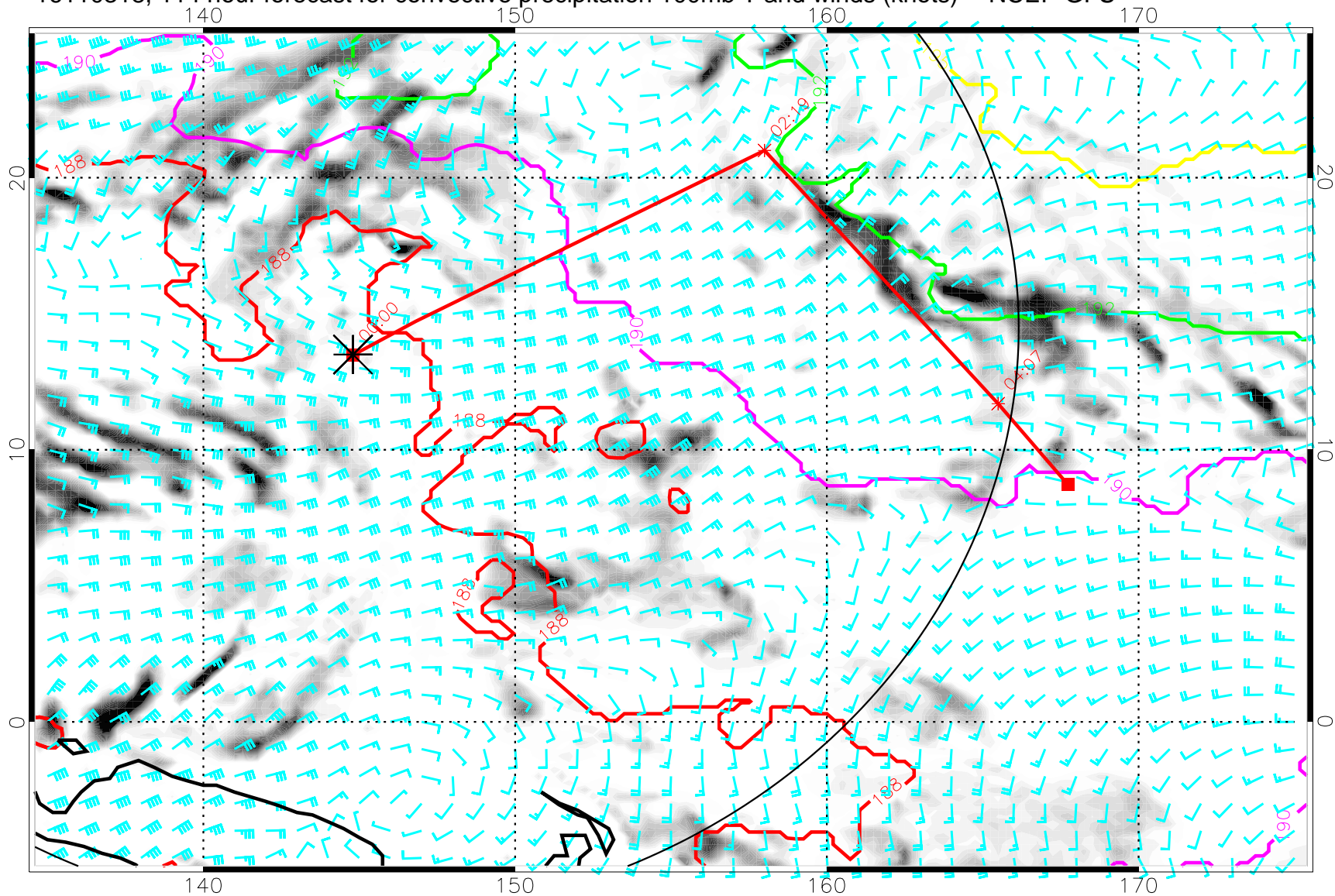
16110318, 114 hour forecast for convective precipitation 100mb T and winds (knots) -- NCEP GFS
