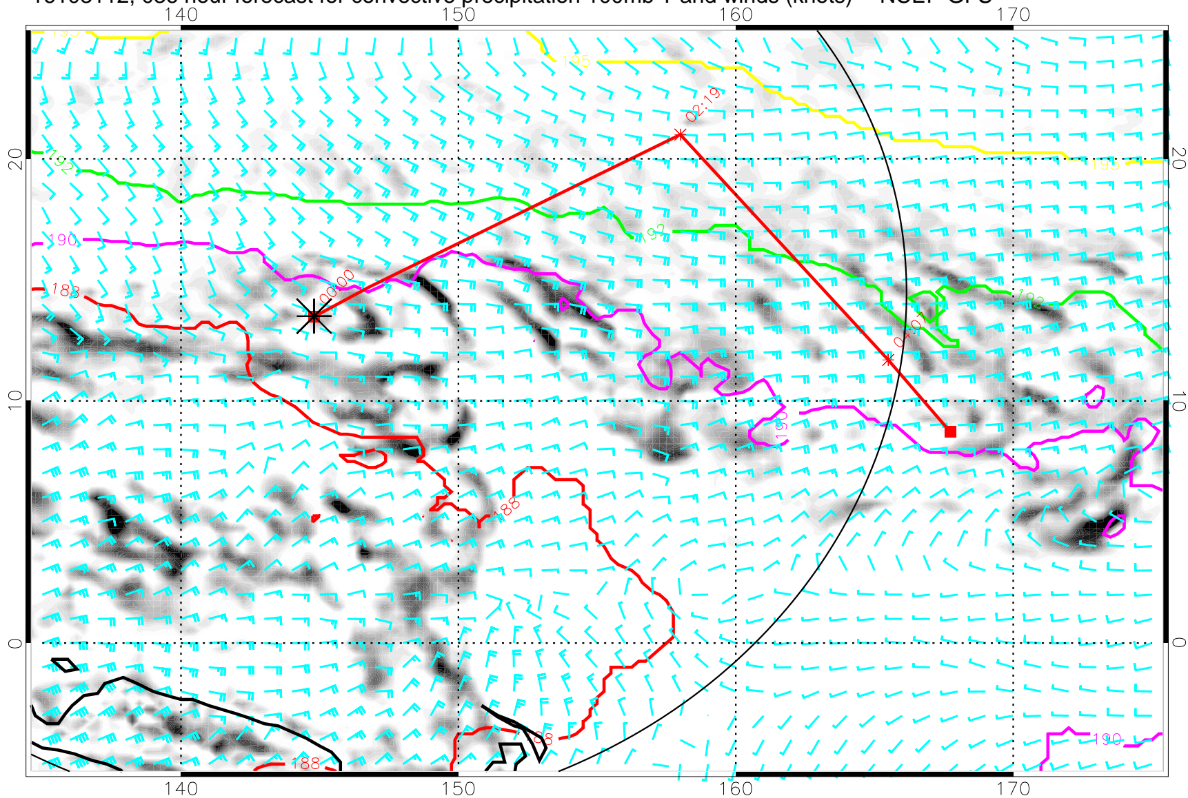
16103112, 036 hour forecast for convective precipitation 100mb T and winds (knots) -- NCEP GFS
