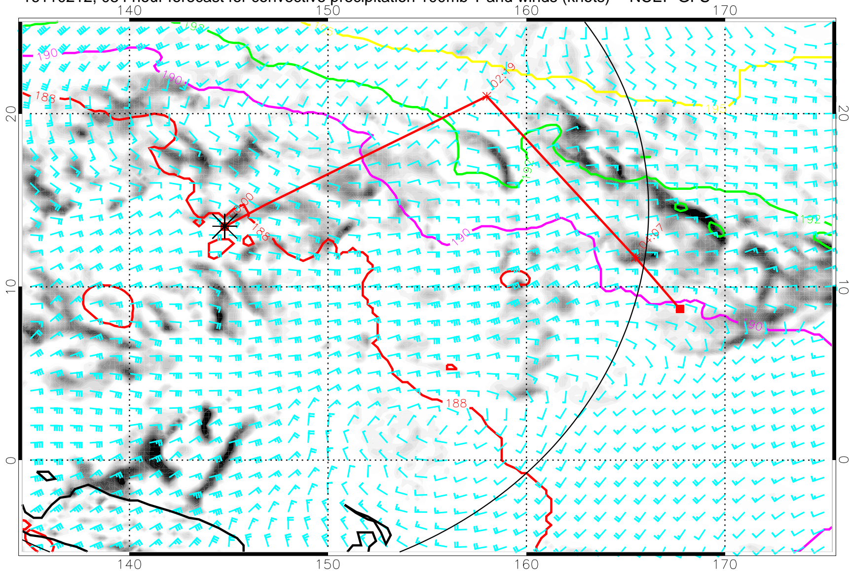
16110212, 084 hour forecast for convective precipitation 100mb T and winds (knots) -- NCEP GFS
