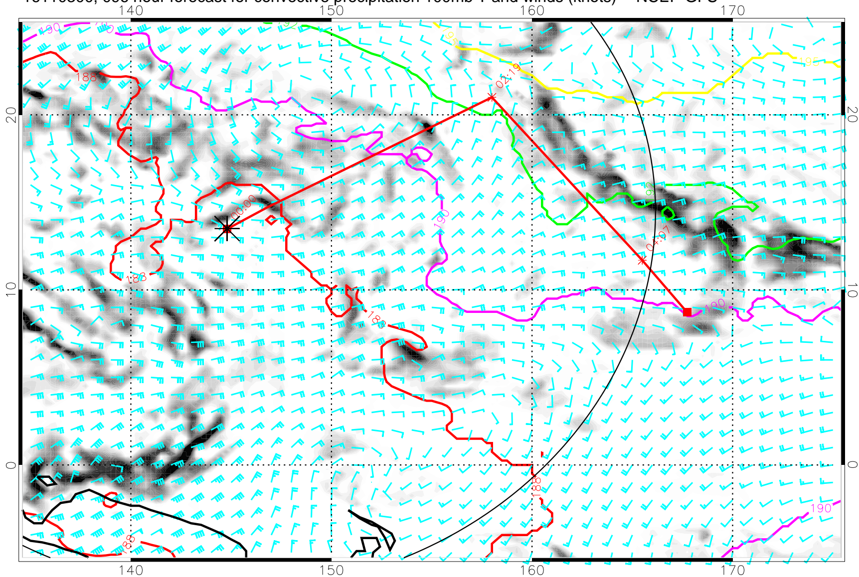
16110300, 096 hour forecast for convective precipitation 100mb T and winds (knots) -- NCEP GFS
