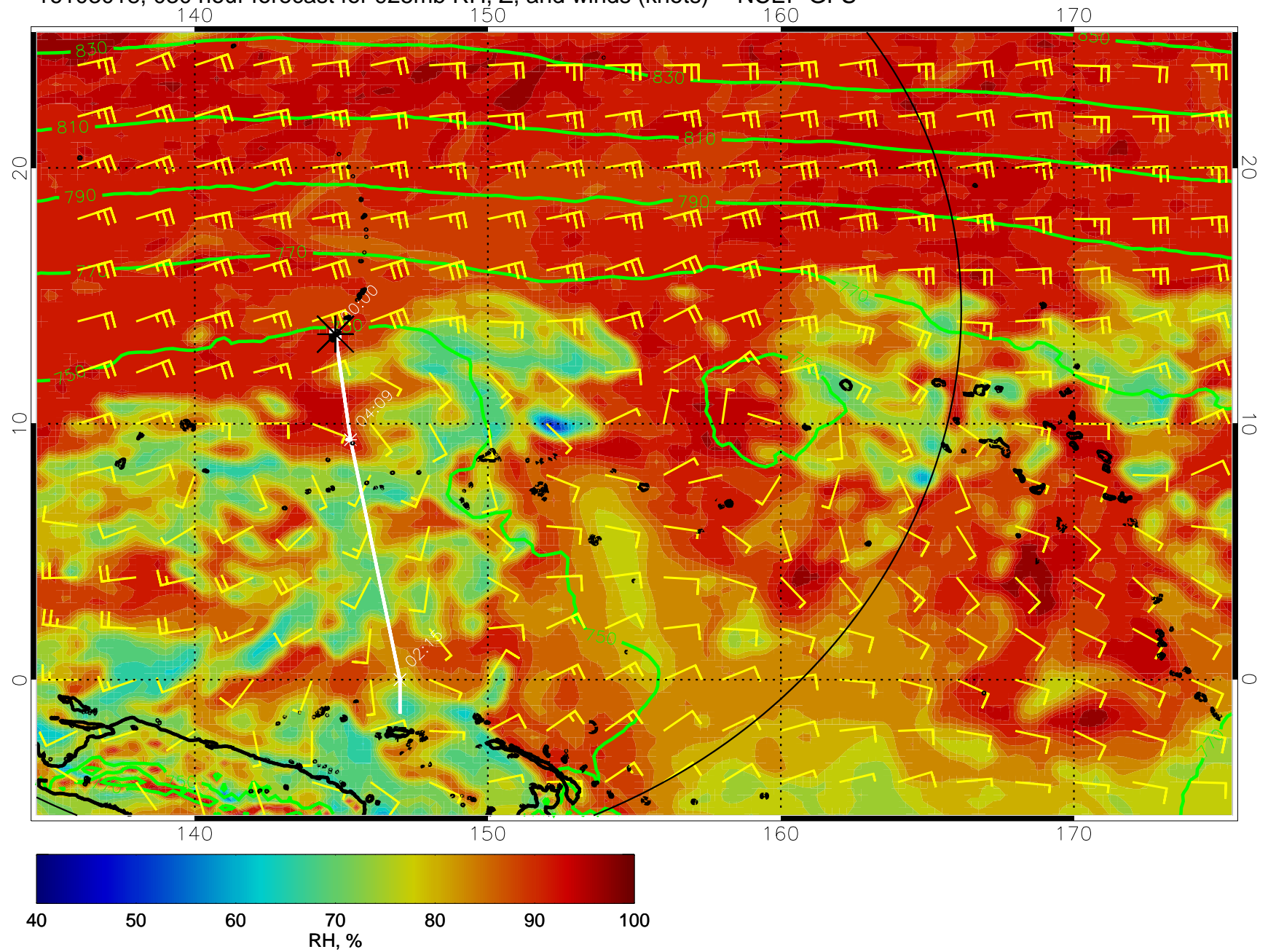
16103018, 030 hour forecast for 925mb RH, Z, and winds (knots) -- NCEP GFS
