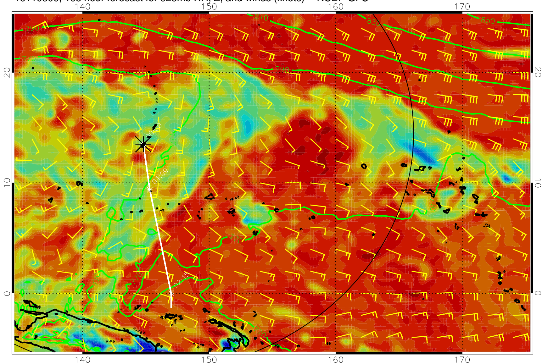
16110300, 108 hour forecast for 925mb RH, Z, and winds (knots) -- NCEP GFS
