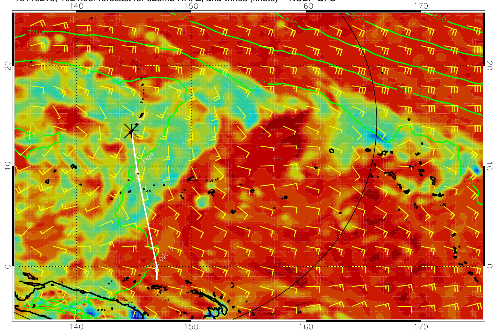
16110218, 102 hour forecast for 925mb RH, Z, and winds (knots) -- NCEP GFS
