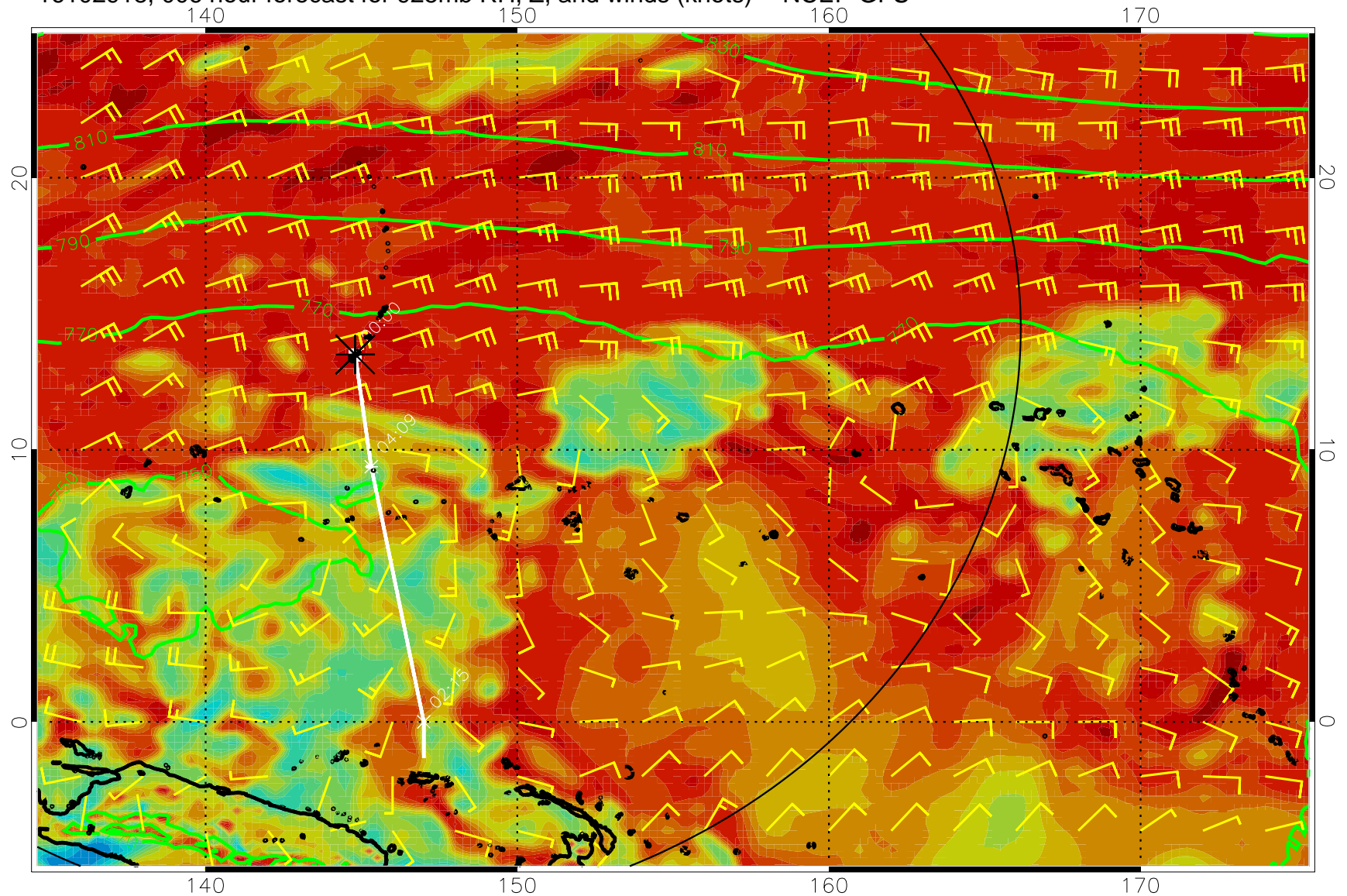
16102918, 006 hour forecast for 925mb RH, Z, and winds (knots) -- NCEP GFS
