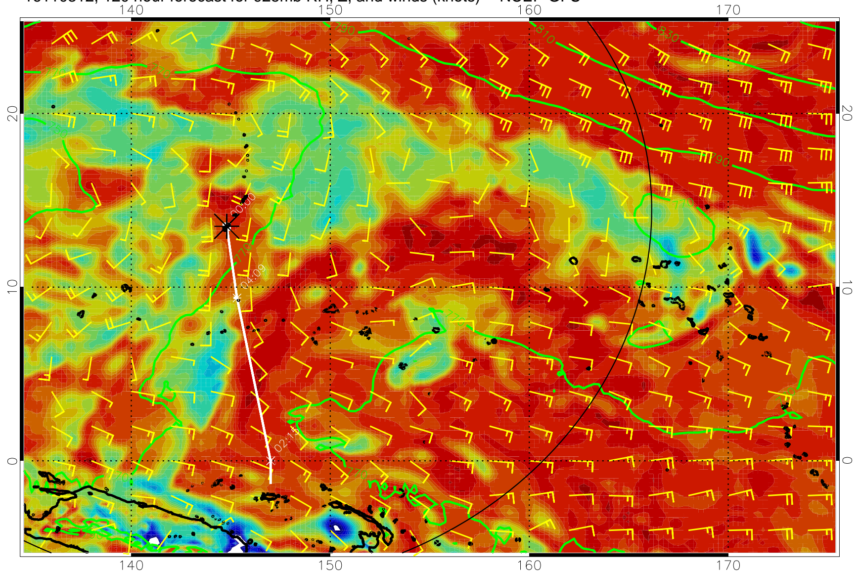
16110312, 120 hour forecast for 925mb RH, Z, and winds (knots) -- NCEP GFS
