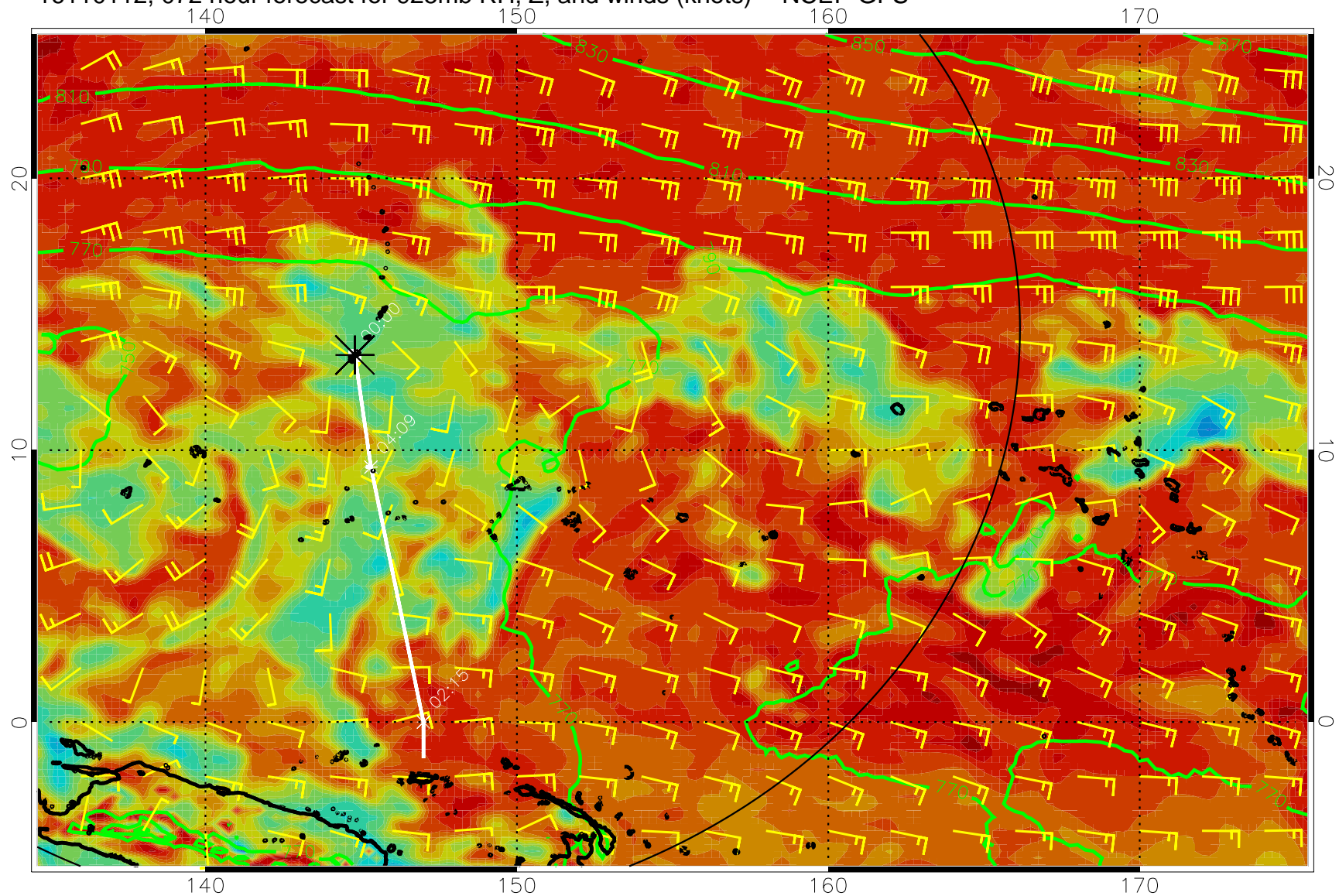
16110112, 072 hour forecast for 925mb RH, Z, and winds (knots) -- NCEP GFS
