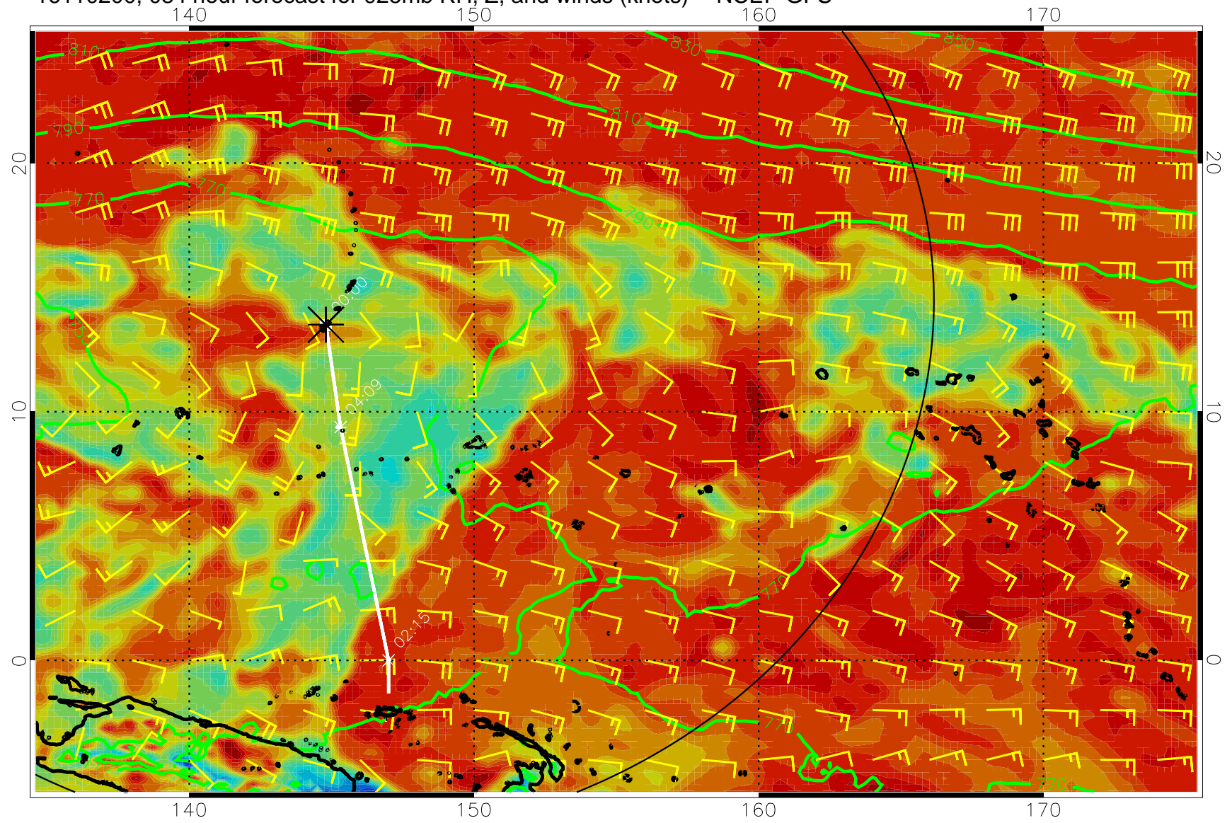
16110200, 084 hour forecast for 925mb RH, Z, and winds (knots) -- NCEP GFS
