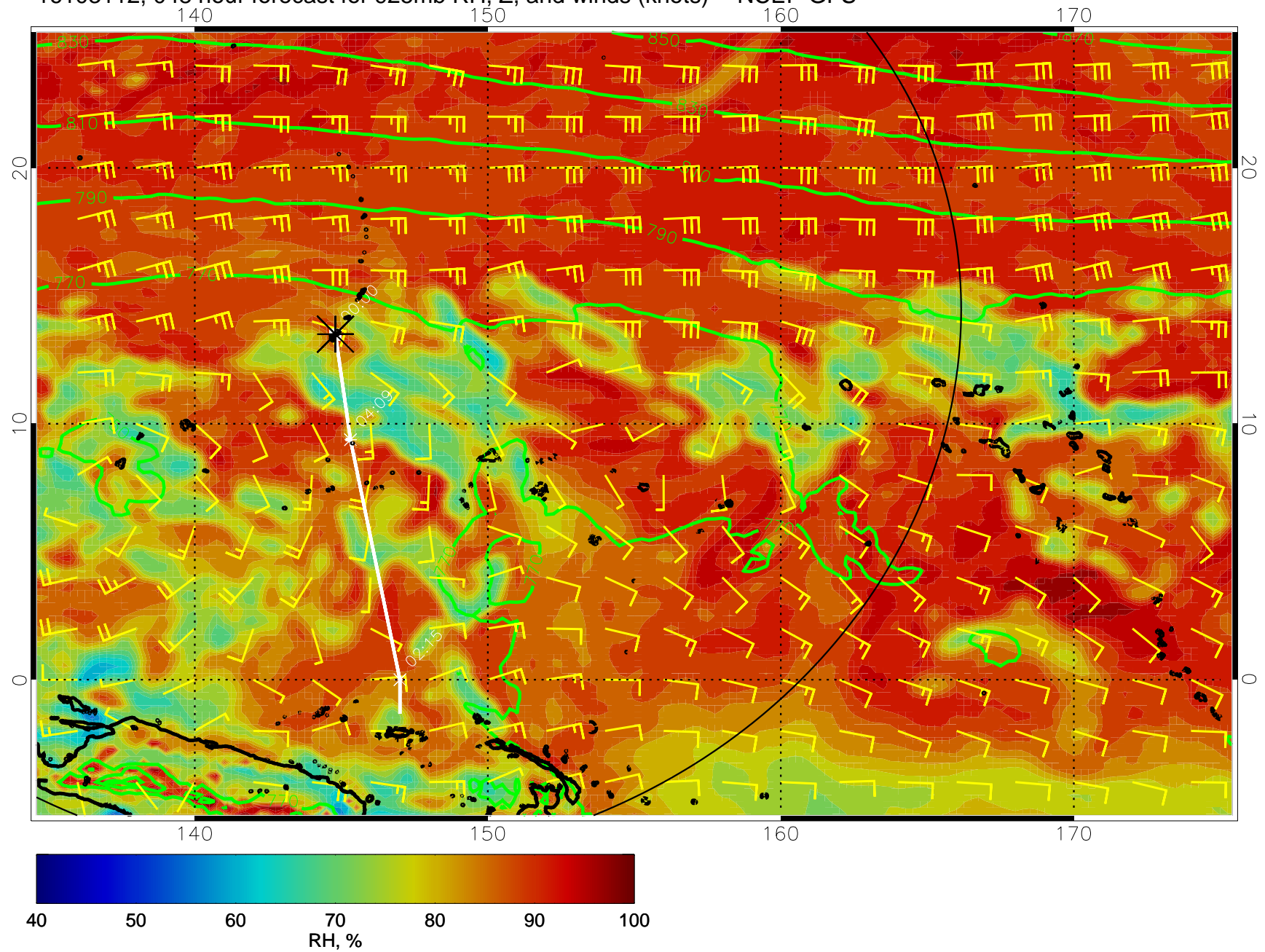
16103112, 048 hour forecast for 925mb RH, Z, and winds (knots) -- NCEP GFS
