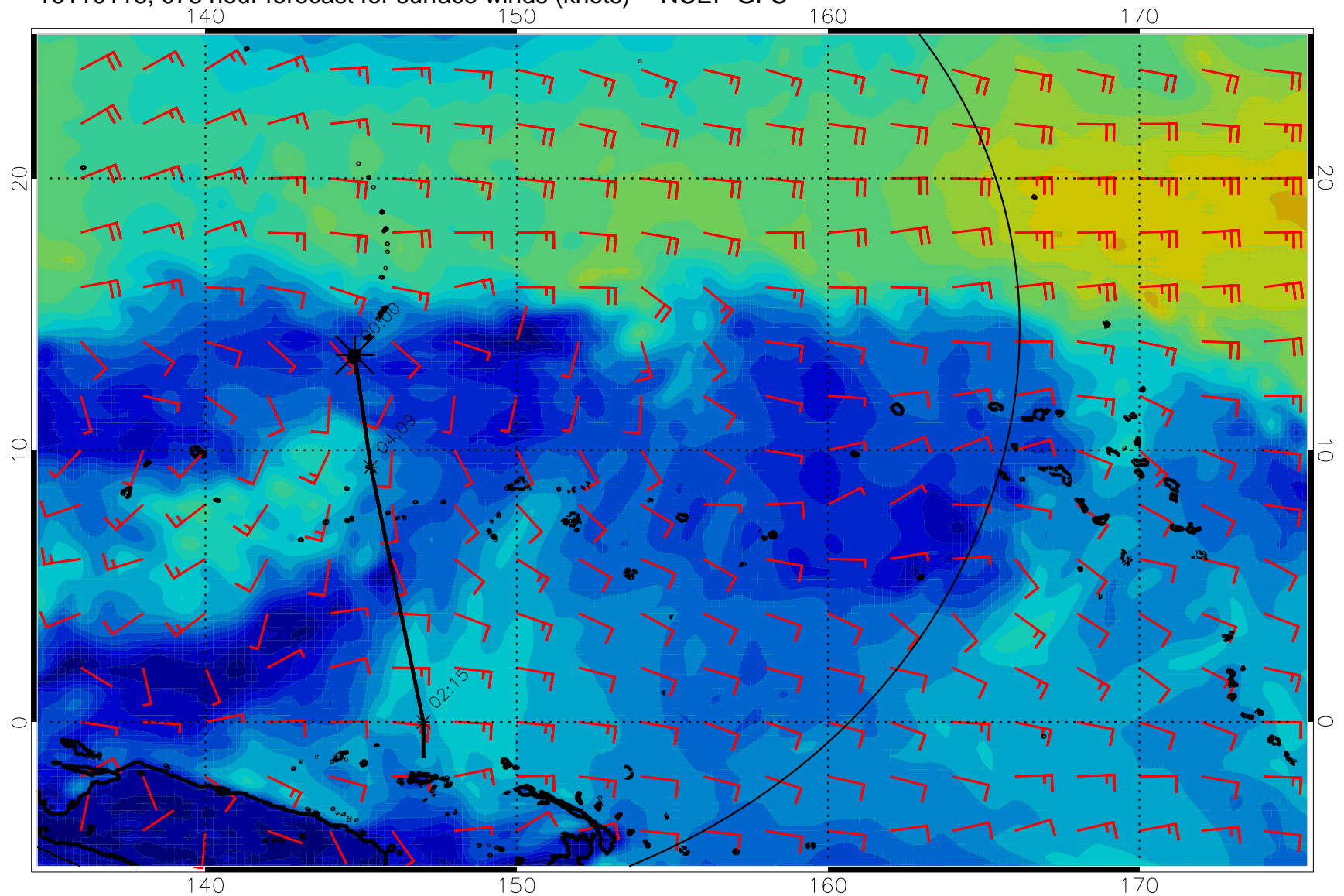
16110118, 078 hour forecast for surface winds (knots) -- NCEP GFS
