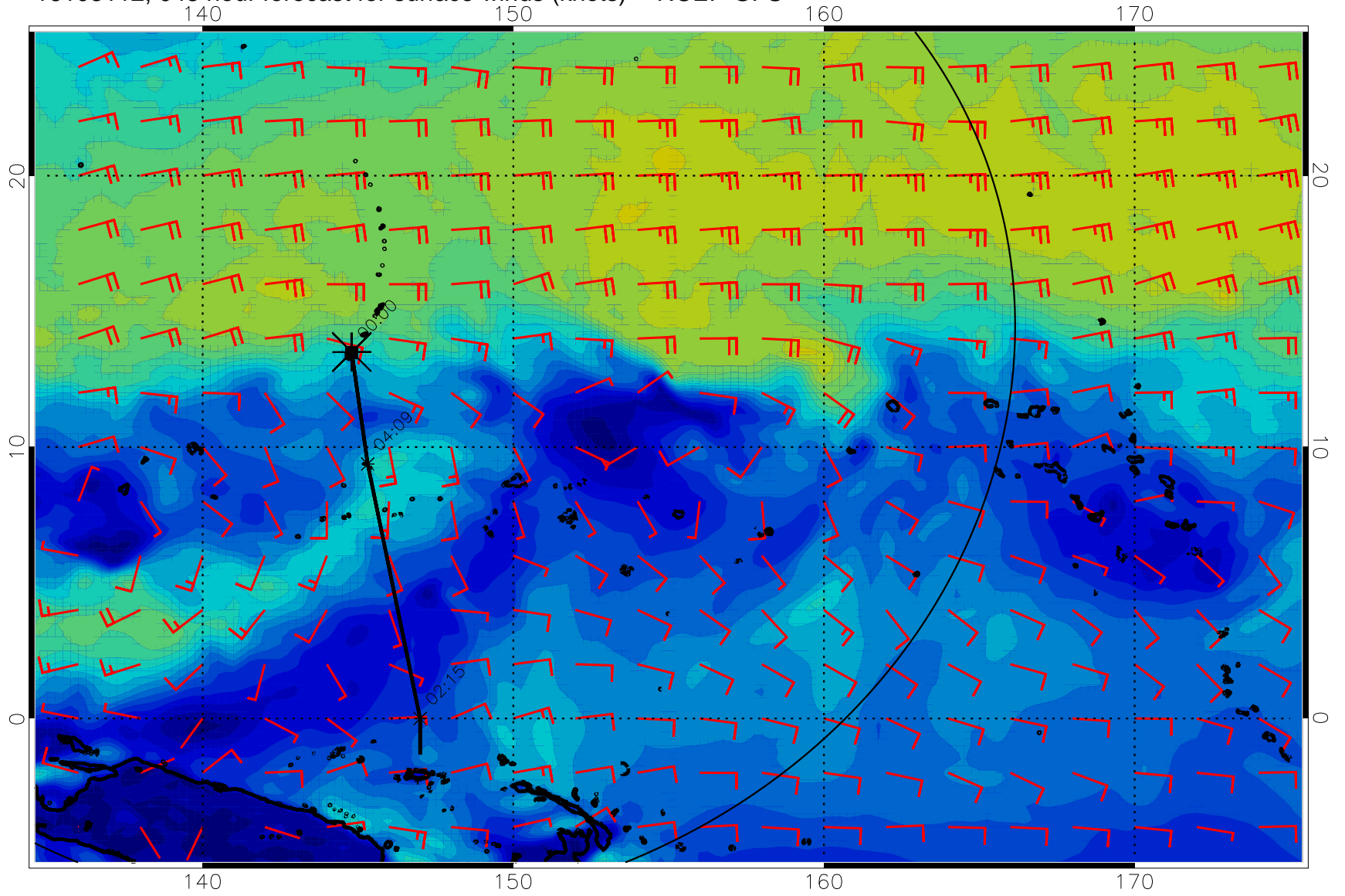
16103112, 048 hour forecast for surface winds (knots) -- NCEP GFS
