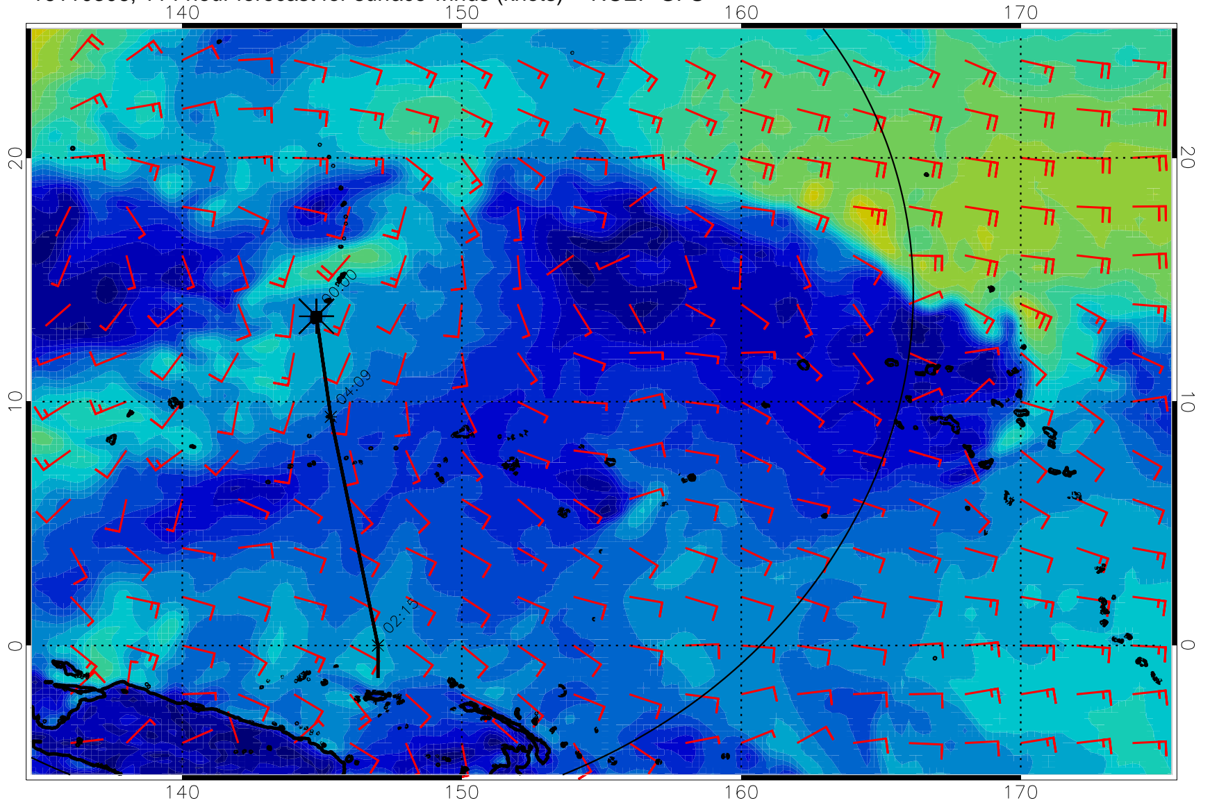
16110306, 114 hour forecast for surface winds (knots) -- NCEP GFS
