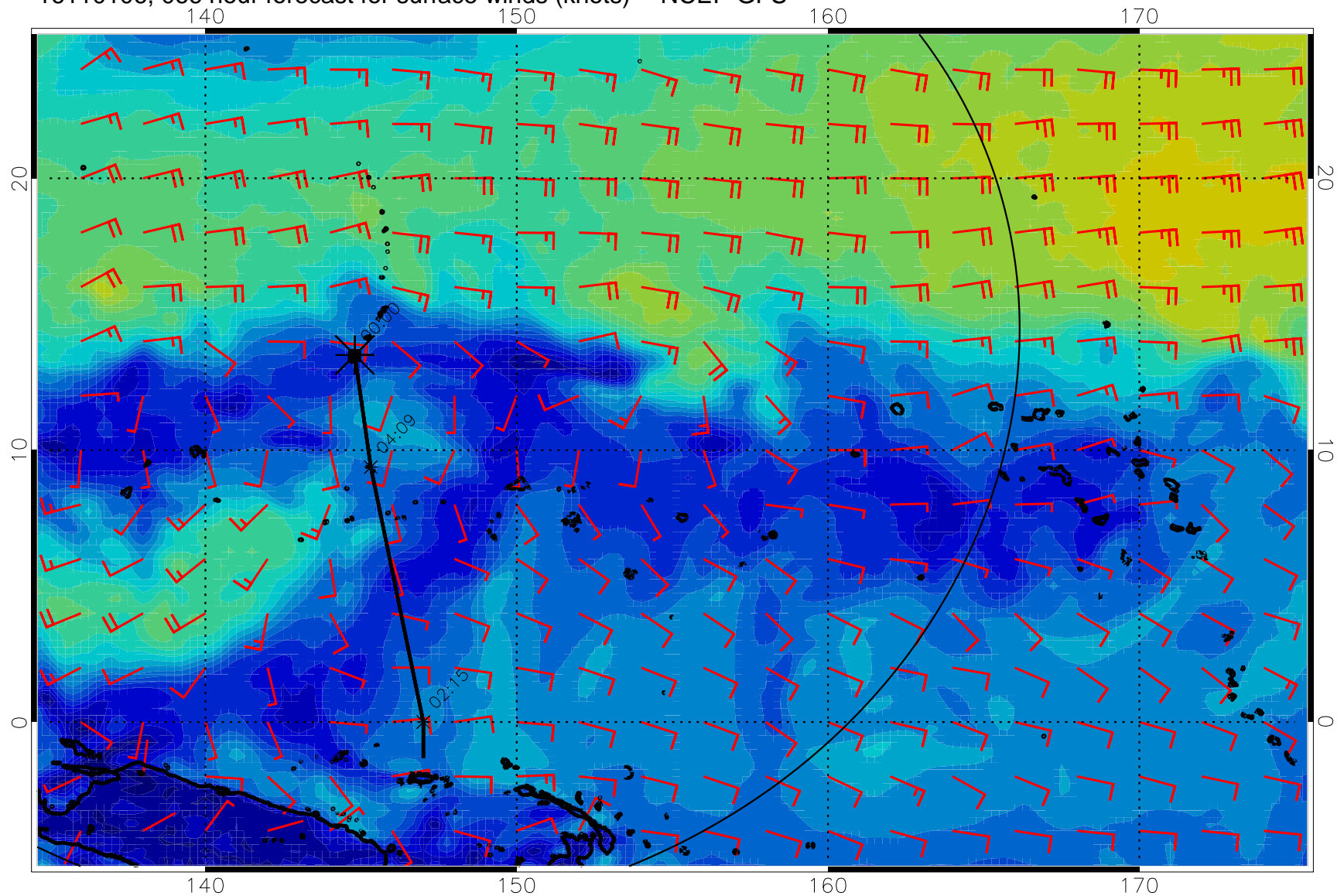
16110106, 066 hour forecast for surface winds (knots) -- NCEP GFS
