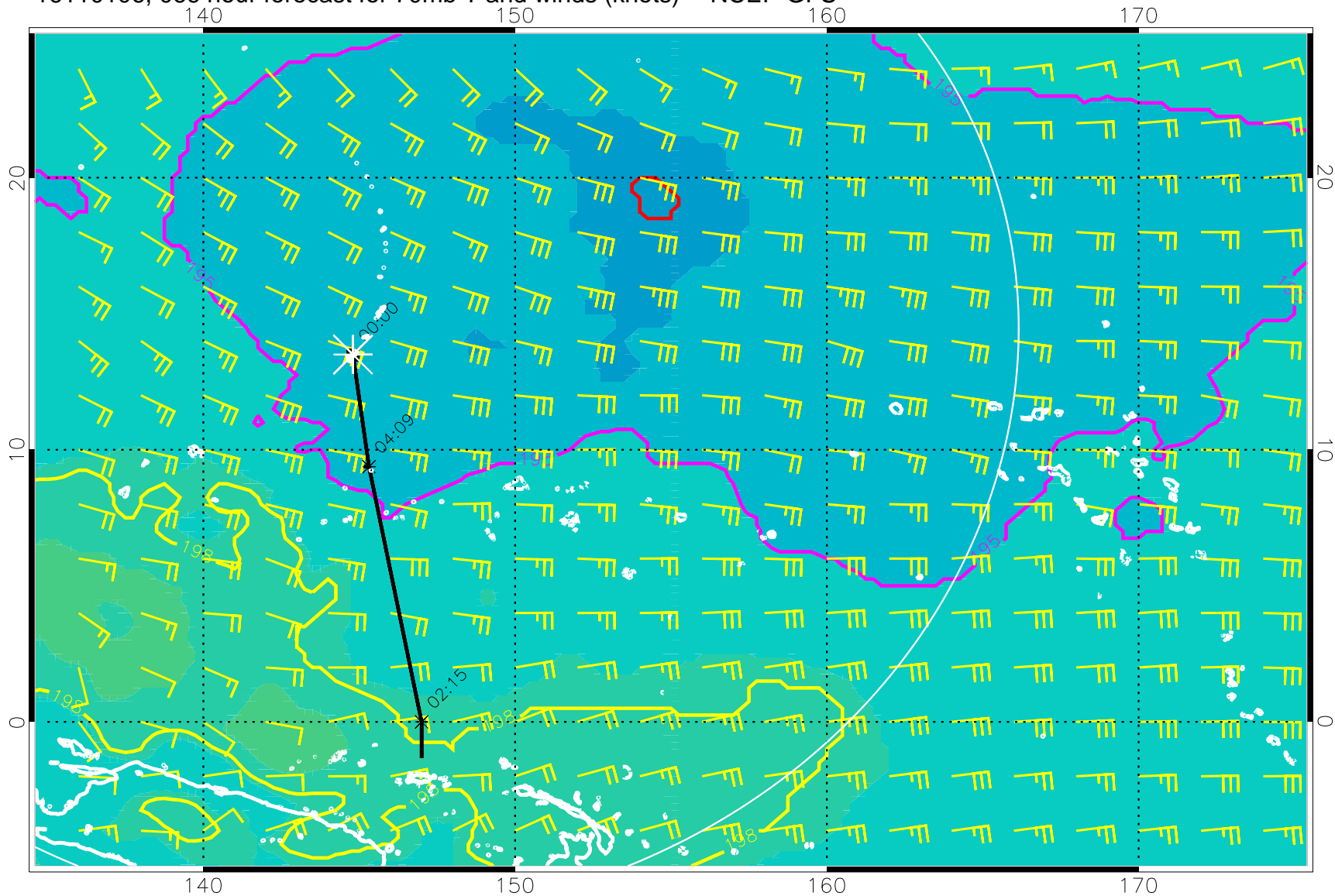
16110106, 066 hour forecast for 70mb T and winds (knots) -- NCEP GFS
