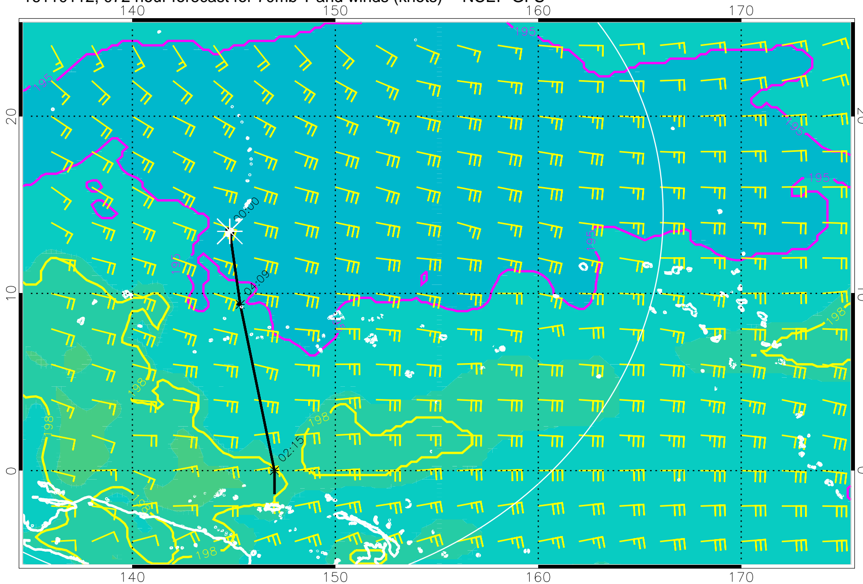
16110112, 072 hour forecast for 70mb T and winds (knots) -- NCEP GFS
