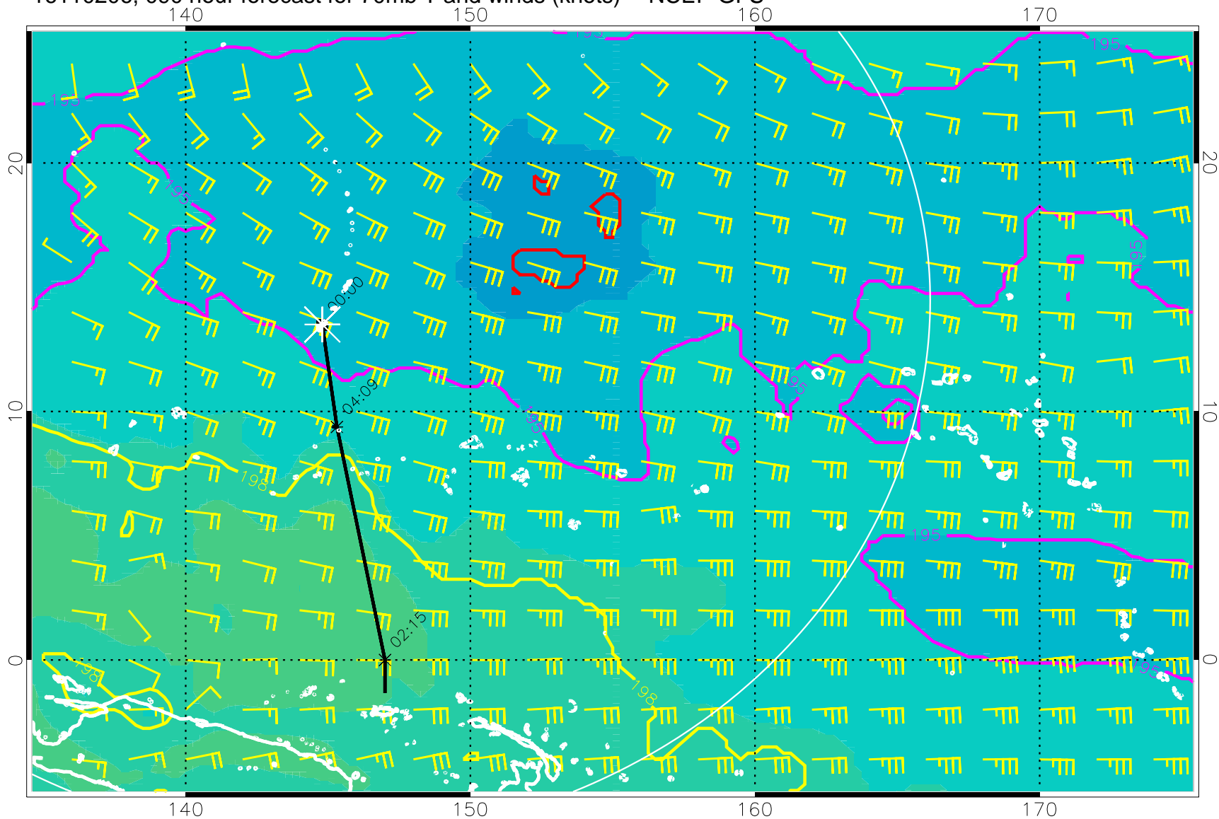
16110206, 090 hour forecast for 70mb T and winds (knots) -- NCEP GFS
