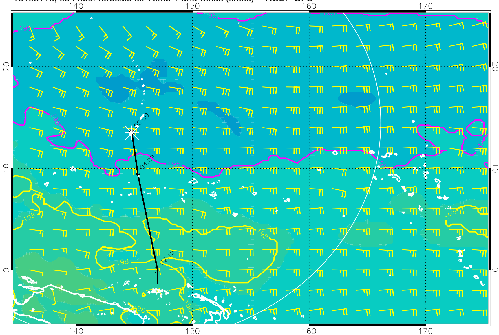
16103118, 054 hour forecast for 70mb T and winds (knots) -- NCEP GFS
