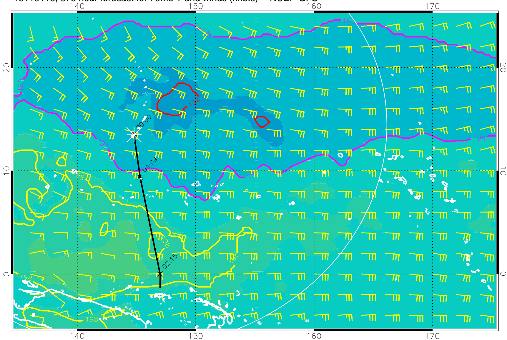
16110118, 078 hour forecast for 70mb T and winds (knots) -- NCEP GFS
