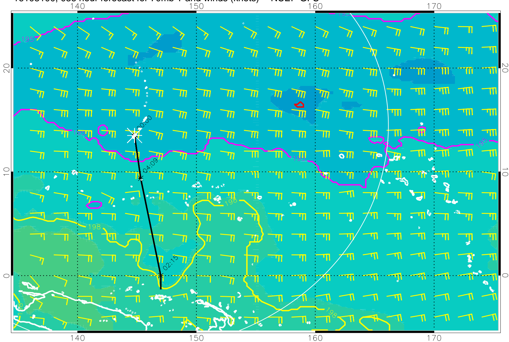
16103100, 036 hour forecast for 70mb T and winds (knots) -- NCEP GFS
