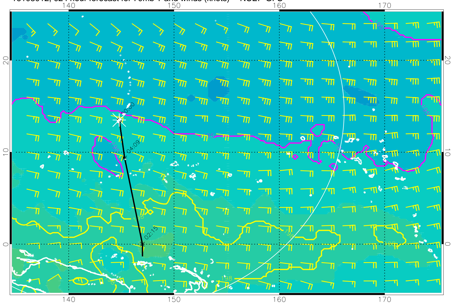
16103012, 024 hour forecast for 70mb T and winds (knots) -- NCEP GFS
