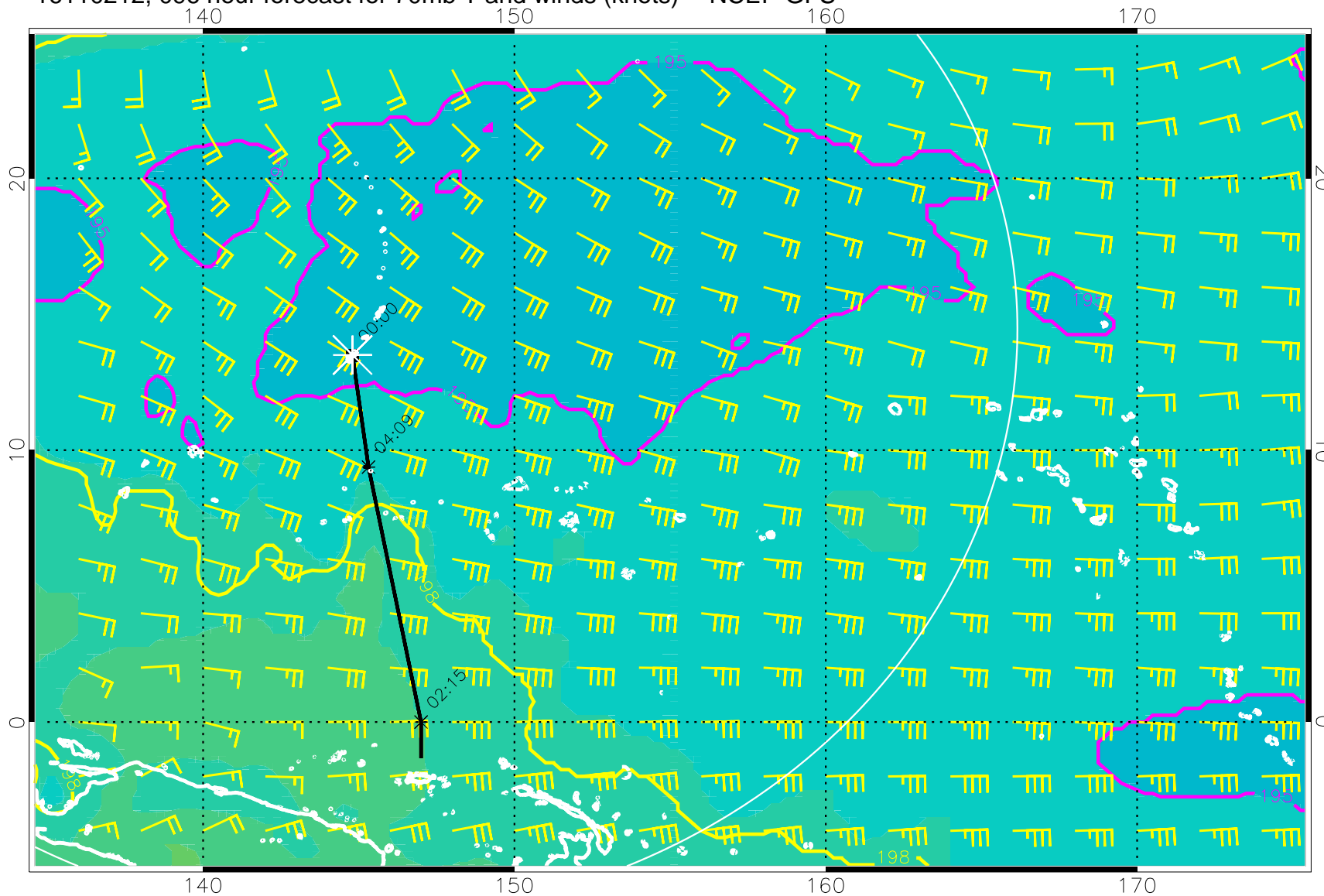
16110212, 096 hour forecast for 70mb T and winds (knots) -- NCEP GFS
