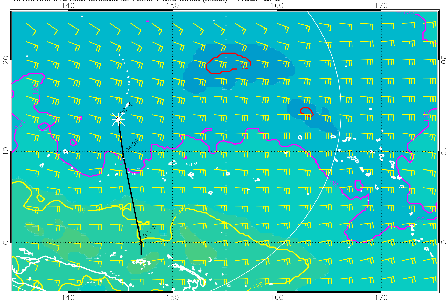
16103106, 042 hour forecast for 70mb T and winds (knots) -- NCEP GFS
