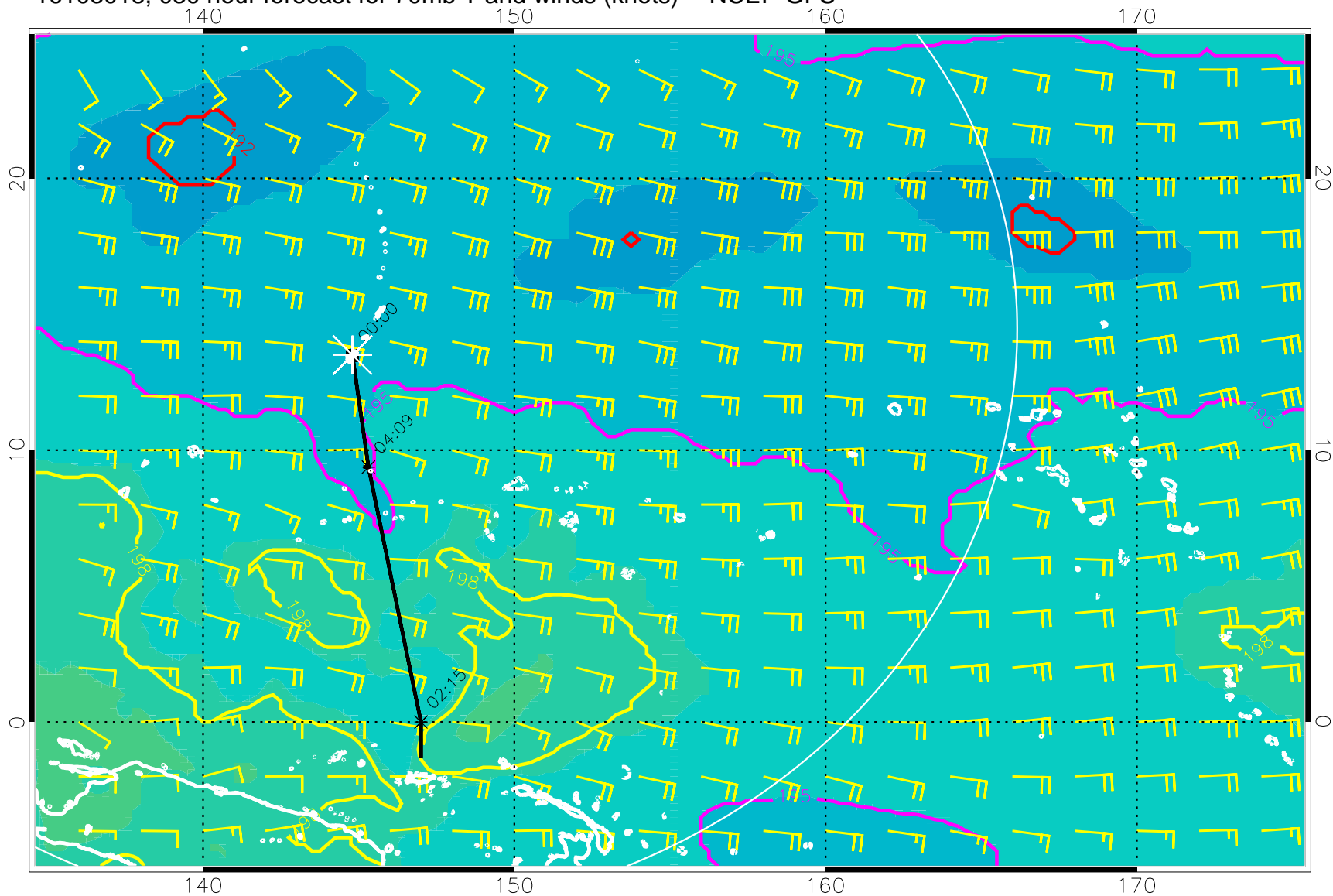
16103018, 030 hour forecast for 70mb T and winds (knots) -- NCEP GFS
