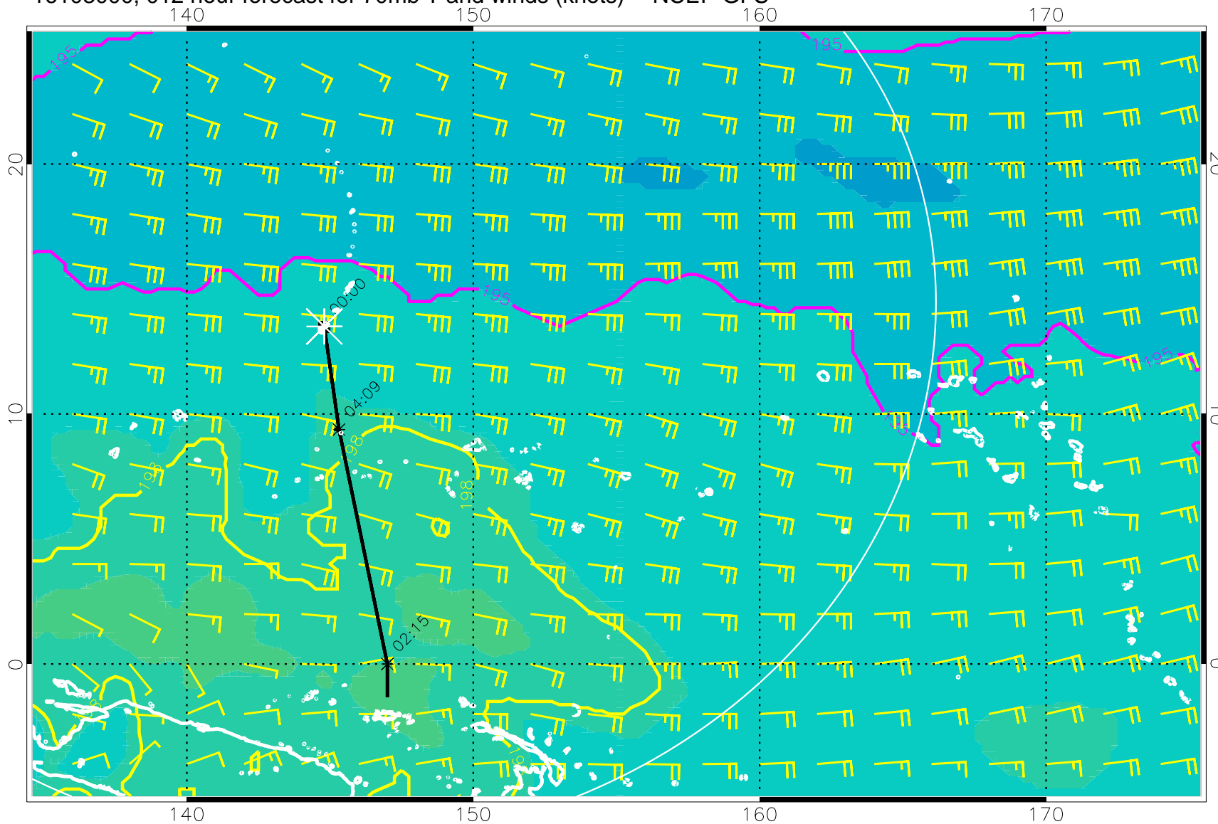
16103000, 012 hour forecast for 70mb T and winds (knots) -- NCEP GFS
