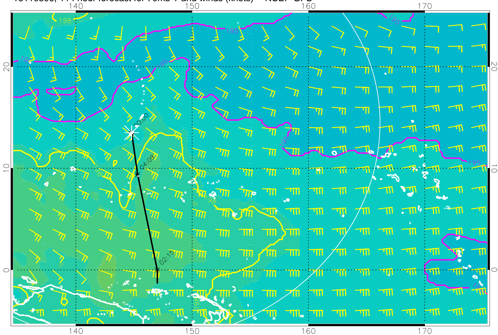
16110306, 114 hour forecast for 70mb T and winds (knots) -- NCEP GFS
