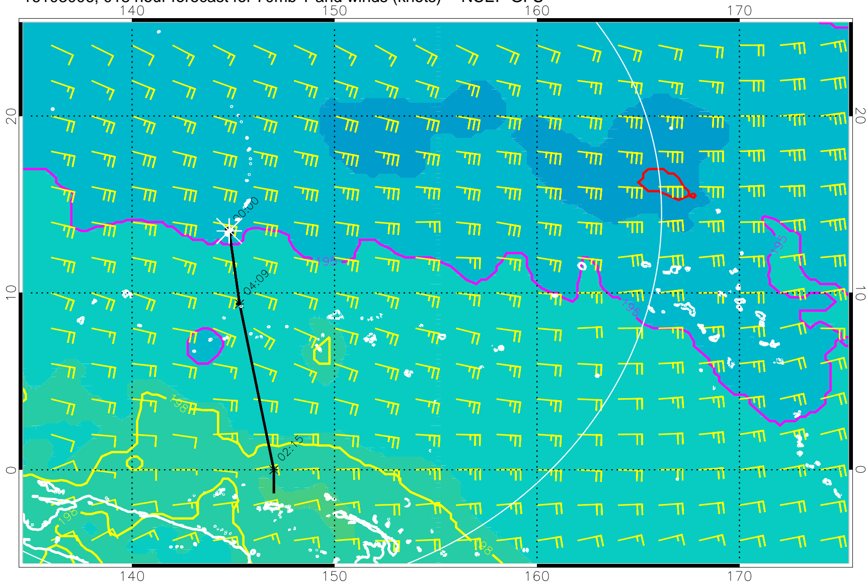
16103006, 018 hour forecast for 70mb T and winds (knots) -- NCEP GFS
