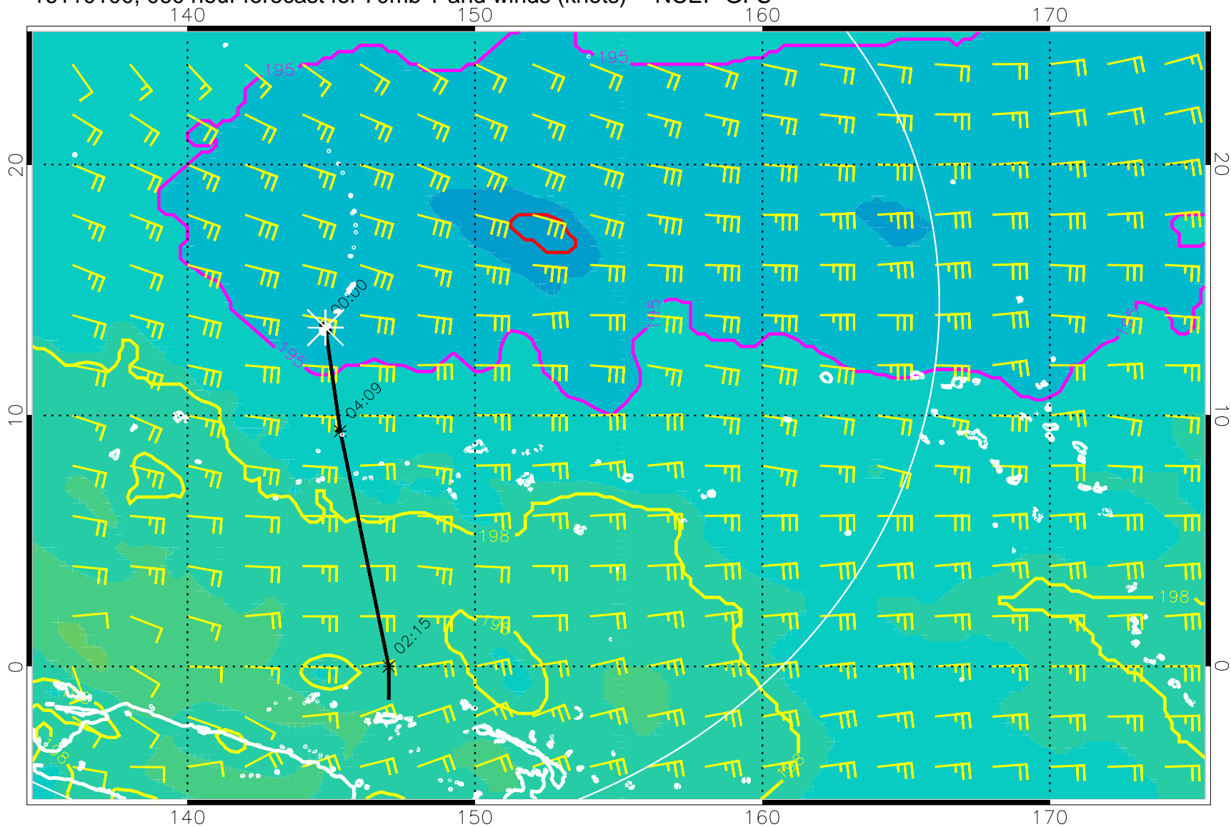
16110100, 060 hour forecast for 70mb T and winds (knots) -- NCEP GFS
