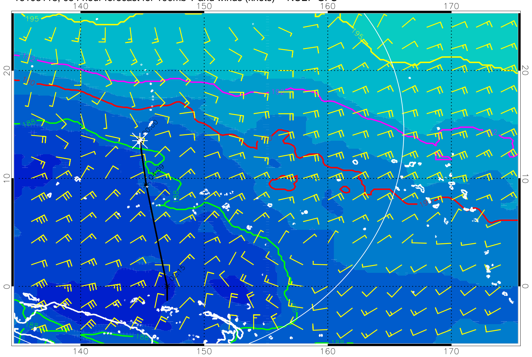
16103118, 054 hour forecast for 100mb T and winds (knots) -- NCEP GFS
