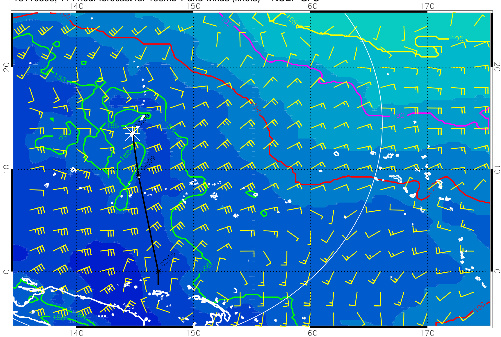
16110306, 114 hour forecast for 100mb T and winds (knots) -- NCEP GFS
