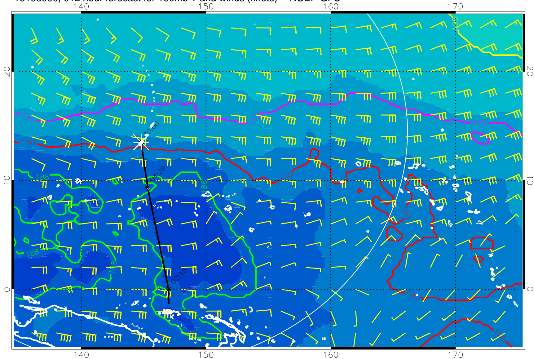
16103000, 012 hour forecast for 100mb T and winds (knots) -- NCEP GFS
