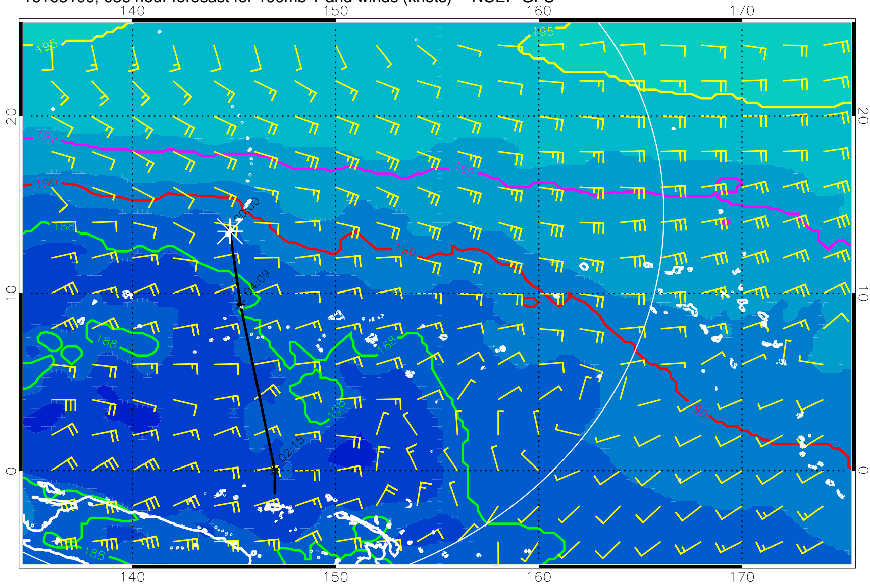
16103100, 036 hour forecast for 100mb T and winds (knots) -- NCEP GFS
