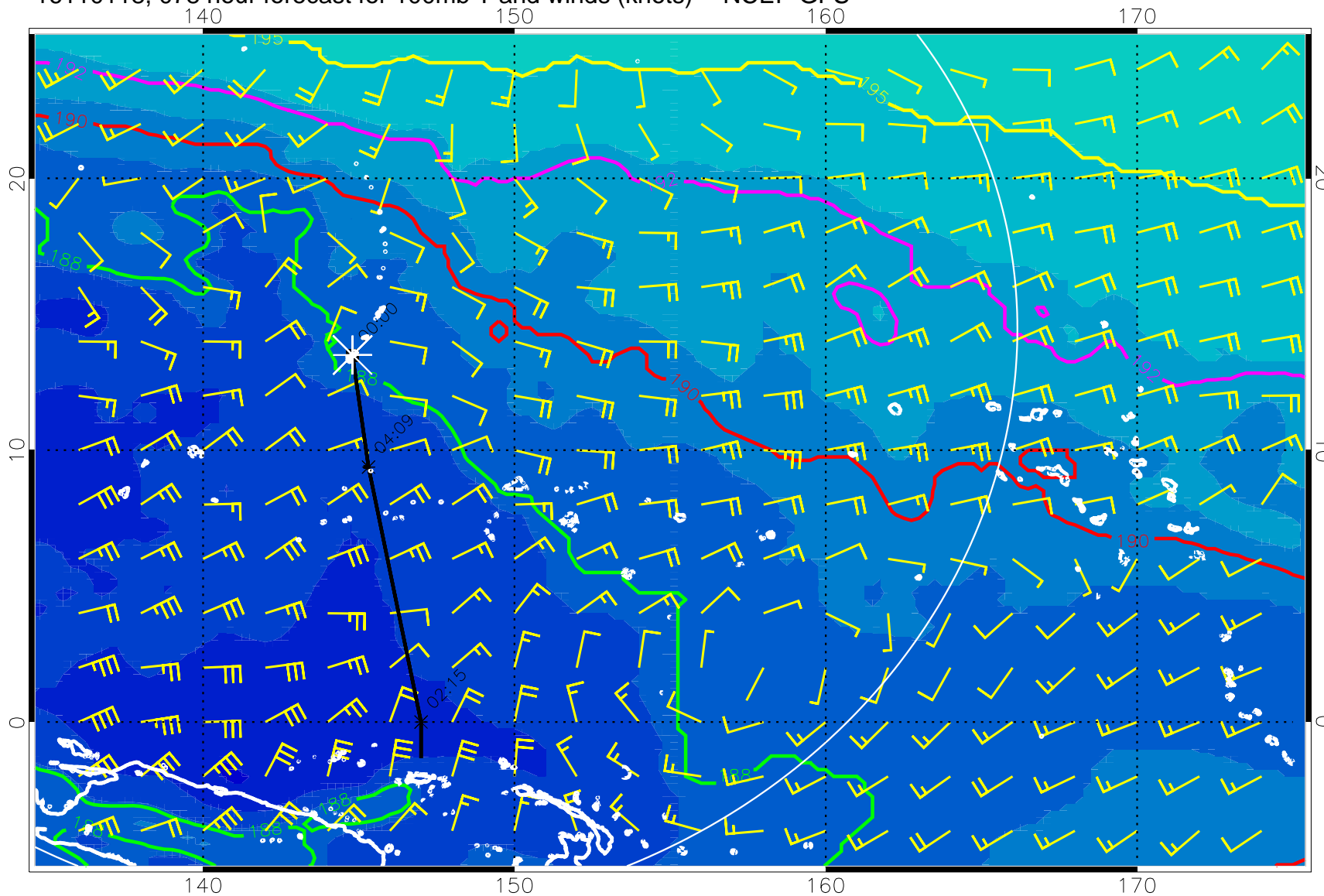
16110118, 078 hour forecast for 100mb T and winds (knots) -- NCEP GFS
