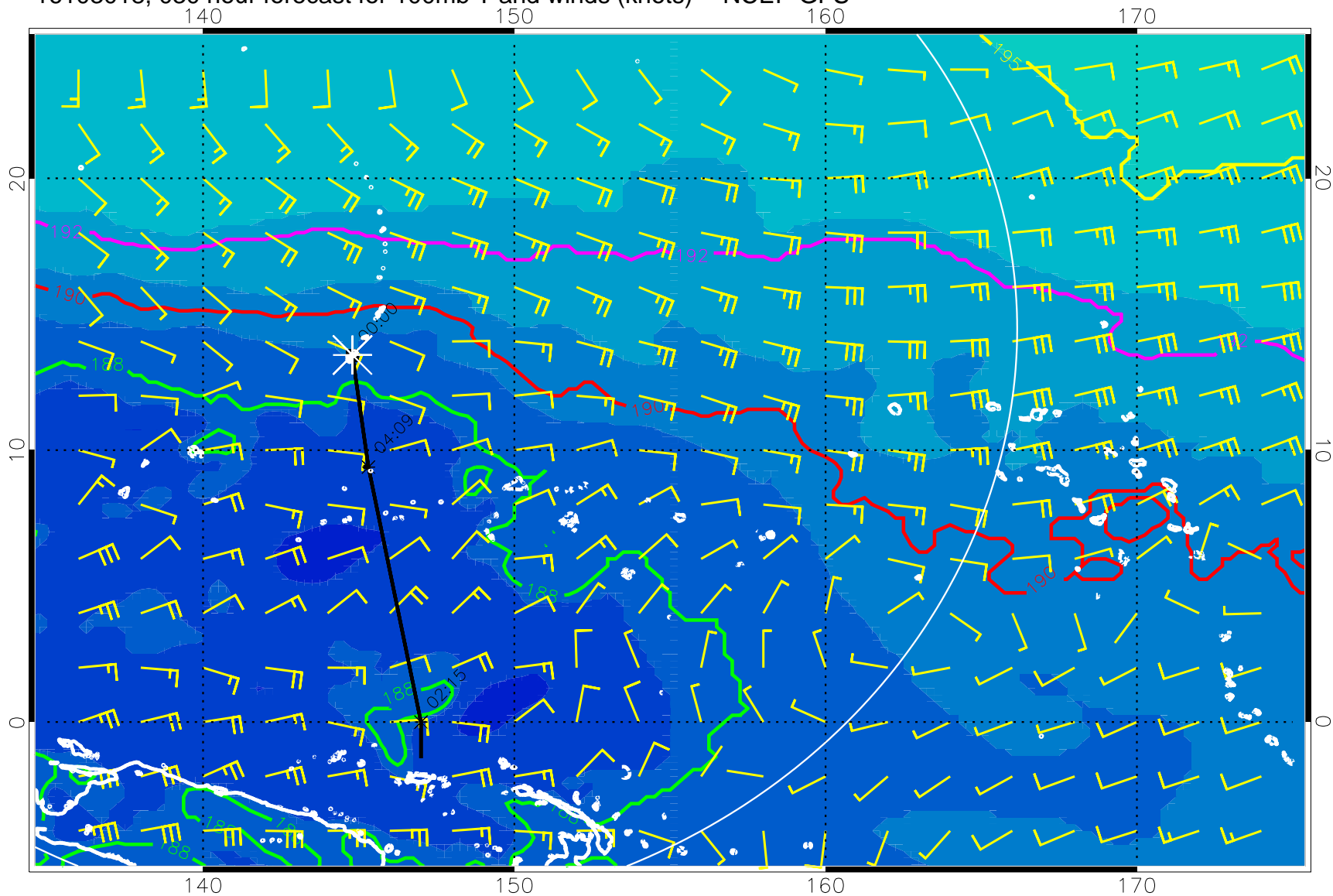
16103018, 030 hour forecast for 100mb T and winds (knots) -- NCEP GFS
