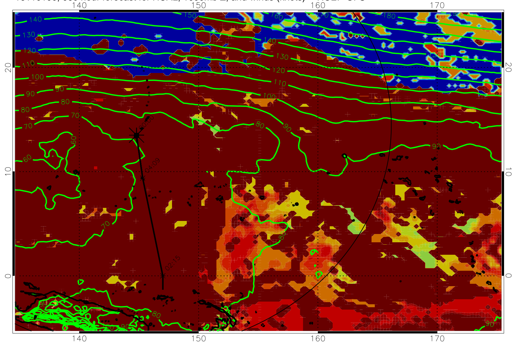
16110100, 060 hour forecast for HCAL, 1000mb Z, and winds (knots) -- NCEP GFS
