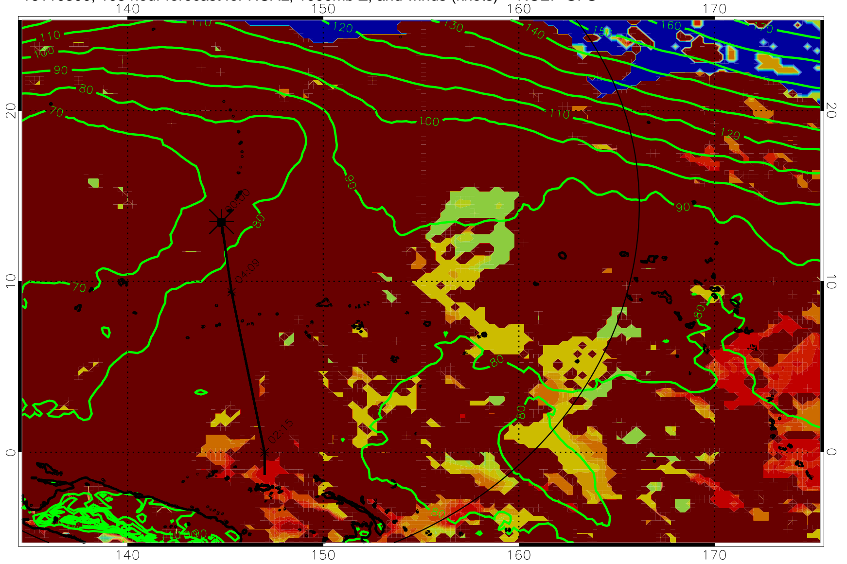
16110300, 108 hour forecast for HCAL, 1000mb Z, and winds (knots) -- NCEP GFS
