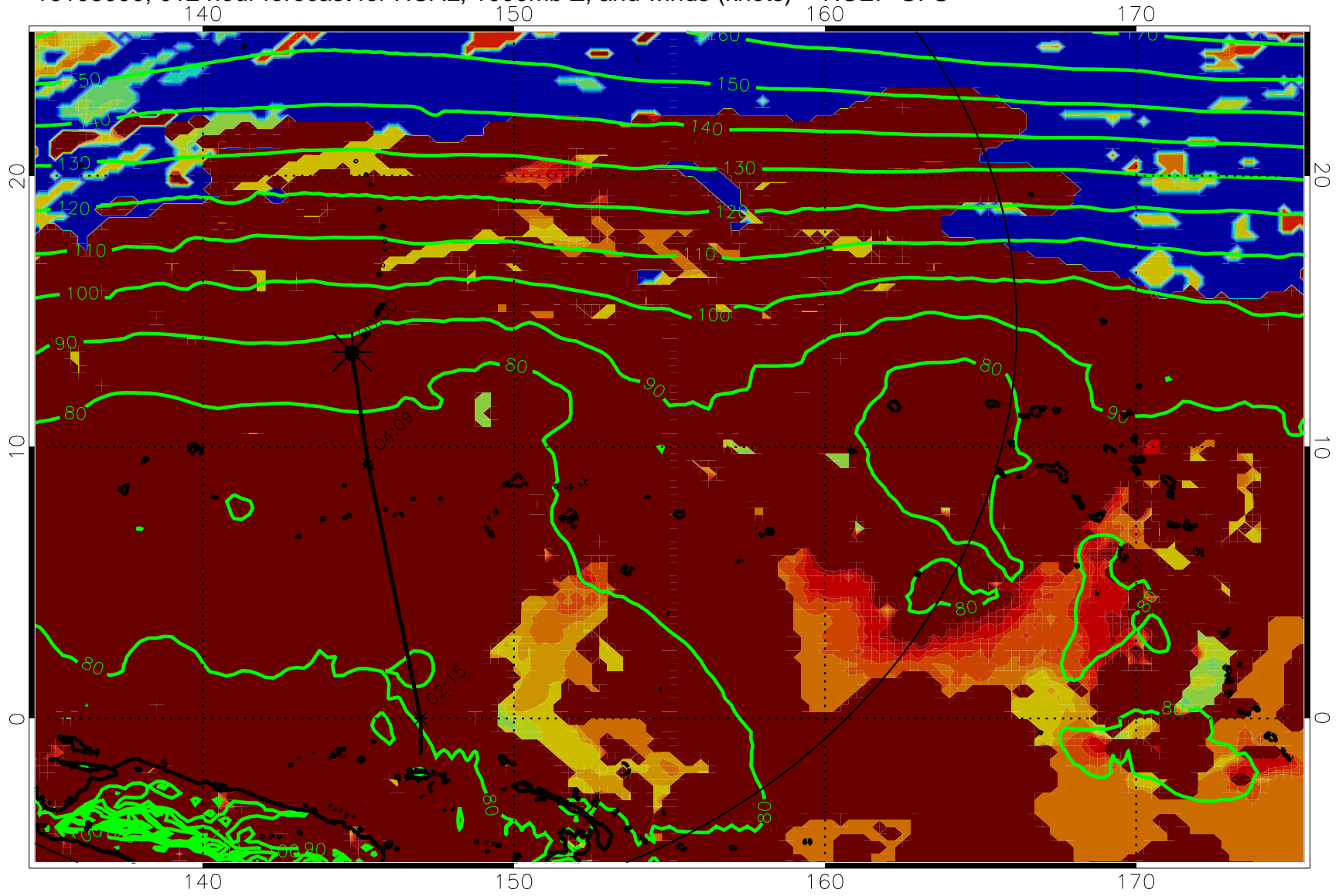
16103000, 012 hour forecast for HCAL, 1000mb Z, and winds (knots) -- NCEP GFS
