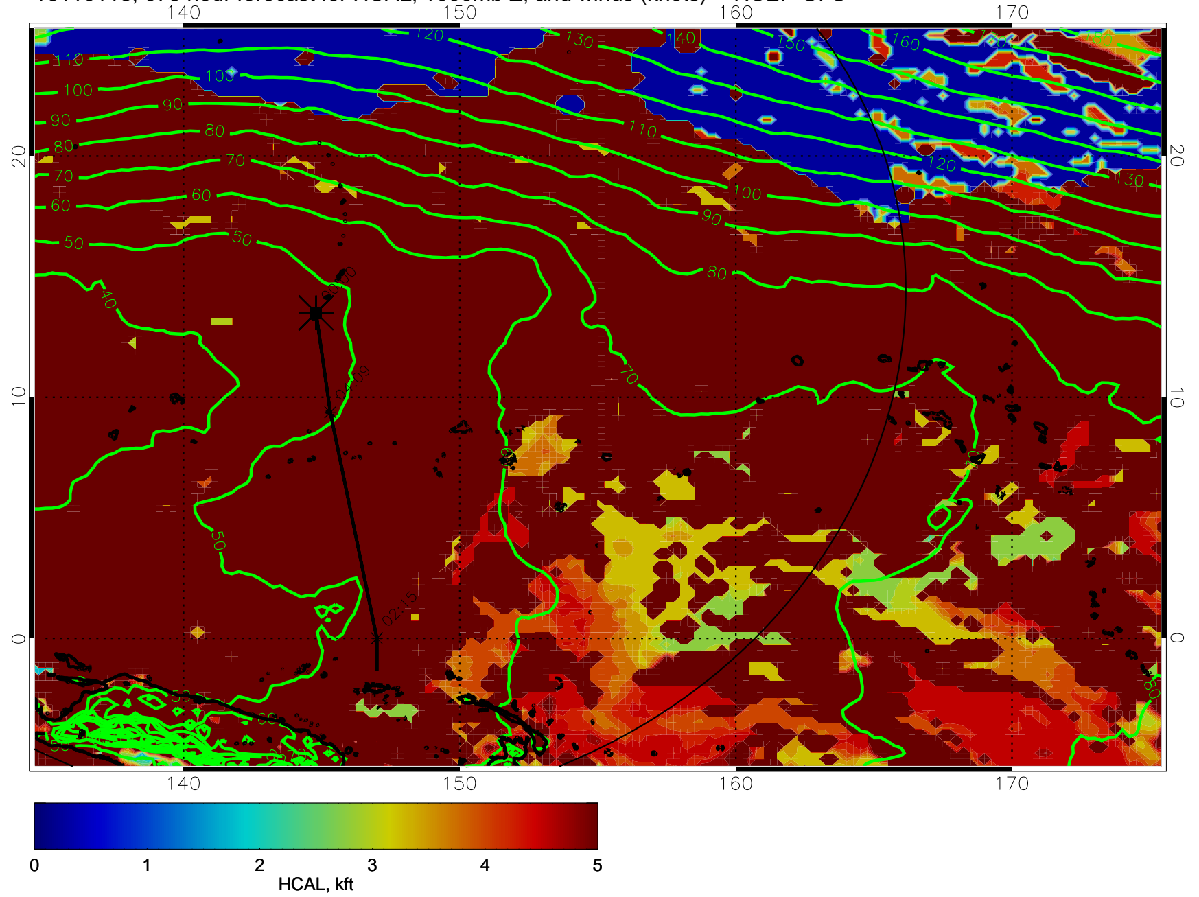
16110118, 078 hour forecast for HCAL, 1000mb Z, and winds (knots) -- NCEP GFS
