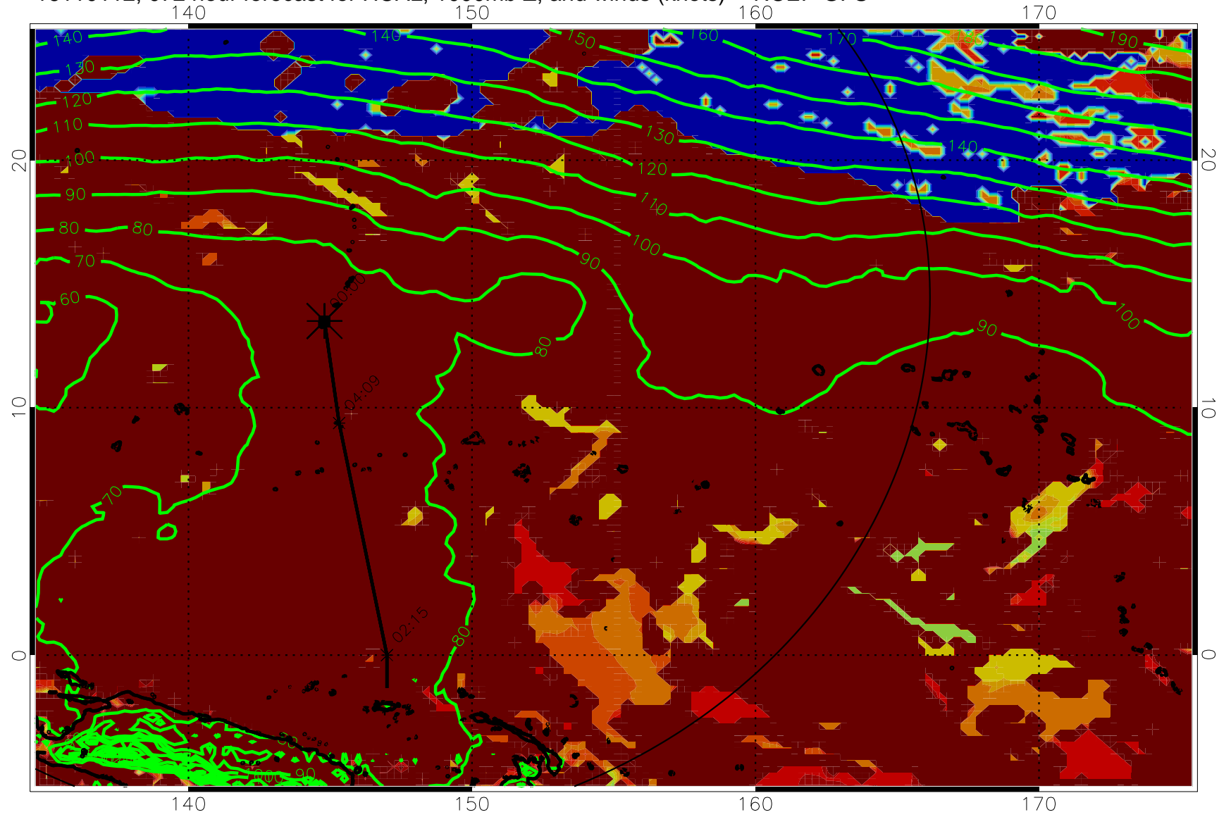
16110112, 072 hour forecast for HCAL, 1000mb Z, and winds (knots) -- NCEP GFS
