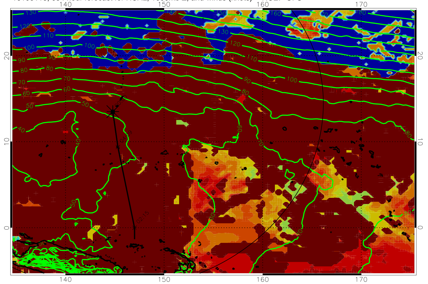
16103118, 054 hour forecast for HCAL, 1000mb Z, and winds (knots) -- NCEP GFS
