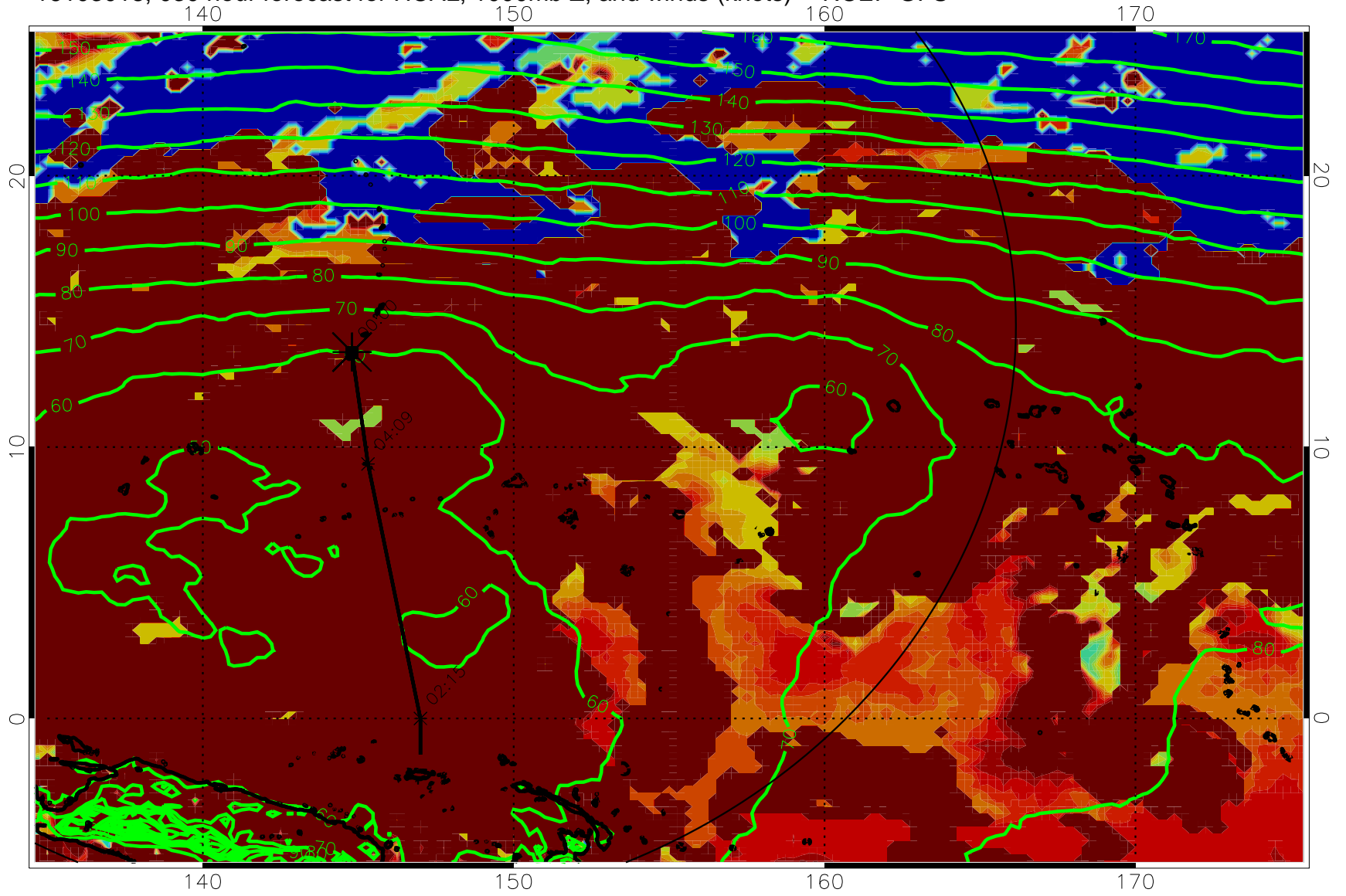
16103018, 030 hour forecast for HCAL, 1000mb Z, and winds (knots) -- NCEP GFS
