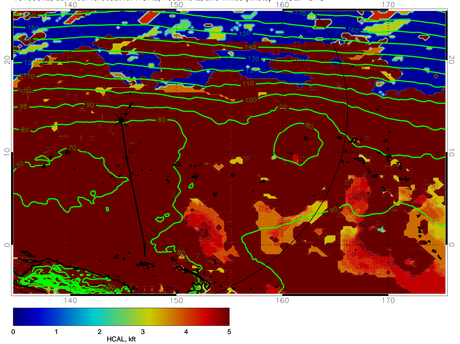
16103012, 024 hour forecast for HCAL, 1000mb Z, and winds (knots) -- NCEP GFS
