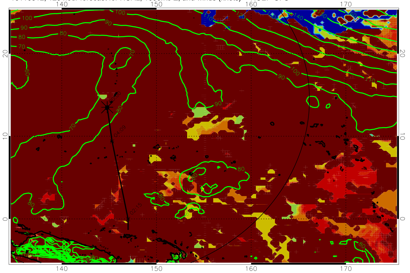
16110312, 120 hour forecast for HCAL, 1000mb Z, and winds (knots) -- NCEP GFS
