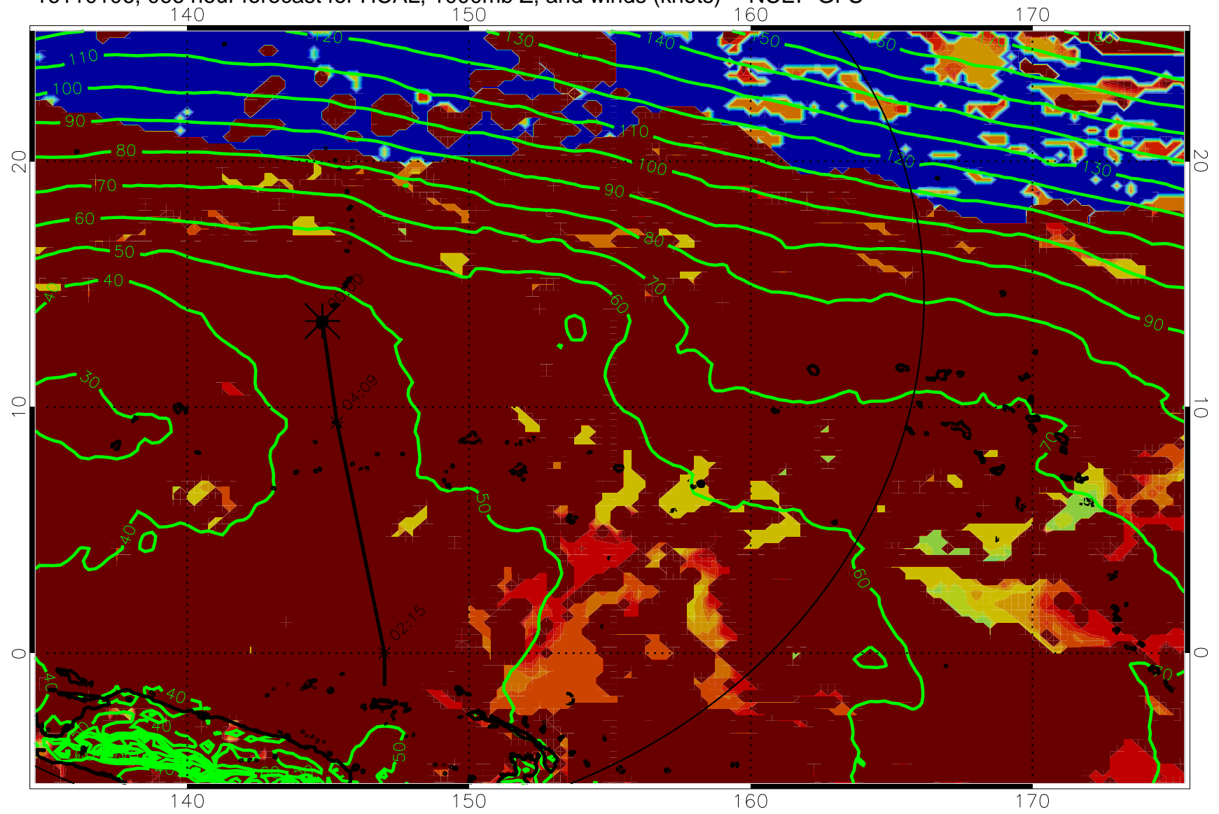
16110106, 066 hour forecast for HCAL, 1000mb Z, and winds (knots) -- NCEP GFS
