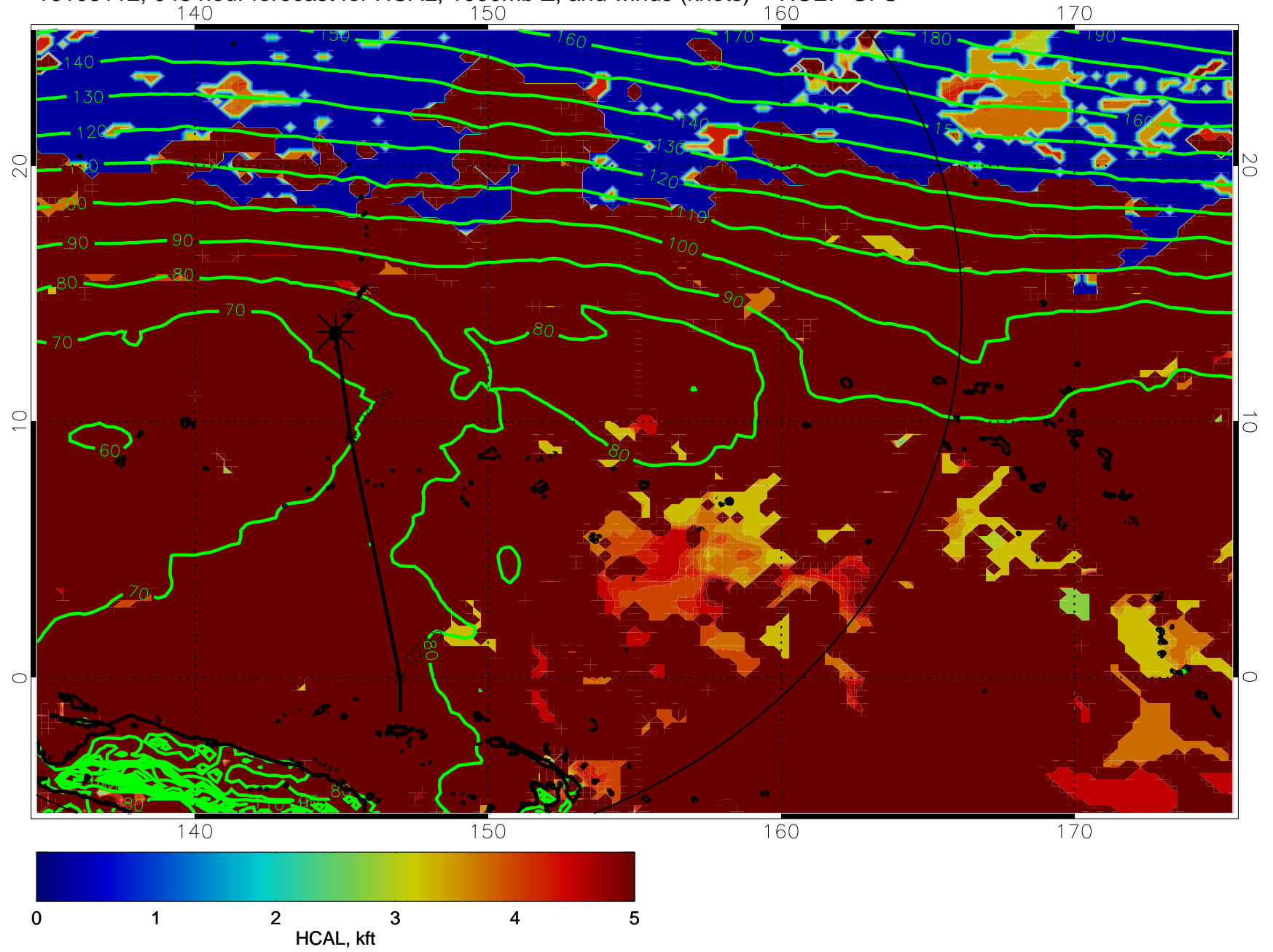
16103112, 048 hour forecast for HCAL, 1000mb Z, and winds (knots) -- NCEP GFS
