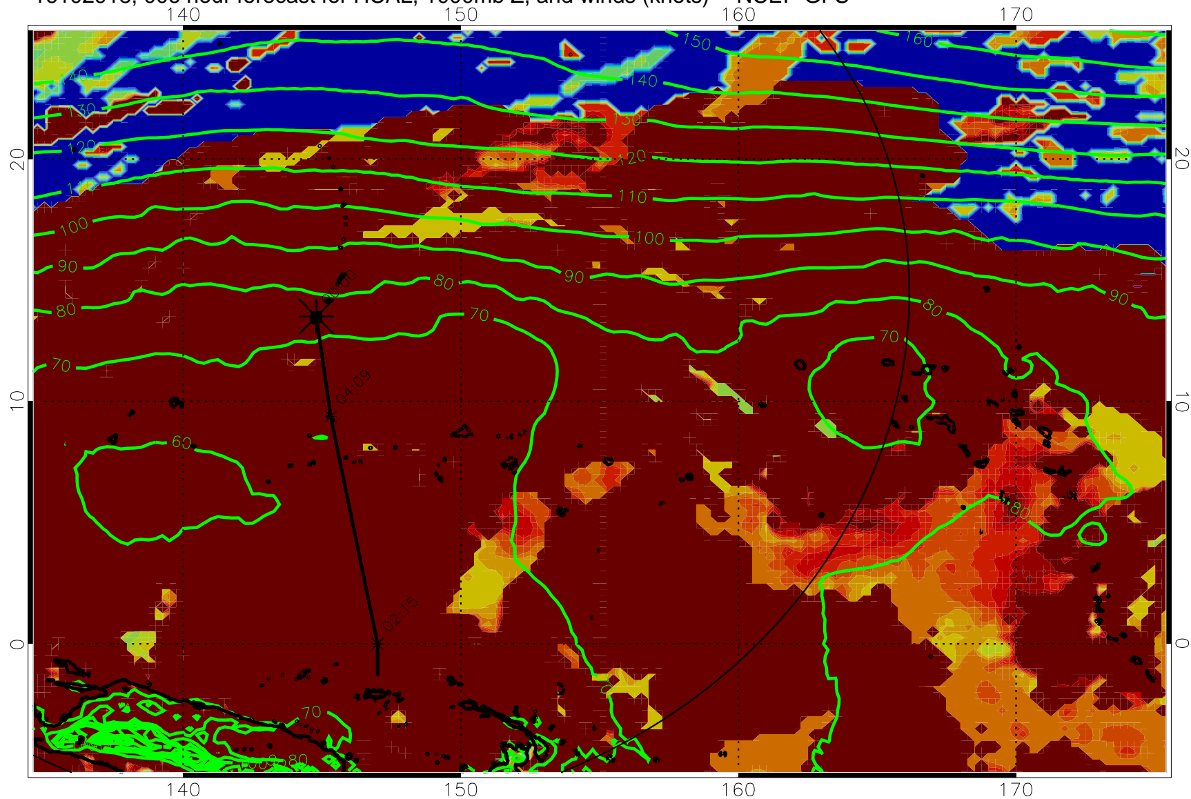
16102918, 006 hour forecast for HCAL, 1000mb Z, and winds (knots) -- NCEP GFS
