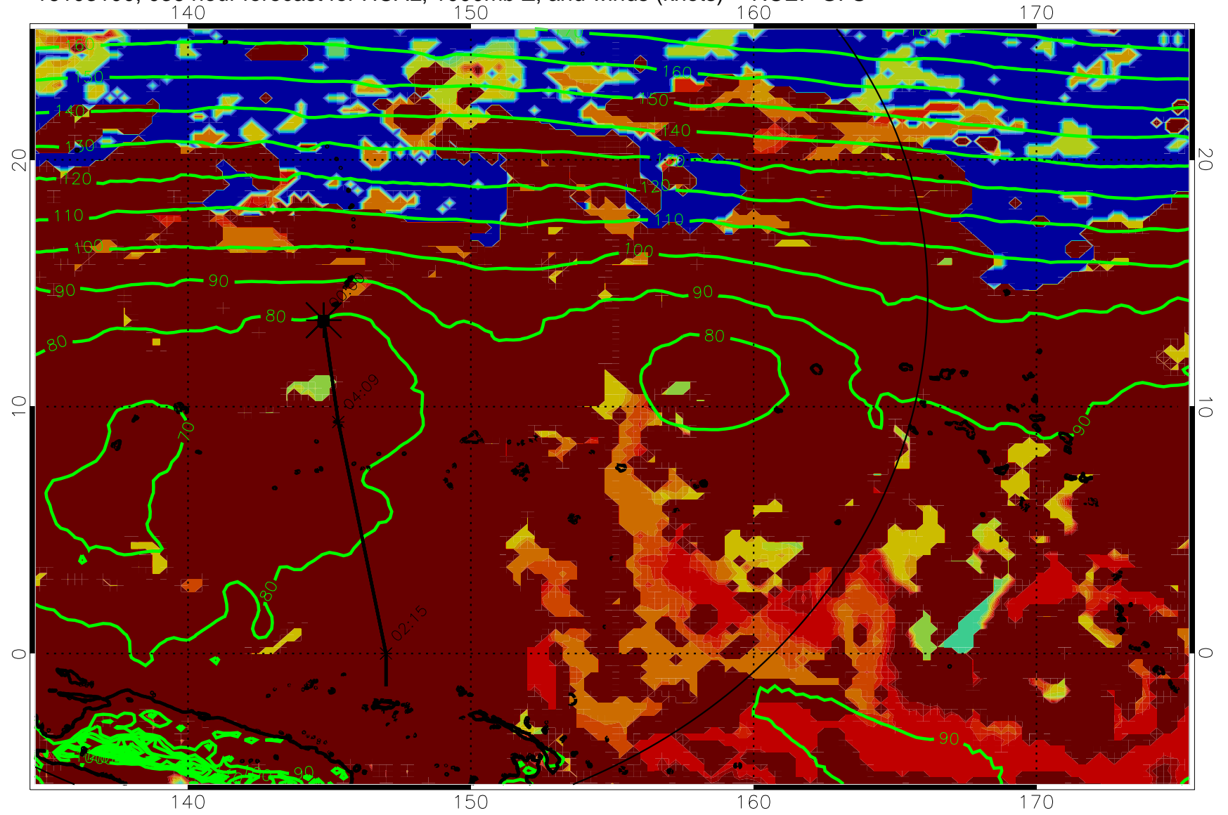
16103100, 036 hour forecast for HCAL, 1000mb Z, and winds (knots) -- NCEP GFS
