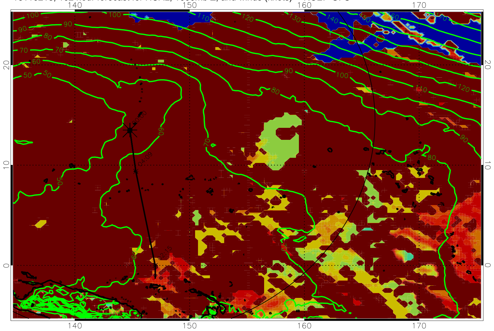
16110218, 102 hour forecast for HCAL, 1000mb Z, and winds (knots) -- NCEP GFS
