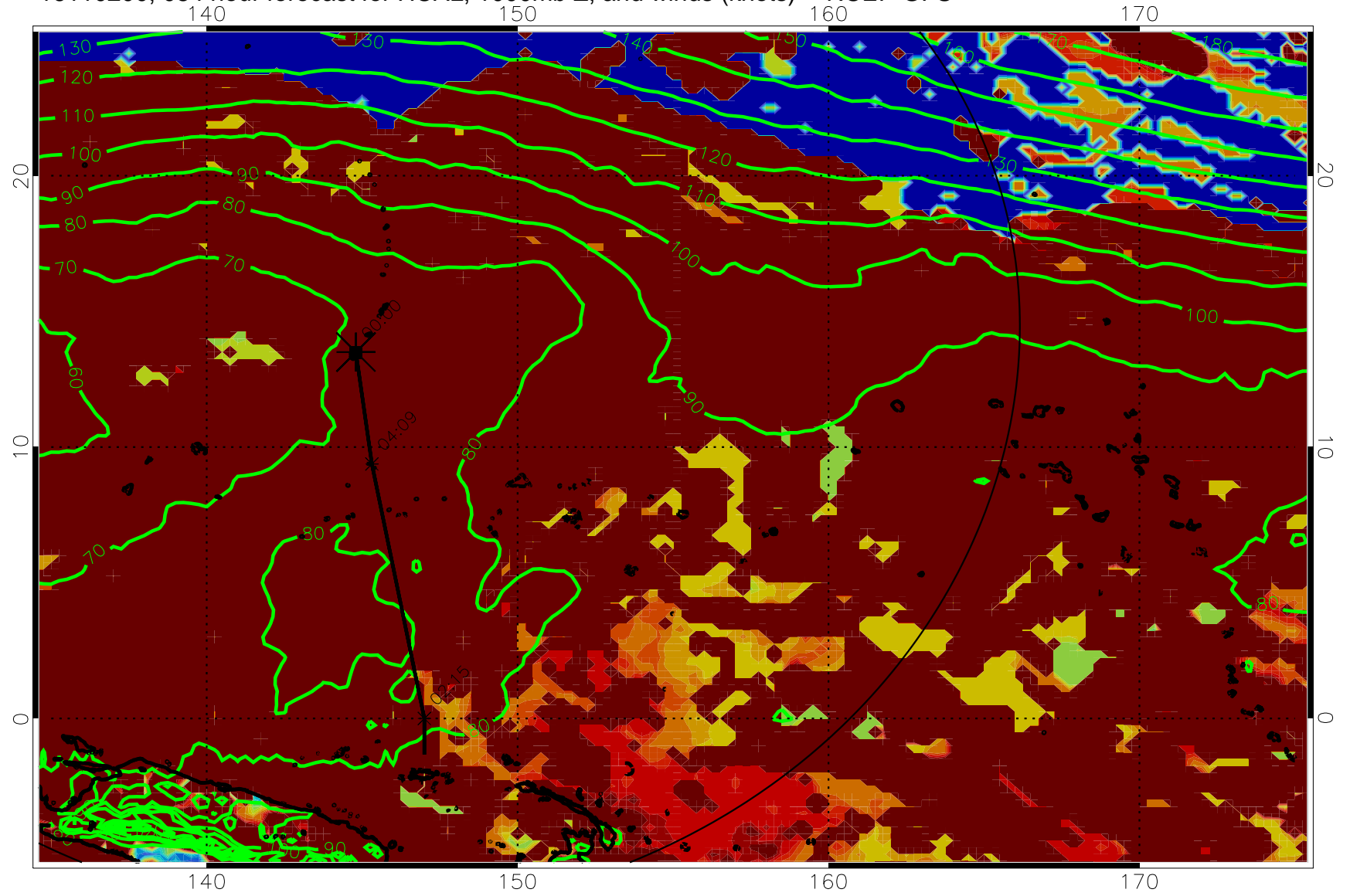
16110200, 084 hour forecast for HCAL, 1000mb Z, and winds (knots) -- NCEP GFS
