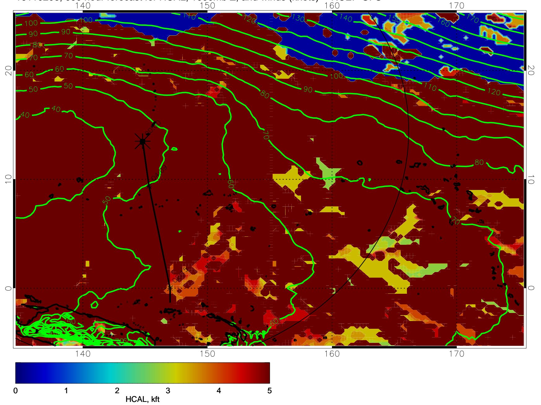
16110206, 090 hour forecast for HCAL, 1000mb Z, and winds (knots) -- NCEP GFS
