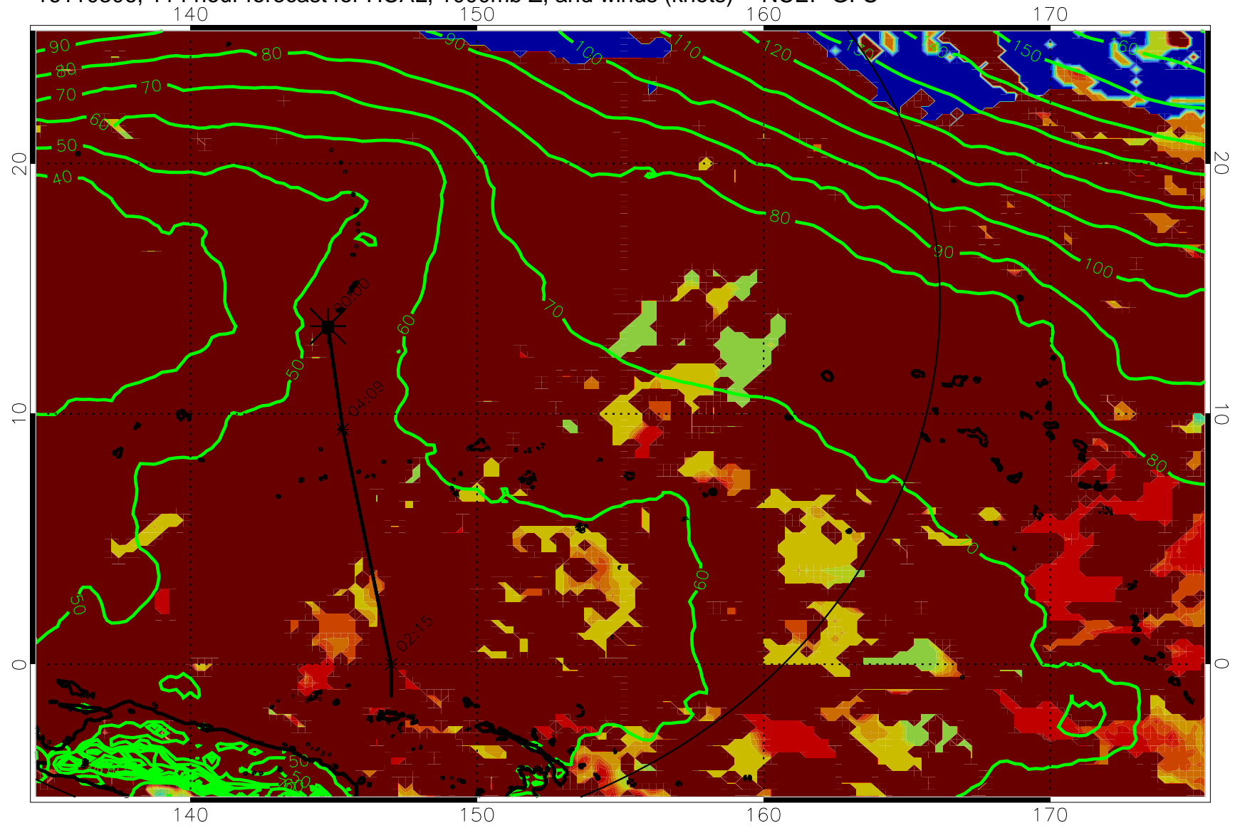
16110306, 114 hour forecast for HCAL, 1000mb Z, and winds (knots) -- NCEP GFS
