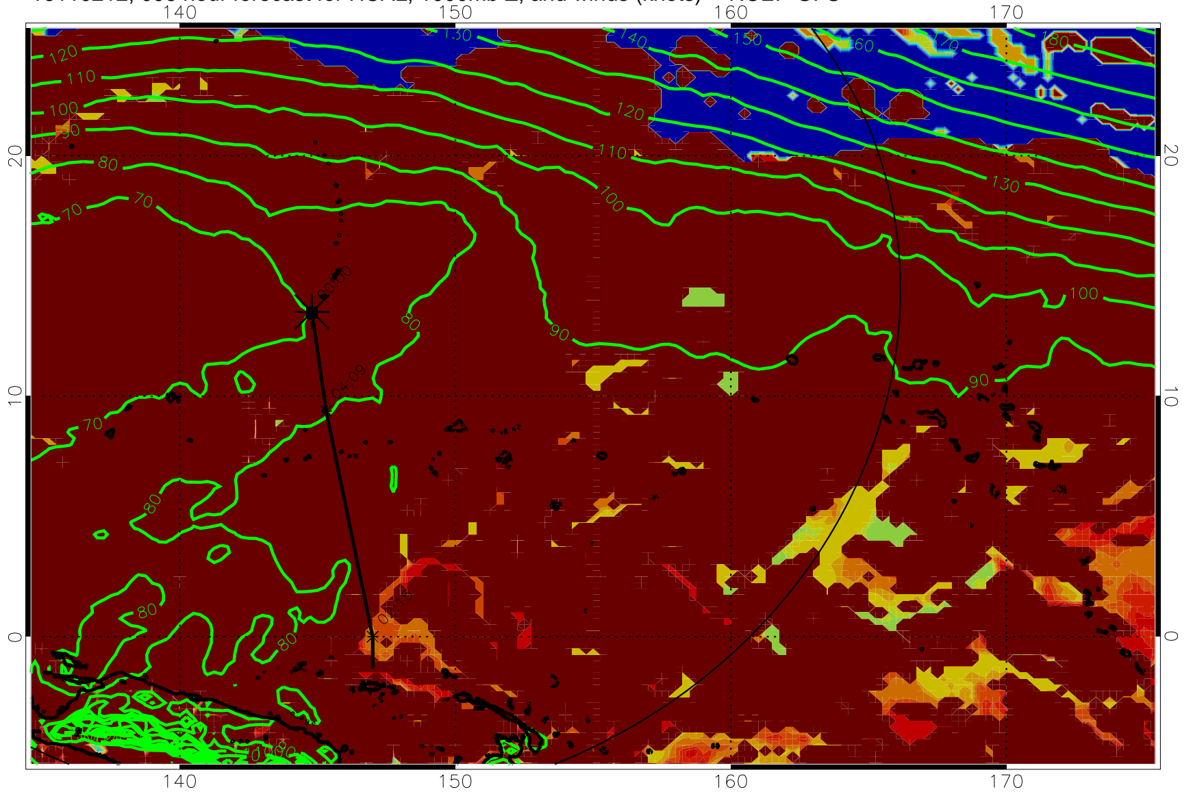
16110212, 096 hour forecast for HCAL, 1000mb Z, and winds (knots) -- NCEP GFS
