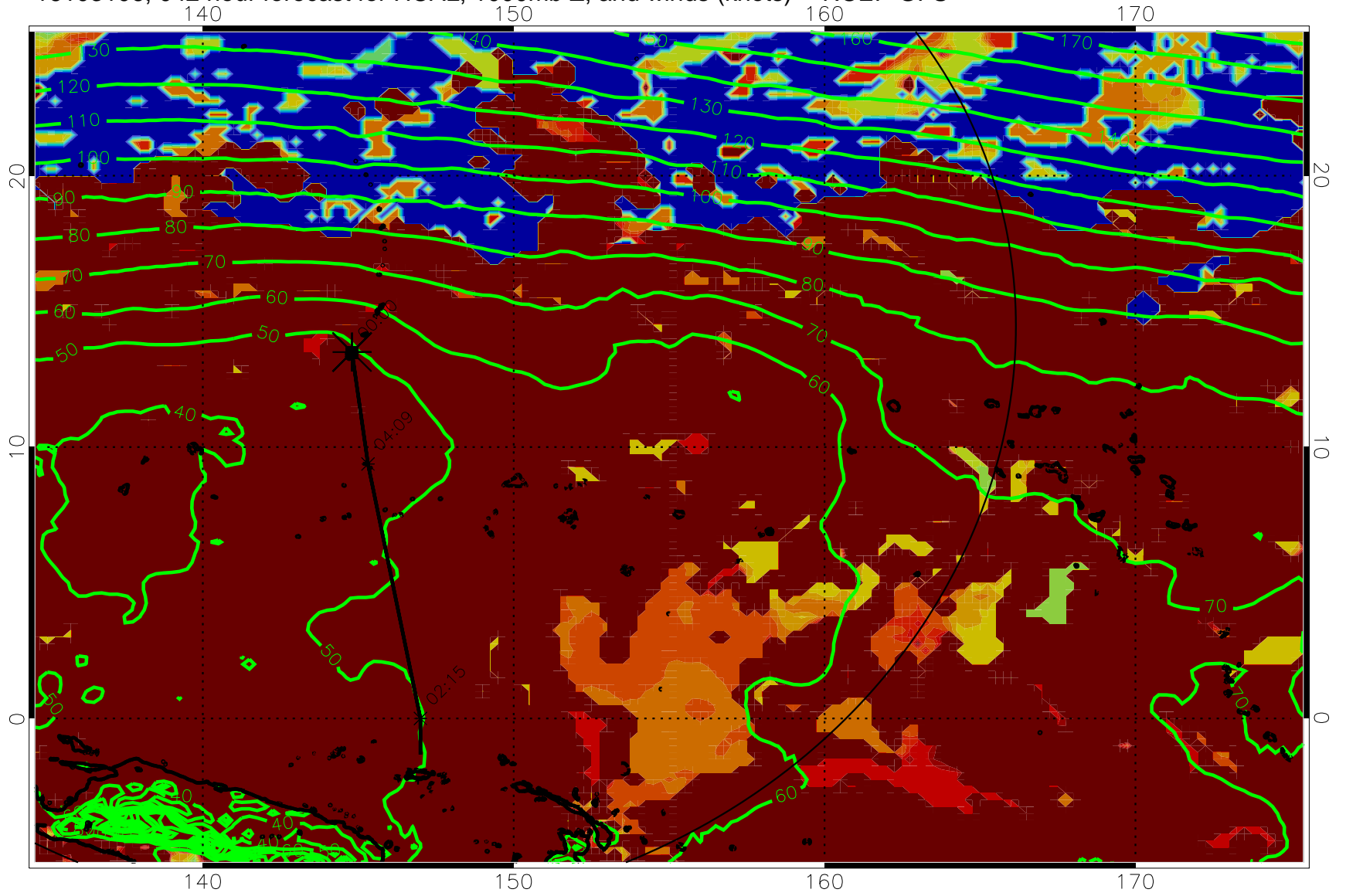
16103106, 042 hour forecast for HCAL, 1000mb Z, and winds (knots) -- NCEP GFS
