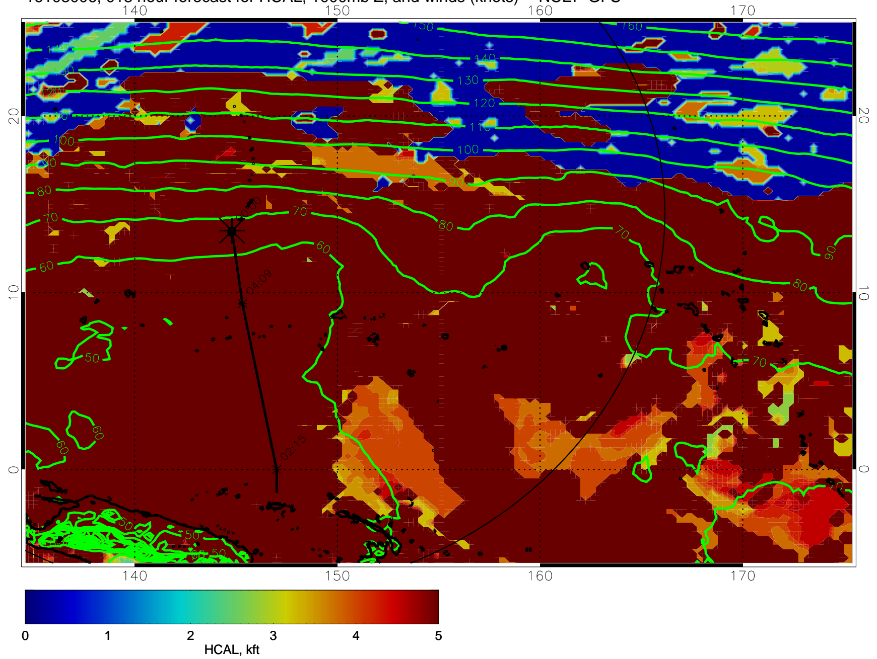
16103006, 018 hour forecast for HCAL, 1000mb Z, and winds (knots) -- NCEP GFS
