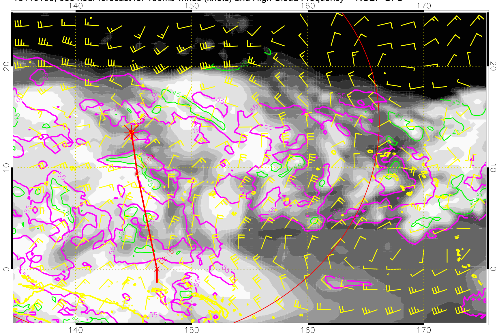
16110106, 066 hour forecast for 150mb winds (knots) and High Cloud Frequency -- NCEP GFS
