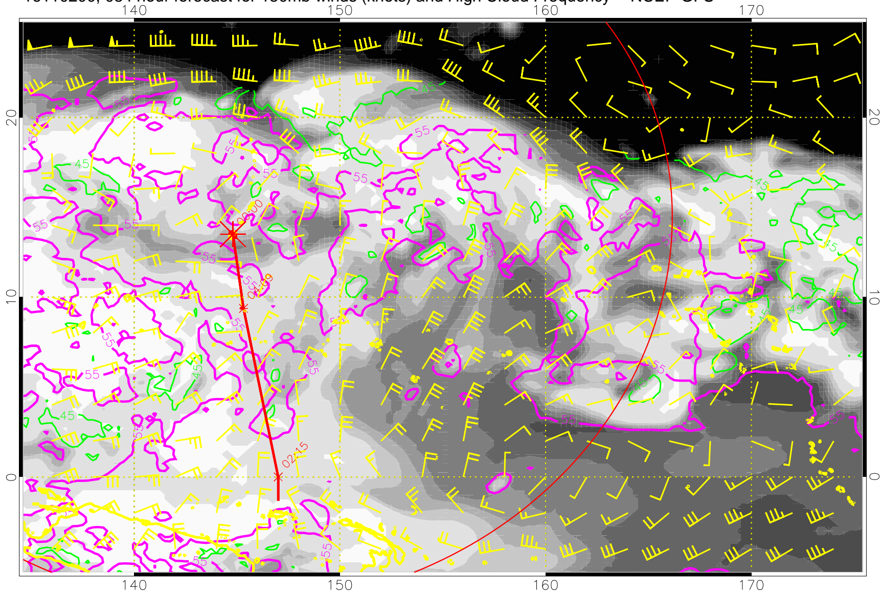
16110200, 084 hour forecast for 150mb winds (knots) and High Cloud Frequency -- NCEP GFS
