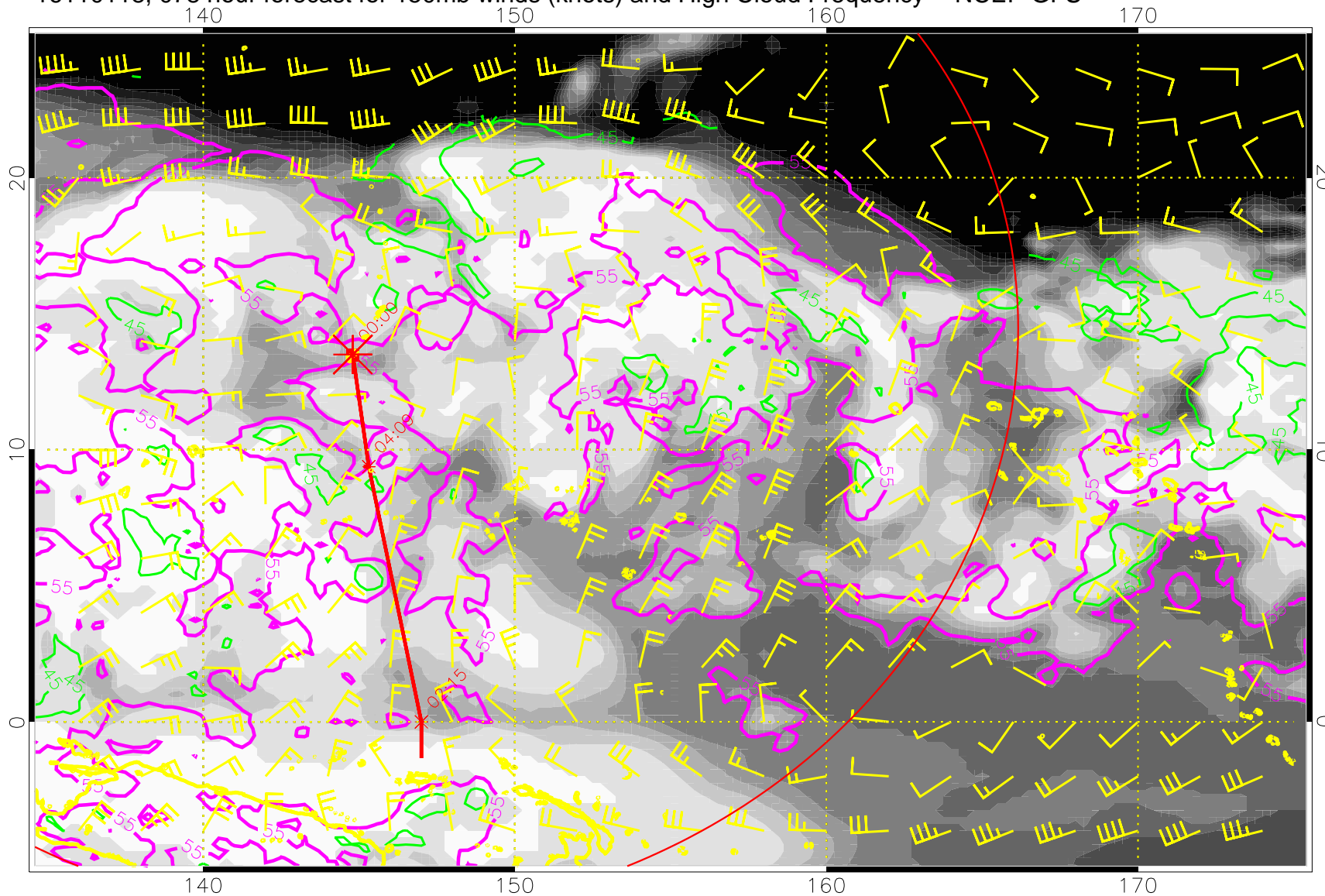
16110118, 078 hour forecast for 150mb winds (knots) and High Cloud Frequency -- NCEP GFS
