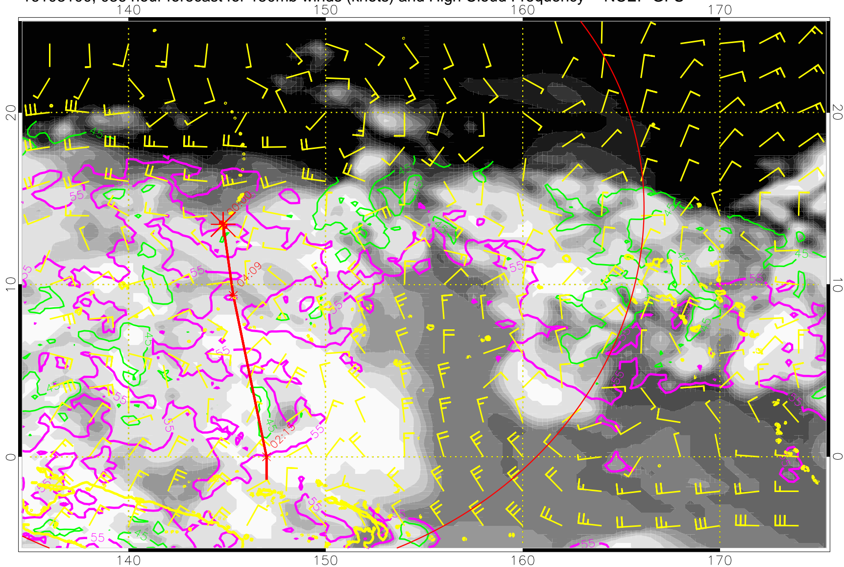
16103100, 036 hour forecast for 150mb winds (knots) and High Cloud Frequency -- NCEP GFS
