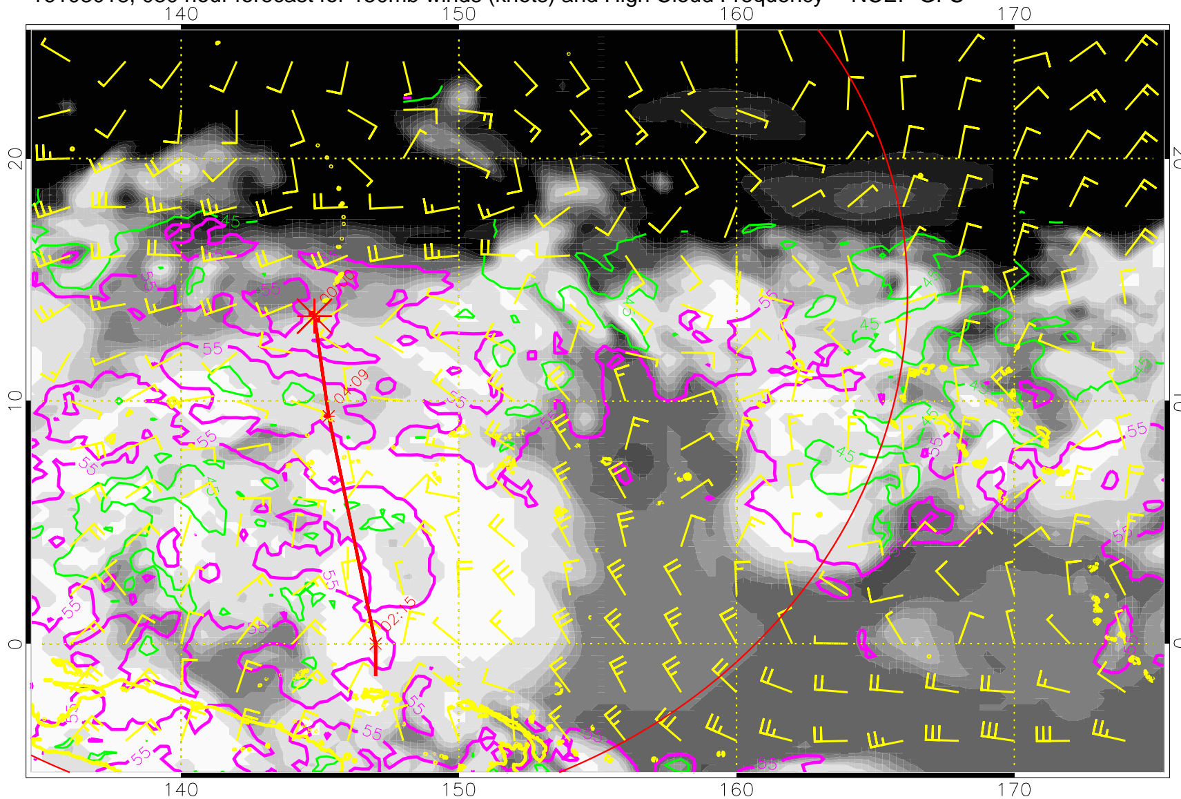
16103018, 030 hour forecast for 150mb winds (knots) and High Cloud Frequency -- NCEP GFS
