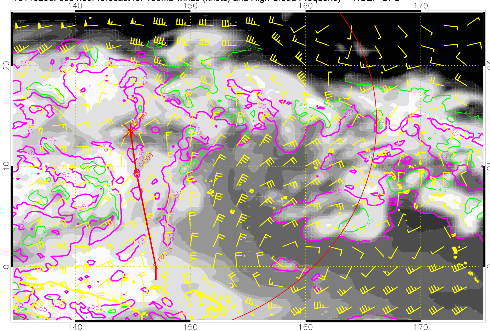
16110206, 090 hour forecast for 150mb winds (knots) and High Cloud Frequency -- NCEP GFS
