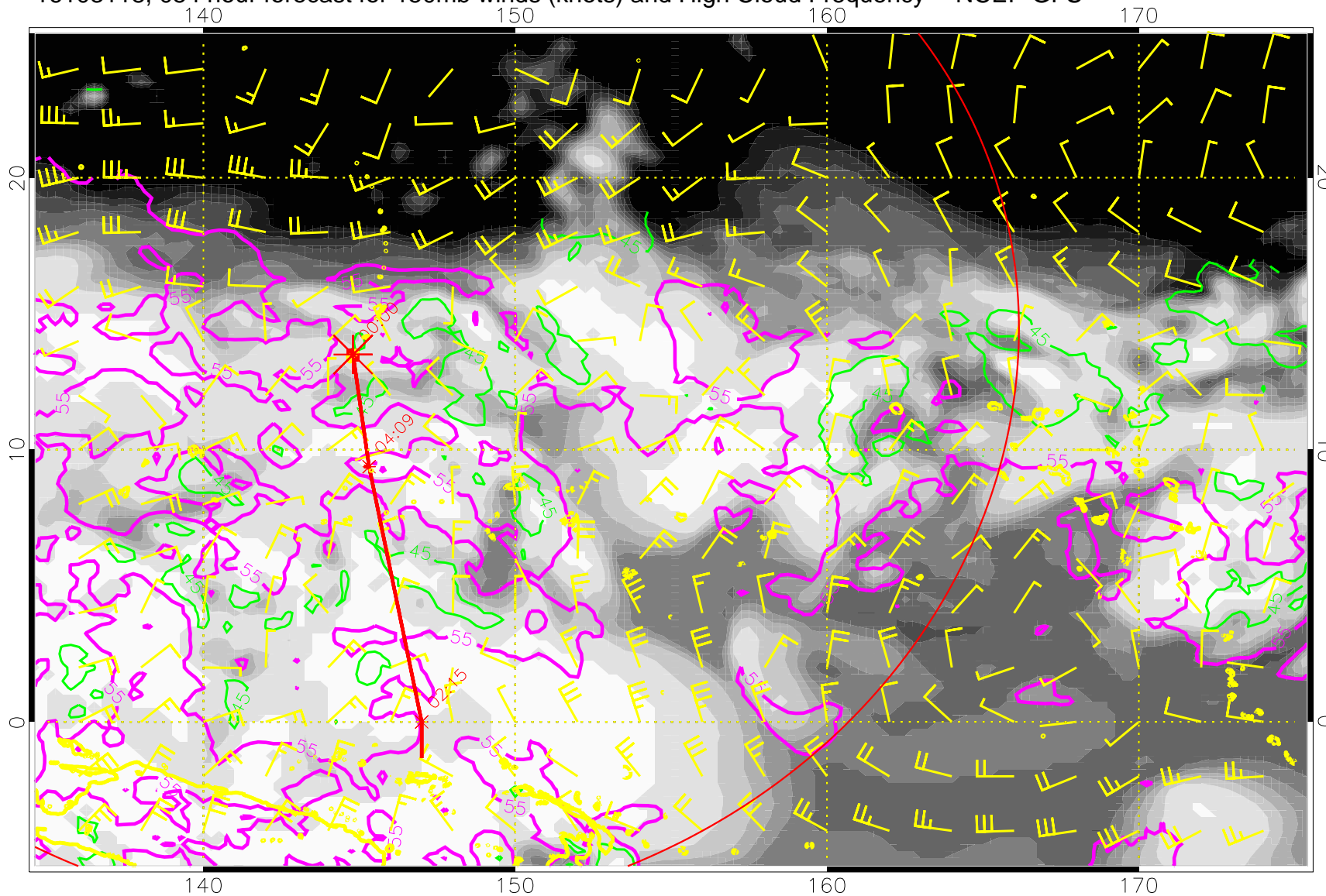
16103118, 054 hour forecast for 150mb winds (knots) and High Cloud Frequency -- NCEP GFS
