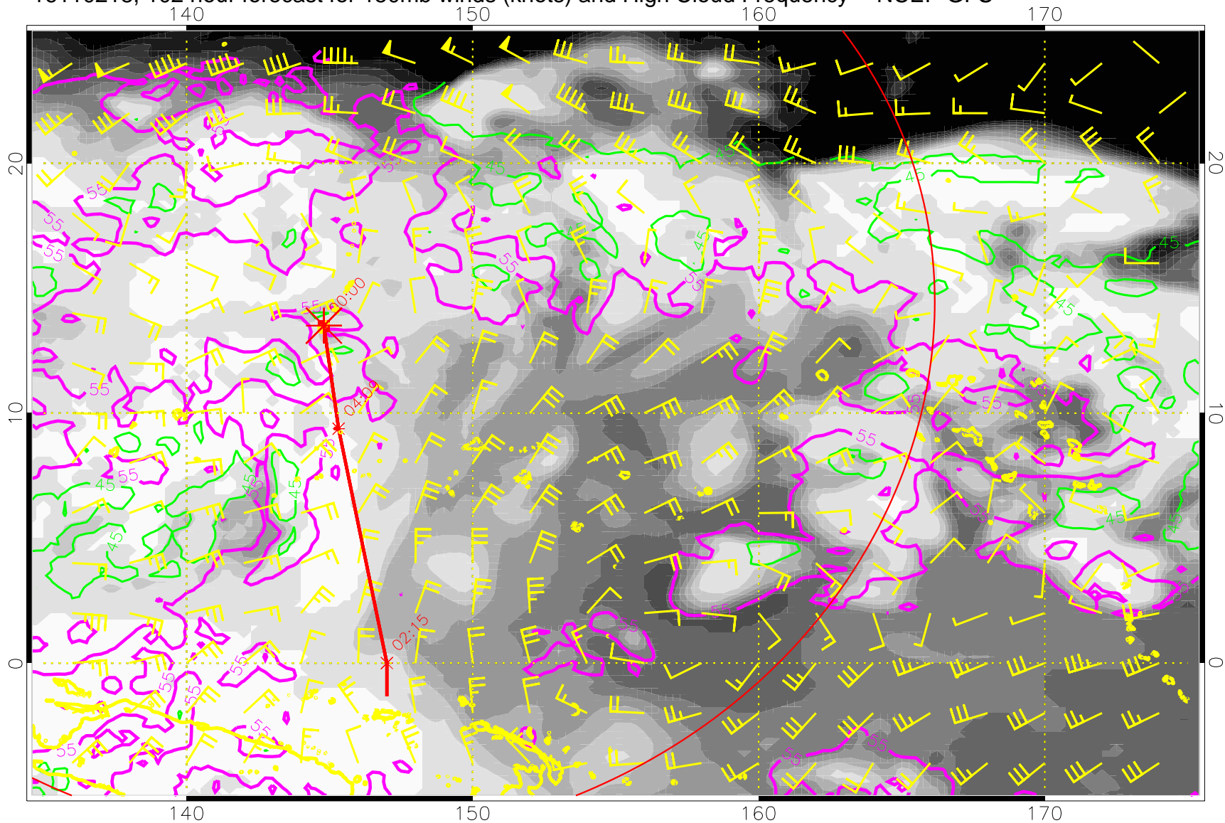
16110218, 102 hour forecast for 150mb winds (knots) and High Cloud Frequency -- NCEP GFS
