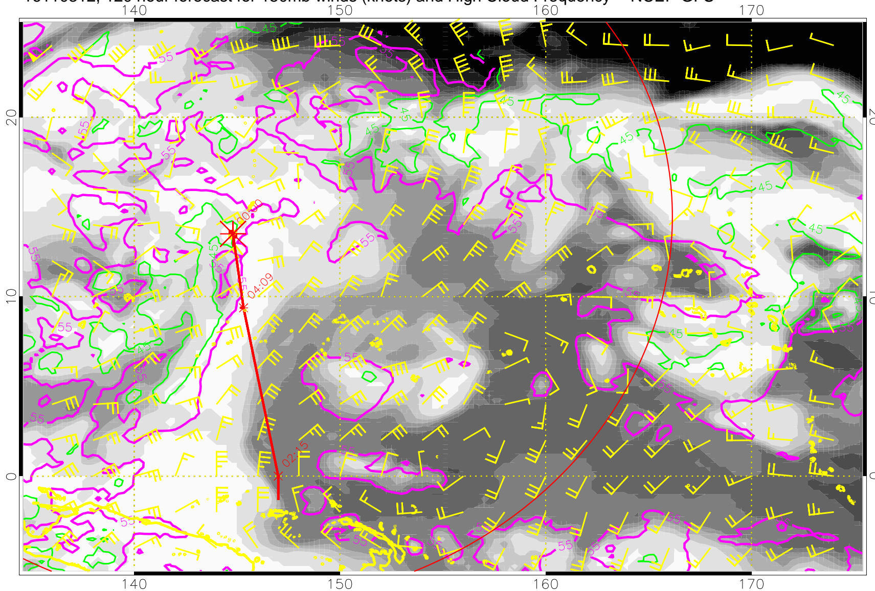
16110312, 120 hour forecast for 150mb winds (knots) and High Cloud Frequency -- NCEP GFS
