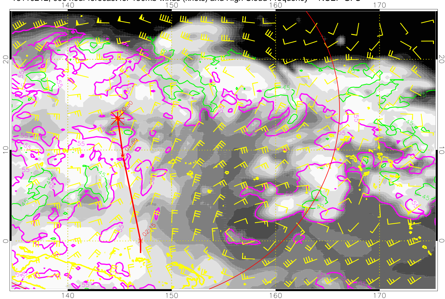
16110212, 096 hour forecast for 150mb winds (knots) and High Cloud Frequency -- NCEP GFS
