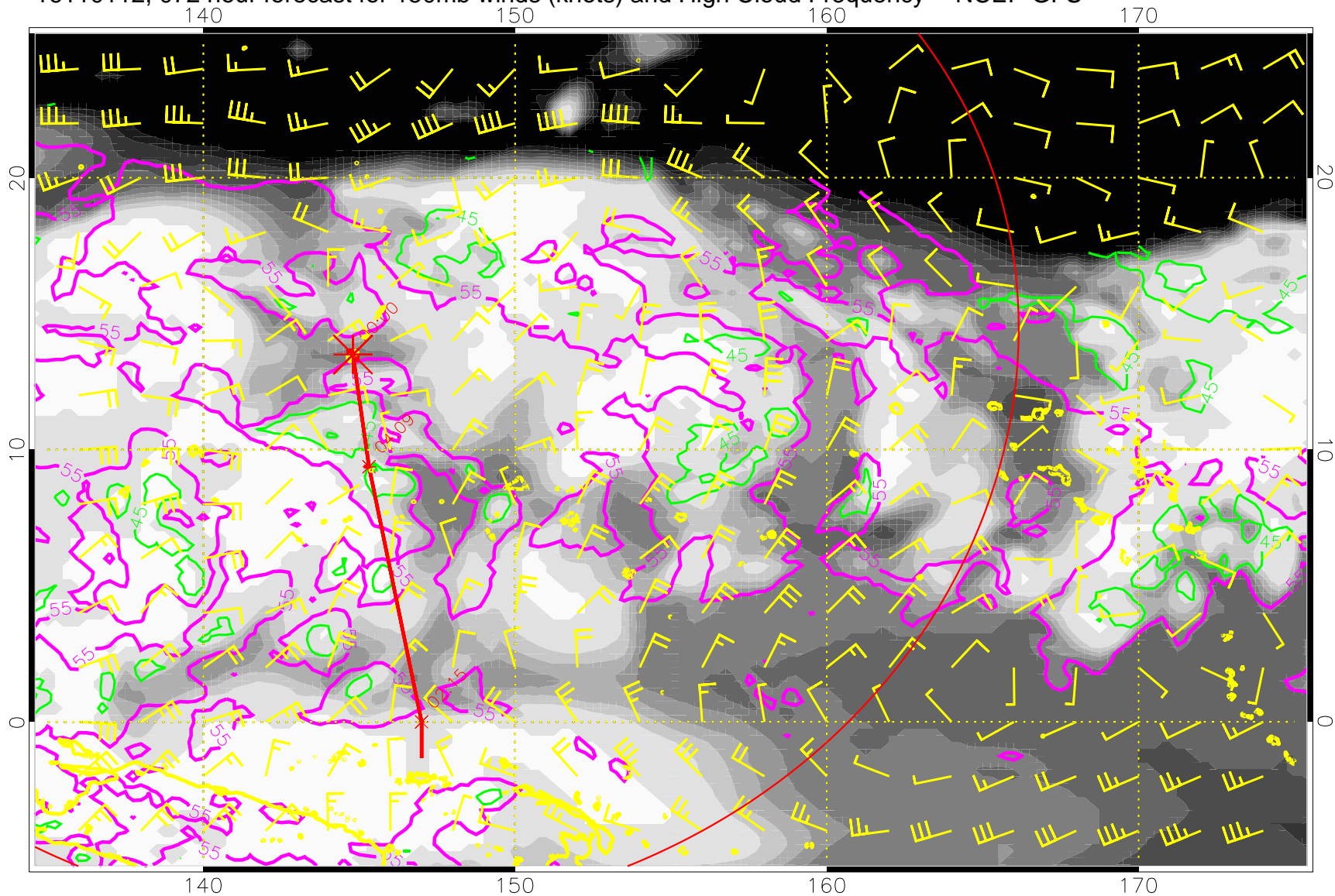
16110112, 072 hour forecast for 150mb winds (knots) and High Cloud Frequency -- NCEP GFS
