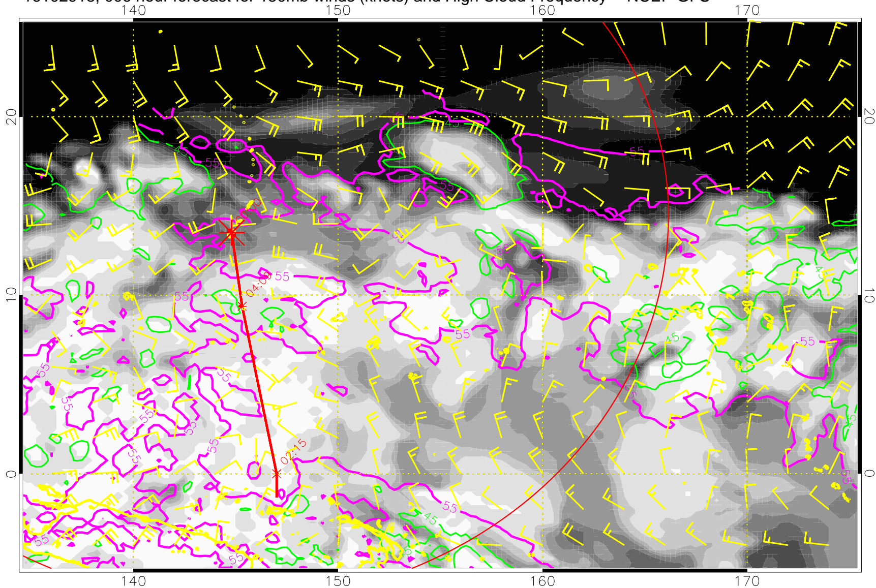
16102918, 006 hour forecast for 150mb winds (knots) and High Cloud Frequency -- NCEP GFS
