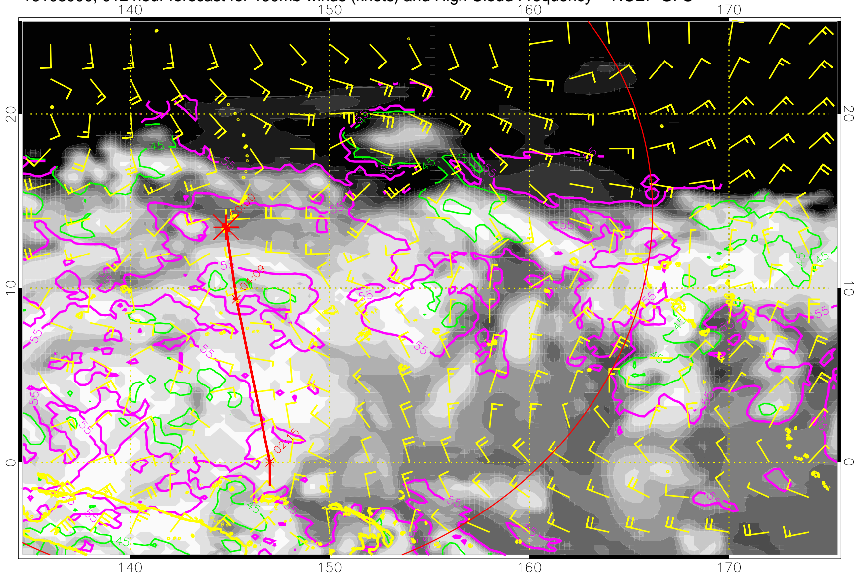
16103000, 012 hour forecast for 150mb winds (knots) and High Cloud Frequency -- NCEP GFS
