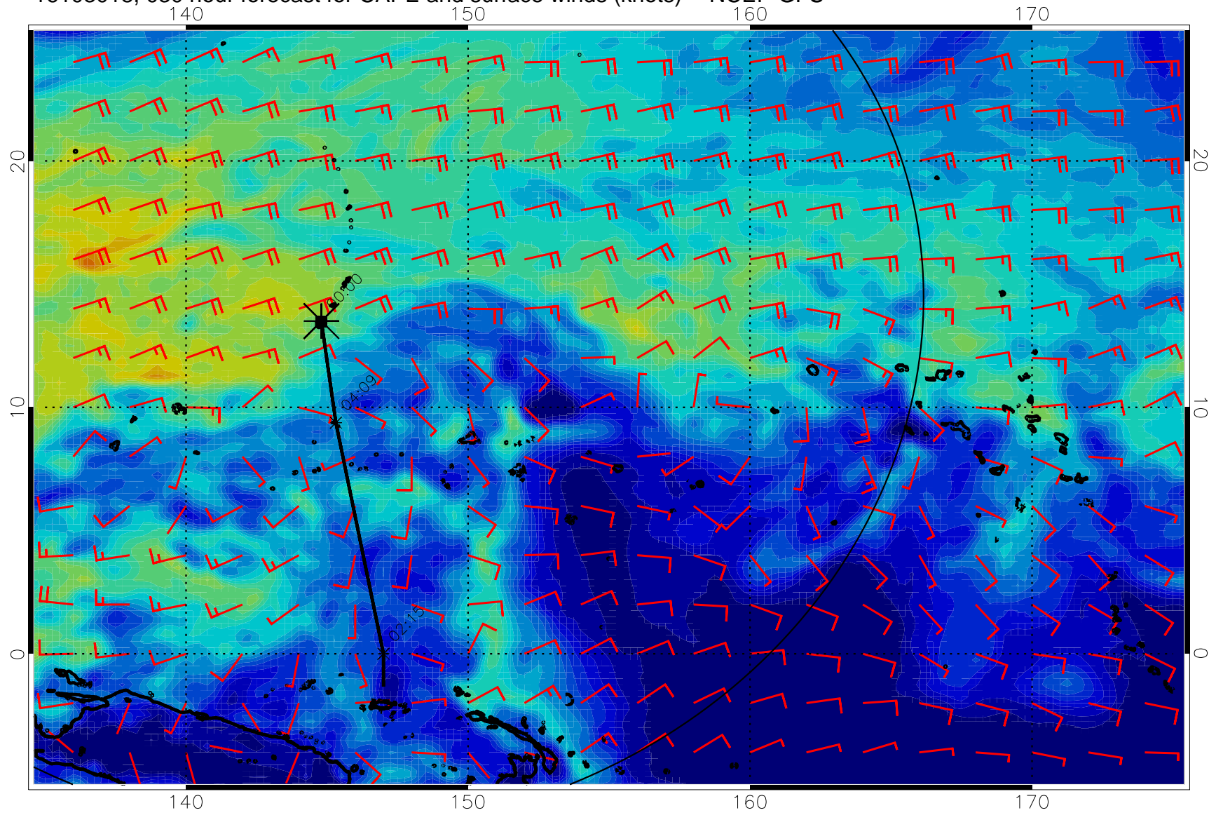
16103018, 0300 hour forecast for CAPE and surface winds (knots) -- NCEP GFS
