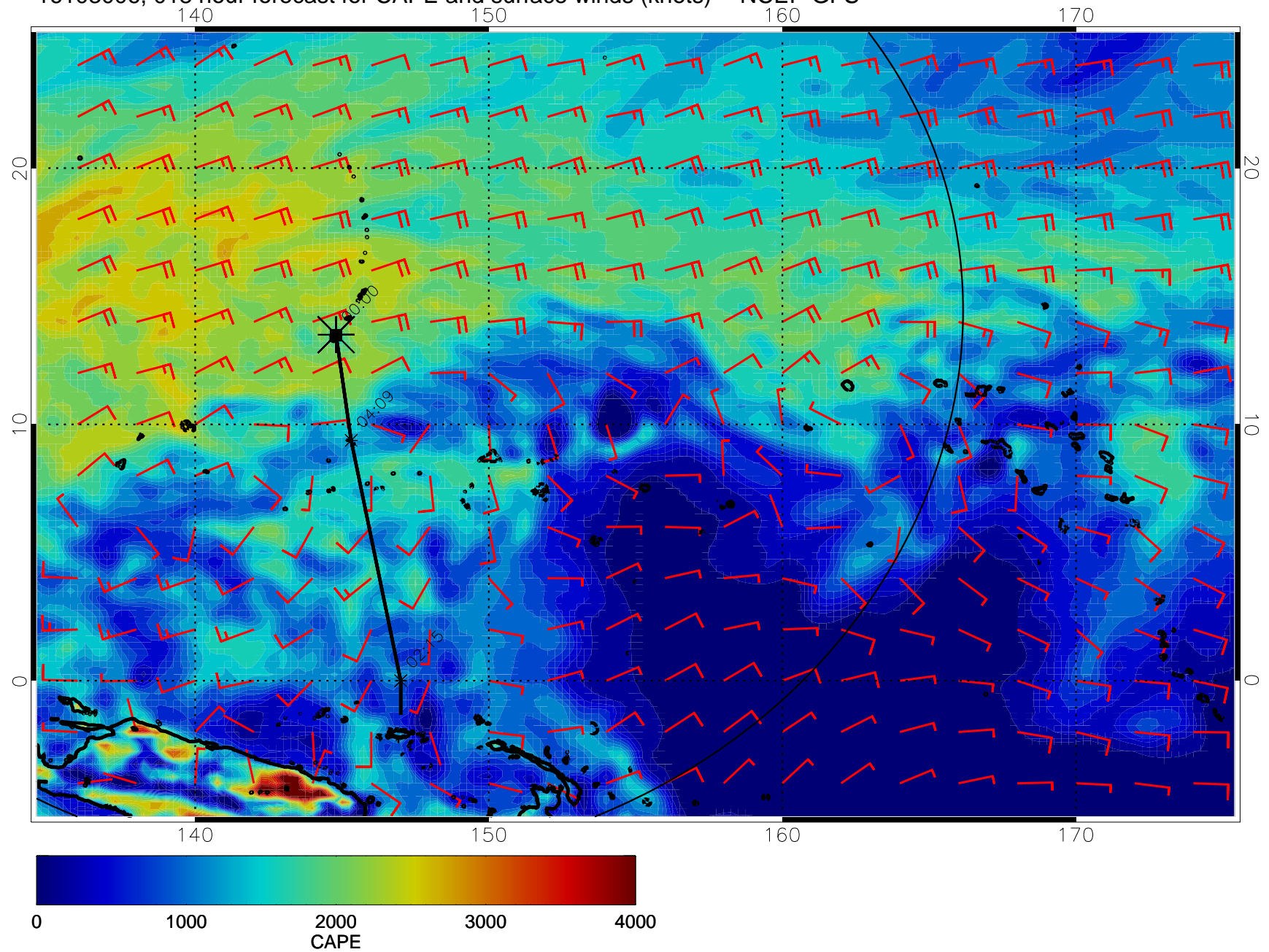
16103006, 018 hour forecast for CAPE and surface winds (knots) -- NCEP GFS
