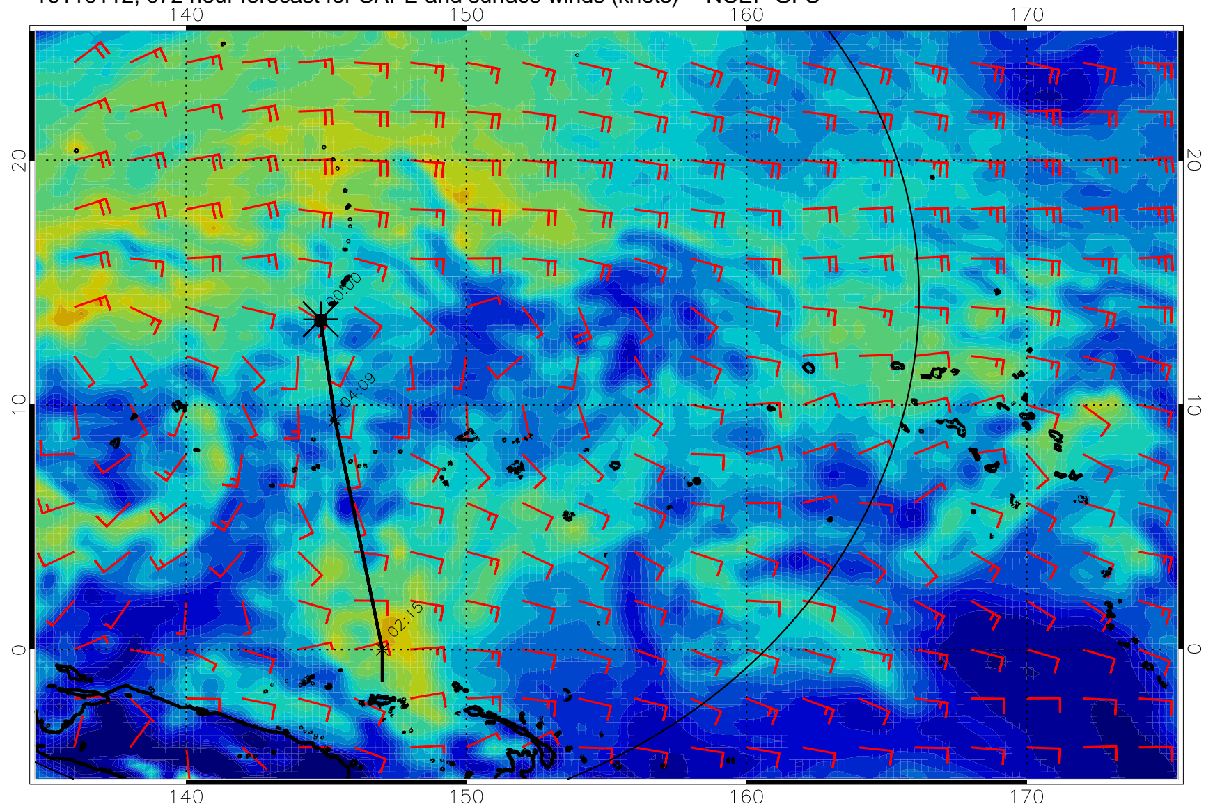
16110112, 072 hour forecast for CAPE and surface winds (knots) -- NCEP GFS
