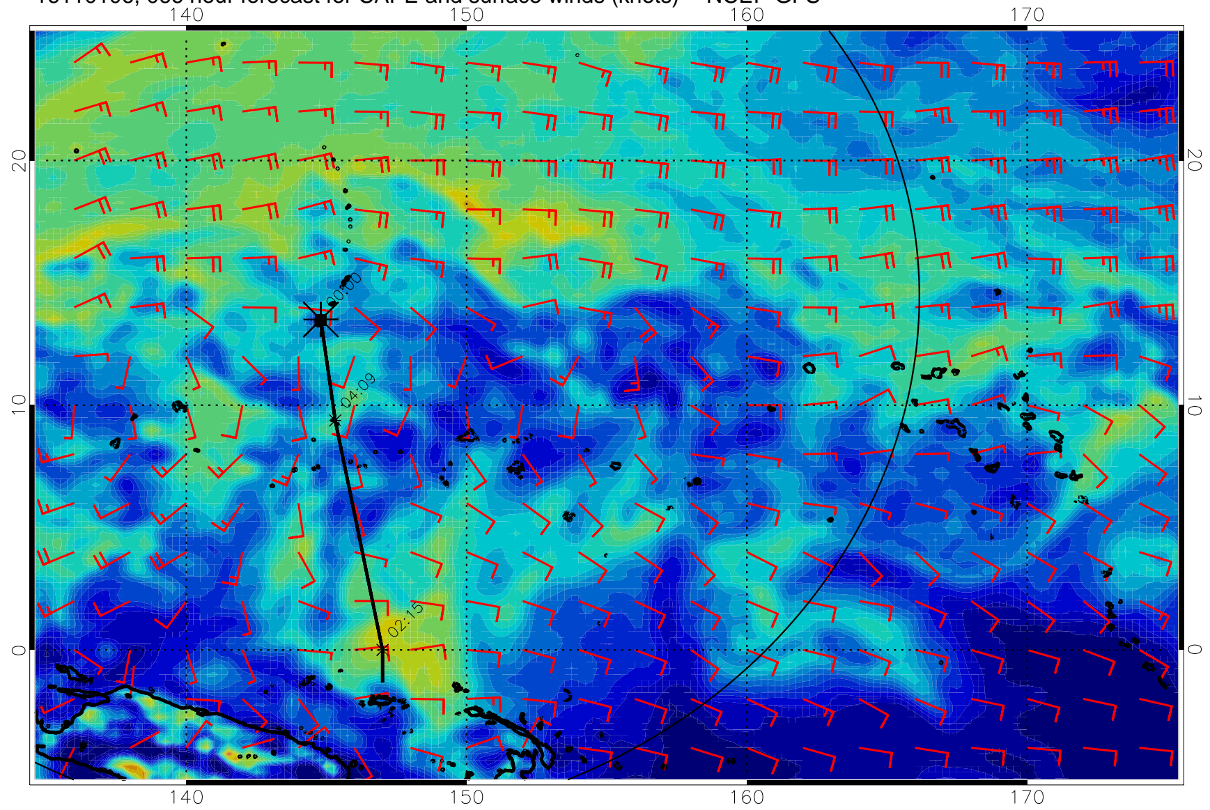
16110106, 066 hour forecast for CAPE and surface winds (knots) -- NCEP GFS
