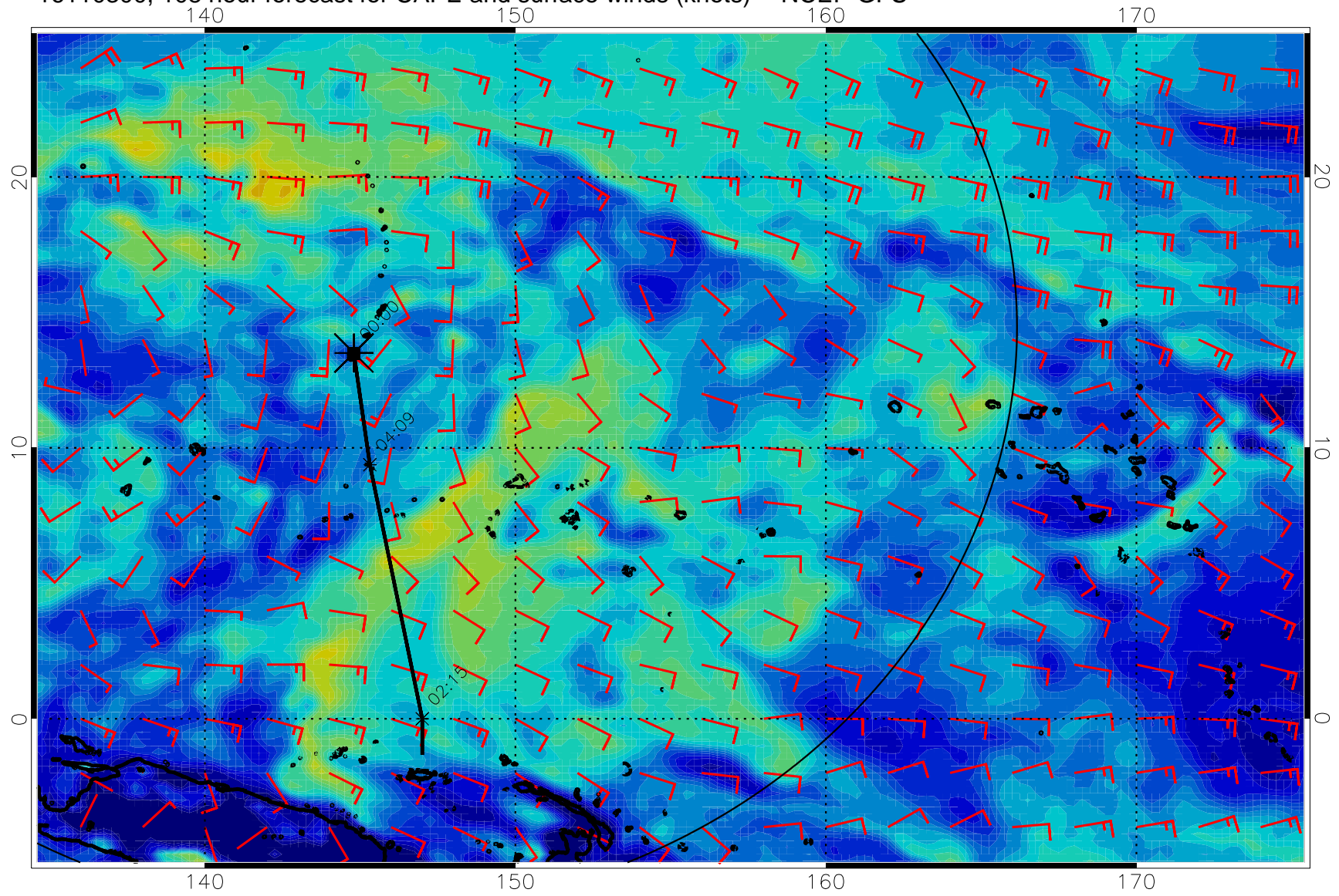
16110300, 108 hour forecast for CAPE and surface winds (knots) -- NCEP GFS
