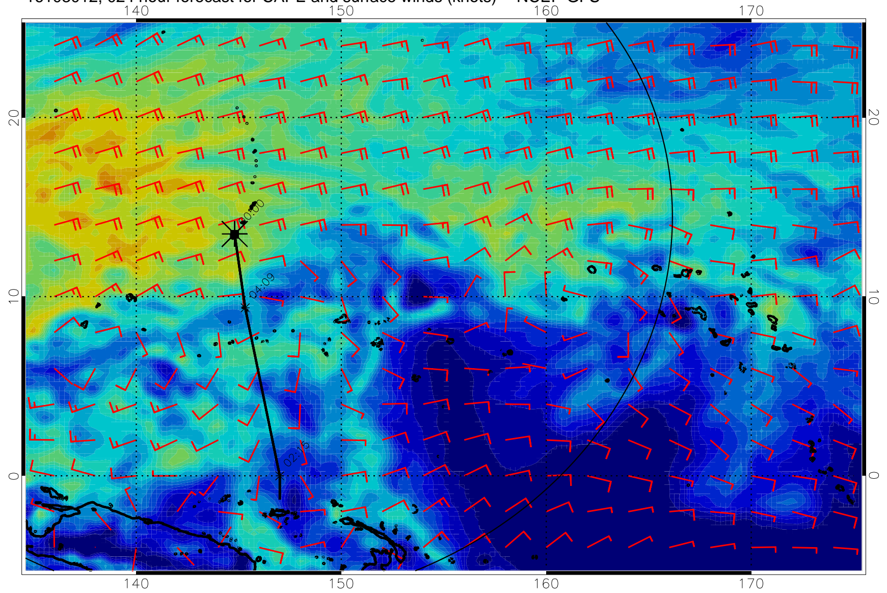
16103012, 024 hour forecast for CAPE and surface winds (knots) -- NCEP GFS
