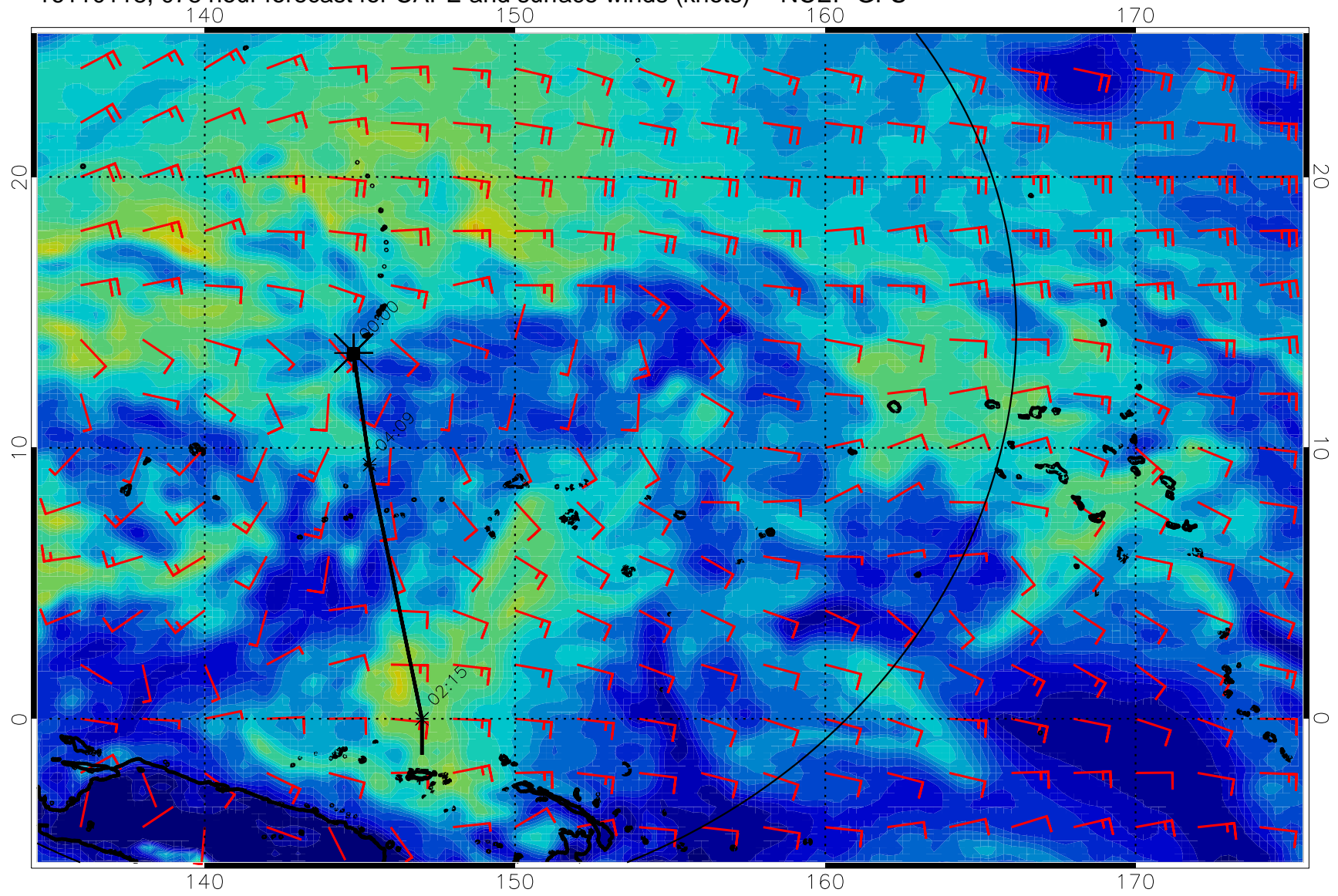
16110118, 078 hour forecast for CAPE and surface winds (knots) -- NCEP GFS
