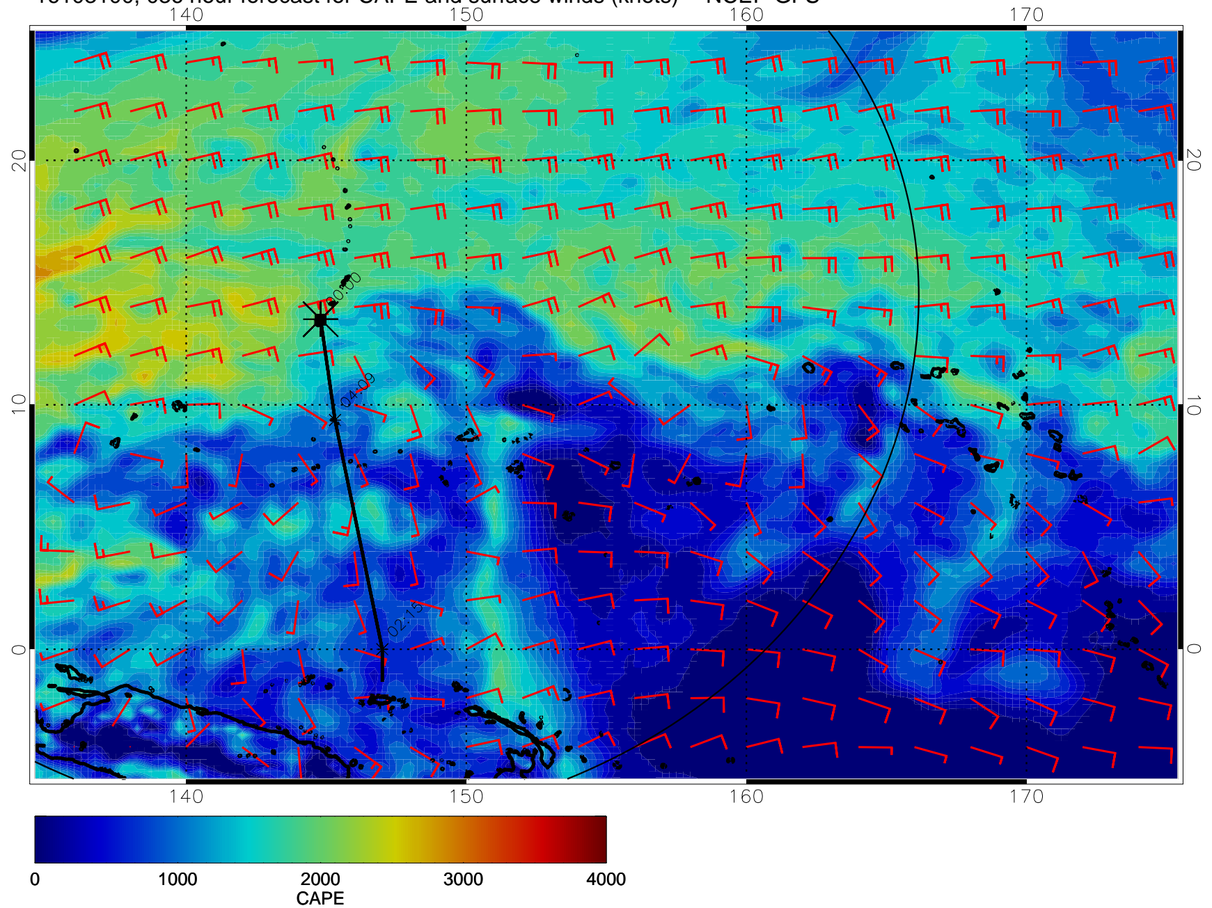
16103100, 036 hour forecast for CAPE and surface winds (knots) -- NCEP GFS
