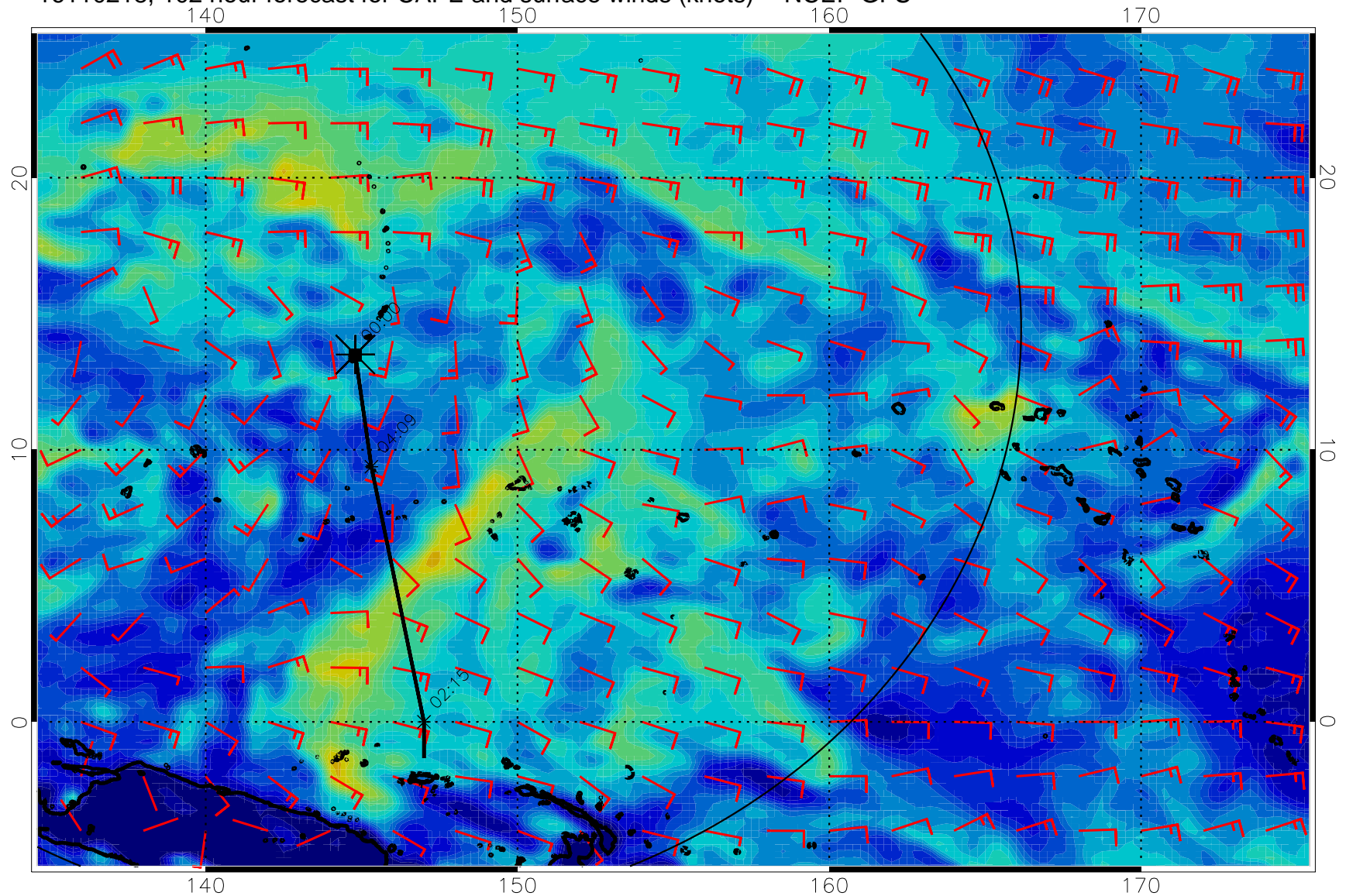
16110218, 102 hour forecast for CAPE and surface winds (knots) -- NCEP GFS
