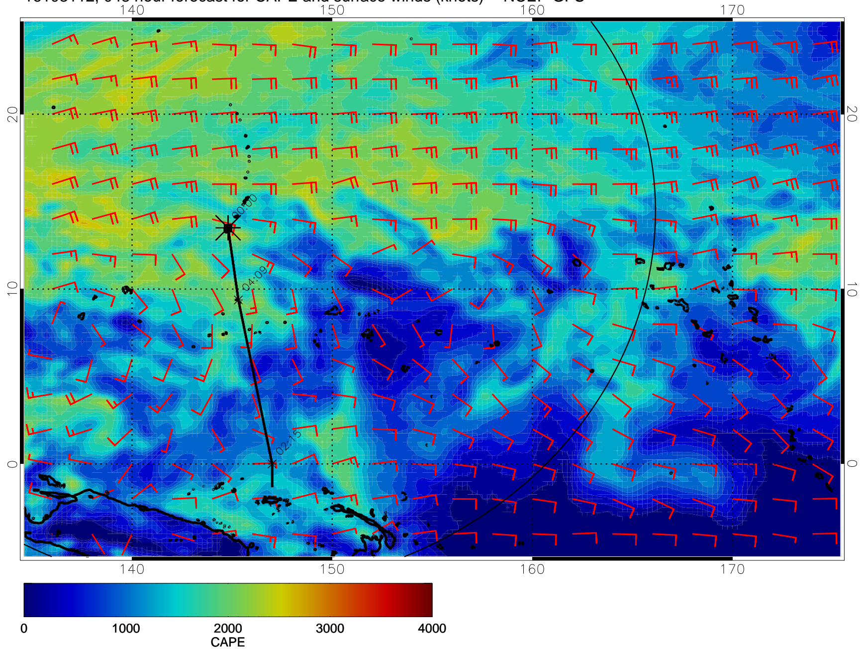
16103112, 048 hour forecast for CAPE and surface winds (knots) -- NCEP GFS
