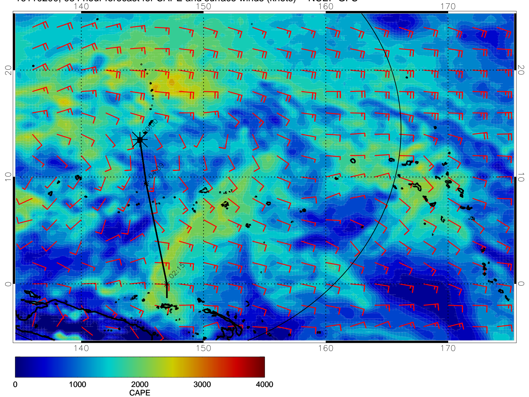
16110200, 084 hour forecast for CAPE and surface winds (knots) -- NCEP GFS
