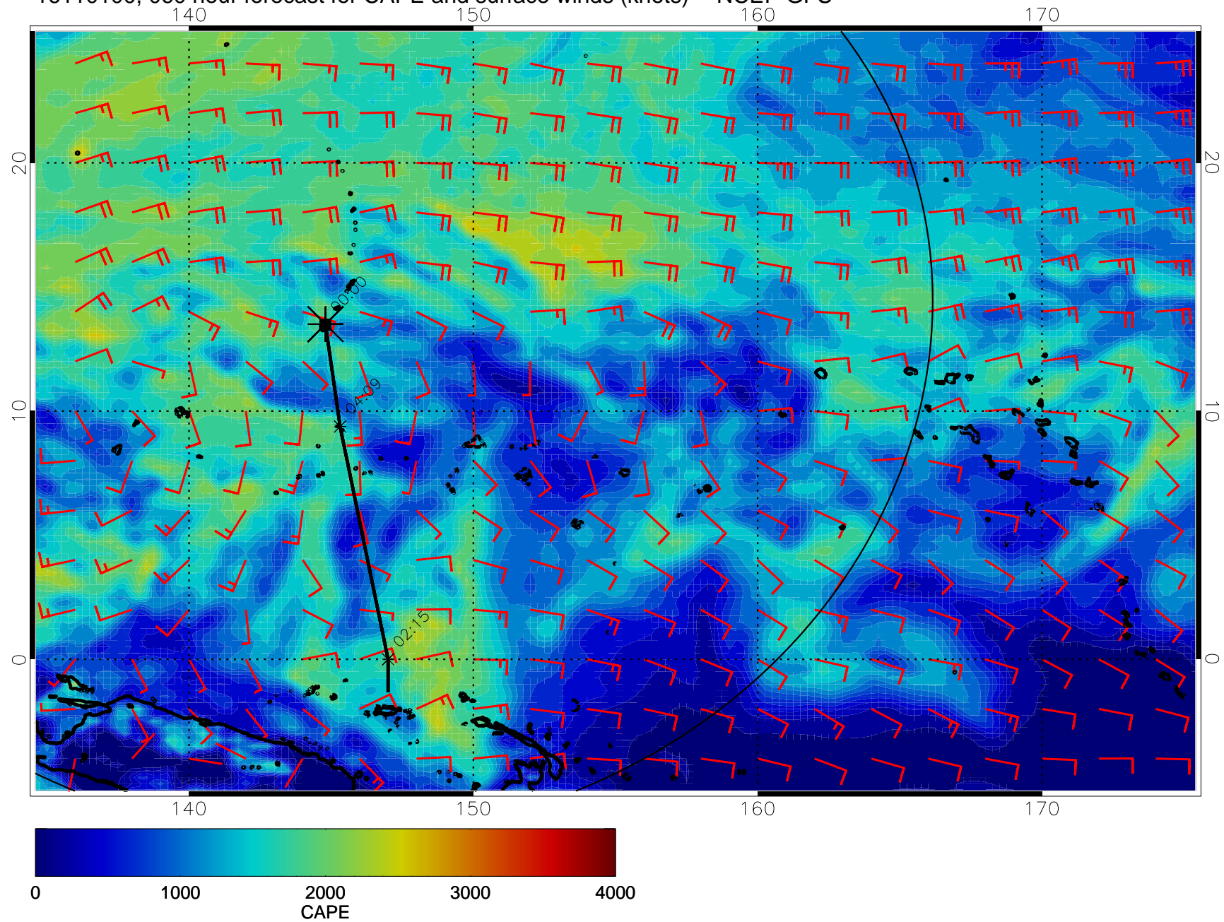
16110100, 060 hour forecast for CAPE and surface winds (knots) -- NCEP GFS
