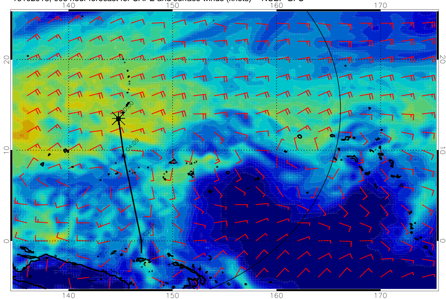
16102918, 006 hour forecast for CAPE and surface winds (knots) -- NCEP GFS
