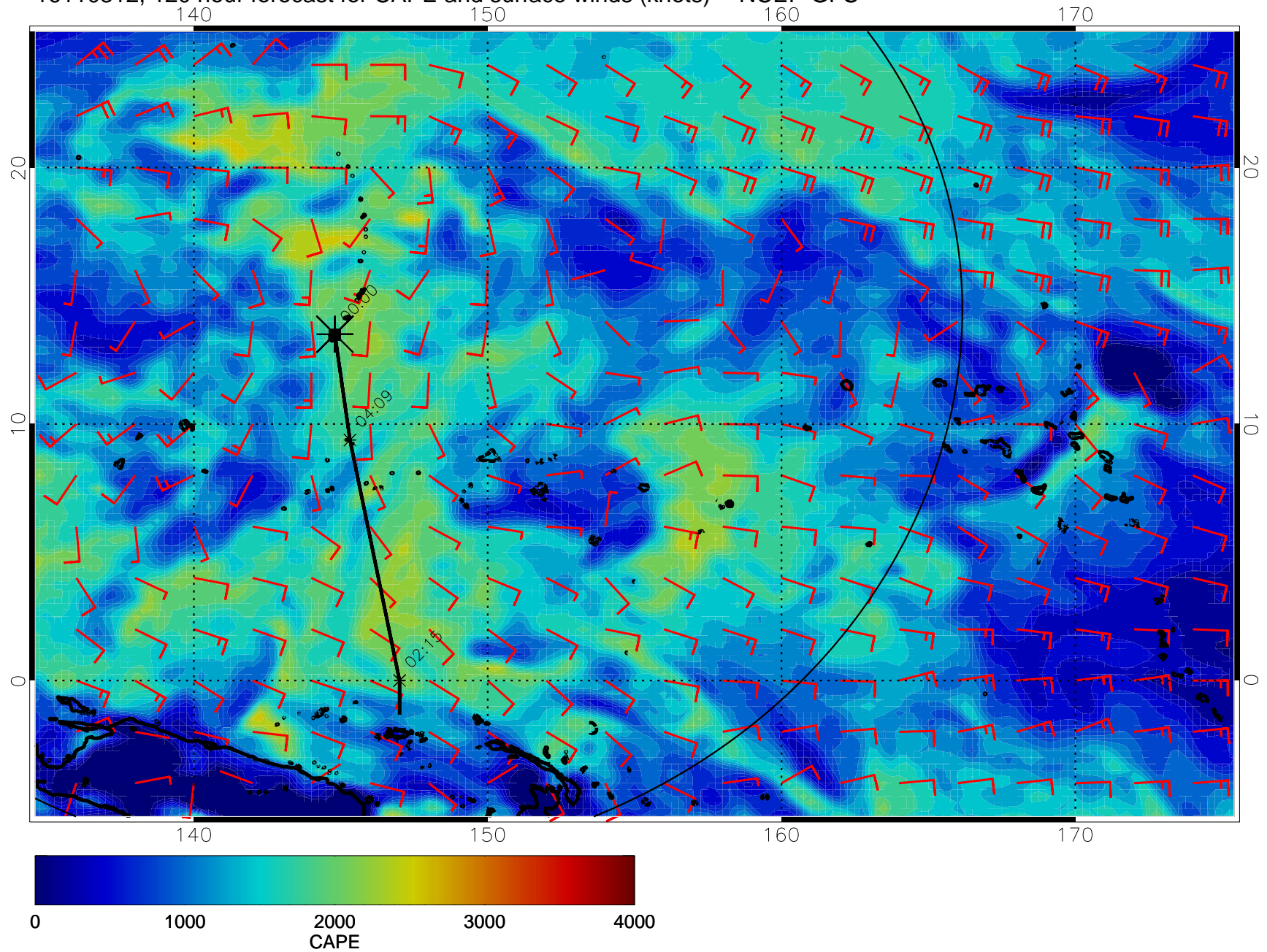
16110312, 120 hour forecast for CAPE and surface winds (knots) -- NCEP GFS
