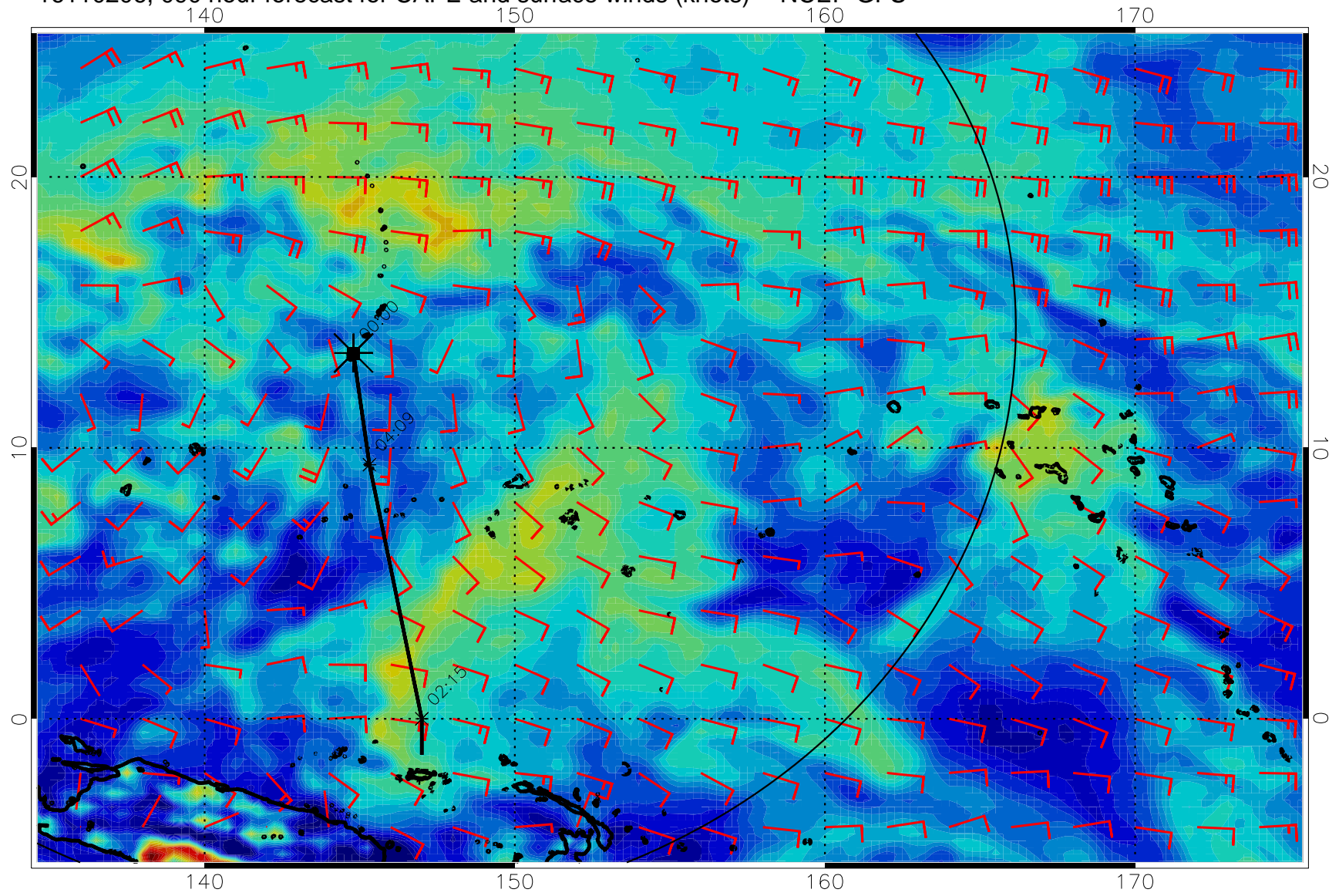
16110206, 090 hour forecast for CAPE and surface winds (knots) -- NCEP GFS
