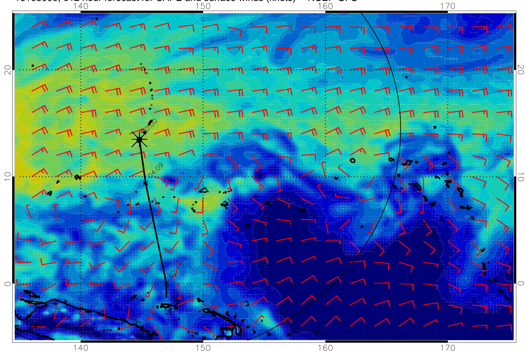
16103000, 012 hour forecast for CAPE and surface winds (knots) -- NCEP GFS
