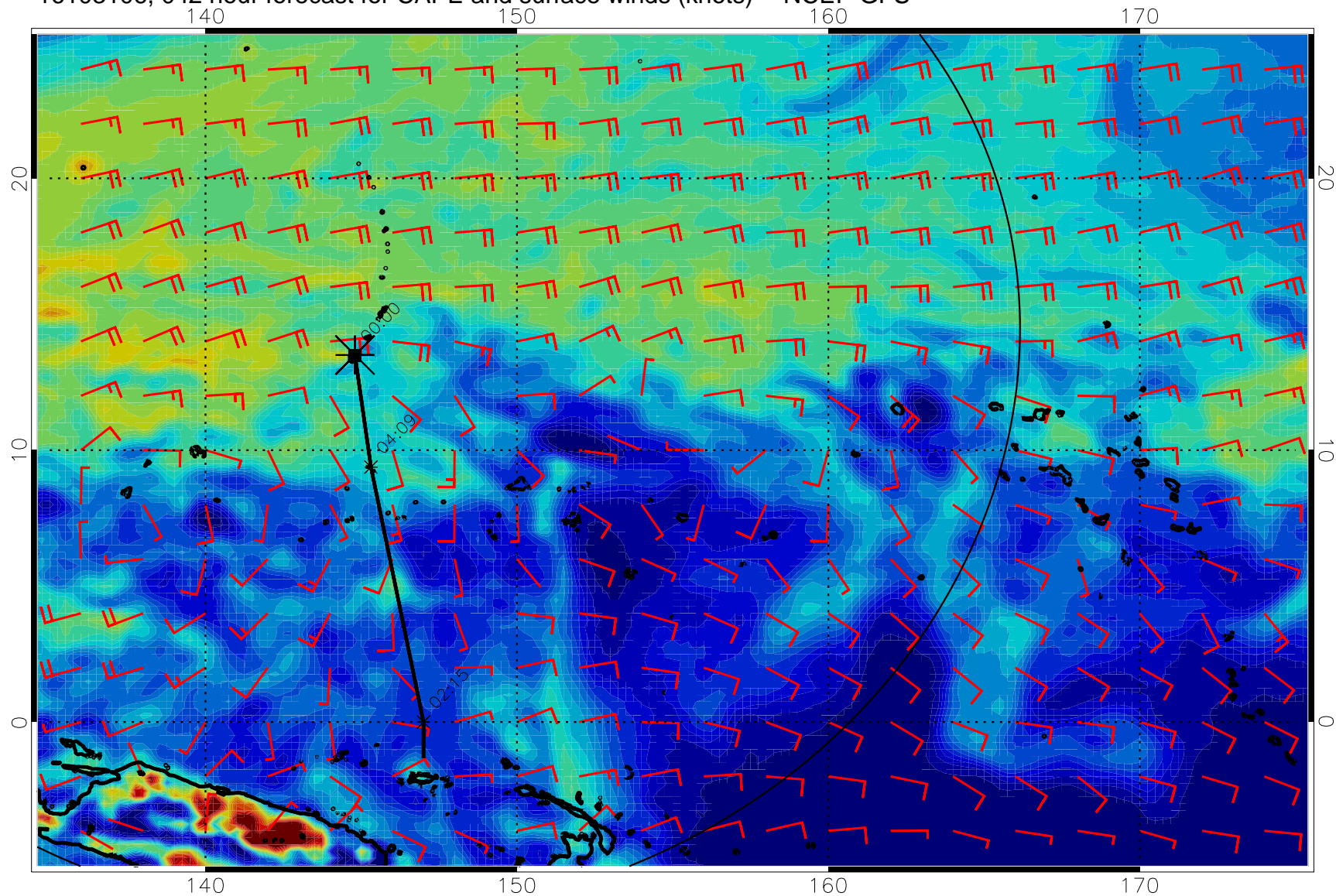
16103106, 042 hour forecast for CAPE and surface winds (knots) -- NCEP GFS
