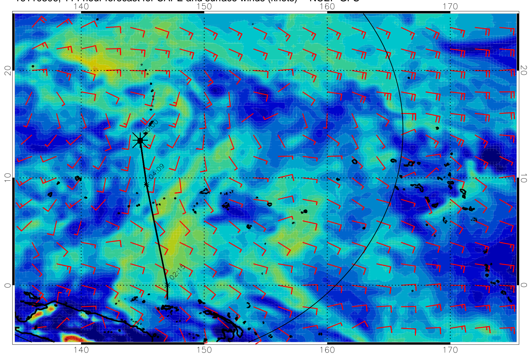
16110306, 114 hour forecast for CAPE and surface winds (knots) -- NCEP GFS
