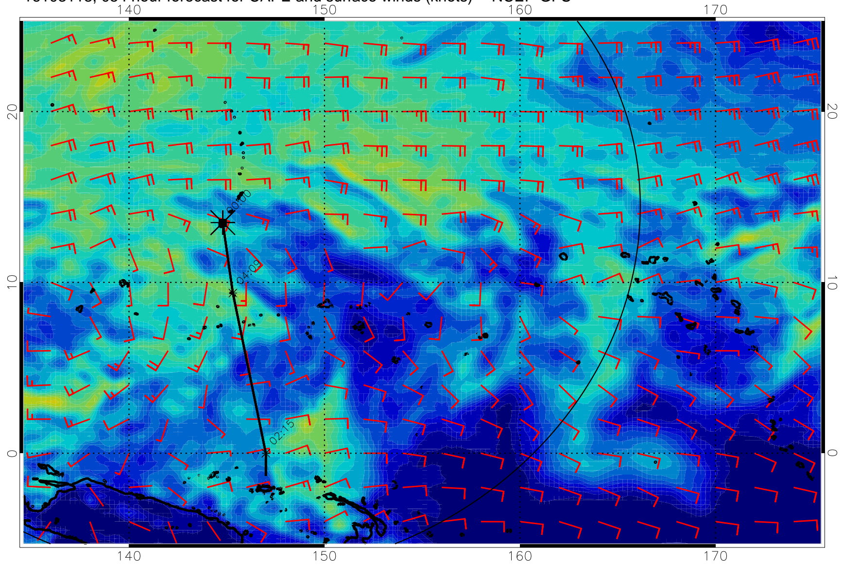
16103118, 054 hour forecast for CAPE and surface winds (knots) -- NCEP GFS
