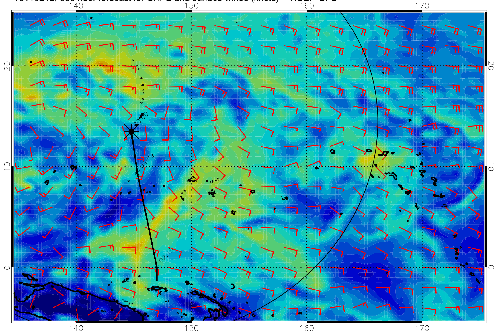
16110212, 096 hour forecast for CAPE and surface winds (knots) -- NCEP GFS
