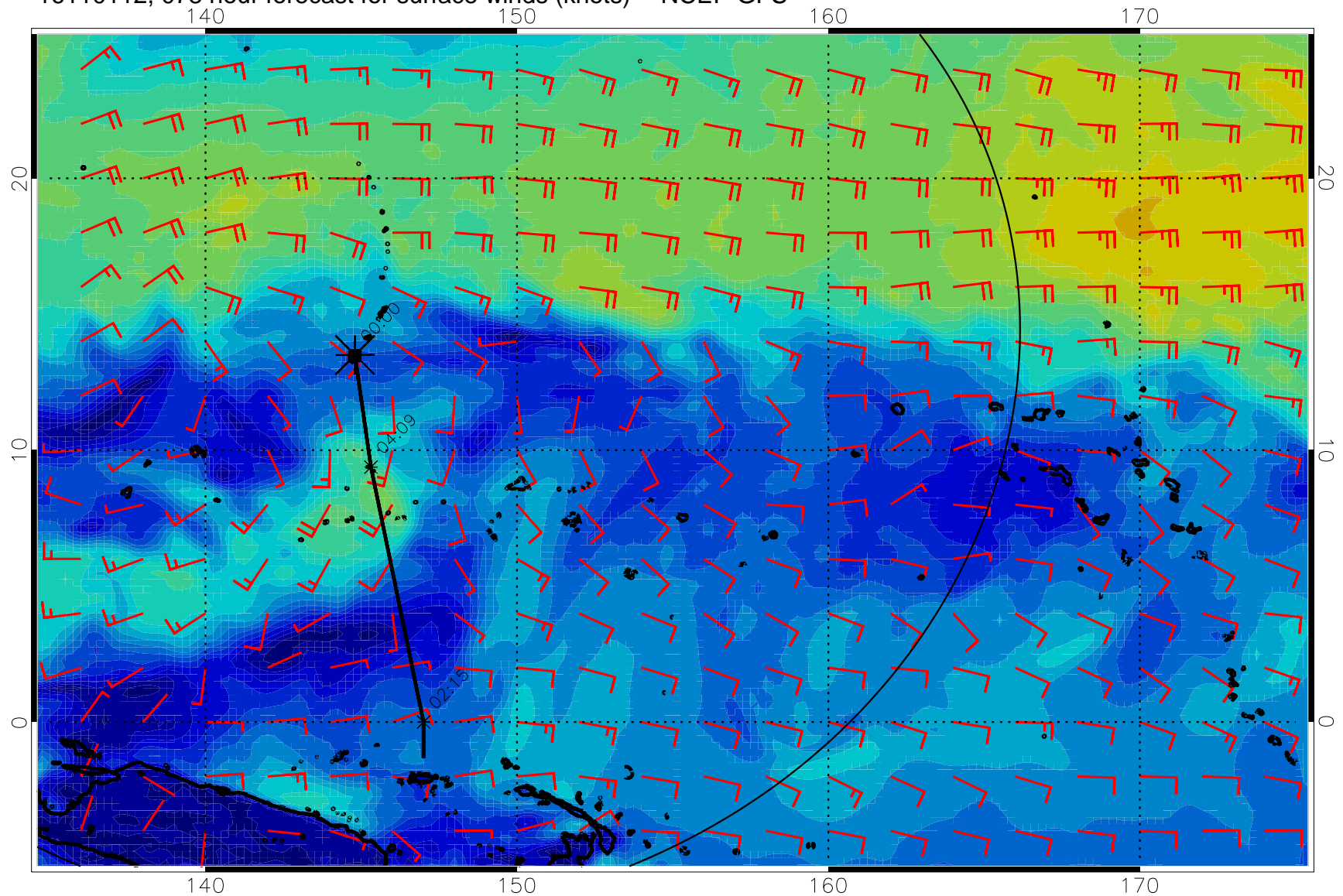
16110112, 078 hour forecast for surface winds (knots) -- NCEP GFS
