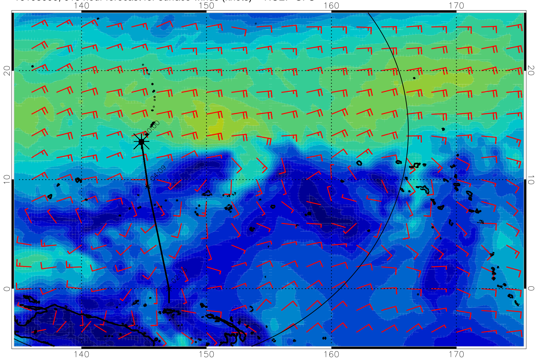
16103000, 018 hour forecast for surface winds (knots) -- NCEP GFS
