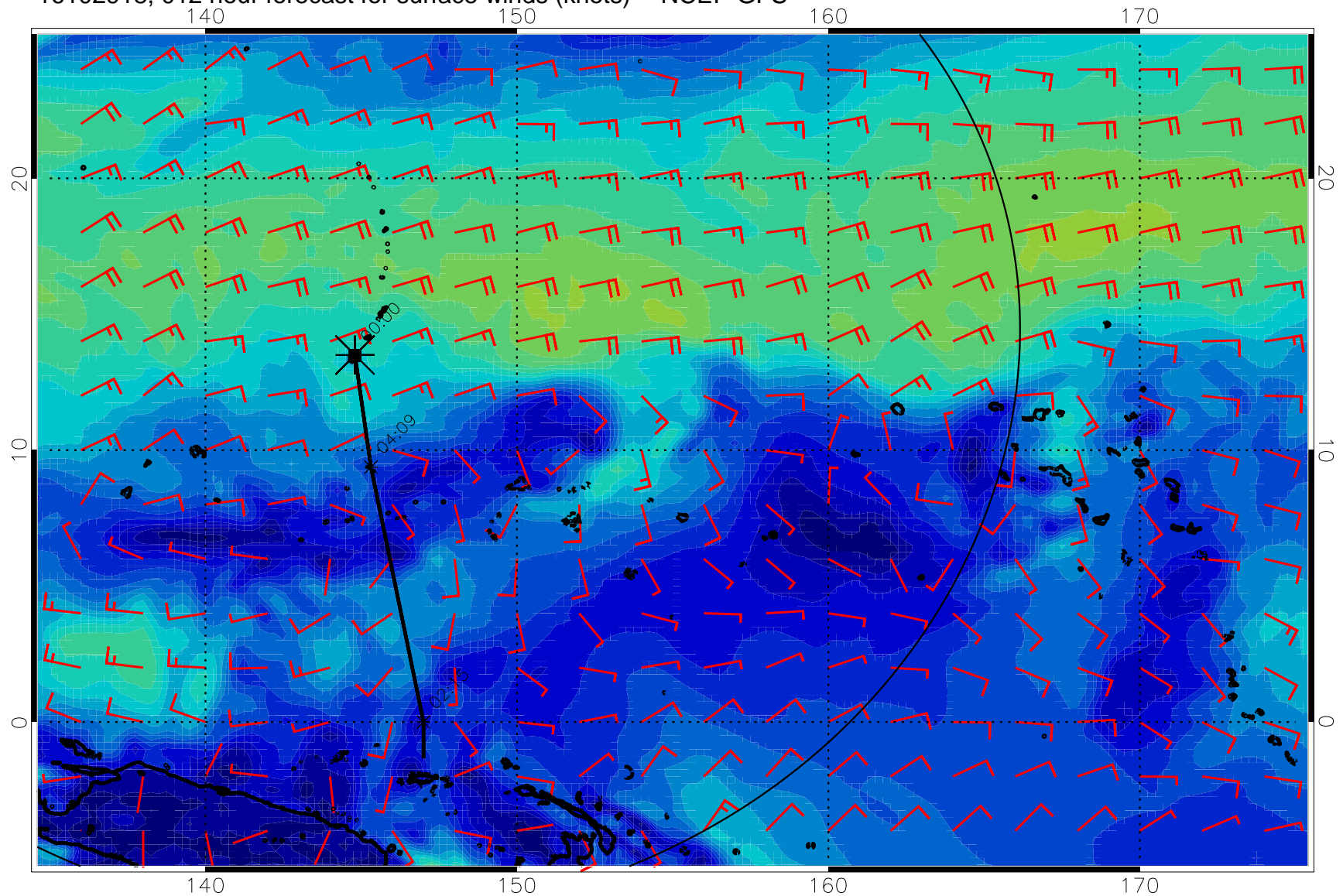
16102918, 012 hour forecast for surface winds (knots) -- NCEP GFS
