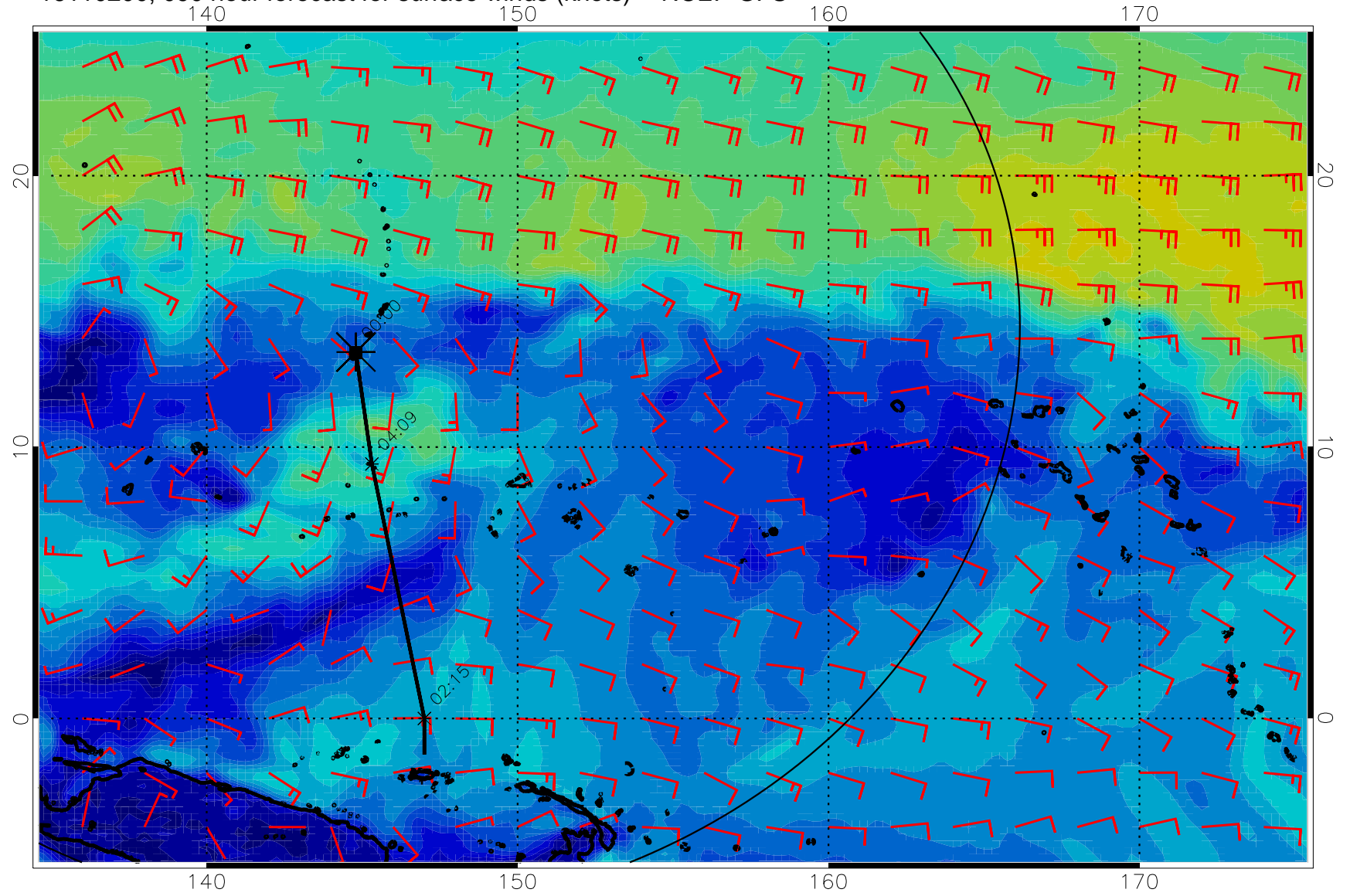
16110200, 090 hour forecast for surface winds (knots) -- NCEP GFS
