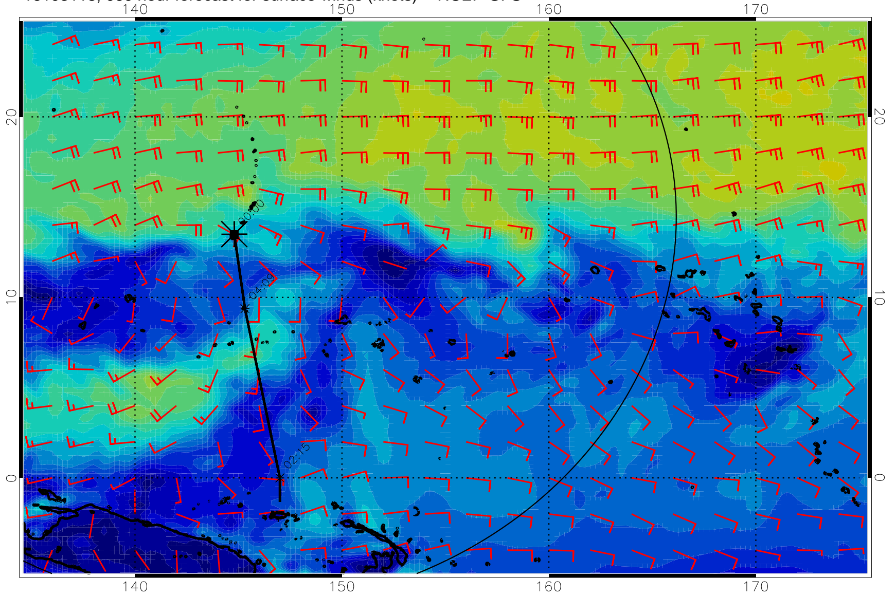
16103118, 060 hour forecast for surface winds (knots) -- NCEP GFS
