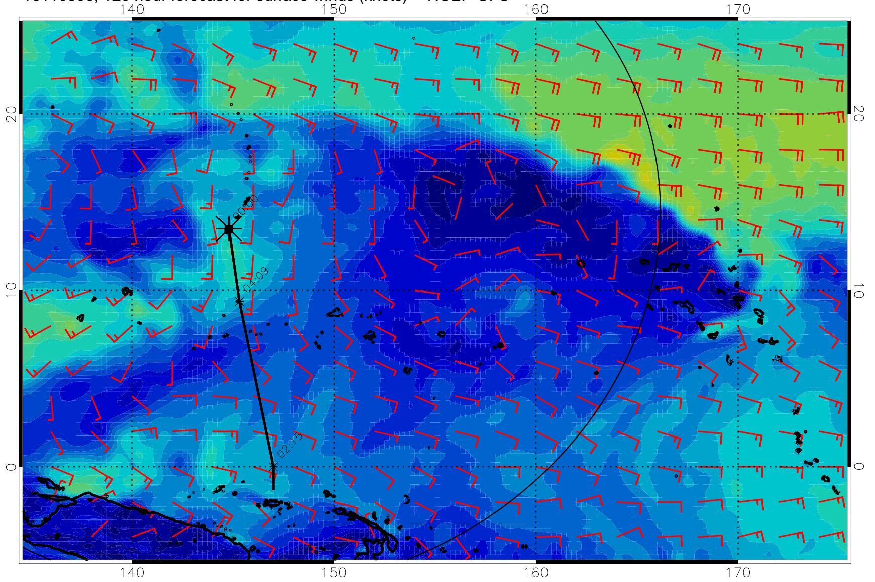
16110306, 120 hour forecast for surface winds (knots) -- NCEP GFS
