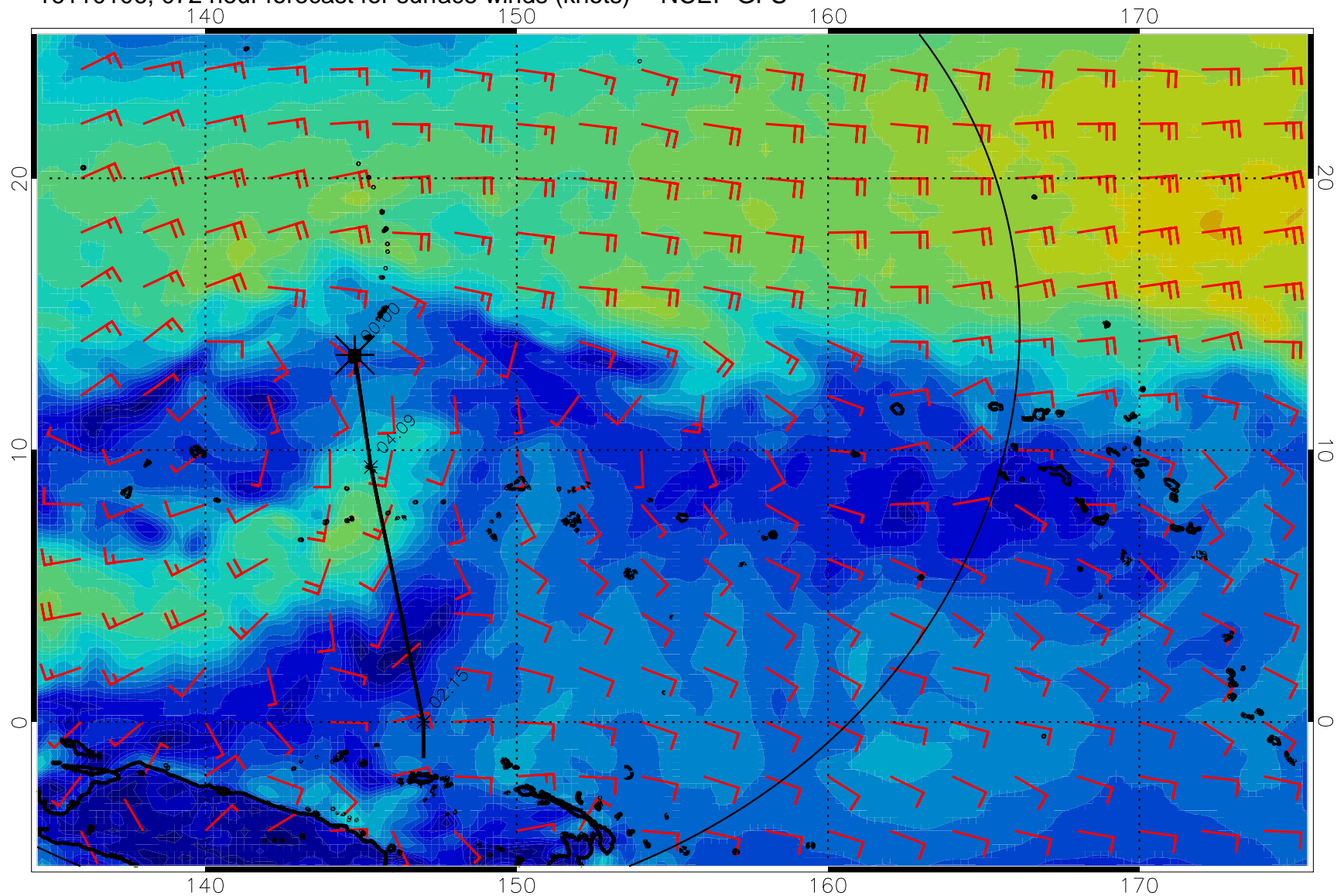
16110106, 072 hour forecast for surface winds (knots) -- NCEP GFS
