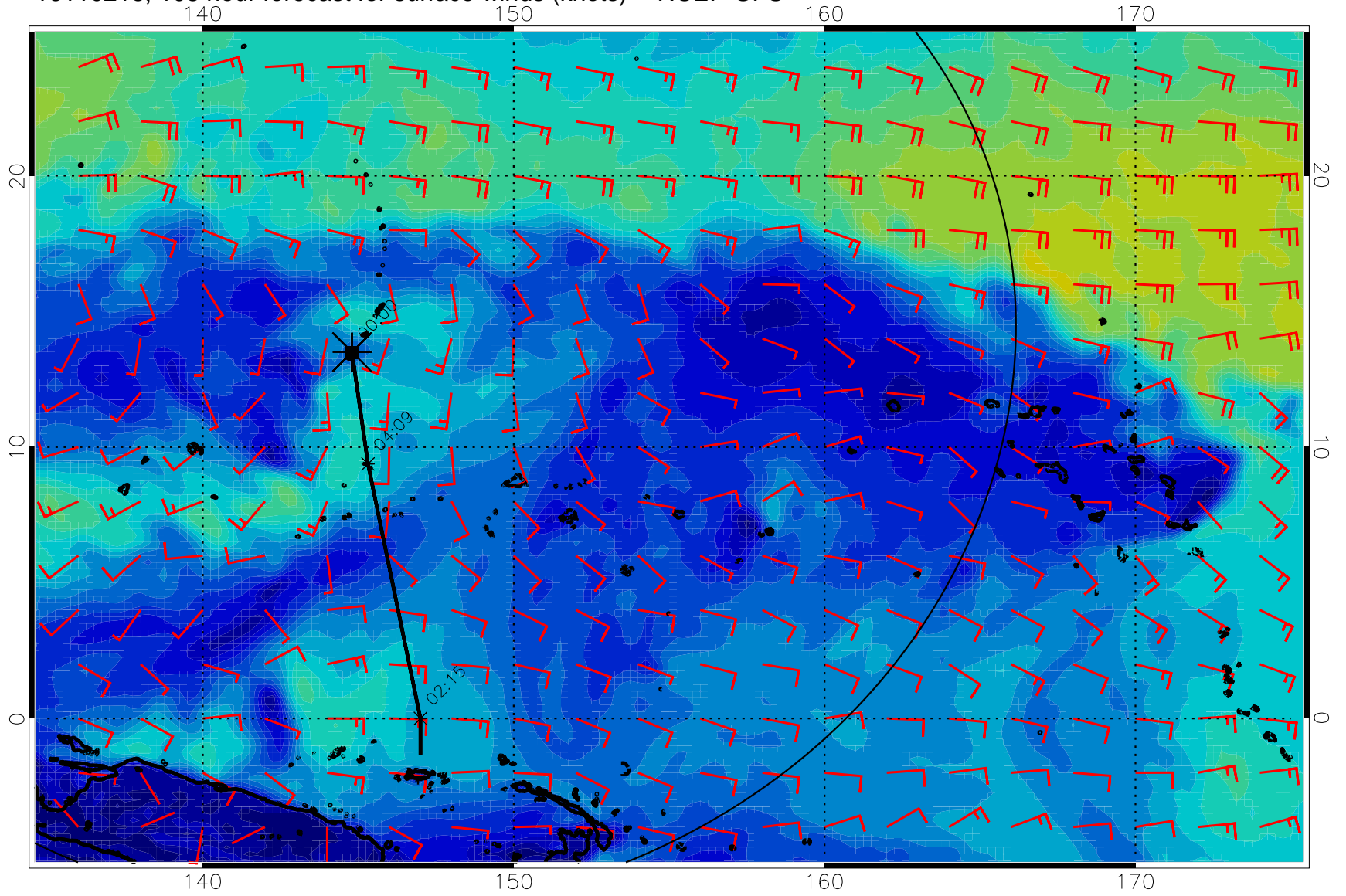
16110218, 108 hour forecast for surface winds (knots) -- NCEP GFS
