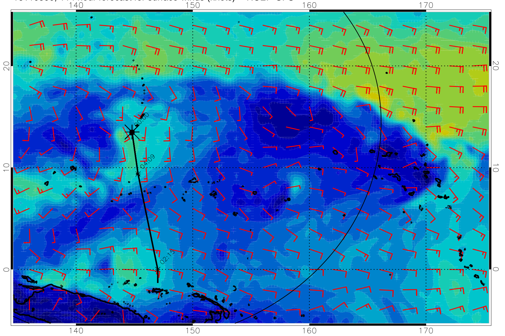
16110300, 114 hour forecast for surface winds (knots) -- NCEP GFS
