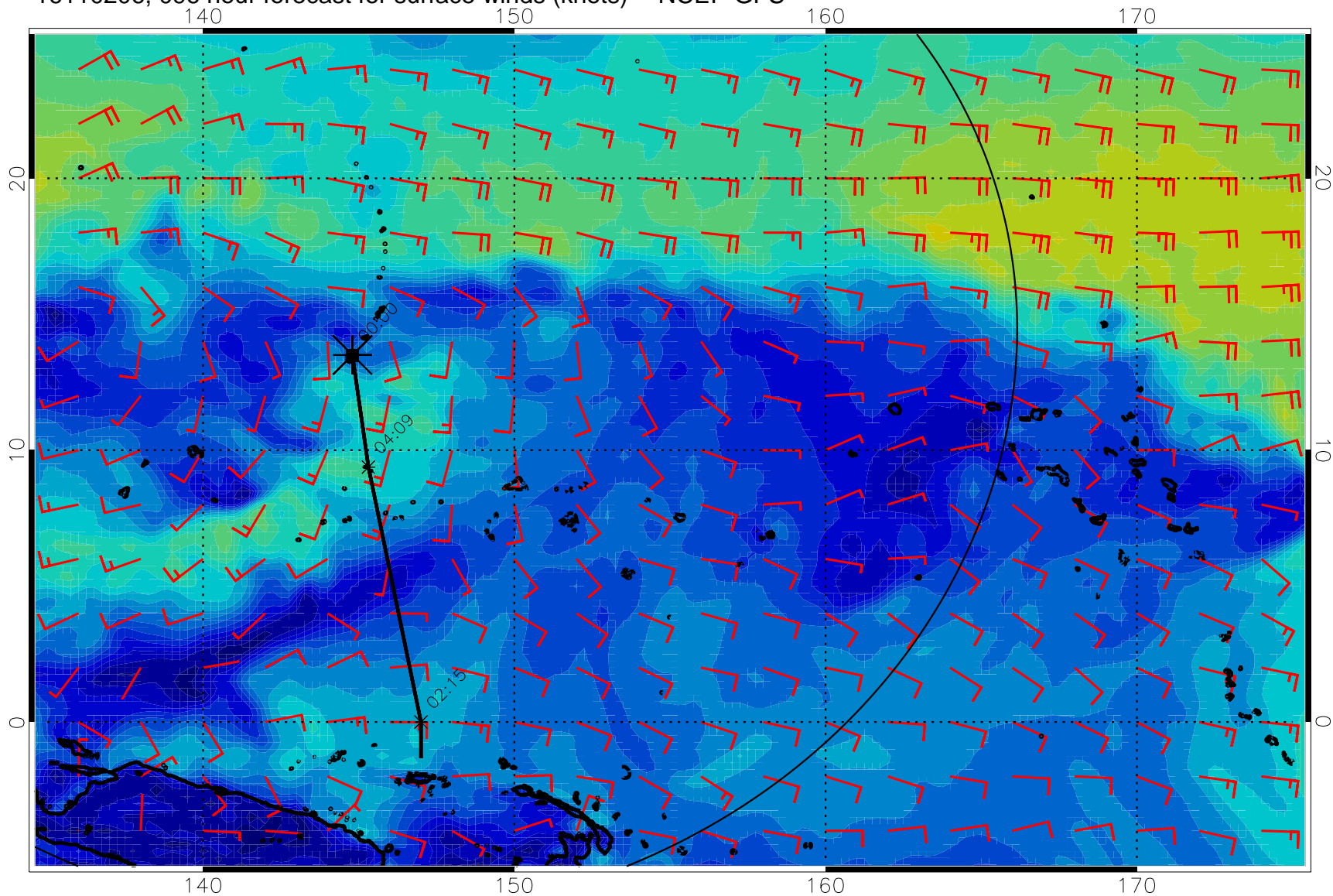
16110206, 096 hour forecast for surface winds (knots) -- NCEP GFS
