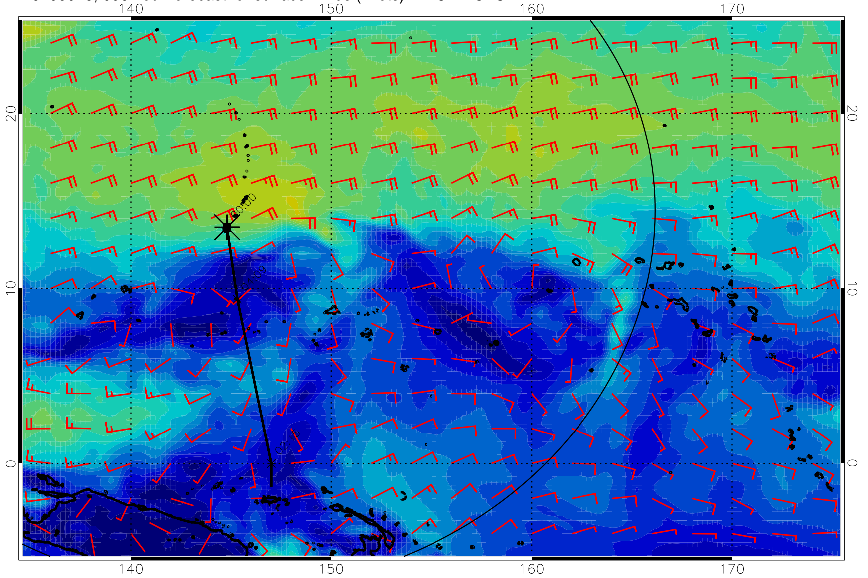
16103018, 036 hour forecast for surface winds (knots) -- NCEP GFS
