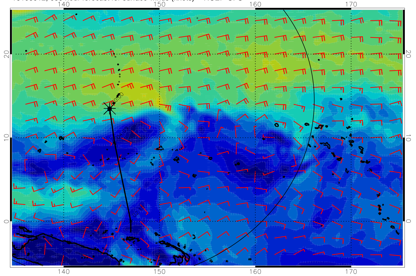
16103012, 0300 hour forecast for surface winds (knots) -- NCEP GFS
