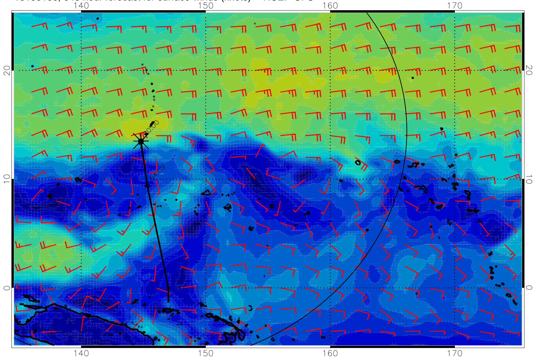
16103106, 048 hour forecast for surface winds (knots) -- NCEP GFS
