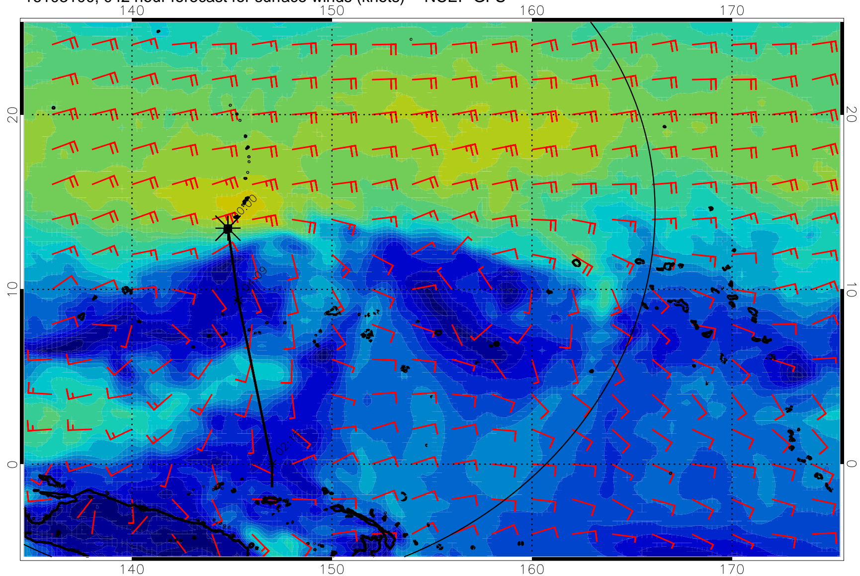
16103100, 042 hour forecast for surface winds (knots) -- NCEP GFS
