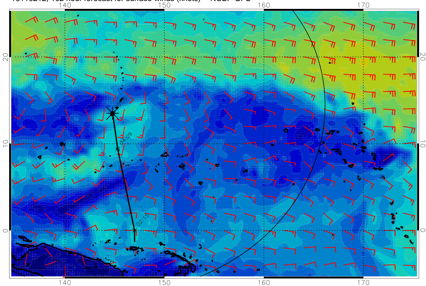
16110212, 102 hour forecast for surface winds (knots) -- NCEP GFS
