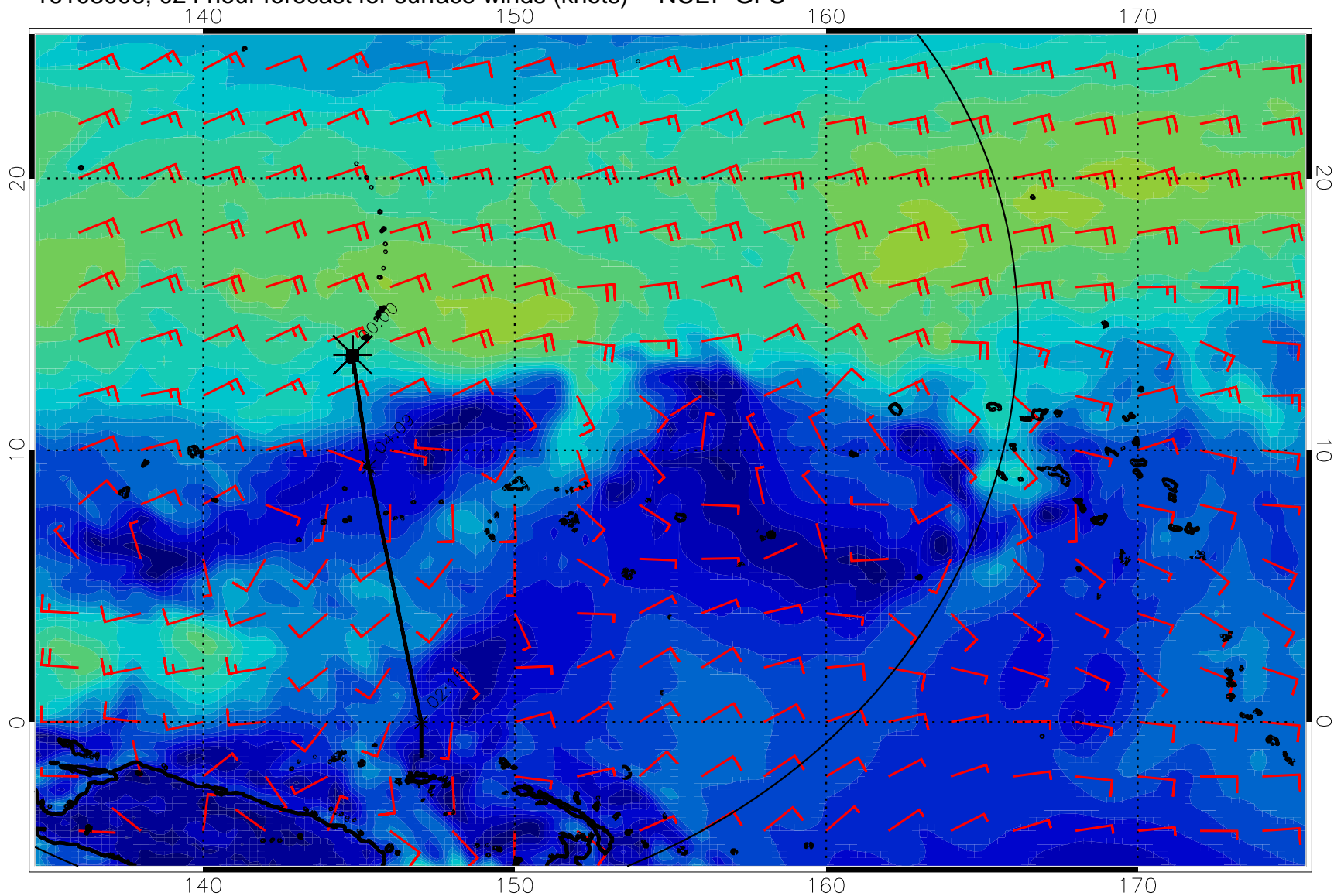
16103006, 024 hour forecast for surface winds (knots) -- NCEP GFS
