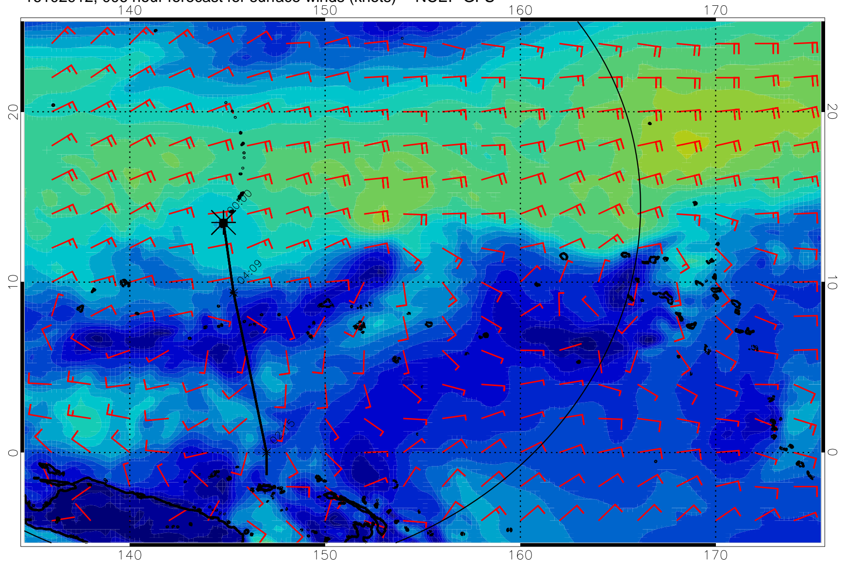
16102912, 006 hour forecast for surface winds (knots) -- NCEP GFS
