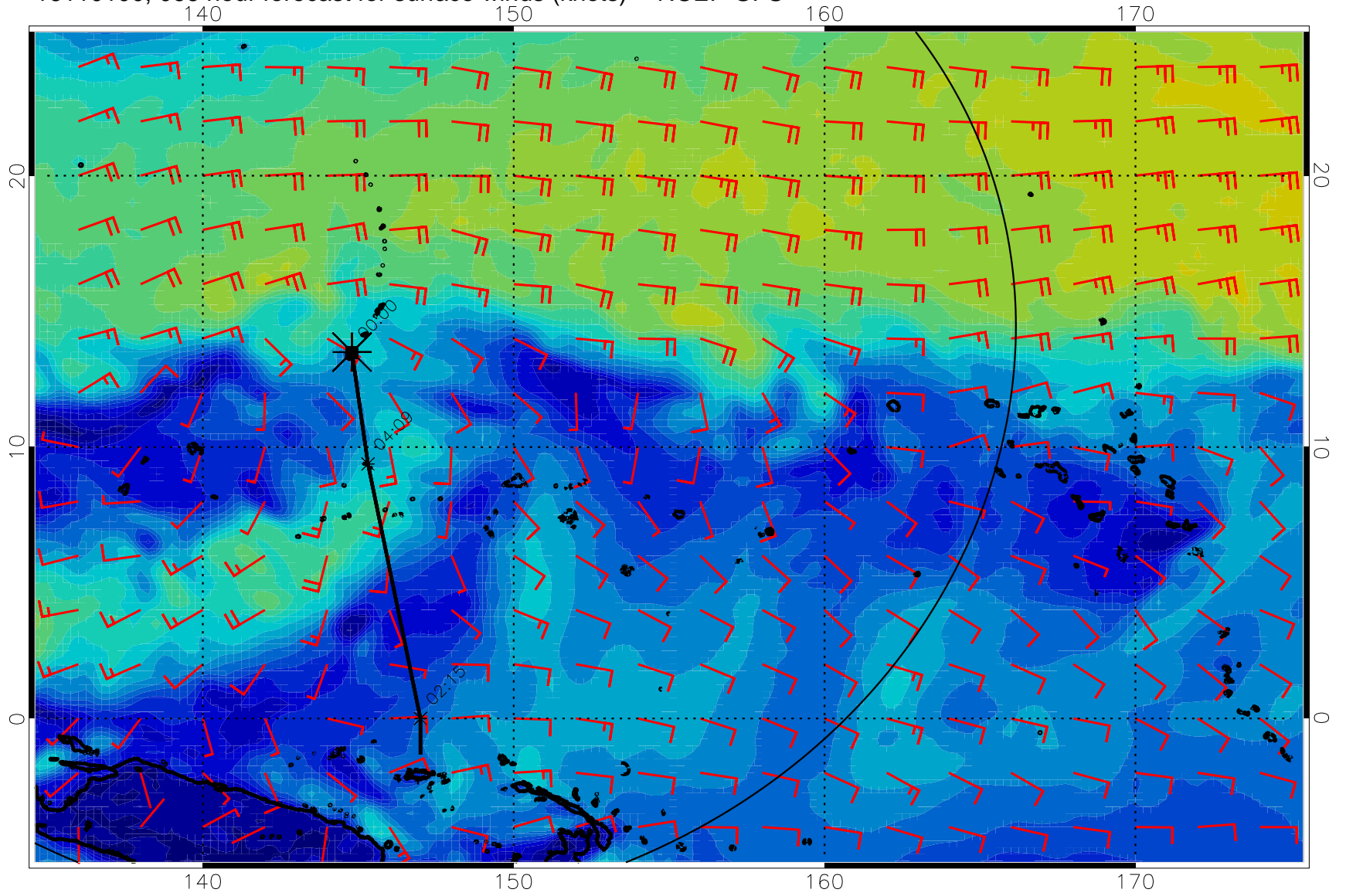
16110100, 066 hour forecast for surface winds (knots) -- NCEP GFS
