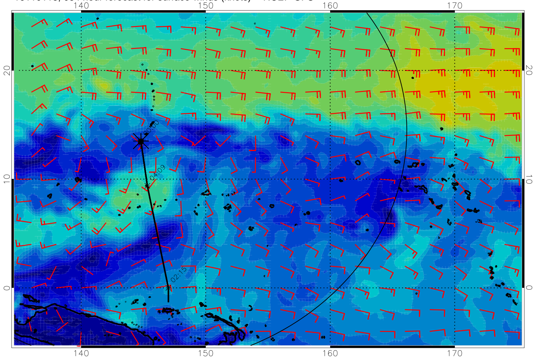
16110118, 084 hour forecast for surface winds (knots) -- NCEP GFS
