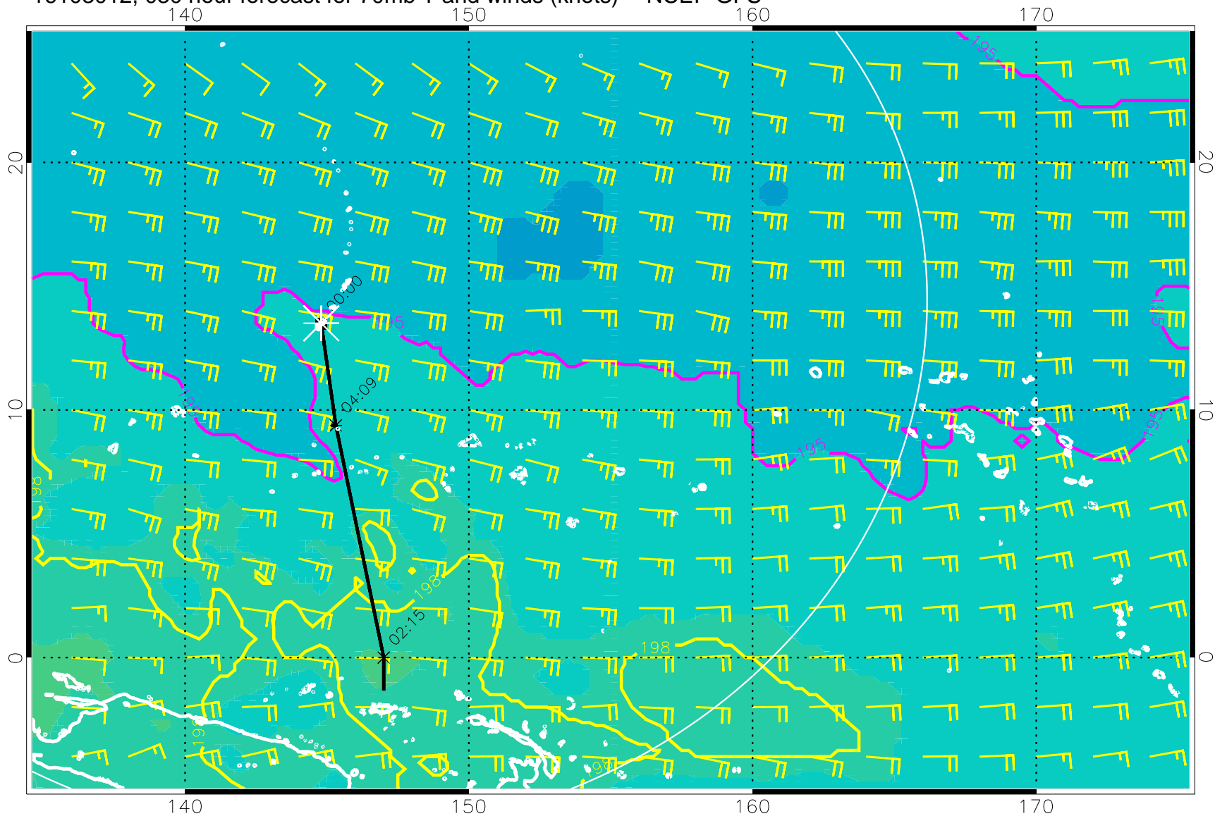
16103012, 030 hour forecast for 70mb T and winds (knots) -- NCEP GFS
