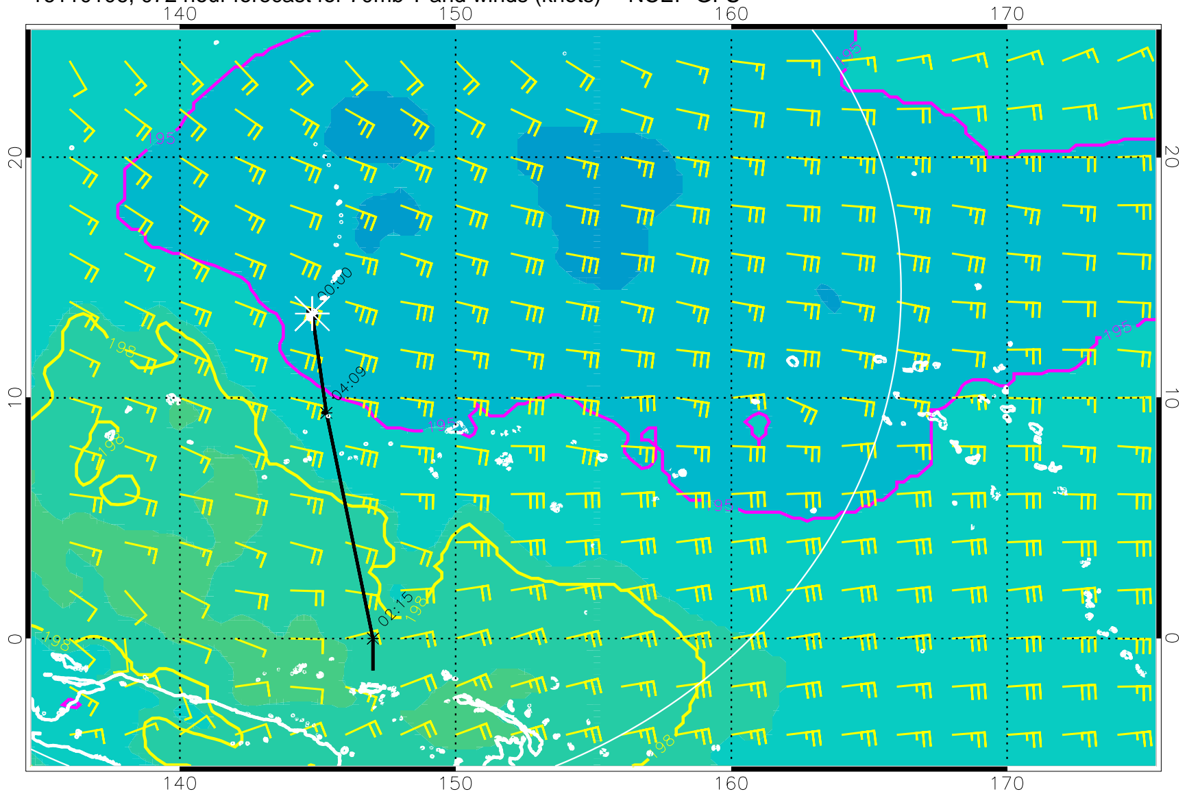
16110106, 072 hour forecast for 70mb T and winds (knots) -- NCEP GFS
