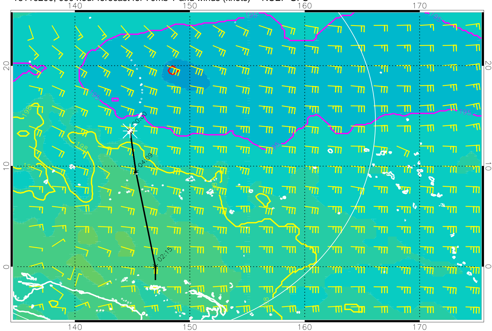
16110200, 090 hour forecast for 70mb T and winds (knots) -- NCEP GFS
