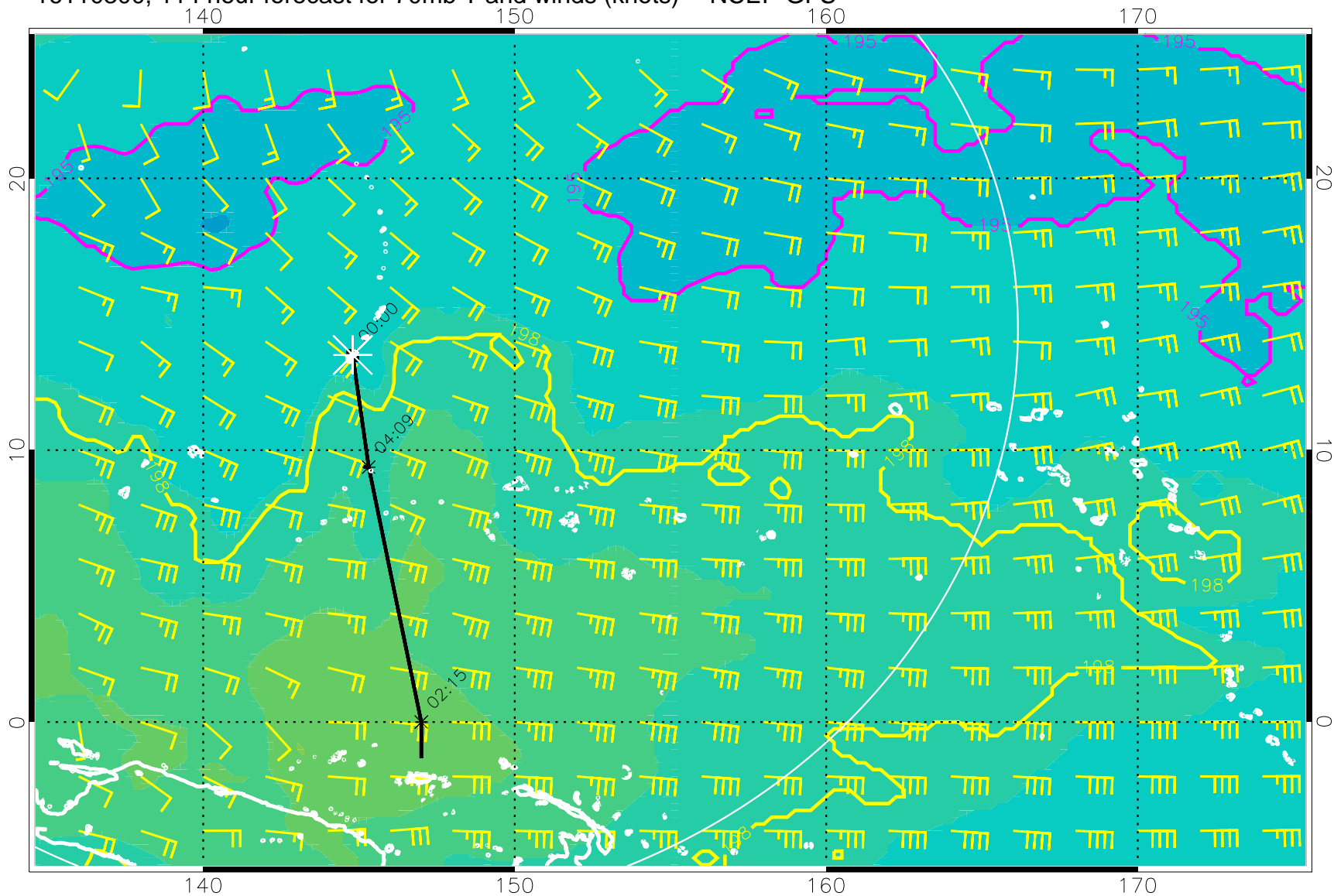
16110300, 114 hour forecast for 70mb T and winds (knots) -- NCEP GFS
