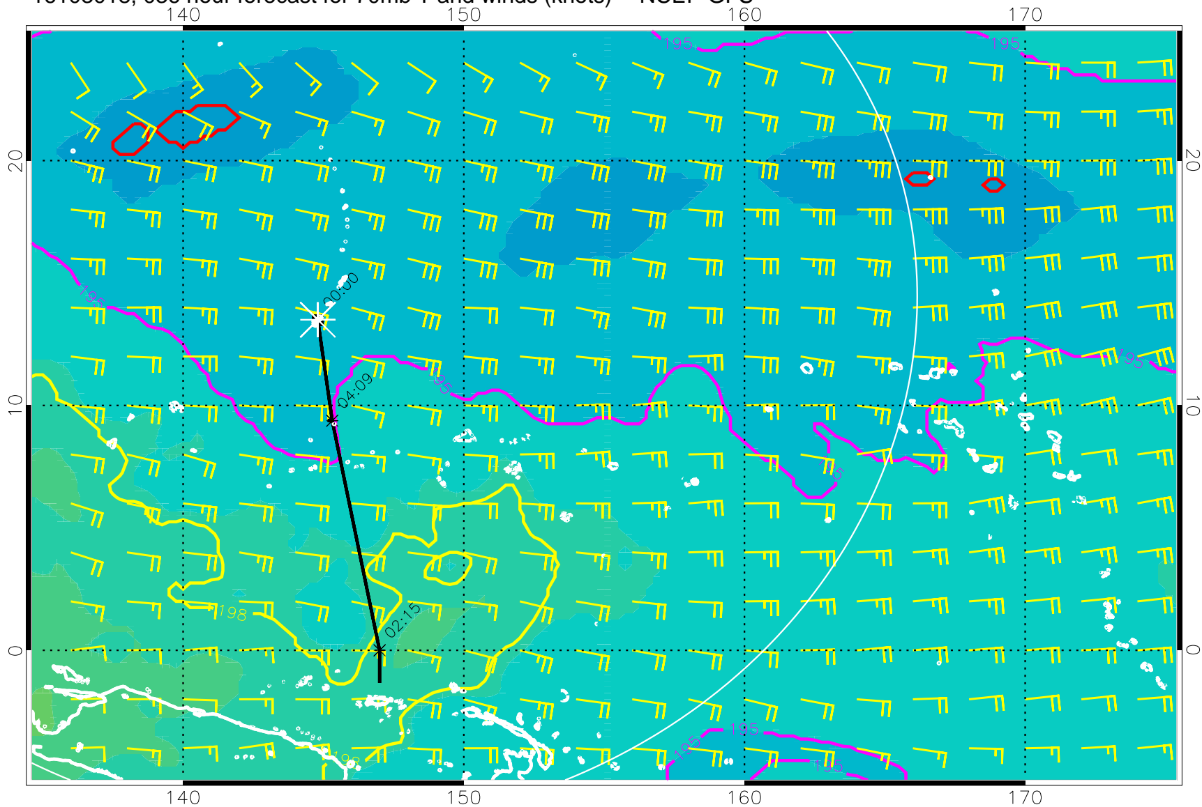
16103018, 036 hour forecast for 70mb T and winds (knots) -- NCEP GFS
