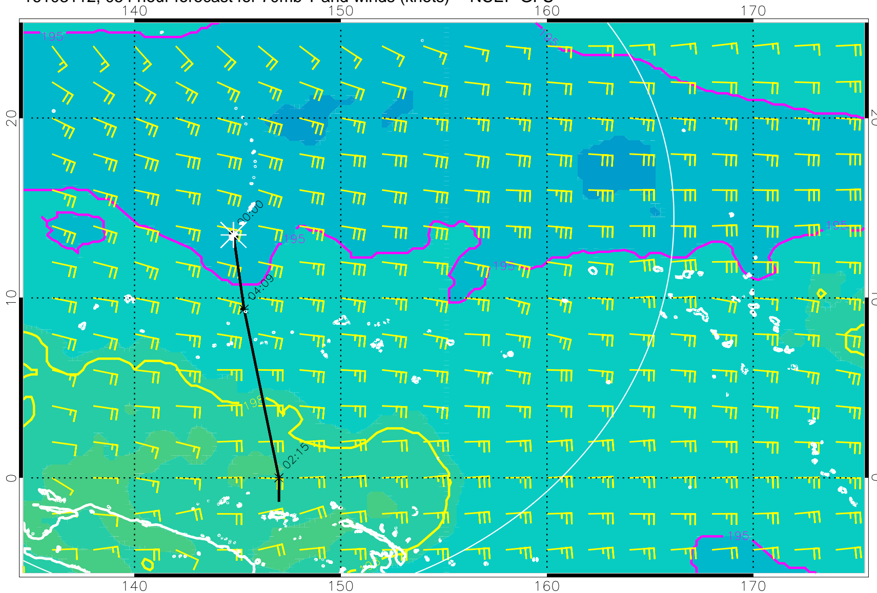
16103112, 054 hour forecast for 70mb T and winds (knots) -- NCEP GFS
