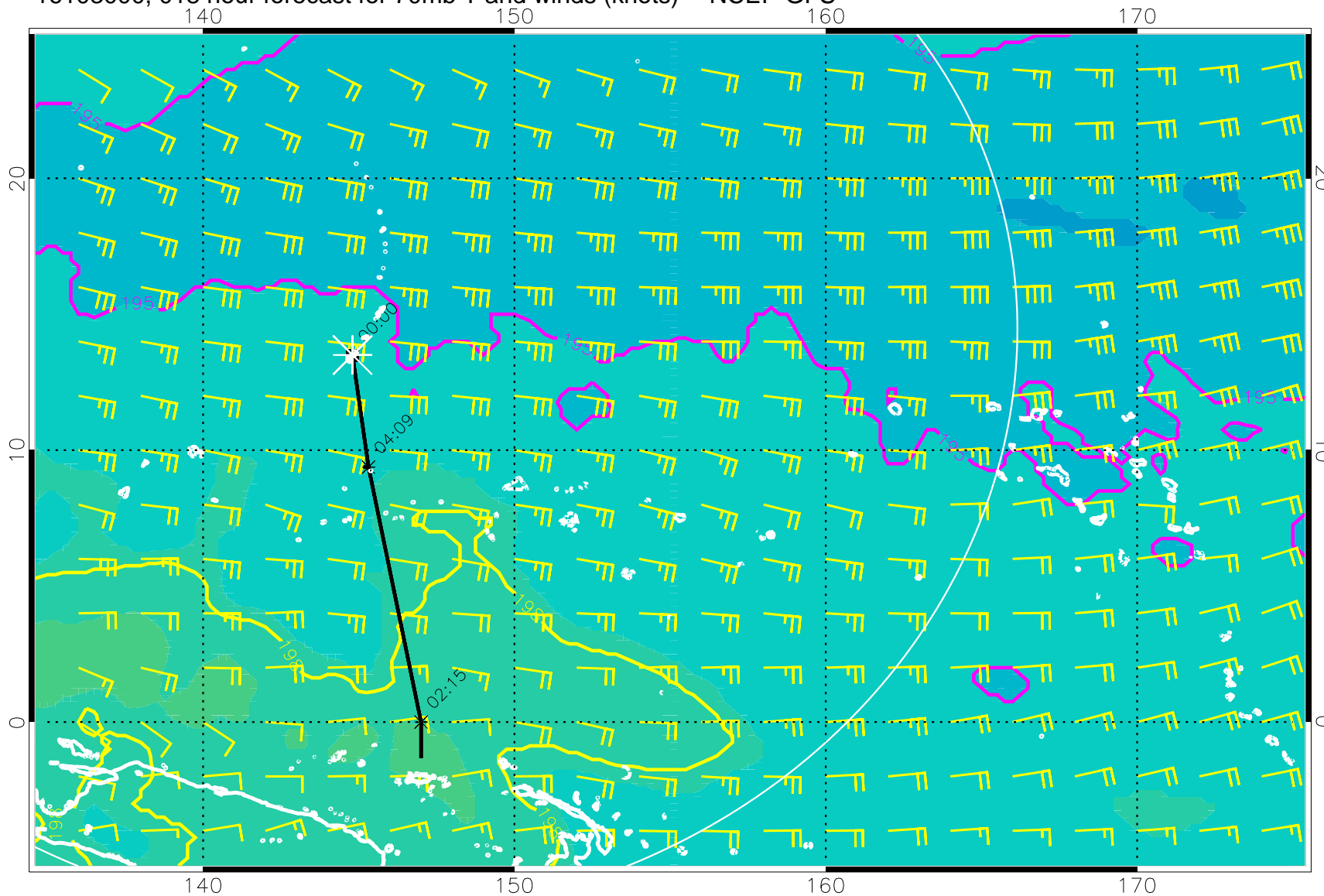
16103000, 018 hour forecast for 70mb T and winds (knots) -- NCEP GFS
