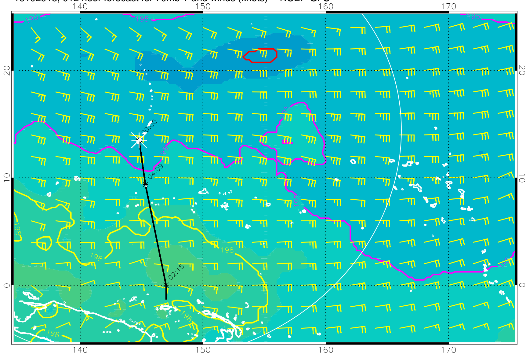
16102918, 012 hour forecast for 70mb T and winds (knots) -- NCEP GFS
