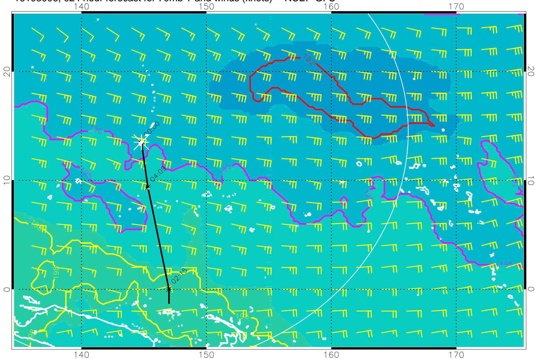
16103006, 024 hour forecast for 70mb T and winds (knots) -- NCEP GFS
