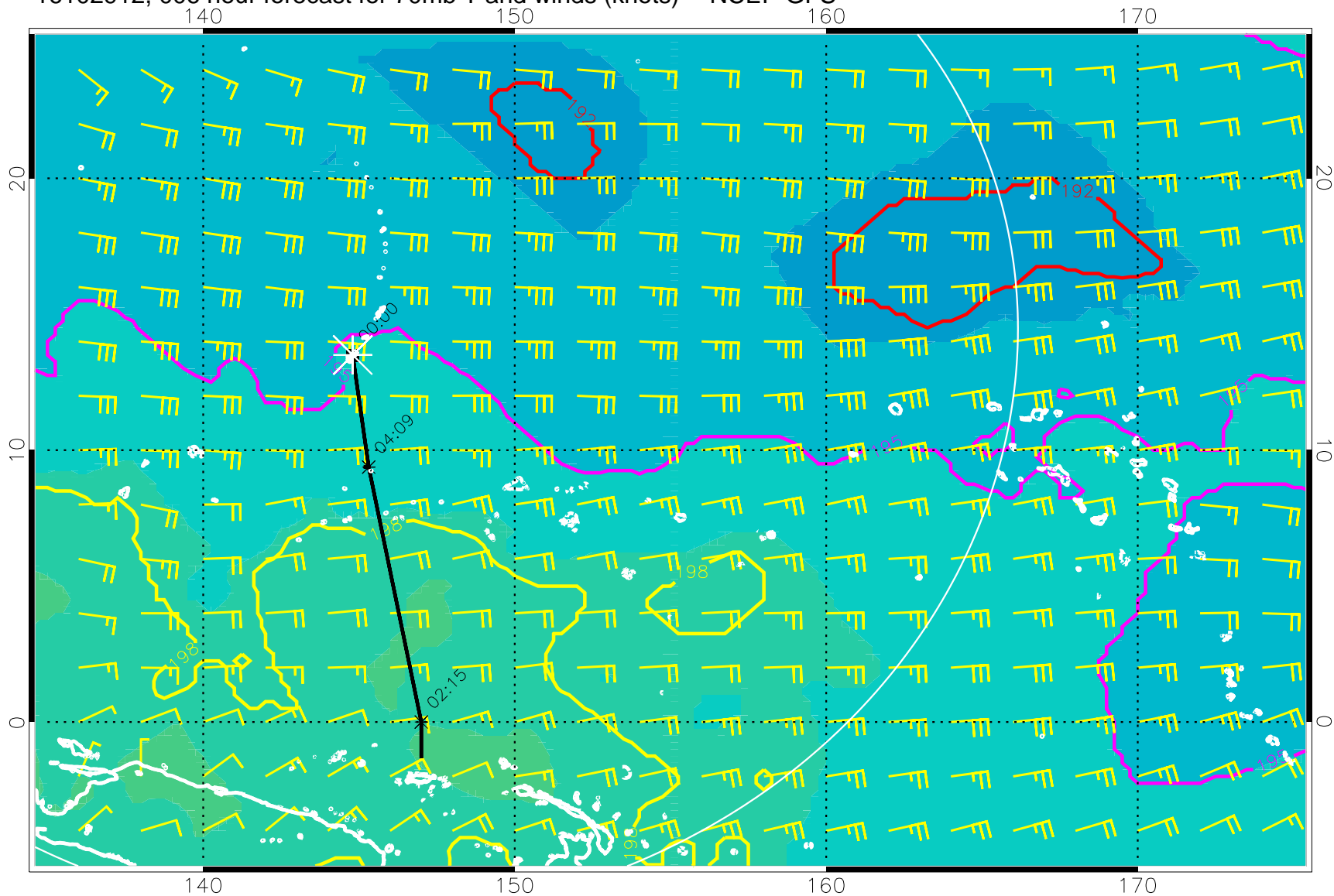
16102912, 006 hour forecast for 70mb T and winds (knots) -- NCEP GFS
