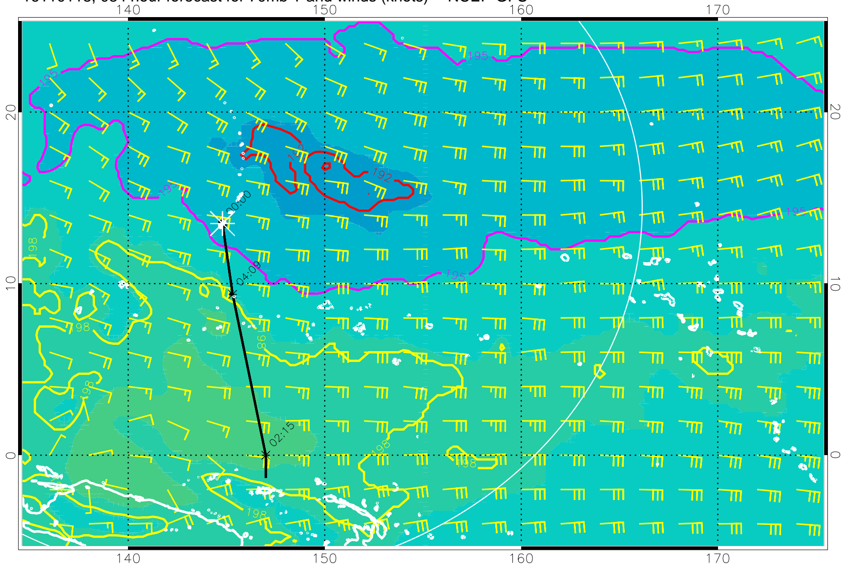
16110118, 084 hour forecast for 70mb T and winds (knots) -- NCEP GFS
