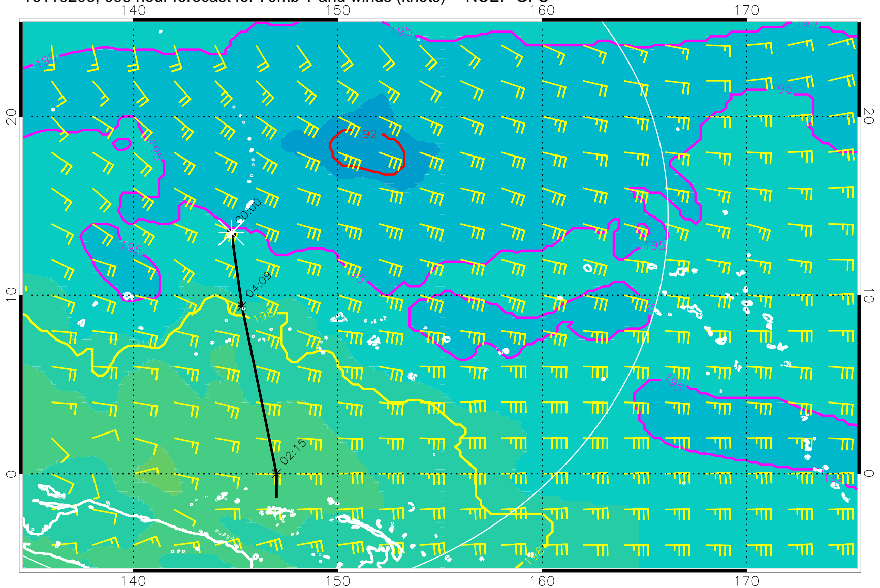
16110206, 096 hour forecast for 70mb T and winds (knots) -- NCEP GFS
