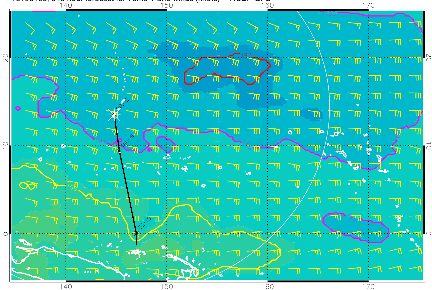
16103106, 048 hour forecast for 70mb T and winds (knots) -- NCEP GFS
