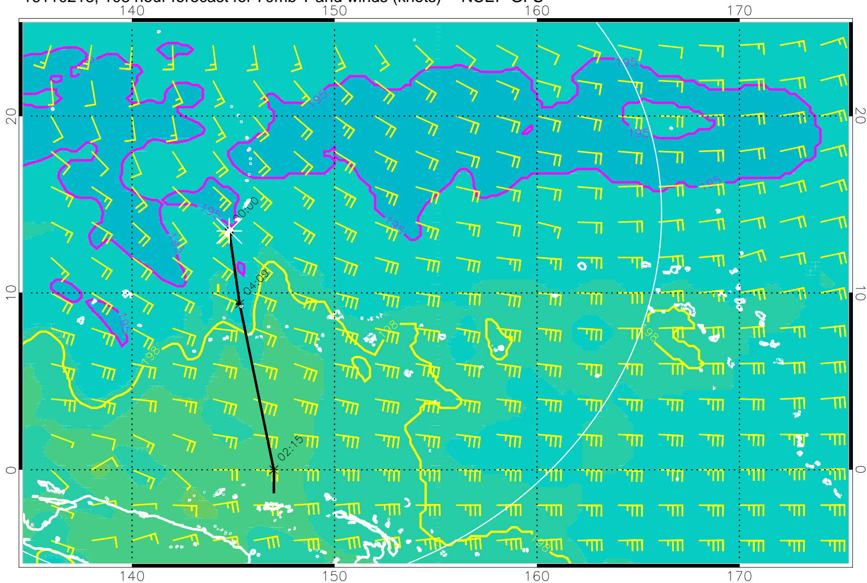
16110218, 108 hour forecast for 70mb T and winds (knots) -- NCEP GFS
