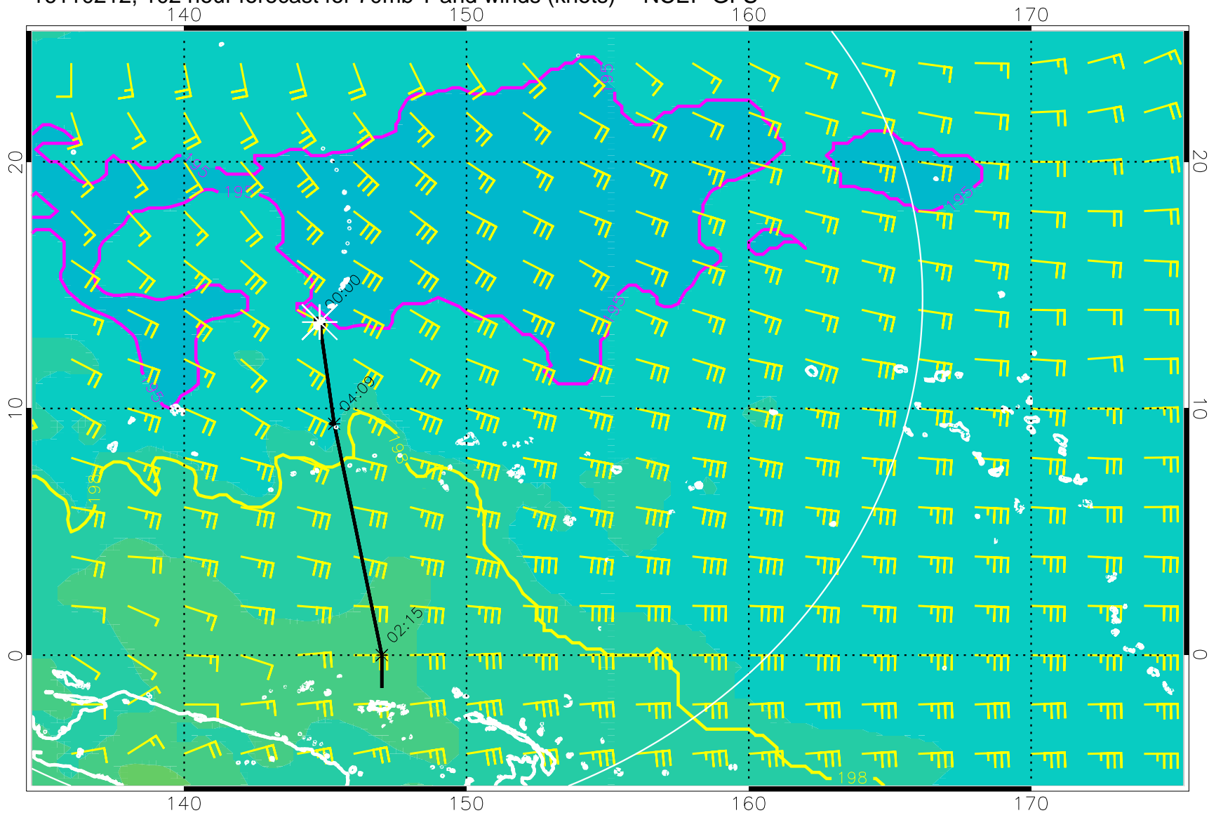
16110212, 102 hour forecast for 70mb T and winds (knots) -- NCEP GFS
