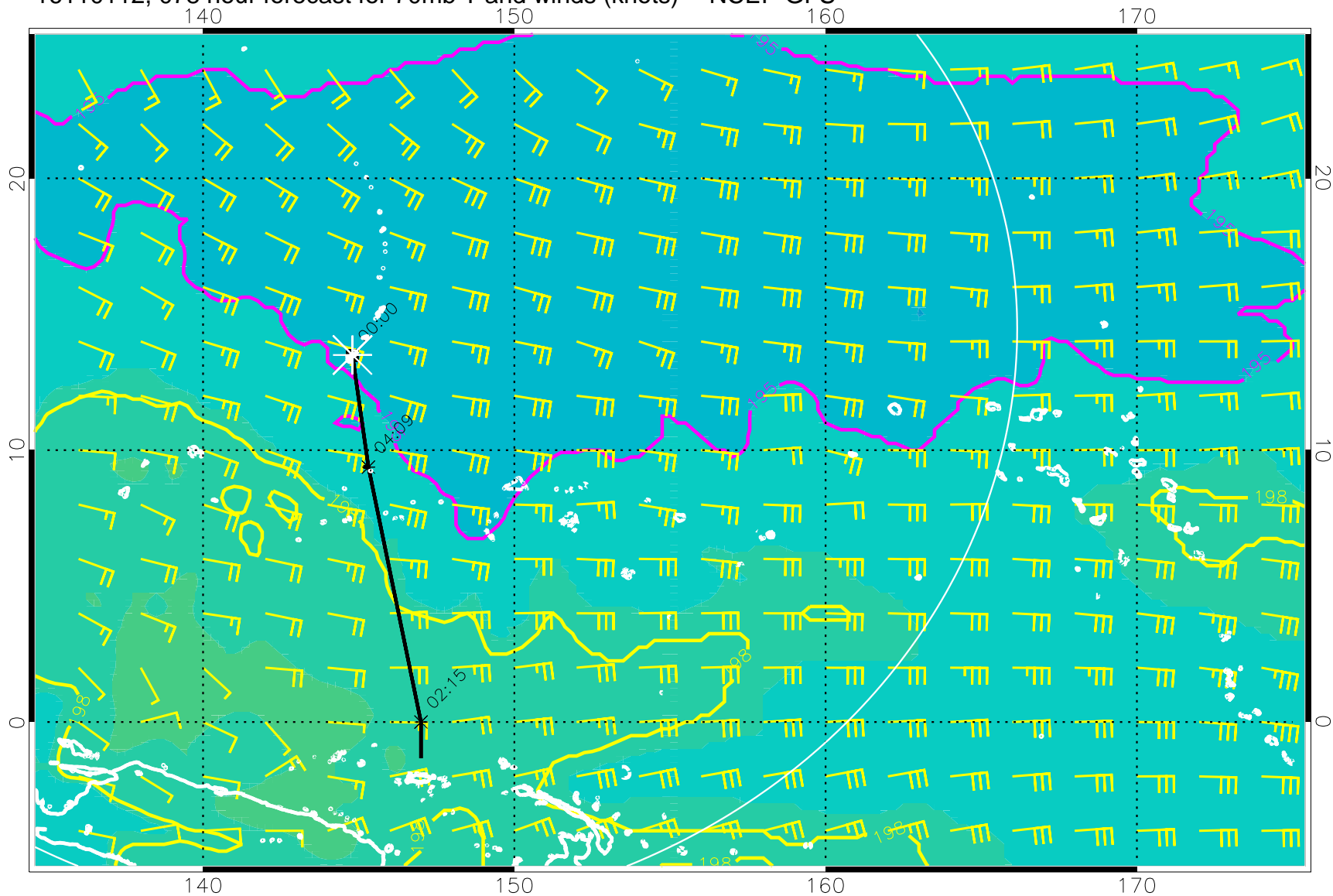
16110112, 078 hour forecast for 70mb T and winds (knots) -- NCEP GFS
