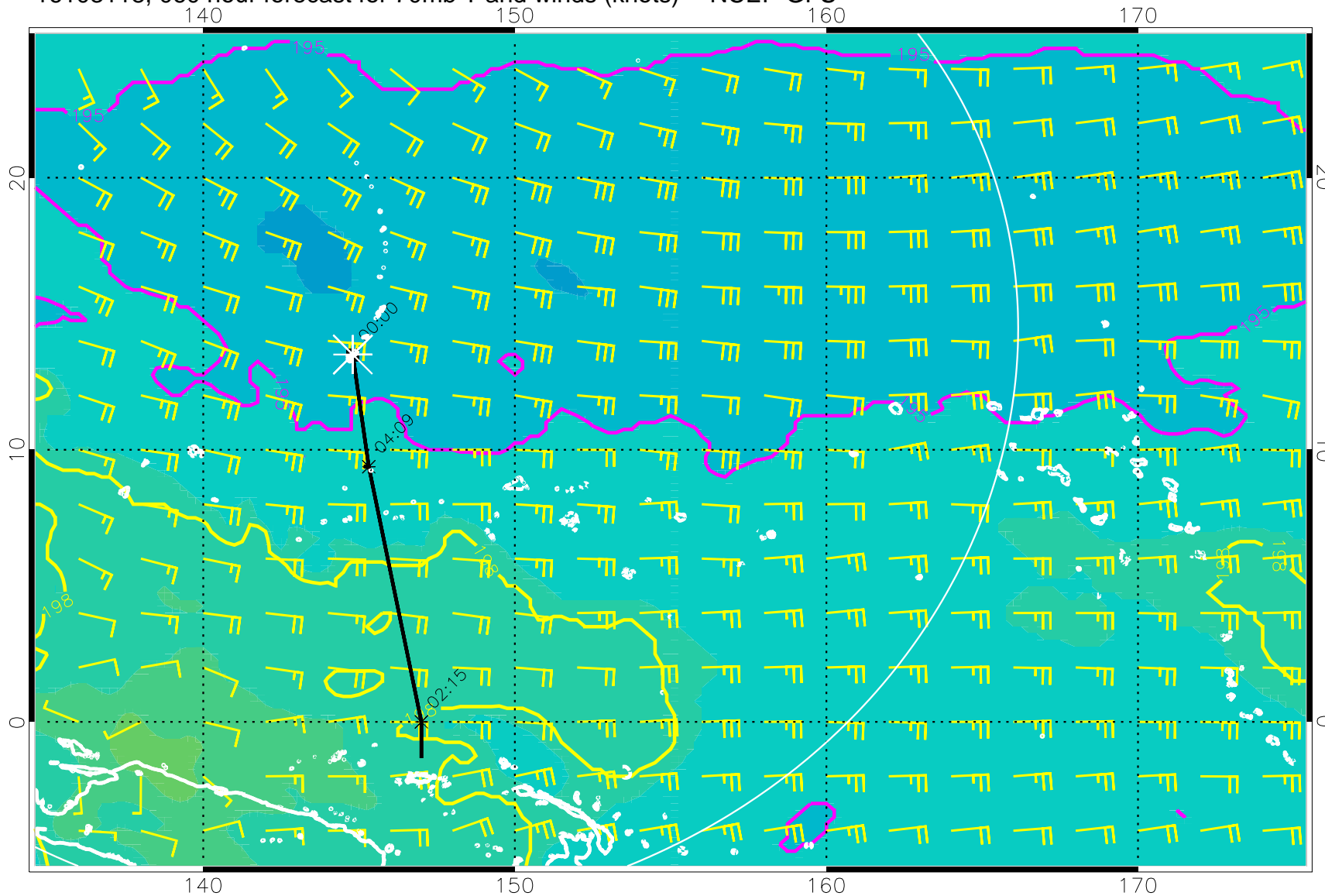
16103118, 060 hour forecast for 70mb T and winds (knots) -- NCEP GFS
