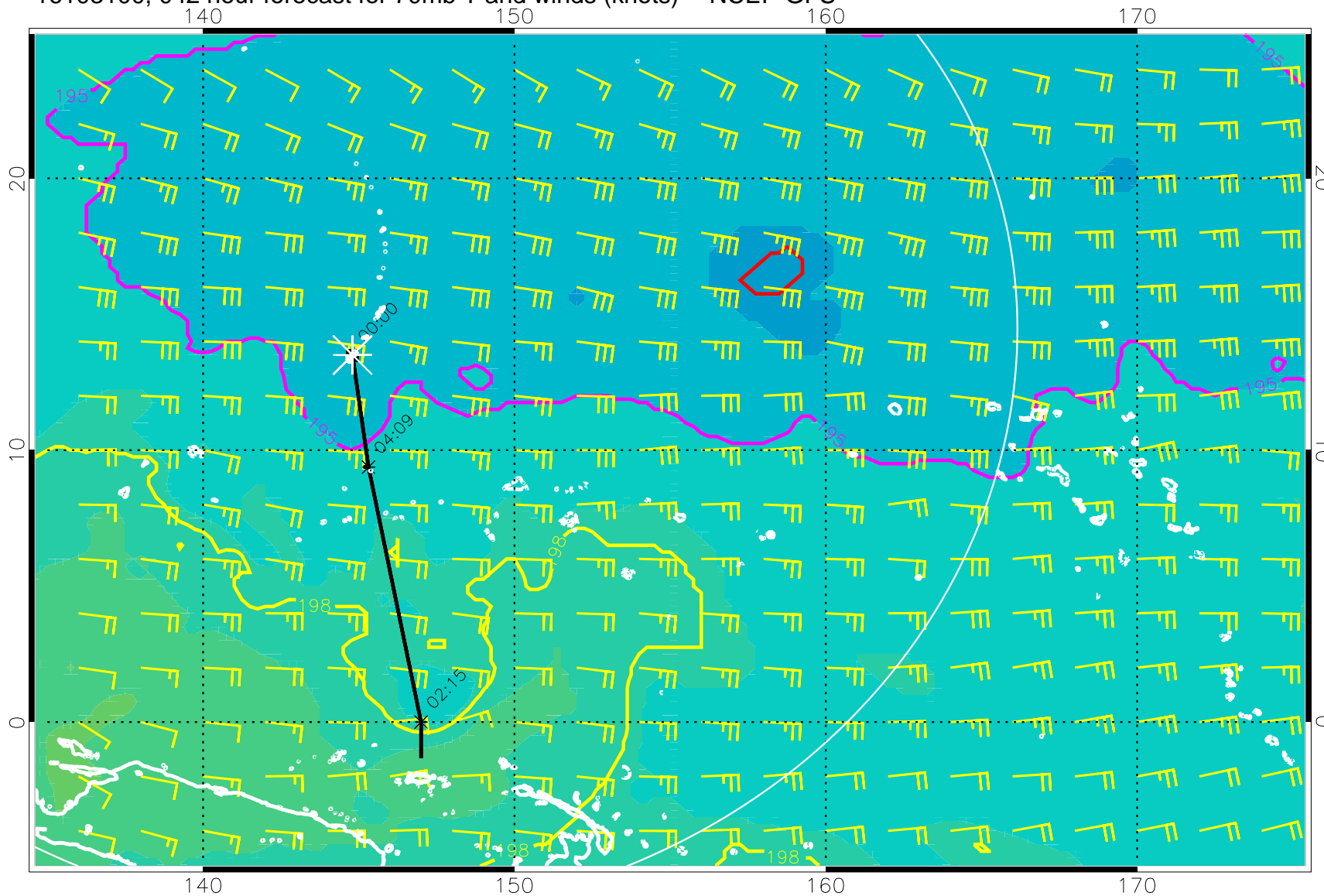
16103100, 042 hour forecast for 70mb T and winds (knots) -- NCEP GFS
