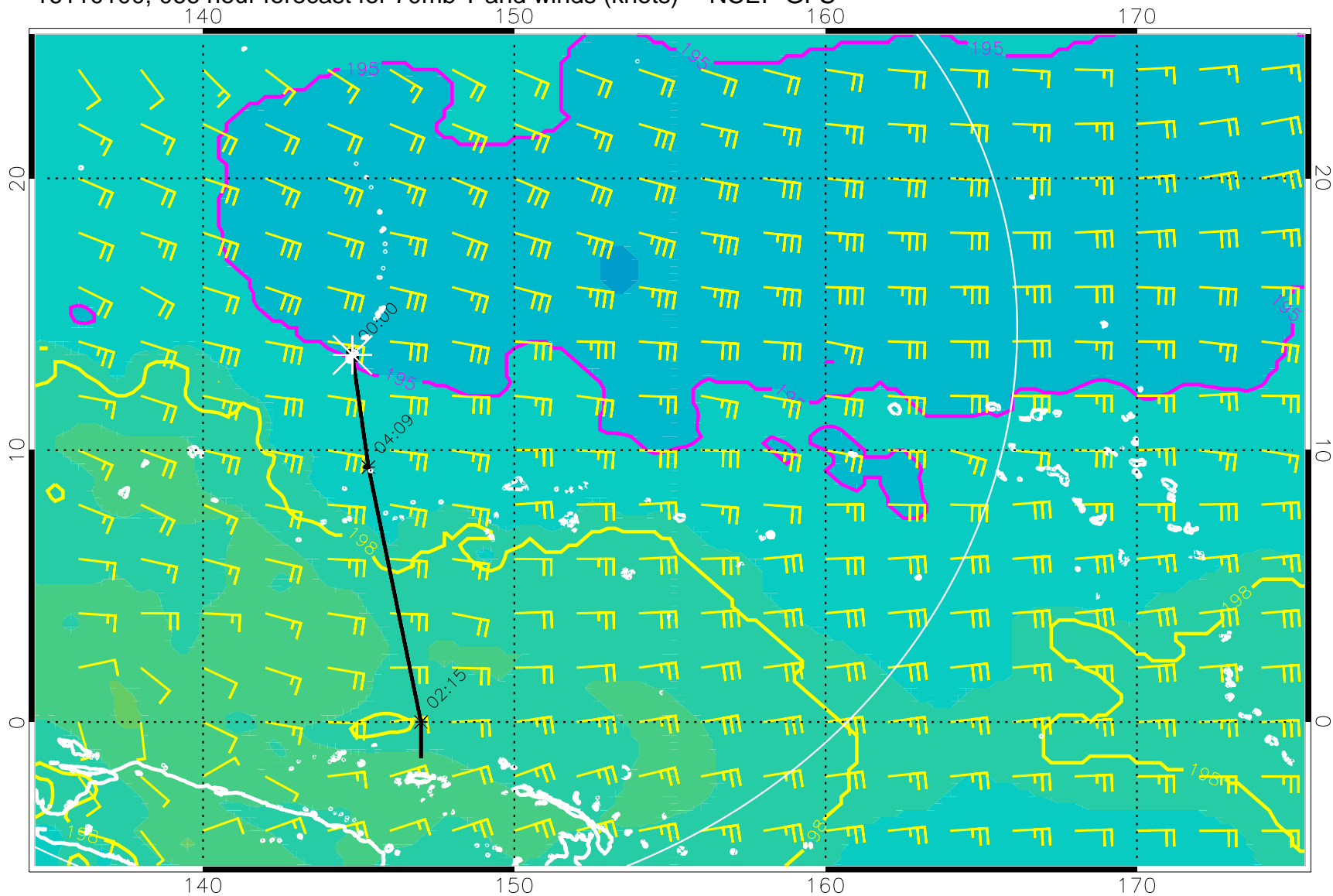
16110100, 066 hour forecast for 70mb T and winds (knots) -- NCEP GFS
