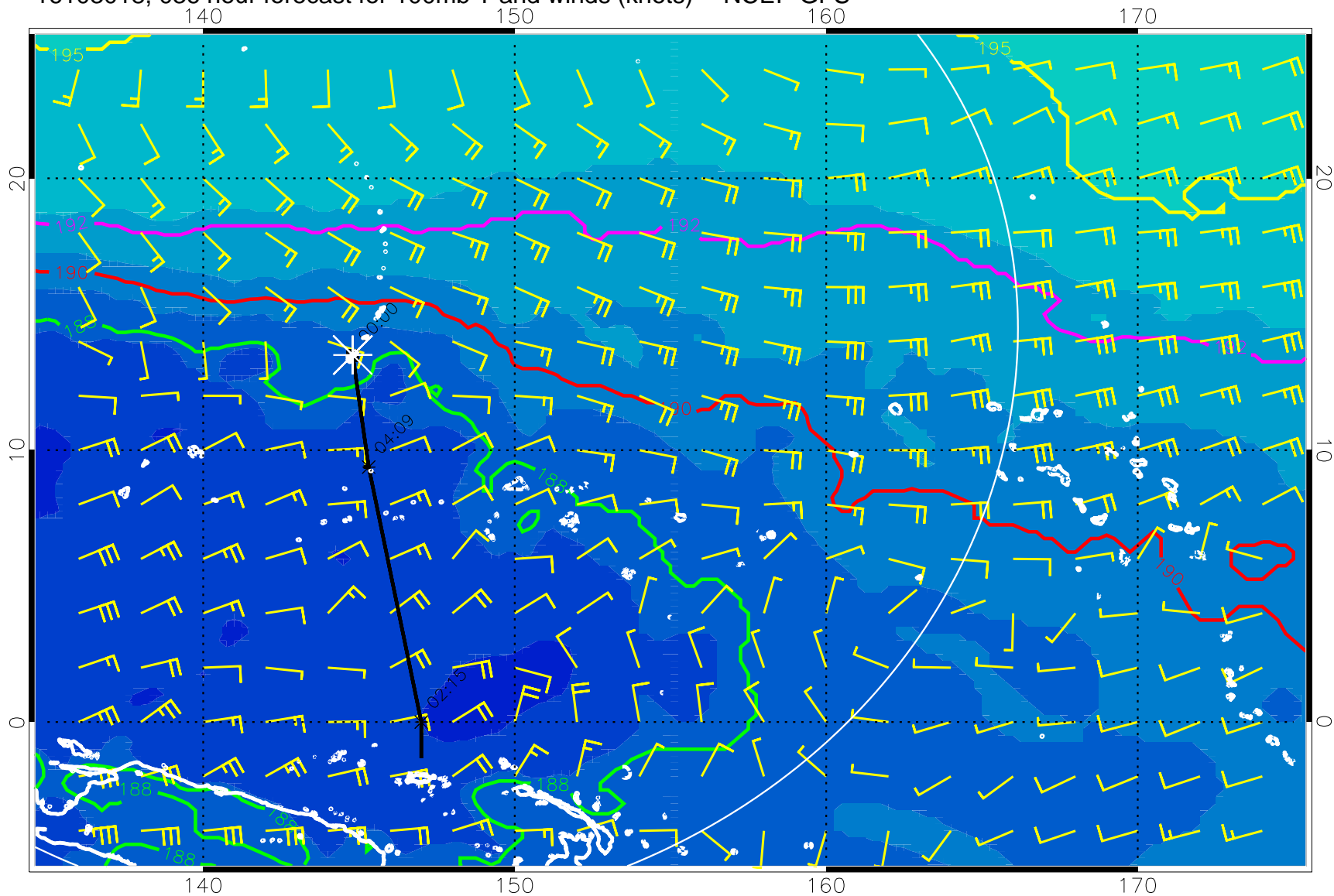
16103018, 036 hour forecast for 100mb T and winds (knots) -- NCEP GFS
