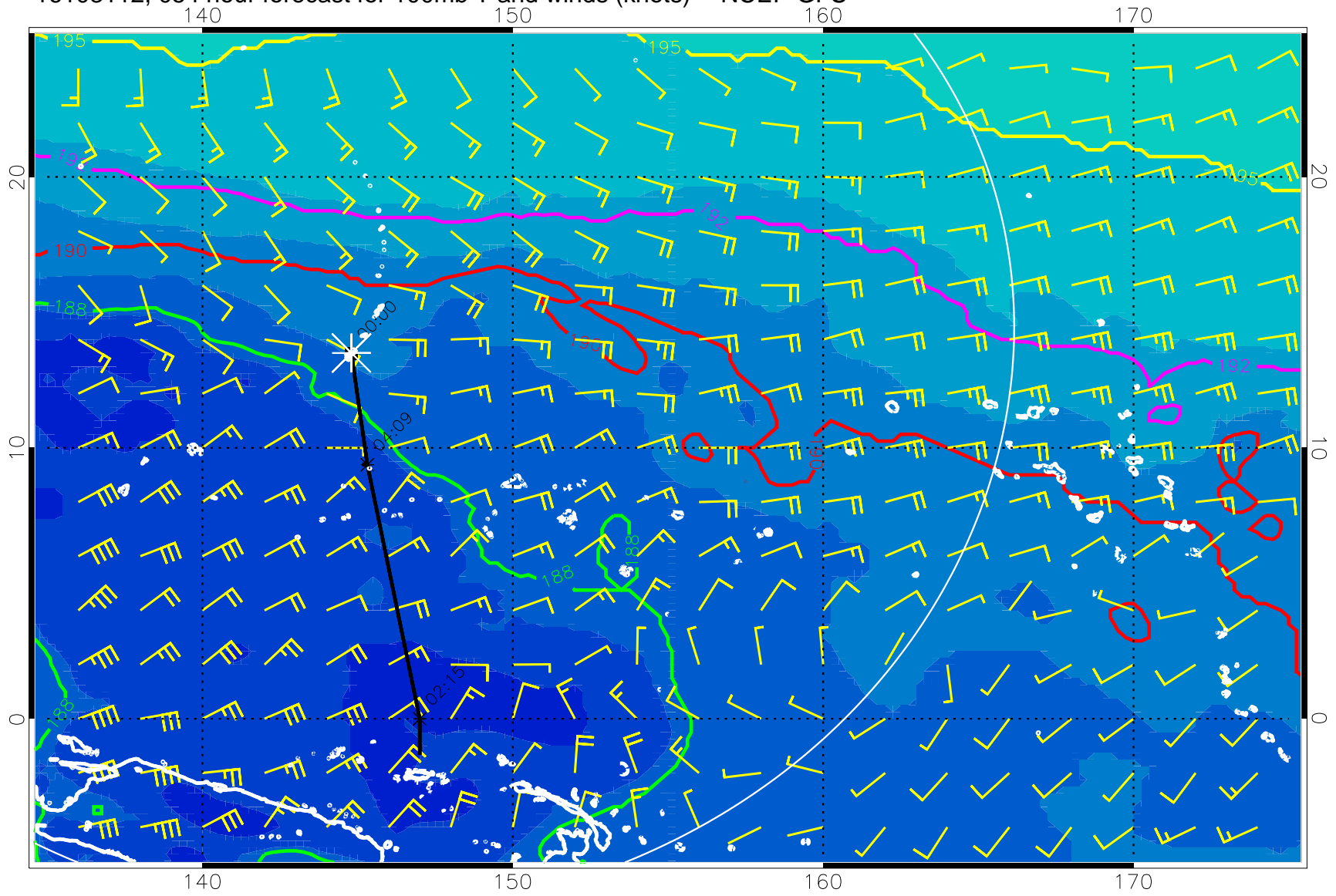
16103112, 054 hour forecast for 100mb T and winds (knots) -- NCEP GFS
