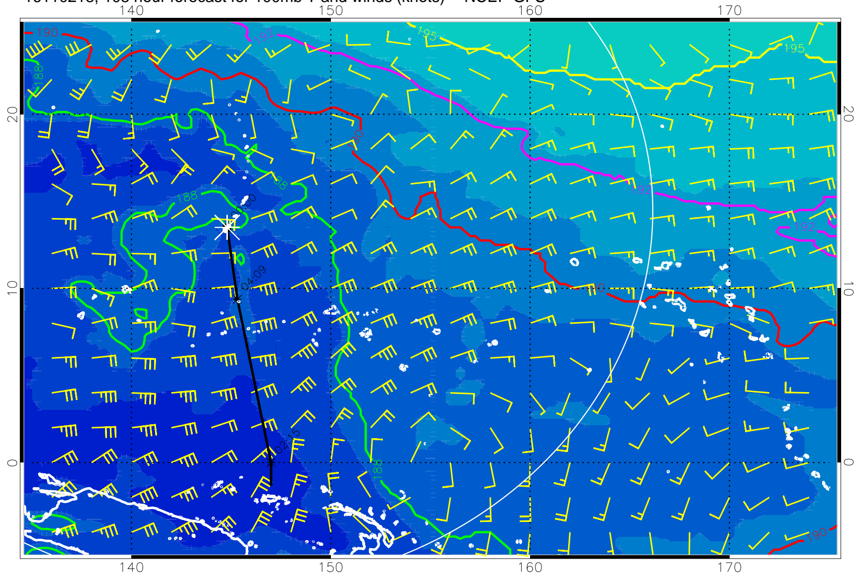
16110218, 108 hour forecast for 100mb T and winds (knots) -- NCEP GFS
