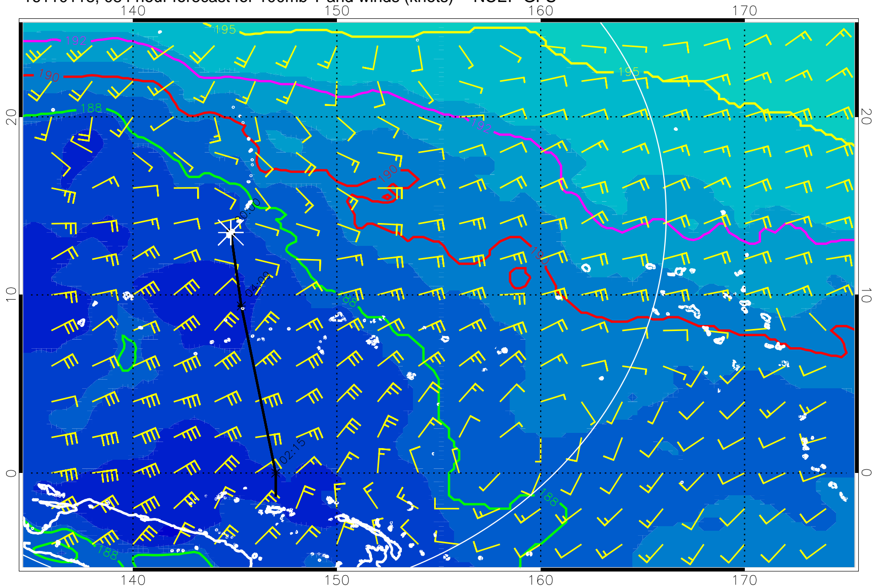
16110118, 084 hour forecast for 100mb T and winds (knots) -- NCEP GFS
