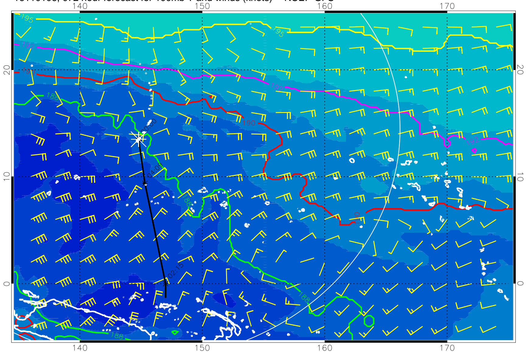
16110106, 072 hour forecast for 100mb T and winds (knots) -- NCEP GFS
