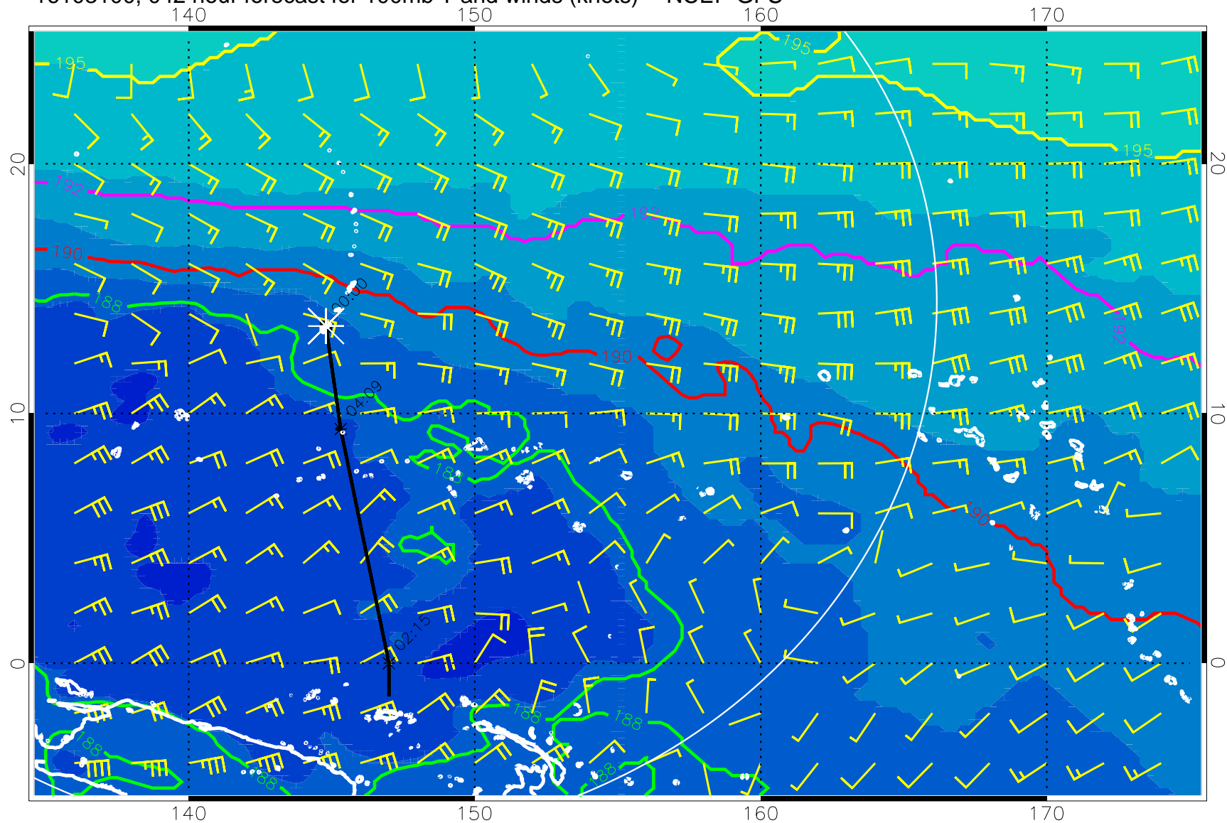
16103100, 042 hour forecast for 100mb T and winds (knots) -- NCEP GFS
