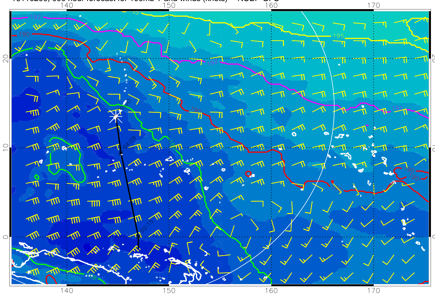
16110200, 090 hour forecast for 100mb T and winds (knots) -- NCEP GFS
