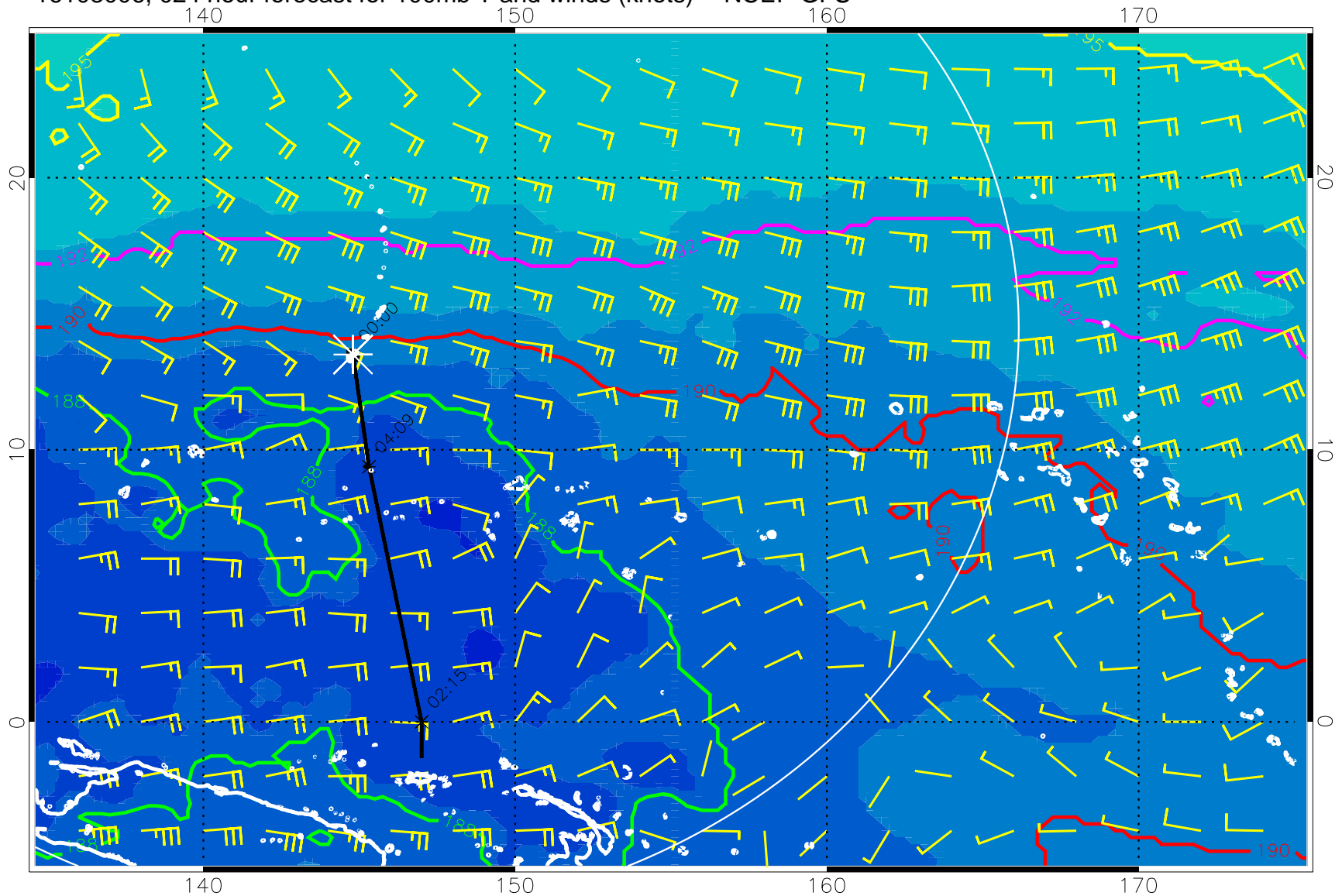
16103006, 024 hour forecast for 100mb T and winds (knots) -- NCEP GFS
