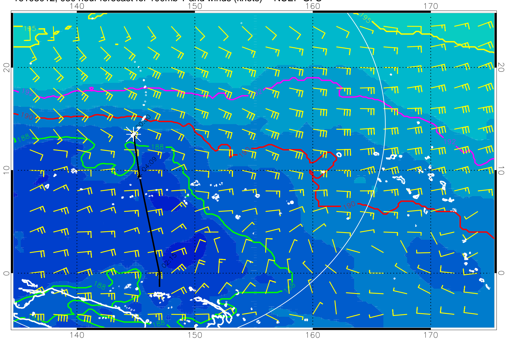
16103012, 030 hour forecast for 100mb T and winds (knots) -- NCEP GFS
