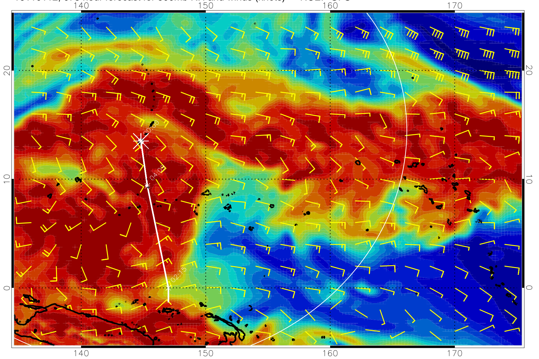
16110112, 078 hour forecast for 500mb RH and winds (knots) -- NCEP GFS
