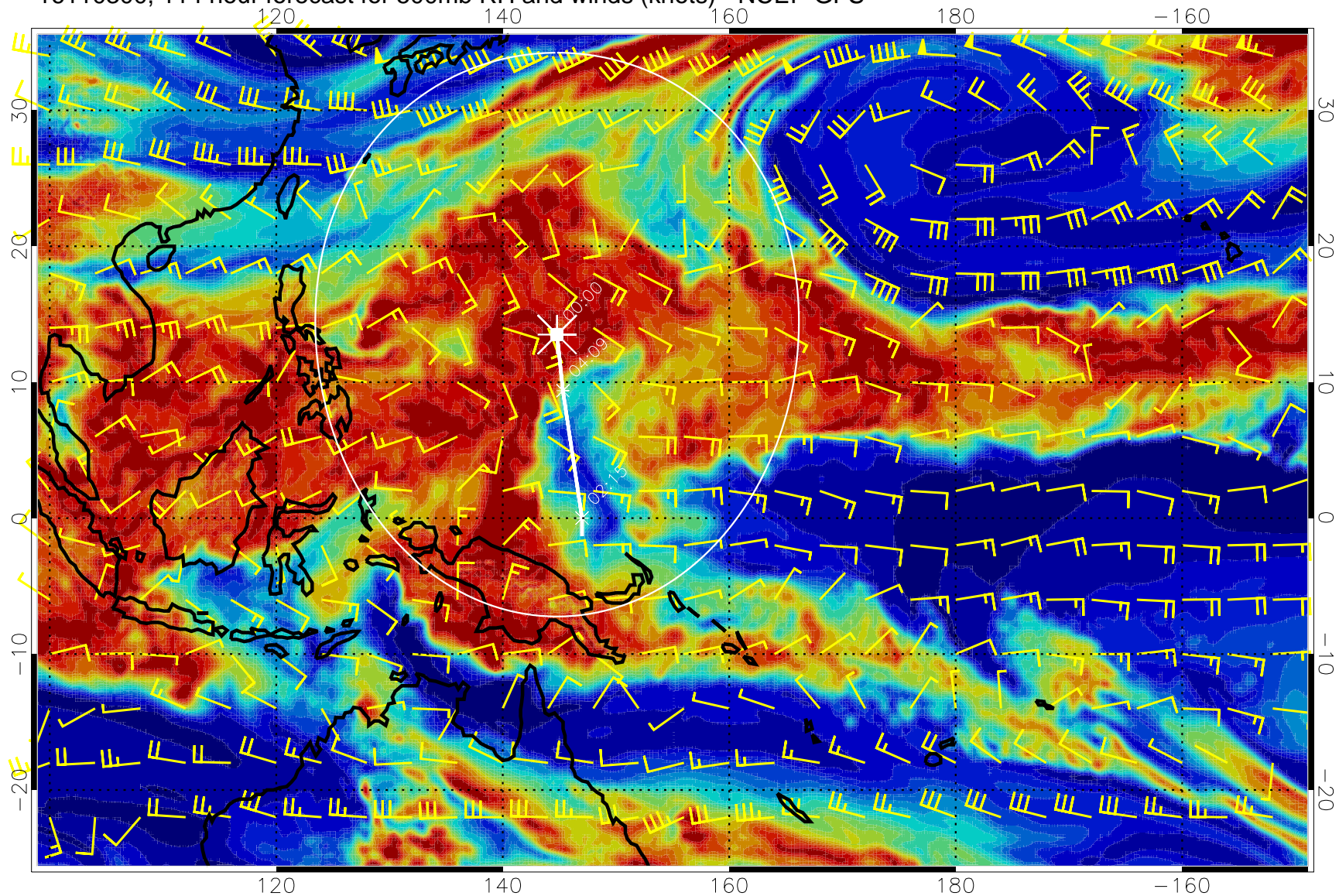
16110300, 114 hour forecast for 500mb RH and winds (knots) - NCEP GFS
