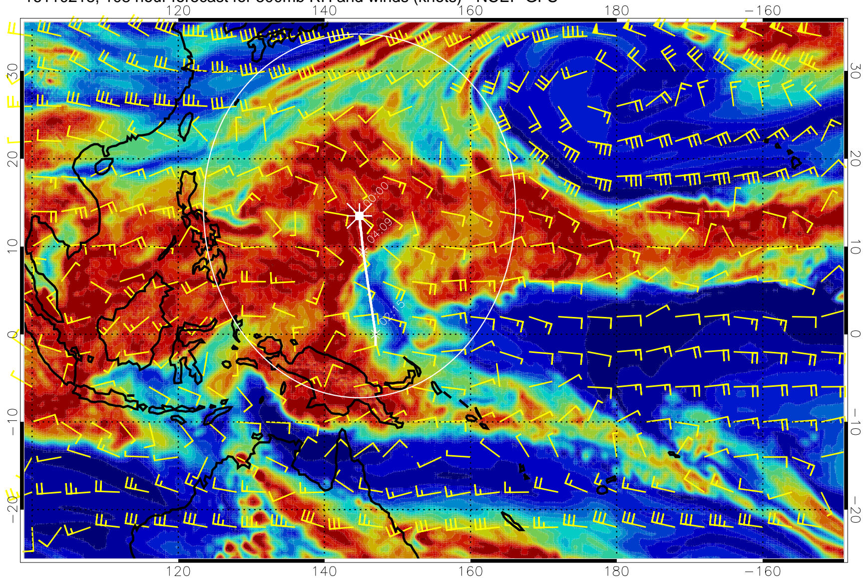
16110218, 108 hour forecast for 500mb RH and winds (knots) - NCEP GFS
