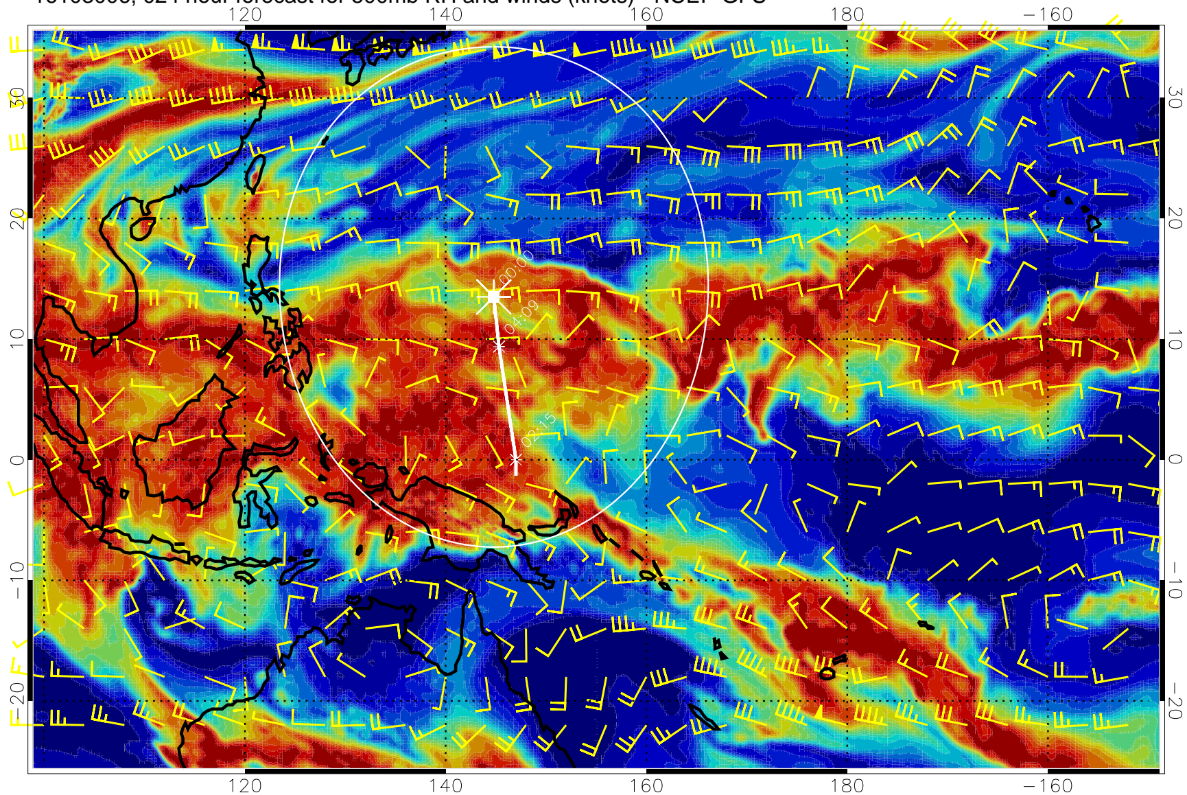
16103006, 024 hour forecast for 500mb RH and winds (knots) - NCEP GFS
