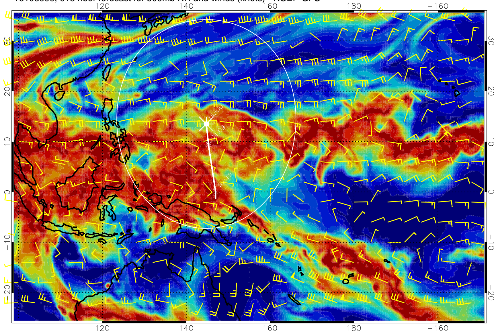
16103000, 018 hour forecast for 500mb RH and winds (knots) - NCEP GFS
