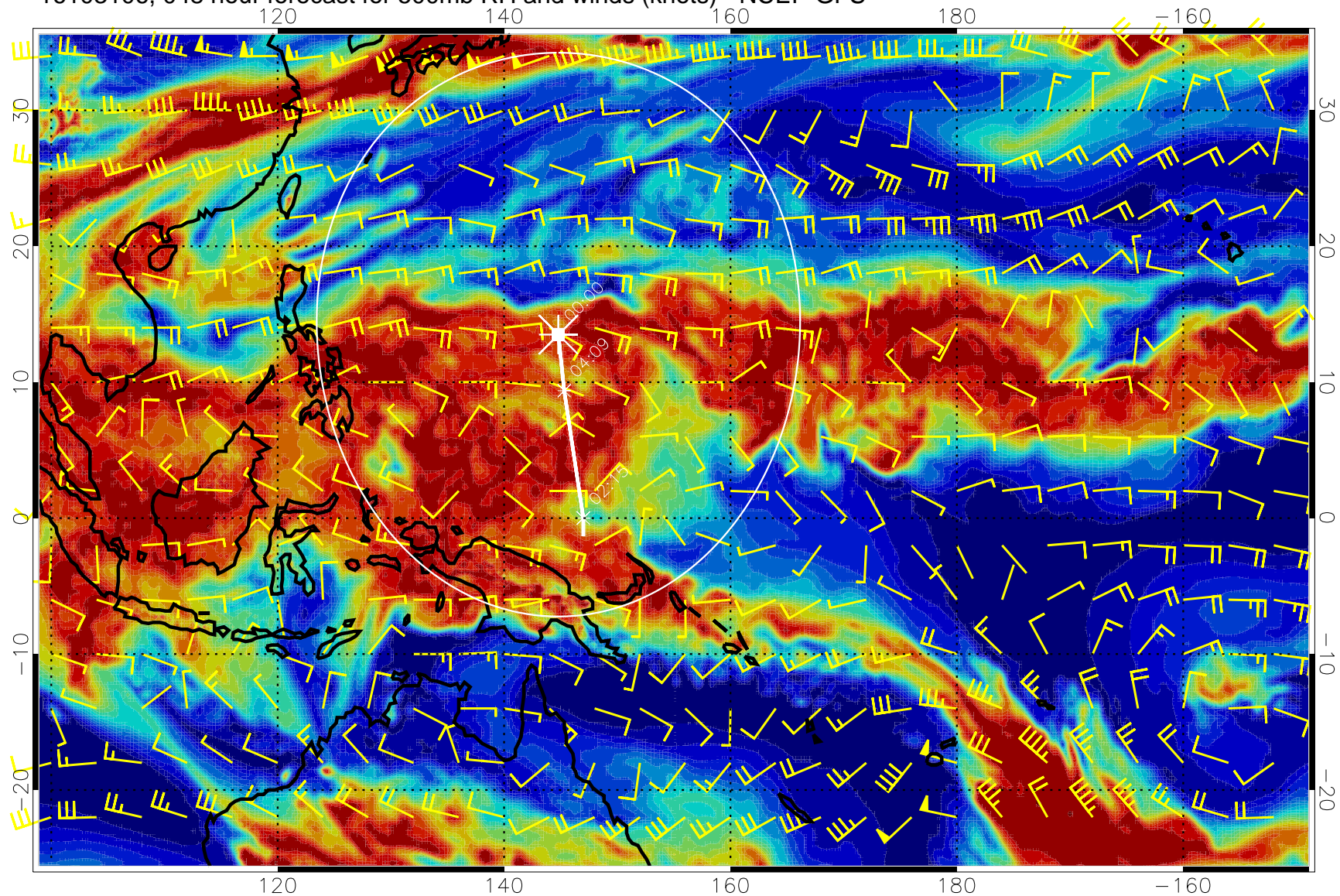
16103106, 048 hour forecast for 500mb RH and winds (knots) - NCEP GFS
