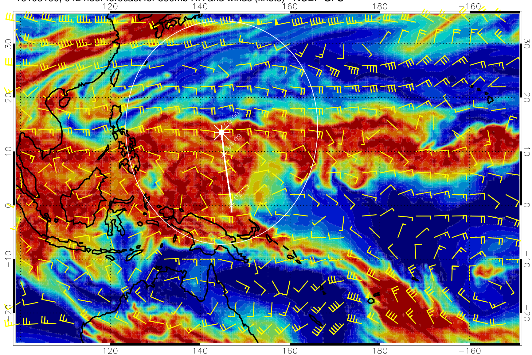
16103100, 042 hour forecast for 500mb RH and winds (knots) - NCEP GFS
