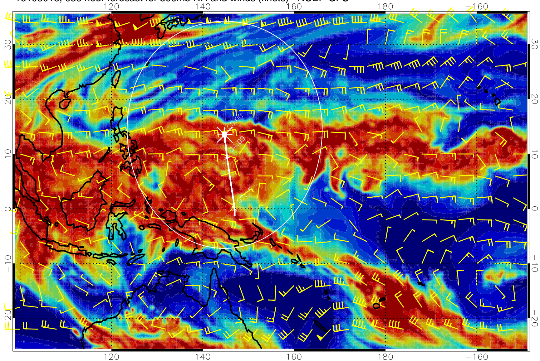
16103018, 036 hour forecast for 500mb RH and winds (knots) - NCEP GFS
