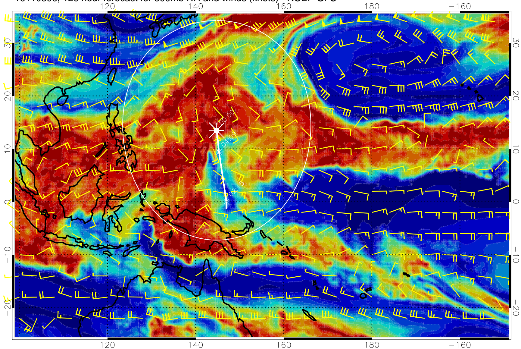
16110306, 120 hour forecast for 500mb RH and winds (knots) - NCEP GFS
