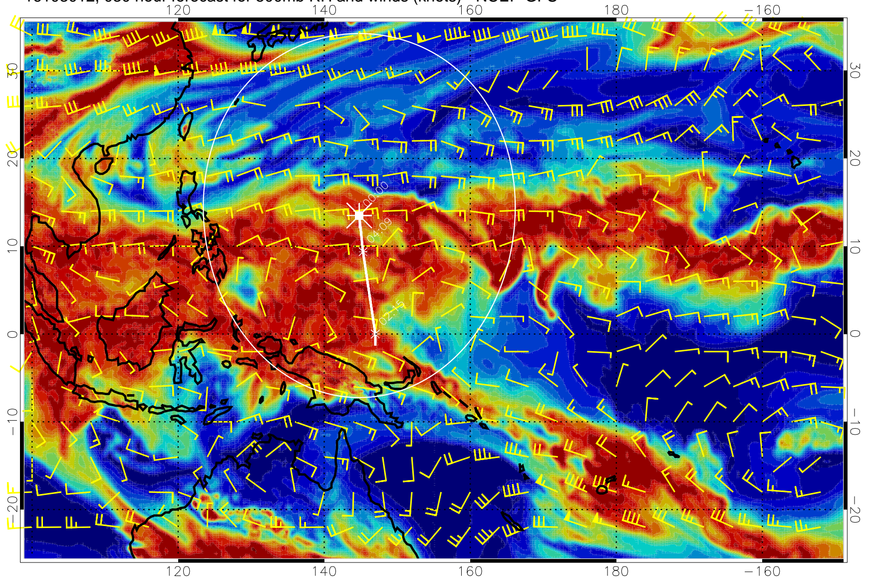
16103012, 030 hour forecast for 500mb RH and winds (knots) - NCEP GFS
