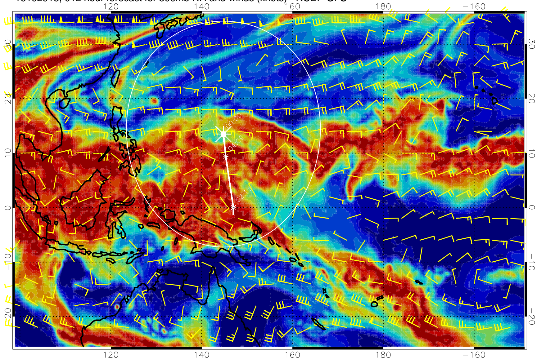
16102918, 012 hour forecast for 500mb RH and winds (knots) - NCEP GFS
