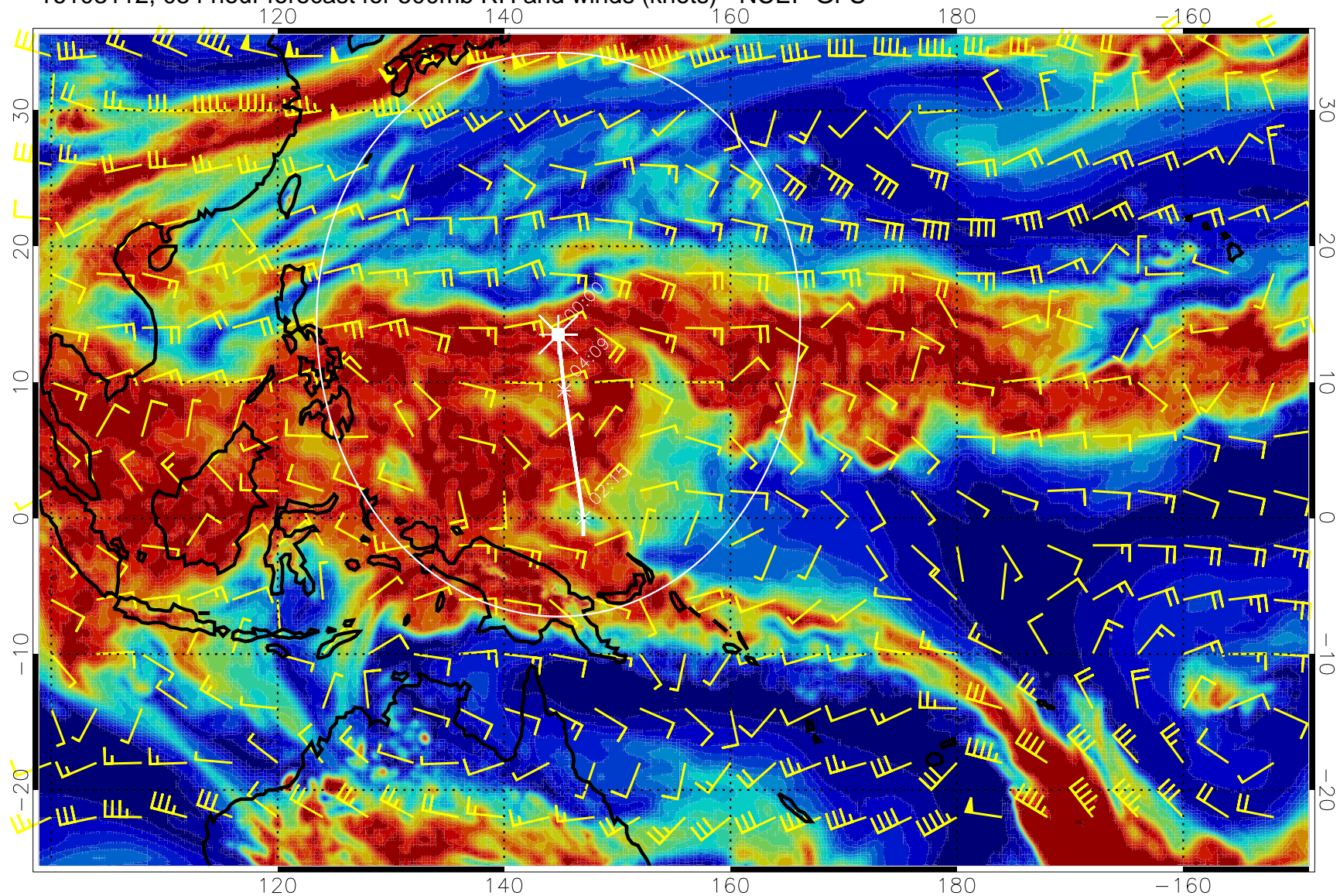
16103112, 054 hour forecast for 500mb RH and winds (knots) - NCEP GFS
