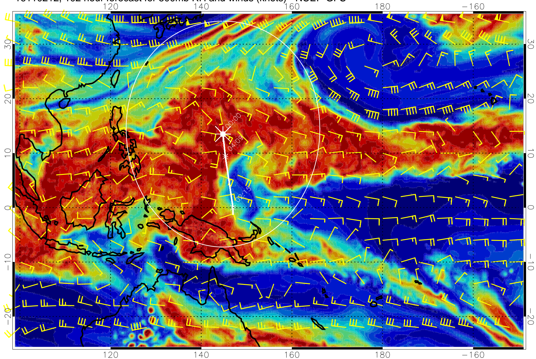
16110212, 102 hour forecast for 500mb RH and winds (knots) - NCEP GFS
