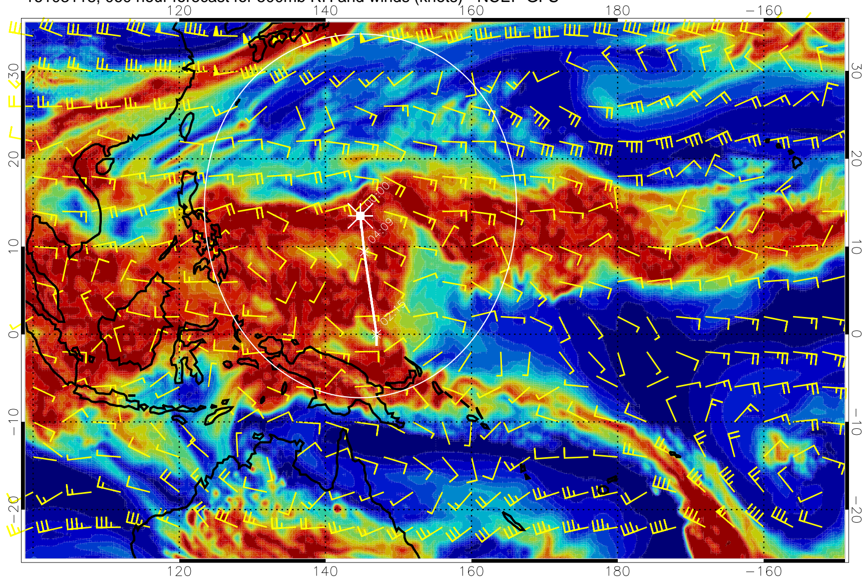
16103118, 060 hour forecast for 500mb RH and winds (knots) - NCEP GFS
