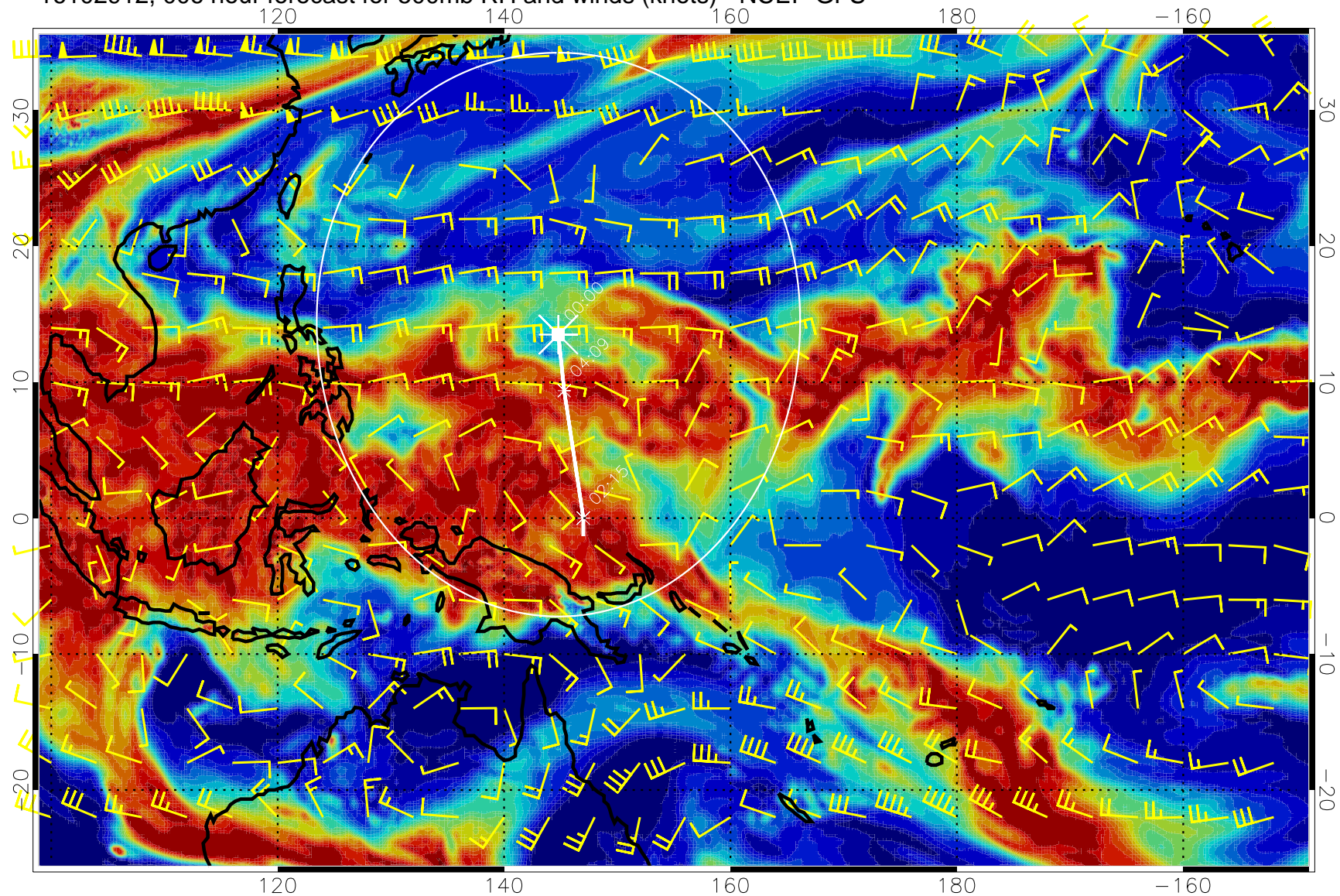
16102912, 006 hour forecast for 500mb RH and winds (knots) - NCEP GFS
