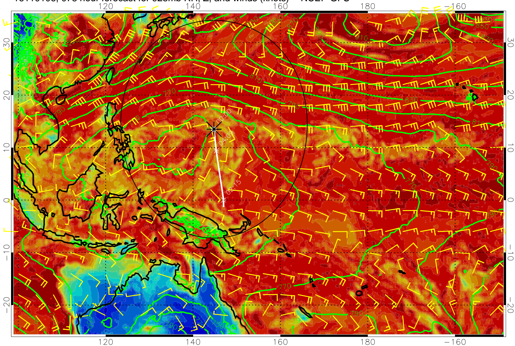
16110106, 078 hour forecast for 925mb RH, Z, and winds (knots) -- NCEP GFS
