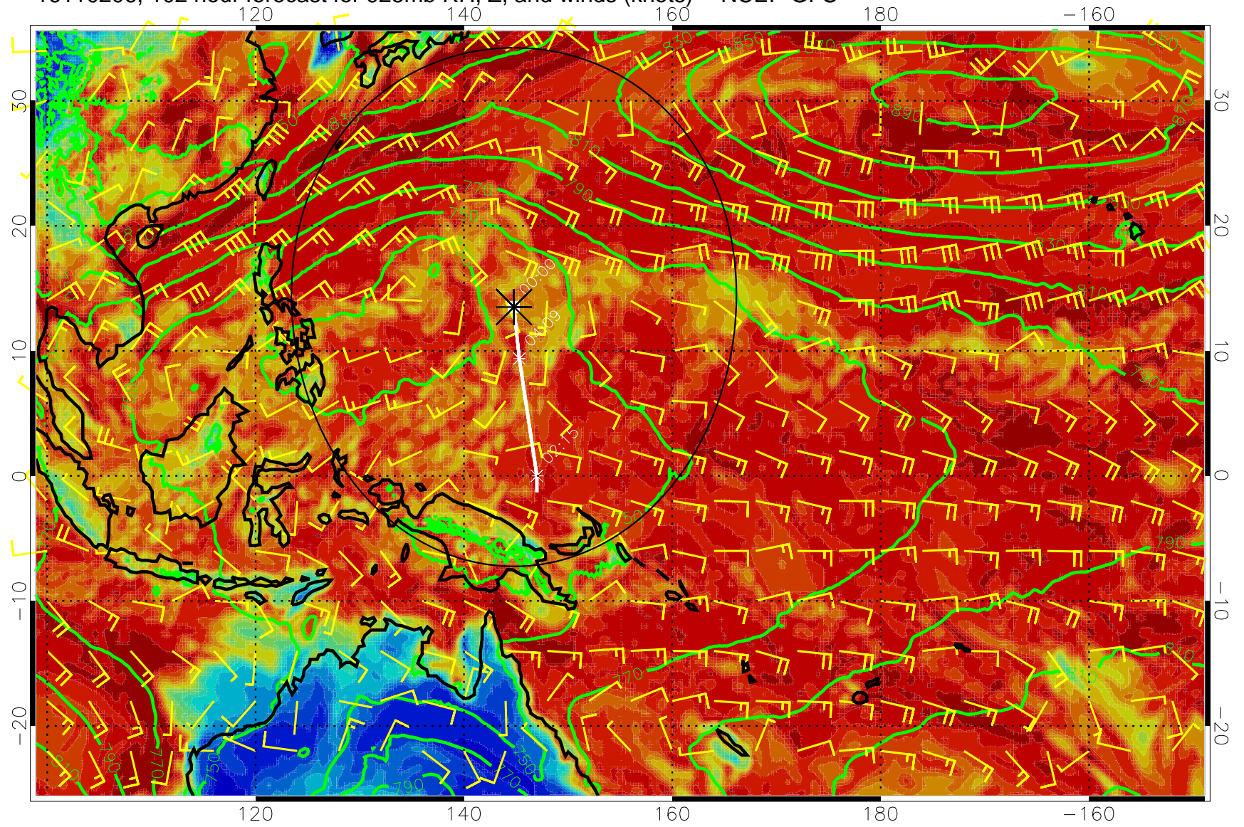
16110206, 102 hour forecast for 925mb RH, Z, and winds (knots) -- NCEP GFS
