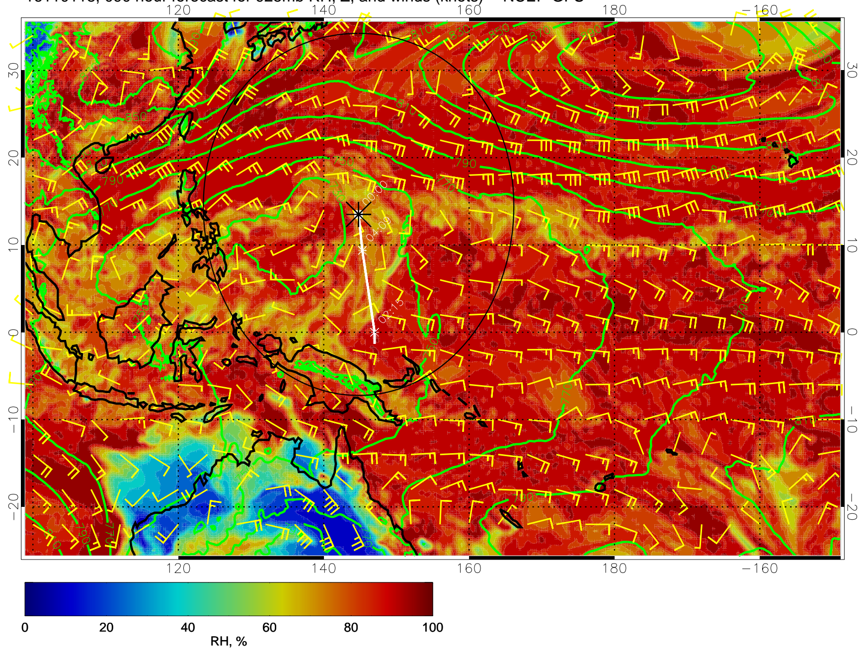
16110118, 090 hour forecast for 925mb RH, Z, and winds (knots) -- NCEP GFS
