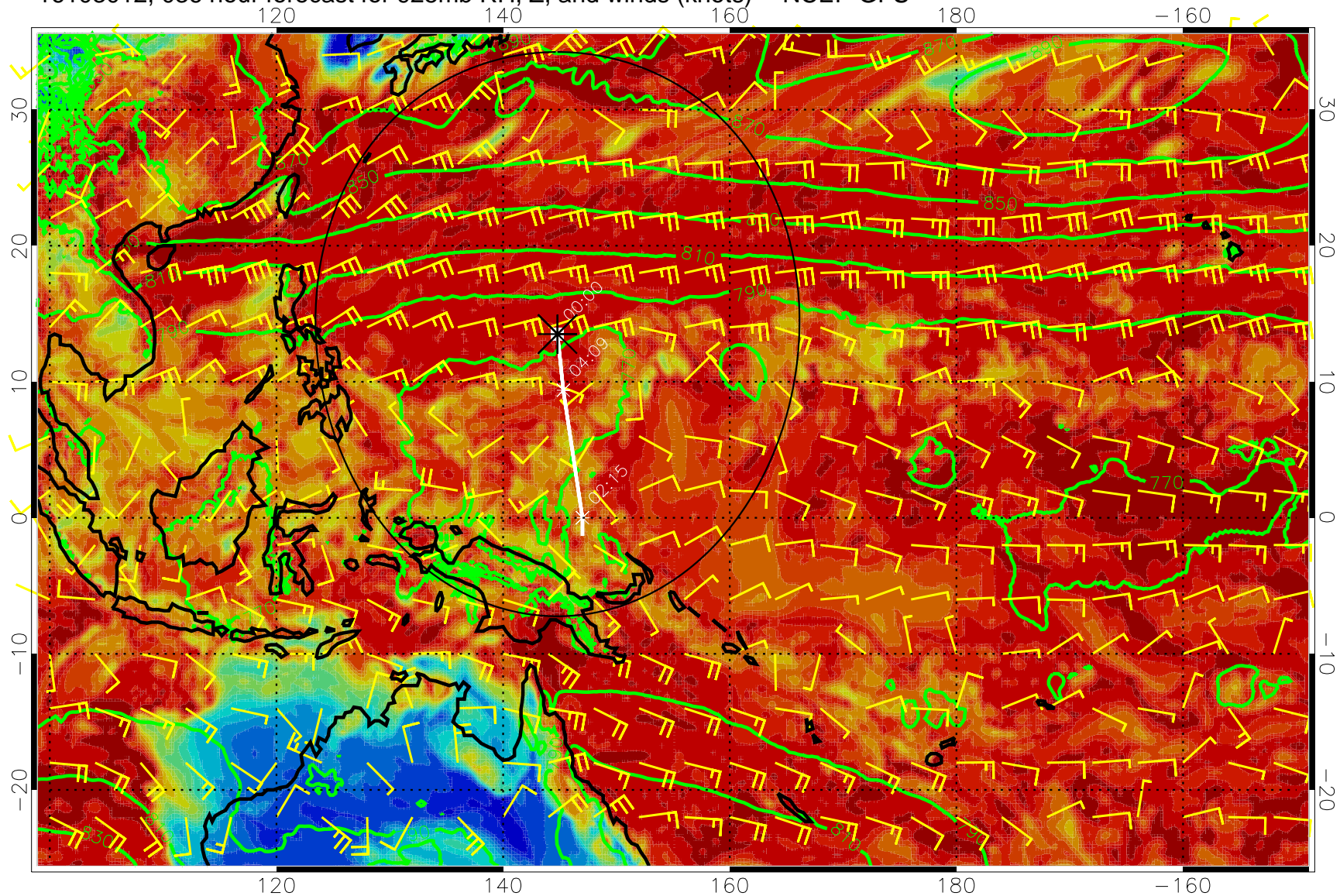
16103012, 036 hour forecast for 925mb RH, Z, and winds (knots) -- NCEP GFS
