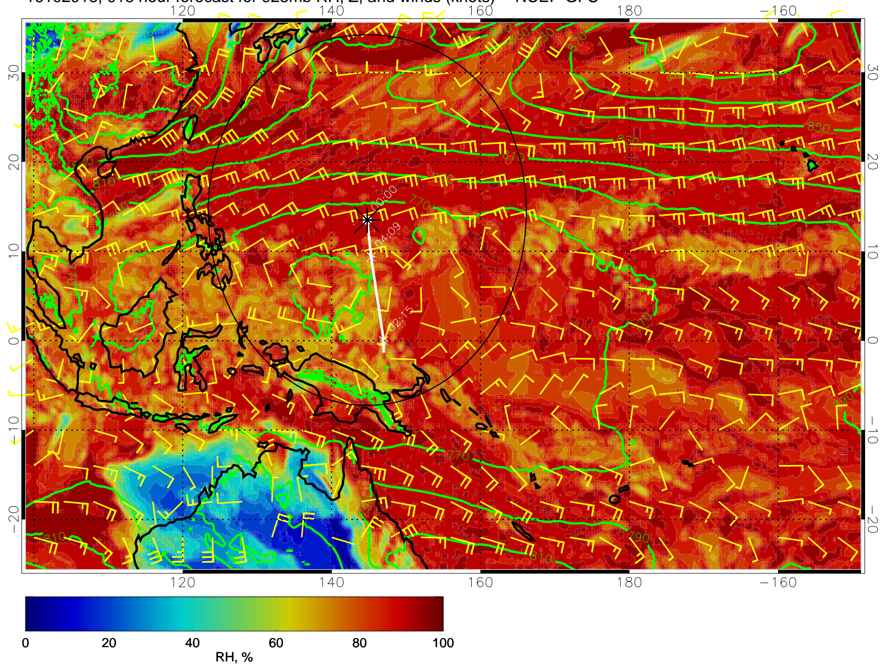
16102918, 018 hour forecast for 925mb RH, Z, and winds (knots) -- NCEP GFS
