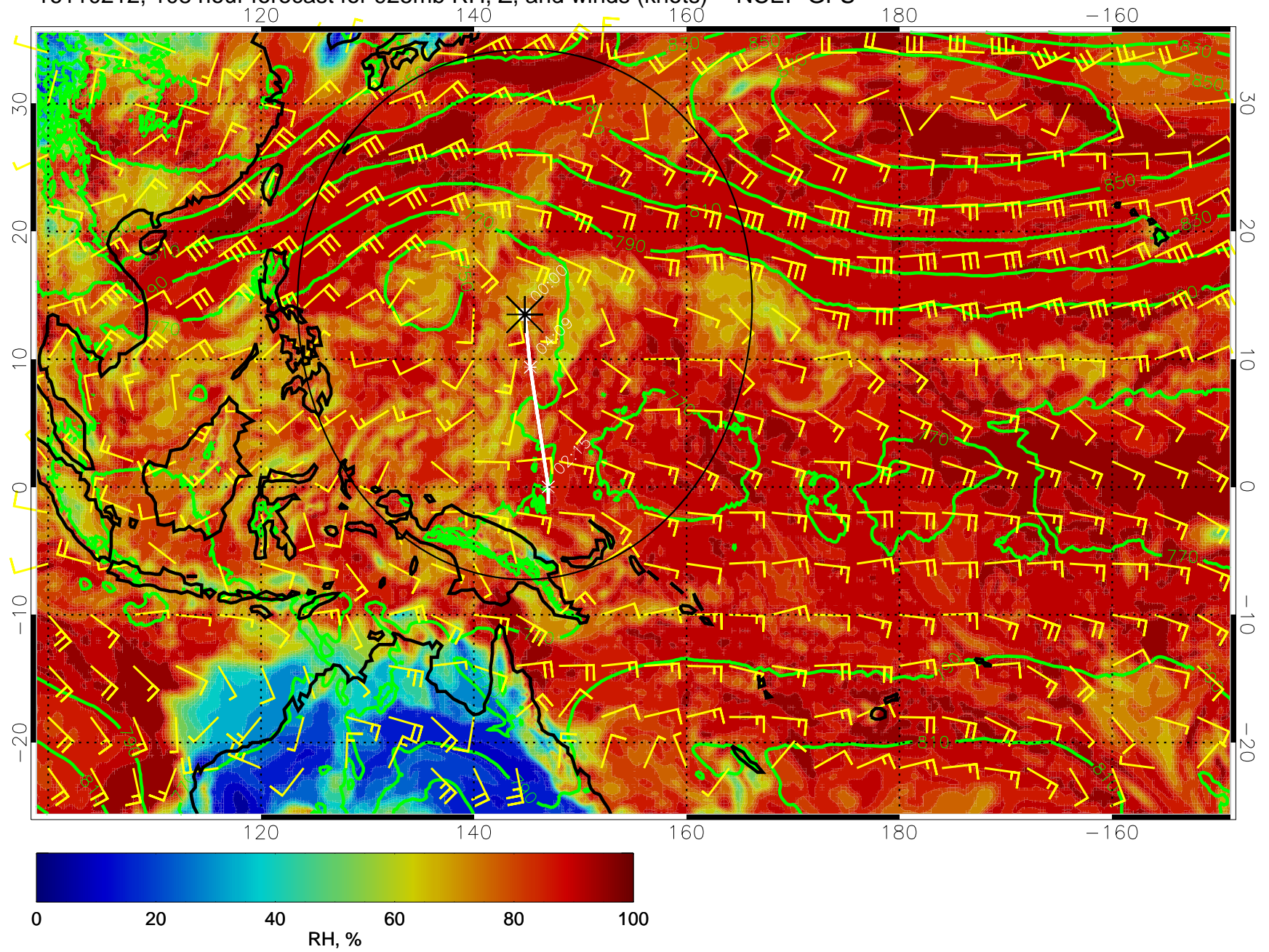
16110212, 108 hour forecast for 925mb RH, Z, and winds (knots) -- NCEP GFS
