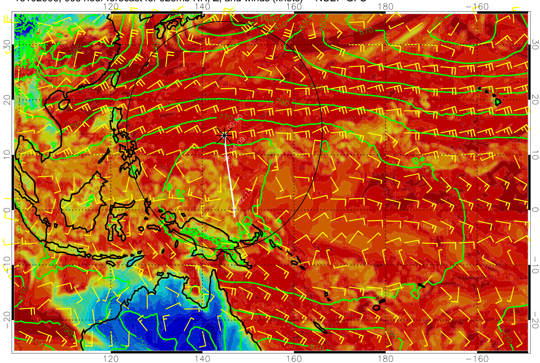
16102906, 006 hour forecast for 925mb RH, Z, and winds (knots) -- NCEP GFS
