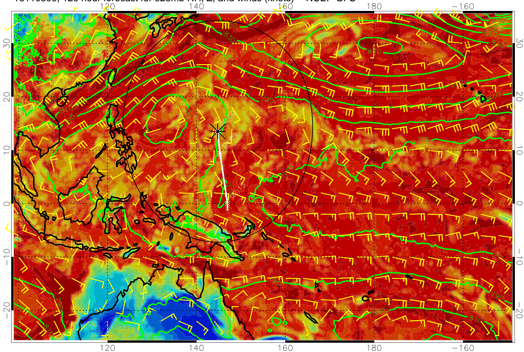
16110300, 120 hour forecast for 925mb RH, Z, and winds (knots) -- NCEP GFS
