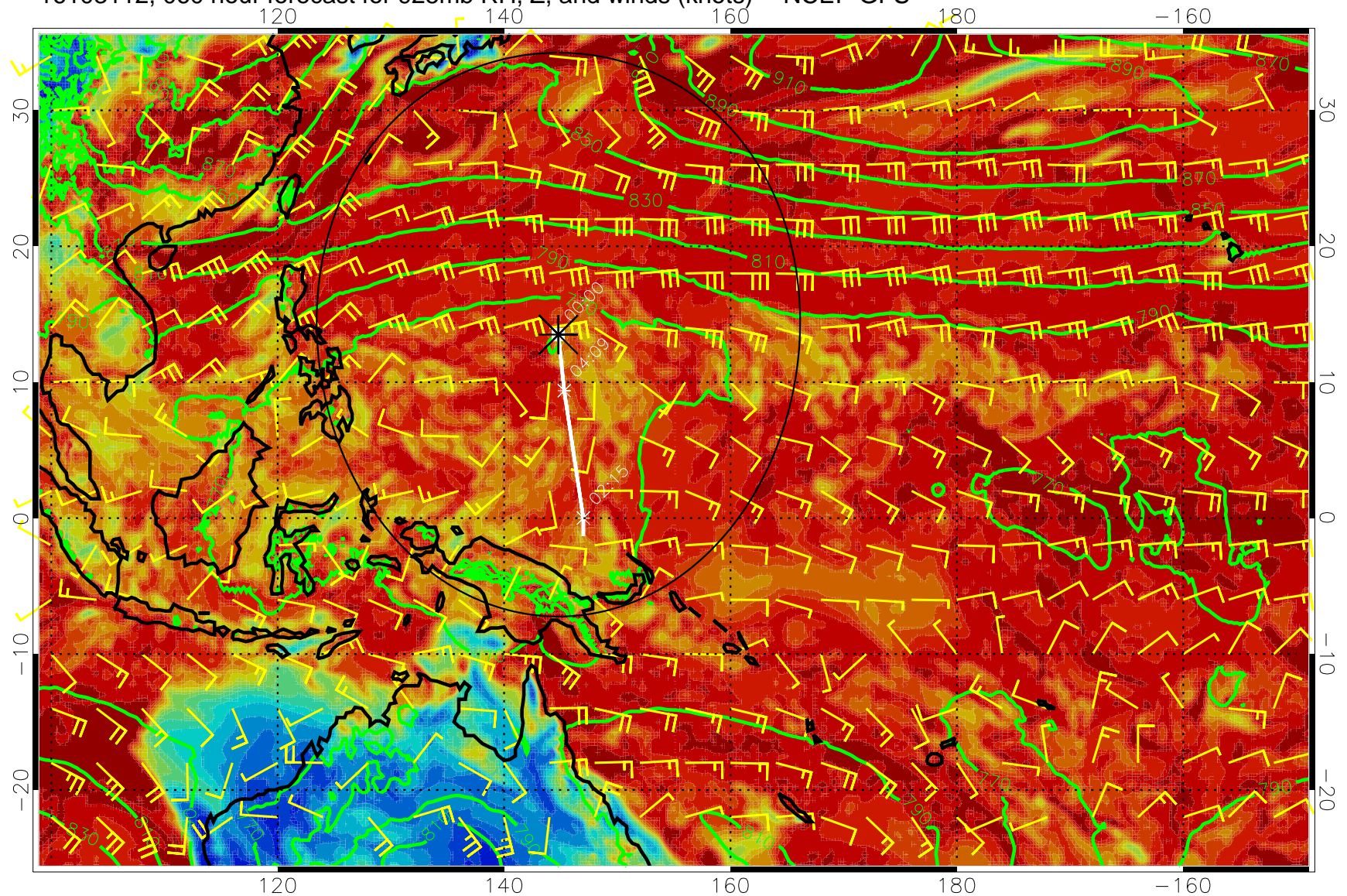
16103112, 060 hour forecast for 925mb RH, Z, and winds (knots) -- NCEP GFS
