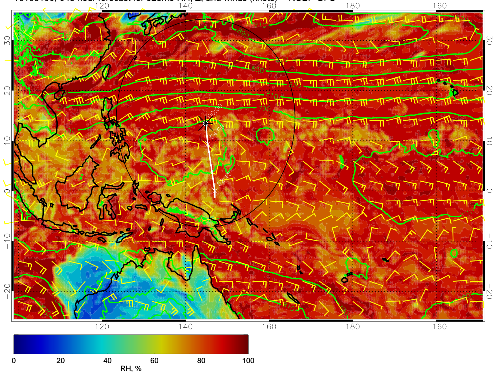
16103100, 048 hour forecast for 925mb RH, Z, and winds (knots) -- NCEP GFS
