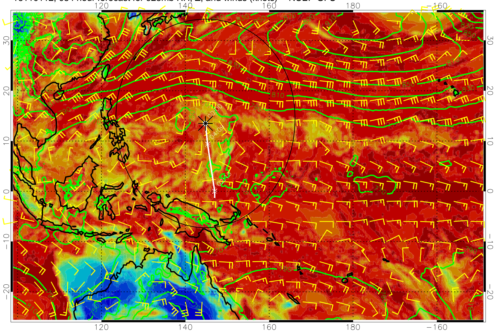
16110112, 084 hour forecast for 925mb RH, Z, and winds (knots) -- NCEP GFS
