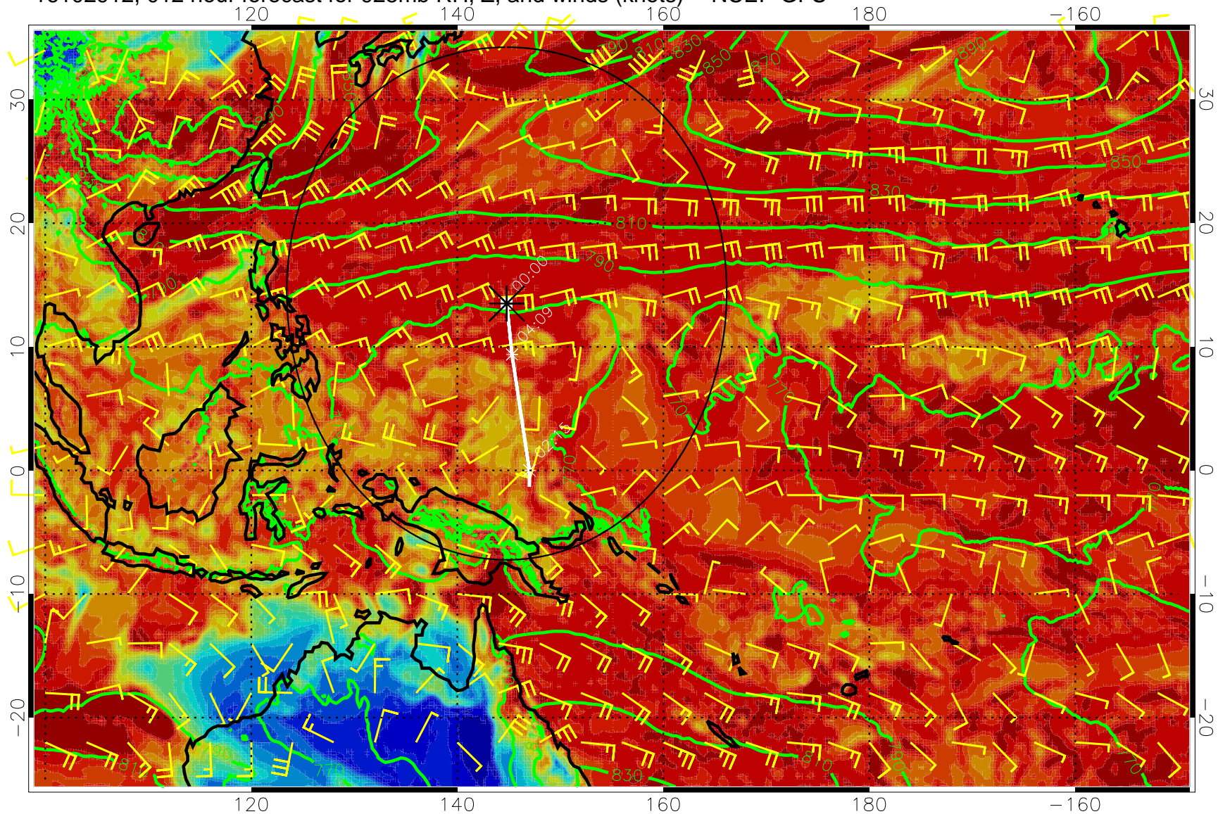
16102912, 012 hour forecast for 925mb RH, Z, and winds (knots) -- NCEP GFS
