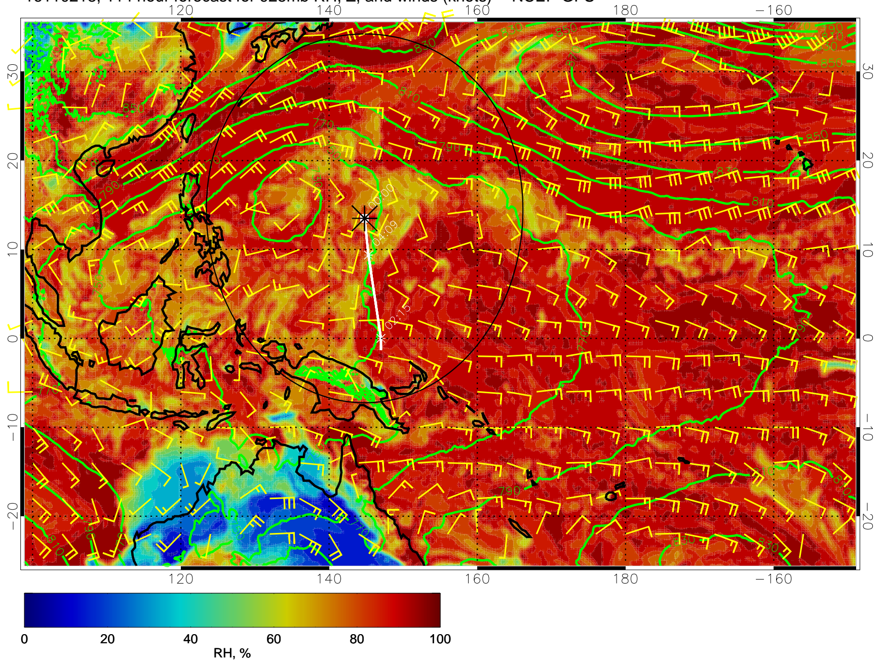
16110218, 114 hour forecast for 925mb RH, Z, and winds (knots) -- NCEP GFS
