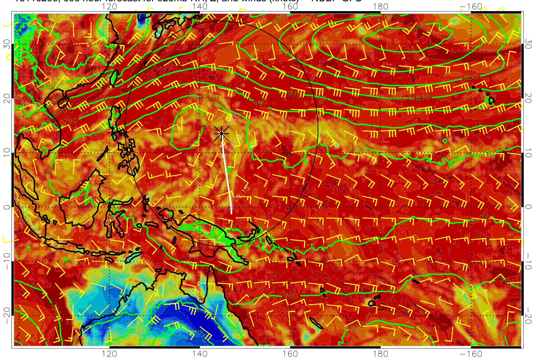
16110200, 096 hour forecast for 925mb RH, Z, and winds (knots) -- NCEP GFS
