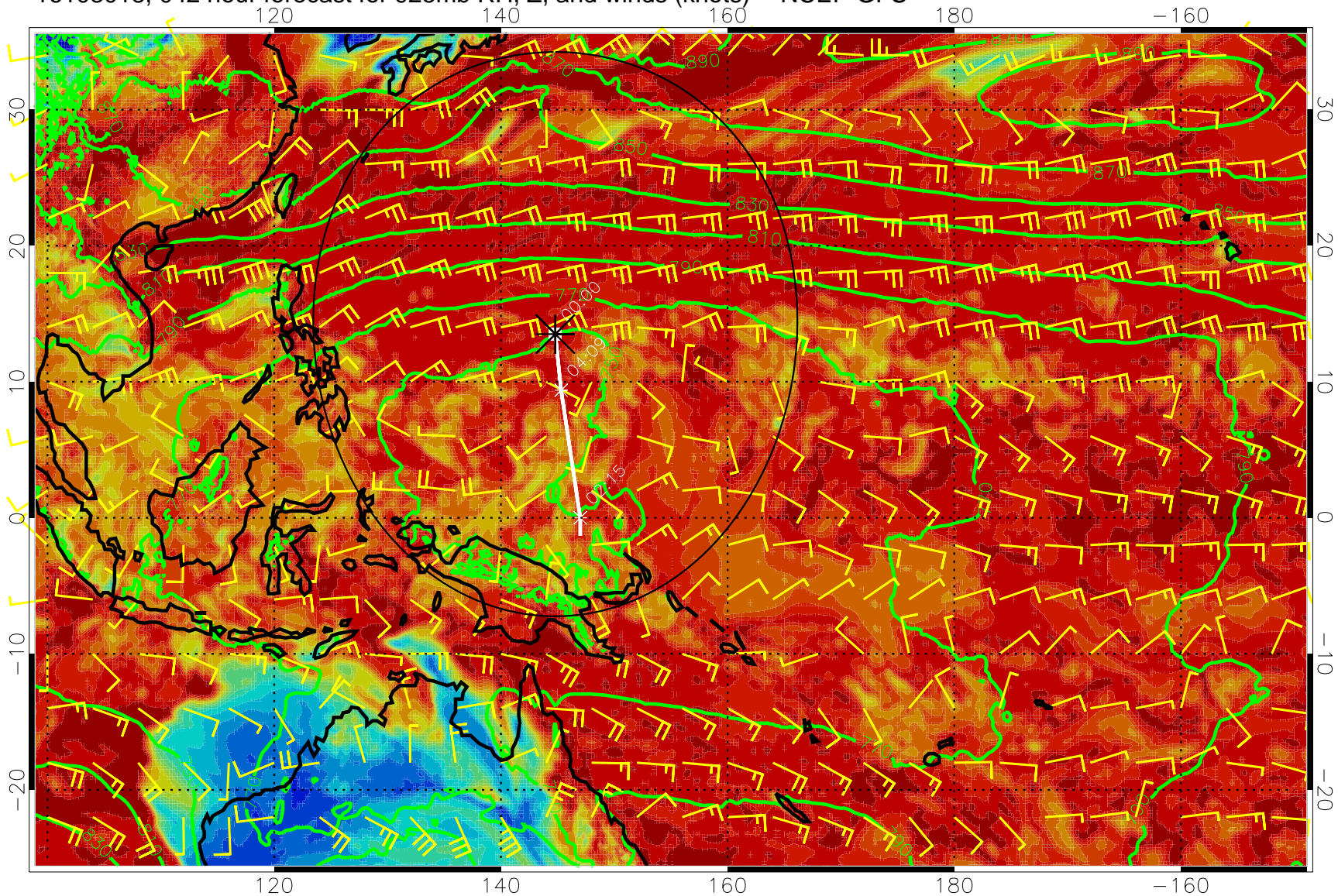
16103018, 042 hour forecast for 925mb RH, Z, and winds (knots) -- NCEP GFS
