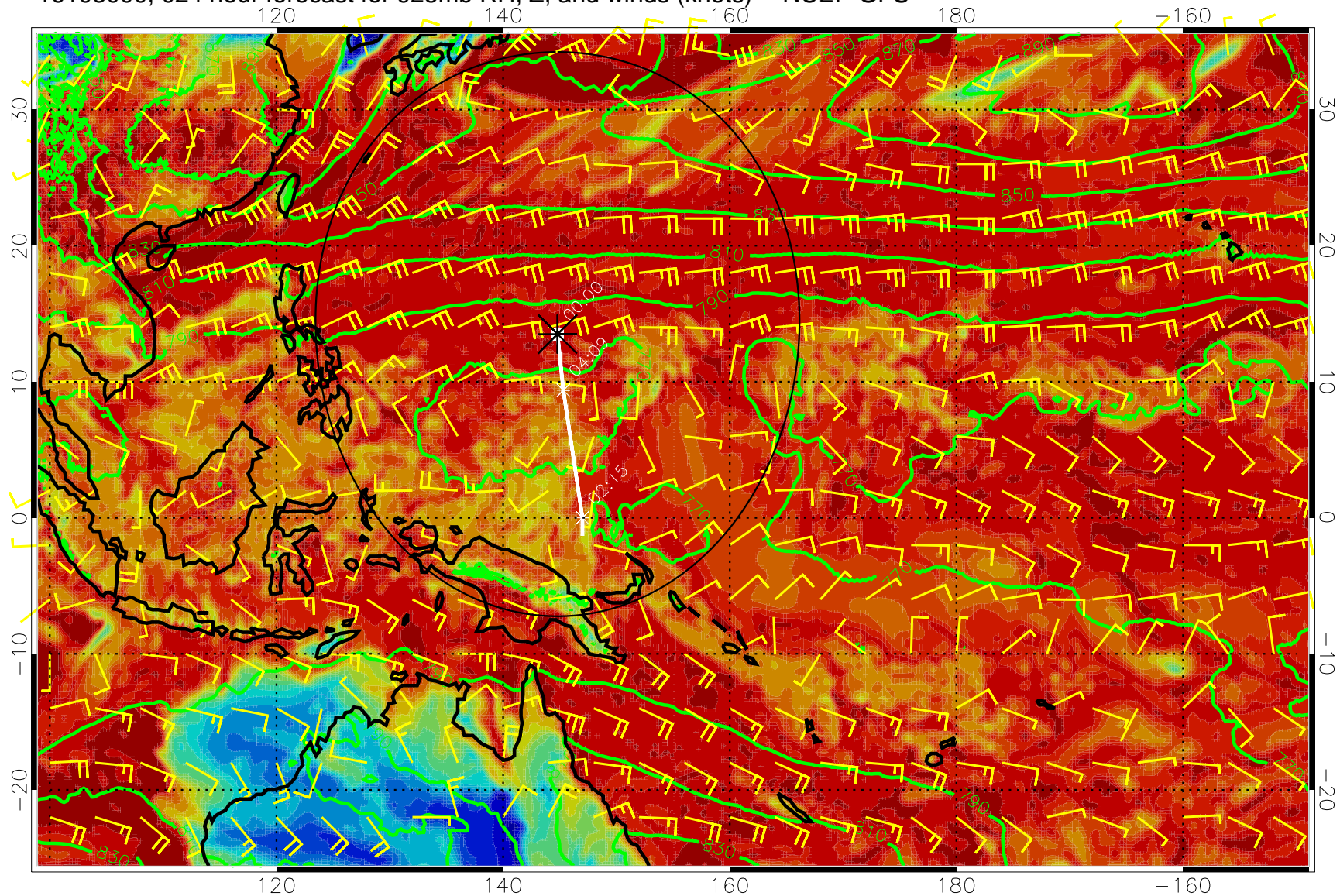
16103000, 024 hour forecast for 925mb RH, Z, and winds (knots) -- NCEP GFS
