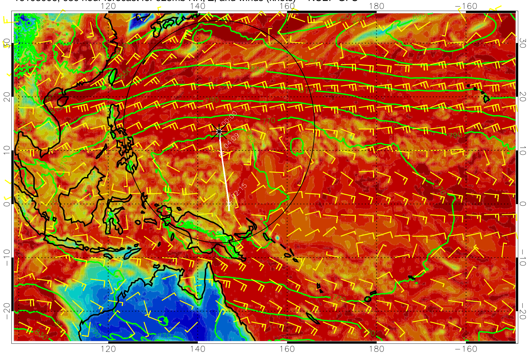
16103006, 030 hour forecast for 925mb RH, Z, and winds (knots) -- NCEP GFS
