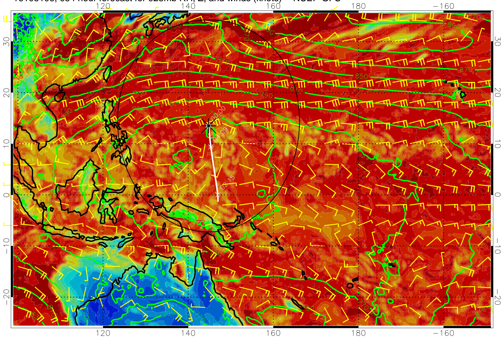
16103106, 054 hour forecast for 925mb RH, Z, and winds (knots) -- NCEP GFS
