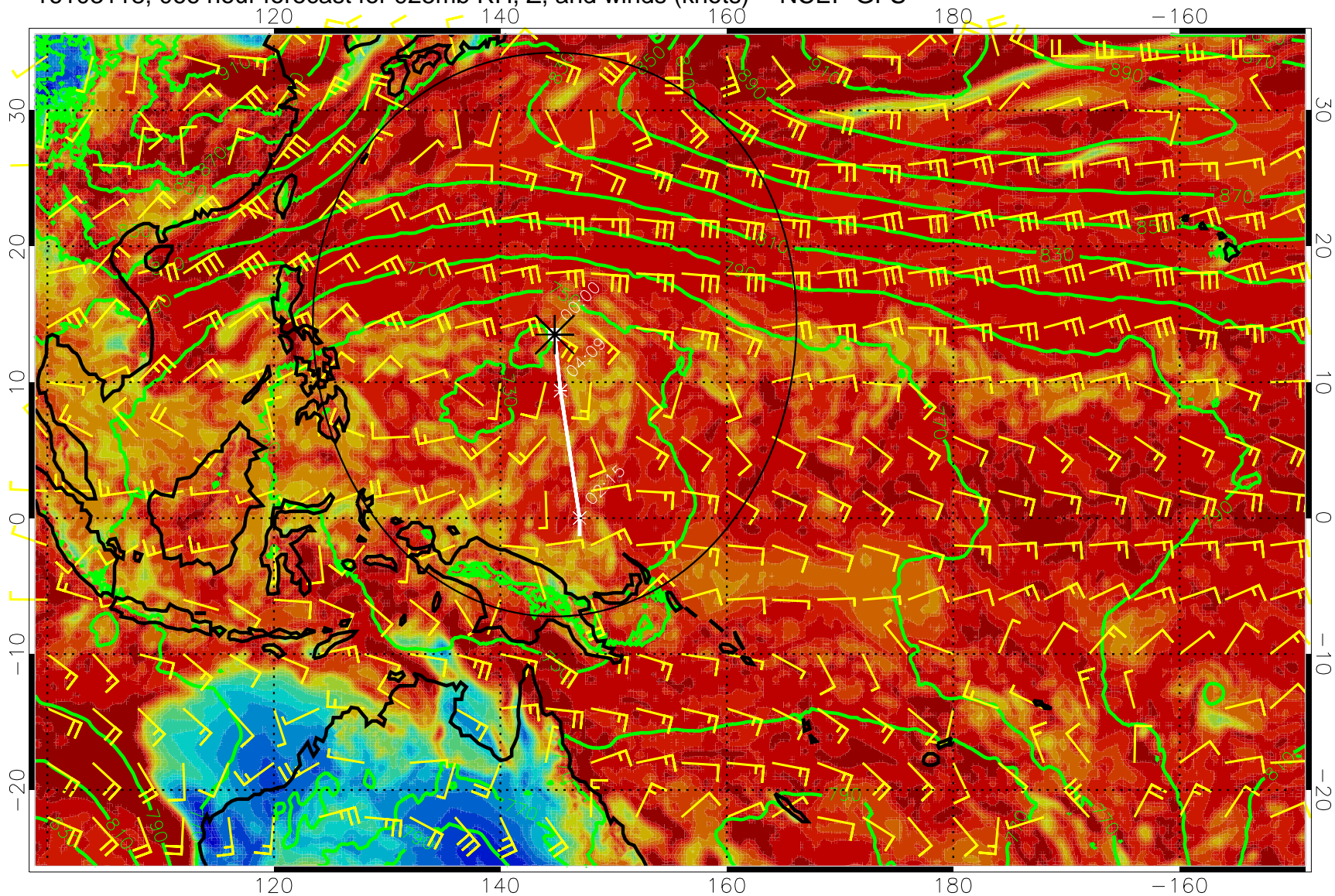
16103118, 066 hour forecast for 925mb RH, Z, and winds (knots) -- NCEP GFS
