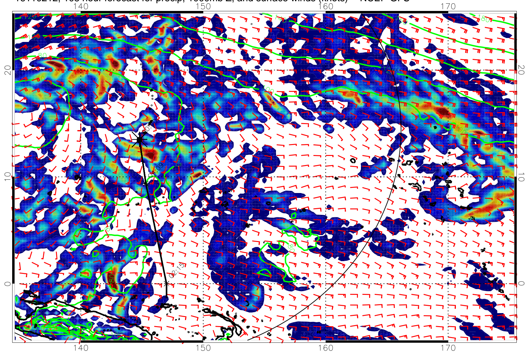
16110212, 108 hour forecast for precip, 1000mb Z, and surface winds (knots) -- NCEP GFS
