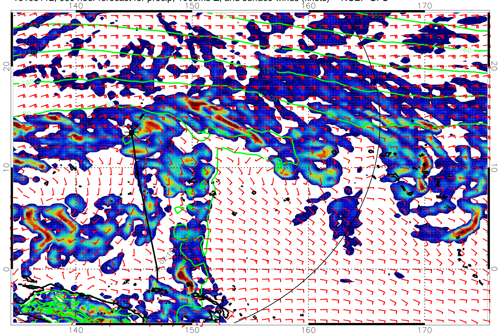
16103112, 060 hour forecast for precip, 1000mb Z, and surface winds (knots) -- NCEP GFS
