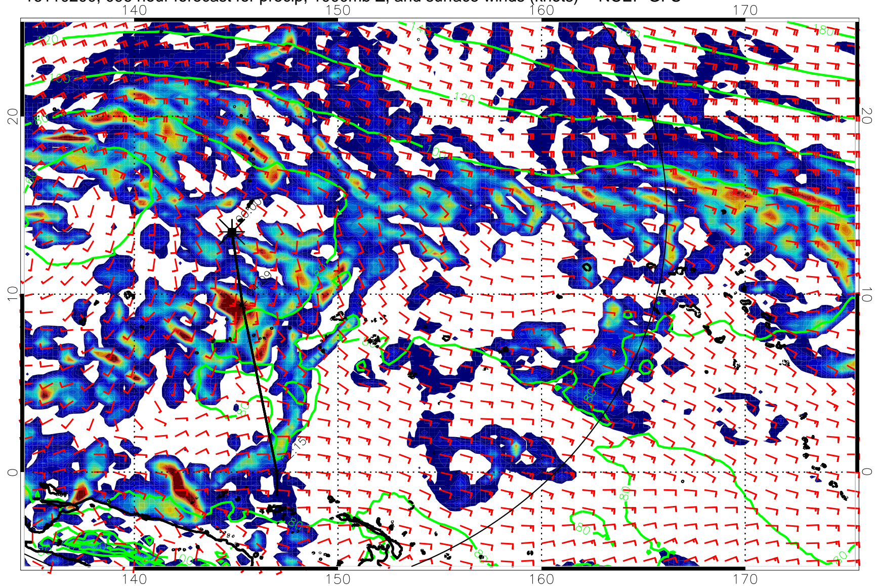
16110200, 096 hour forecast for precip, 1000mb Z, and surface winds (knots) -- NCEP GFS
