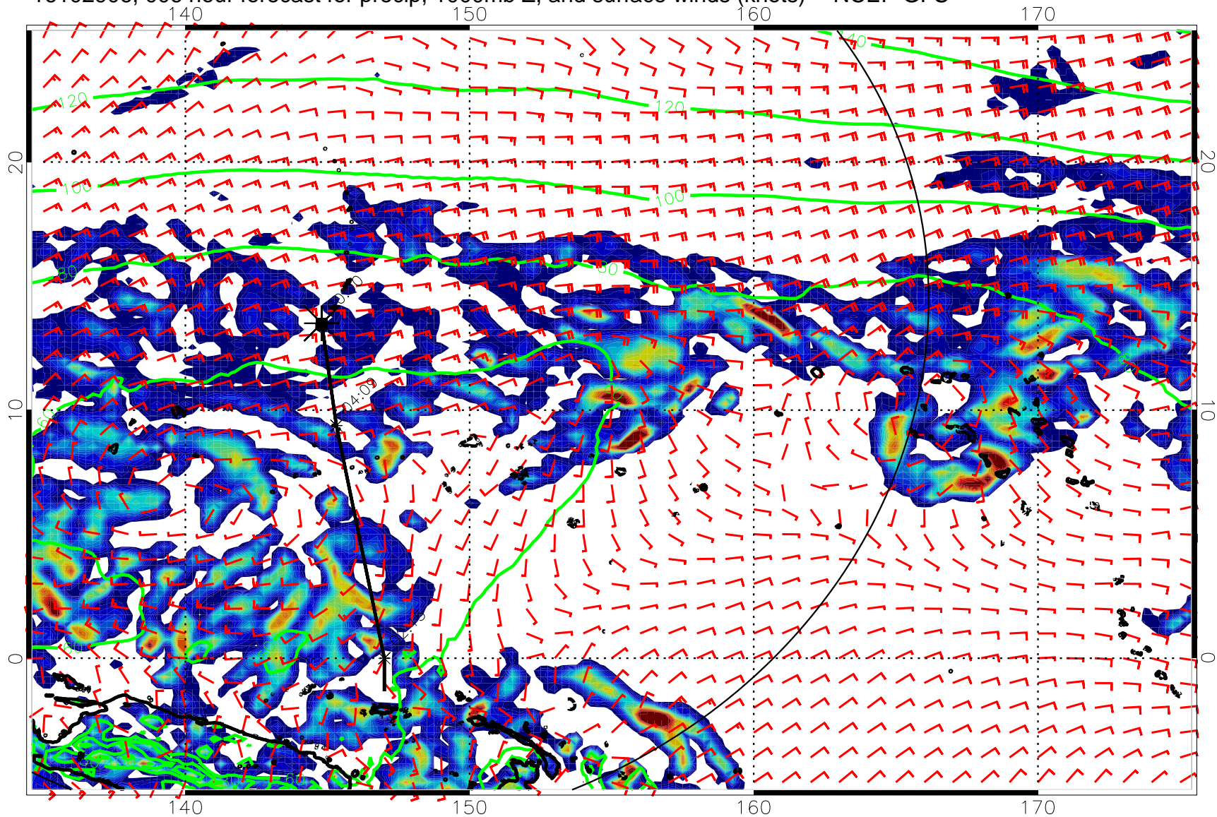
16102906, 006 hour forecast for precip, 1000mb Z, and surface winds (knots) -- NCEP GFS
