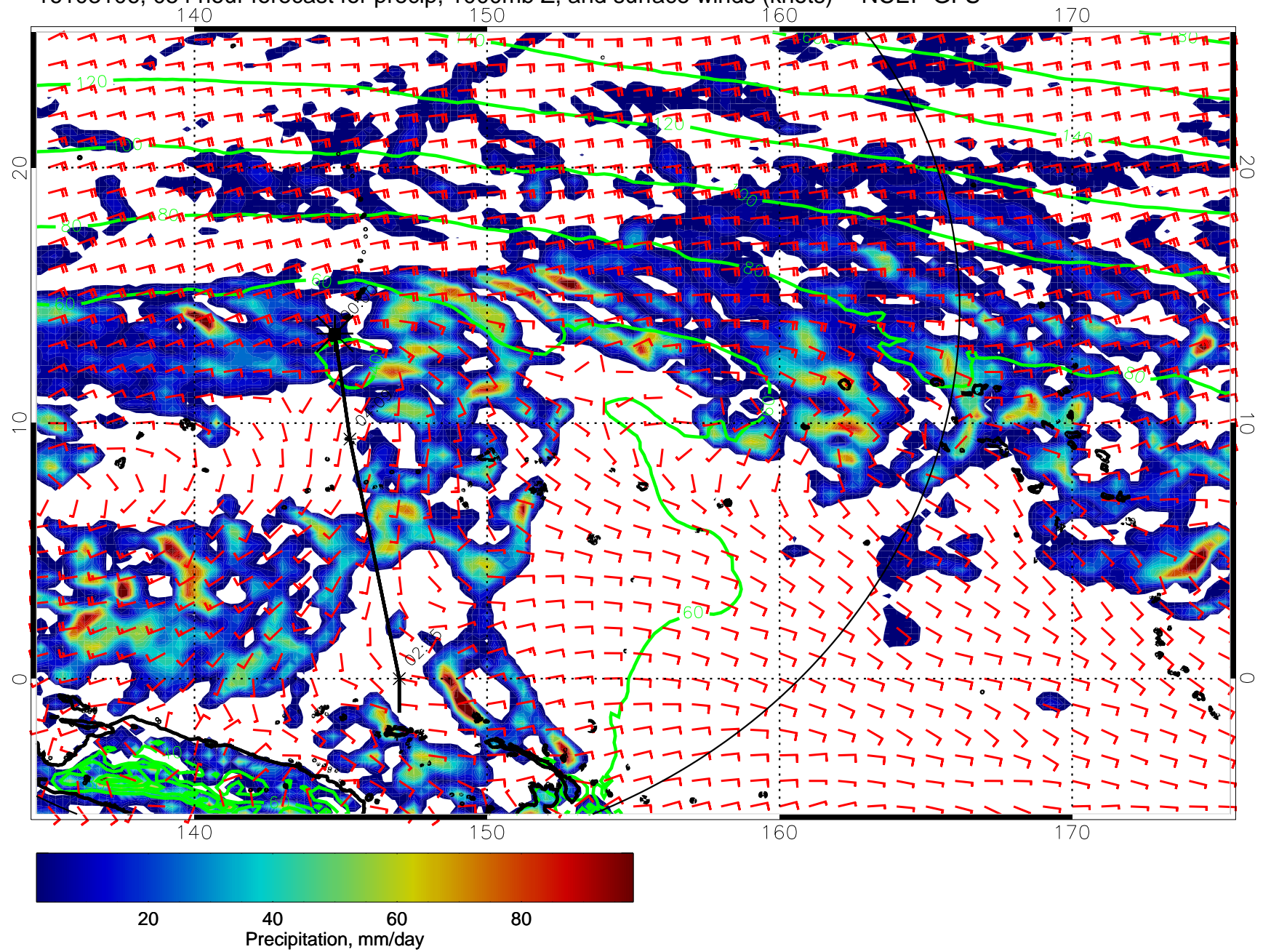
16103106, 054 hour forecast for precip, 1000mb Z, and surface winds (knots) -- NCEP GFS
