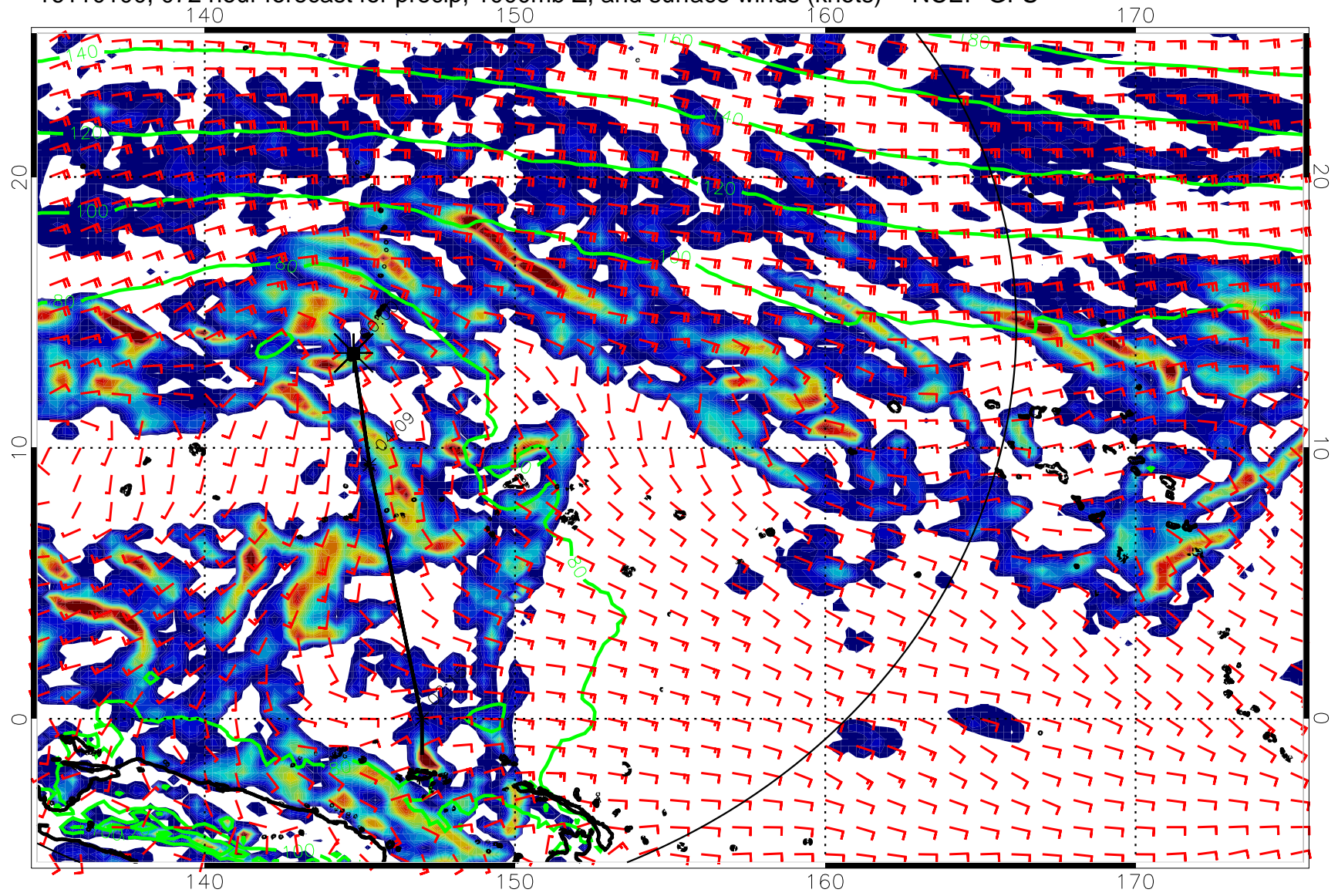
16110100, 072 hour forecast for precip, 1000mb Z, and surface winds (knots) -- NCEP GFS
