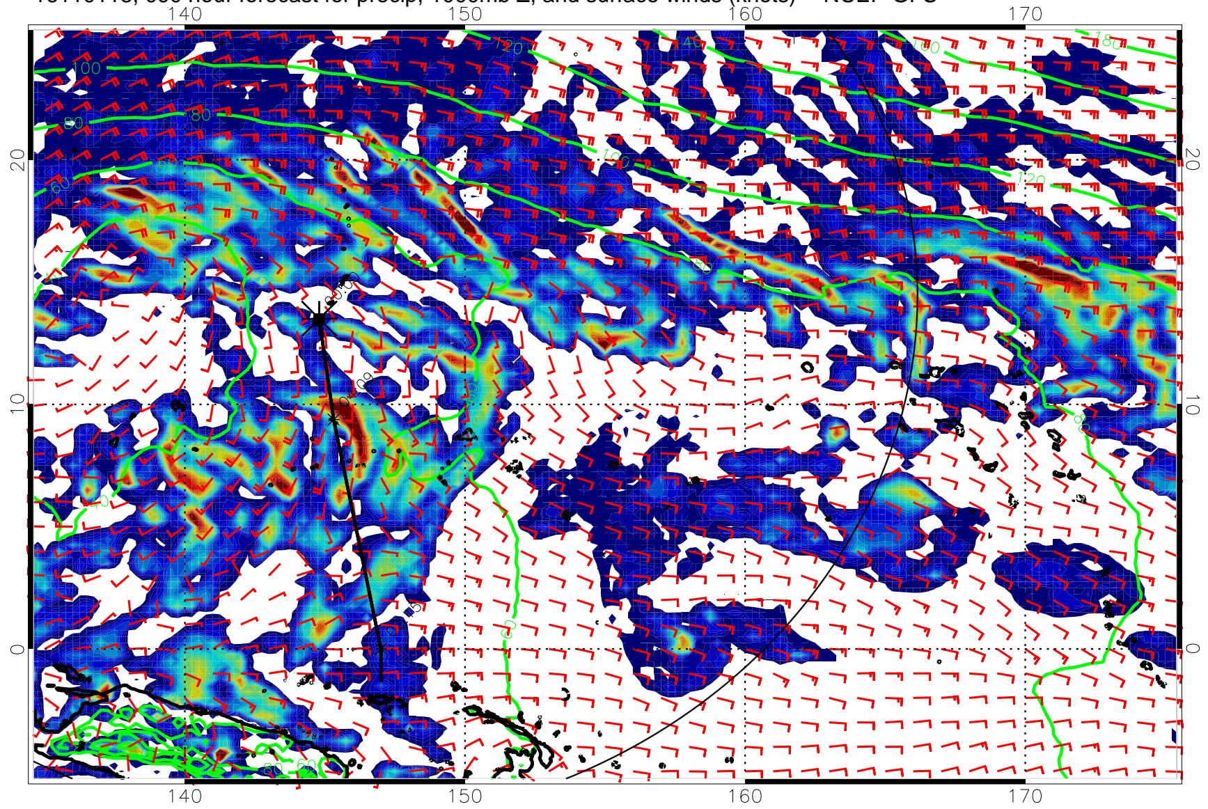
16110118, 090 hour forecast for precip, 1000mb Z, and surface winds (knots) -- NCEP GFS
