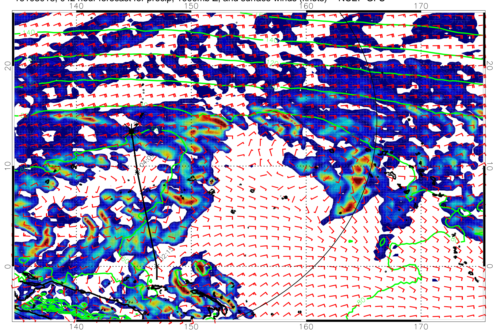
16103018, 042 hour forecast for precip, 1000mb Z, and surface winds (knots) -- NCEP GFS
