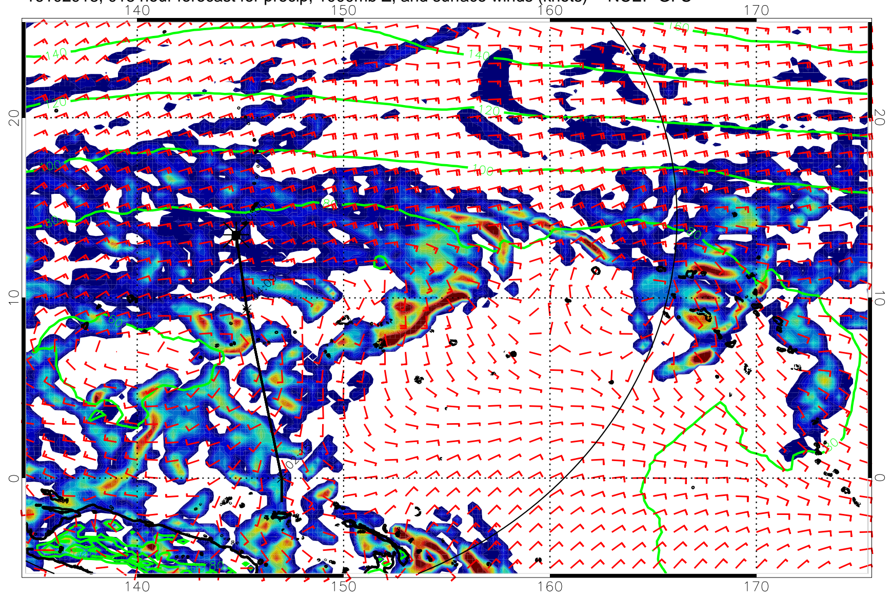
16102918, 018 hour forecast for precip, 1000mb Z, and surface winds (knots) -- NCEP GFS
