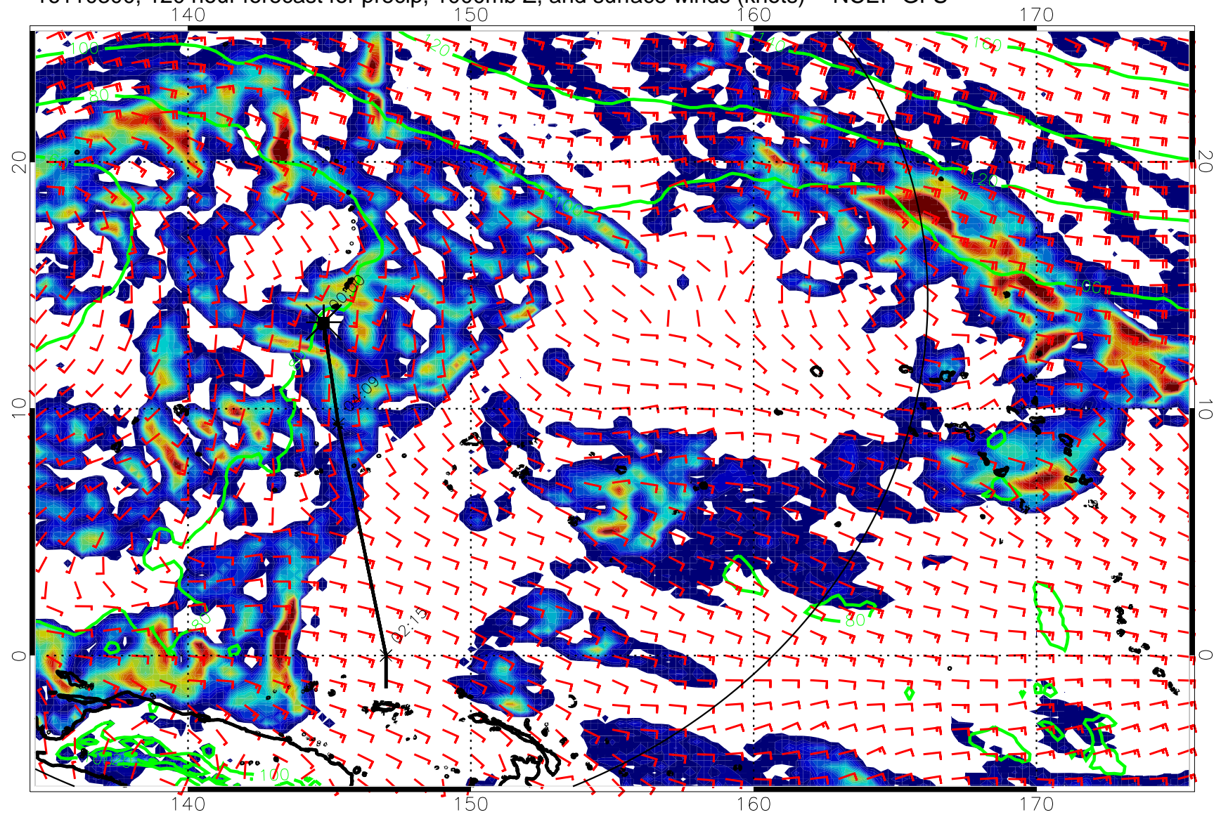
16110300, 120 hour forecast for precip, 1000mb Z, and surface winds (knots) -- NCEP GFS
