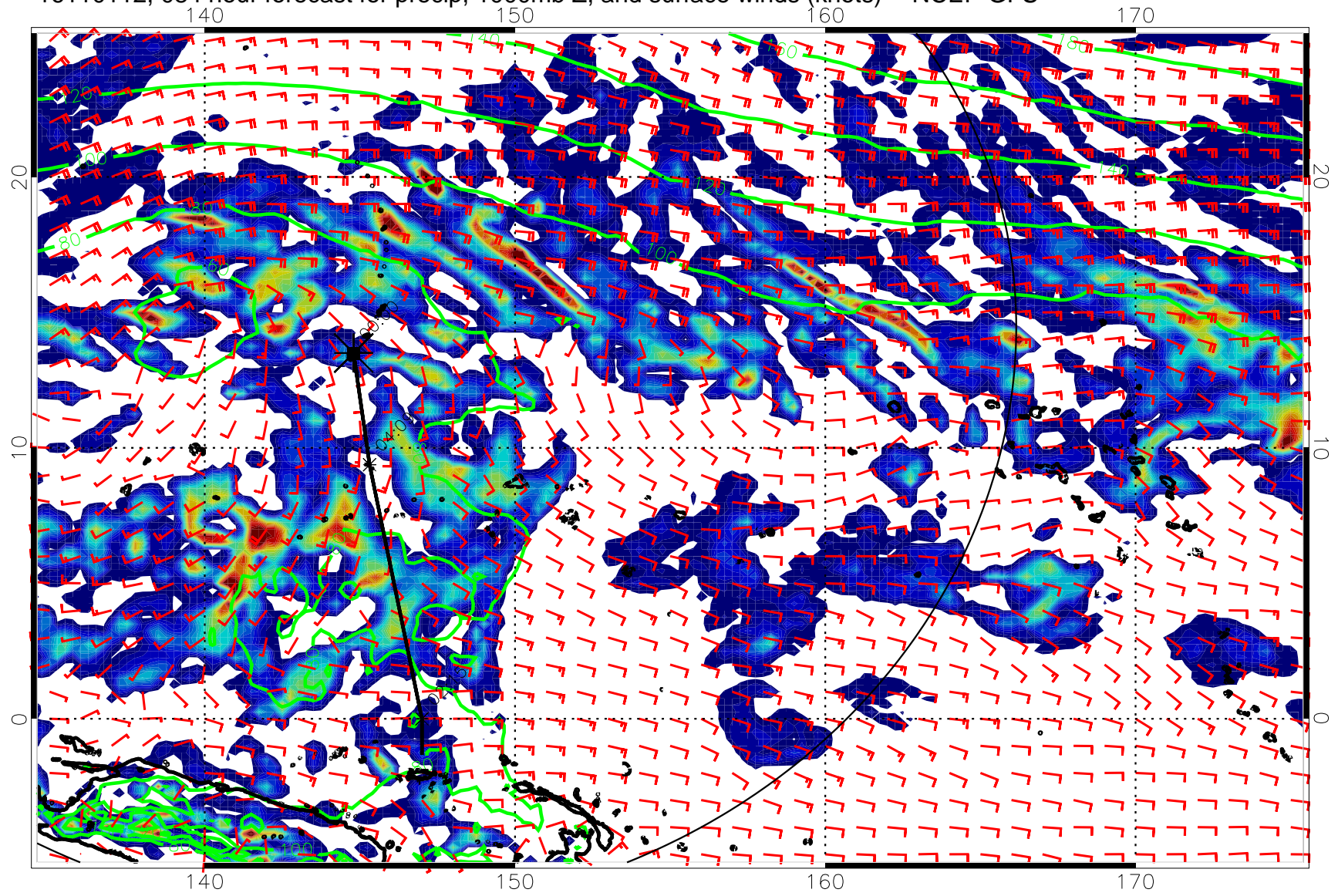
16110112, 084 hour forecast for precip, 1000mb Z, and surface winds (knots) -- NCEP GFS
