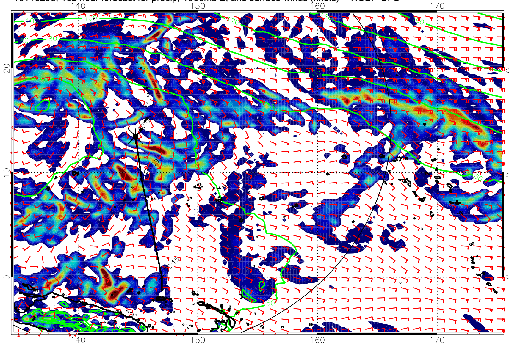
16110206, 102 hour forecast for precip, 1000mb Z, and surface winds (knots) -- NCEP GFS
