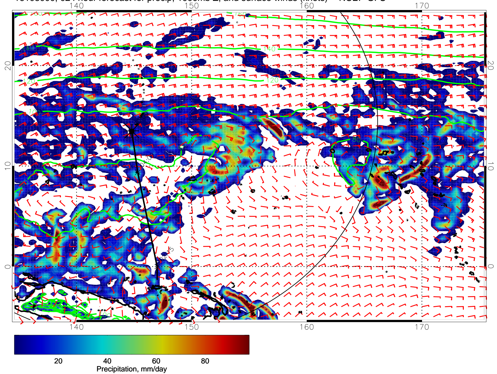
16103000, 024 hour forecast for precip, 1000mb Z, and surface winds (knots) -- NCEP GFS
