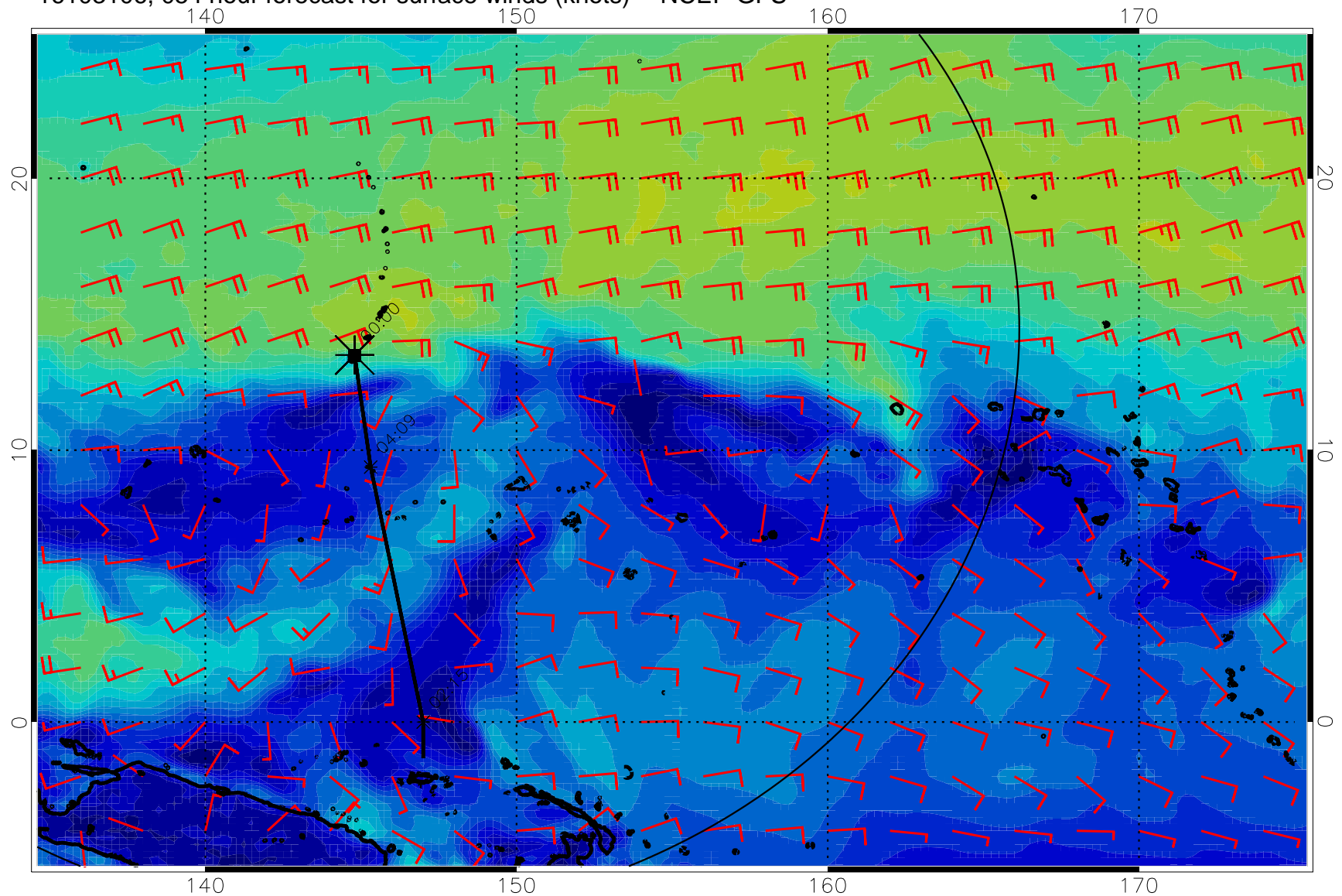
16103106, 054 hour forecast for surface winds (knots) -- NCEP GFS
