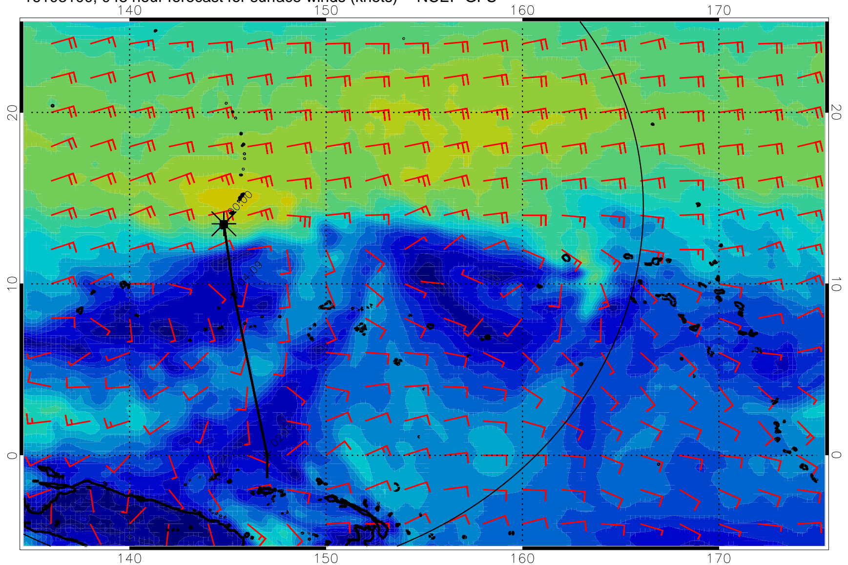
16103100, 048 hour forecast for surface winds (knots) -- NCEP GFS
