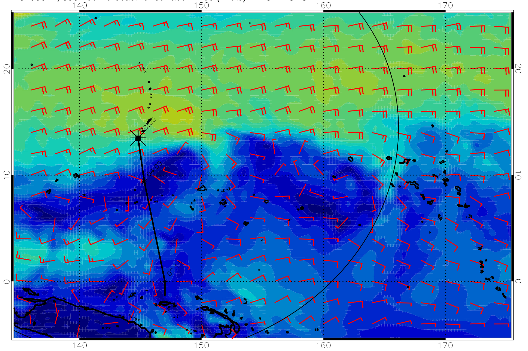
16103012, 036 hour forecast for surface winds (knots) -- NCEP GFS
