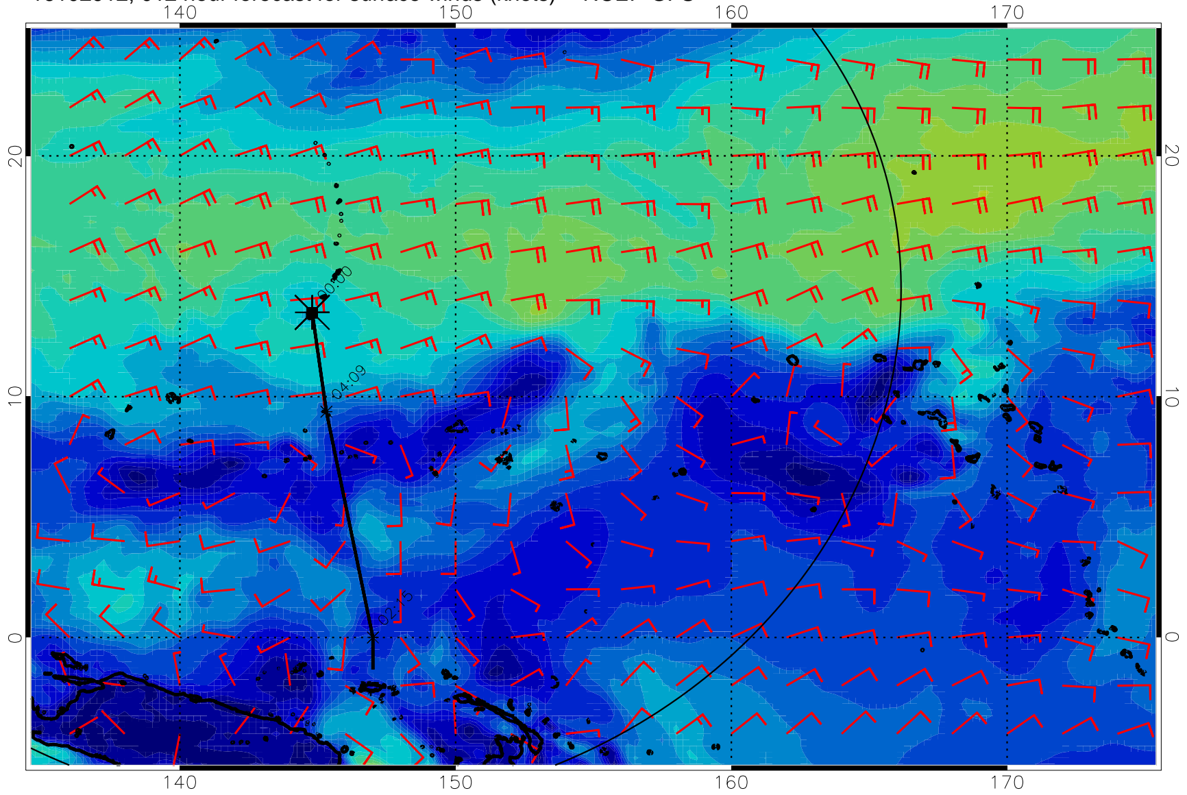
16102912, 012 hour forecast for surface winds (knots) -- NCEP GFS
