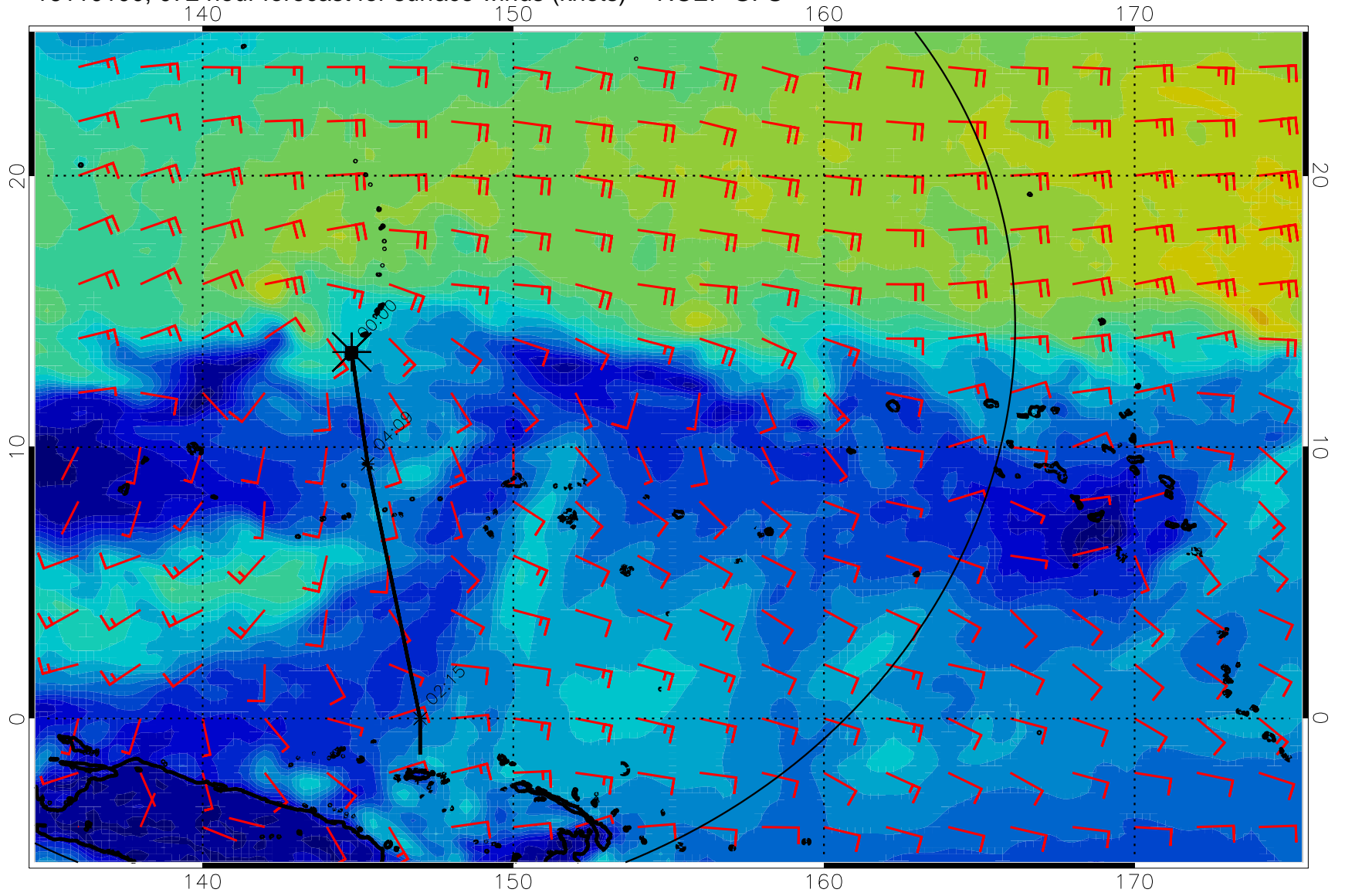
16110100, 072 hour forecast for surface winds (knots) -- NCEP GFS
