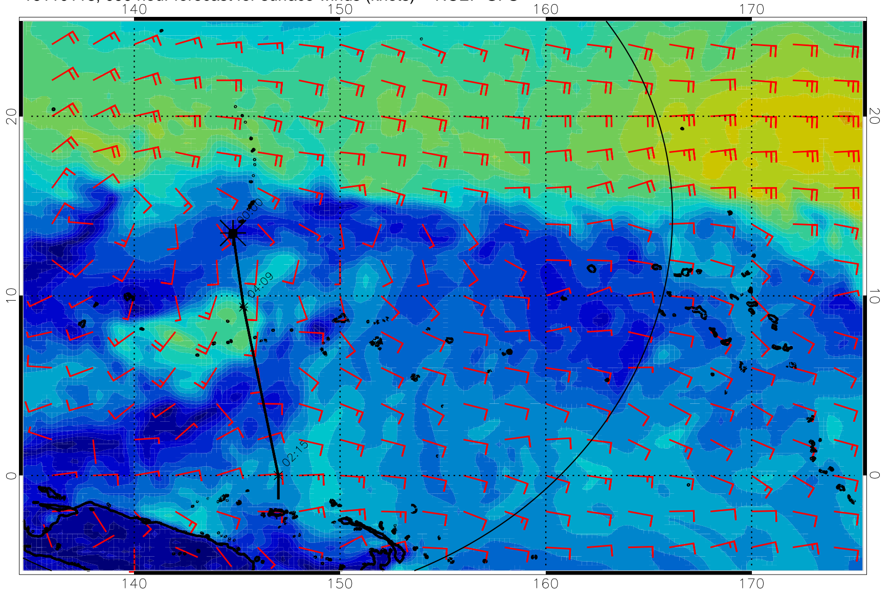
16110118, 090 hour forecast for surface winds (knots) -- NCEP GFS
