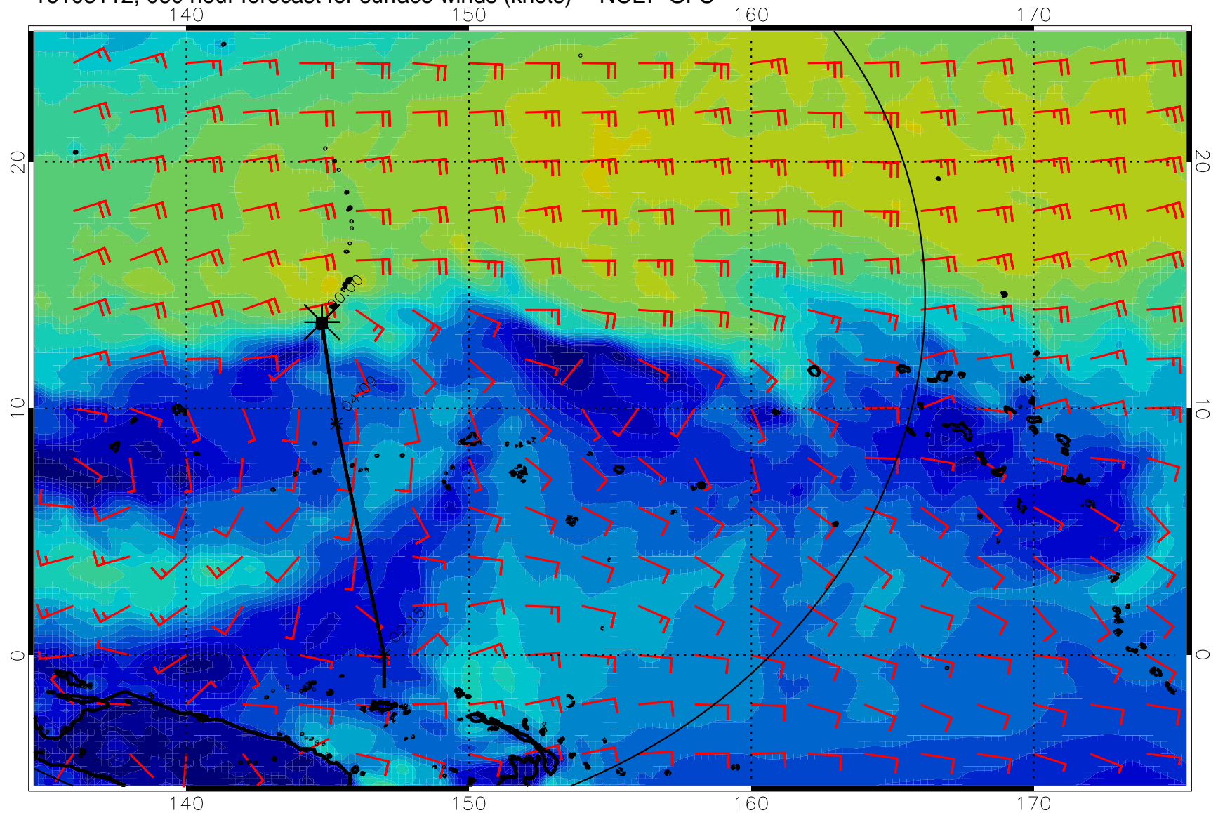
16103112, 060 hour forecast for surface winds (knots) -- NCEP GFS
