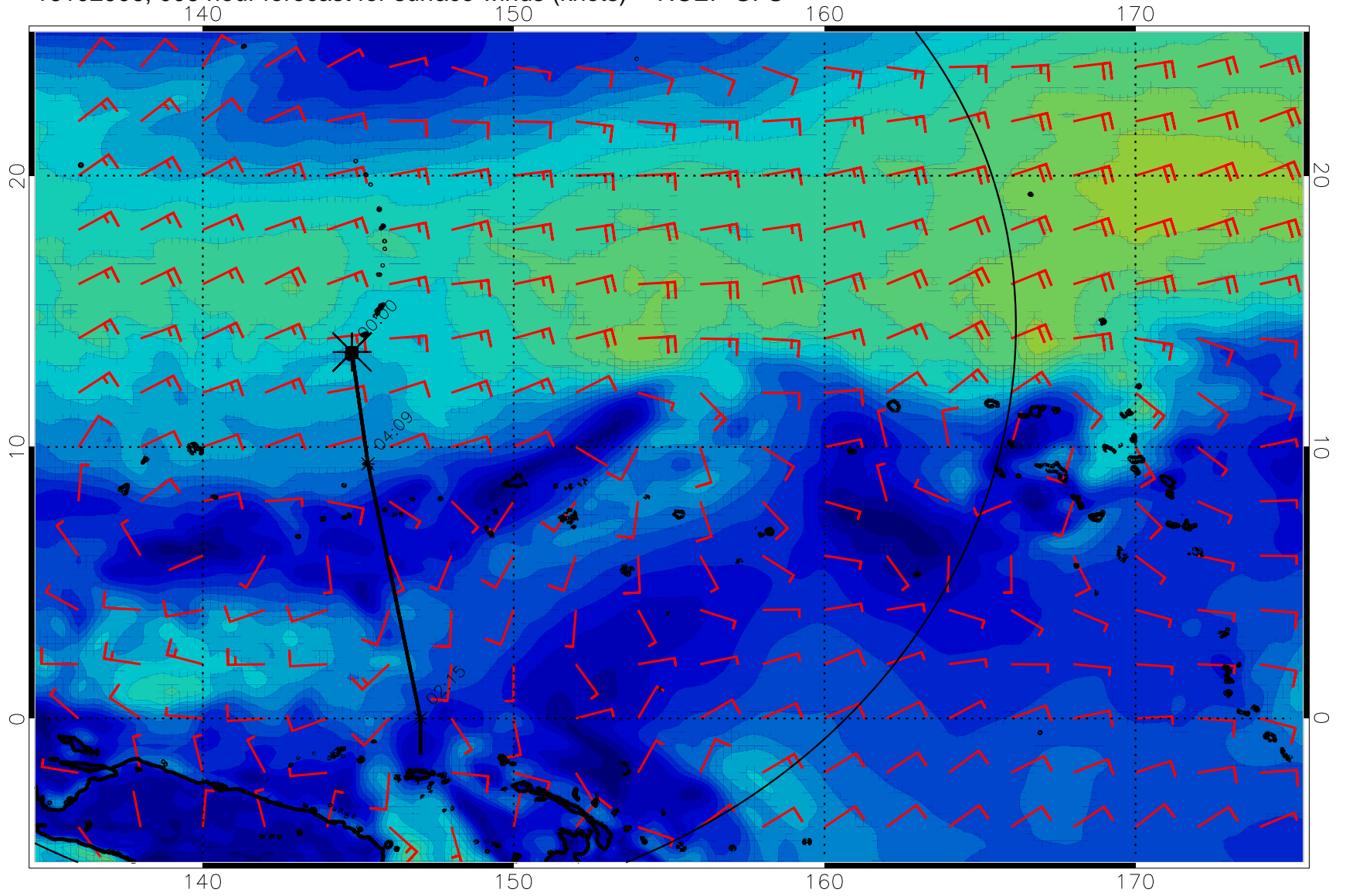
16102906, 006 hour forecast for surface winds (knots) -- NCEP GFS
