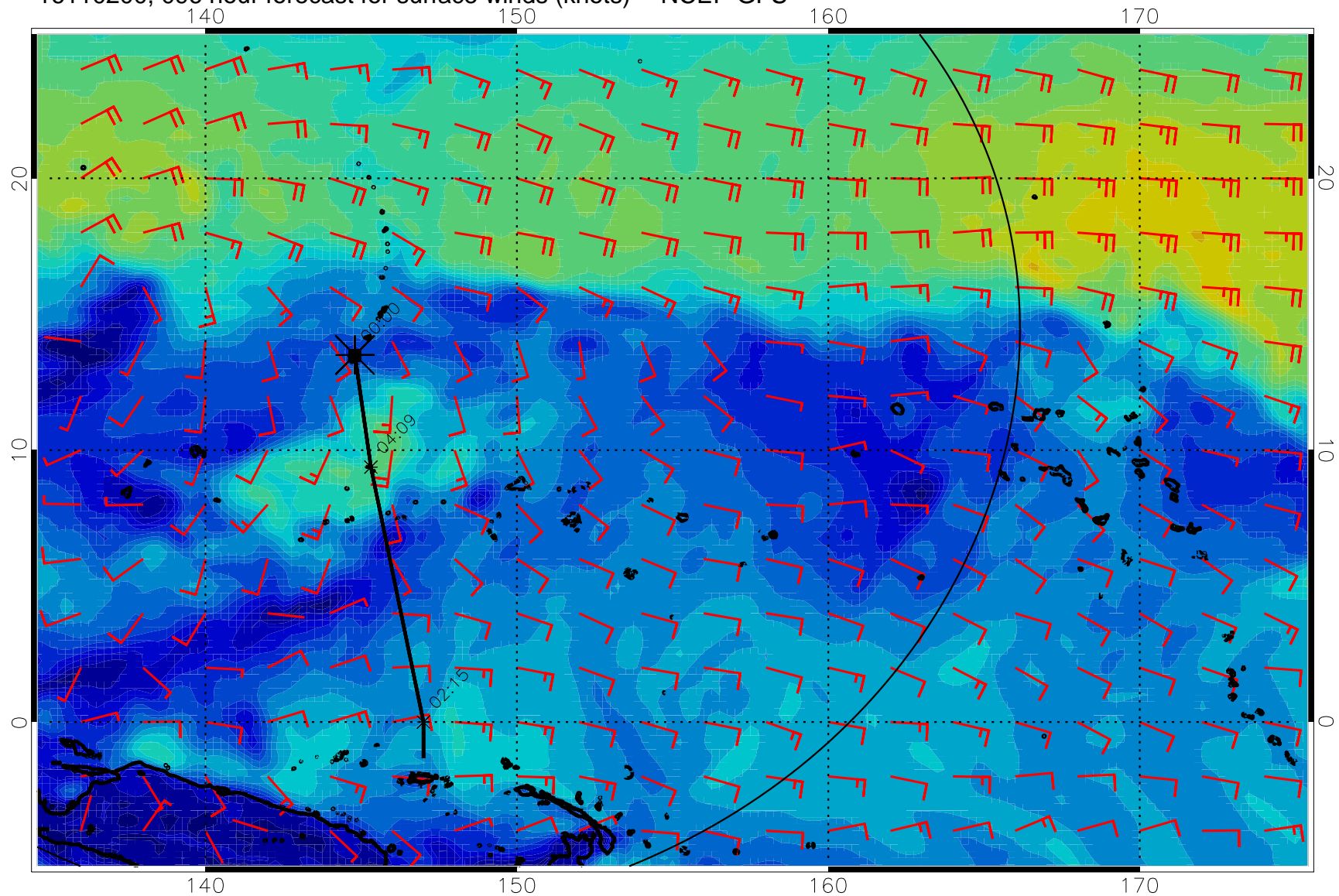
16110200, 096 hour forecast for surface winds (knots) -- NCEP GFS
