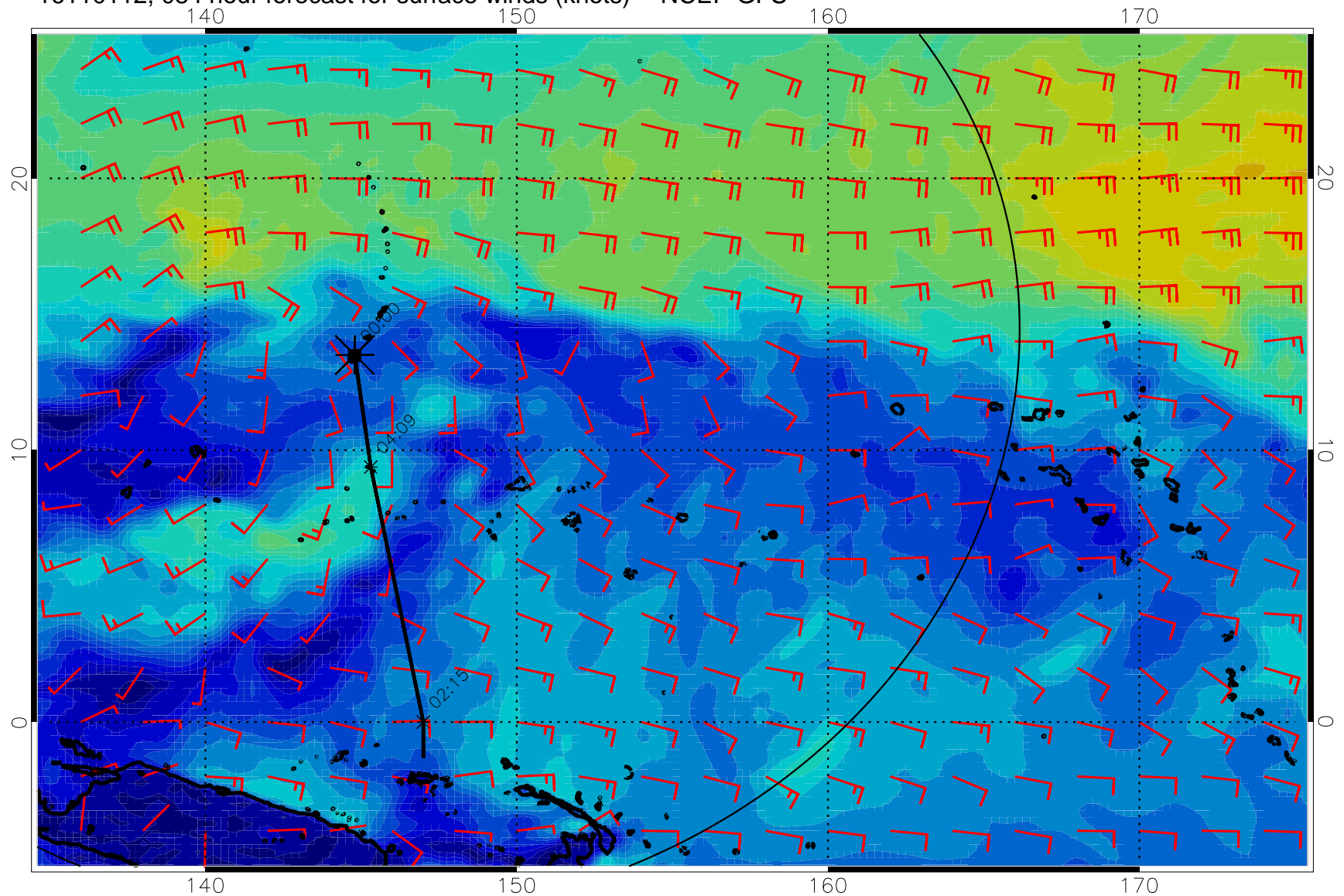
16110112, 084 hour forecast for surface winds (knots) -- NCEP GFS
