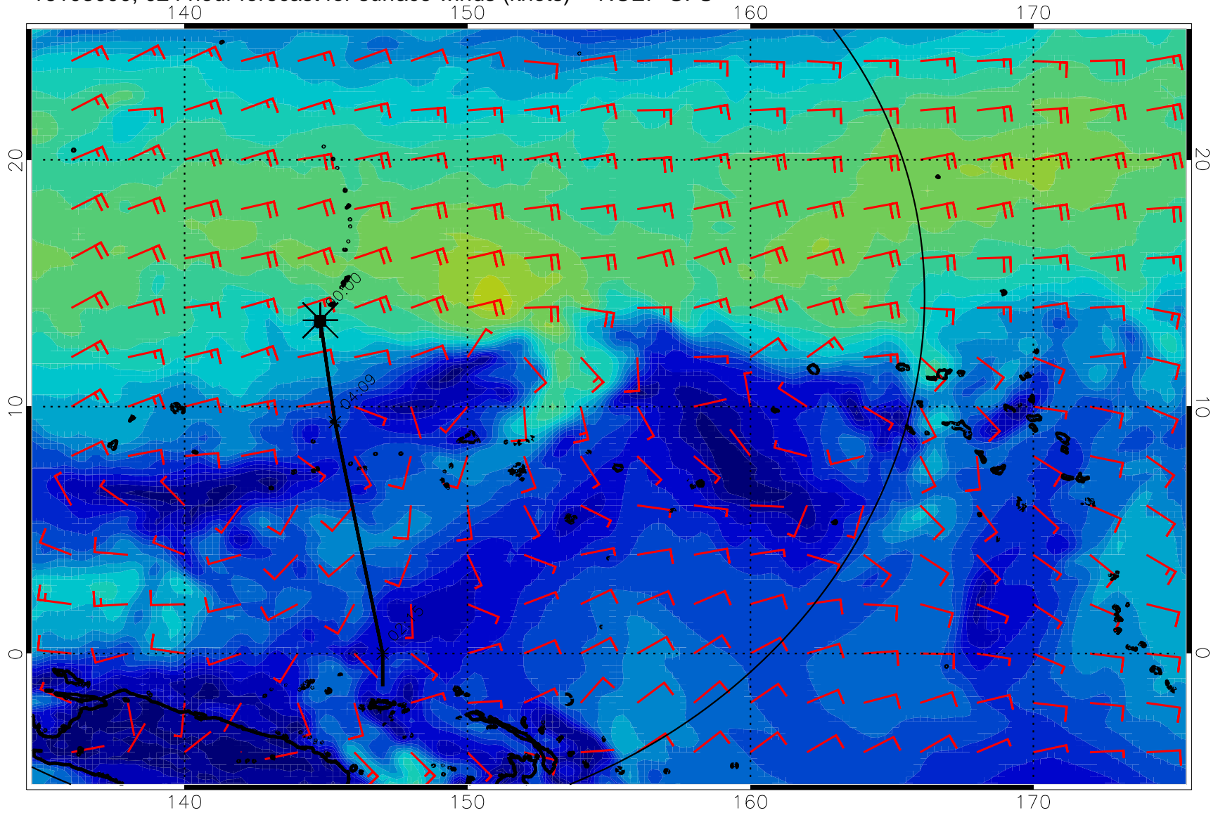
16103000, 024 hour forecast for surface winds (knots) -- NCEP GFS
