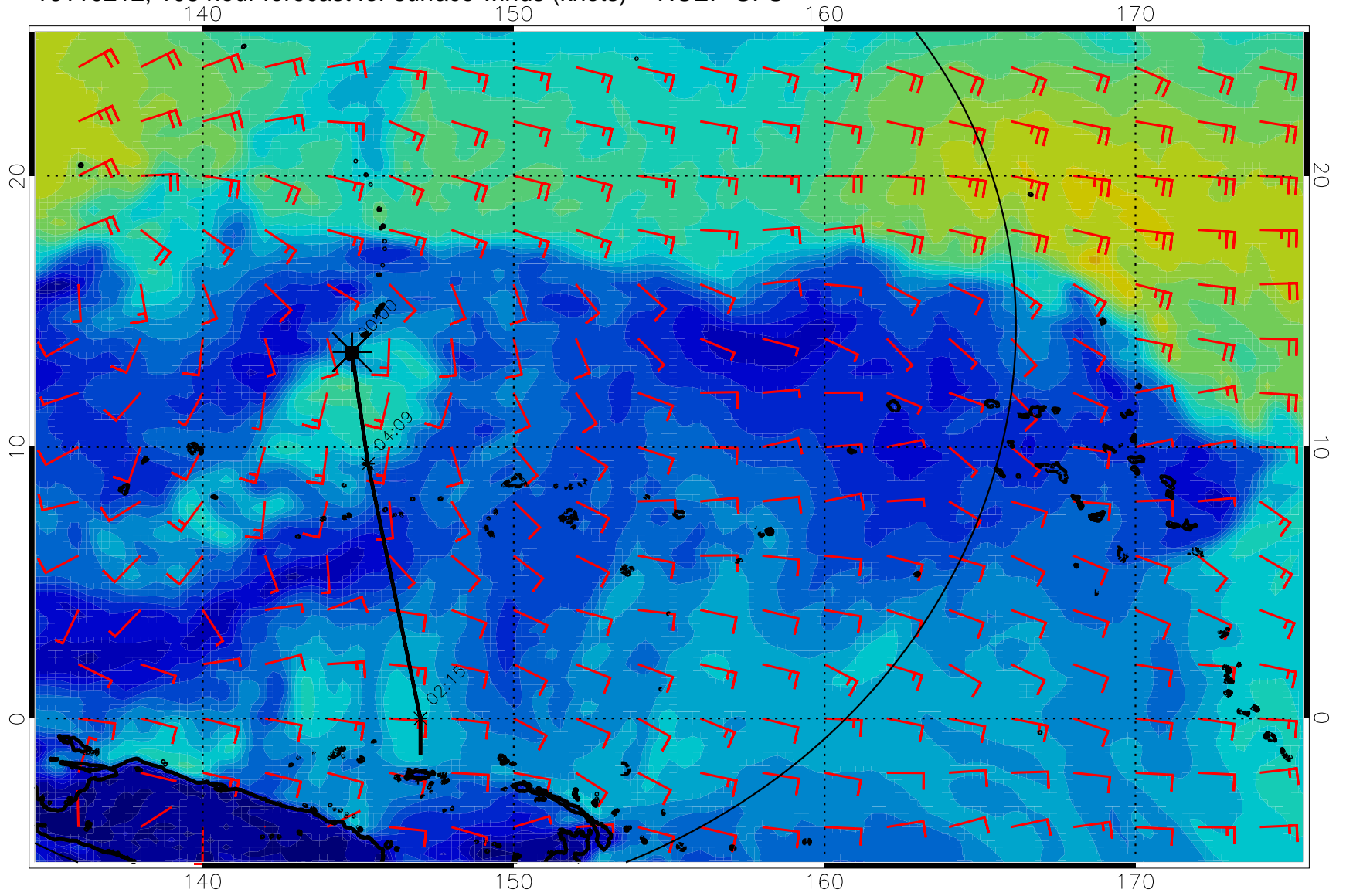
16110212, 108 hour forecast for surface winds (knots) -- NCEP GFS
