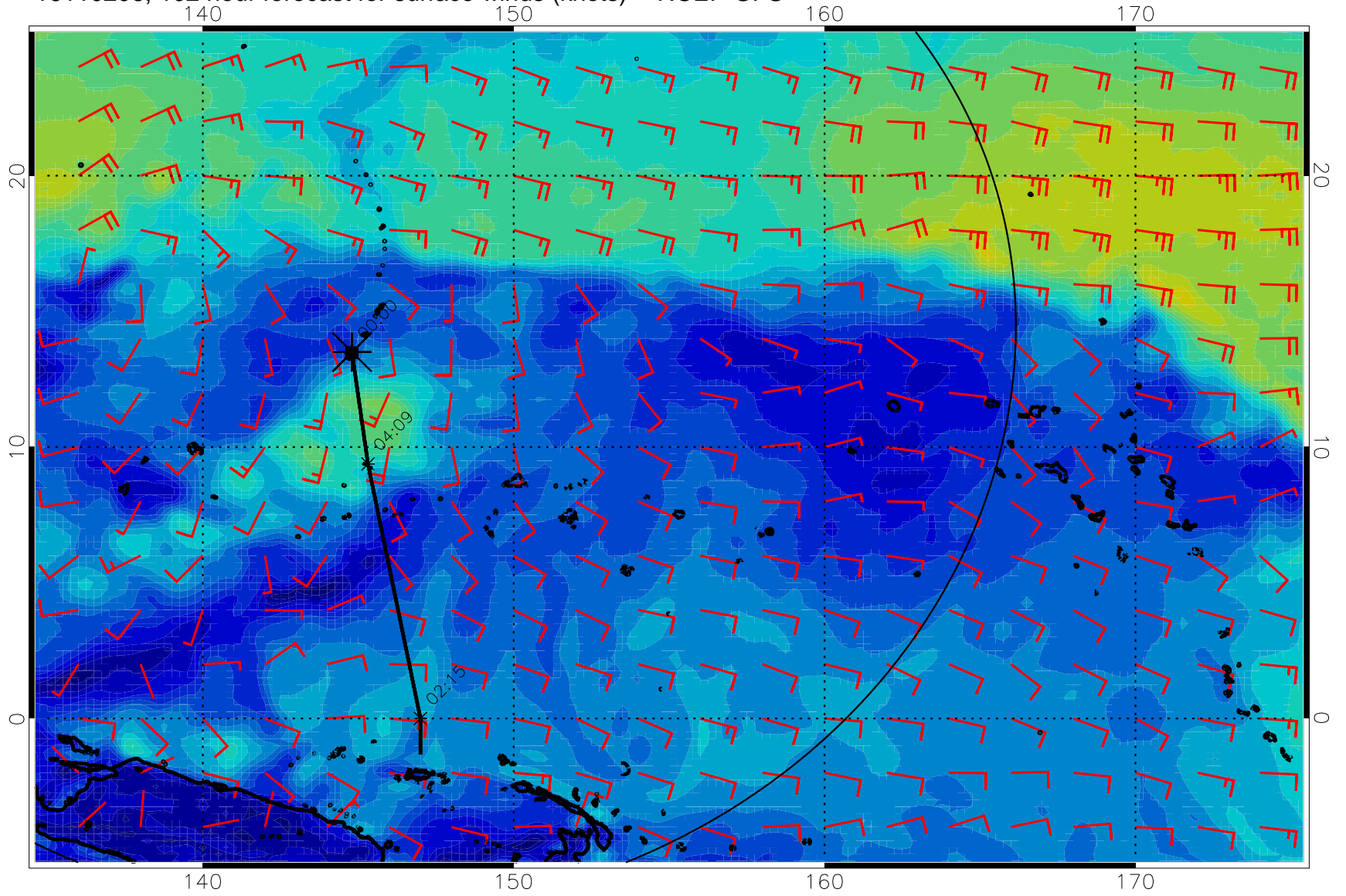
16110206, 102 hour forecast for surface winds (knots) -- NCEP GFS
