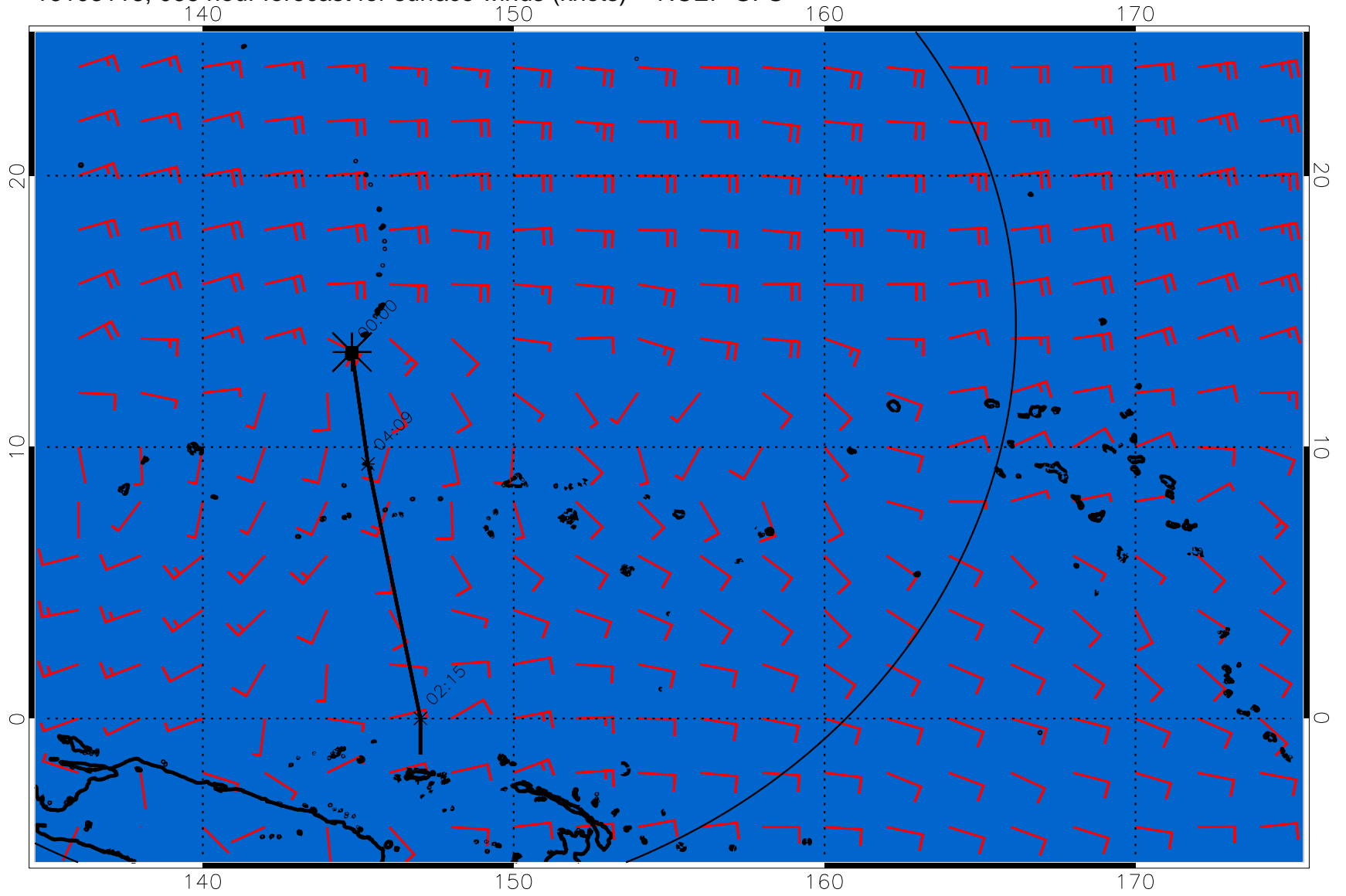
16103118, 066 hour forecast for surface winds (knots) -- NCEP GFS
