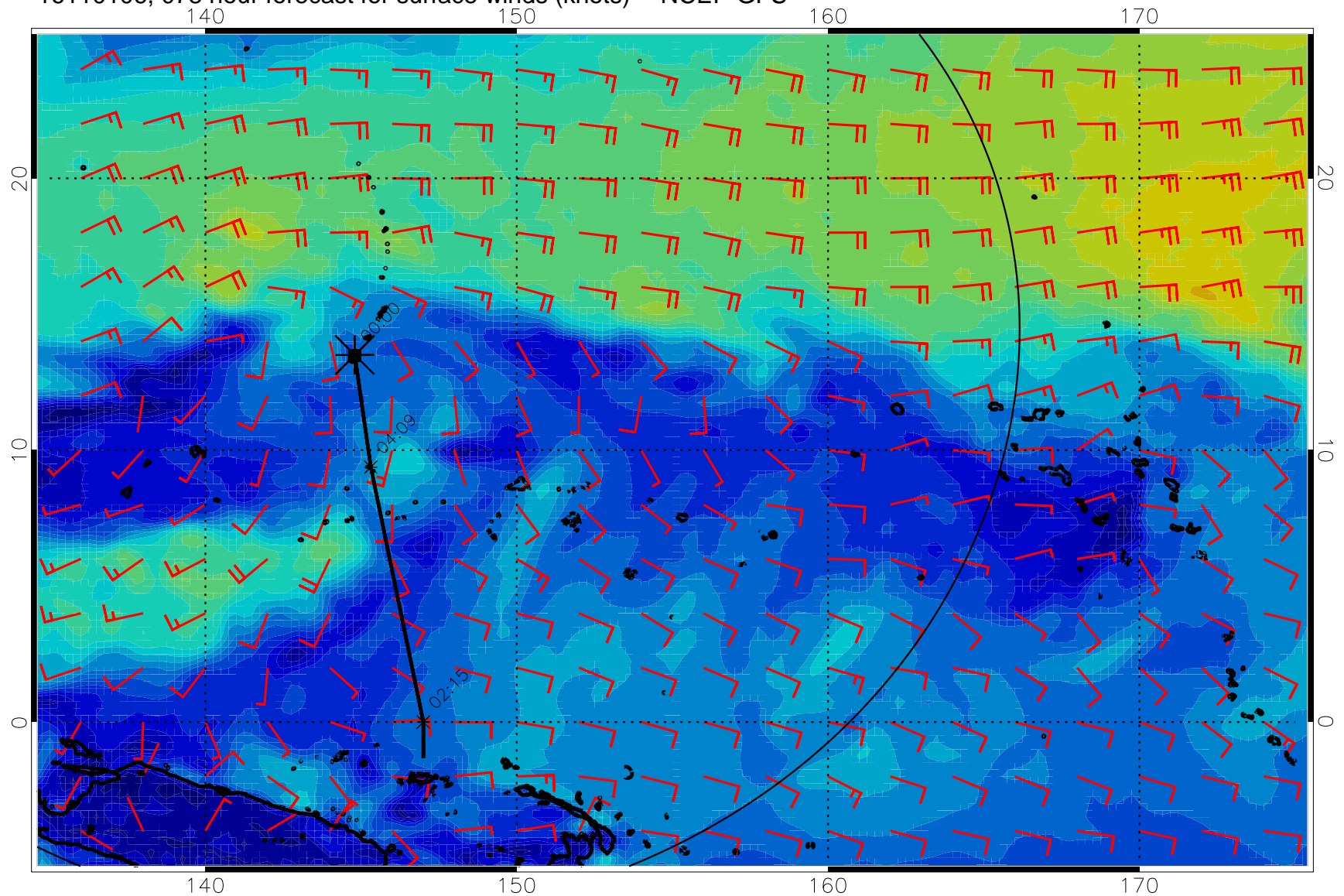
16110106, 078 hour forecast for surface winds (knots) -- NCEP GFS
