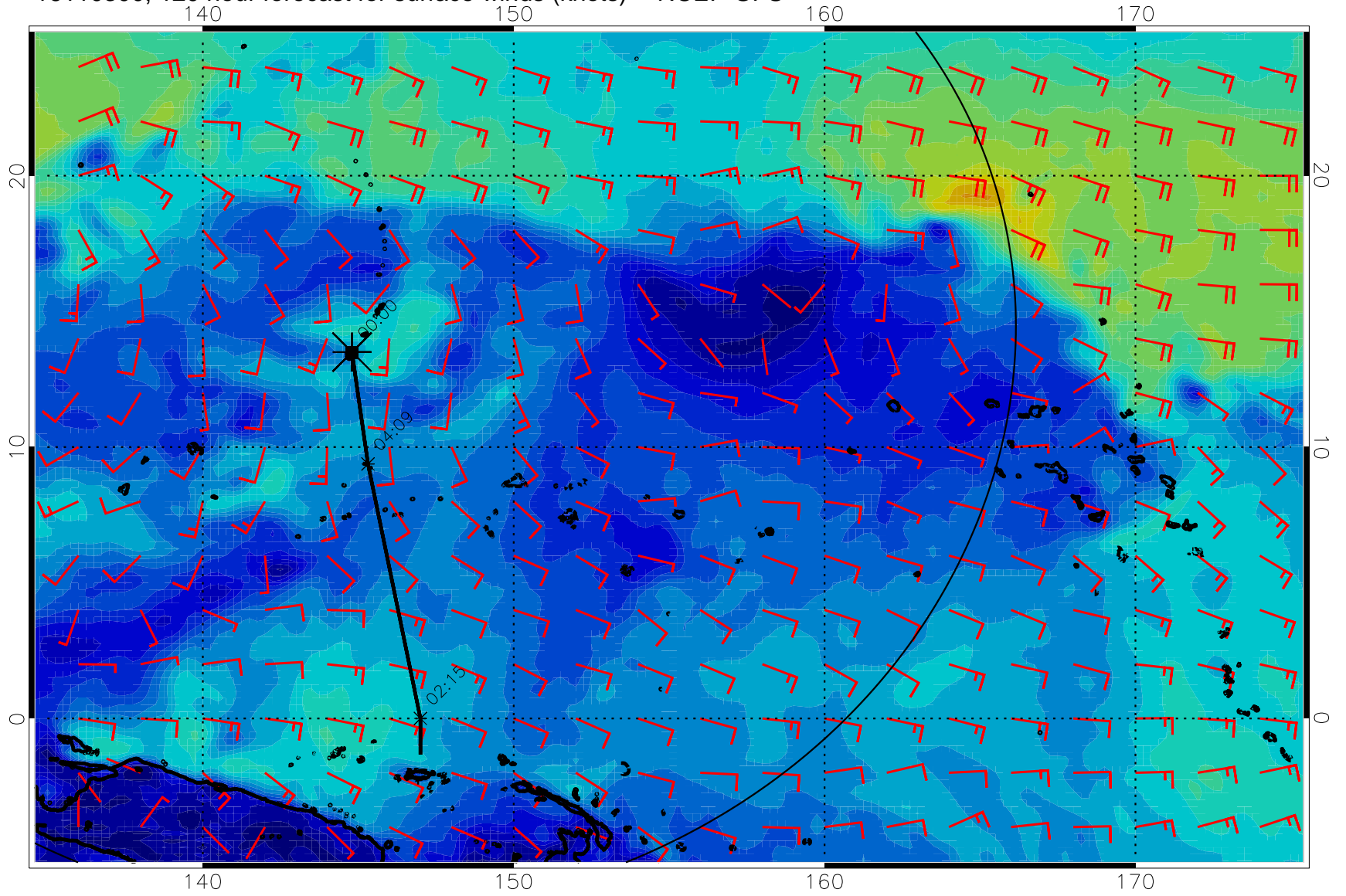
16110300, 120 hour forecast for surface winds (knots) -- NCEP GFS
