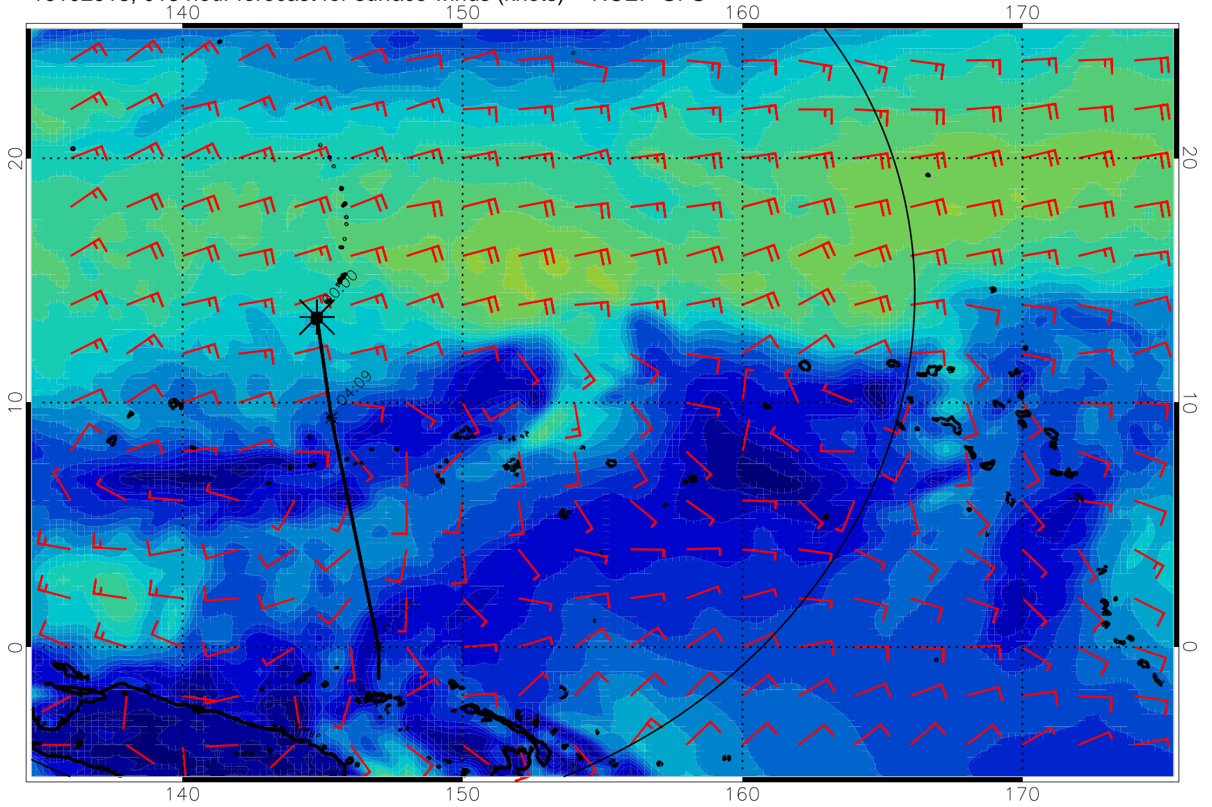
16102918, 018 hour forecast for surface winds (knots) -- NCEP GFS
