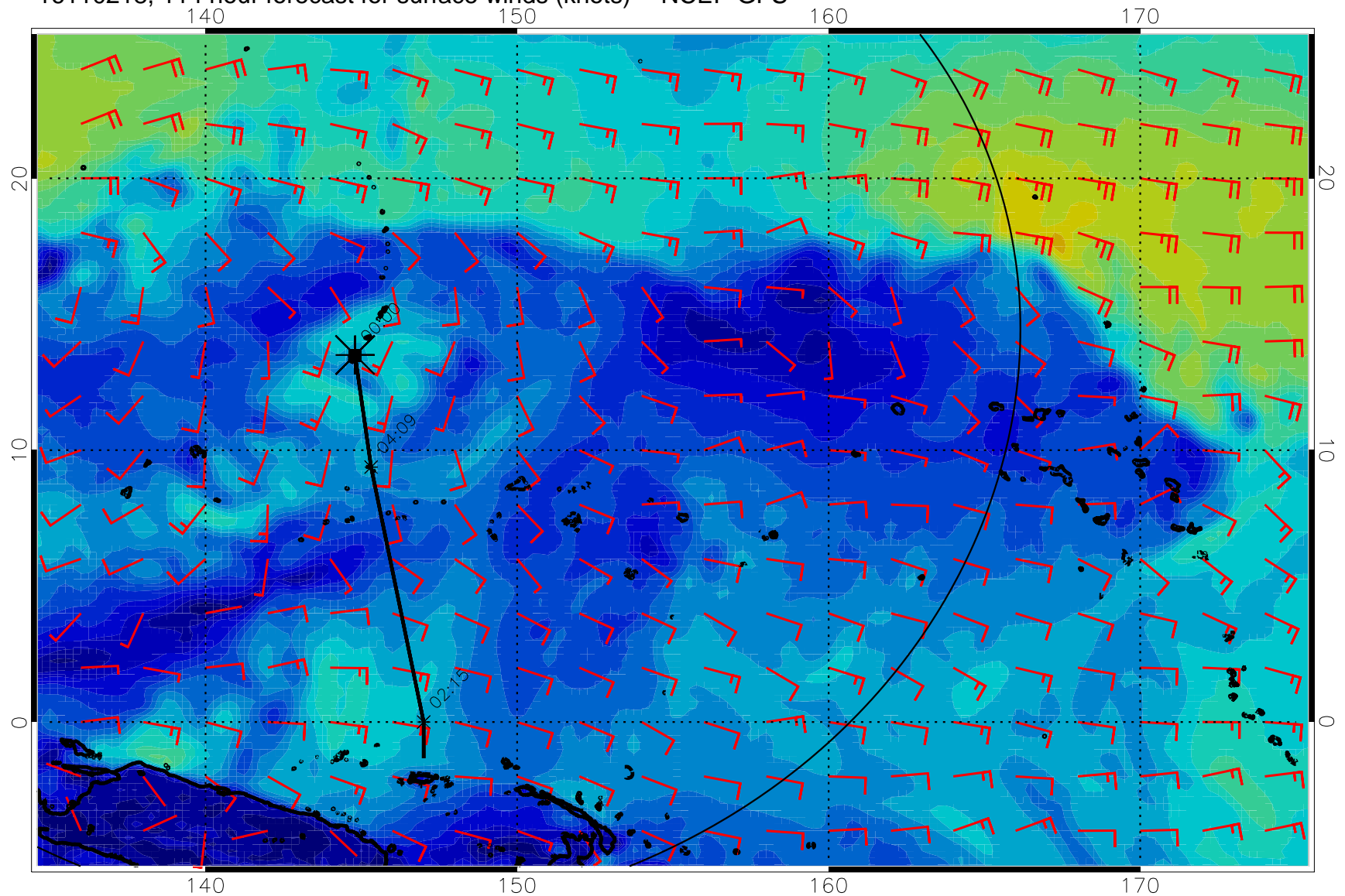
16110218, 114 hour forecast for surface winds (knots) -- NCEP GFS
