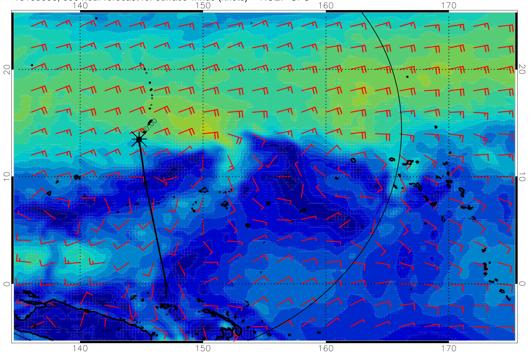
16103006, 0300 hour forecast for surface winds (knots) -- NCEP GFS
