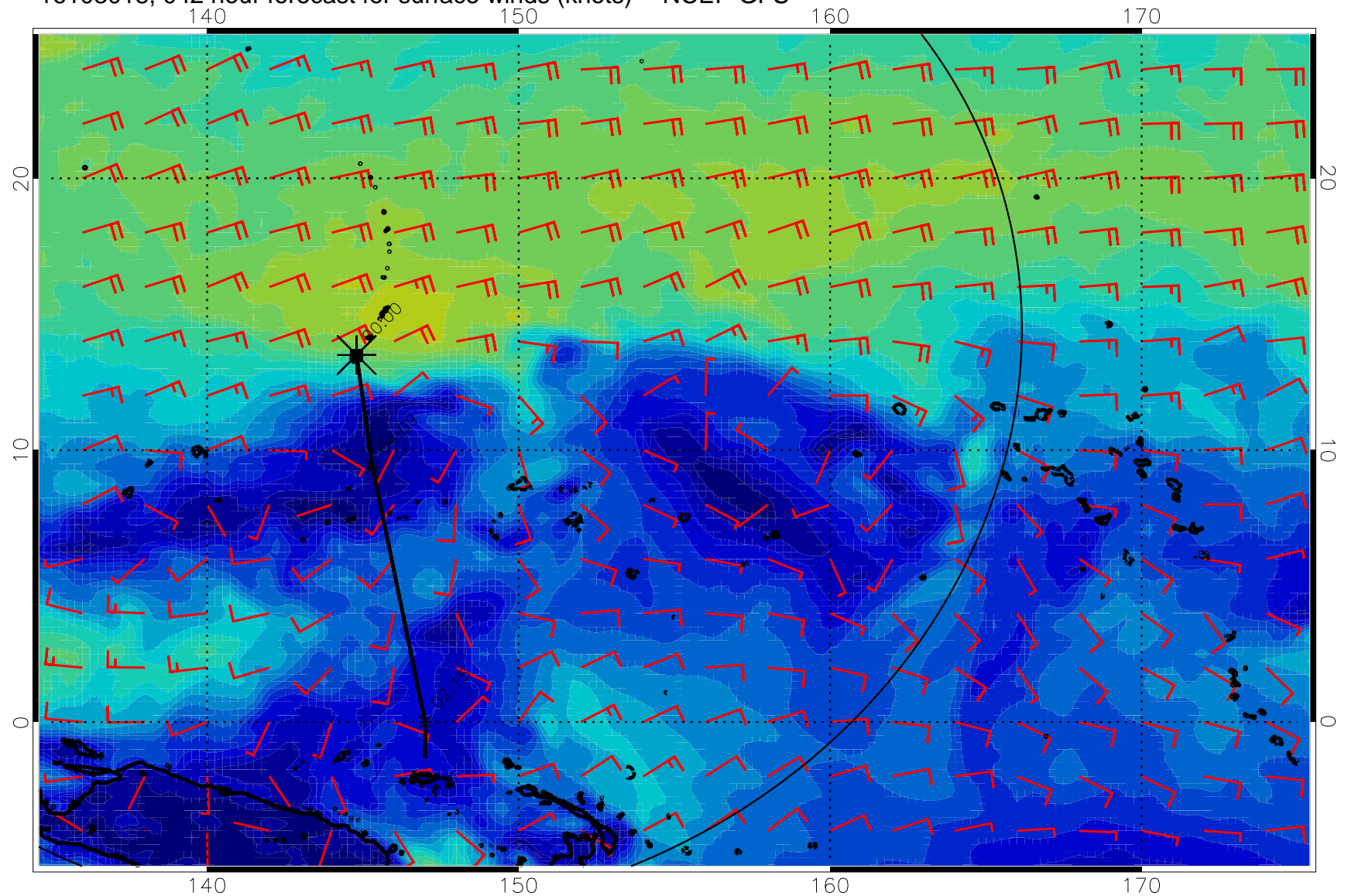
16103018, 042 hour forecast for surface winds (knots) -- NCEP GFS
