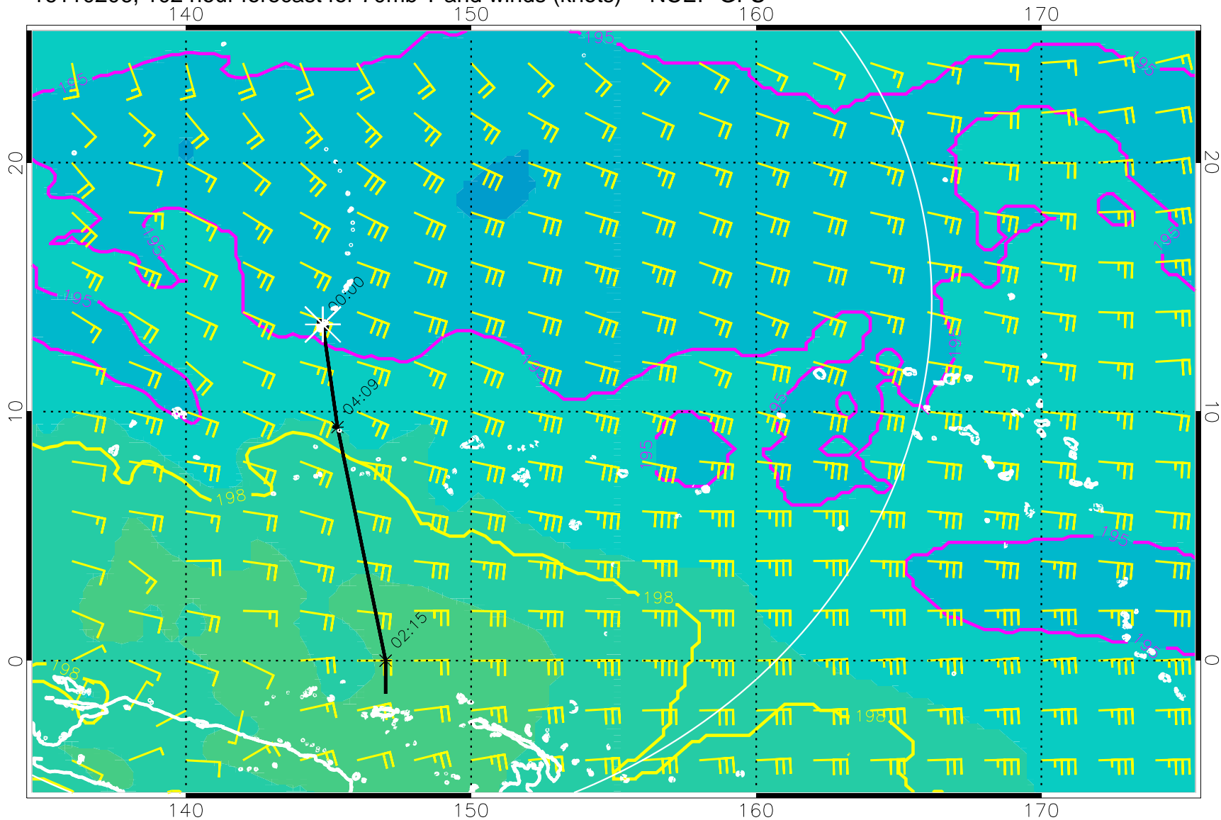
16110206, 102 hour forecast for 70mb T and winds (knots) -- NCEP GFS
