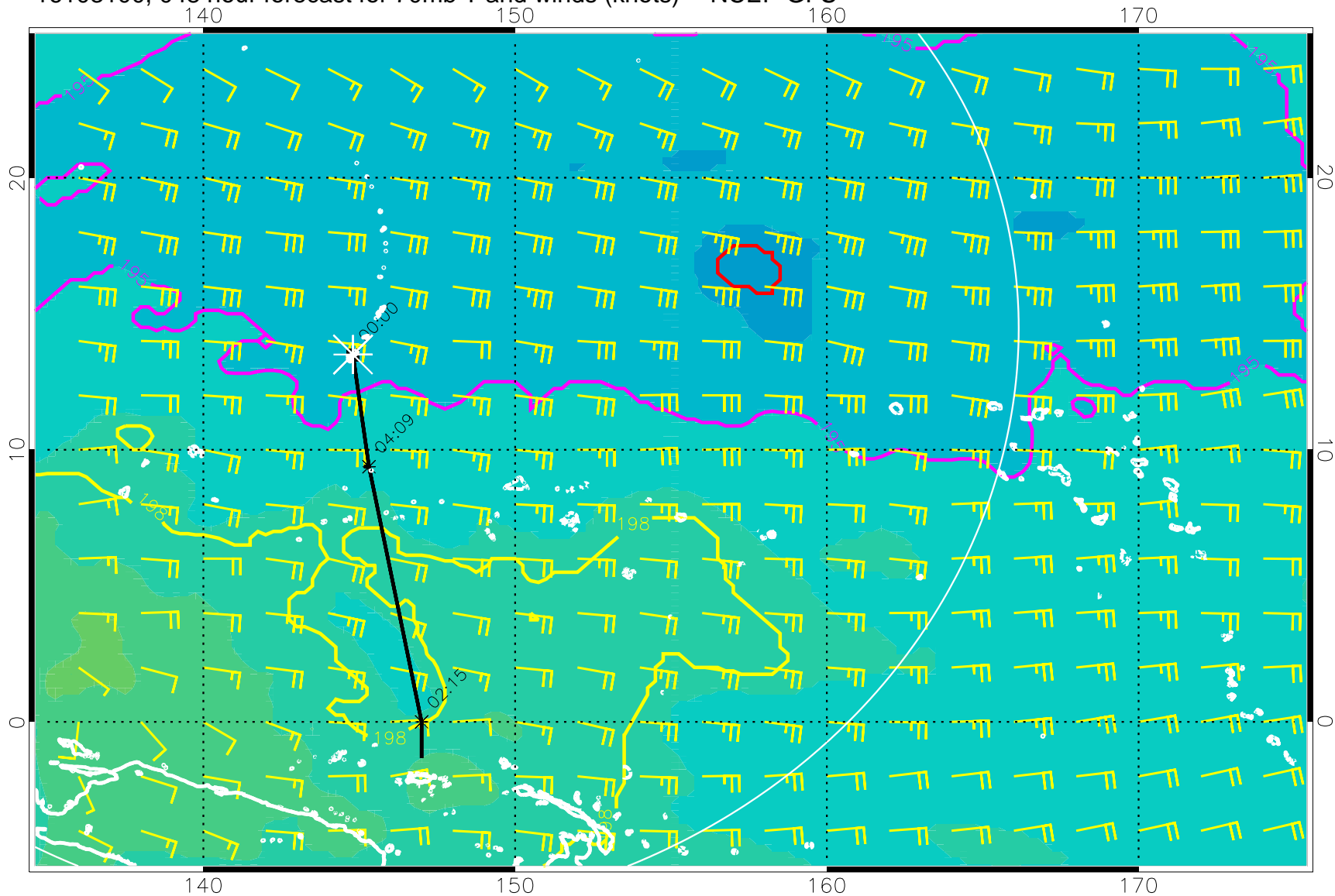
16103100, 048 hour forecast for 70mb T and winds (knots) -- NCEP GFS
