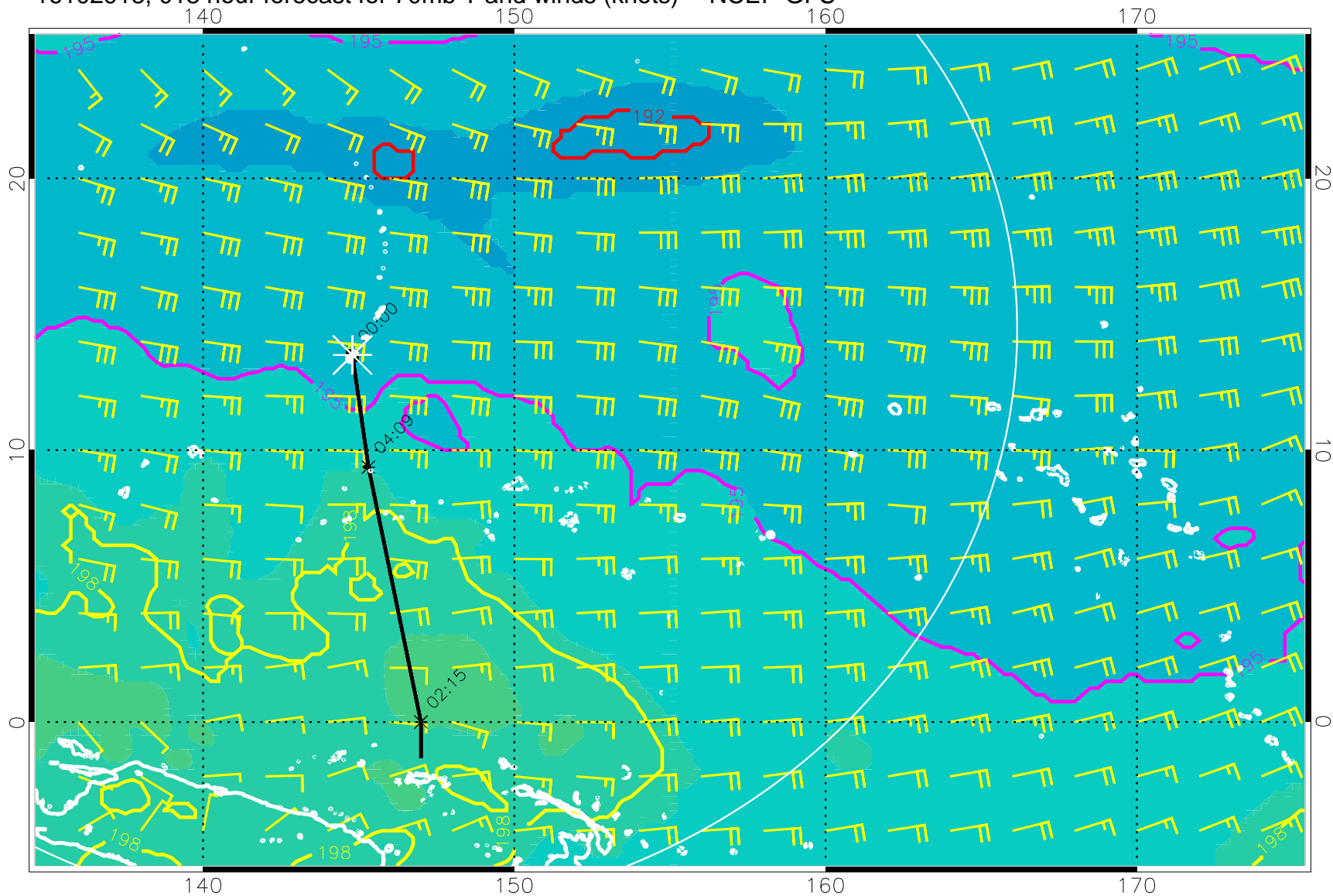
16102918, 018 hour forecast for 70mb T and winds (knots) -- NCEP GFS
