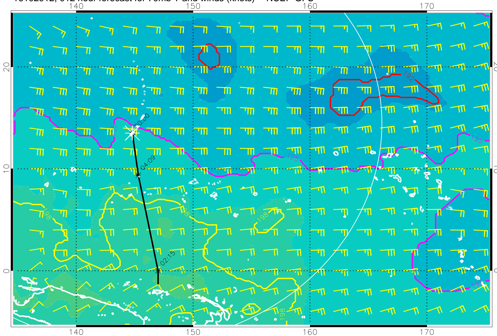
16102912, 012 hour forecast for 70mb T and winds (knots) -- NCEP GFS
