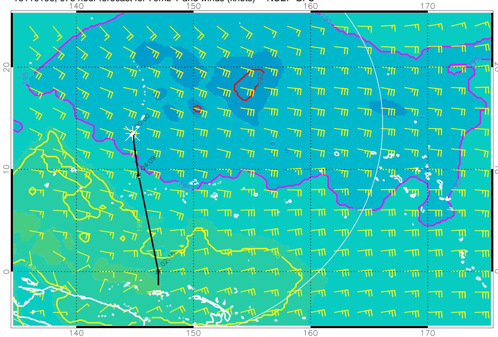
16110106, 078 hour forecast for 70mb T and winds (knots) -- NCEP GFS
