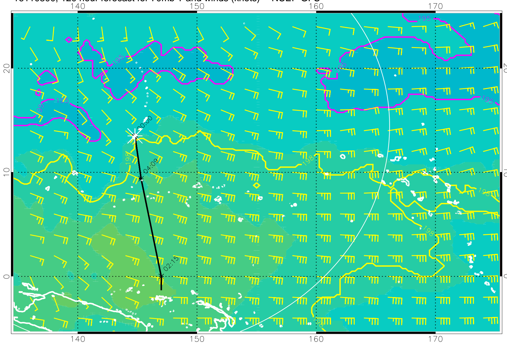
16110300, 120 hour forecast for 70mb T and winds (knots) -- NCEP GFS
