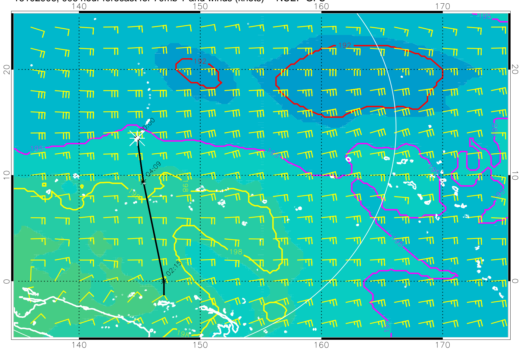
16102906, 006 hour forecast for 70mb T and winds (knots) -- NCEP GFS
