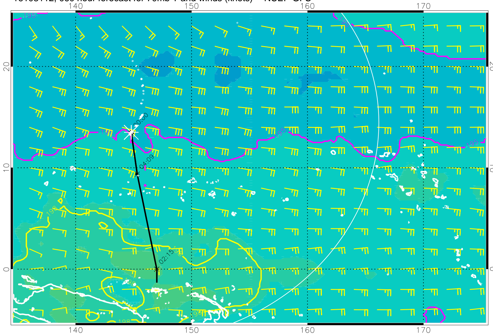
16103112, 060 hour forecast for 70mb T and winds (knots) -- NCEP GFS
