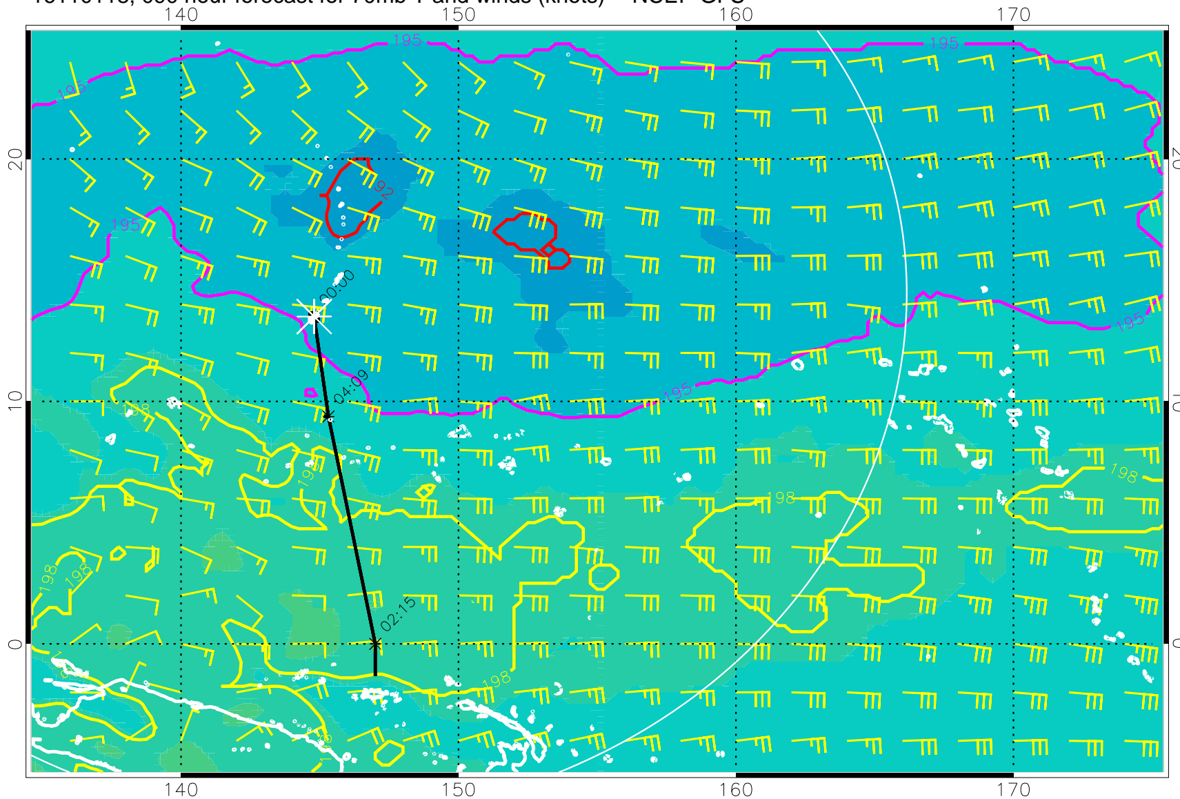
16110118, 090 hour forecast for 70mb T and winds (knots) -- NCEP GFS
