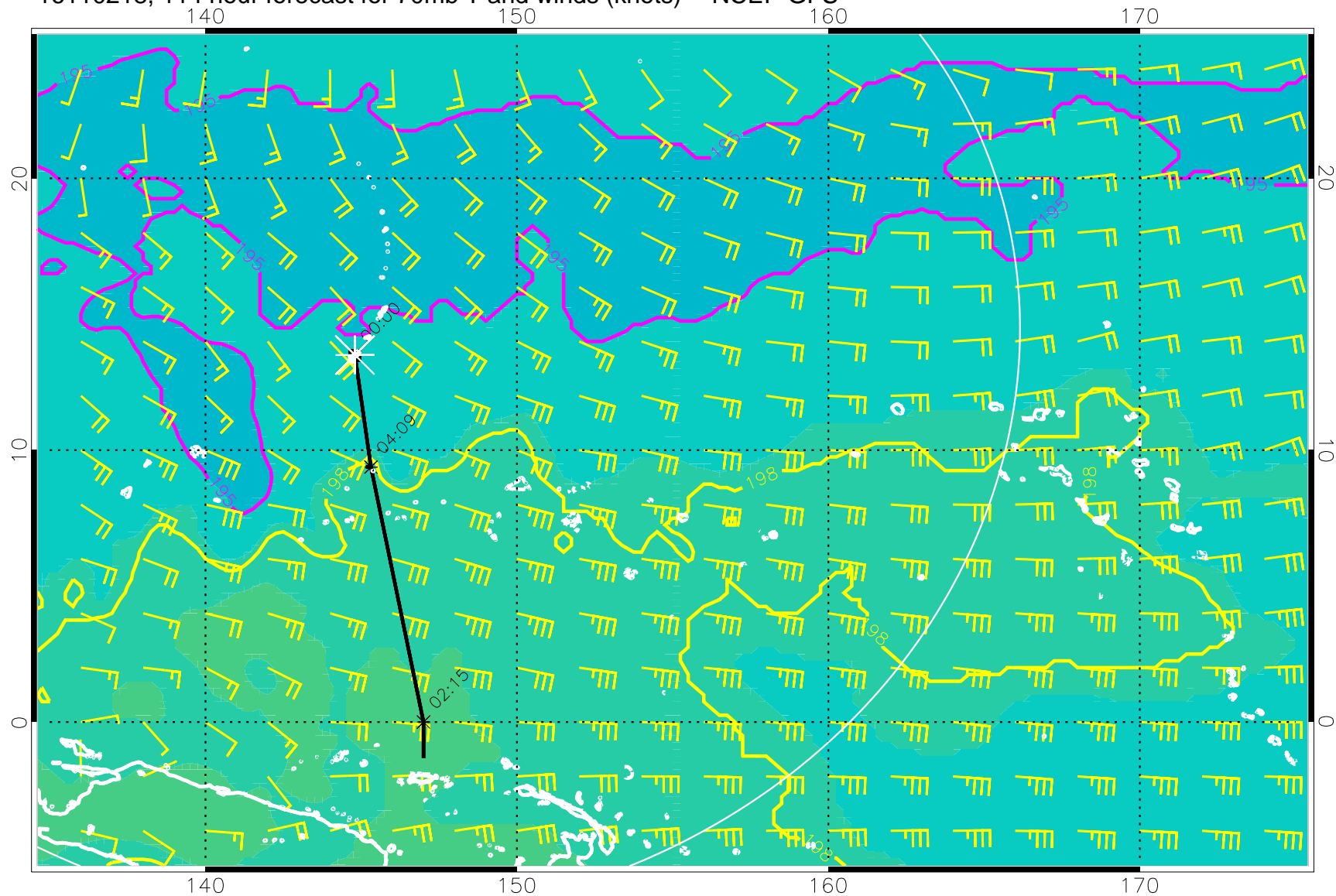
16110218, 114 hour forecast for 70mb T and winds (knots) -- NCEP GFS
