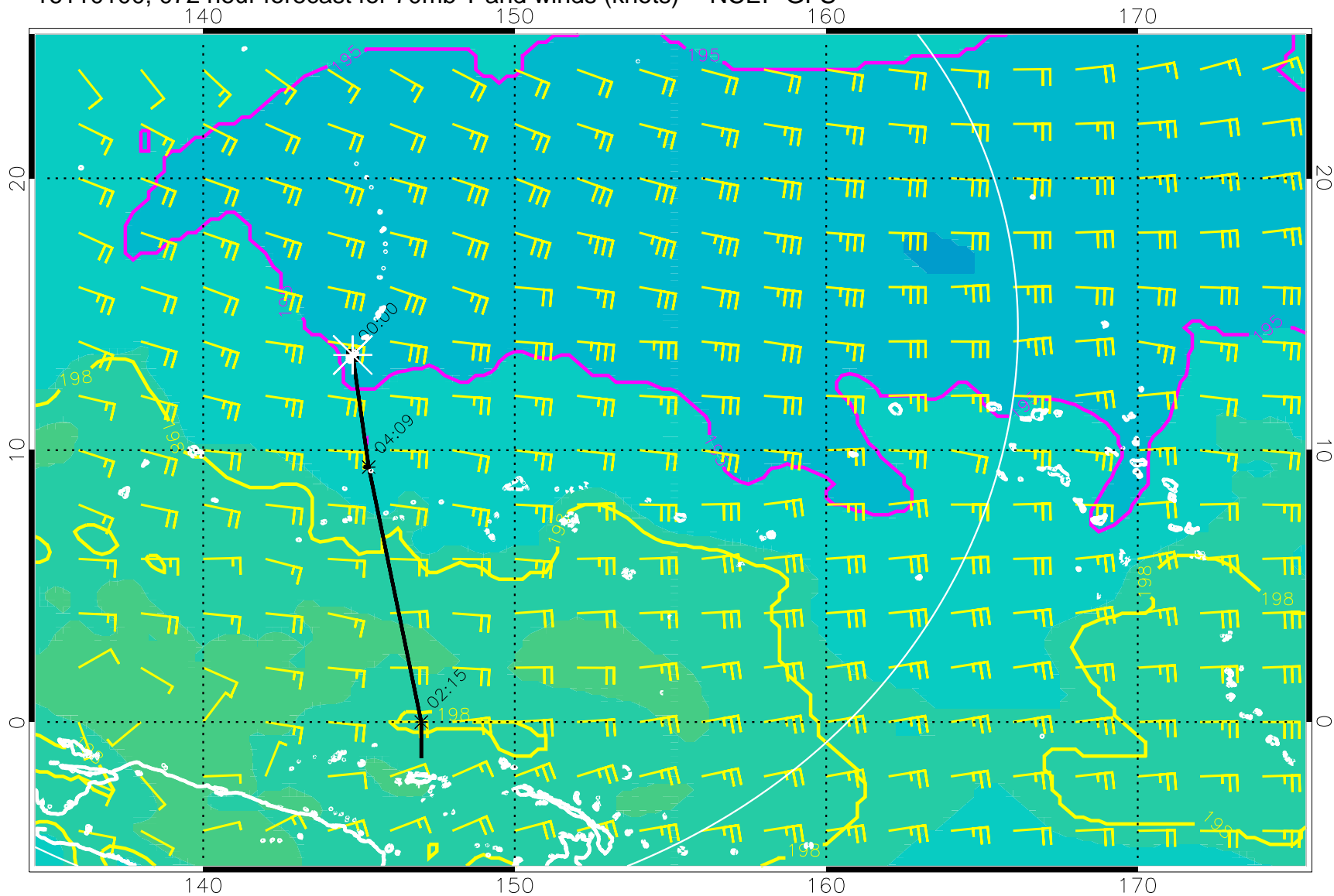
16110100, 072 hour forecast for 70mb T and winds (knots) -- NCEP GFS
