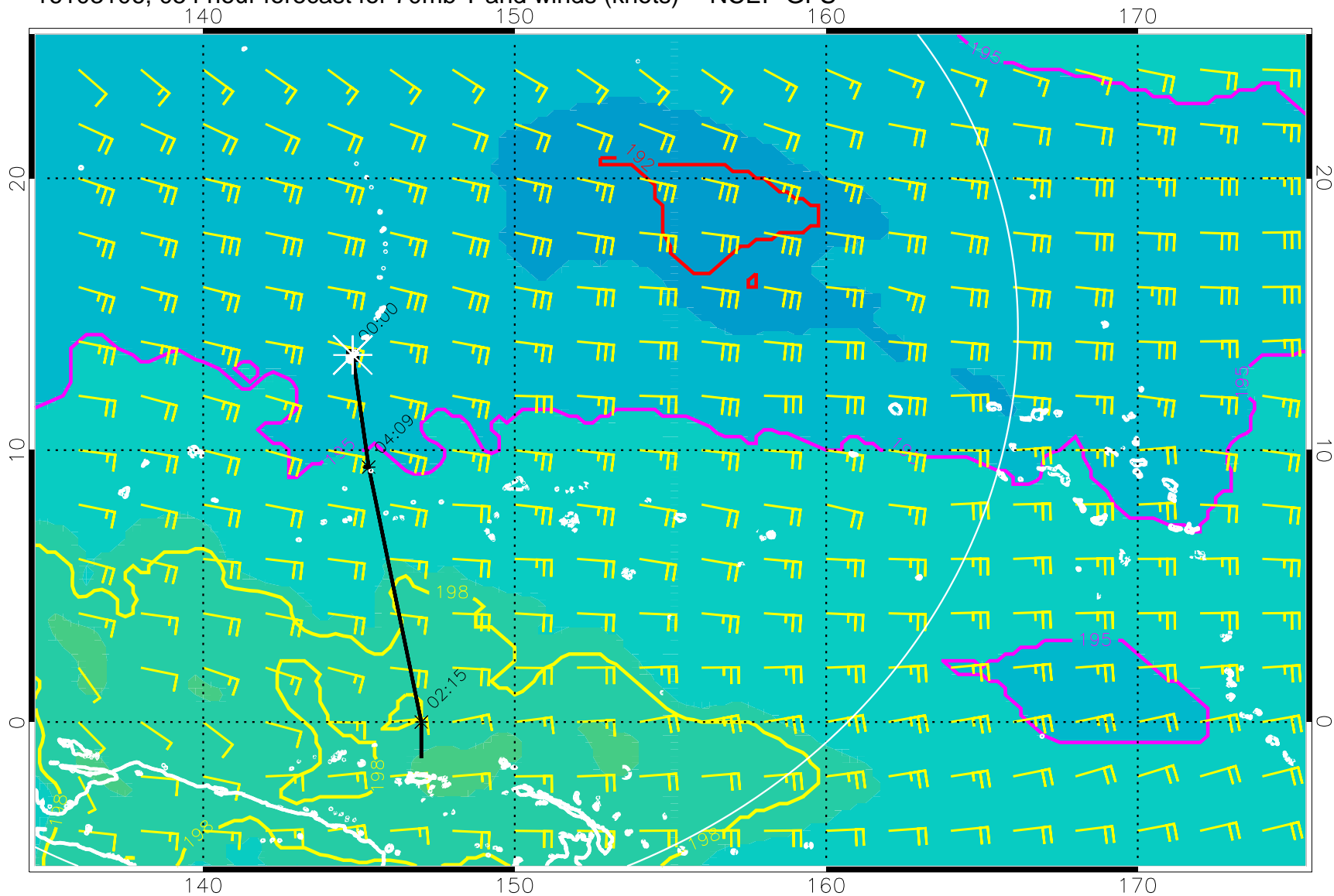
16103106, 054 hour forecast for 70mb T and winds (knots) -- NCEP GFS
