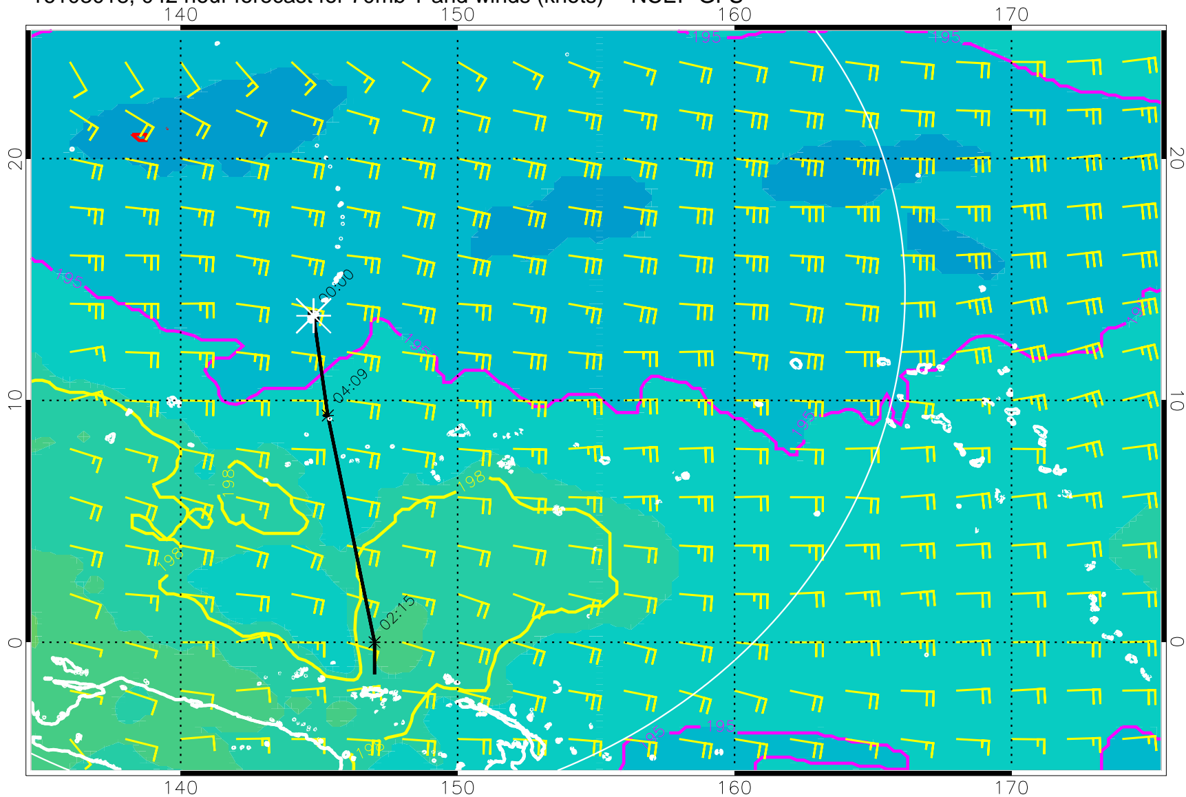
16103018, 042 hour forecast for 70mb T and winds (knots) -- NCEP GFS
