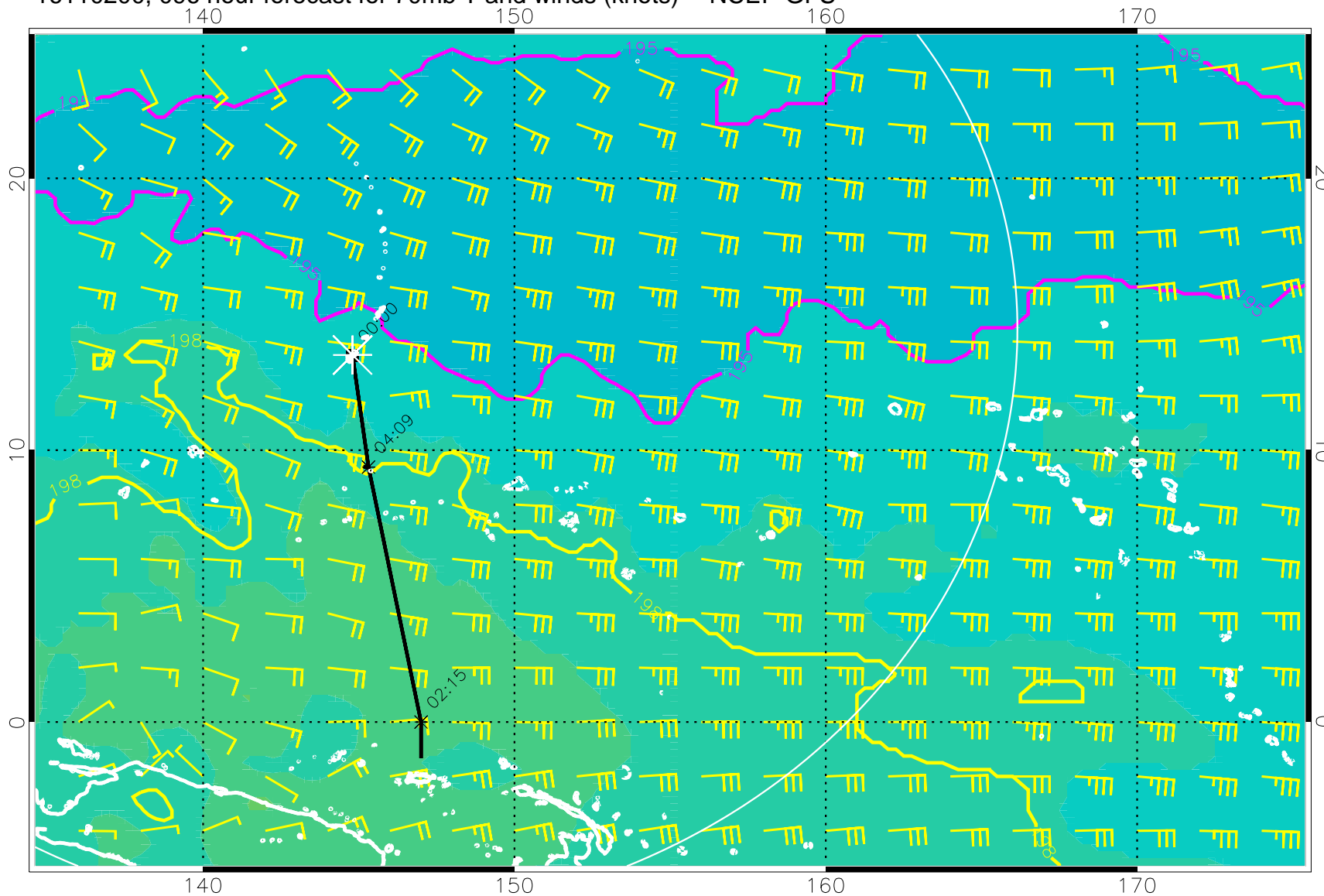
16110200, 096 hour forecast for 70mb T and winds (knots) -- NCEP GFS
