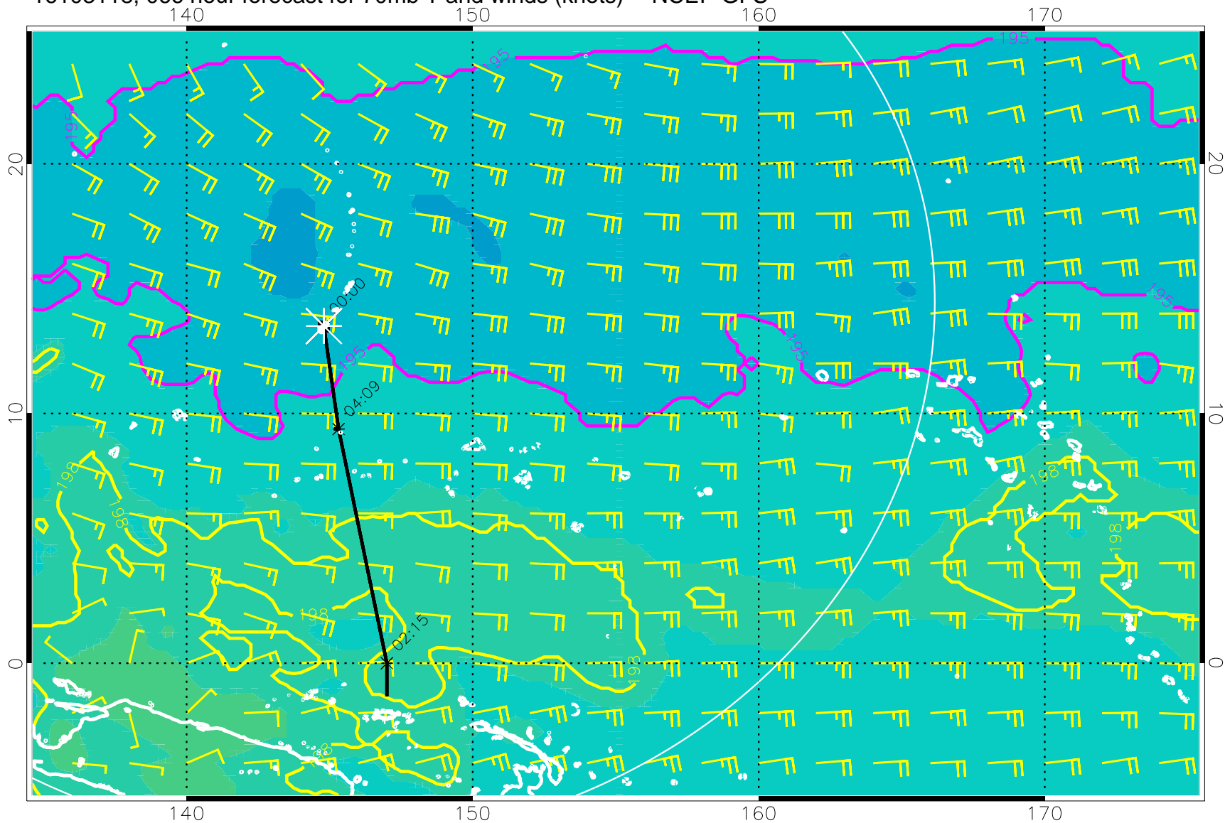
16103118, 066 hour forecast for 70mb T and winds (knots) -- NCEP GFS
