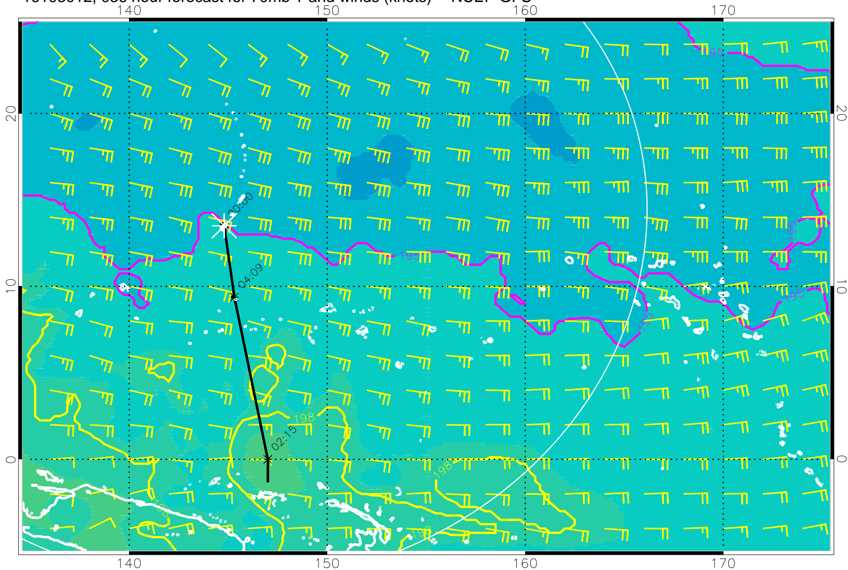
16103012, 036 hour forecast for 70mb T and winds (knots) -- NCEP GFS
