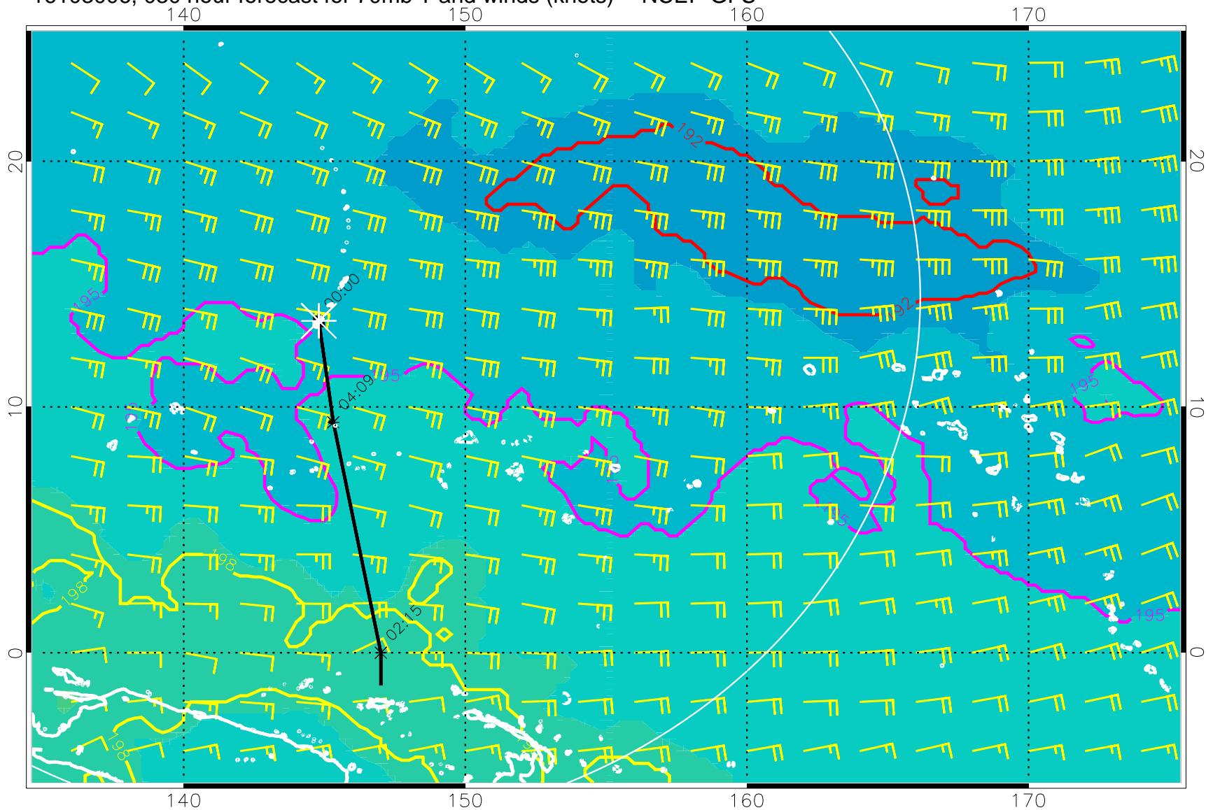
16103006, 030 hour forecast for 70mb T and winds (knots) -- NCEP GFS
