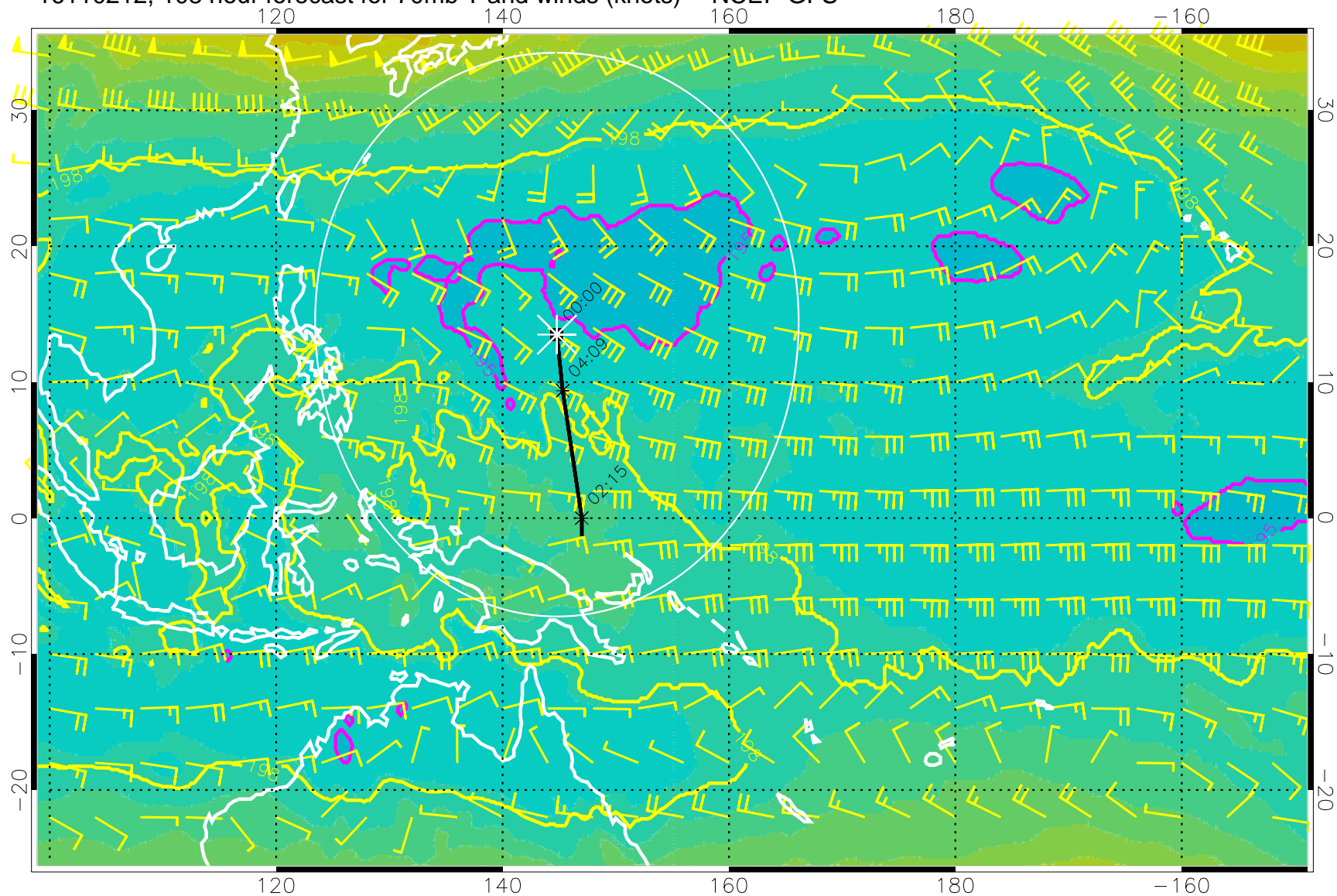
16110212, 108 hour forecast for 70mb T and winds (knots) -- NCEP GFS
