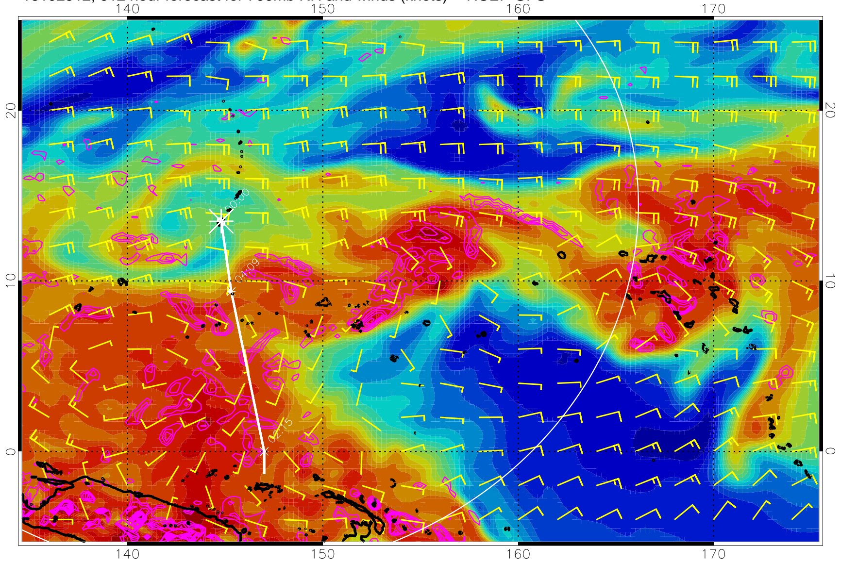
16102912, 012 hour forecast for 700mb RH and winds (knots) -- NCEP GFS
