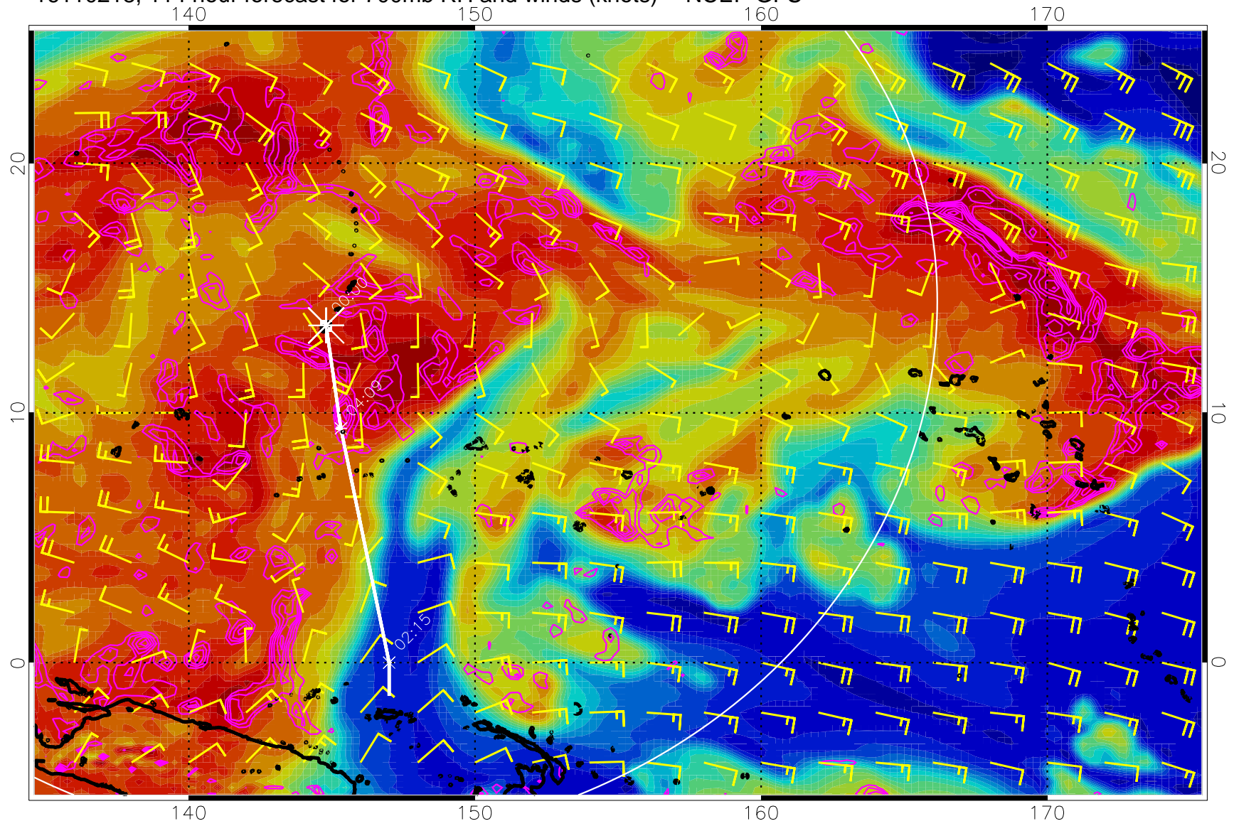
16110218, 114 hour forecast for 700mb RH and winds (knots) -- NCEP GFS
