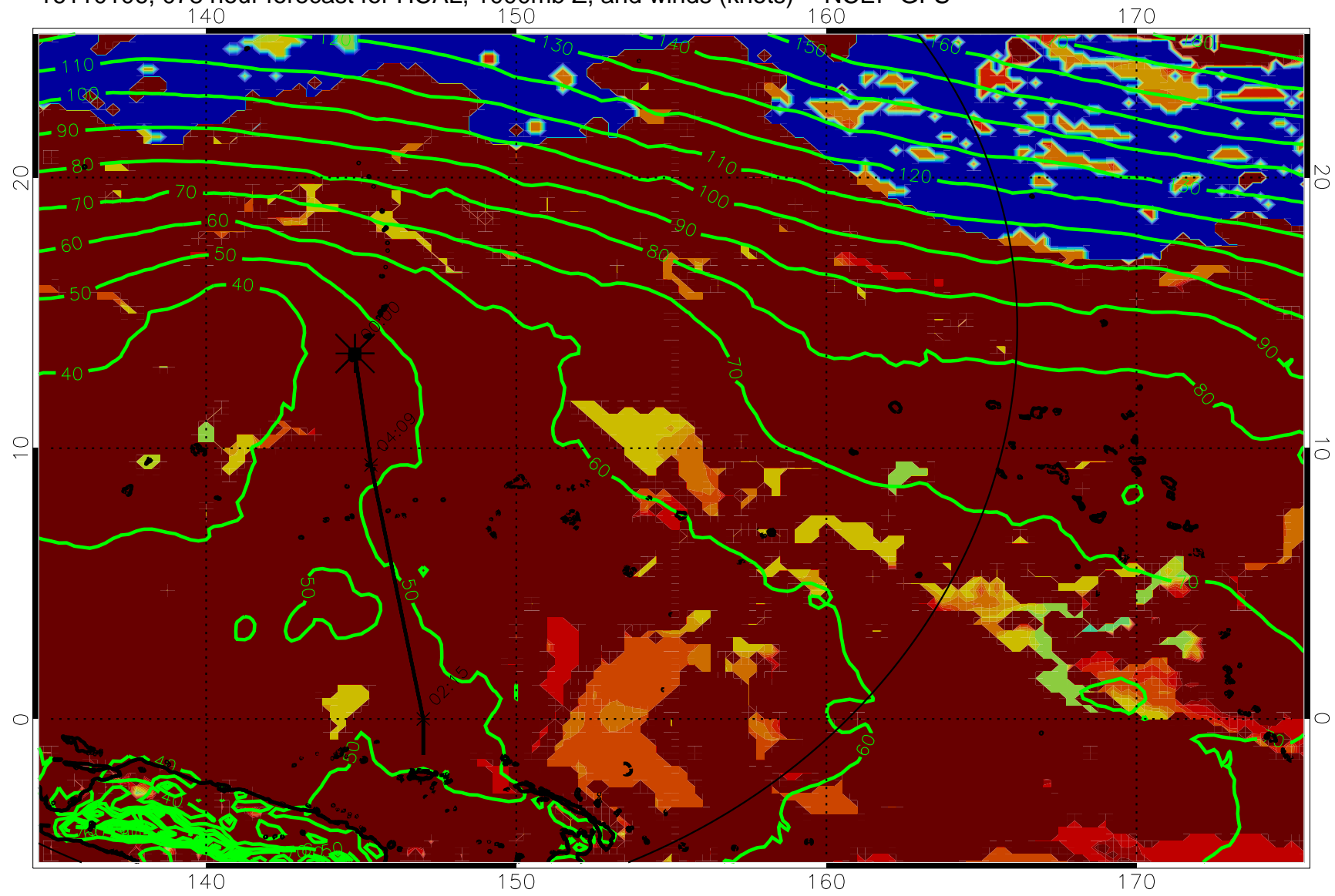
16110106, 078 hour forecast for HCAL, 1000mb Z, and winds (knots) -- NCEP GFS
