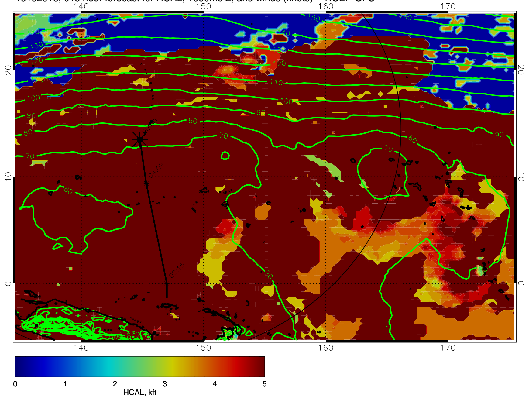
16102918, 018 hour forecast for HCAL, 1000mb Z, and winds (knots) -- NCEP GFS
