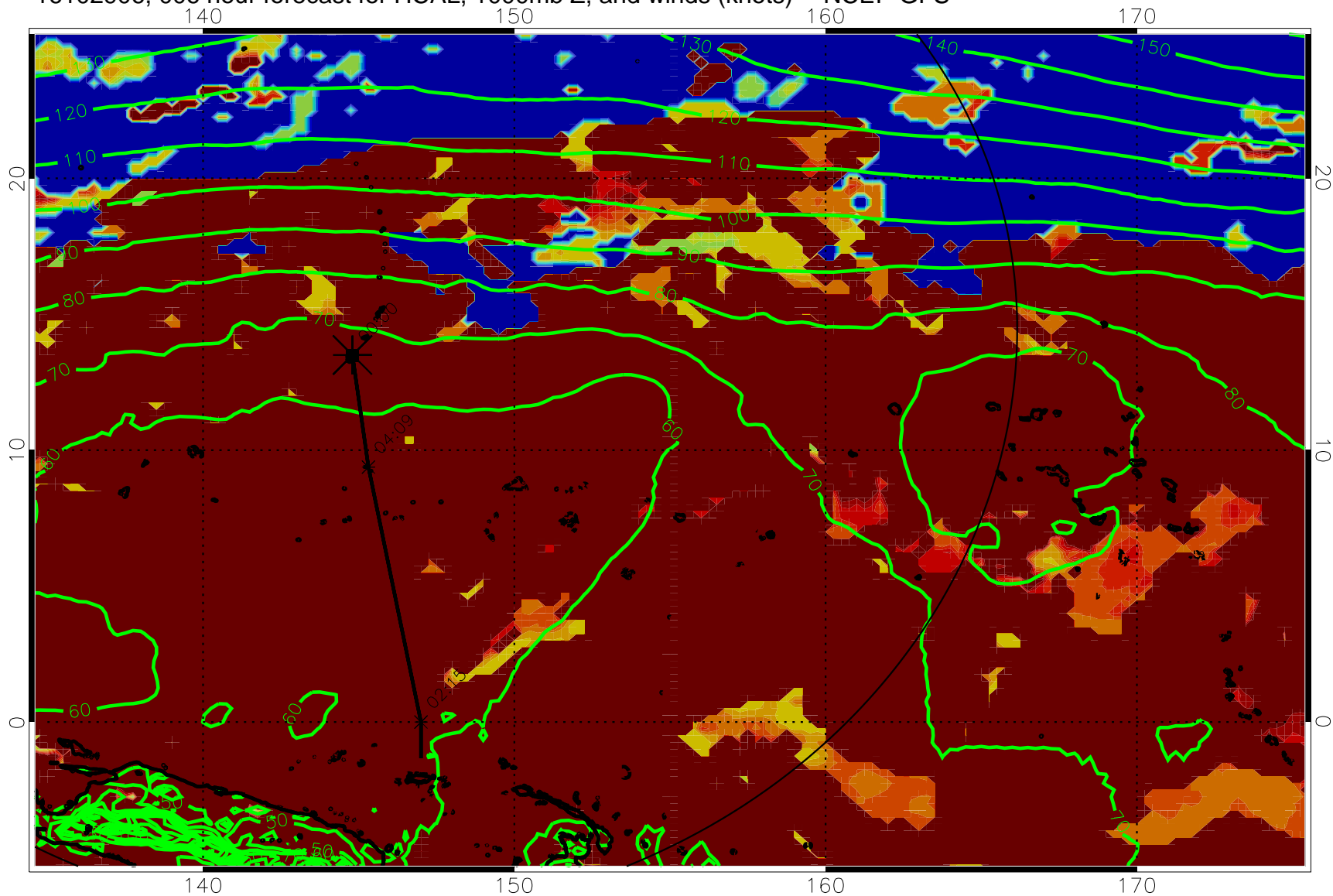
16102906, 006 hour forecast for HCAL, 1000mb Z, and winds (knots) -- NCEP GFS
