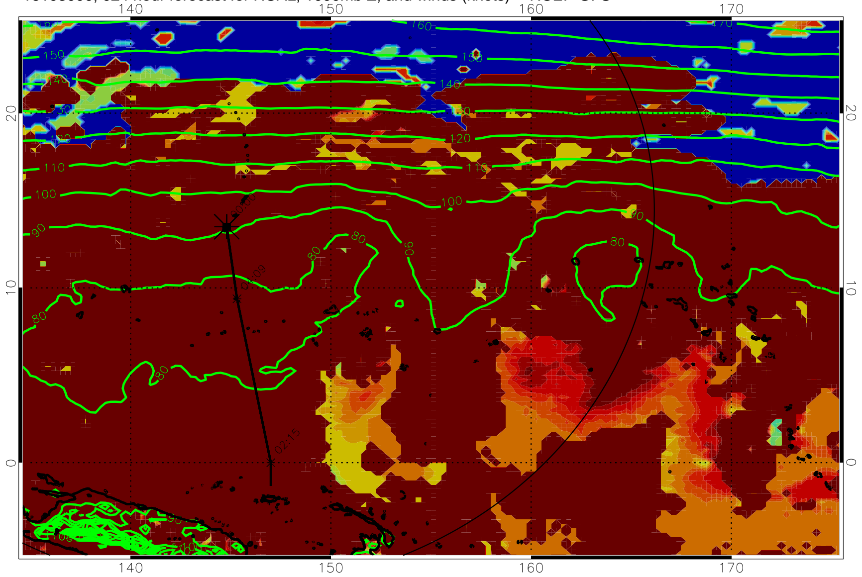
16103000, 024 hour forecast for HCAL, 1000mb Z, and winds (knots) -- NCEP GFS
