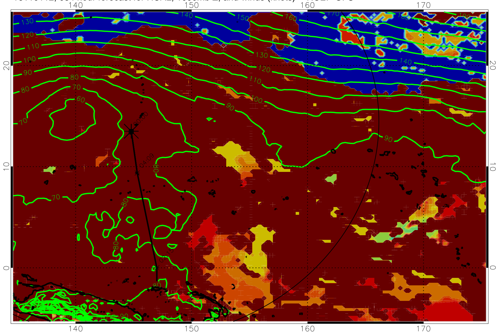
16110112, 084 hour forecast for HCAL, 1000mb Z, and winds (knots) -- NCEP GFS
