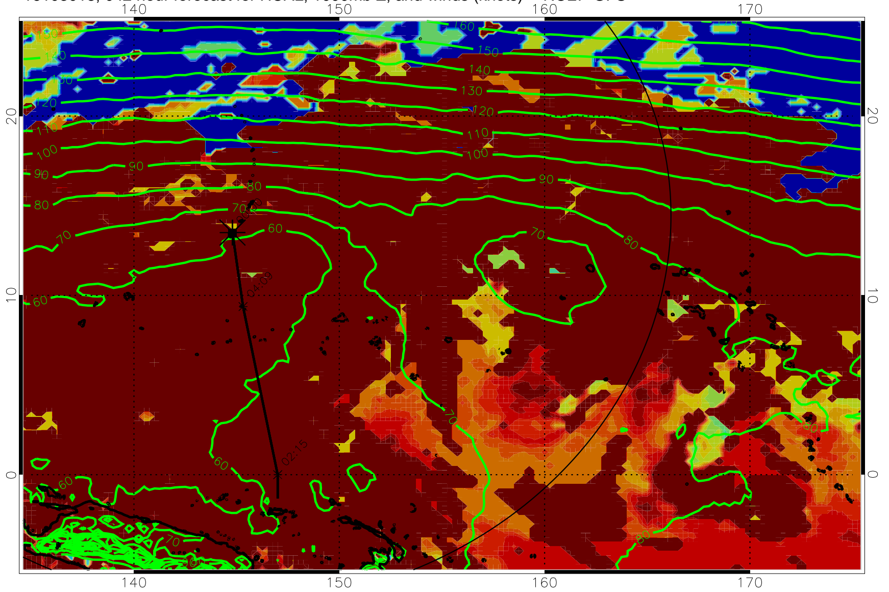
16103018, 042 hour forecast for HCAL, 1000mb Z, and winds (knots) -- NCEP GFS
