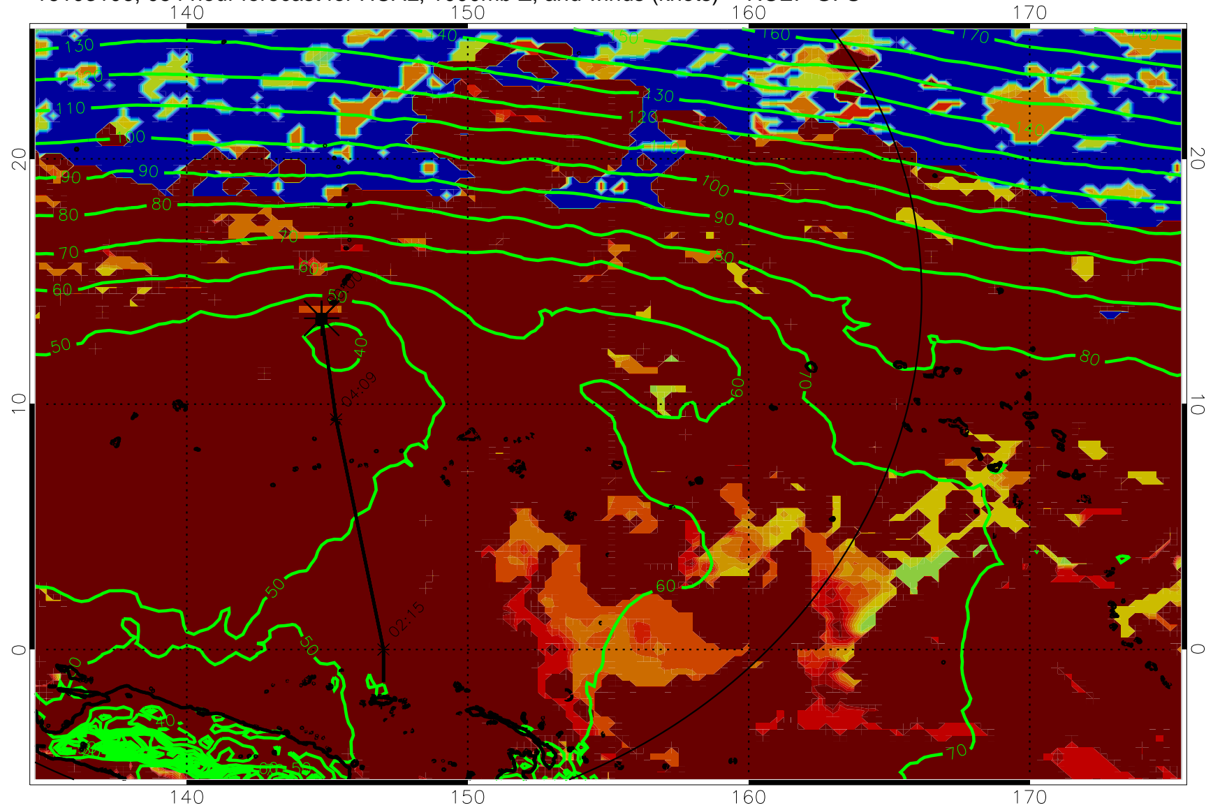
16103106, 054 hour forecast for HCAL, 1000mb Z, and winds (knots) -- NCEP GFS
