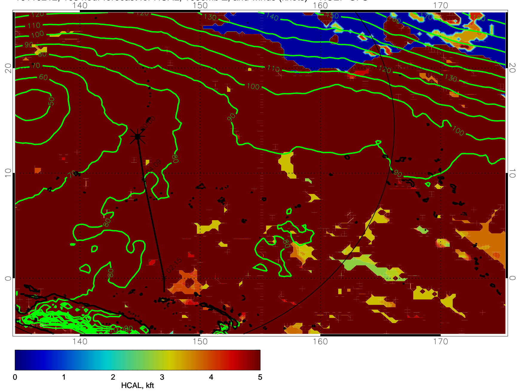
16110212, 108 hour forecast for HCAL, 1000mb Z, and winds (knots) -- NCEP GFS
