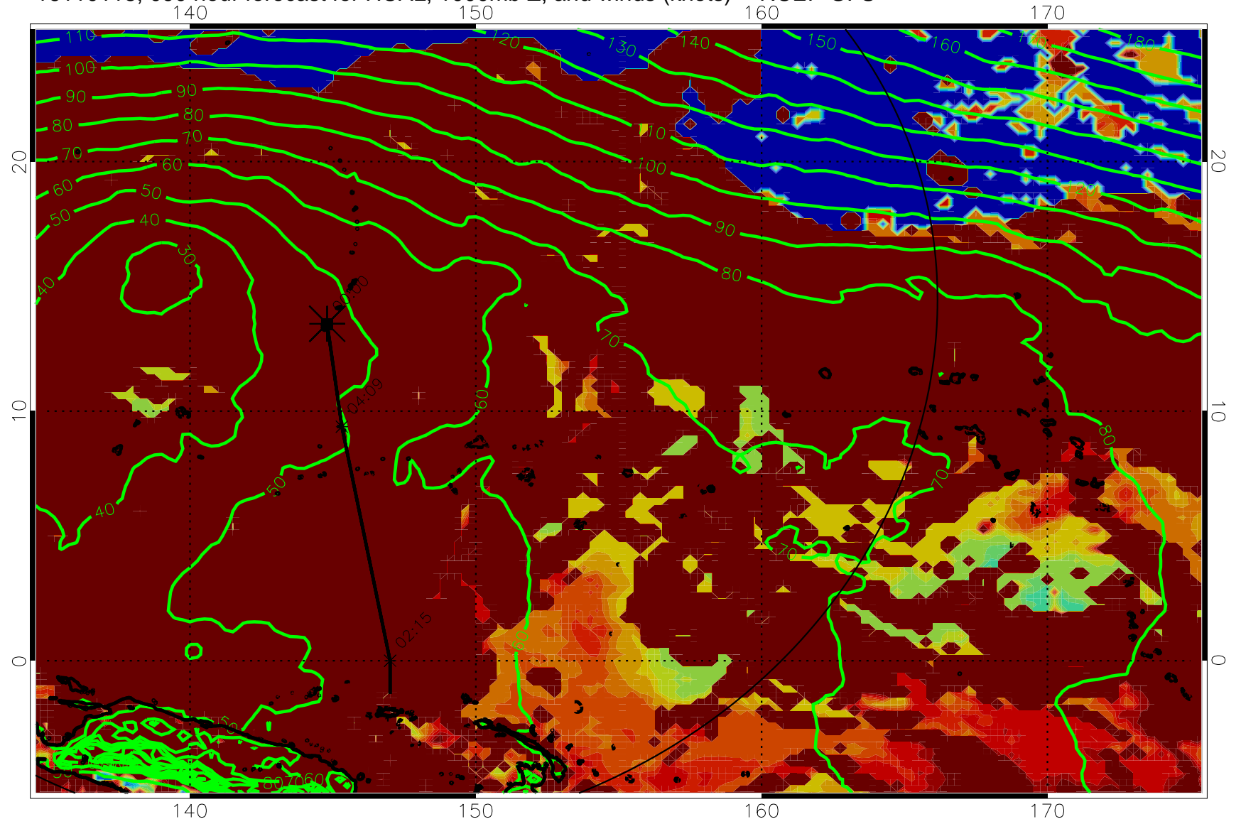
16110118, 090 hour forecast for HCAL, 1000mb Z, and winds (knots) -- NCEP GFS
