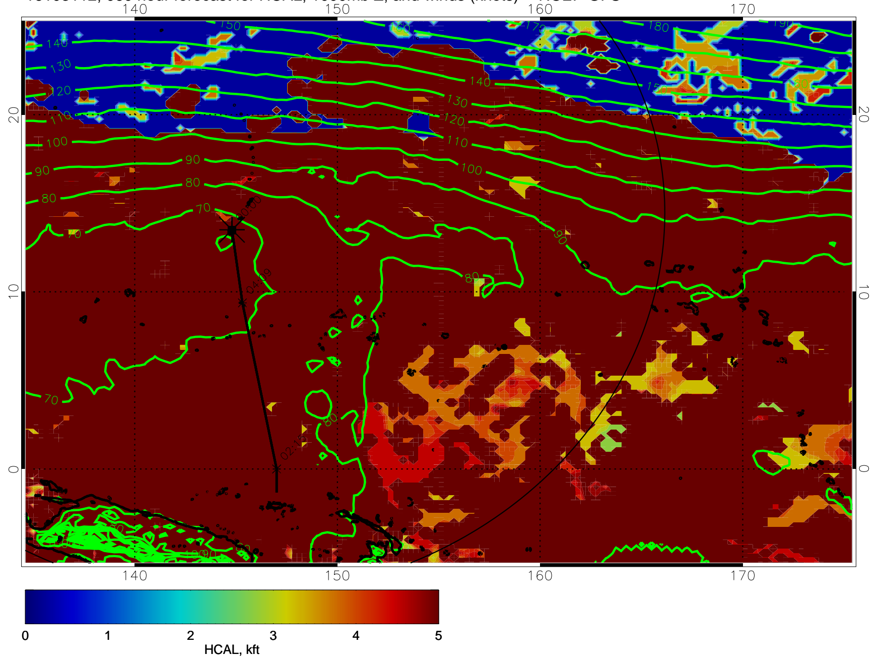
16103112, 060 hour forecast for HCAL, 1000mb Z, and winds (knots) -- NCEP GFS
