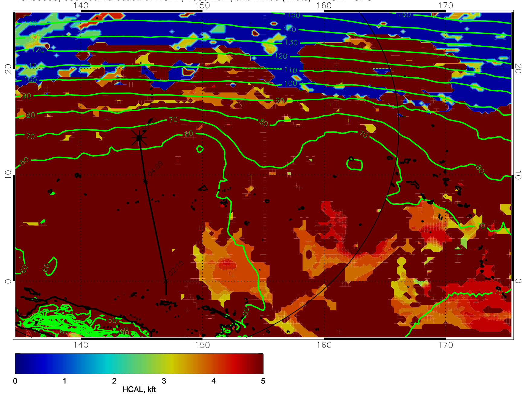
16103006, 030 hour forecast for HCAL, 1000mb Z, and winds (knots) -- NCEP GFS
