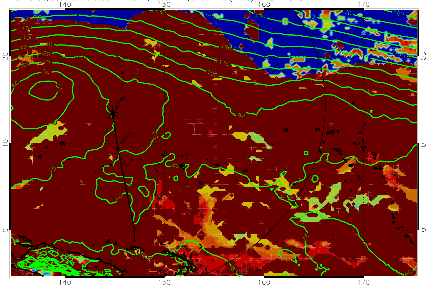
16110200, 096 hour forecast for HCAL, 1000mb Z, and winds (knots) -- NCEP GFS
