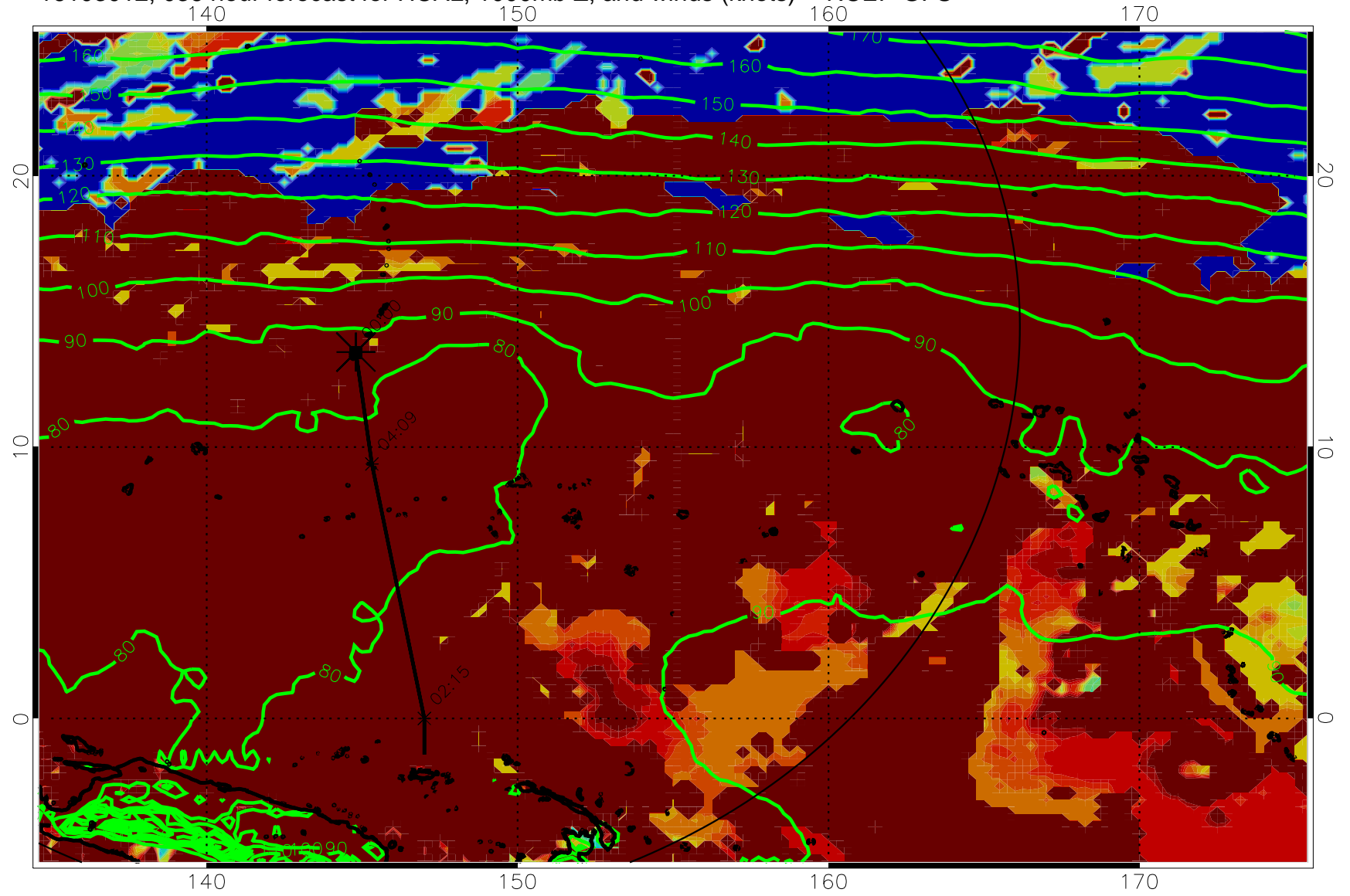
16103012, 036 hour forecast for HCAL, 1000mb Z, and winds (knots) -- NCEP GFS
