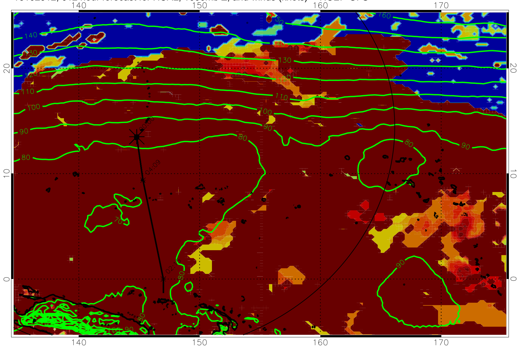
16102912, 012 hour forecast for HCAL, 1000mb Z, and winds (knots) -- NCEP GFS
