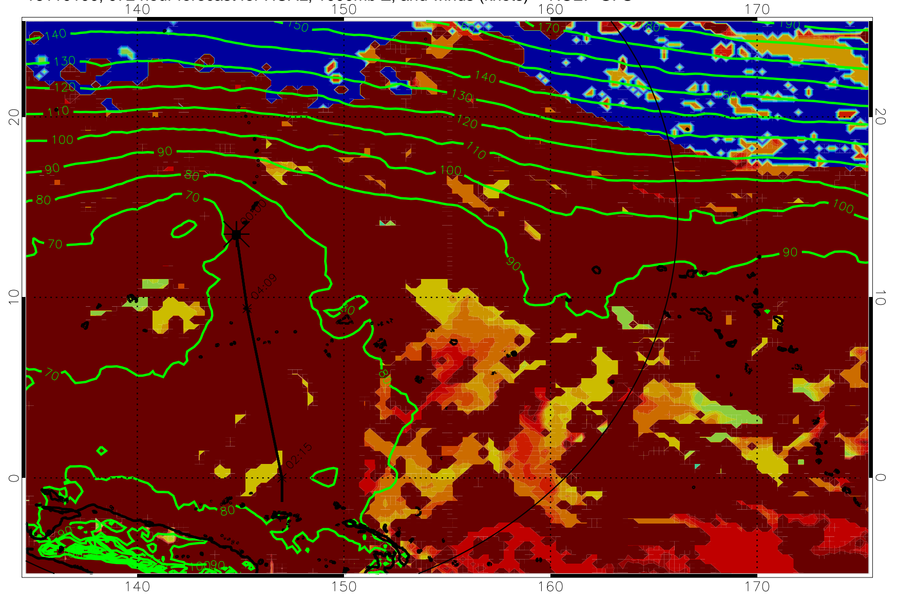
16110100, 072 hour forecast for HCAL, 1000mb Z, and winds (knots) -- NCEP GFS
