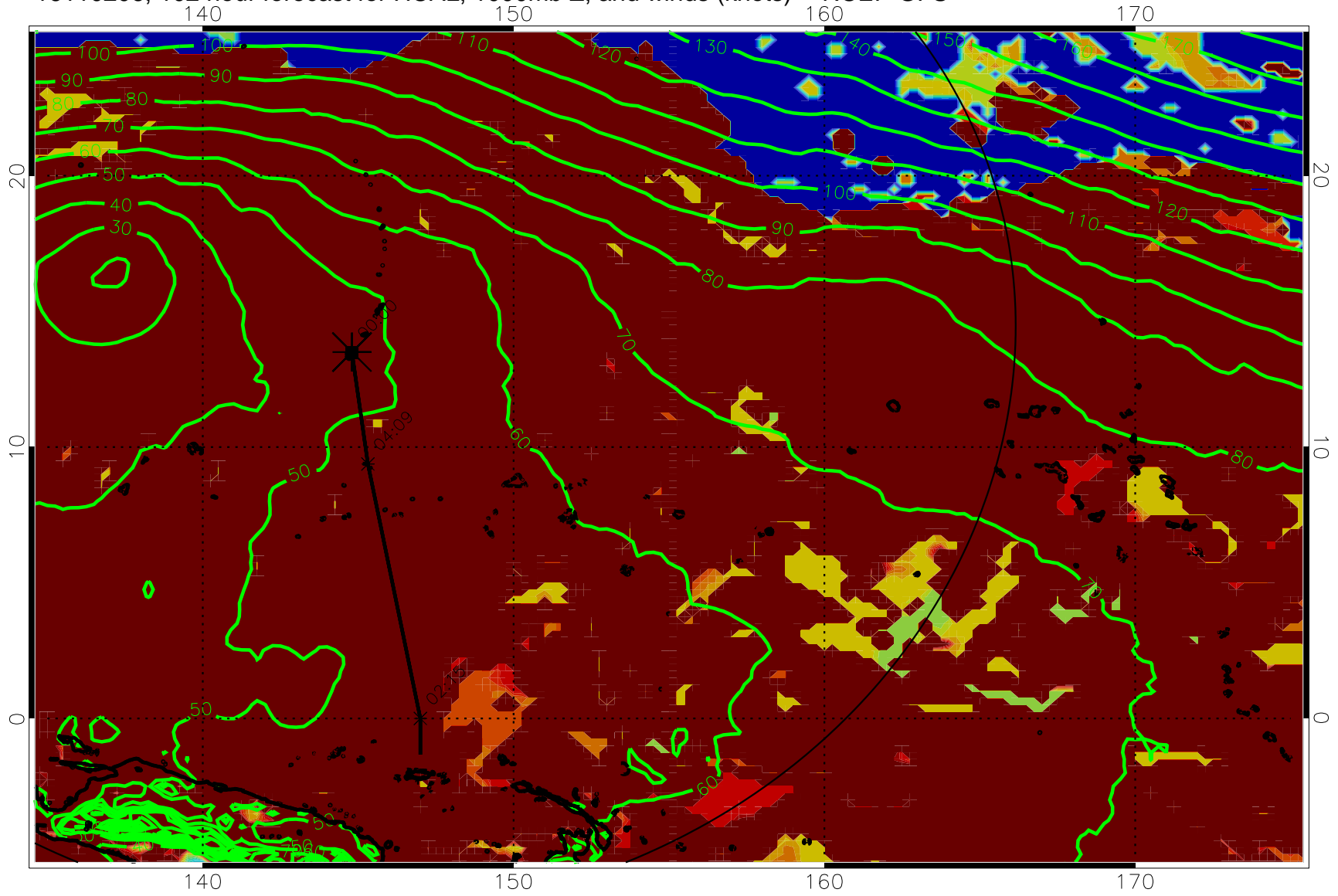
16110206, 102 hour forecast for HCAL, 1000mb Z, and winds (knots) -- NCEP GFS
