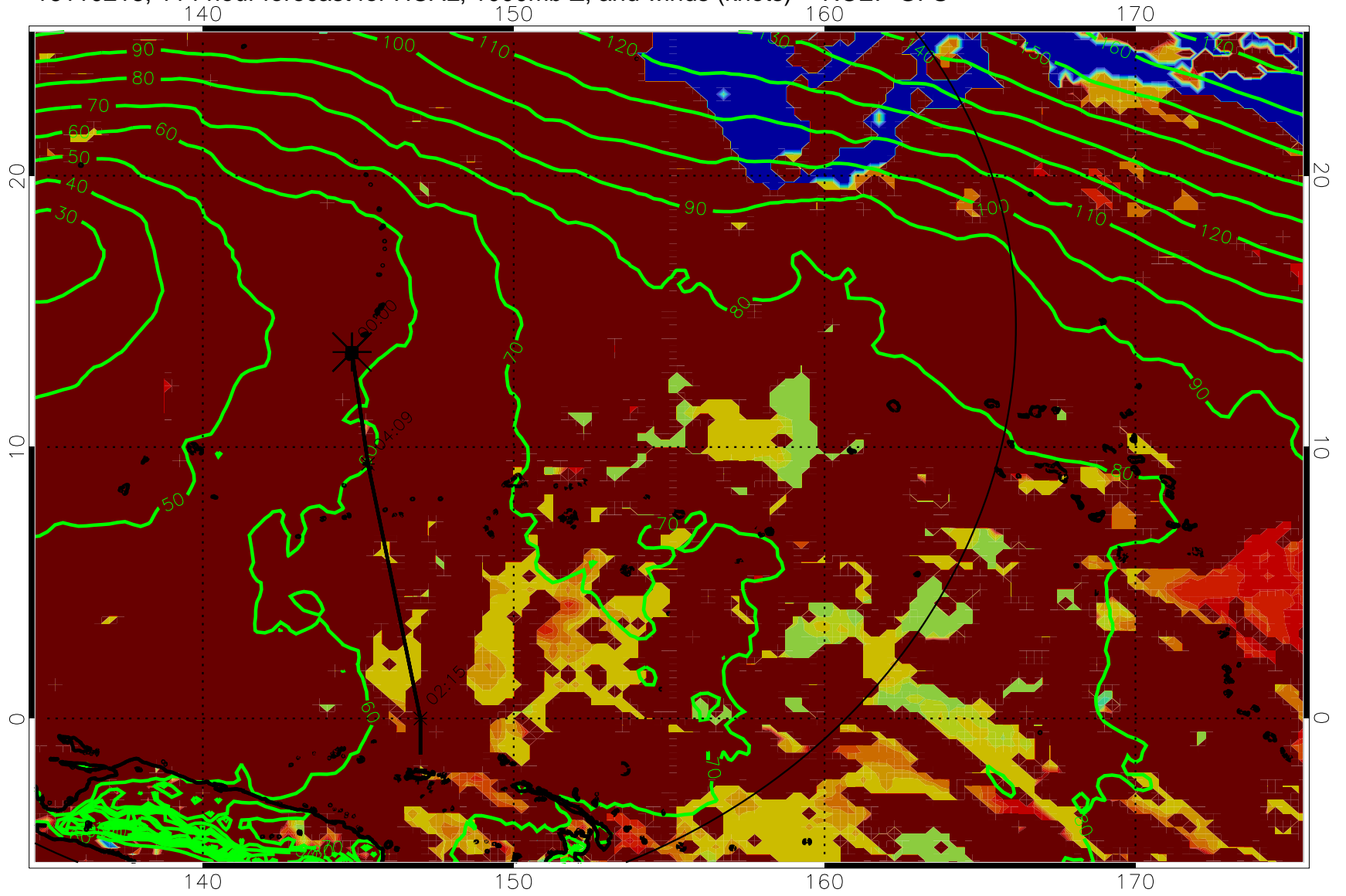
16110218, 114 hour forecast for HCAL, 1000mb Z, and winds (knots) -- NCEP GFS
