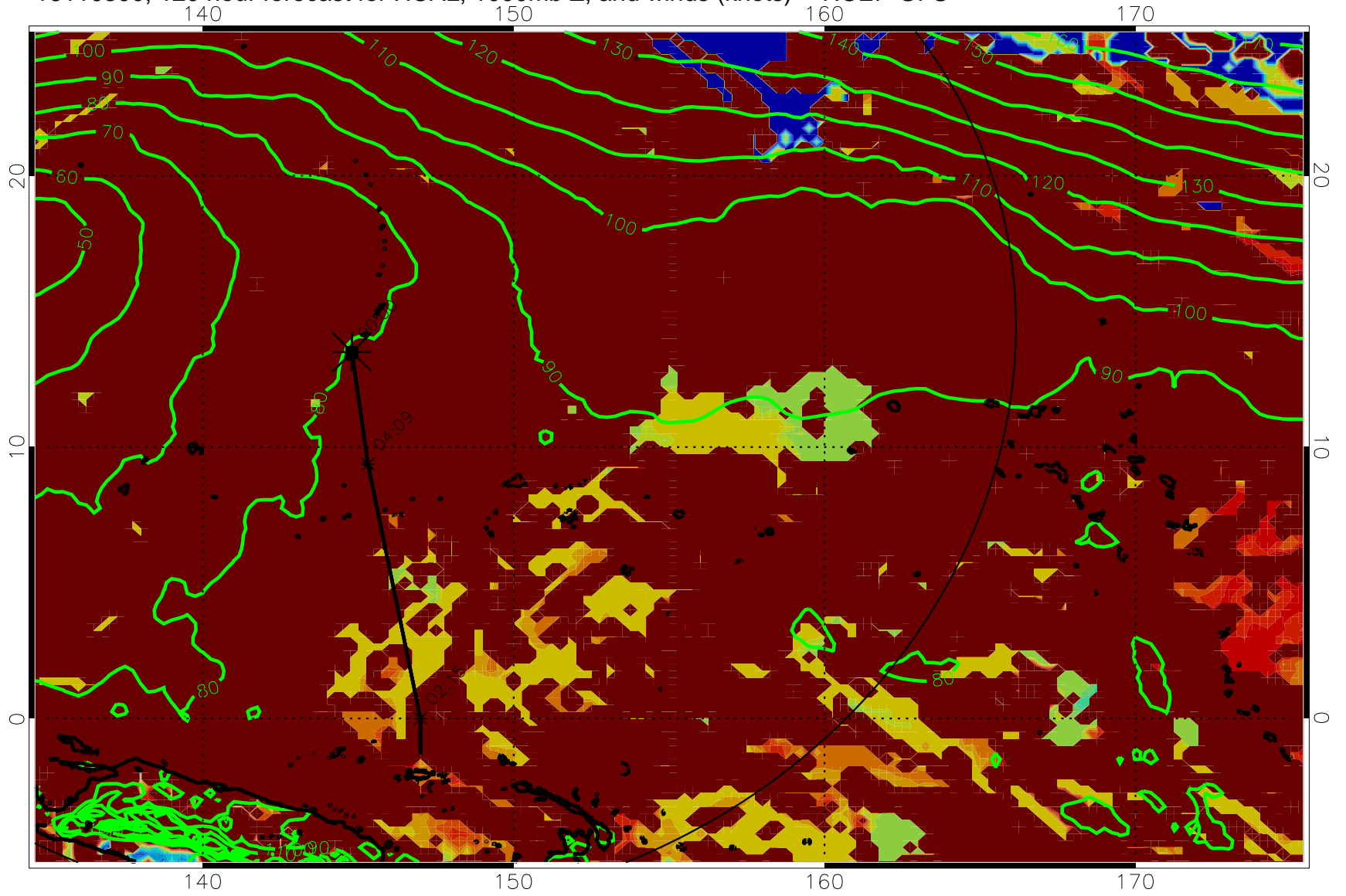
16110300, 120 hour forecast for HCAL, 1000mb Z, and winds (knots) -- NCEP GFS
