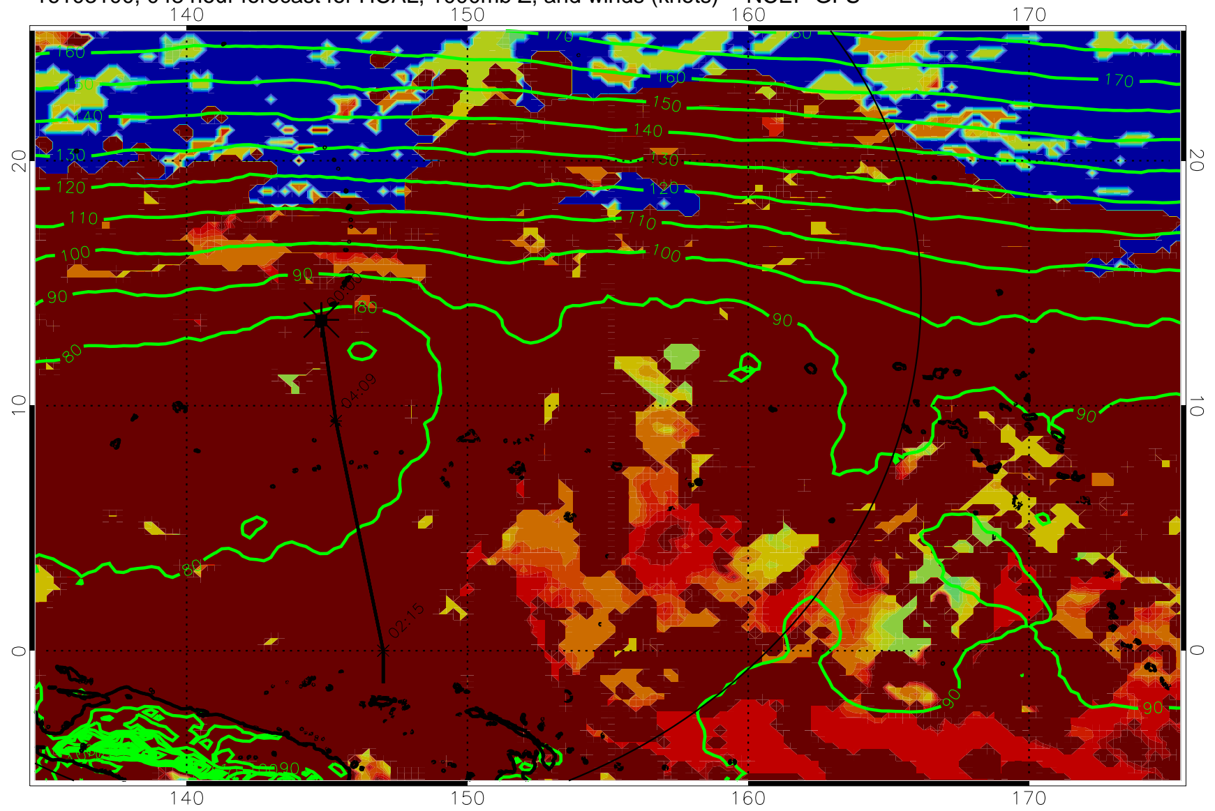
16103100, 048 hour forecast for HCAL, 1000mb Z, and winds (knots) -- NCEP GFS
