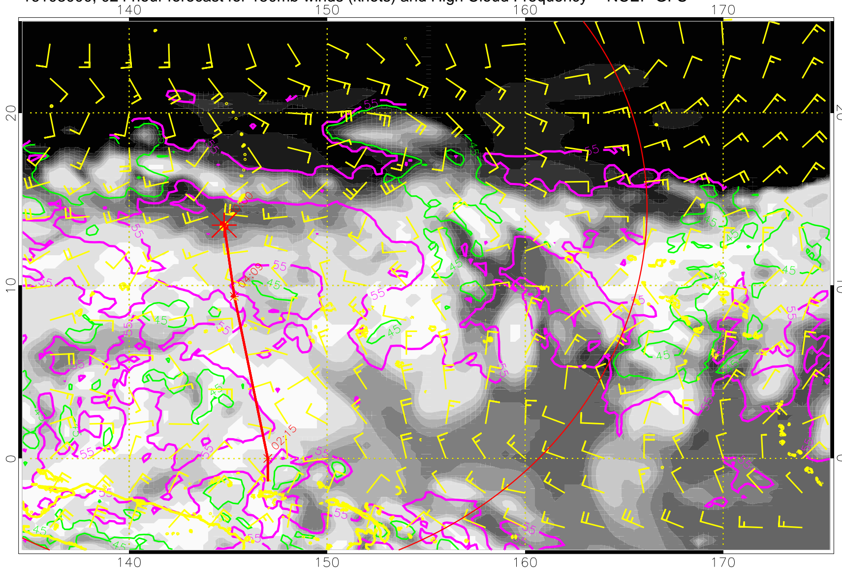
16103000, 024 hour forecast for 150mb winds (knots) and High Cloud Frequency -- NCEP GFS
