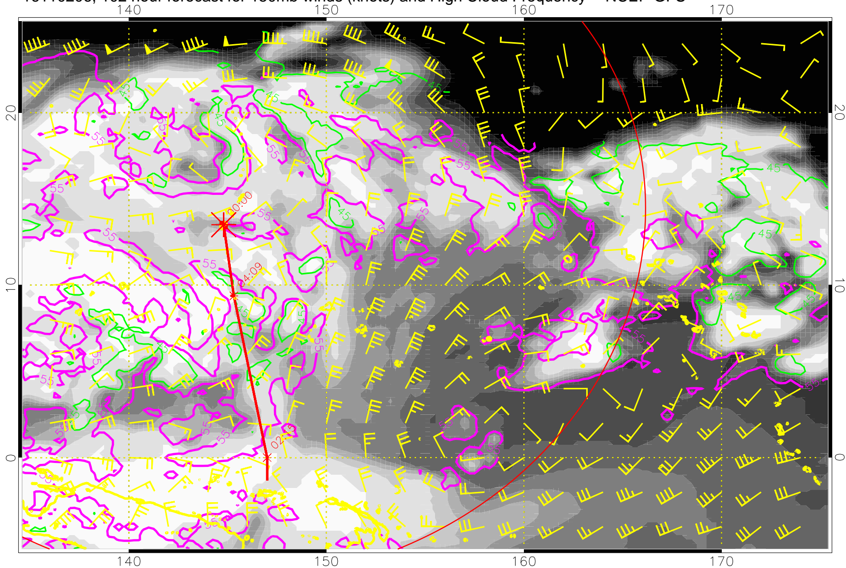
16110206, 102 hour forecast for 150mb winds (knots) and High Cloud Frequency -- NCEP GFS
