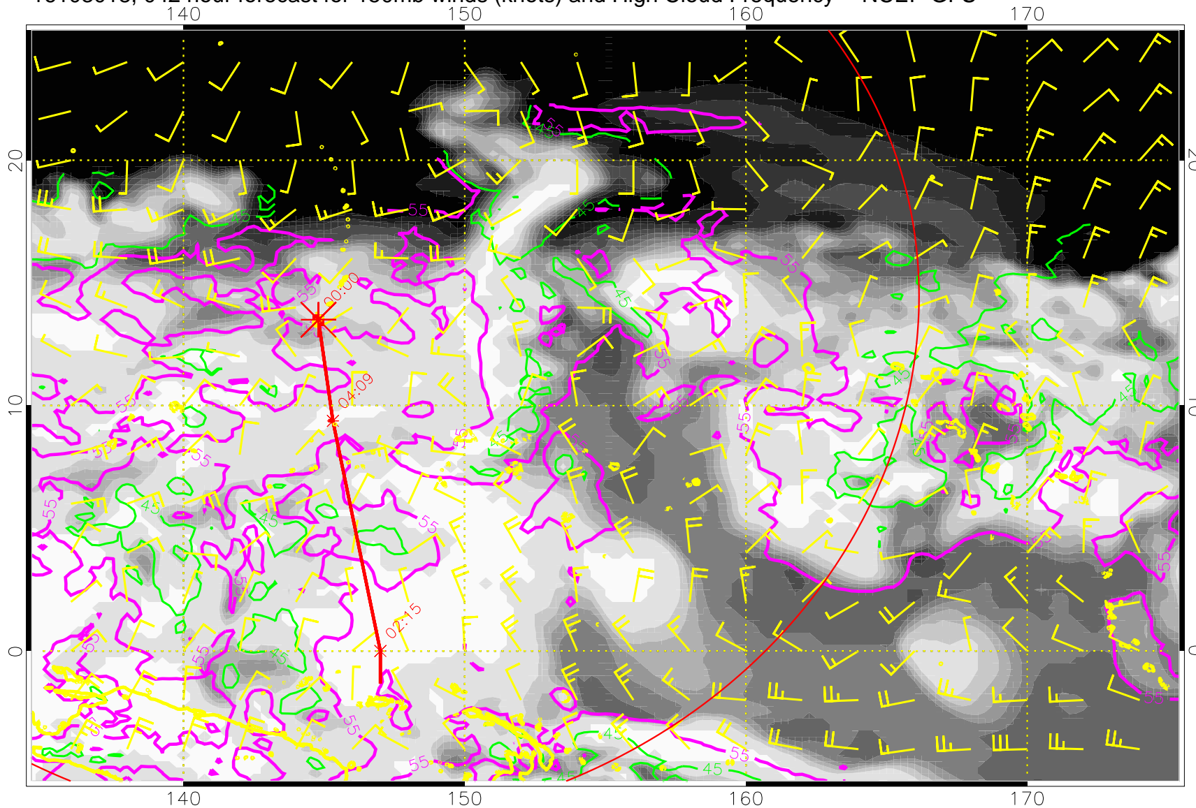
16103018, 042 hour forecast for 150mb winds (knots) and High Cloud Frequency -- NCEP GFS
