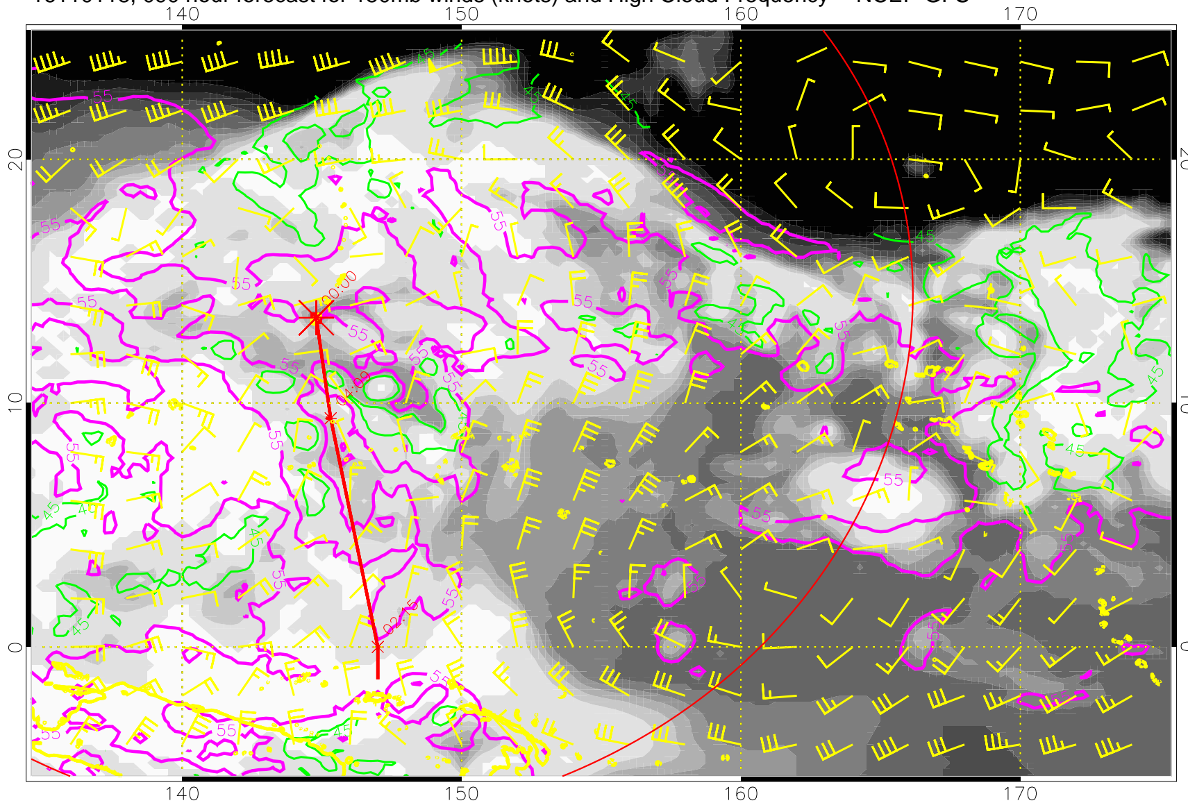
16110118, 090 hour forecast for 150mb winds (knots) and High Cloud Frequency -- NCEP GFS
