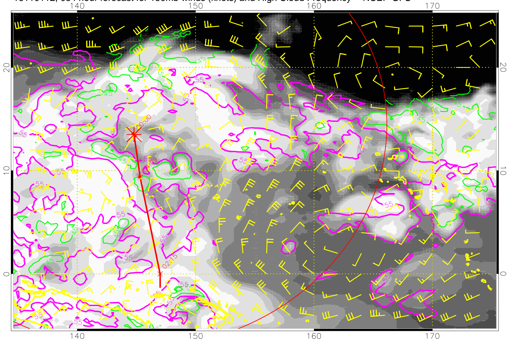
16110112, 084 hour forecast for 150mb winds (knots) and High Cloud Frequency -- NCEP GFS
