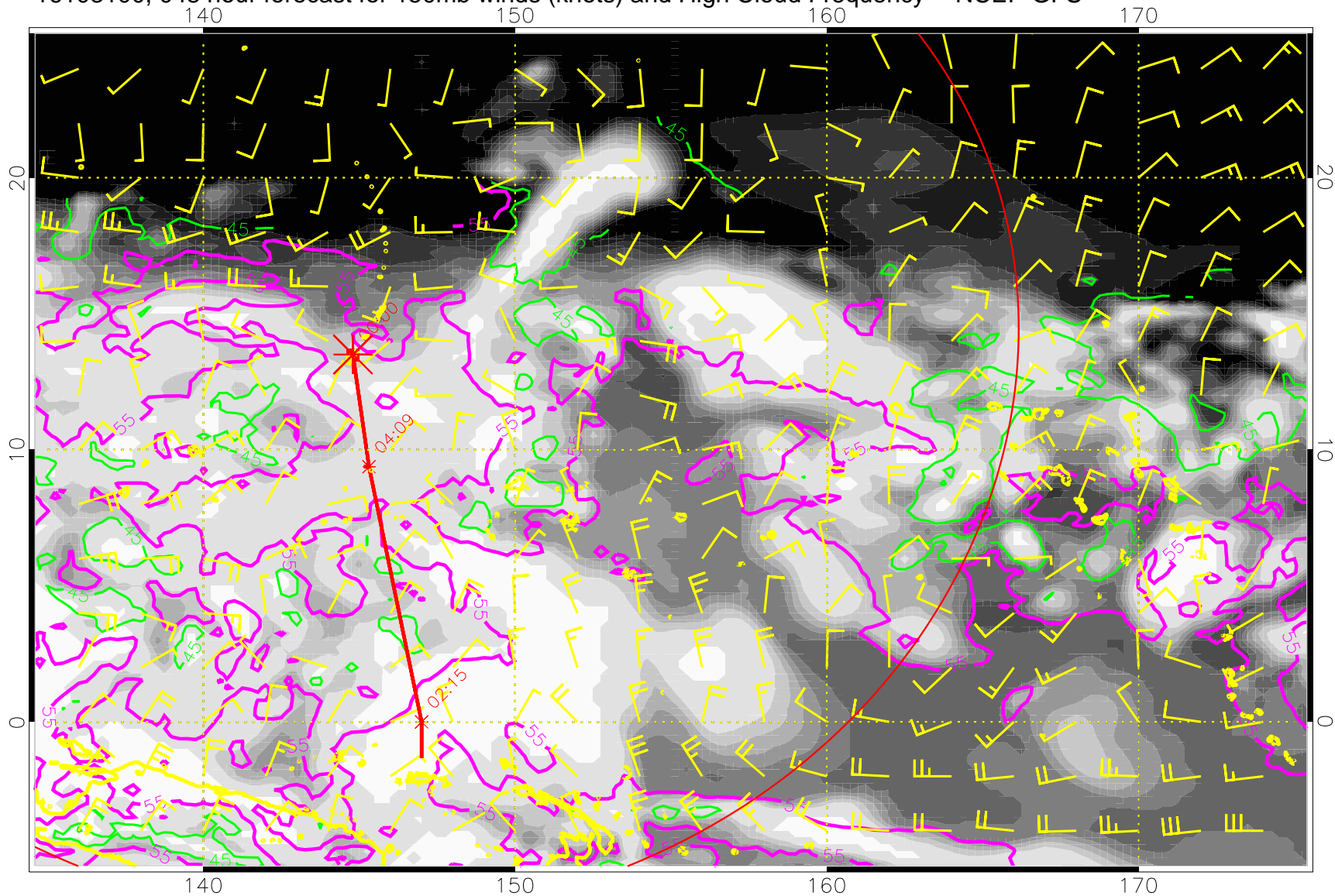
16103100, 048 hour forecast for 150mb winds (knots) and High Cloud Frequency -- NCEP GFS
