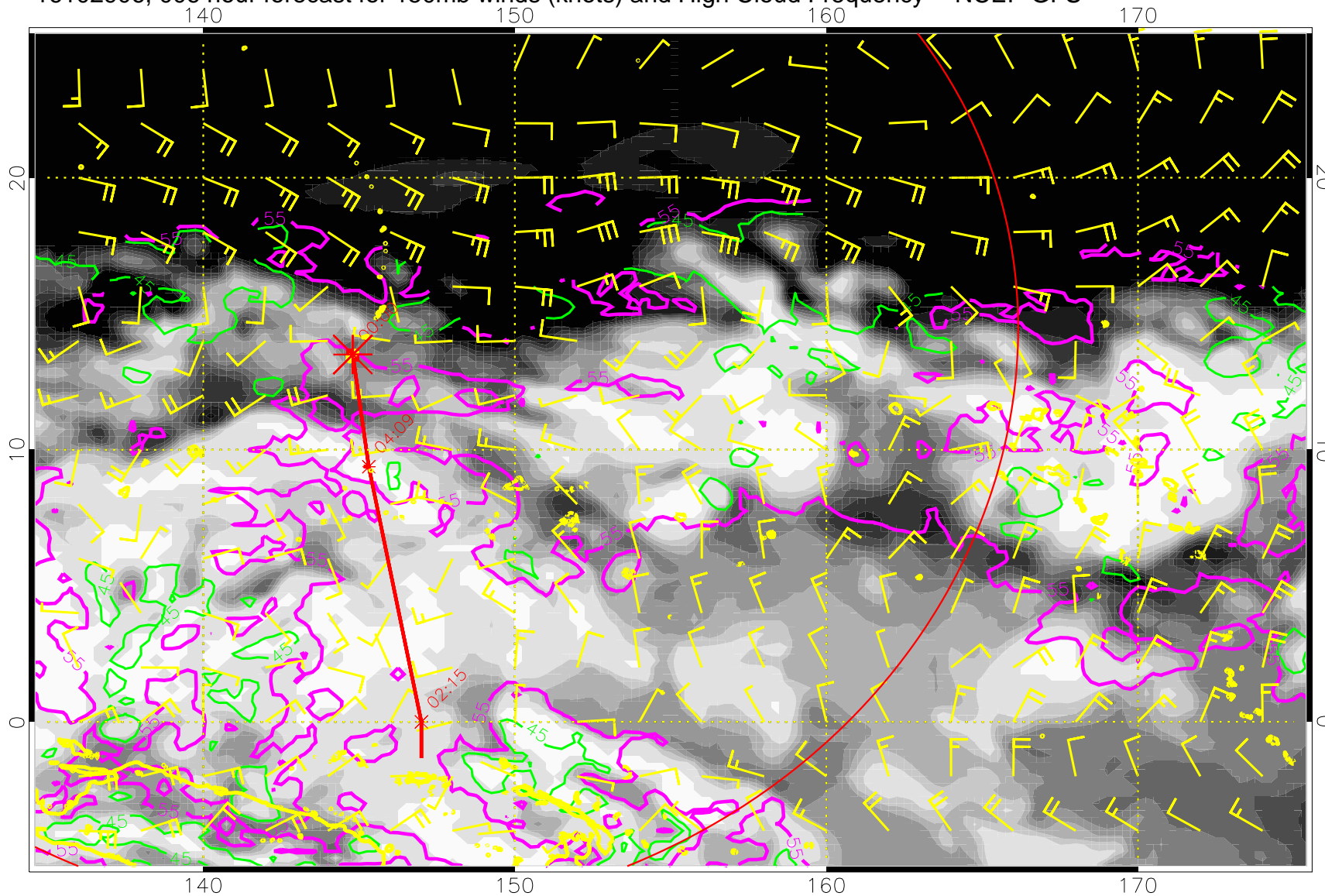
16102906, 006 hour forecast for 150mb winds (knots) and High Cloud Frequency -- NCEP GFS
