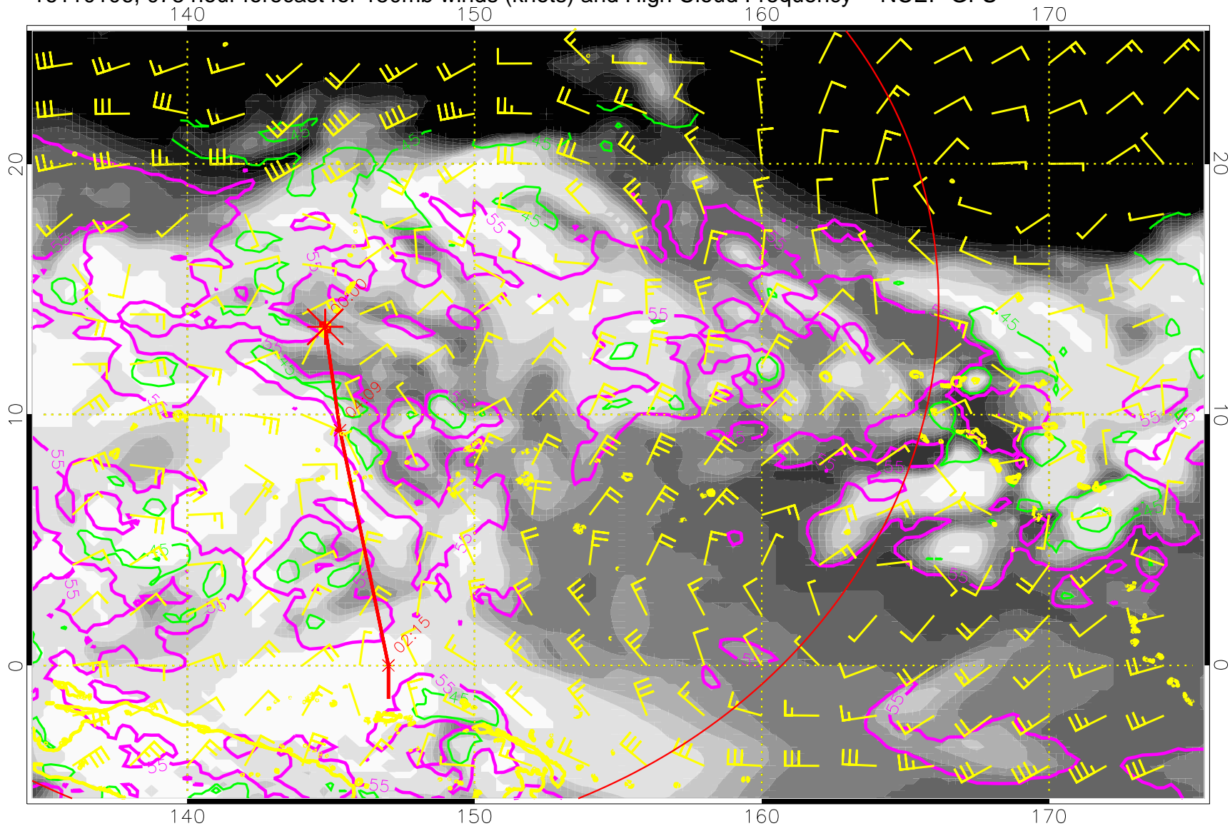
16110106, 078 hour forecast for 150mb winds (knots) and High Cloud Frequency -- NCEP GFS
