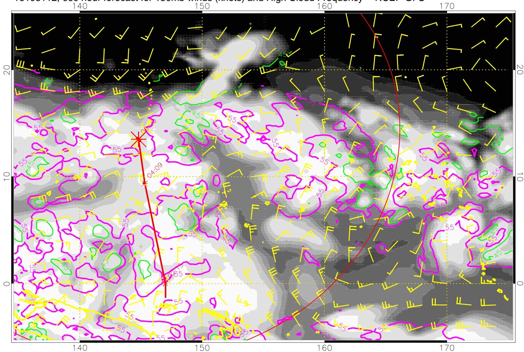
16103112, 060 hour forecast for 150mb winds (knots) and High Cloud Frequency -- NCEP GFS
