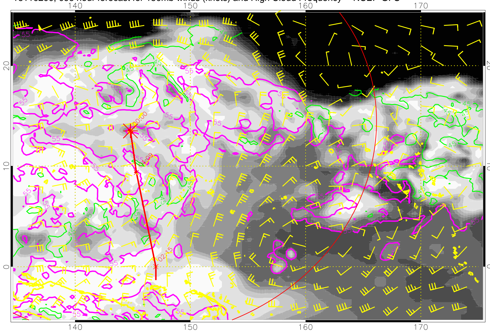
16110200, 096 hour forecast for 150mb winds (knots) and High Cloud Frequency -- NCEP GFS
