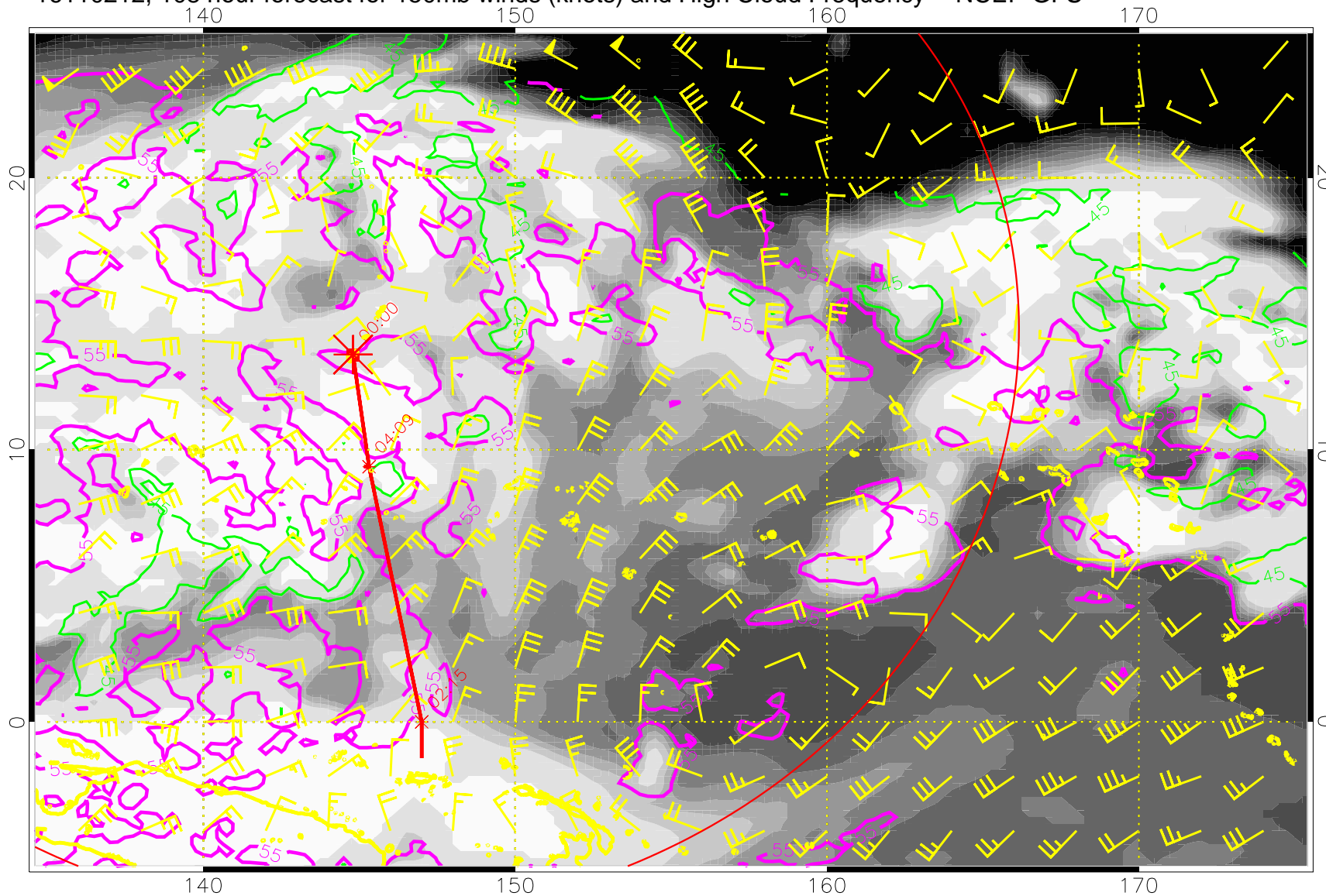
16110212, 108 hour forecast for 150mb winds (knots) and High Cloud Frequency -- NCEP GFS
