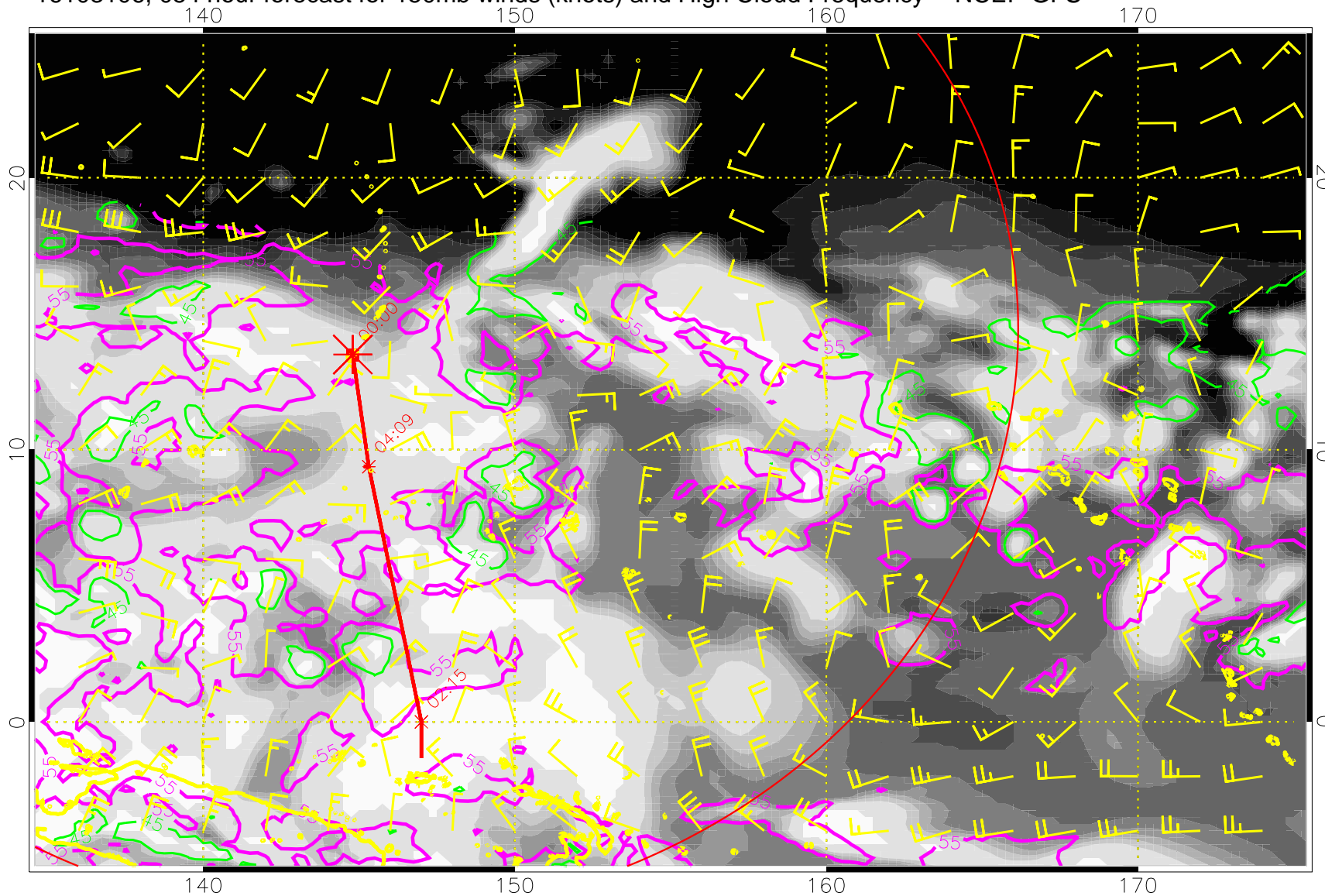
16103106, 054 hour forecast for 150mb winds (knots) and High Cloud Frequency -- NCEP GFS
