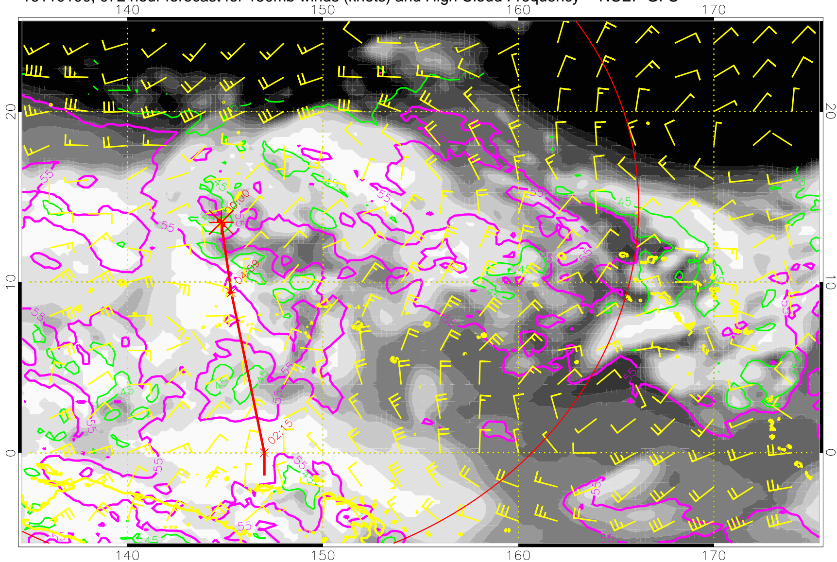
16110100, 072 hour forecast for 150mb winds (knots) and High Cloud Frequency -- NCEP GFS
