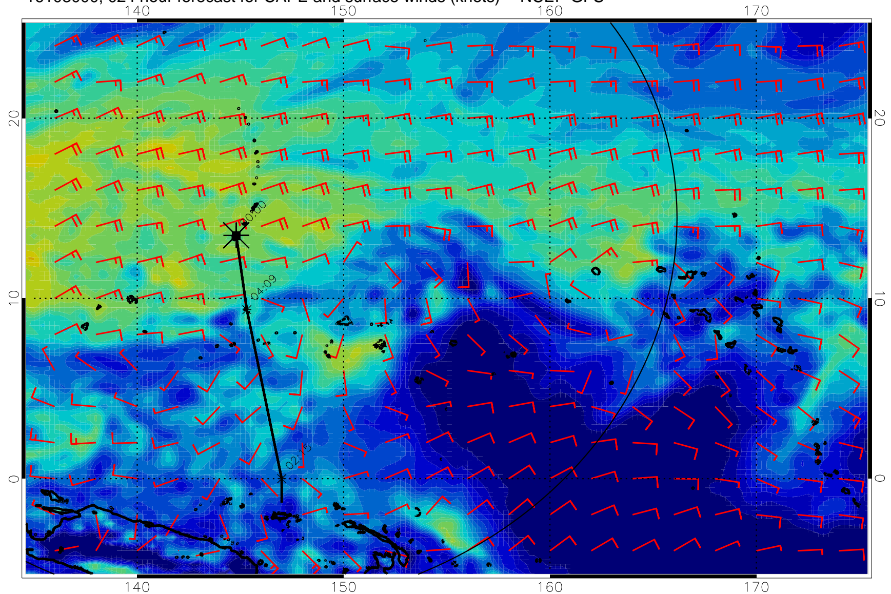
16103000, 024 hour forecast for CAPE and surface winds (knots) -- NCEP GFS
