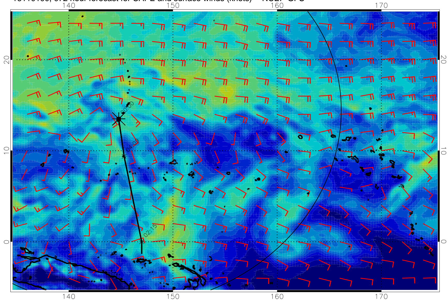
16110100, 072 hour forecast for CAPE and surface winds (knots) -- NCEP GFS
