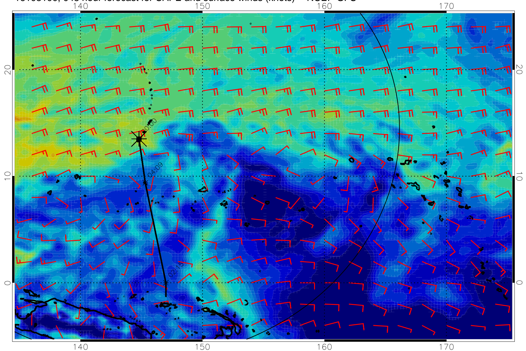
16103100, 048 hour forecast for CAPE and surface winds (knots) -- NCEP GFS
