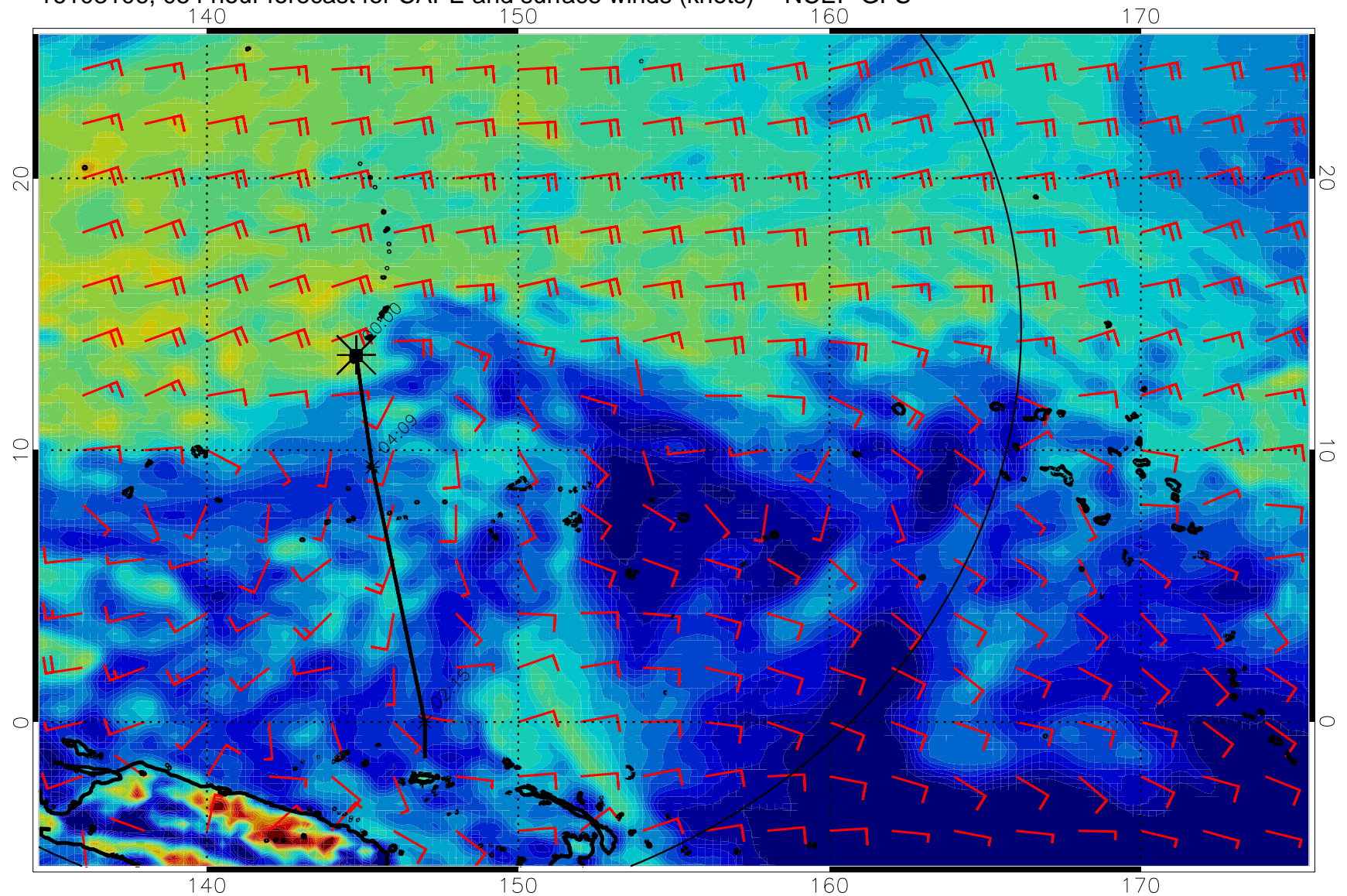
16103106, 054 hour forecast for CAPE and surface winds (knots) -- NCEP GFS
