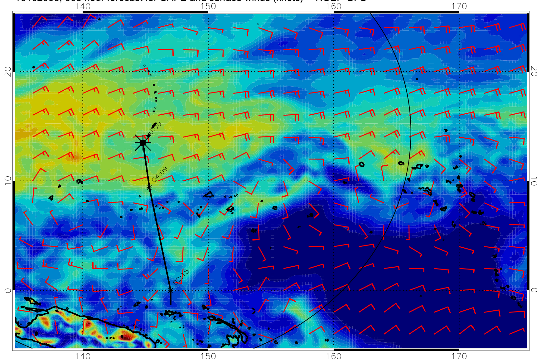
16102906, 006 hour forecast for CAPE and surface winds (knots) -- NCEP GFS
