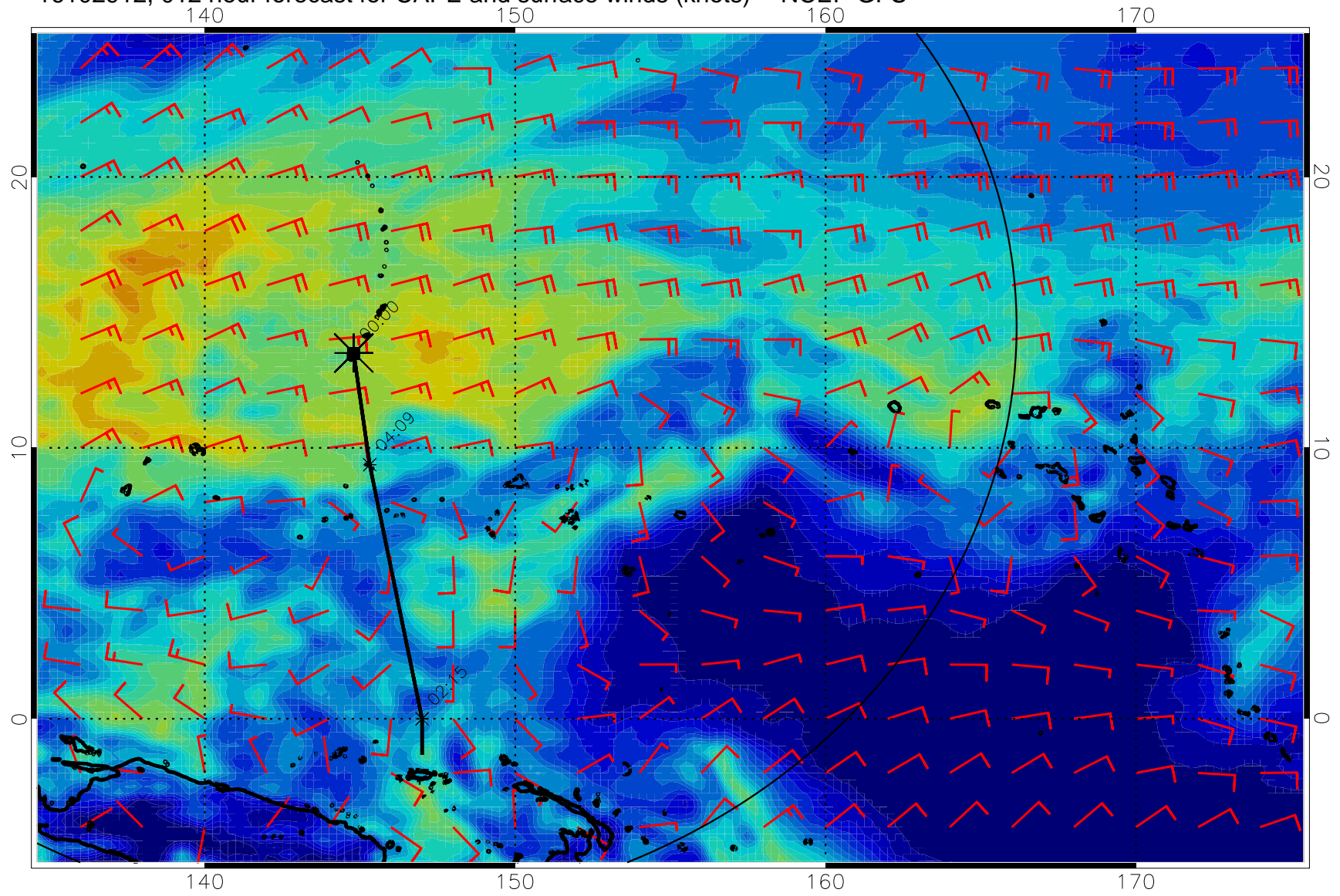
16102912, 012 hour forecast for CAPE and surface winds (knots) -- NCEP GFS
