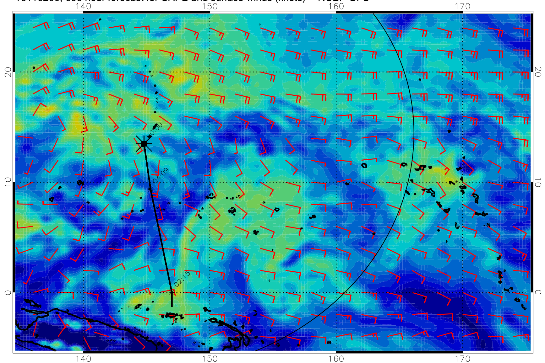
16110200, 096 hour forecast for CAPE and surface winds (knots) -- NCEP GFS
