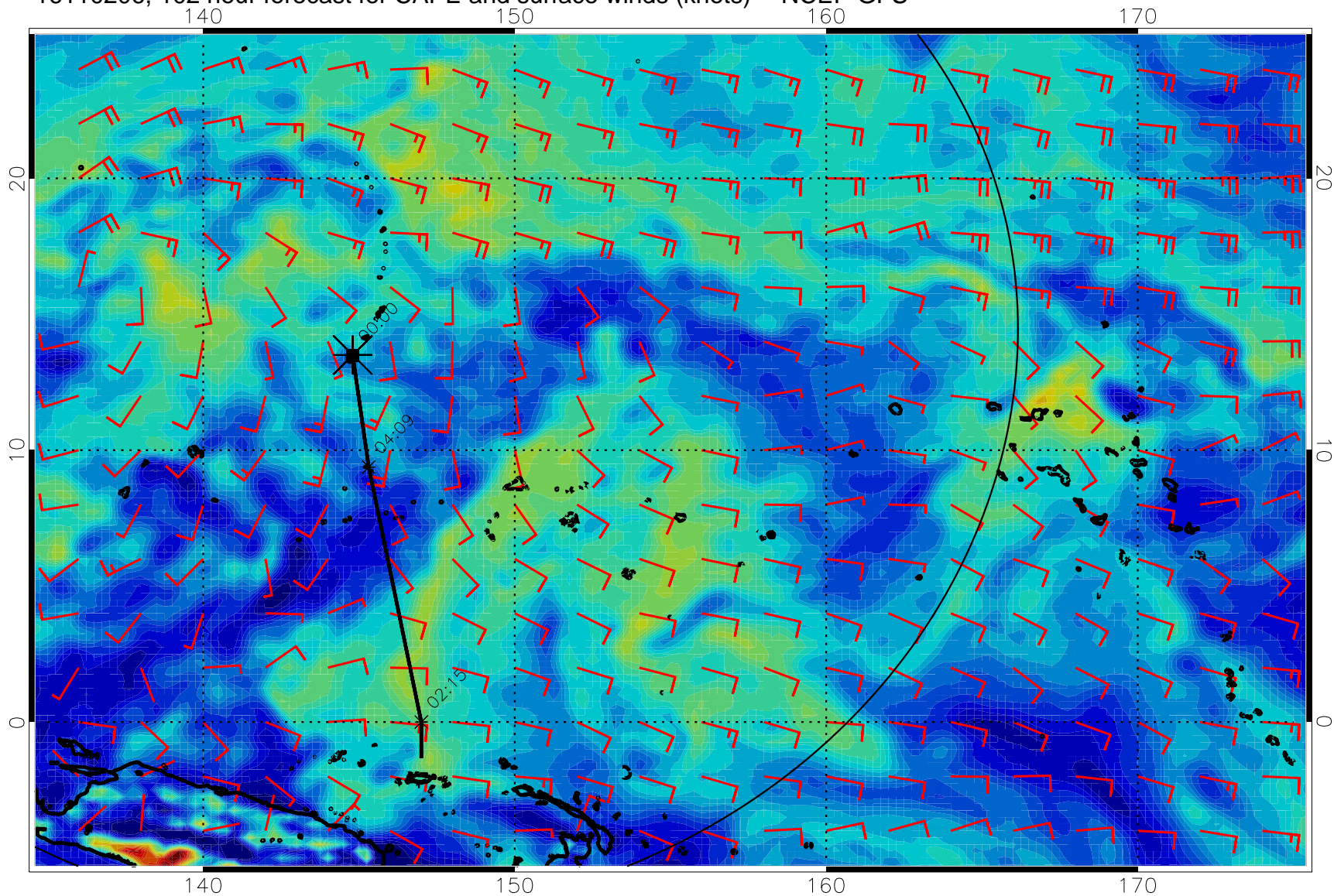
16110206, 102 hour forecast for CAPE and surface winds (knots) -- NCEP GFS
