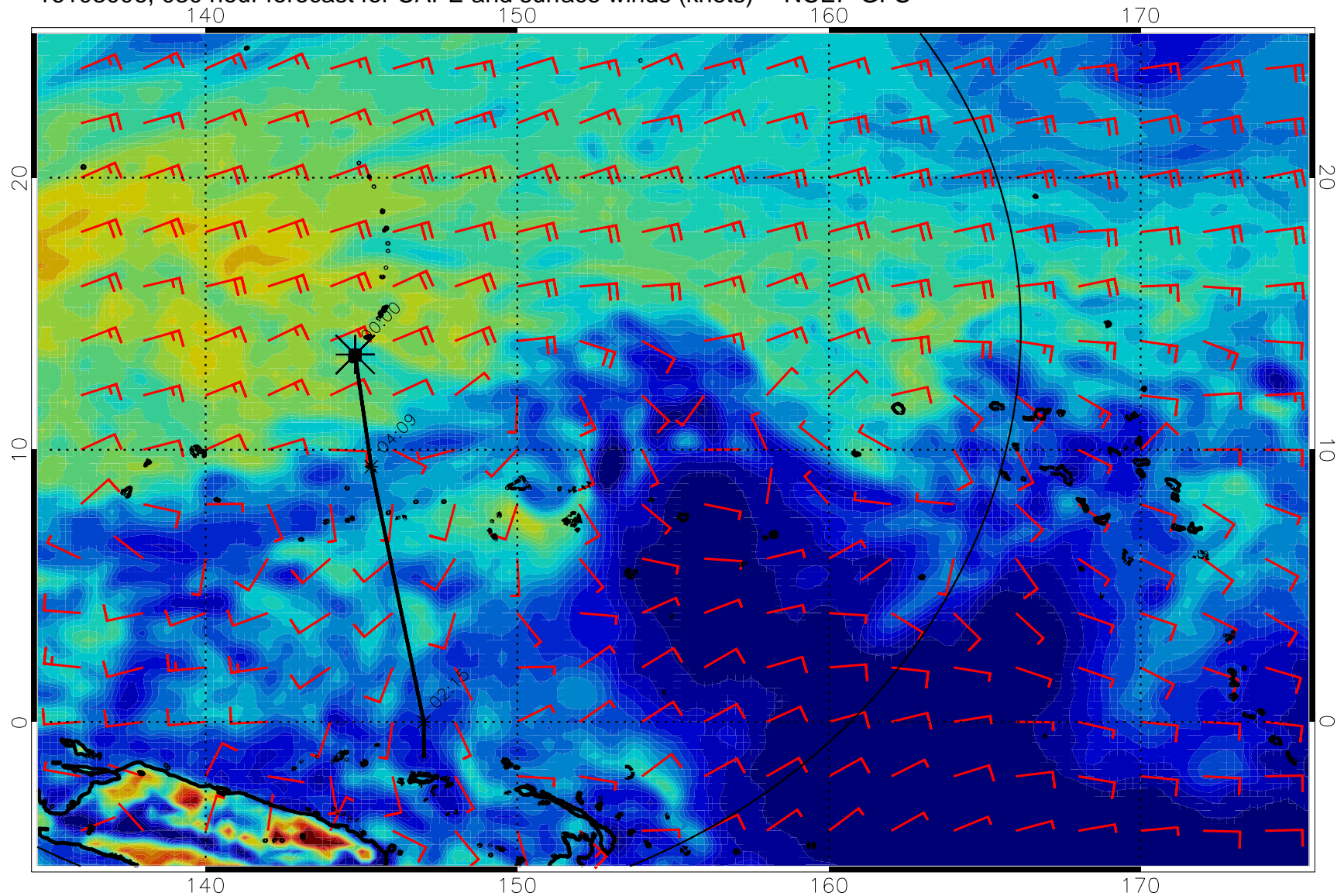
16103006, 030 hour forecast for CAPE and surface winds (knots) -- NCEP GFS
