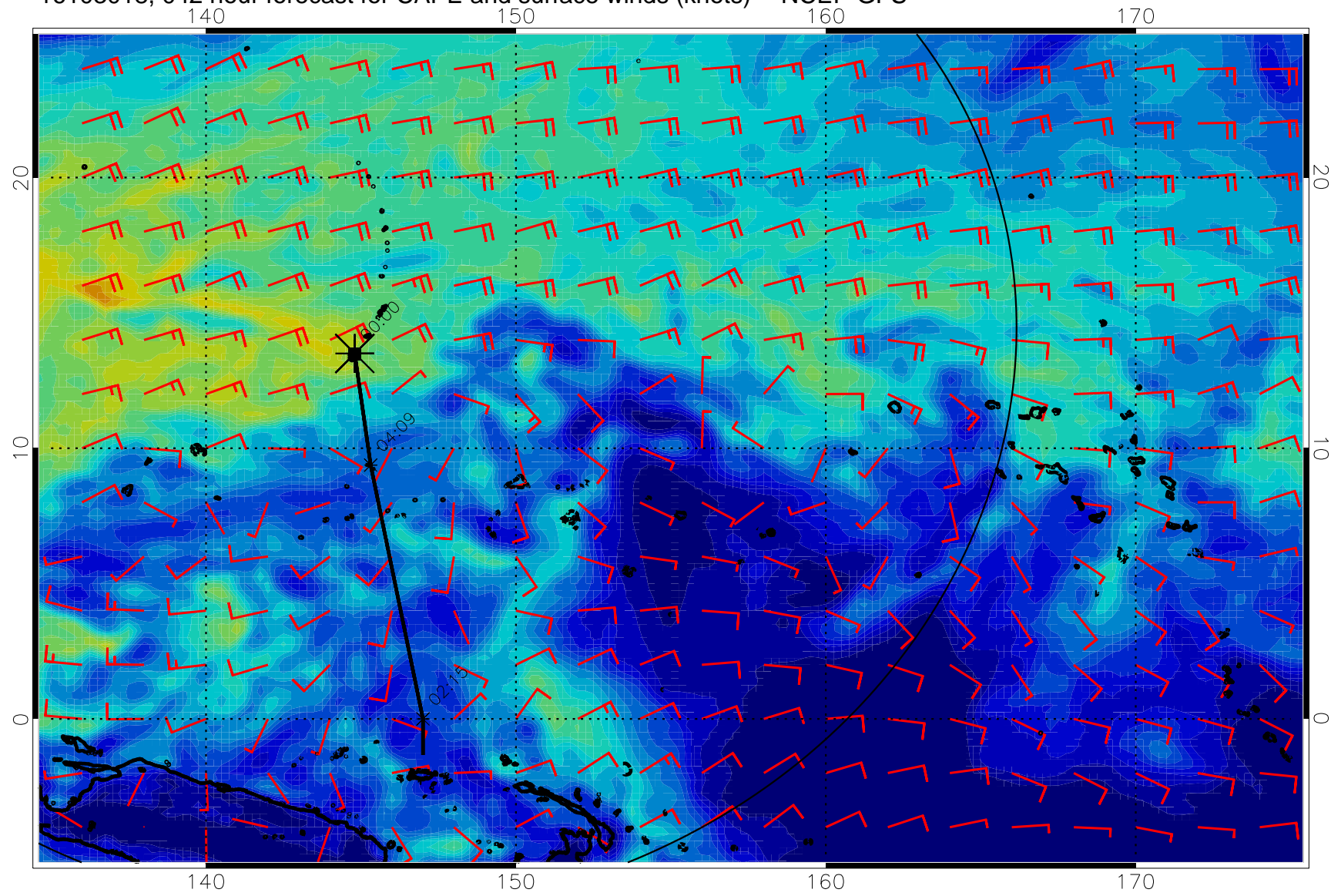
16103018, 042 hour forecast for CAPE and surface winds (knots) -- NCEP GFS
