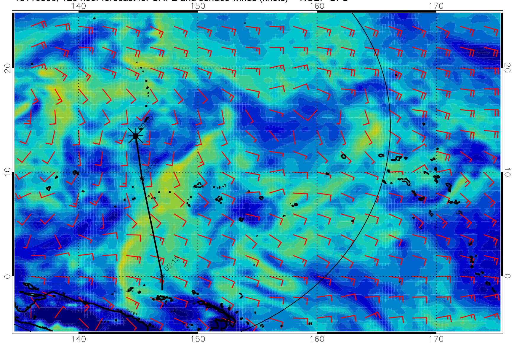
16110300, 120 hour forecast for CAPE and surface winds (knots) -- NCEP GFS
