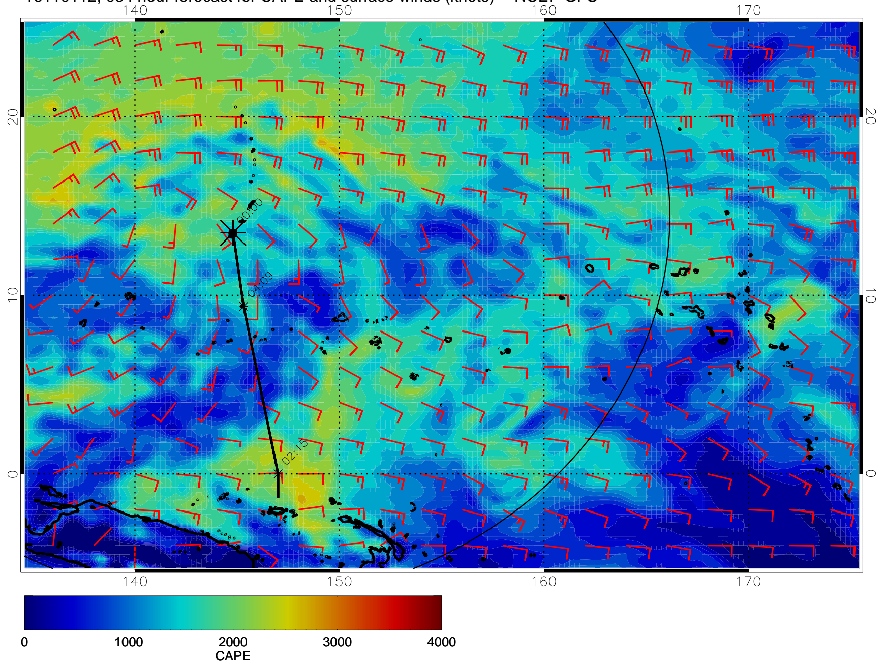
16110112, 084 hour forecast for CAPE and surface winds (knots) -- NCEP GFS
