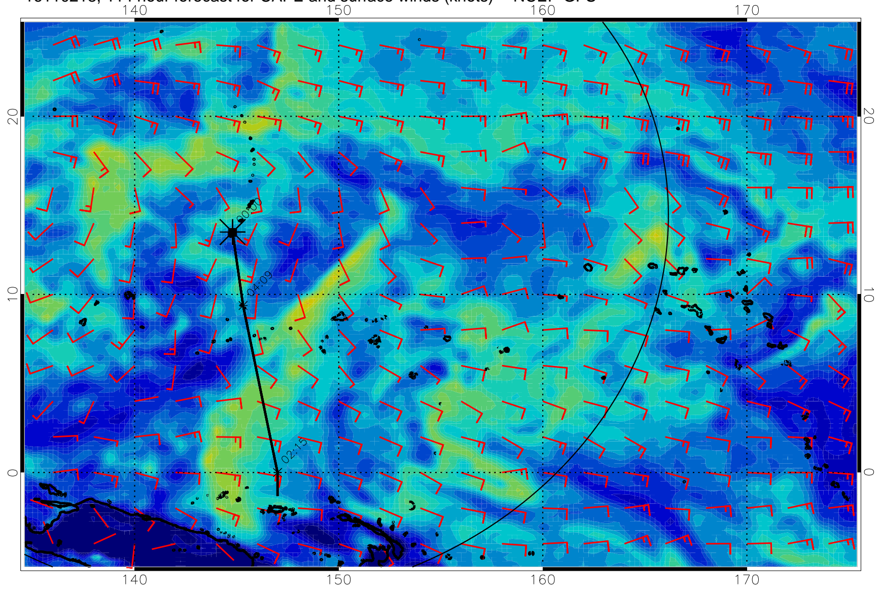
16110218, 114 hour forecast for CAPE and surface winds (knots) -- NCEP GFS
