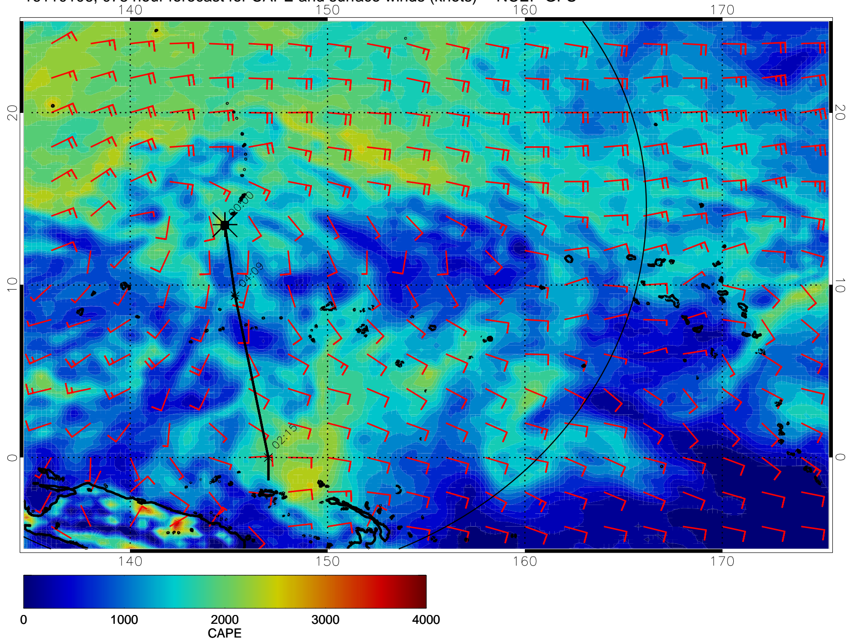
16110106, 078 hour forecast for CAPE and surface winds (knots) -- NCEP GFS
