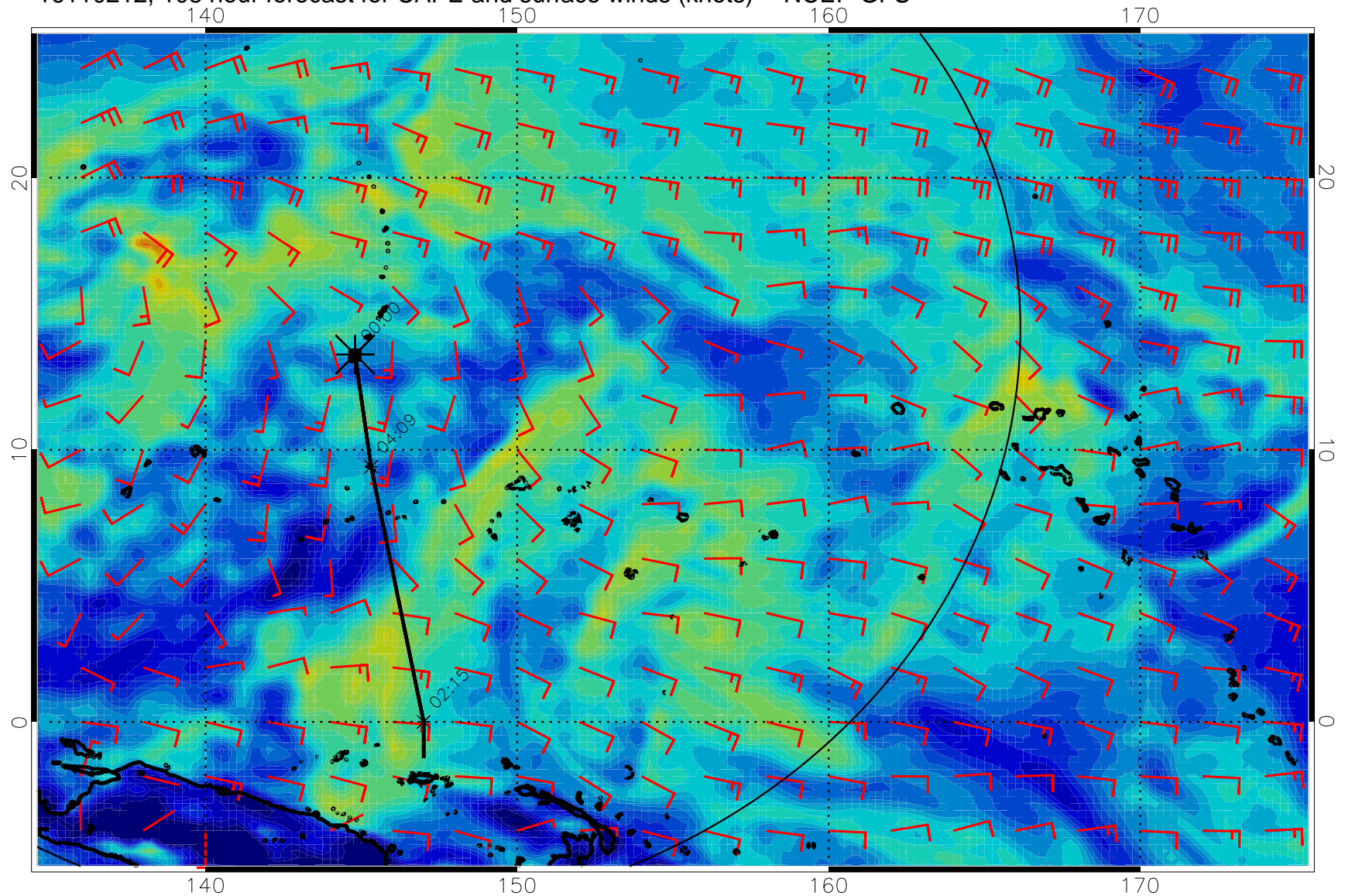
16110212, 108 hour forecast for CAPE and surface winds (knots) -- NCEP GFS
