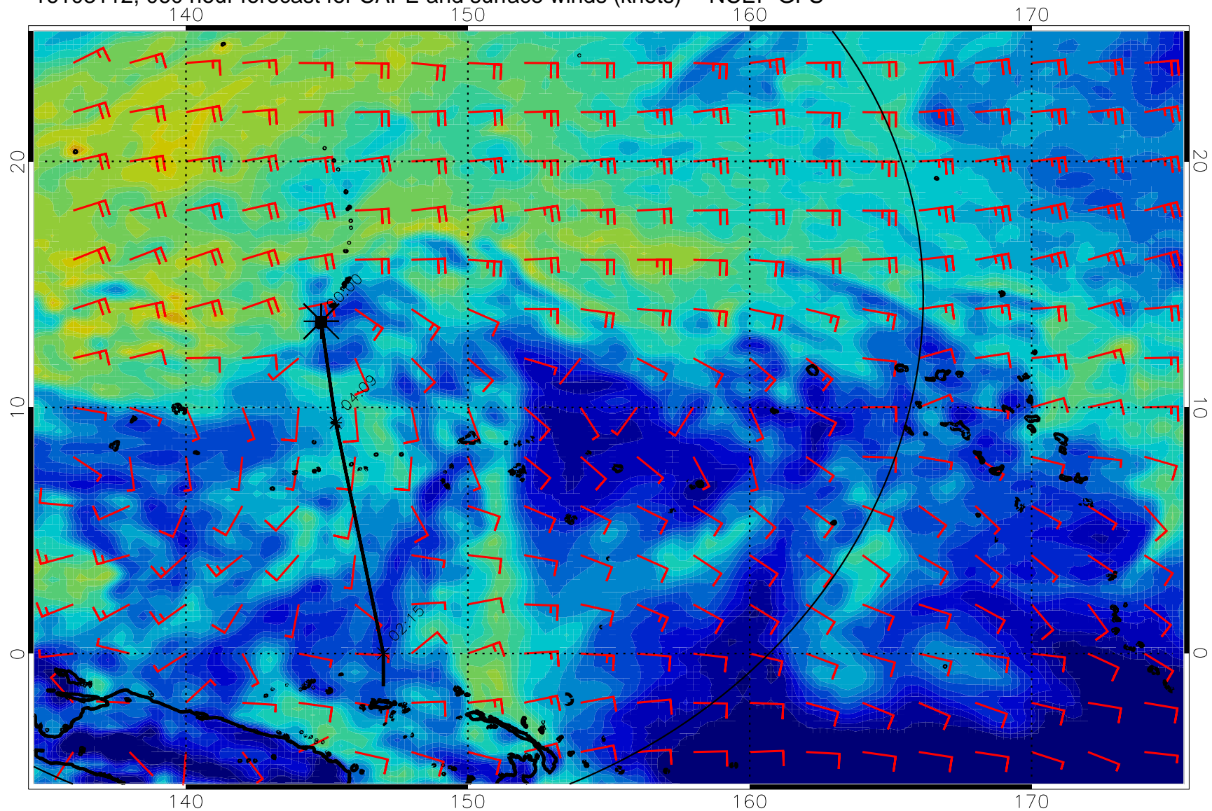
16103112, 060 hour forecast for CAPE and surface winds (knots) -- NCEP GFS
