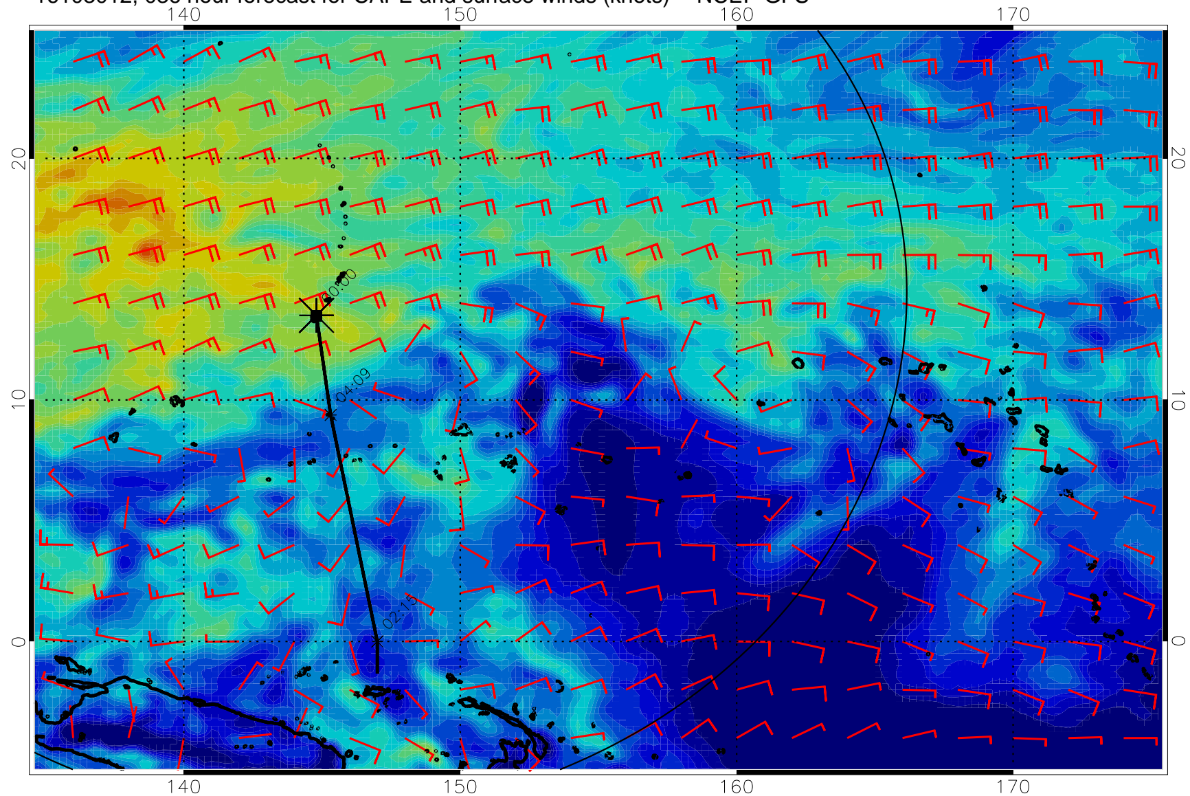
16103012, 036 hour forecast for CAPE and surface winds (knots) -- NCEP GFS
