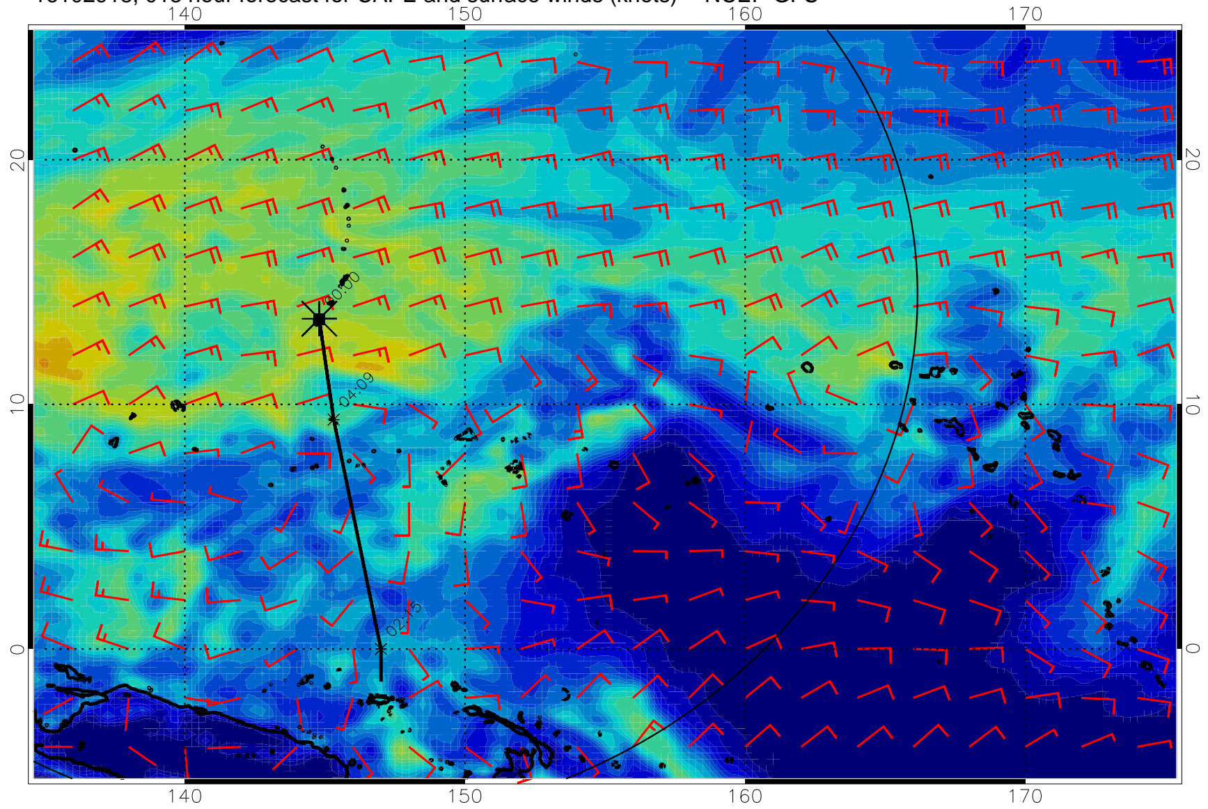
16102918, 018 hour forecast for CAPE and surface winds (knots) -- NCEP GFS
