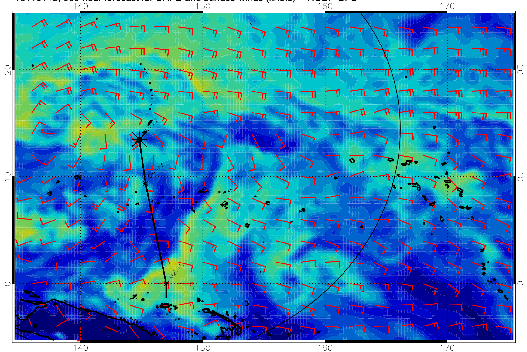
16110118, 090 hour forecast for CAPE and surface winds (knots) -- NCEP GFS
