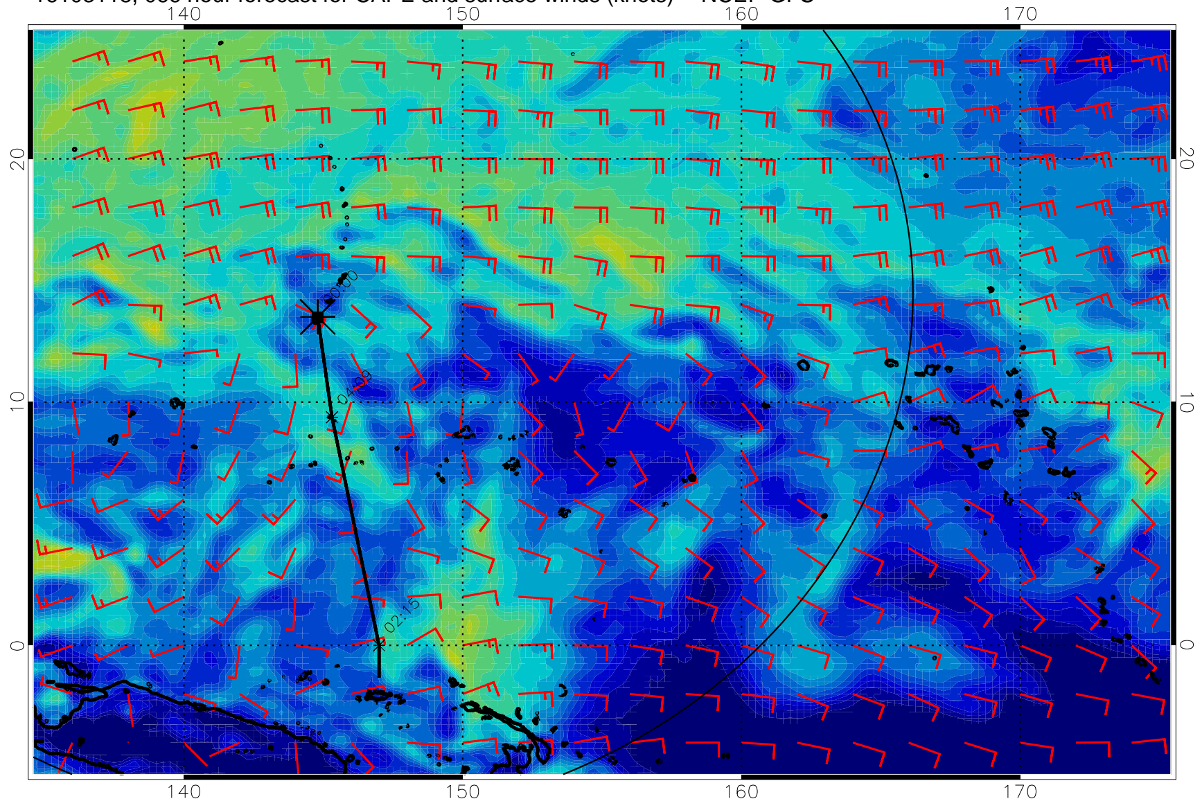
16103118, 066 hour forecast for CAPE and surface winds (knots) -- NCEP GFS
