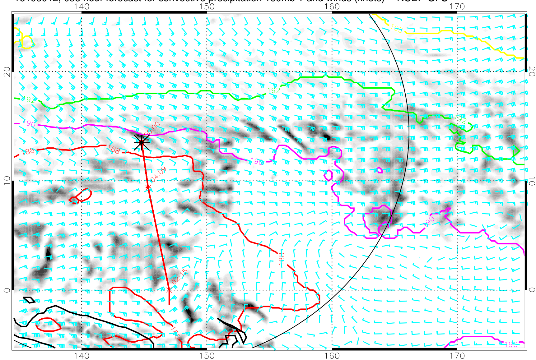
16103012, 036 hour forecast for convective precipitation 100mb T and winds (knots) -- NCEP GFS
