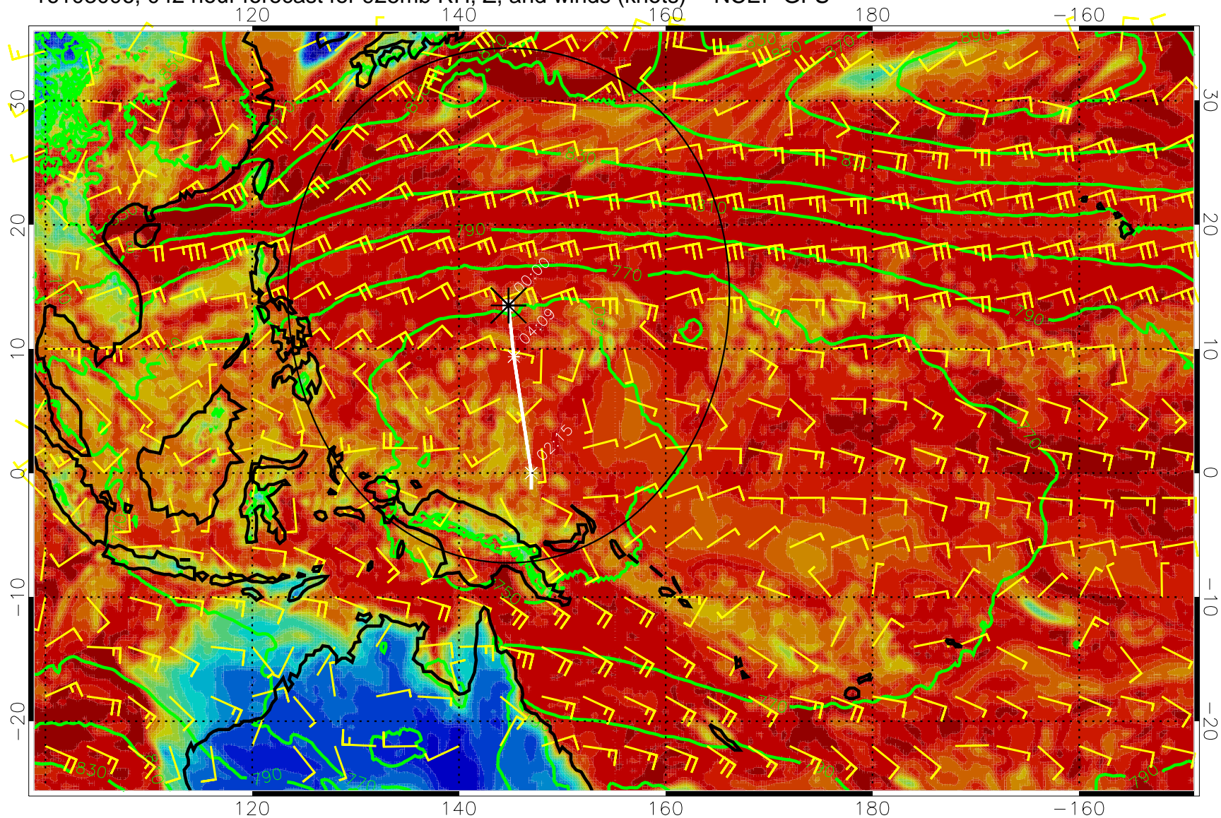
16103006, 042 hour forecast for 925mb RH, Z, and winds (knots) -- NCEP GFS
