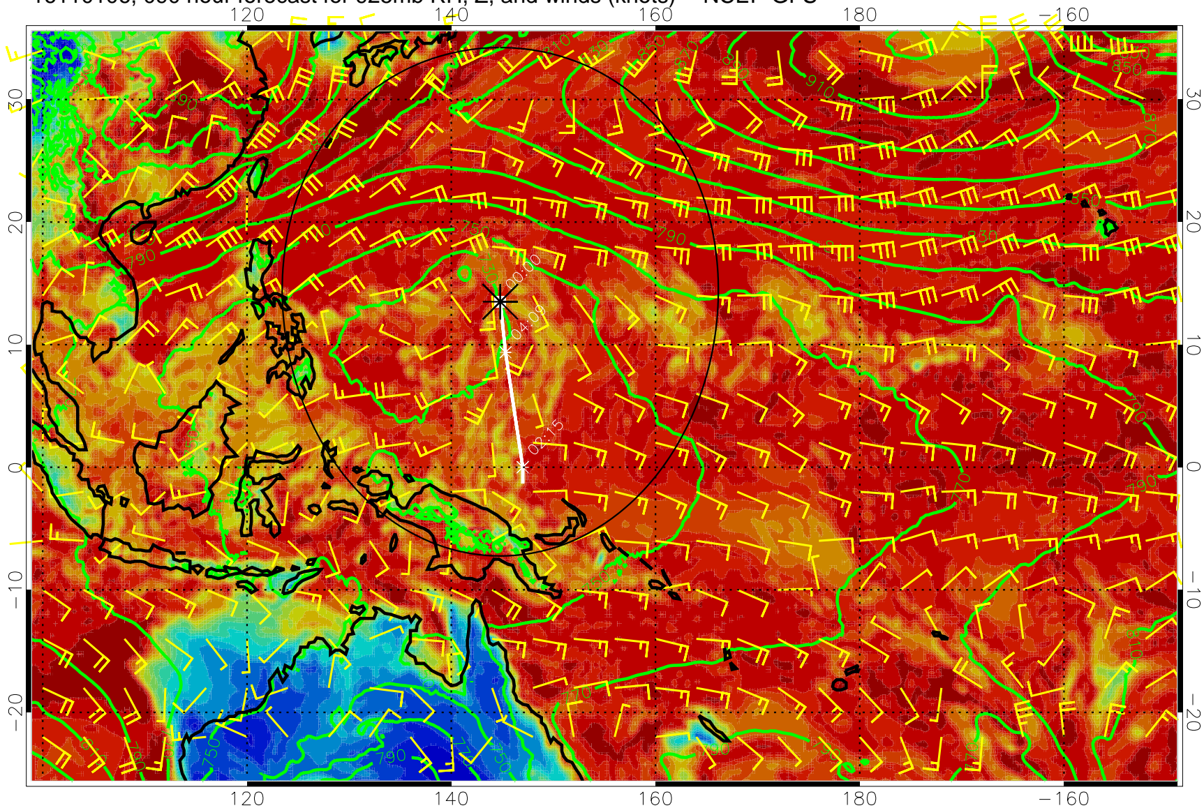
16110106, 090 hour forecast for 925mb RH, Z, and winds (knots) -- NCEP GFS
