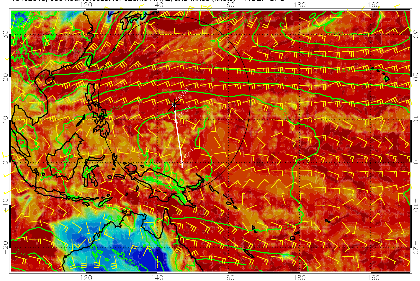
16102918, 030 hour forecast for 925mb RH, Z, and winds (knots) -- NCEP GFS
