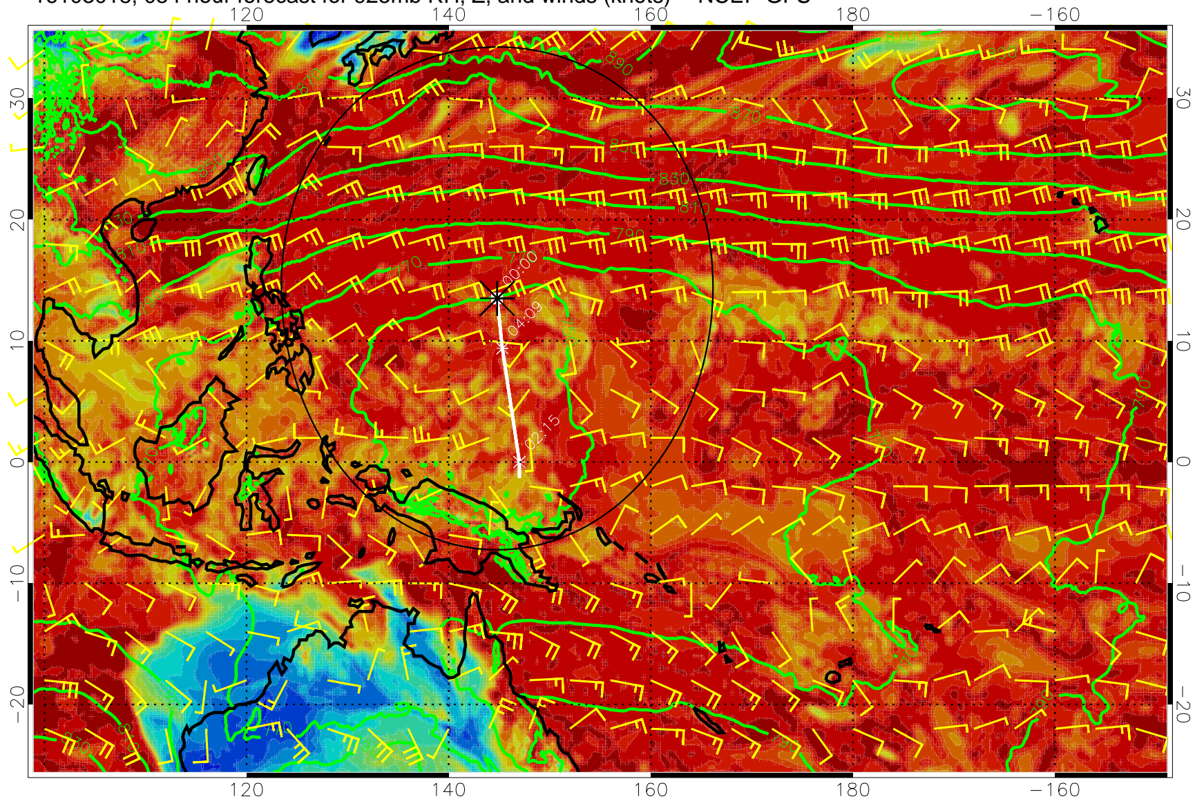
16103018, 054 hour forecast for 925mb RH, Z, and winds (knots) -- NCEP GFS
