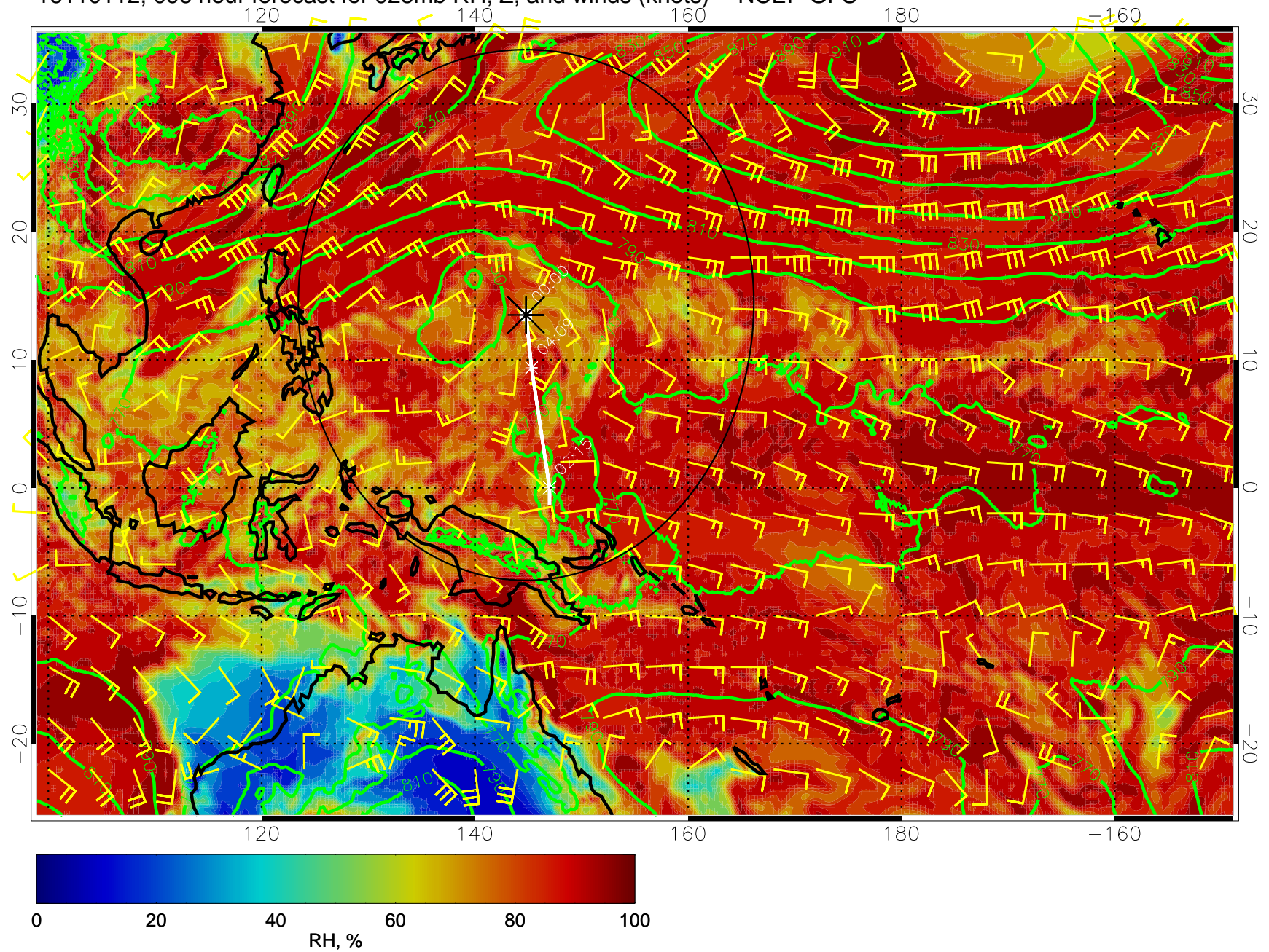
16110112, 096 hour forecast for 925mb RH, Z, and winds (knots) -- NCEP GFS
