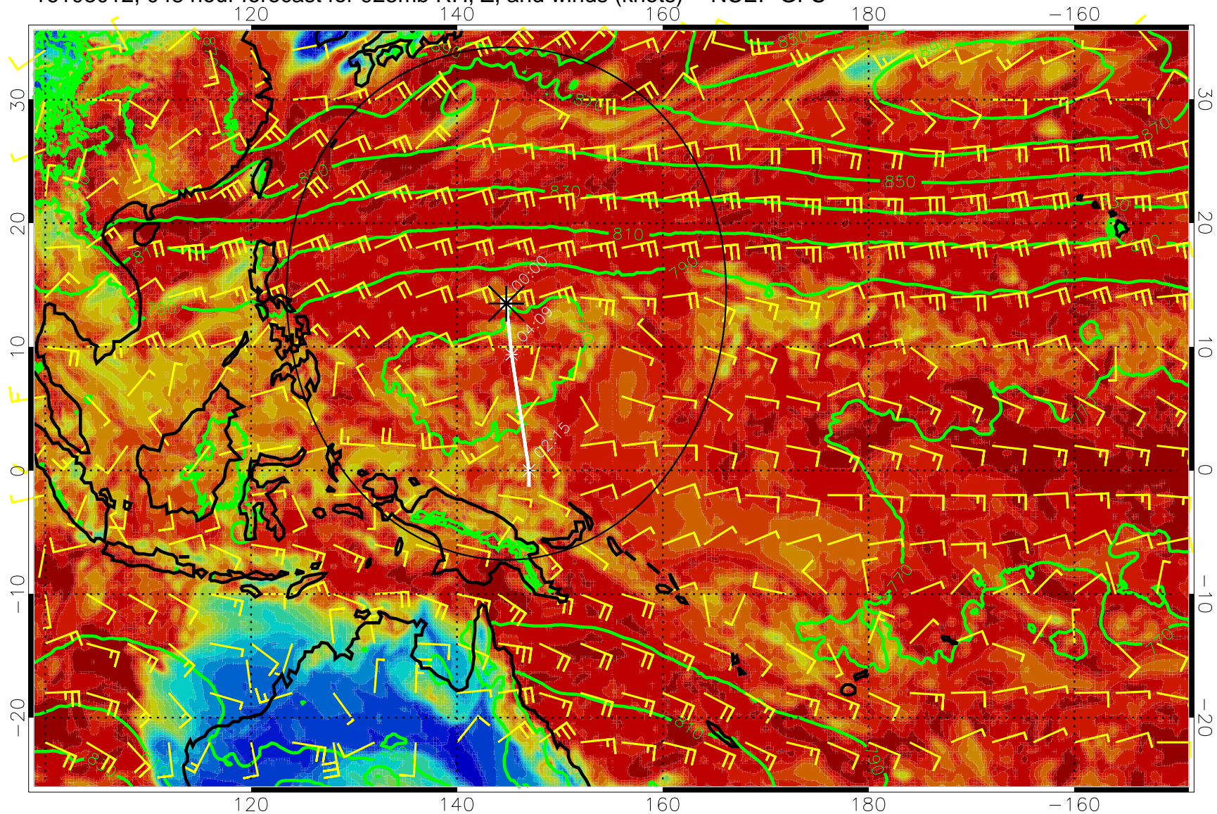
16103012, 048 hour forecast for 925mb RH, Z, and winds (knots) -- NCEP GFS
