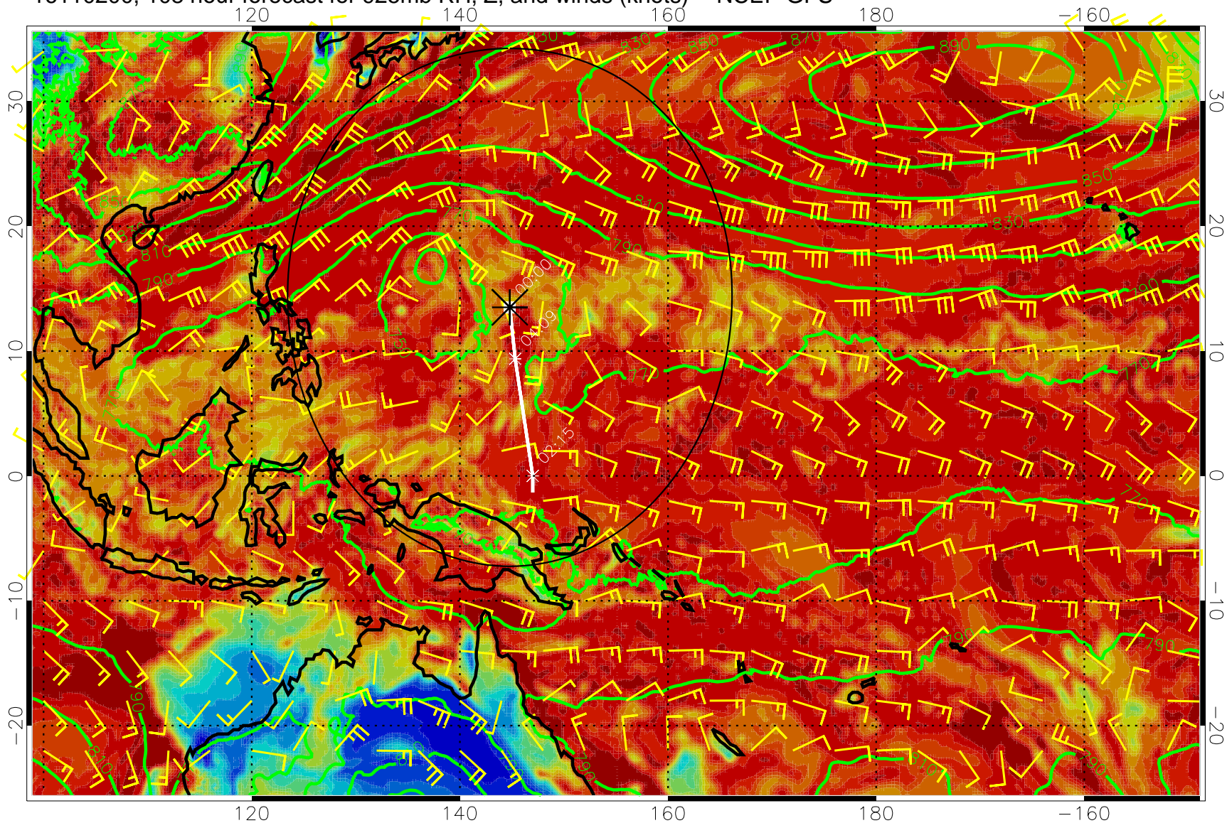
16110200, 108 hour forecast for 925mb RH, Z, and winds (knots) -- NCEP GFS
