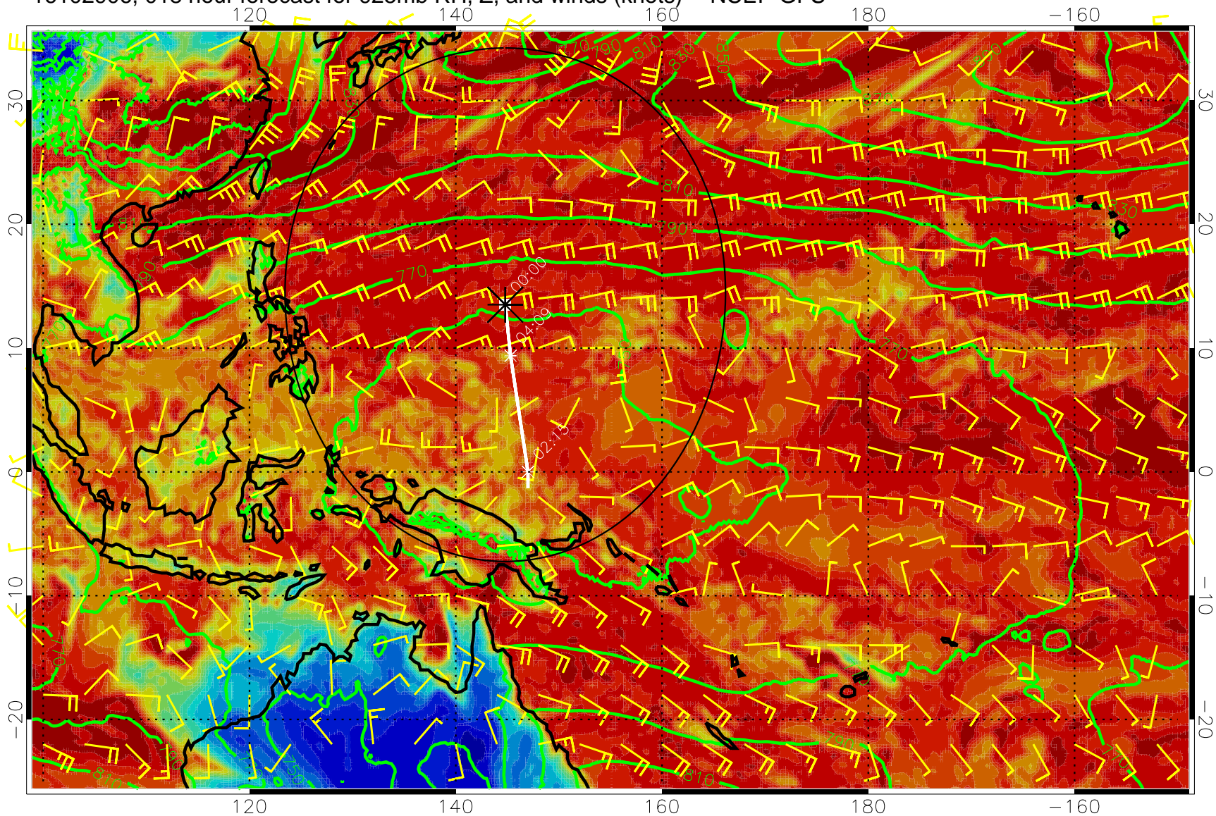
16102906, 018 hour forecast for 925mb RH, Z, and winds (knots) -- NCEP GFS
