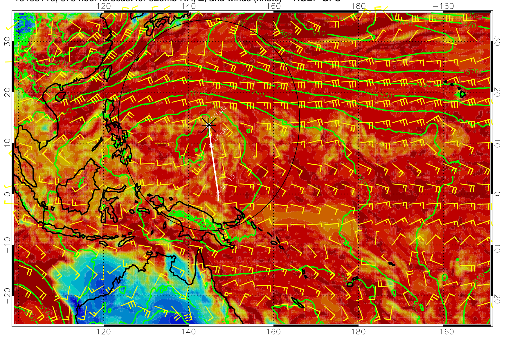
16103118, 078 hour forecast for 925mb RH, Z, and winds (knots) -- NCEP GFS
