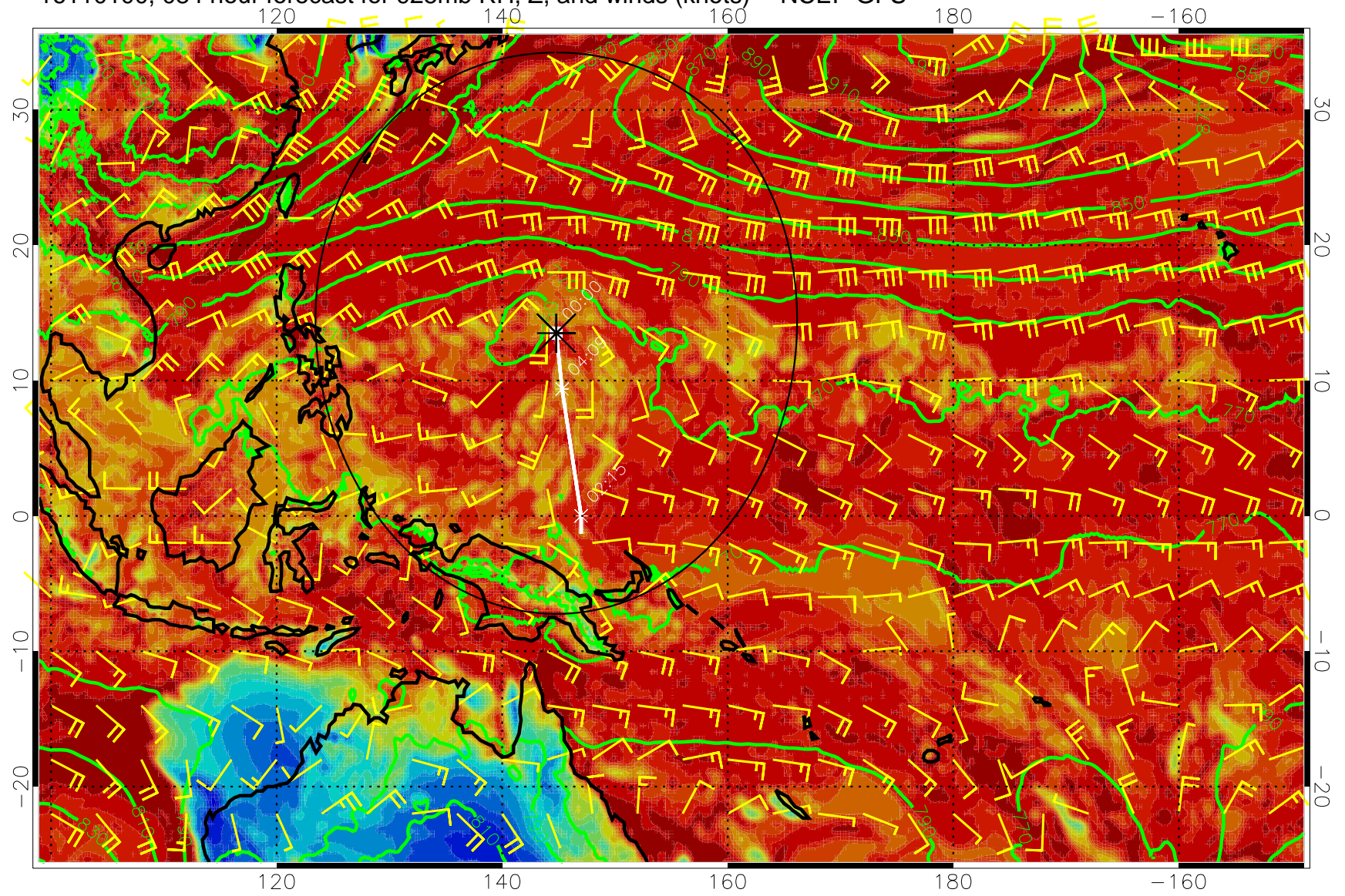
16110100, 084 hour forecast for 925mb RH, Z, and winds (knots) -- NCEP GFS
