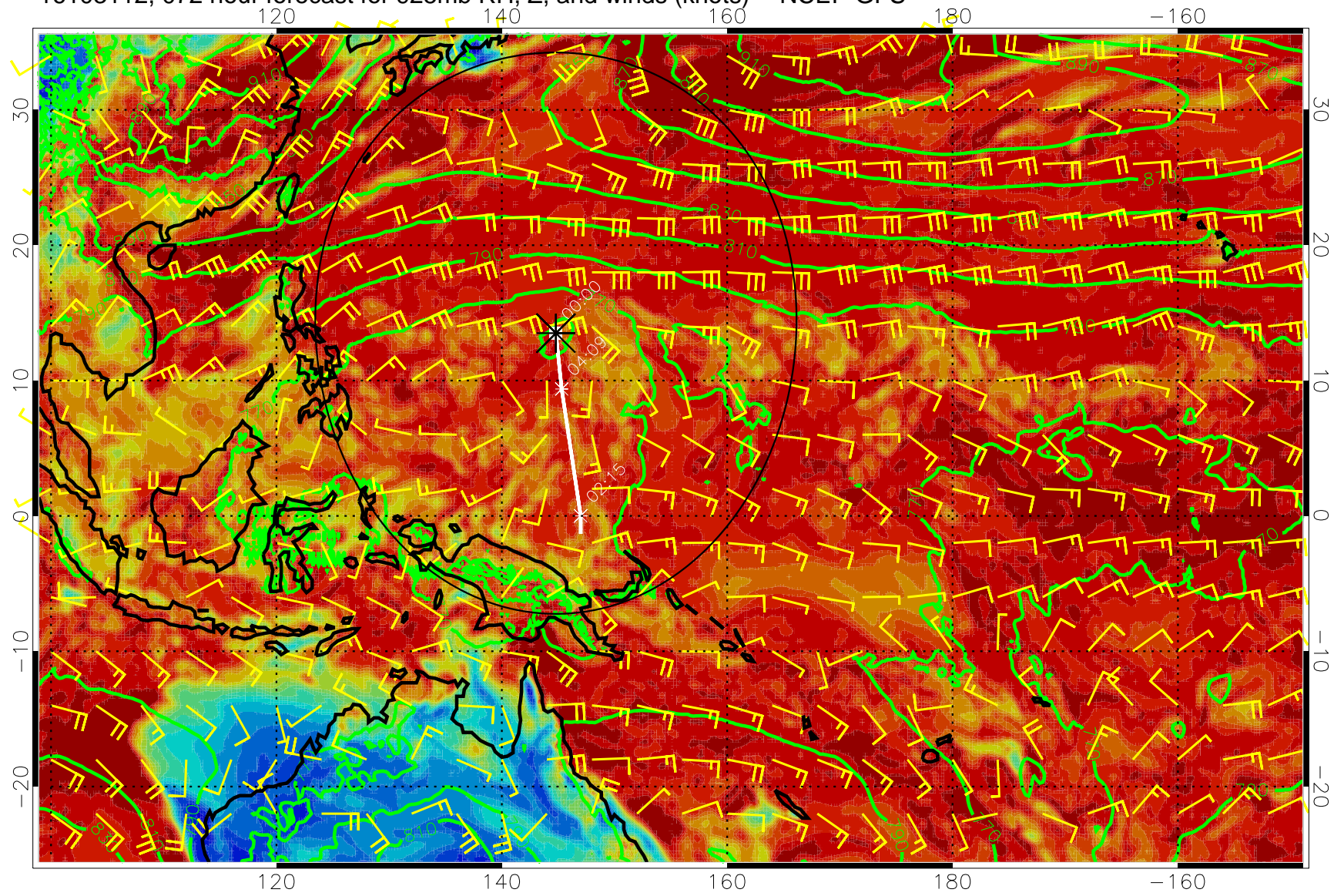
16103112, 072 hour forecast for 925mb RH, Z, and winds (knots) -- NCEP GFS
