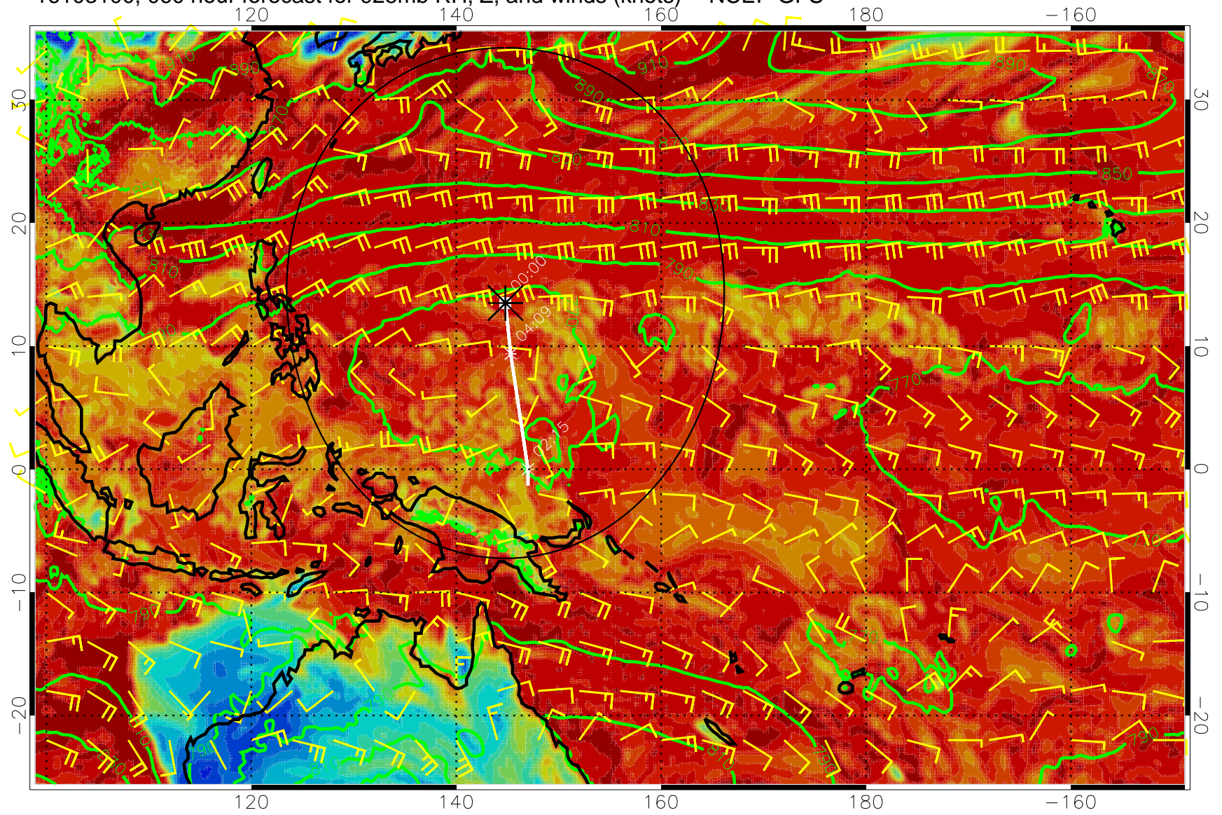
16103100, 060 hour forecast for 925mb RH, Z, and winds (knots) -- NCEP GFS
