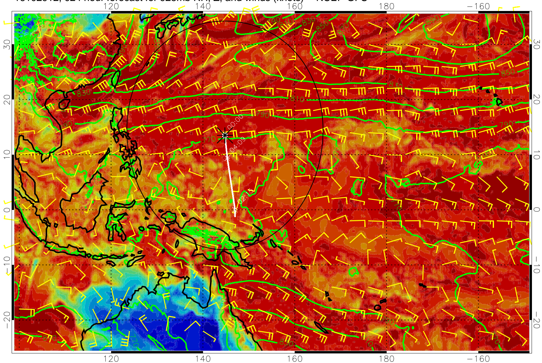
16102912, 024 hour forecast for 925mb RH, Z, and winds (knots) -- NCEP GFS
