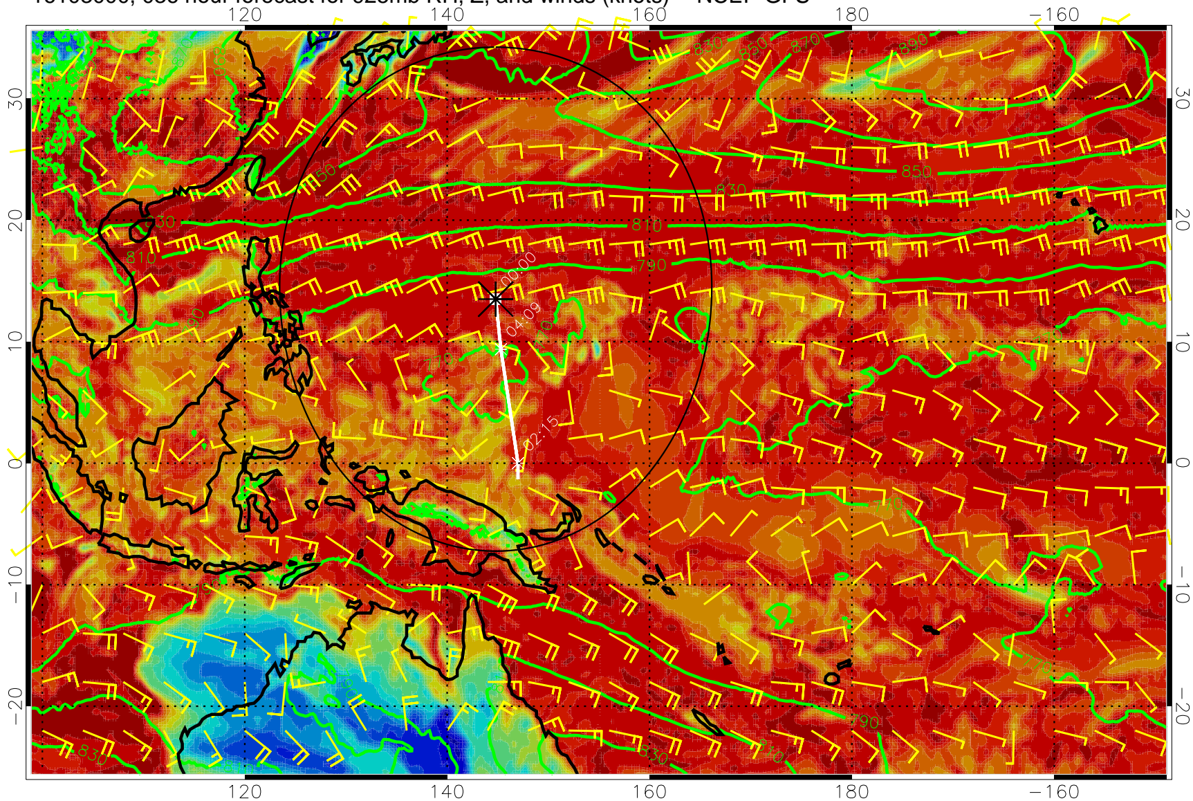
16103000, 036 hour forecast for 925mb RH, Z, and winds (knots) -- NCEP GFS
