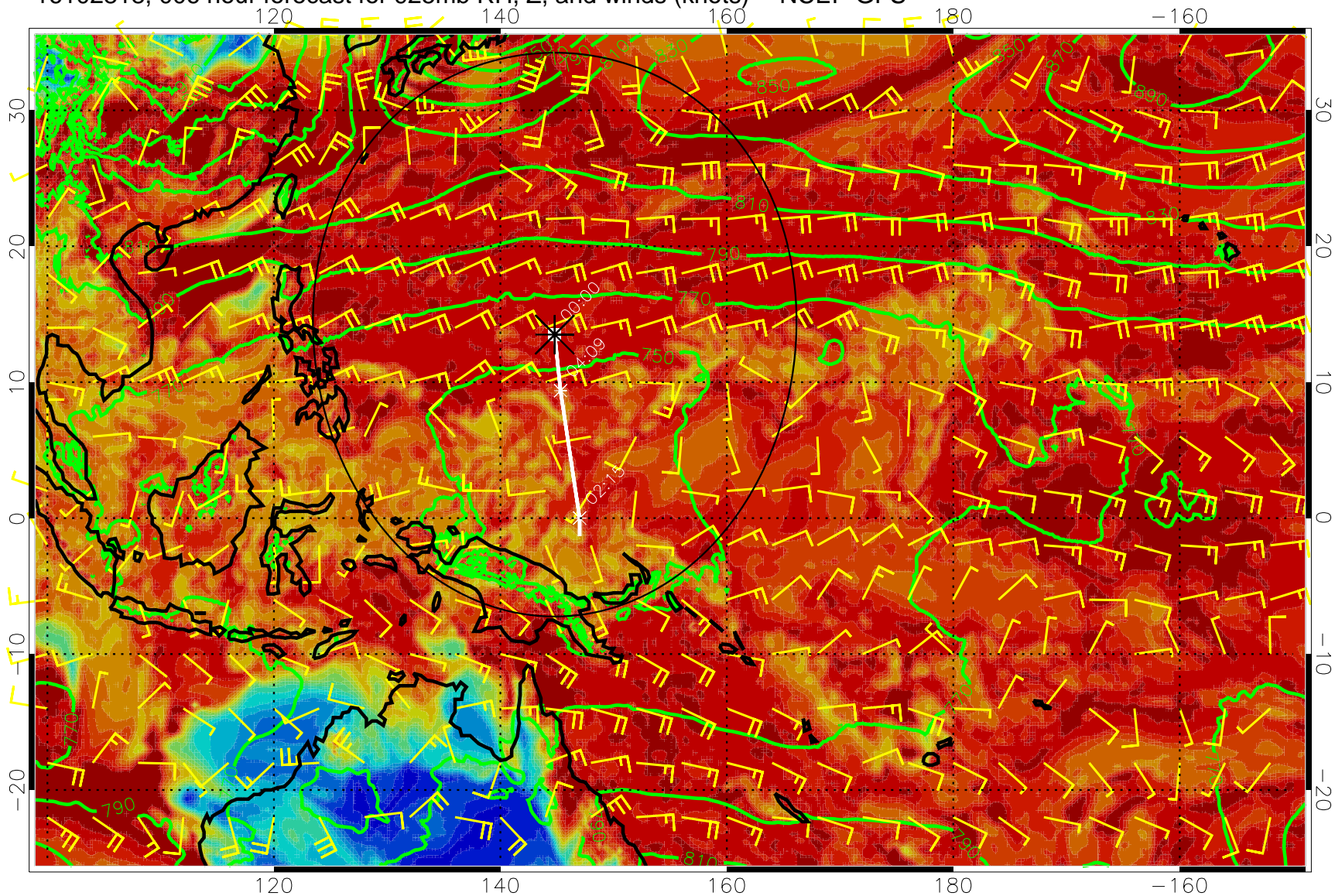
16102818, 006 hour forecast for 925mb RH, Z, and winds (knots) -- NCEP GFS
