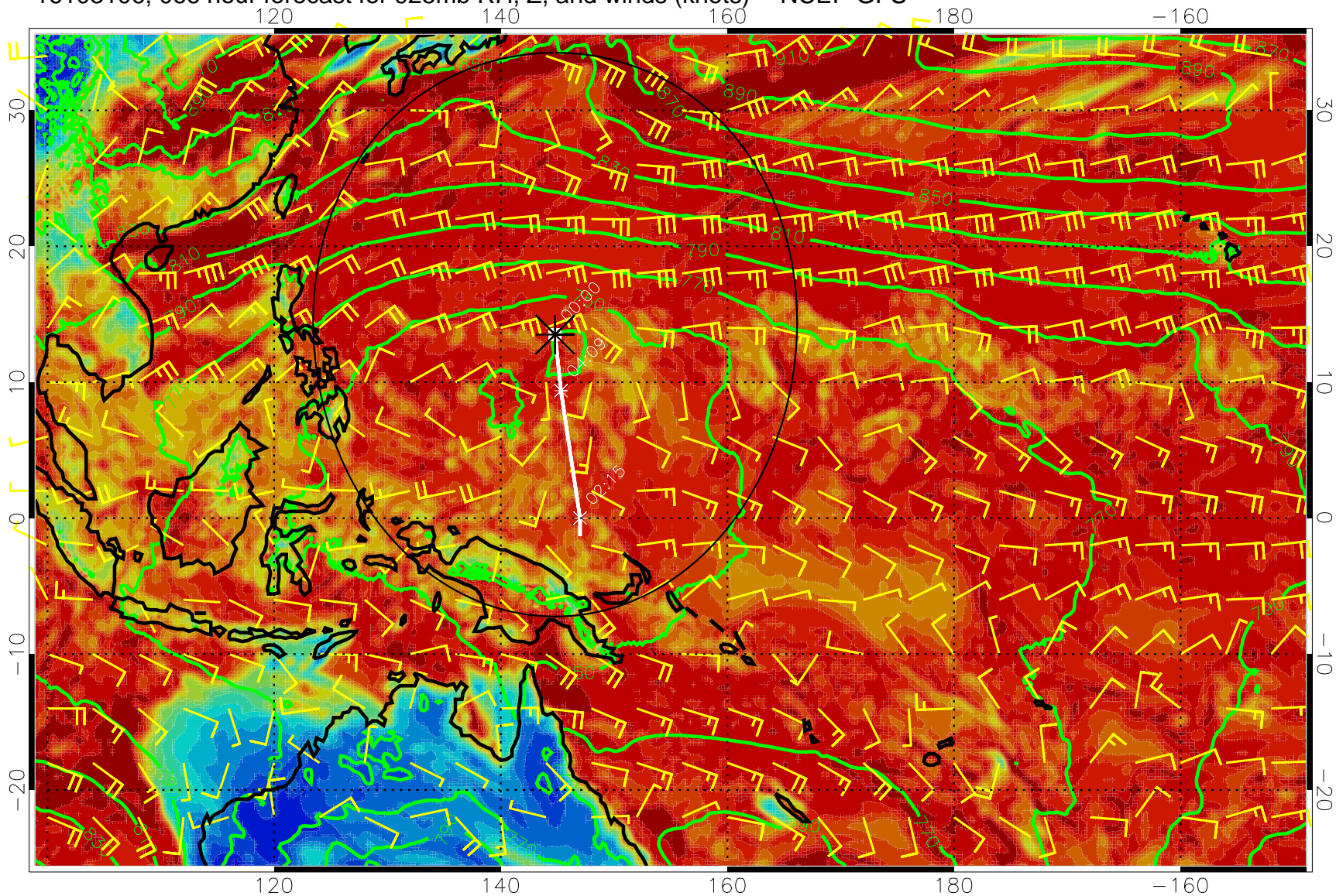
16103106, 066 hour forecast for 925mb RH, Z, and winds (knots) -- NCEP GFS
