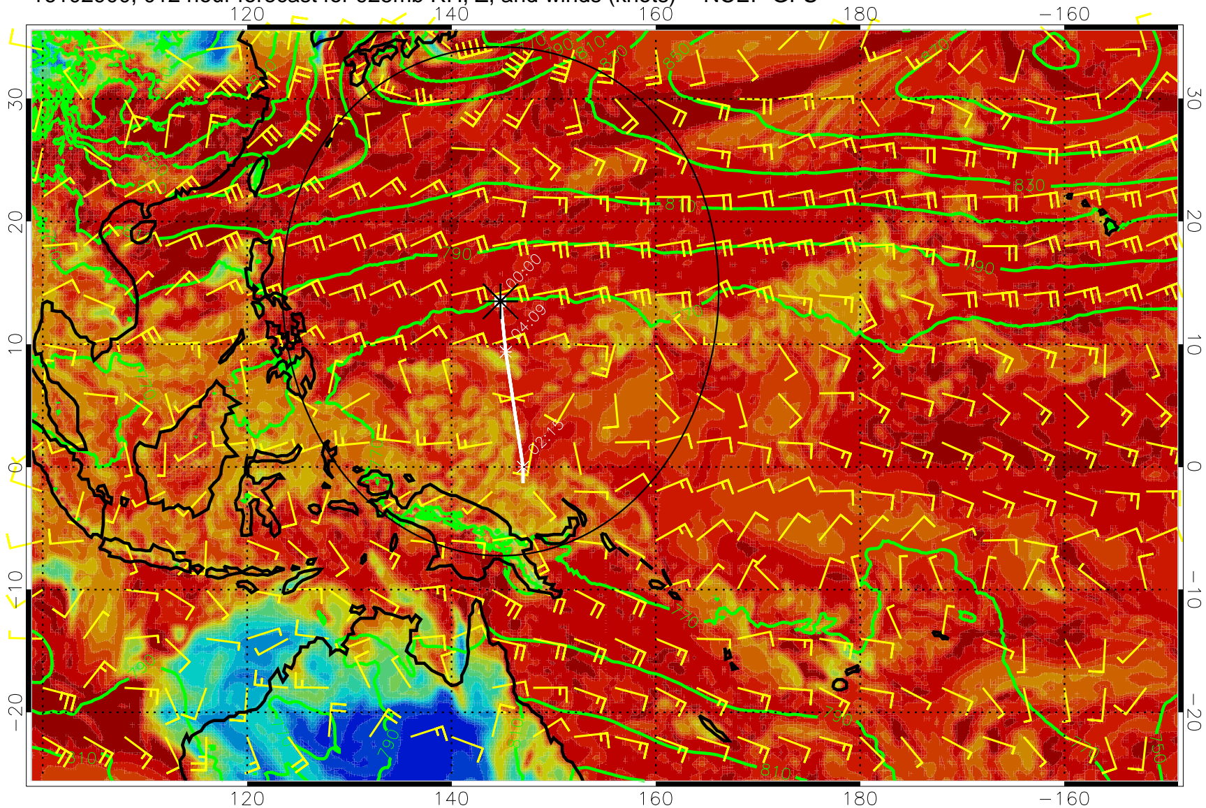
16102900, 012 hour forecast for 925mb RH, Z, and winds (knots) -- NCEP GFS
