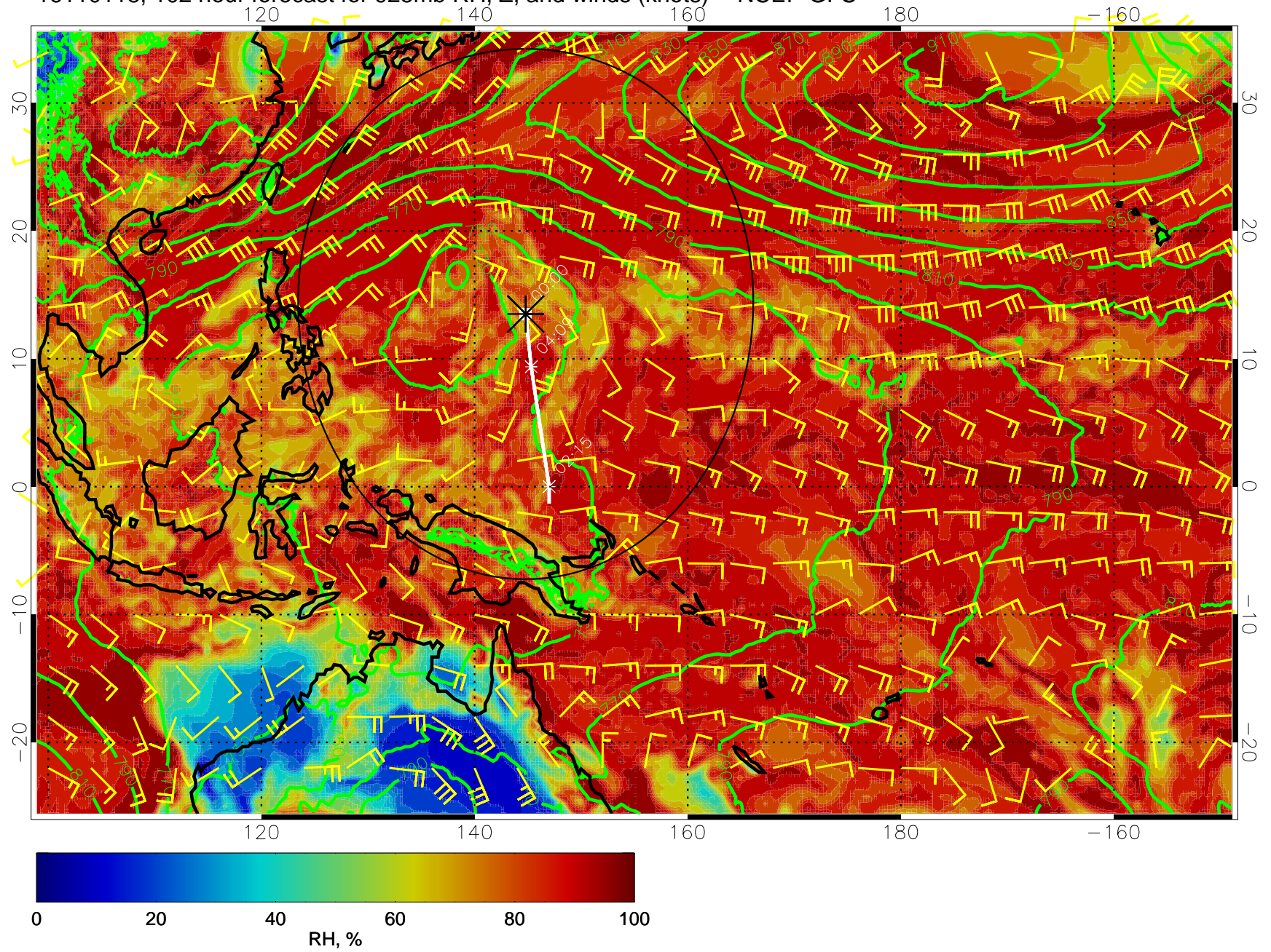
16110118, 102 hour forecast for 925mb RH, Z, and winds (knots) -- NCEP GFS
