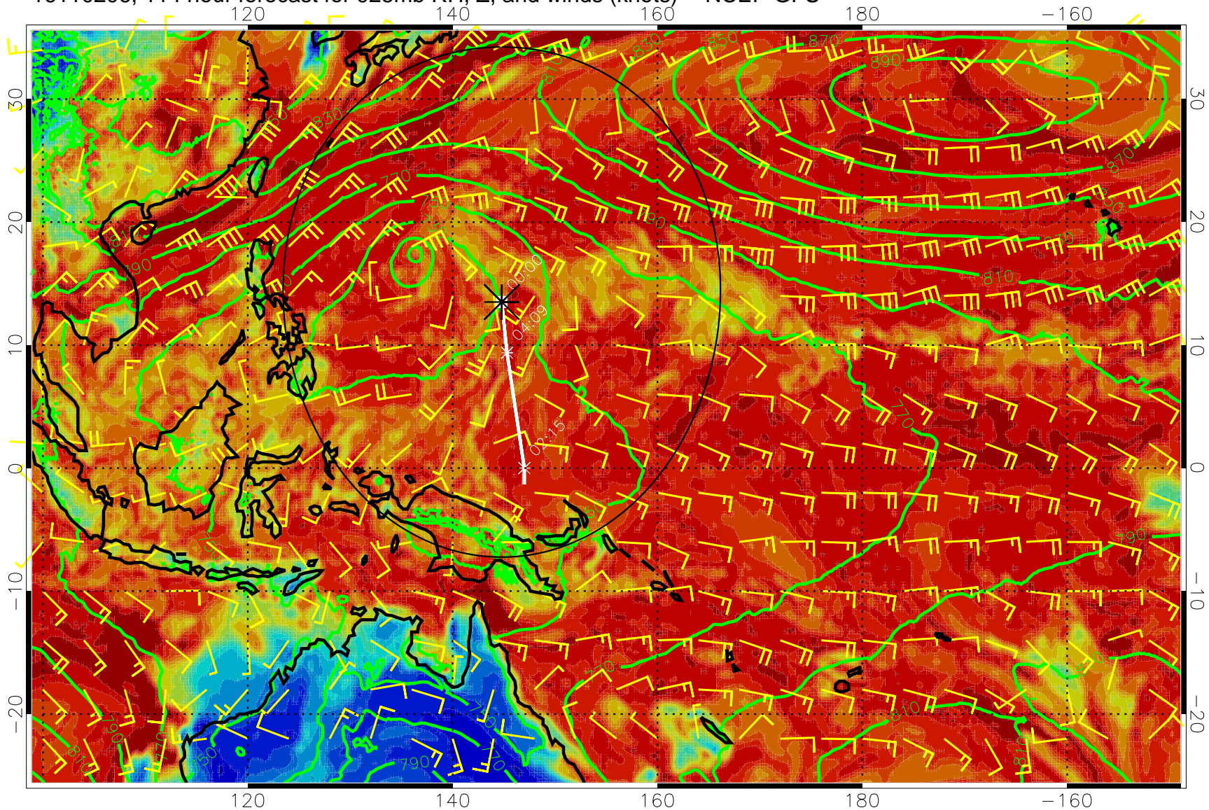
16110206, 114 hour forecast for 925mb RH, Z, and winds (knots) -- NCEP GFS
