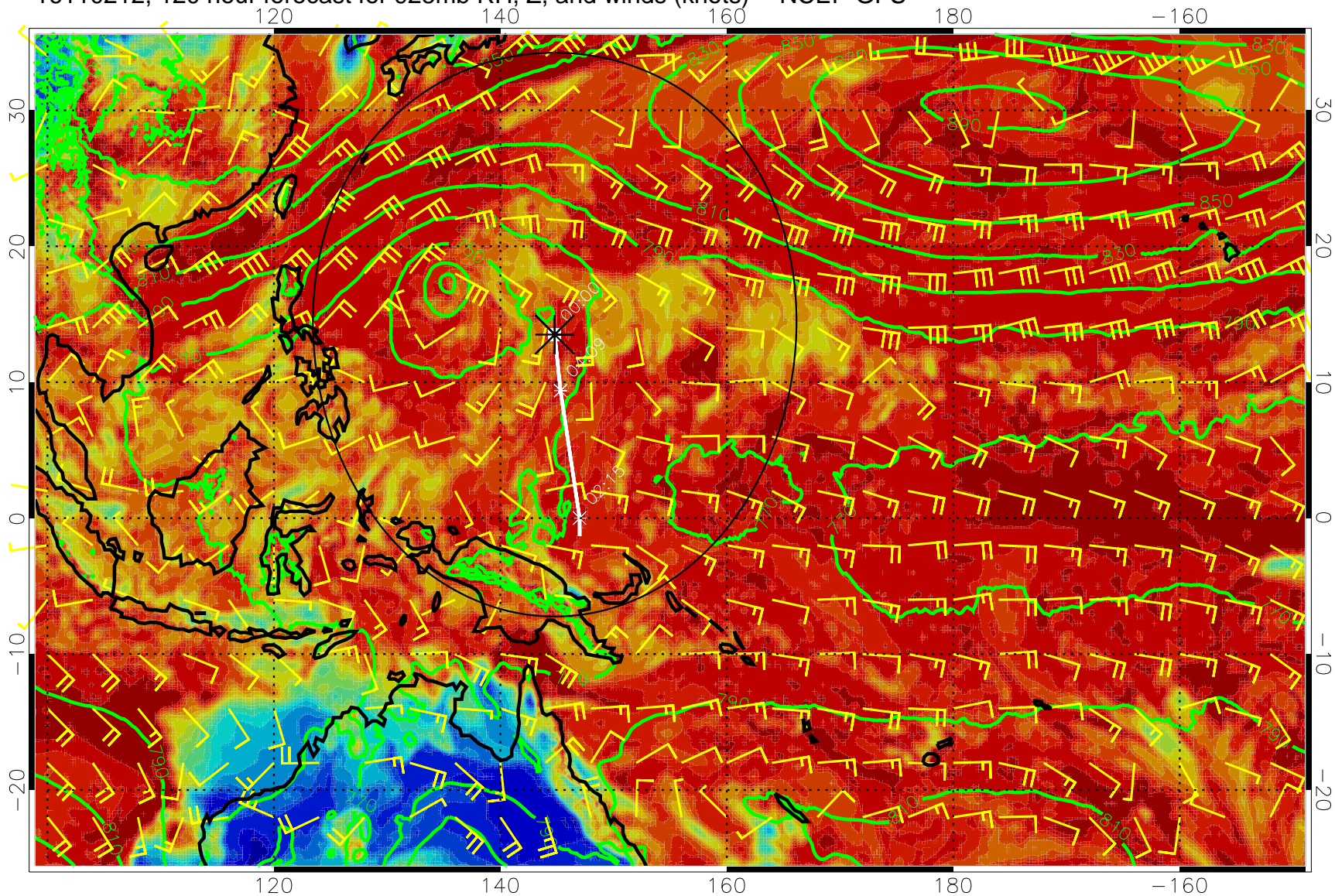
16110212, 120 hour forecast for 925mb RH, Z, and winds (knots) -- NCEP GFS
