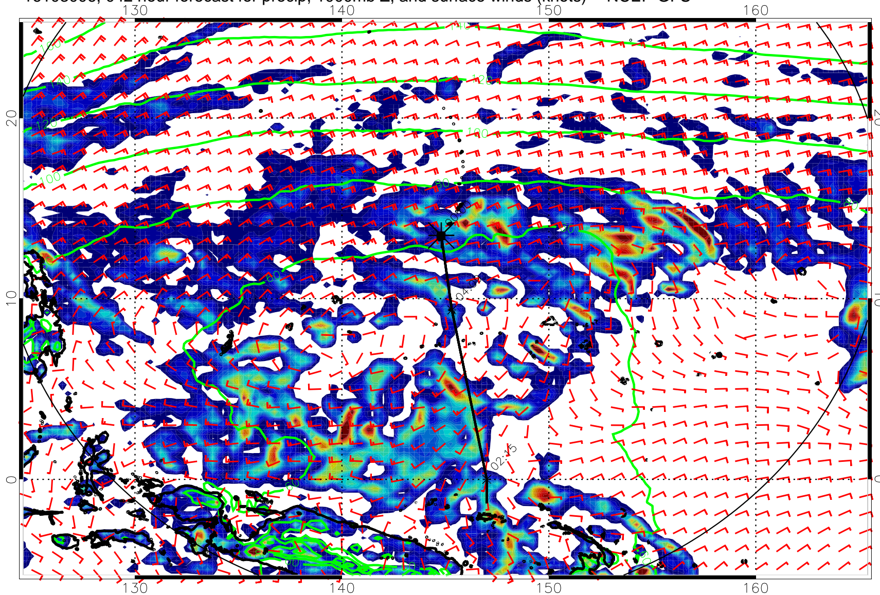
16103006, 04Z hour forecast for precip, 1000mb Z, and surface winds (knots) -- NCEP GFS
