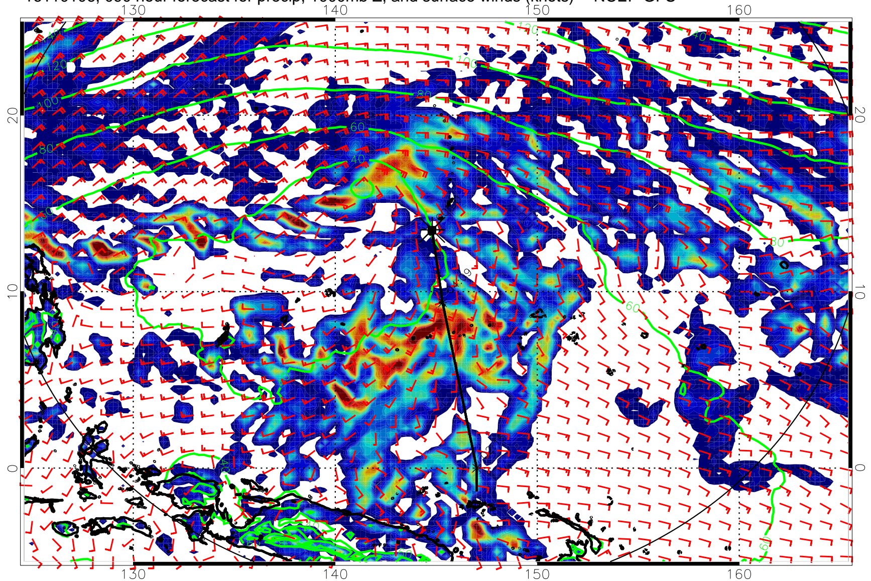
16110106, 090 hour forecast for precip, 1000mb Z, and surface winds (knots) -- NCEP GFS
