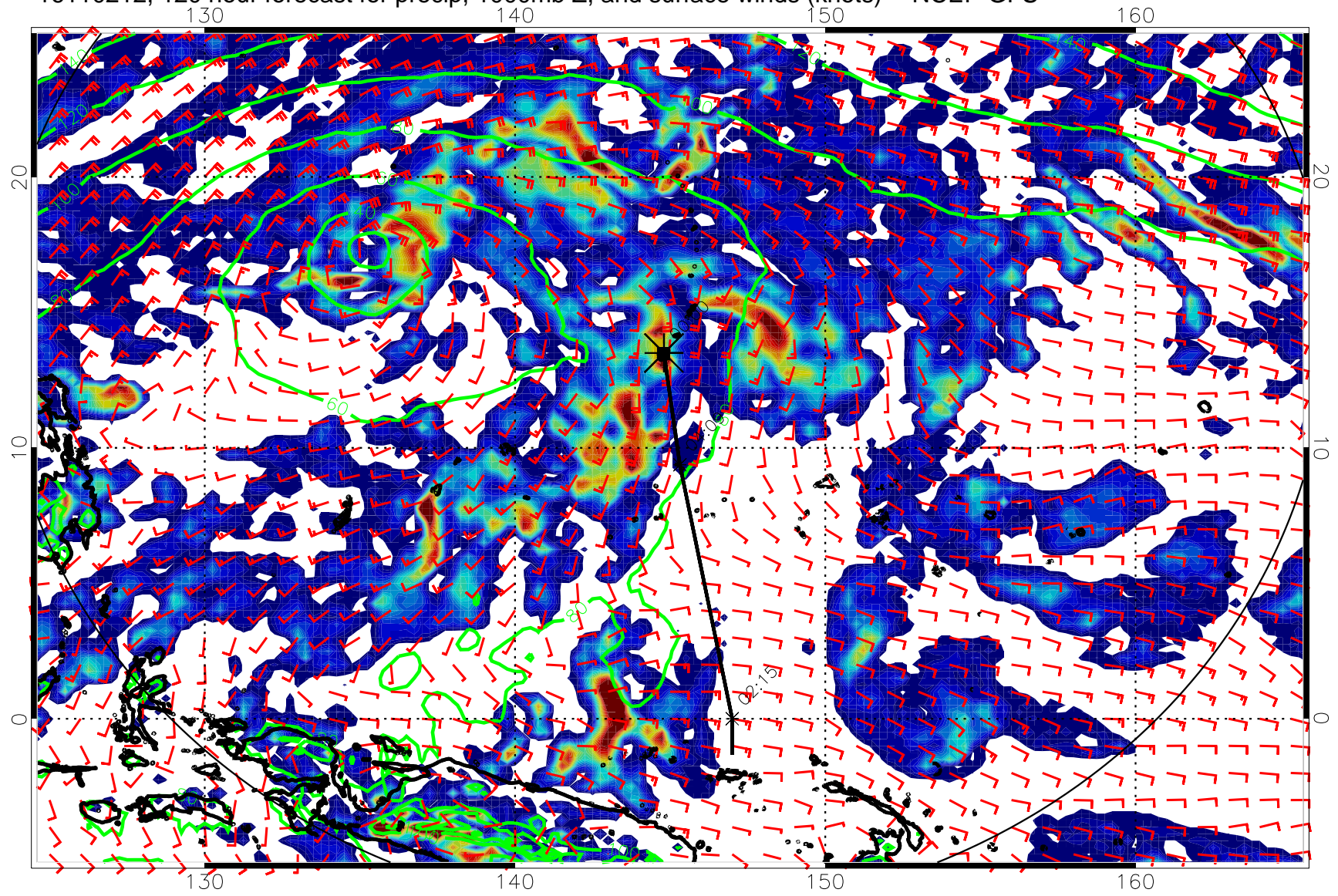
16110212, 120 hour forecast for precip, 1000mb Z, and surface winds (knots) -- NCEP GFS
