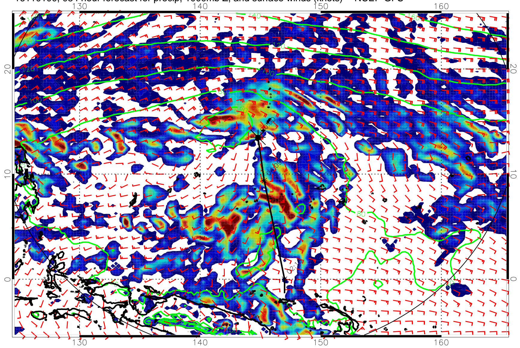
16110100, 084 hour forecast for precip, 1000mb Z, and surface winds (knots) -- NCEP GFS
