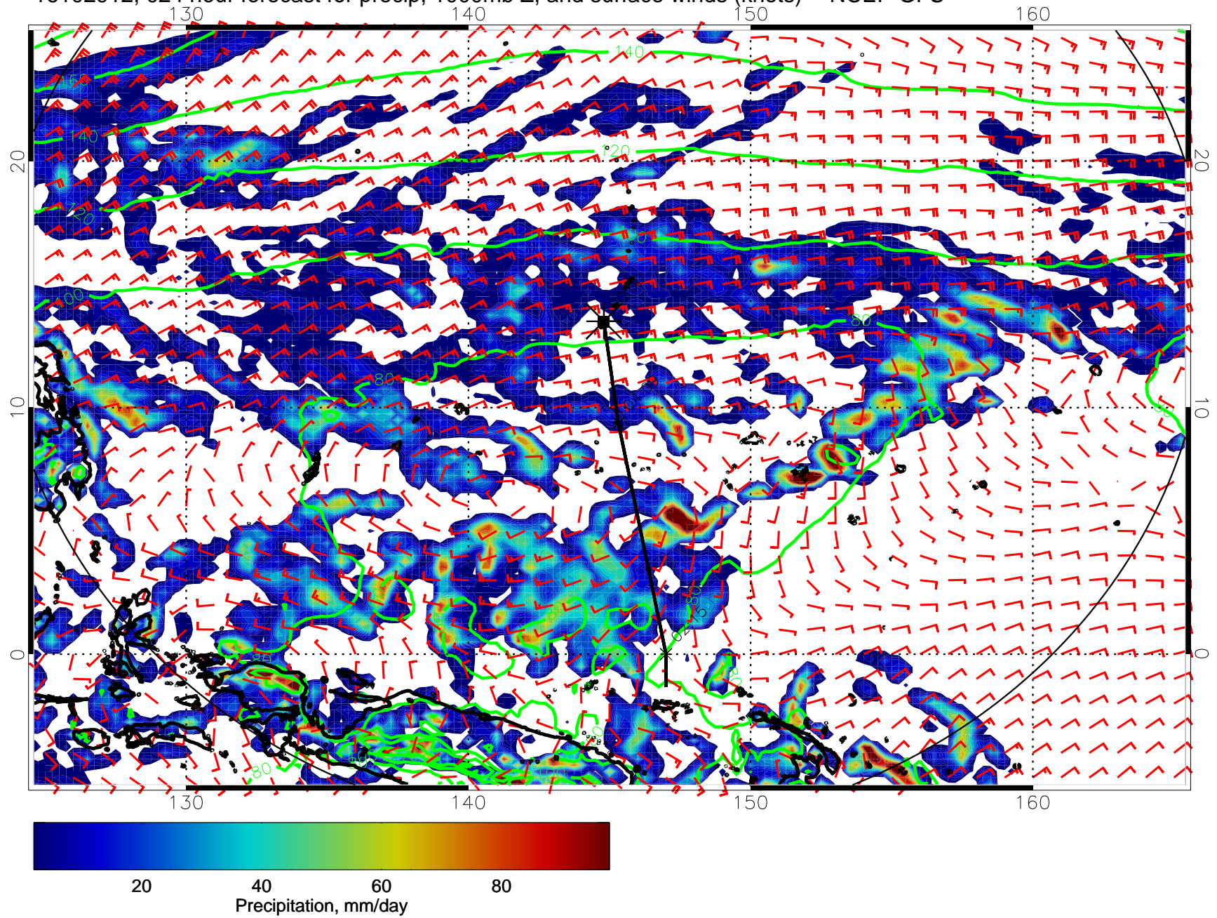
16102912, 024 hour forecast for precip, 1000mb Z, and surface winds (knots) -- NCEP GFS
