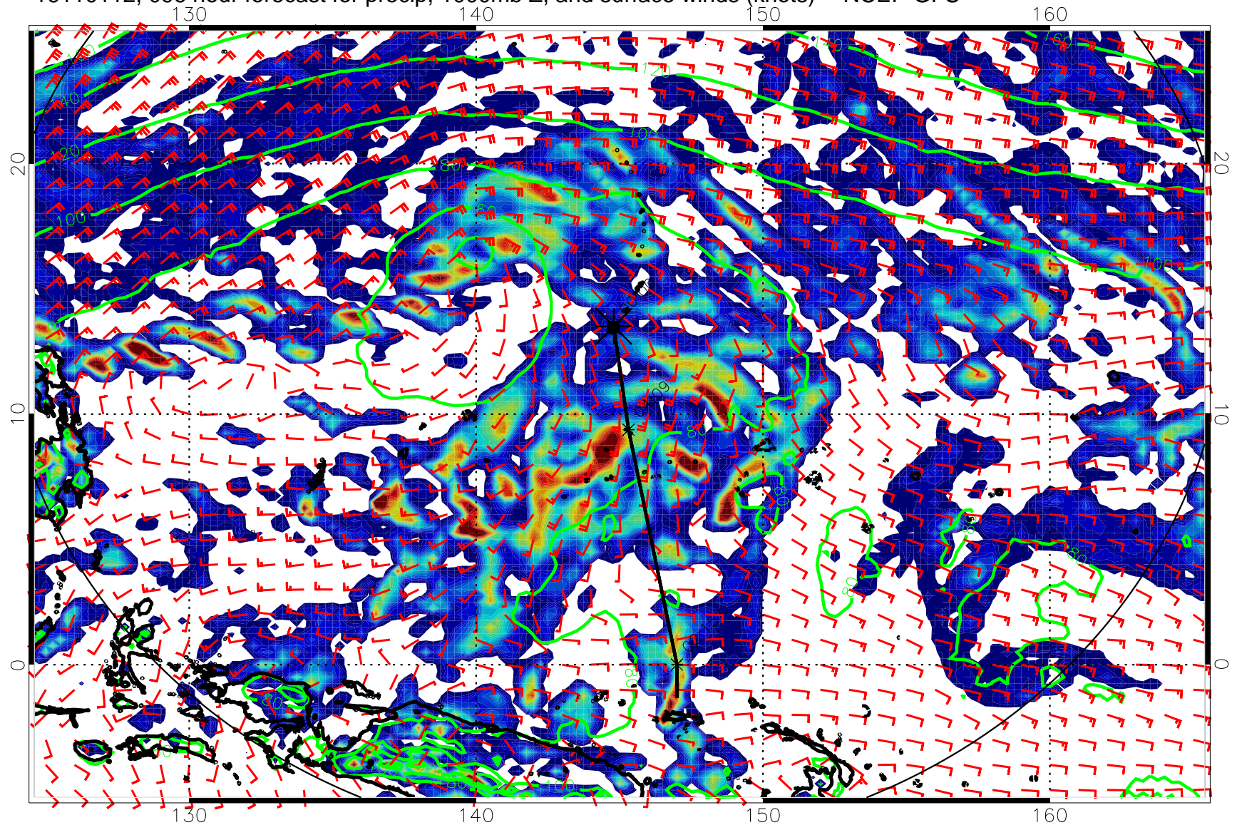
16110112, 096 hour forecast for precip, 1000mb Z, and surface winds (knots) -- NCEP GFS
