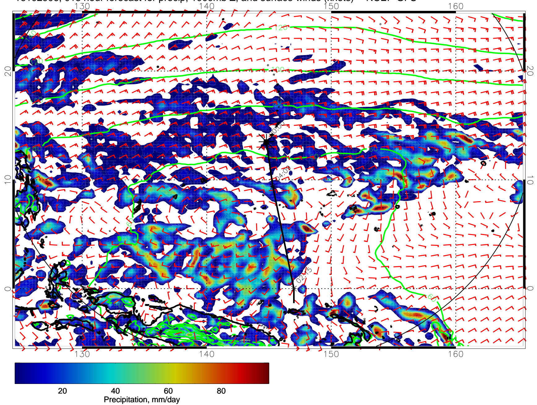
16102906, 018 hour forecast for precip, 1000mb Z, and surface winds (knots) -- NCEP GFS
