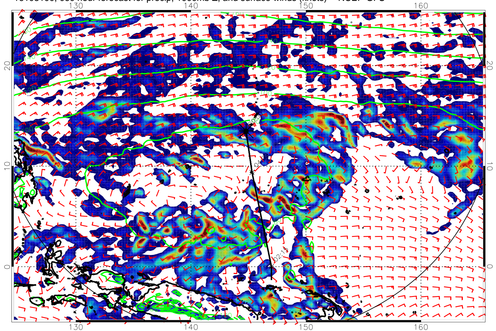
16103100, 060 hour forecast for precip, 1000mb Z, and surface winds (knots) -- NCEP GFS
