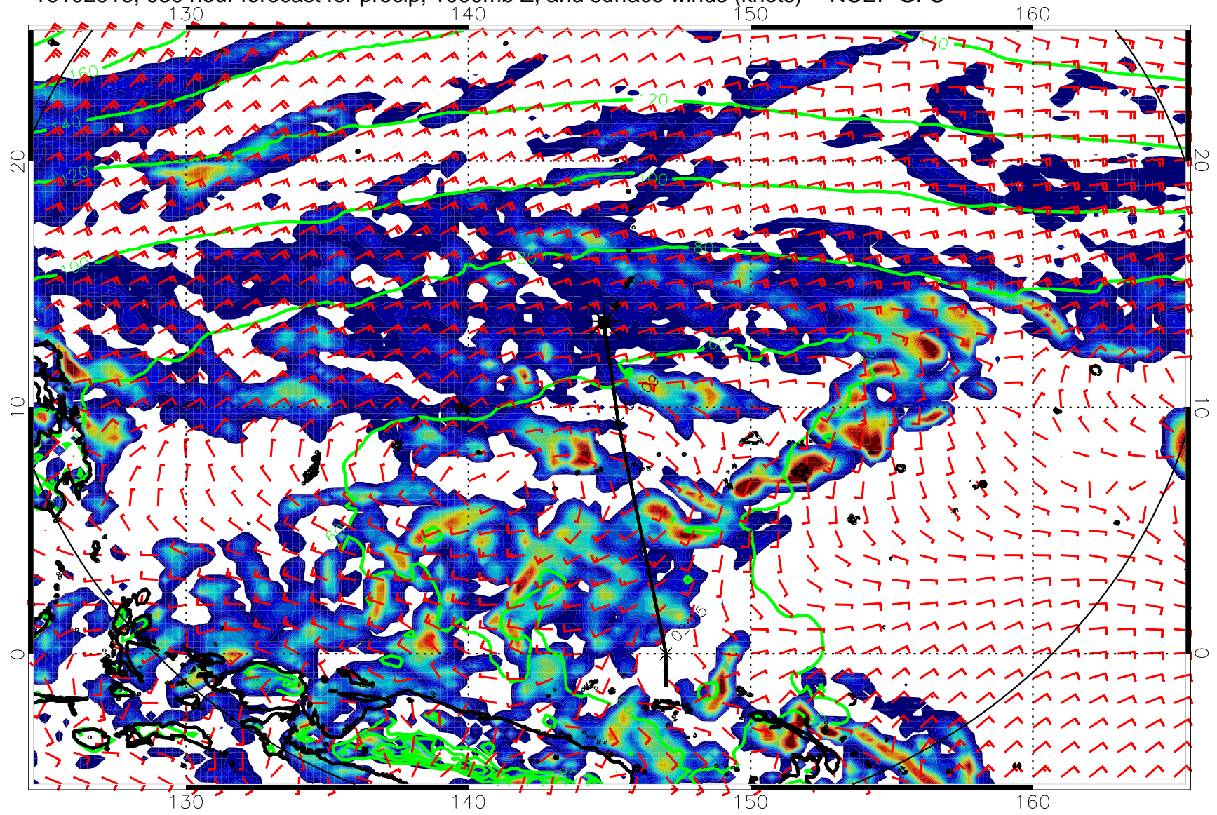
16102918, 030 hour forecast for precip, 1000mb Z, and surface winds (knots) -- NCEP GFS
