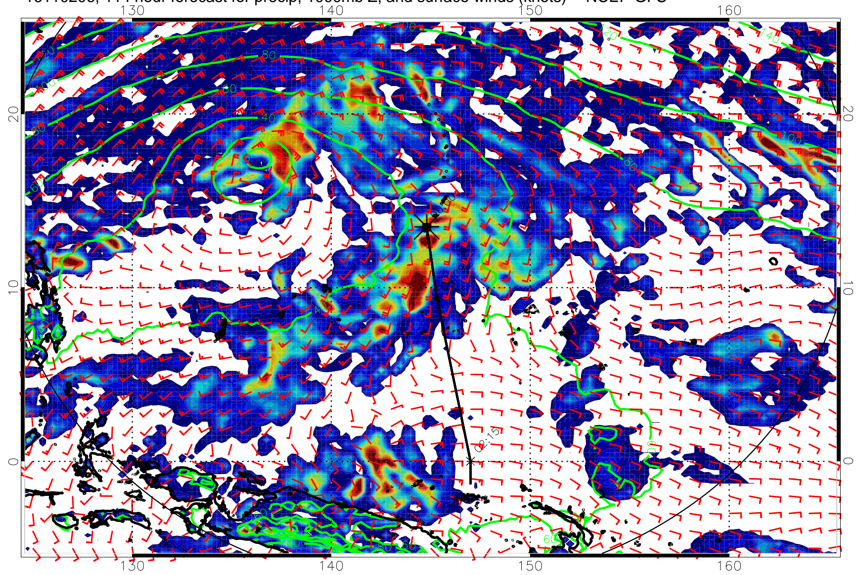
16110206, 114 hour forecast for precip, 1000mb Z, and surface winds (knots) -- NCEP GFS
