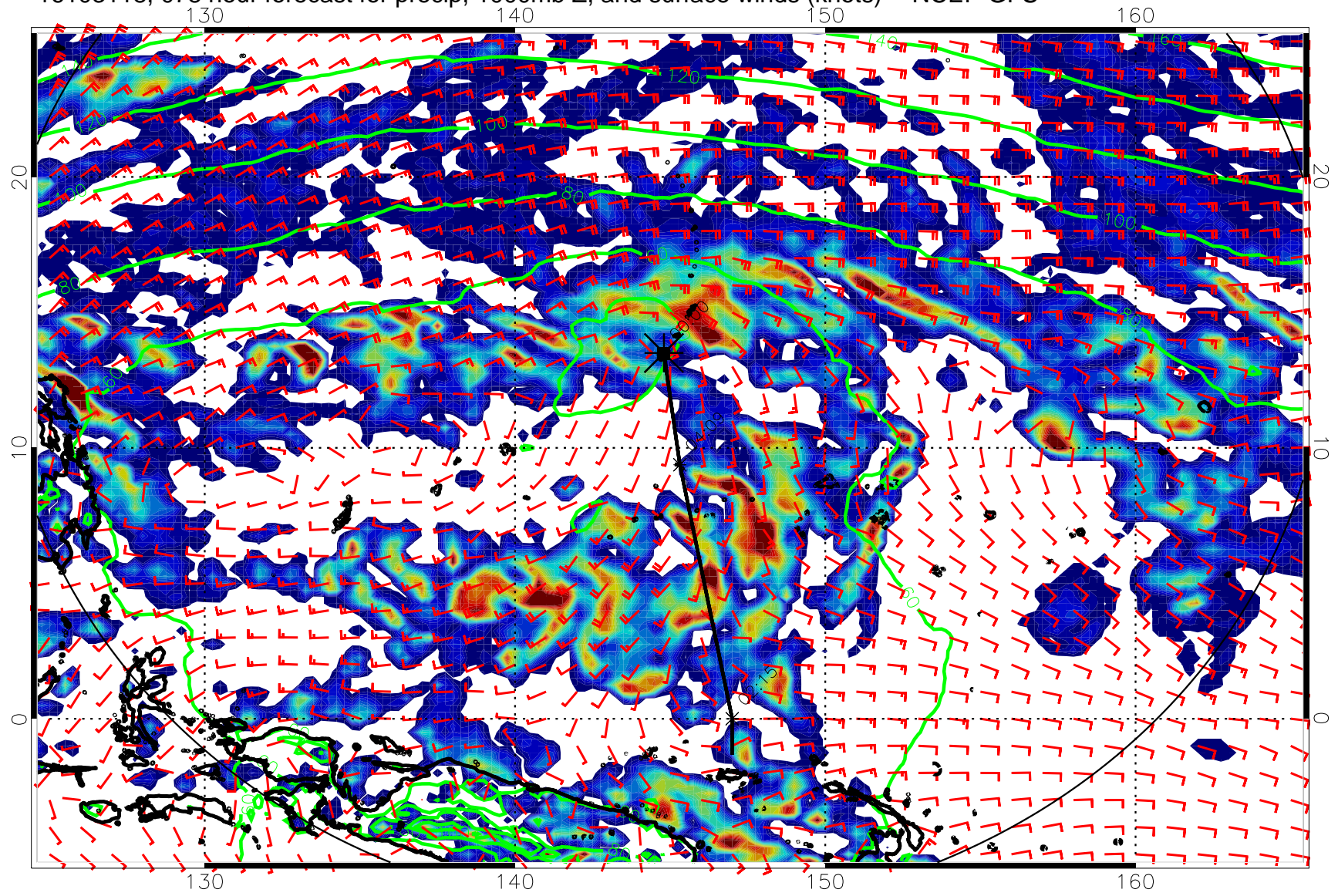
16103118, 078 hour forecast for precip, 1000mb Z, and surface winds (knots) -- NCEP GFS
