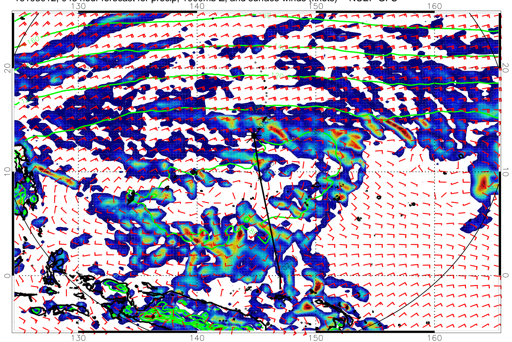
16103012, 048 hour forecast for precip, 1000mb Z, and surface winds (knots) -- NCEP GFS
