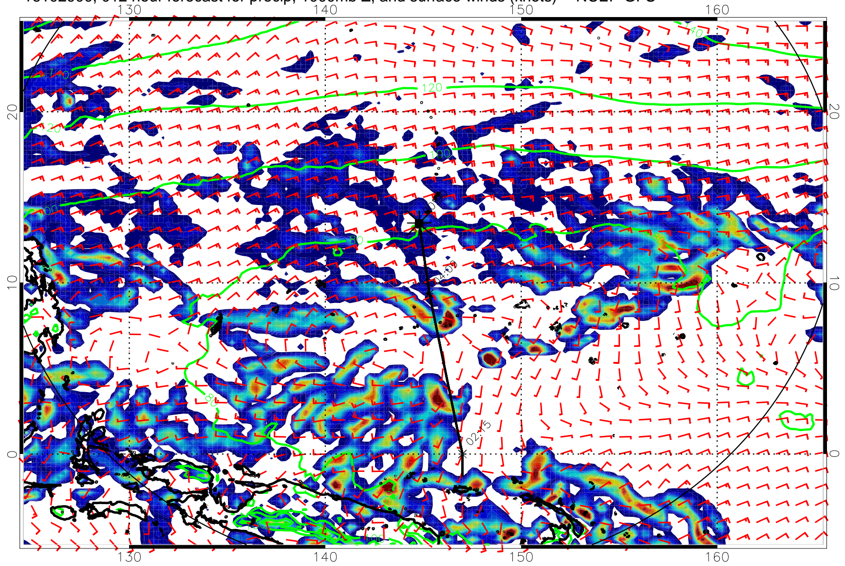
16102900, 012 hour forecast for precip, 1000mb Z, and surface winds (knots) -- NCEP GFS
