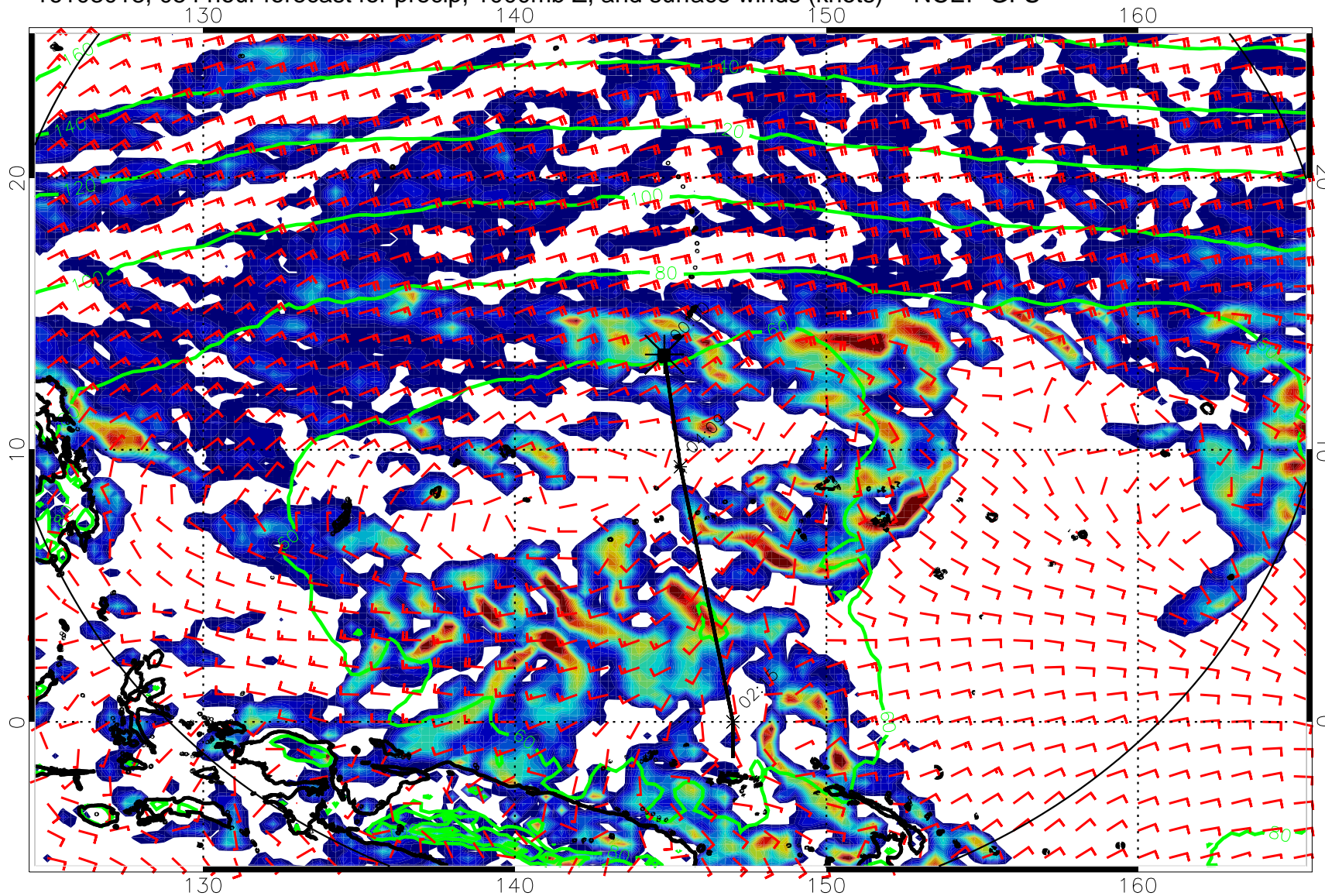
16103018, 054 hour forecast for precip, 1000mb Z, and surface winds (knots) -- NCEP GFS
