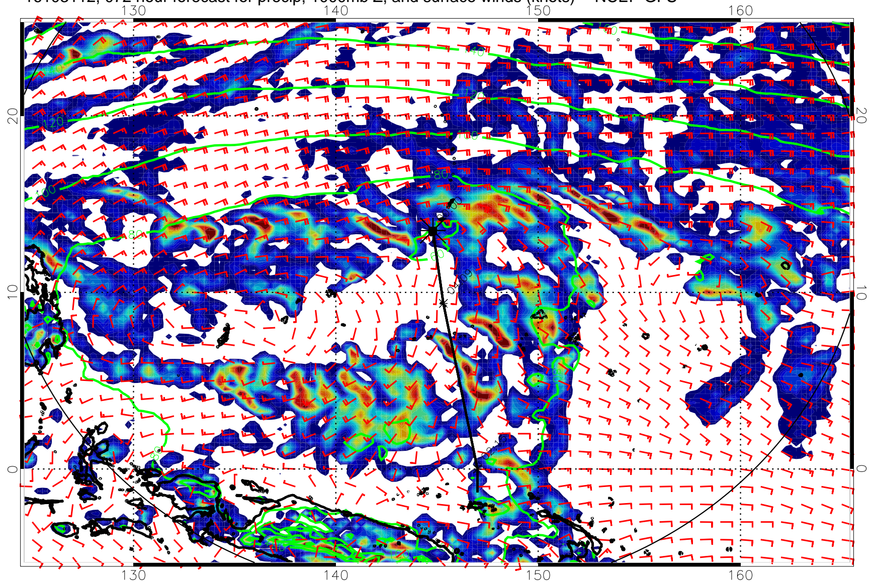
16103112, 072 hour forecast for precip, 1000mb Z, and surface winds (knots) -- NCEP GFS
