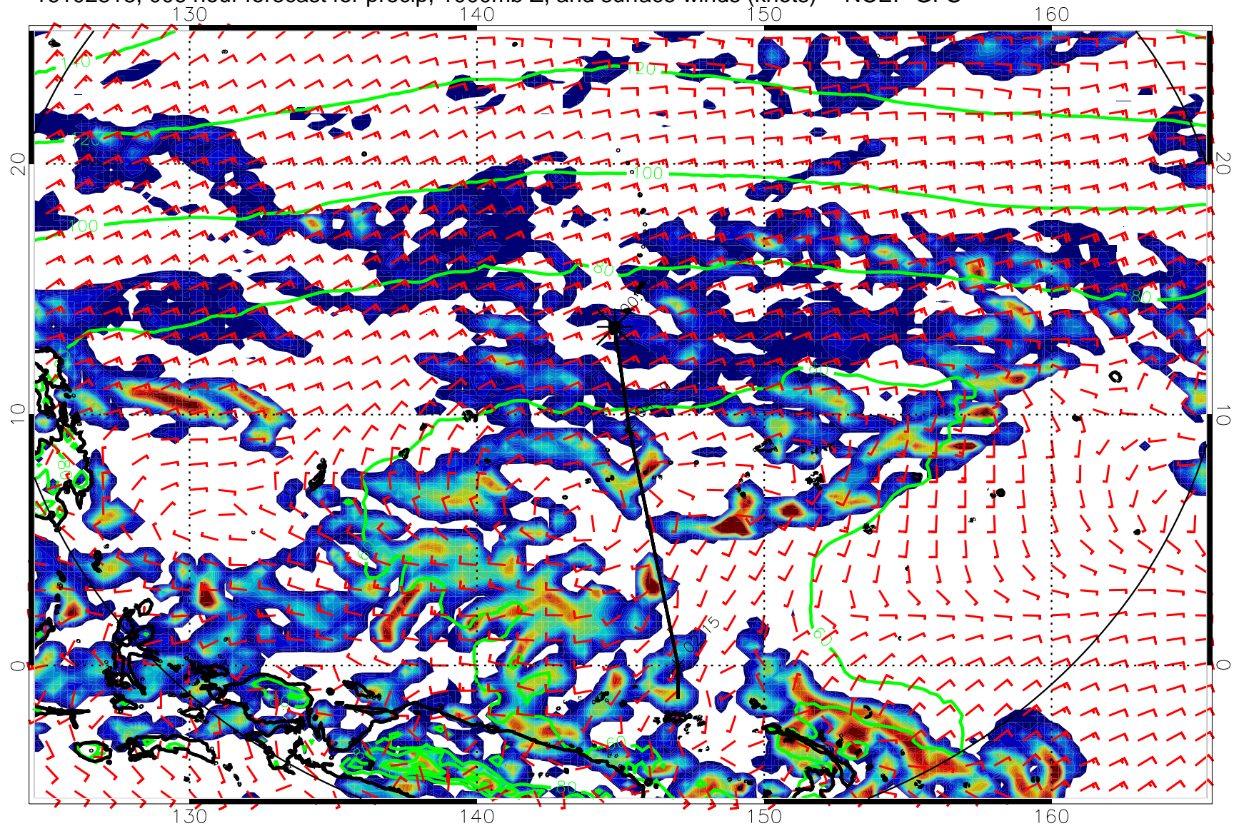
16102818, 006 hour forecast for precip, 1000mb Z, and surface winds (knots) -- NCEP GFS
