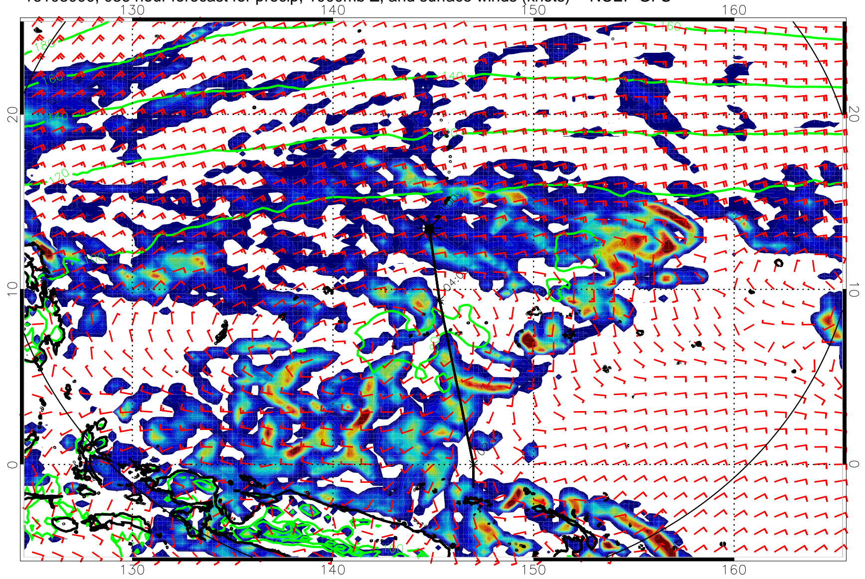
16103000, 036 hour forecast for precip, 1000mb Z, and surface winds (knots) -- NCEP GFS
