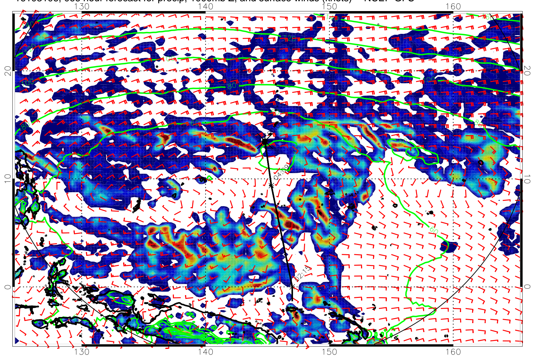
16103106, 066 hour forecast for precip, 1000mb Z, and surface winds (knots) -- NCEP GFS
