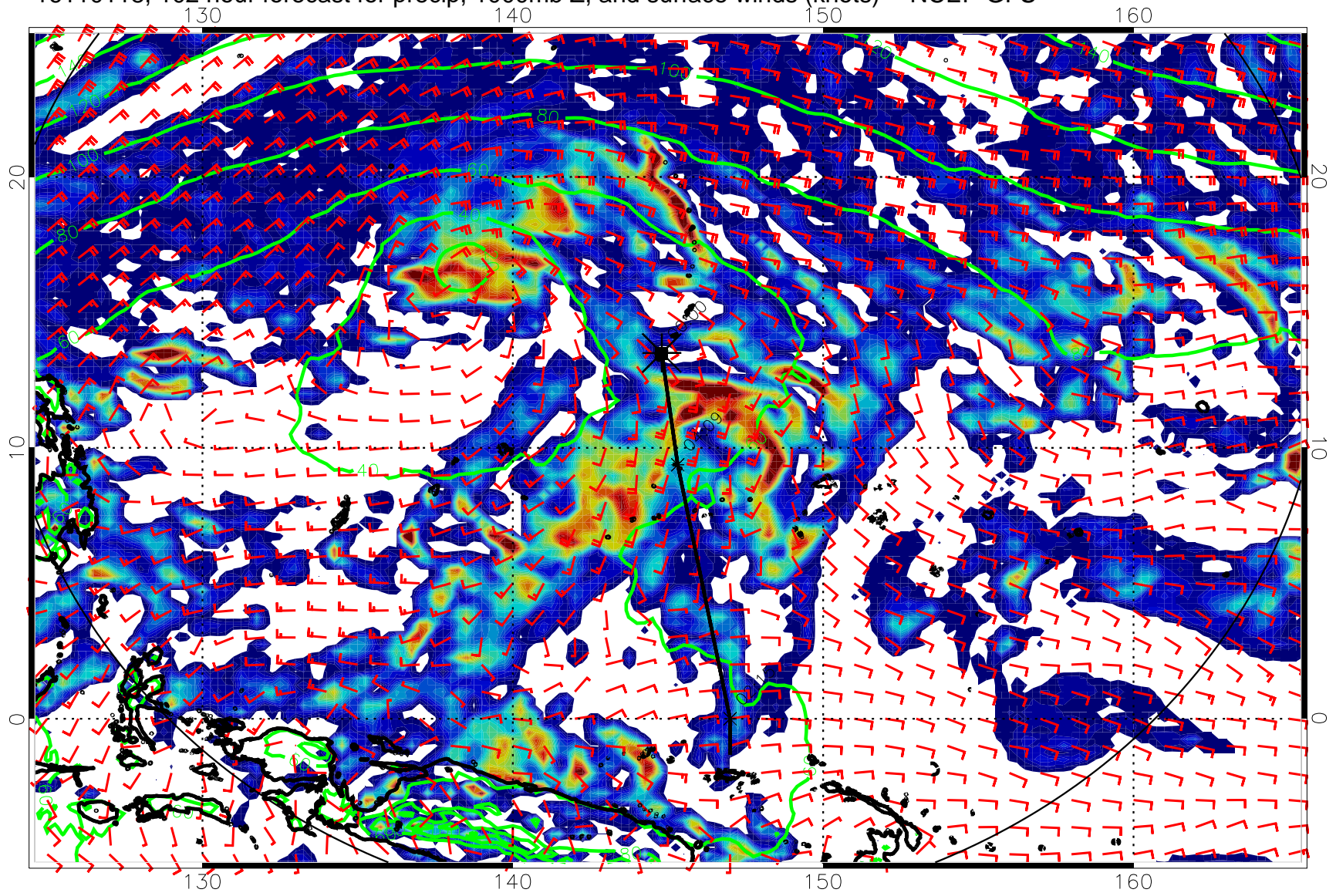
16110118, 102 hour forecast for precip, 1000mb Z, and surface winds (knots) -- NCEP GFS
