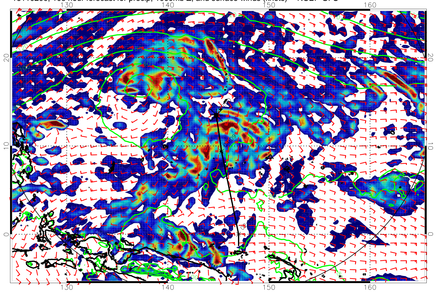
16110200, 108 hour forecast for precip, 1000mb Z, and surface winds (knots) -- NCEP GFS
