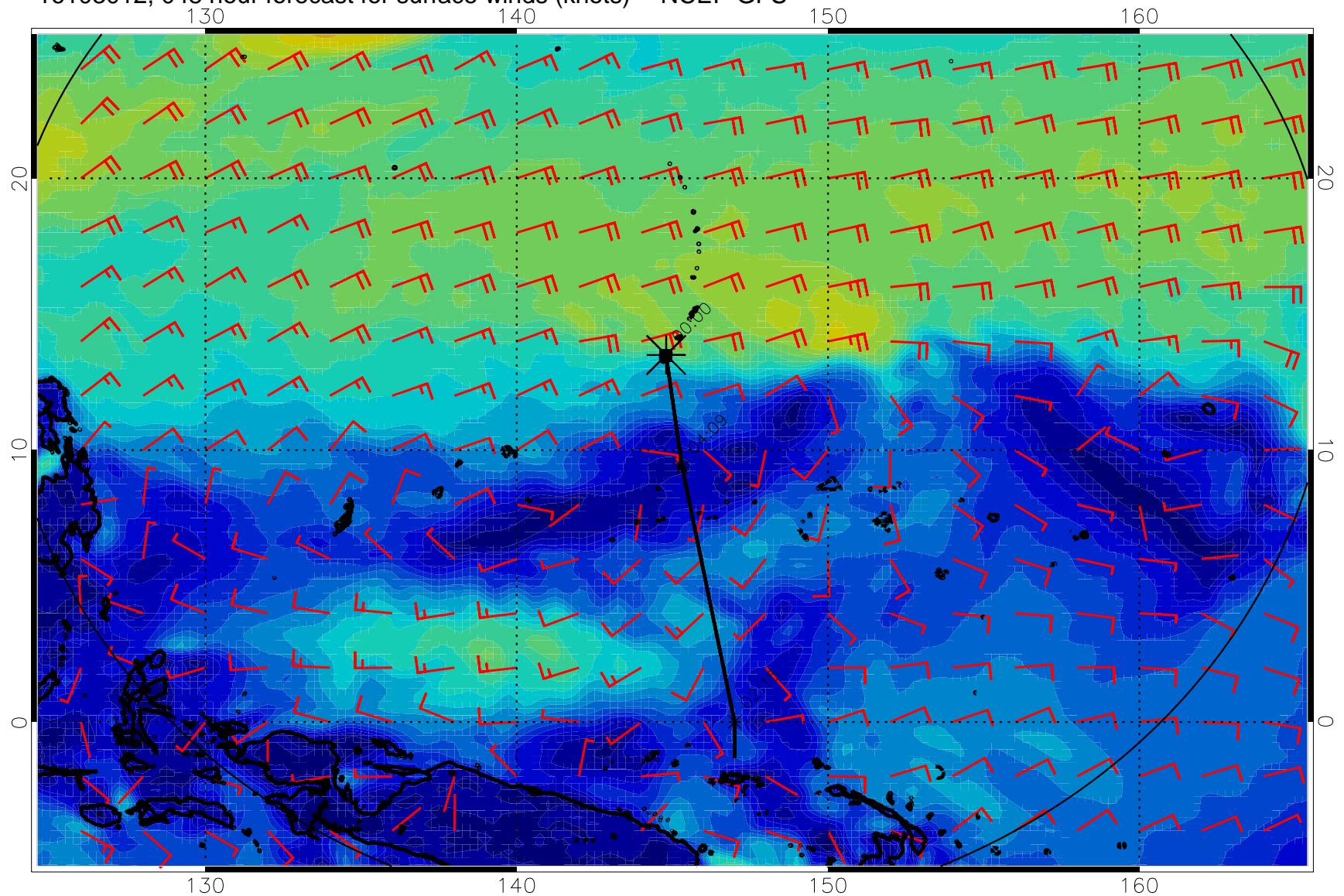
16103012, 048 hour forecast for surface winds (knots) -- NCEP GFS
