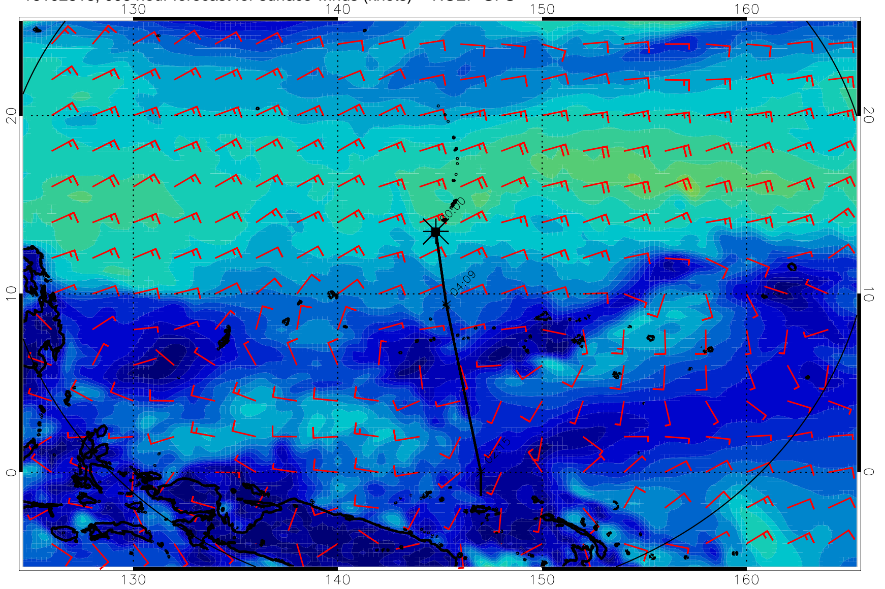
16102818, 006 hour forecast for surface winds (knots) -- NCEP GFS
