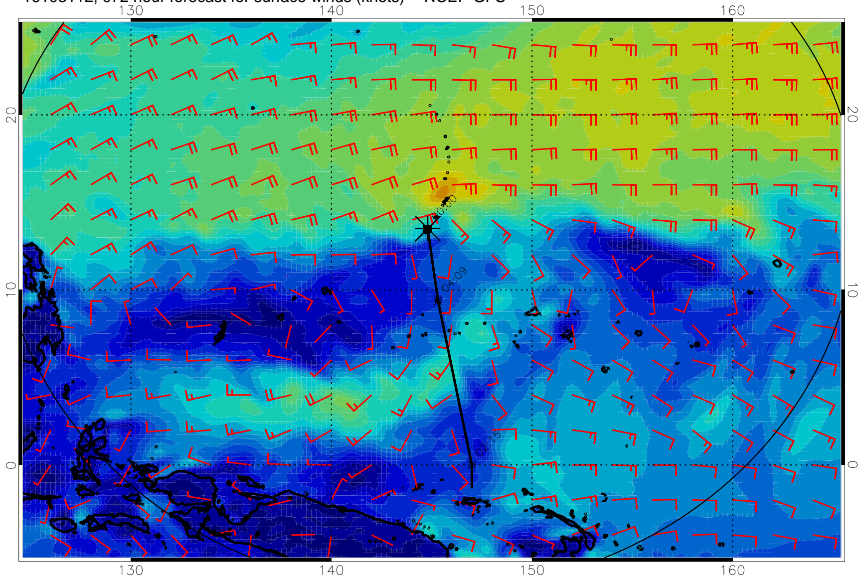
16103112, 072 hour forecast for surface winds (knots) -- NCEP GFS
