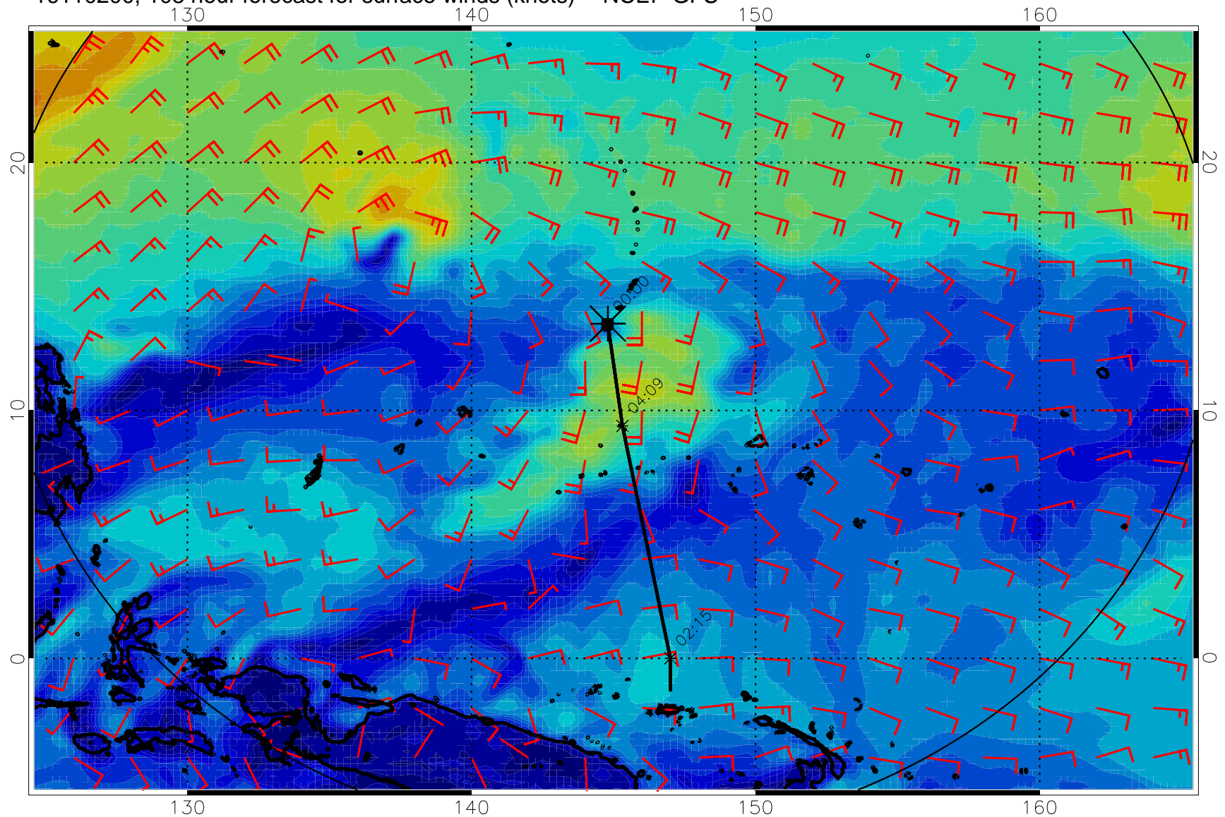
16110200, 108 hour forecast for surface winds (knots) -- NCEP GFS
