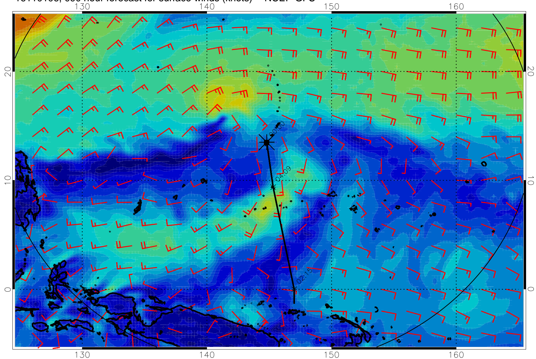
16110106, 090 hour forecast for surface winds (knots) -- NCEP GFS
