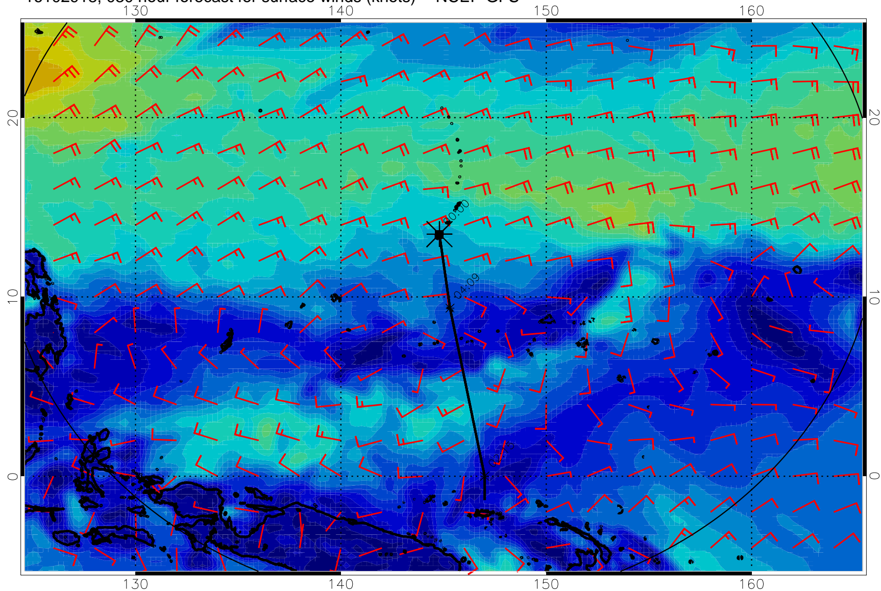
16102918, 030 hour forecast for surface winds (knots) -- NCEP GFS
