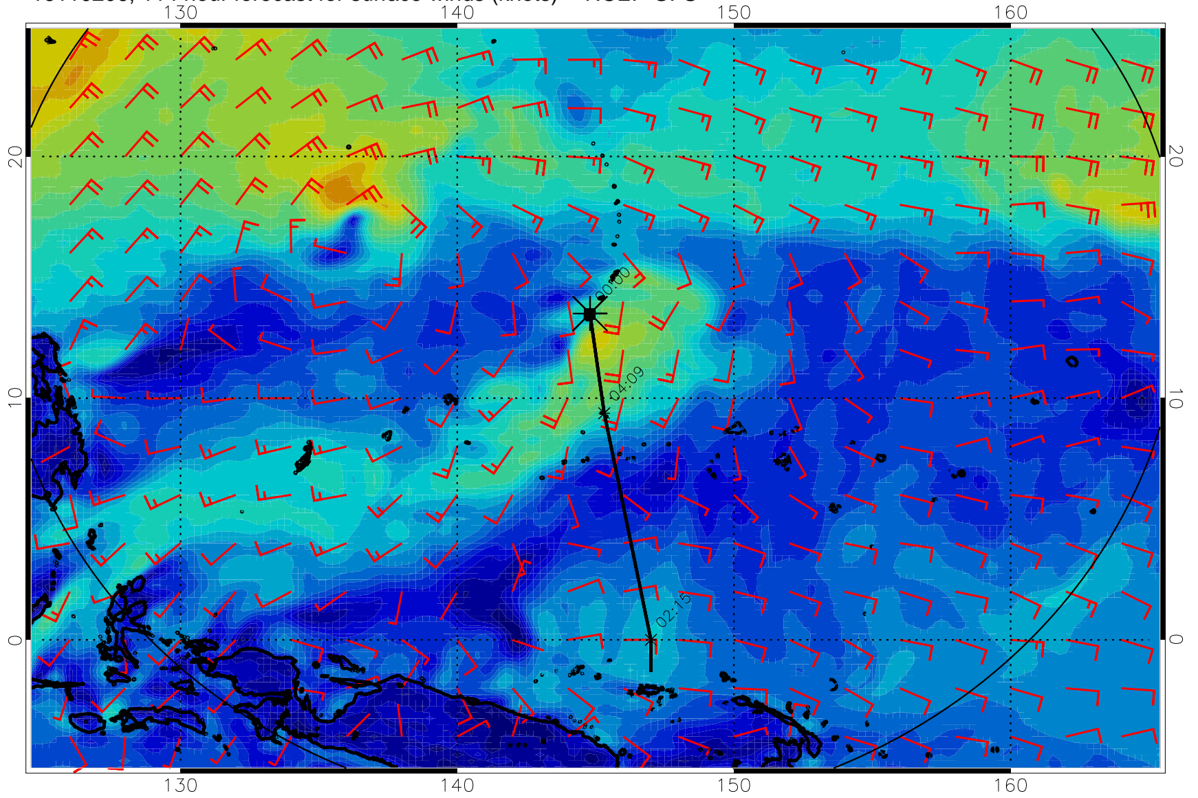
16110206, 114 hour forecast for surface winds (knots) -- NCEP GFS
