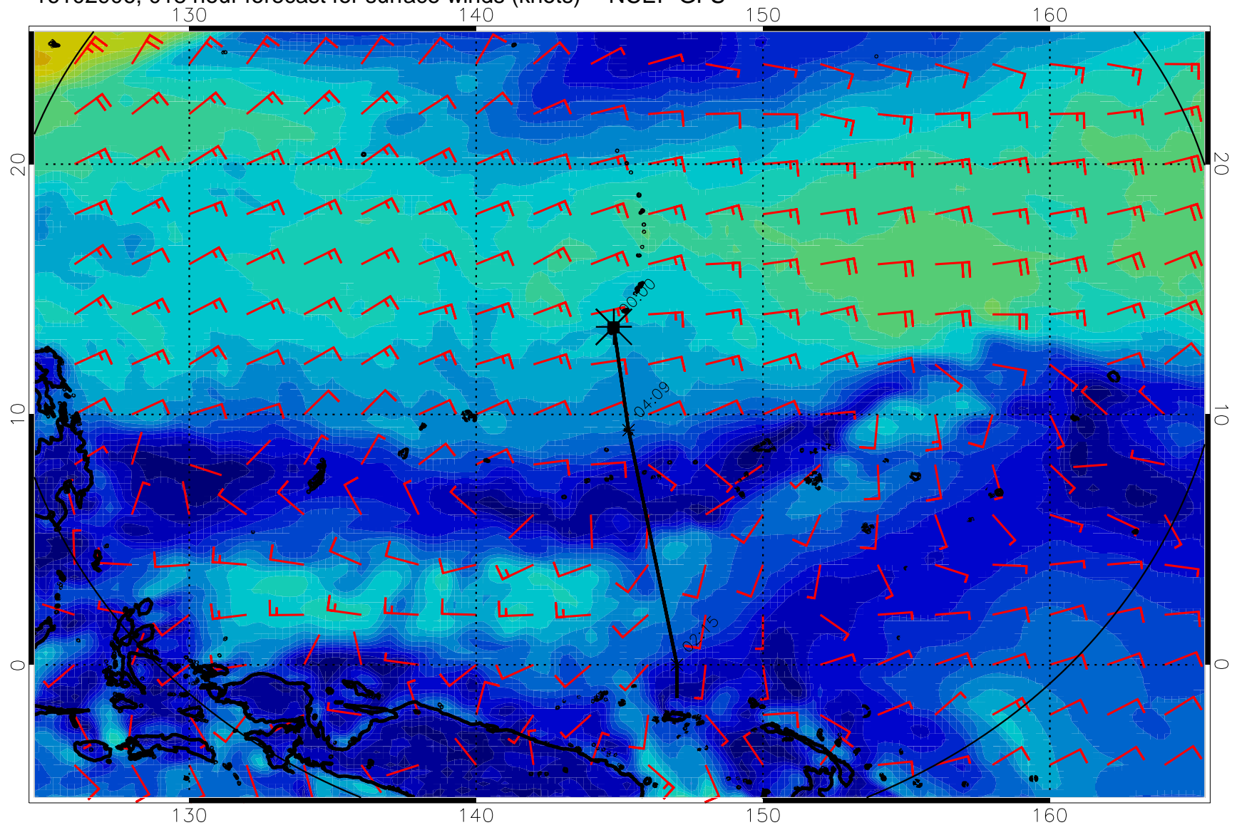
16102906, 018 hour forecast for surface winds (knots) -- NCEP GFS
