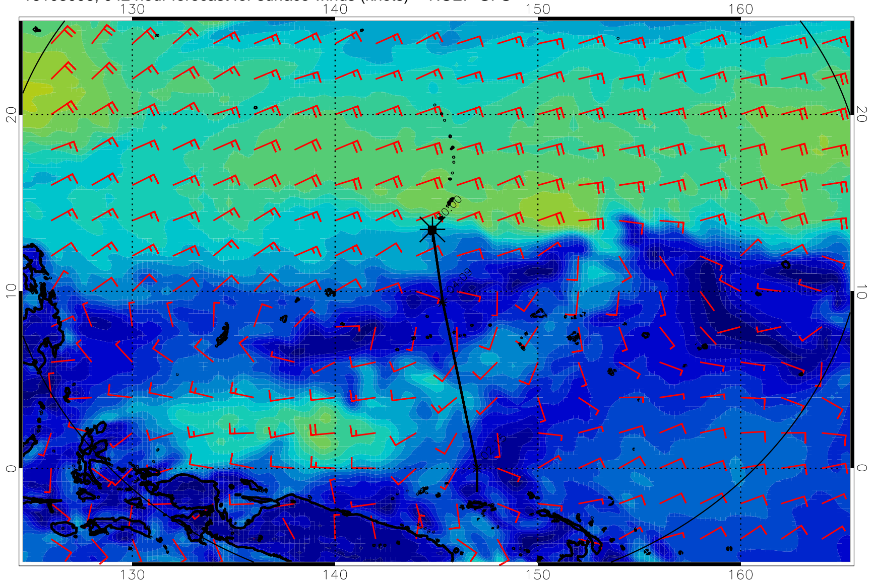
16103006, 042 hour forecast for surface winds (knots) -- NCEP GFS
