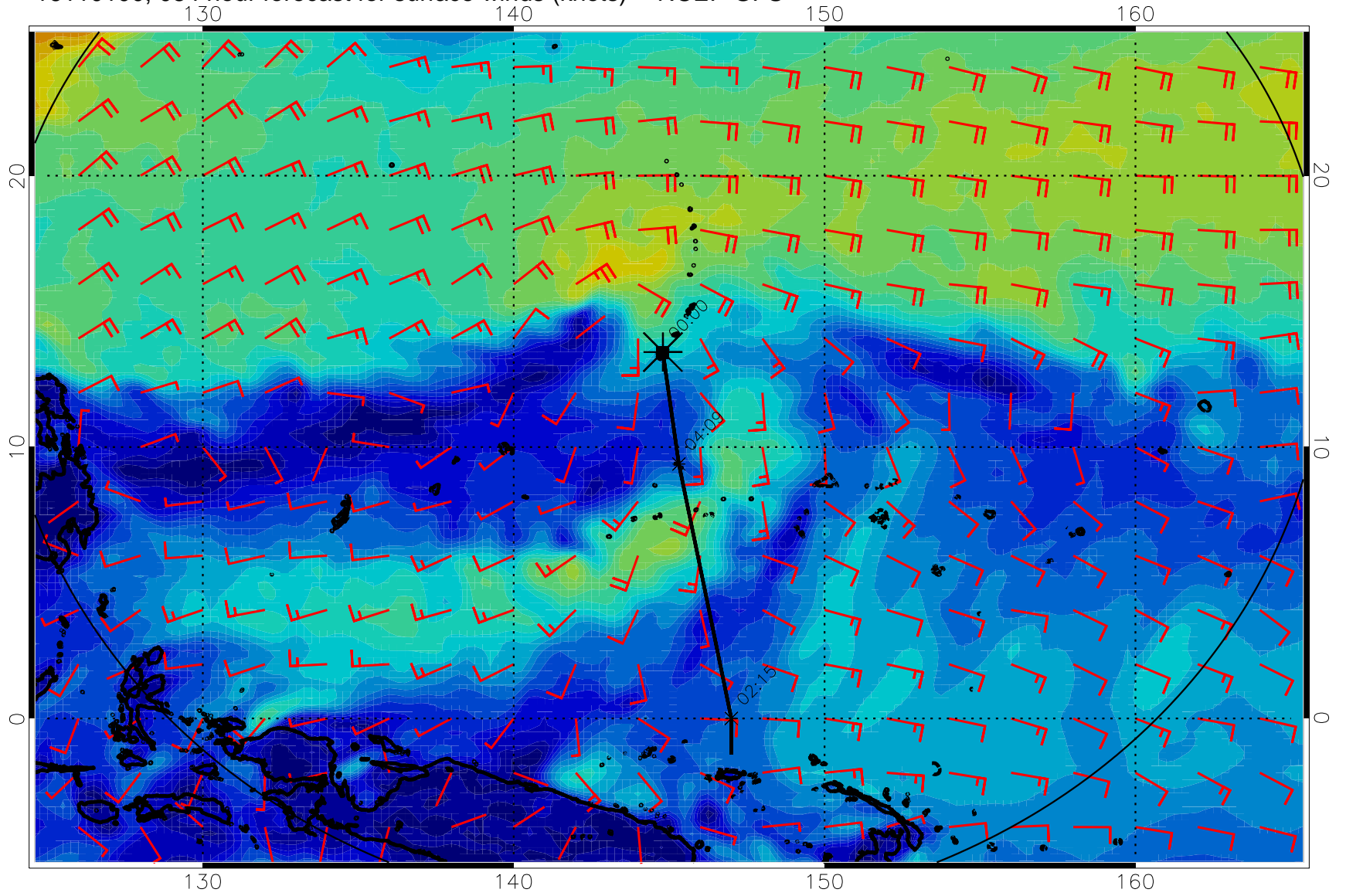
16110100, 084 hour forecast for surface winds (knots) -- NCEP GFS
