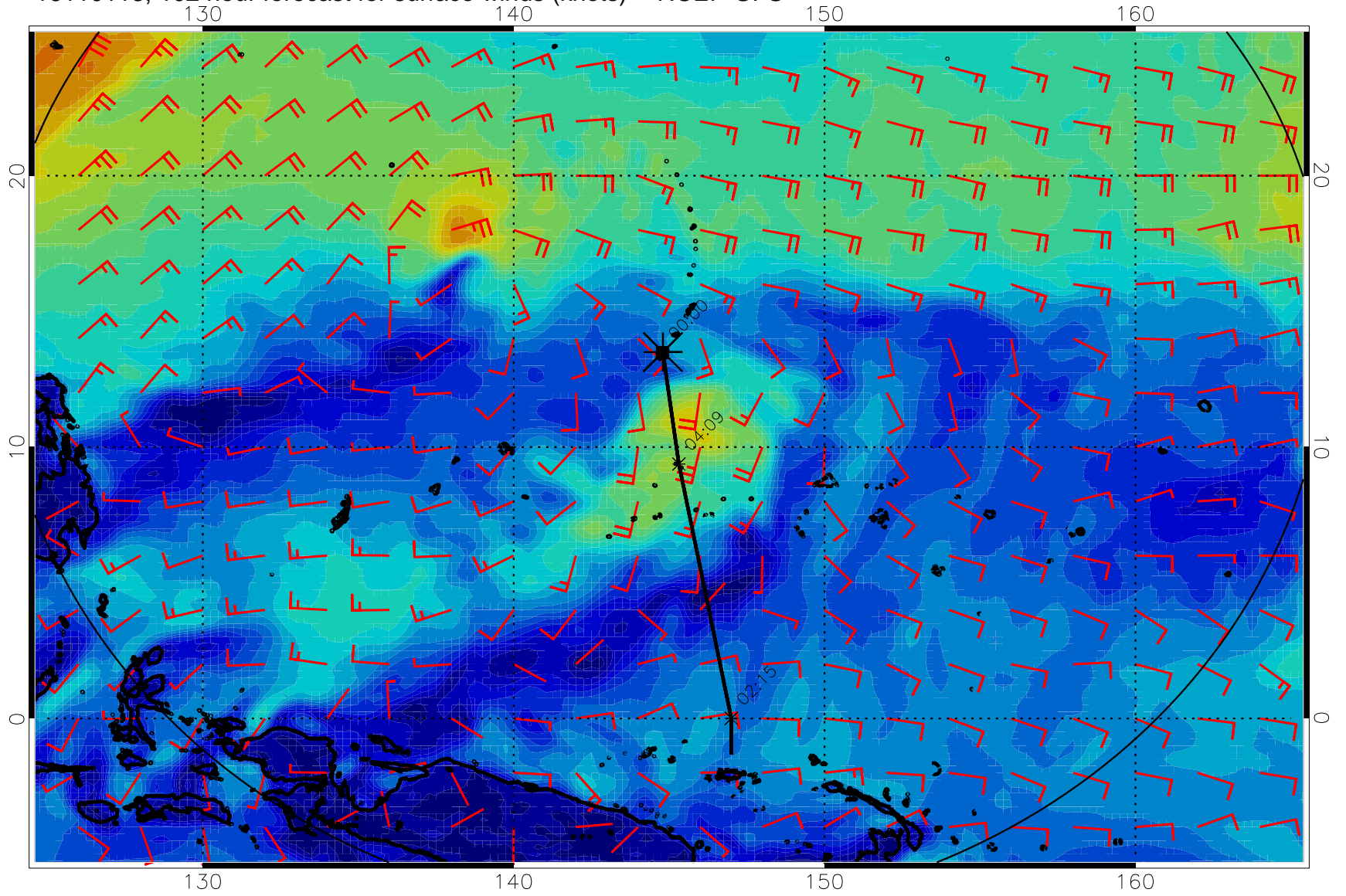
16110118, 102 hour forecast for surface winds (knots) -- NCEP GFS
