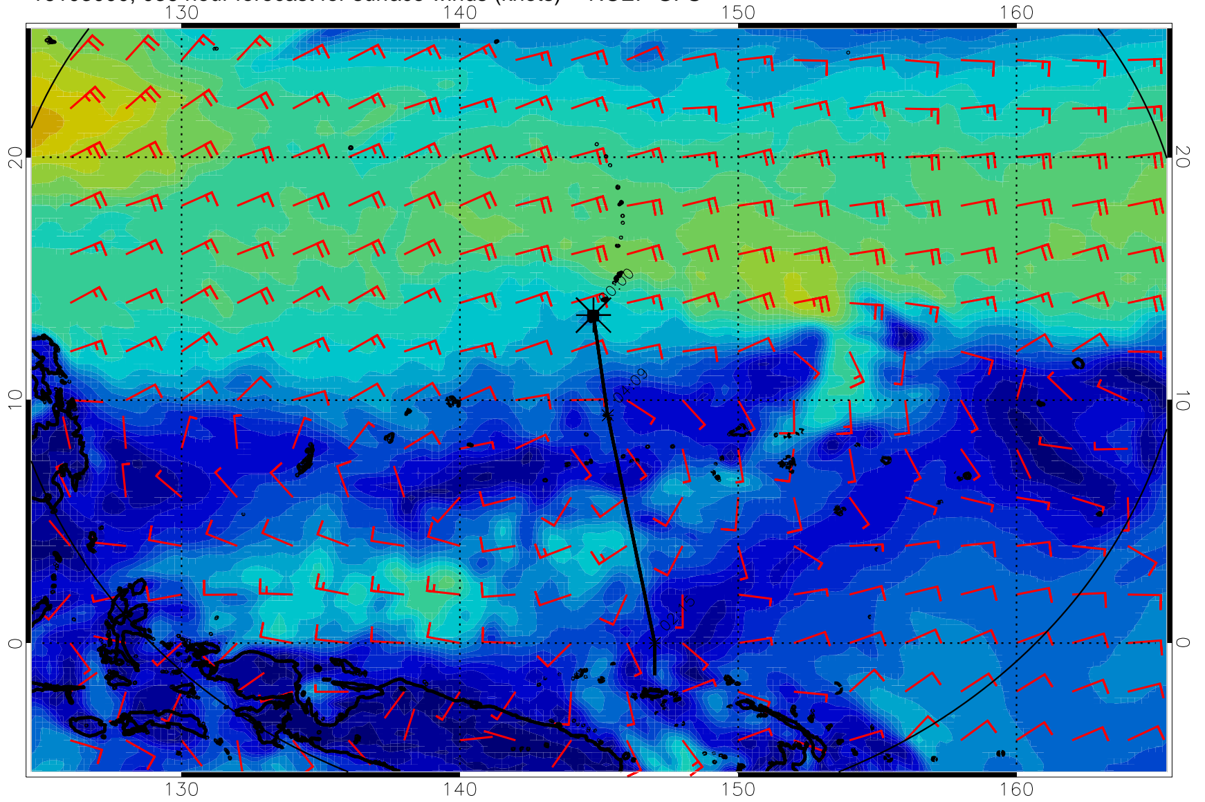
16103000, 036 hour forecast for surface winds (knots) -- NCEP GFS
