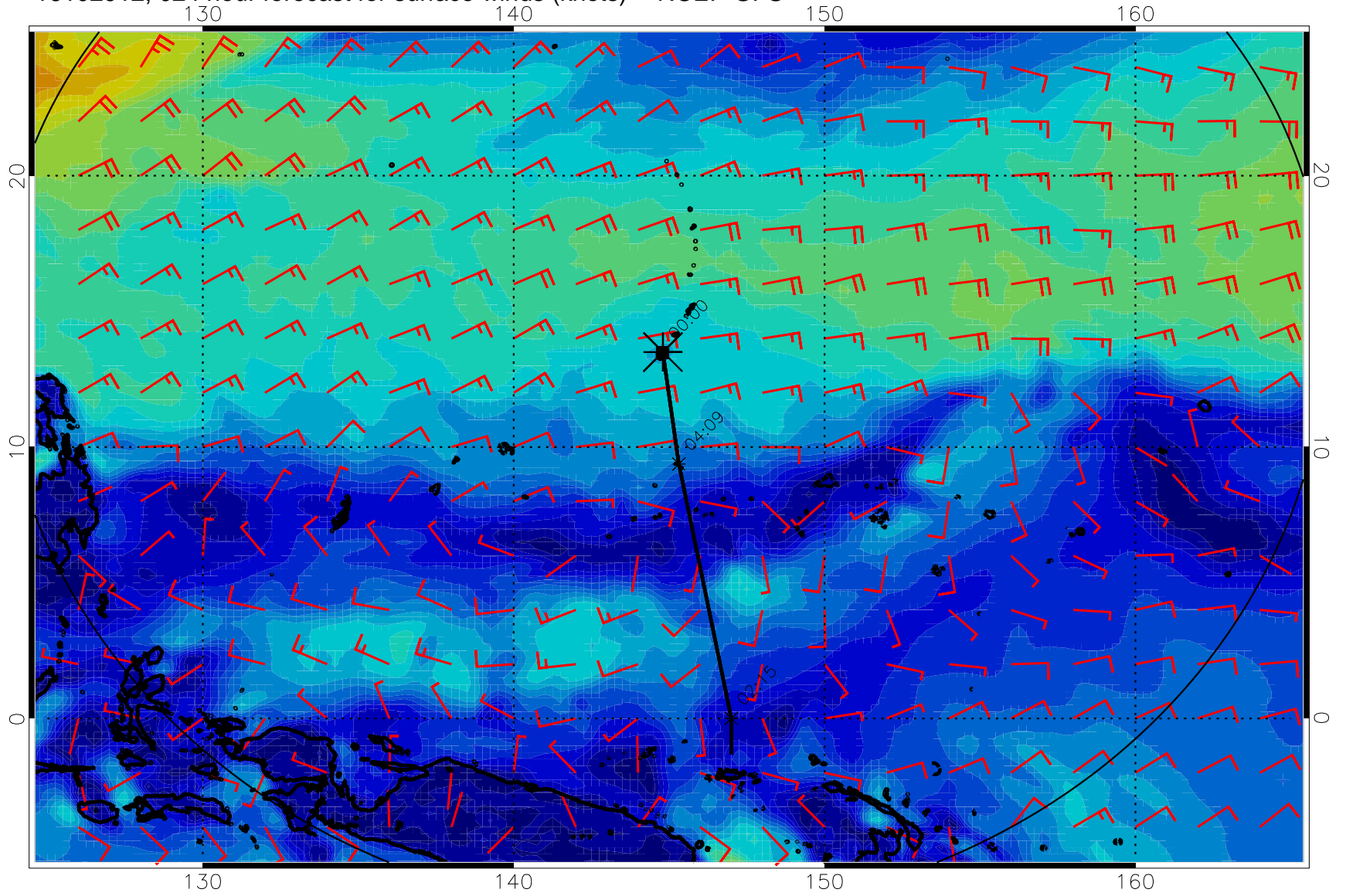
16102912, 024 hour forecast for surface winds (knots) -- NCEP GFS
