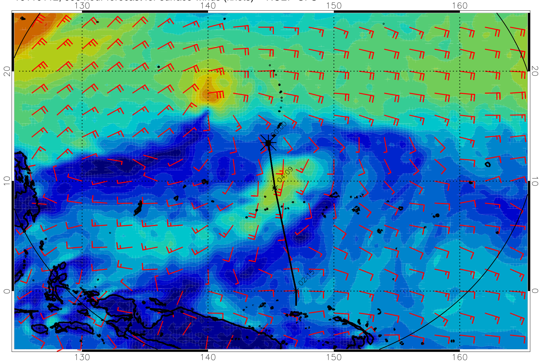
16110112, 096 hour forecast for surface winds (knots) -- NCEP GFS
