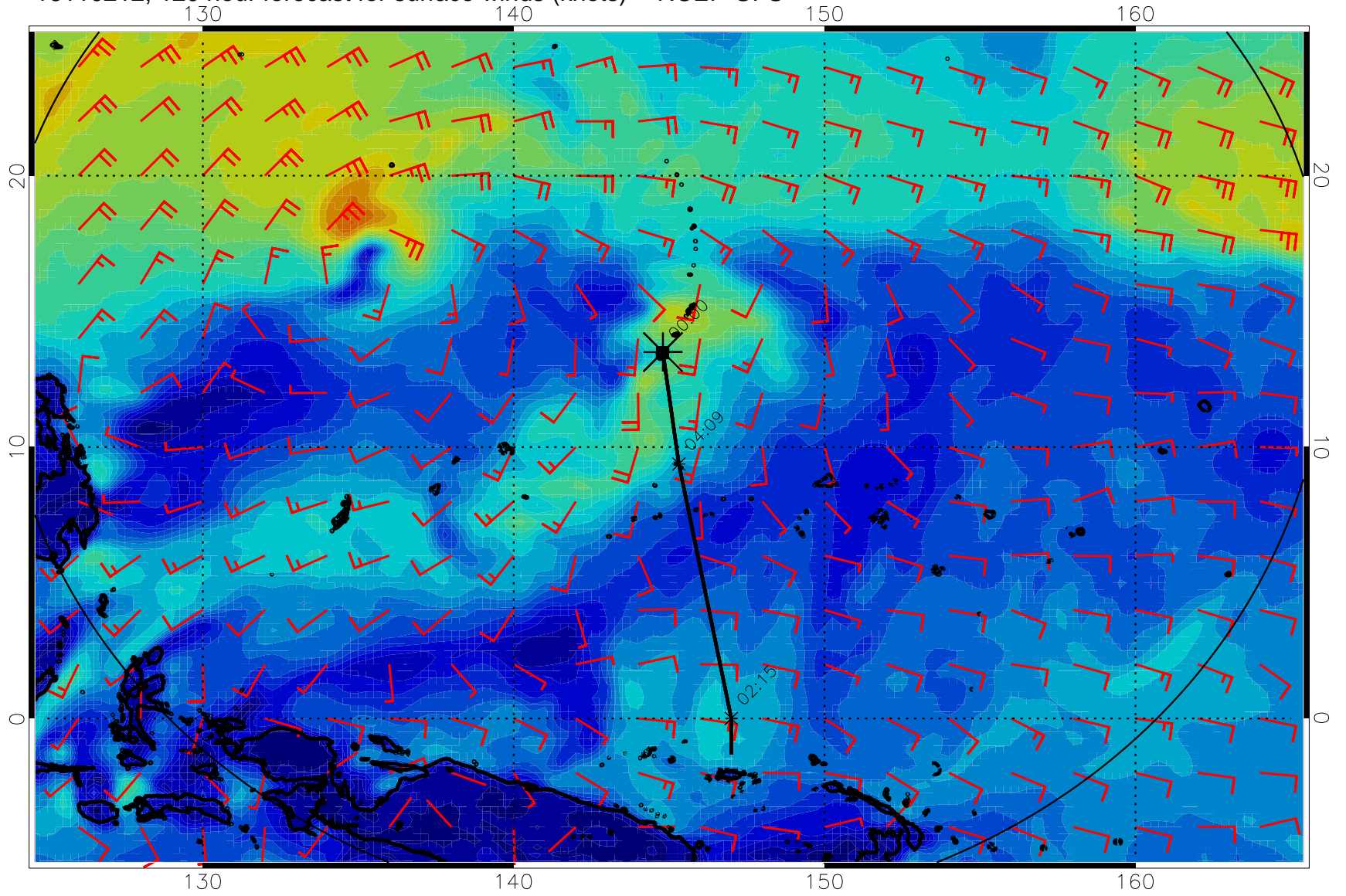
16110212, 120 hour forecast for surface winds (knots) -- NCEP GFS
