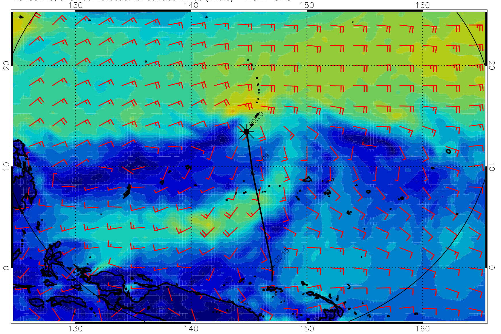
16103118, 078 hour forecast for surface winds (knots) -- NCEP GFS
