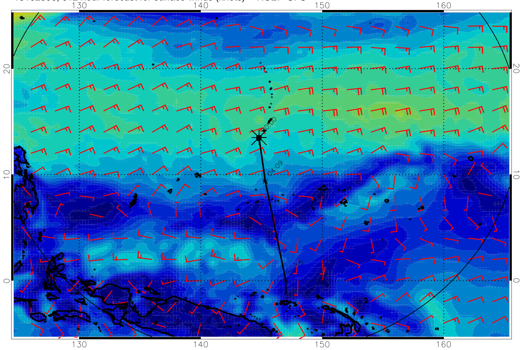
16102900, 012 hour forecast for surface winds (knots) -- NCEP GFS
