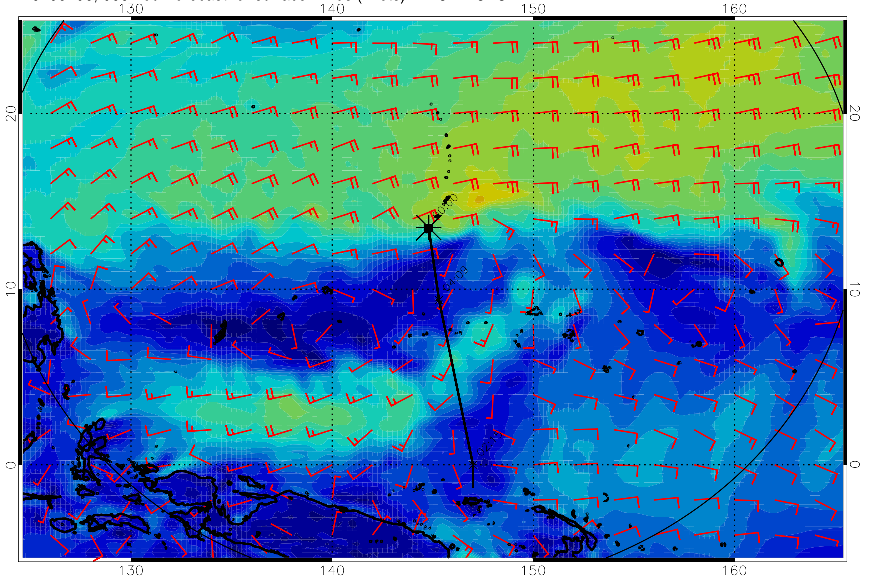
16103106, 066 hour forecast for surface winds (knots) -- NCEP GFS
