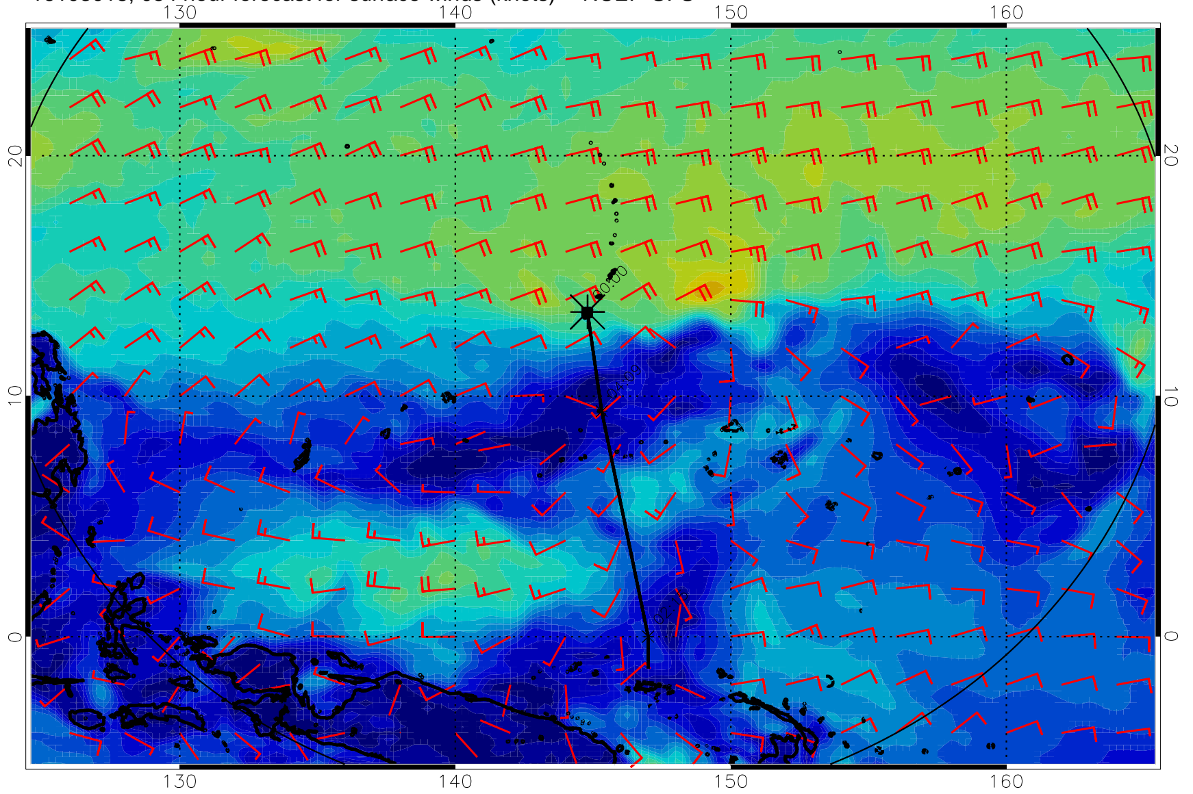
16103018, 054 hour forecast for surface winds (knots) -- NCEP GFS
