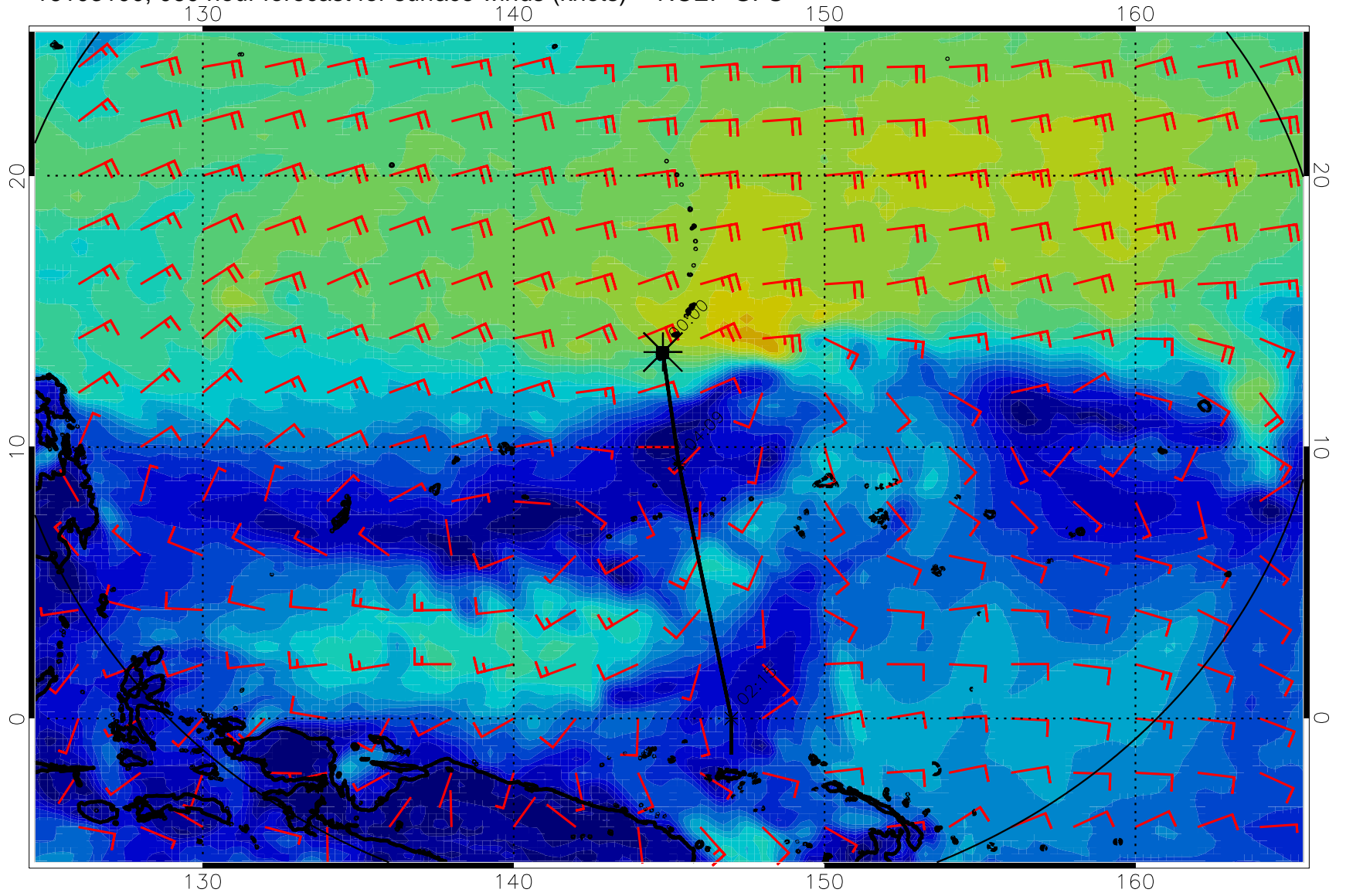
16103100, 060 hour forecast for surface winds (knots) -- NCEP GFS
