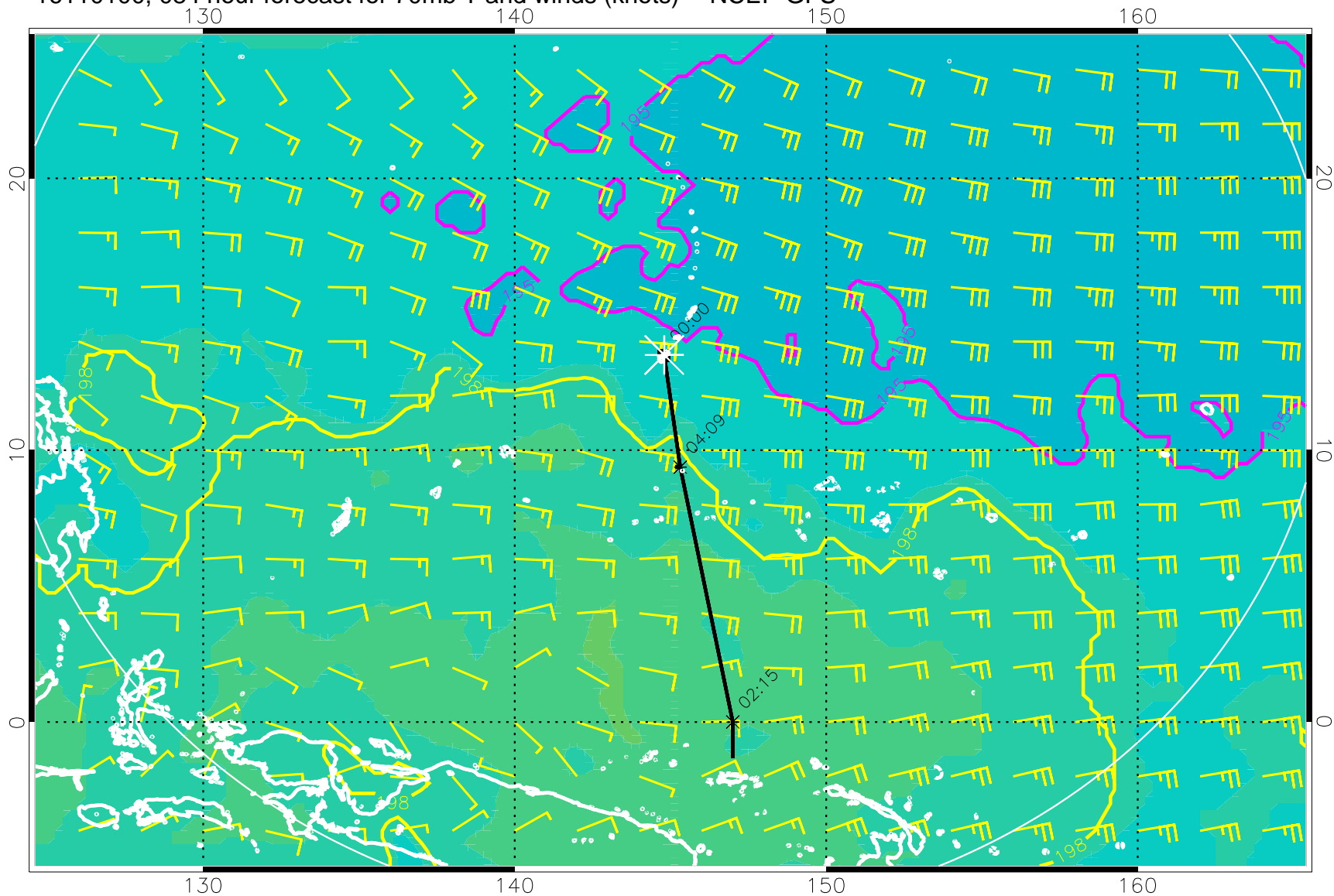
16110100, 084 hour forecast for 70mb T and winds (knots) -- NCEP GFS
