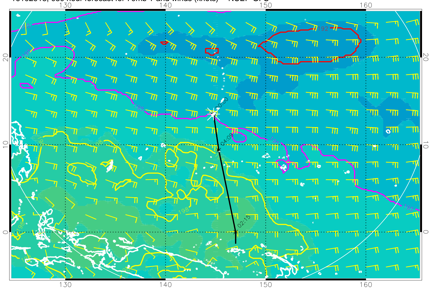
16102918, 030 hour forecast for 70mb T and winds (knots) -- NCEP GFS
