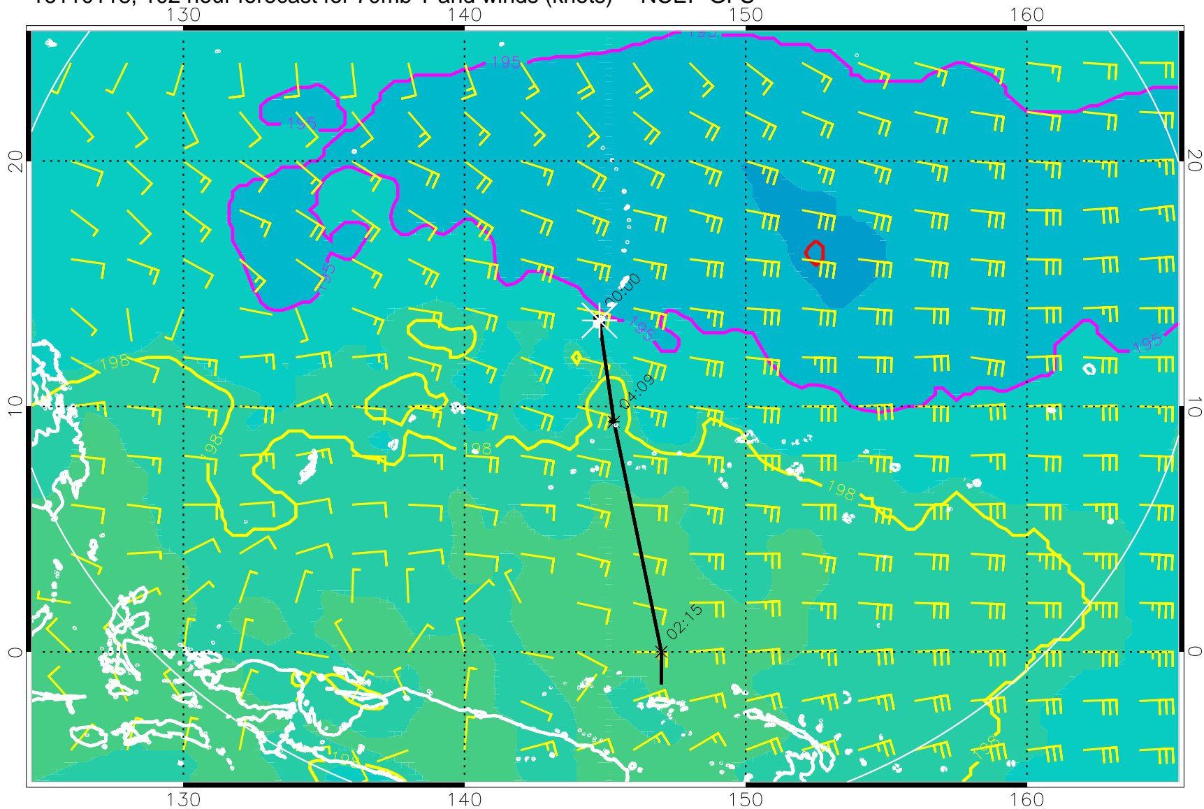
16110118, 102 hour forecast for 70mb T and winds (knots) -- NCEP GFS
