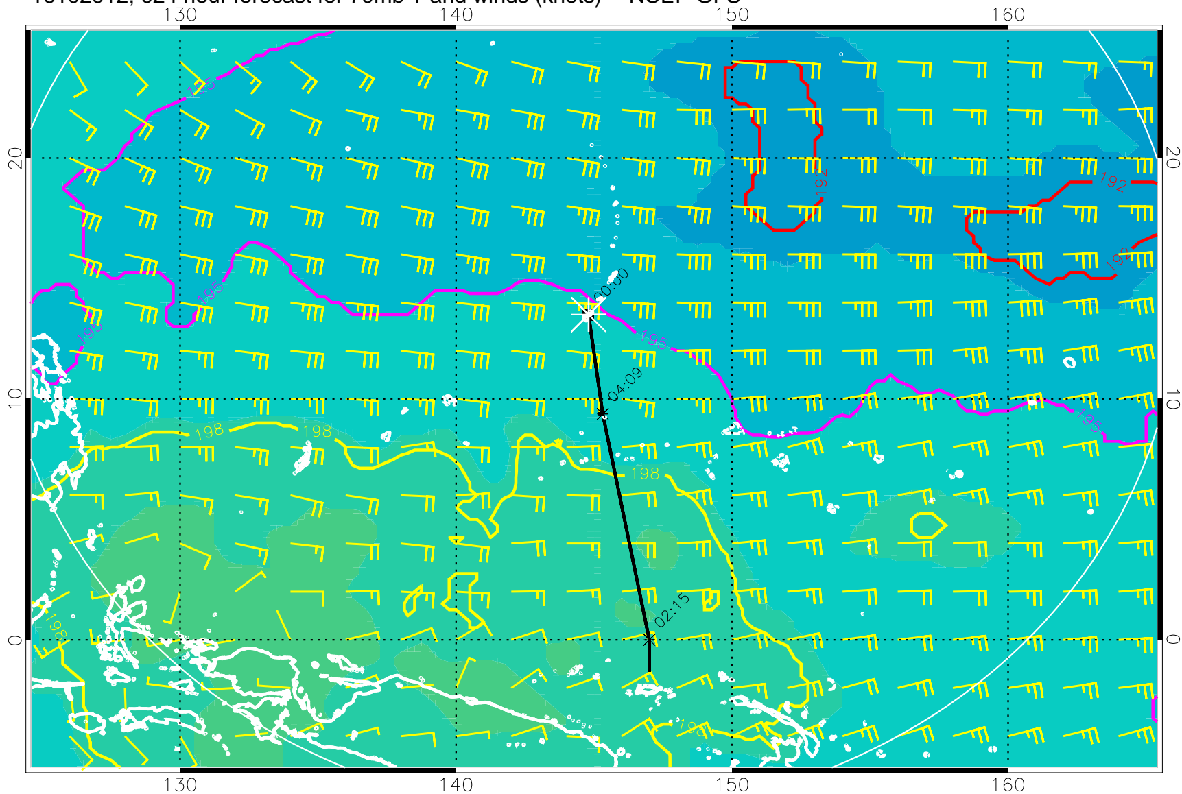
16102912, 024 hour forecast for 70mb T and winds (knots) -- NCEP GFS
