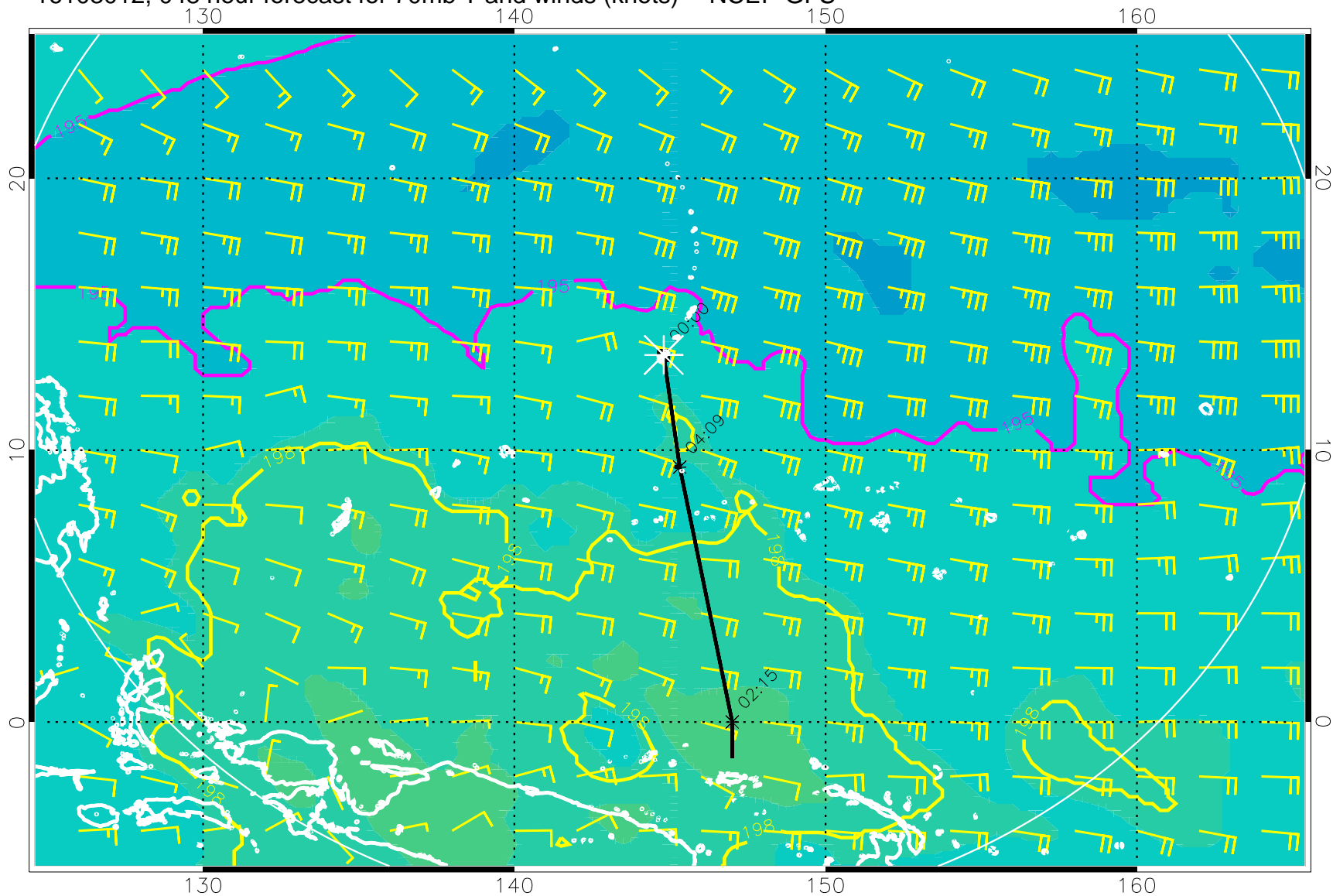
16103012, 048 hour forecast for 70mb T and winds (knots) -- NCEP GFS
