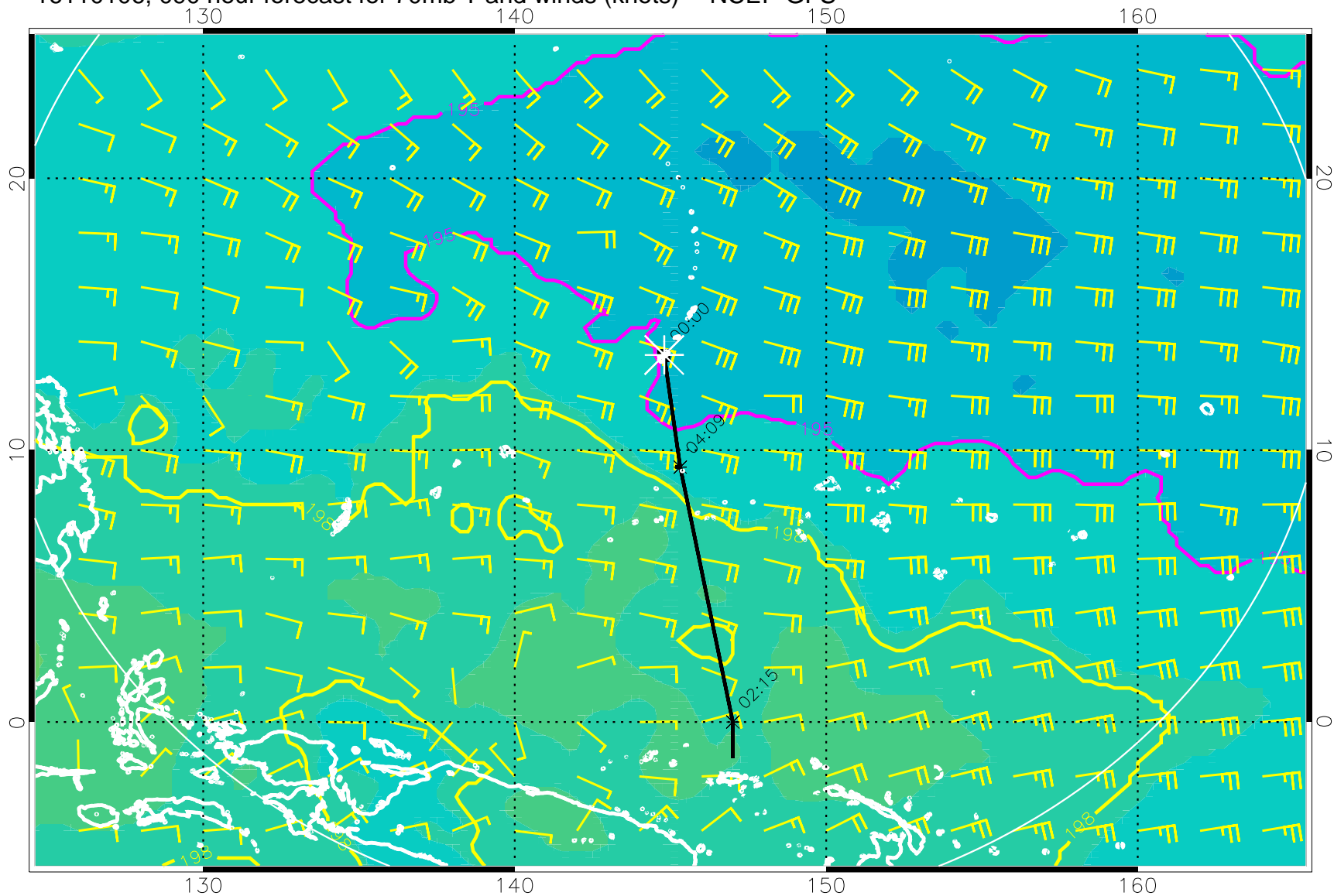
16110106, 090 hour forecast for 70mb T and winds (knots) -- NCEP GFS
