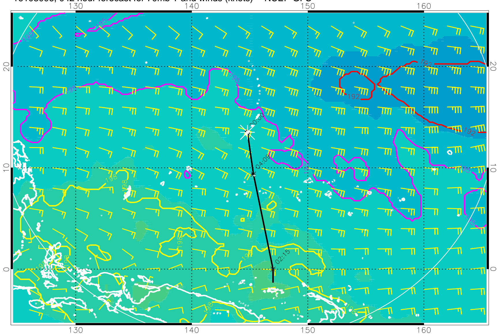
16103006, 042 hour forecast for 70mb T and winds (knots) -- NCEP GFS
