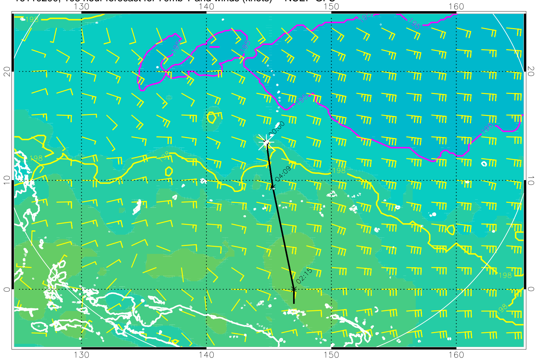
16110200, 108 hour forecast for 70mb T and winds (knots) -- NCEP GFS
