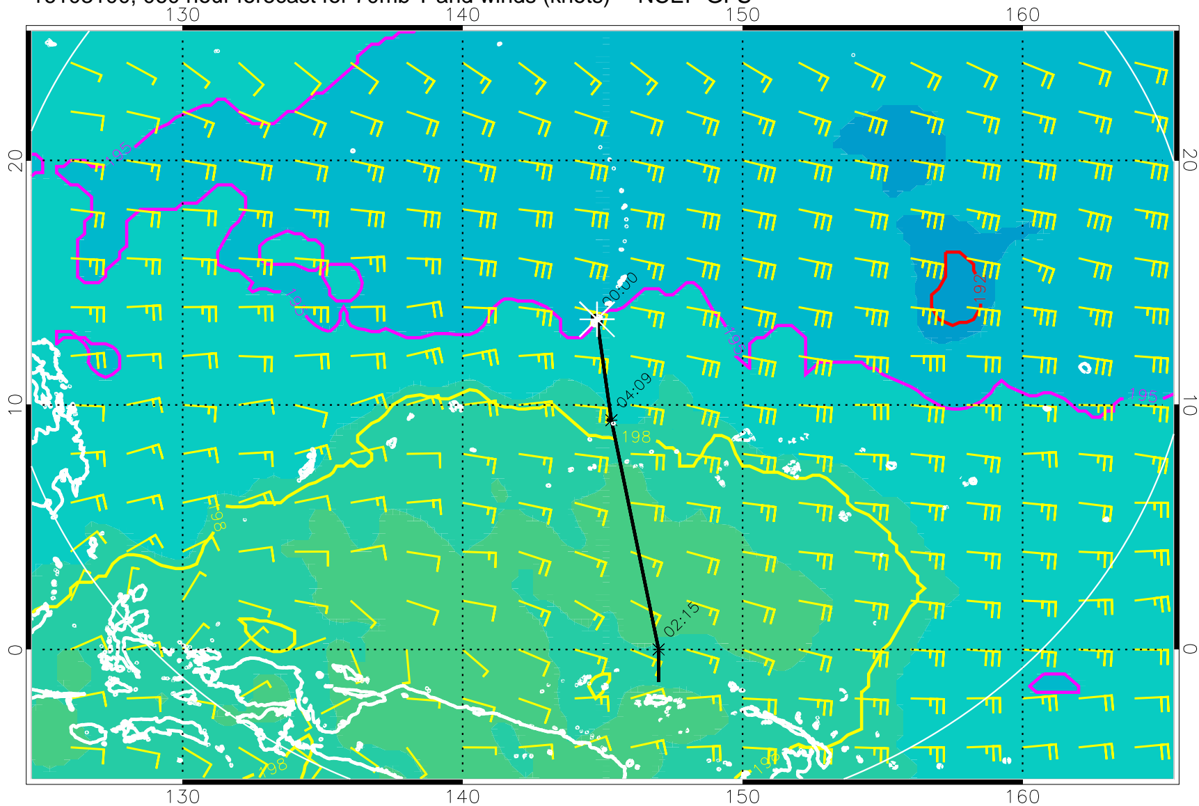
16103100, 060 hour forecast for 70mb T and winds (knots) -- NCEP GFS
