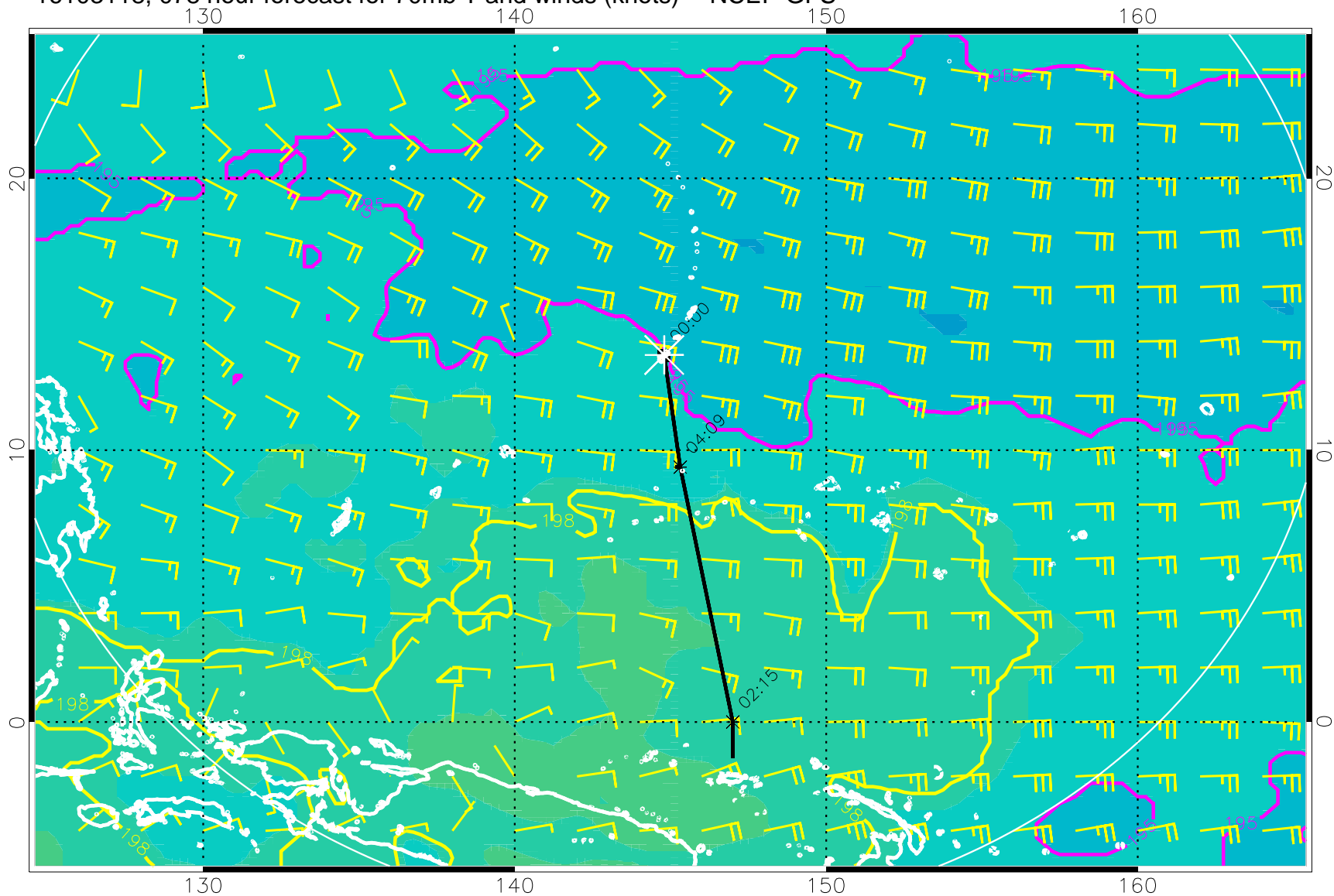
16103118, 078 hour forecast for 70mb T and winds (knots) -- NCEP GFS
