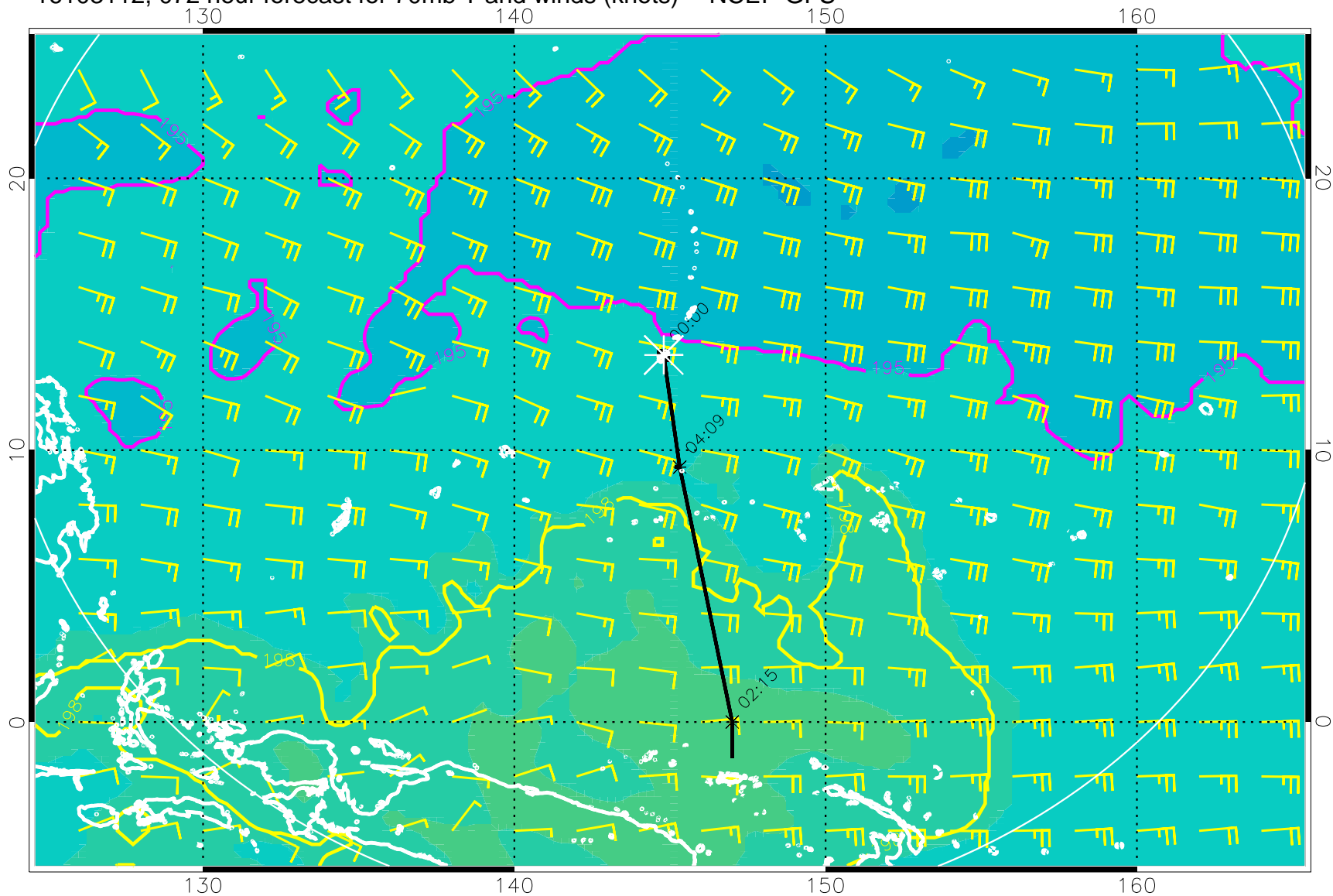
16103112, 072 hour forecast for 70mb T and winds (knots) -- NCEP GFS
