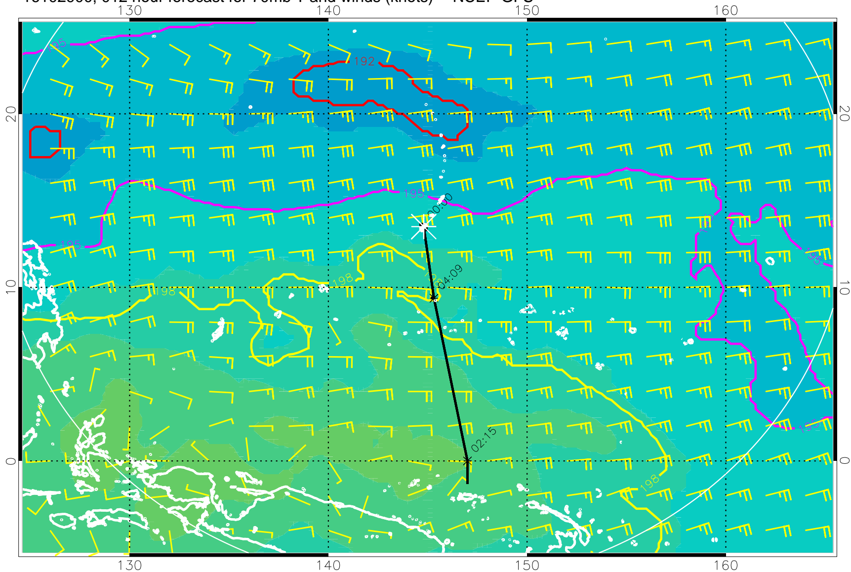
16102900, 012 hour forecast for 70mb T and winds (knots) -- NCEP GFS
