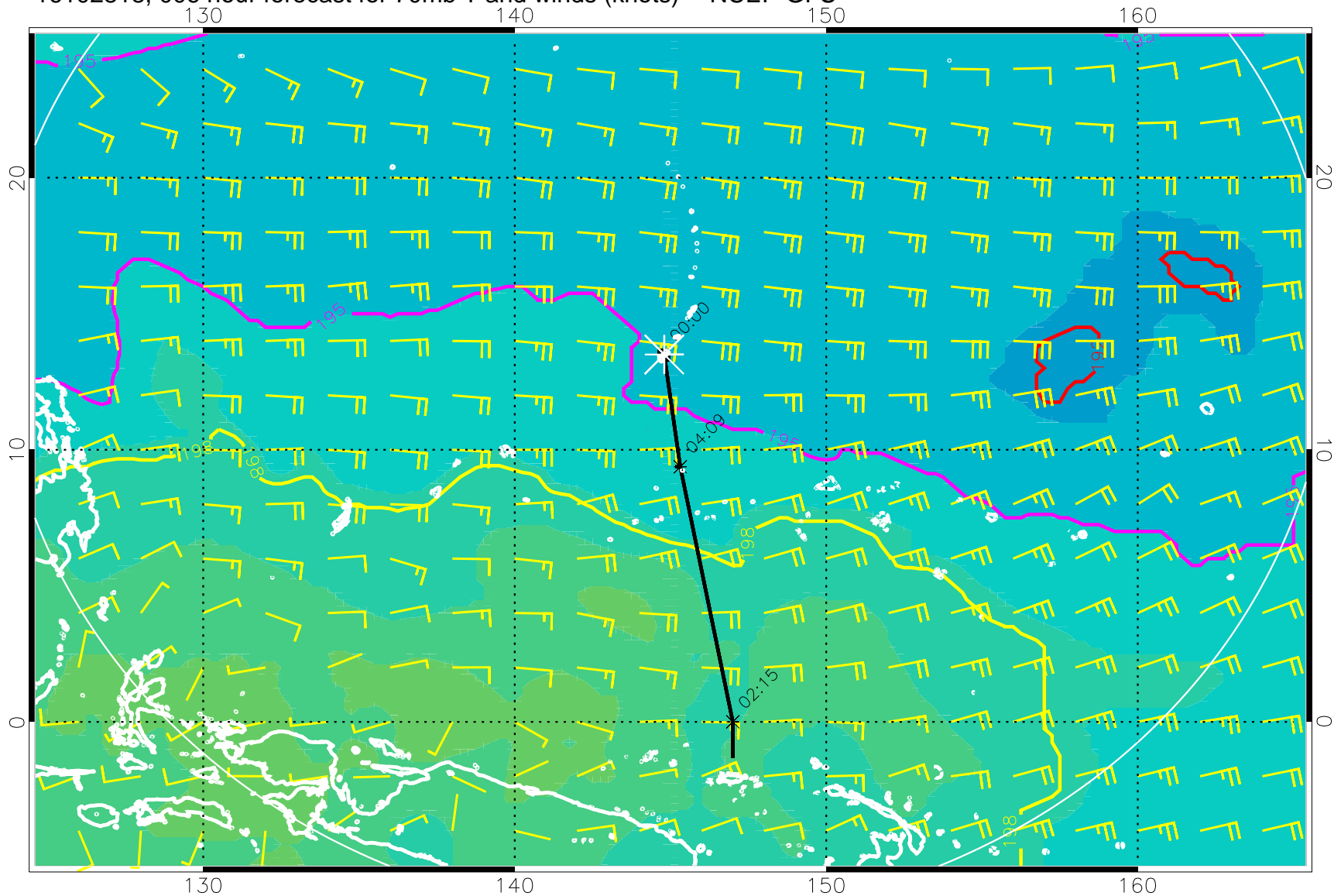
16102818, 006 hour forecast for 70mb T and winds (knots) -- NCEP GFS
