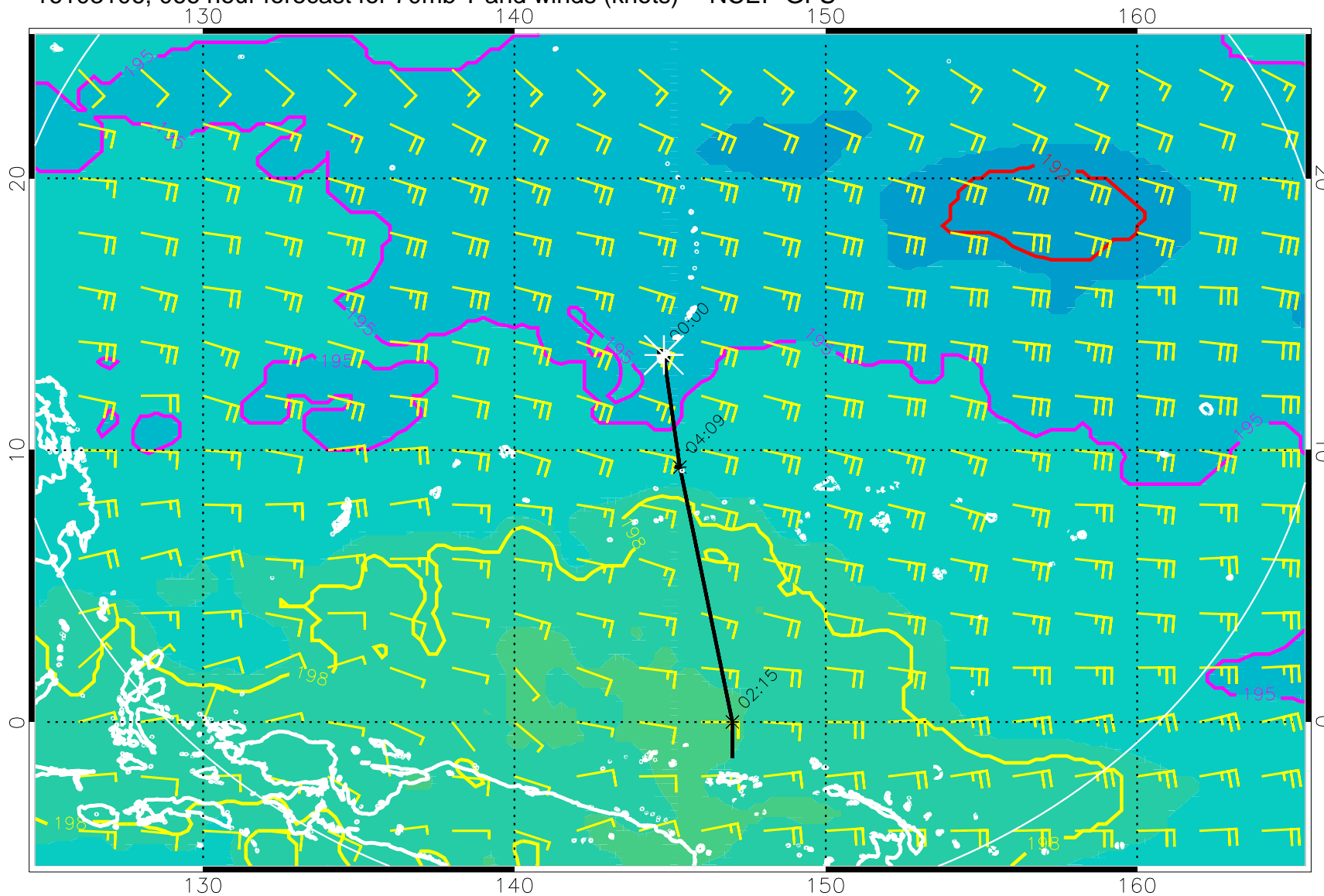
16103106, 066 hour forecast for 70mb T and winds (knots) -- NCEP GFS
