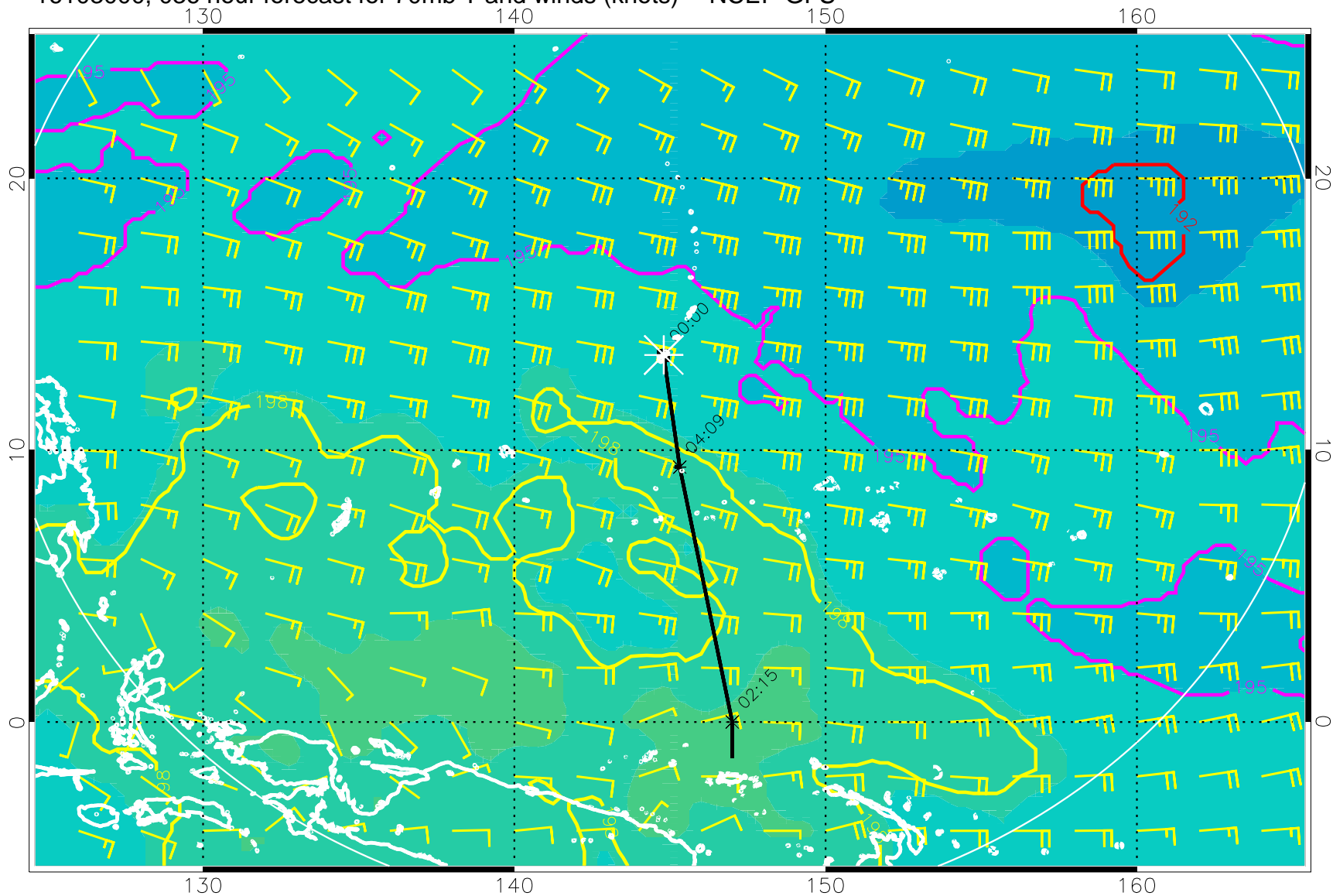
16103000, 036 hour forecast for 70mb T and winds (knots) -- NCEP GFS
