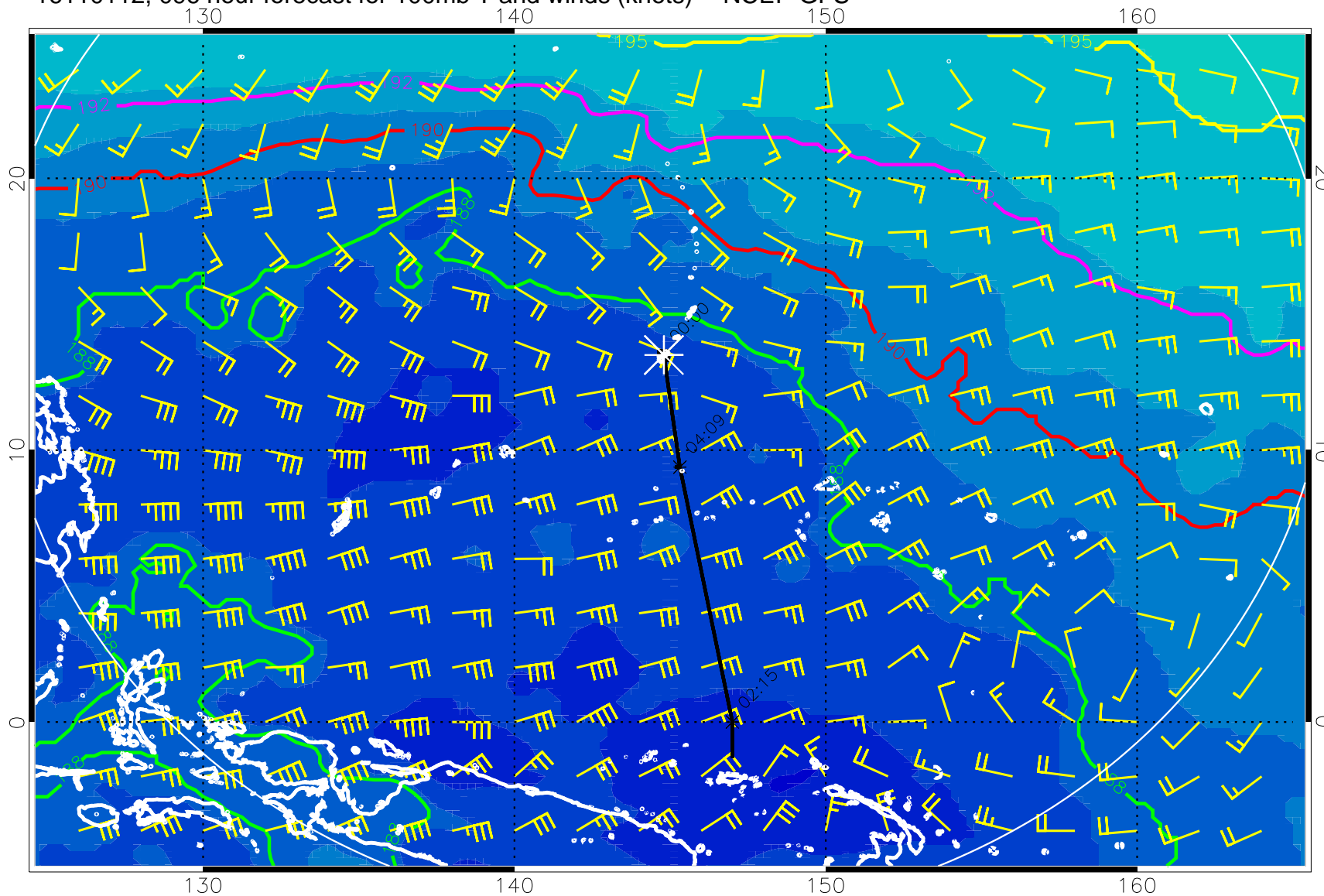
16110112, 096 hour forecast for 100mb T and winds (knots) -- NCEP GFS
