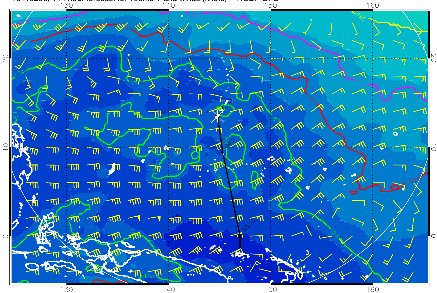
16110206, 114 hour forecast for 100mb T and winds (knots) -- NCEP GFS
