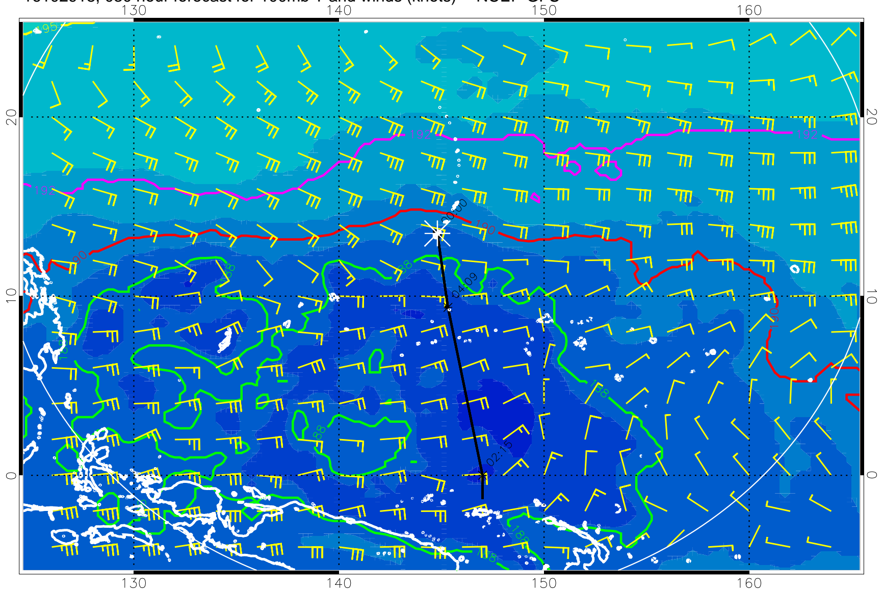
16102918, 030 hour forecast for 100mb T and winds (knots) -- NCEP GFS
