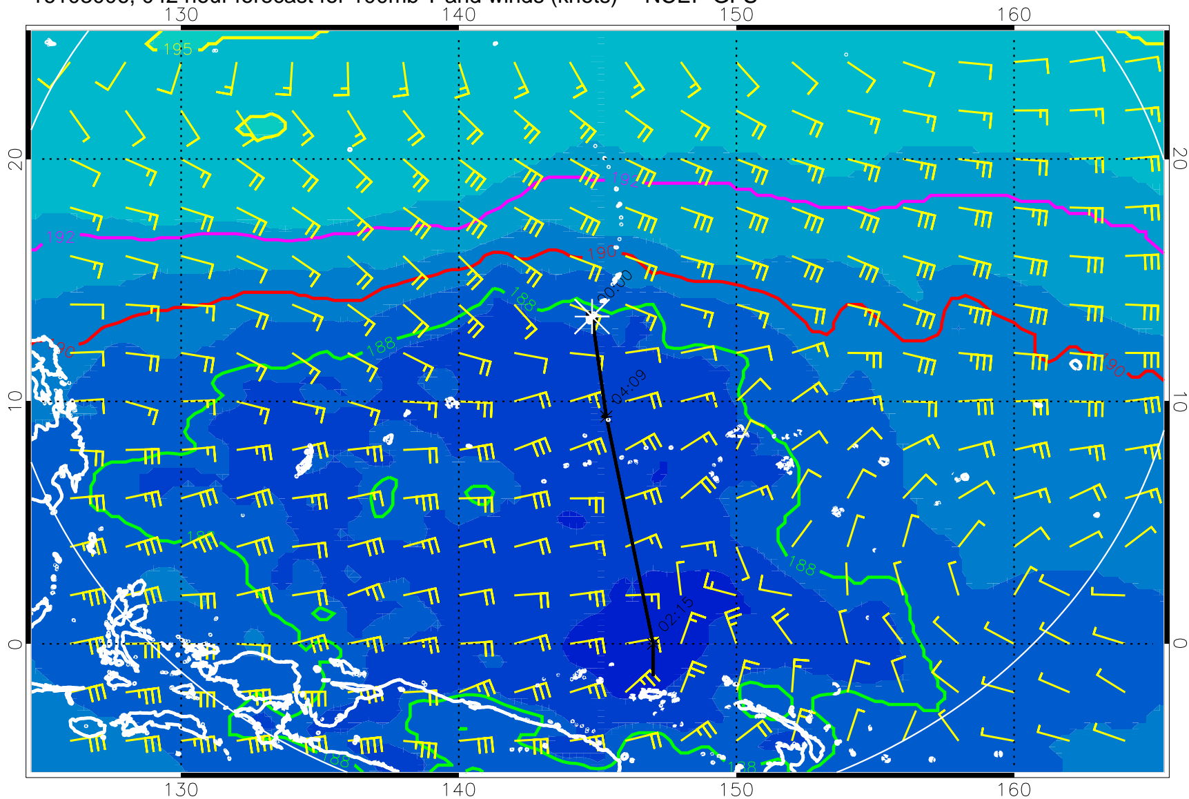
16103006, 042 hour forecast for 100mb T and winds (knots) -- NCEP GFS
