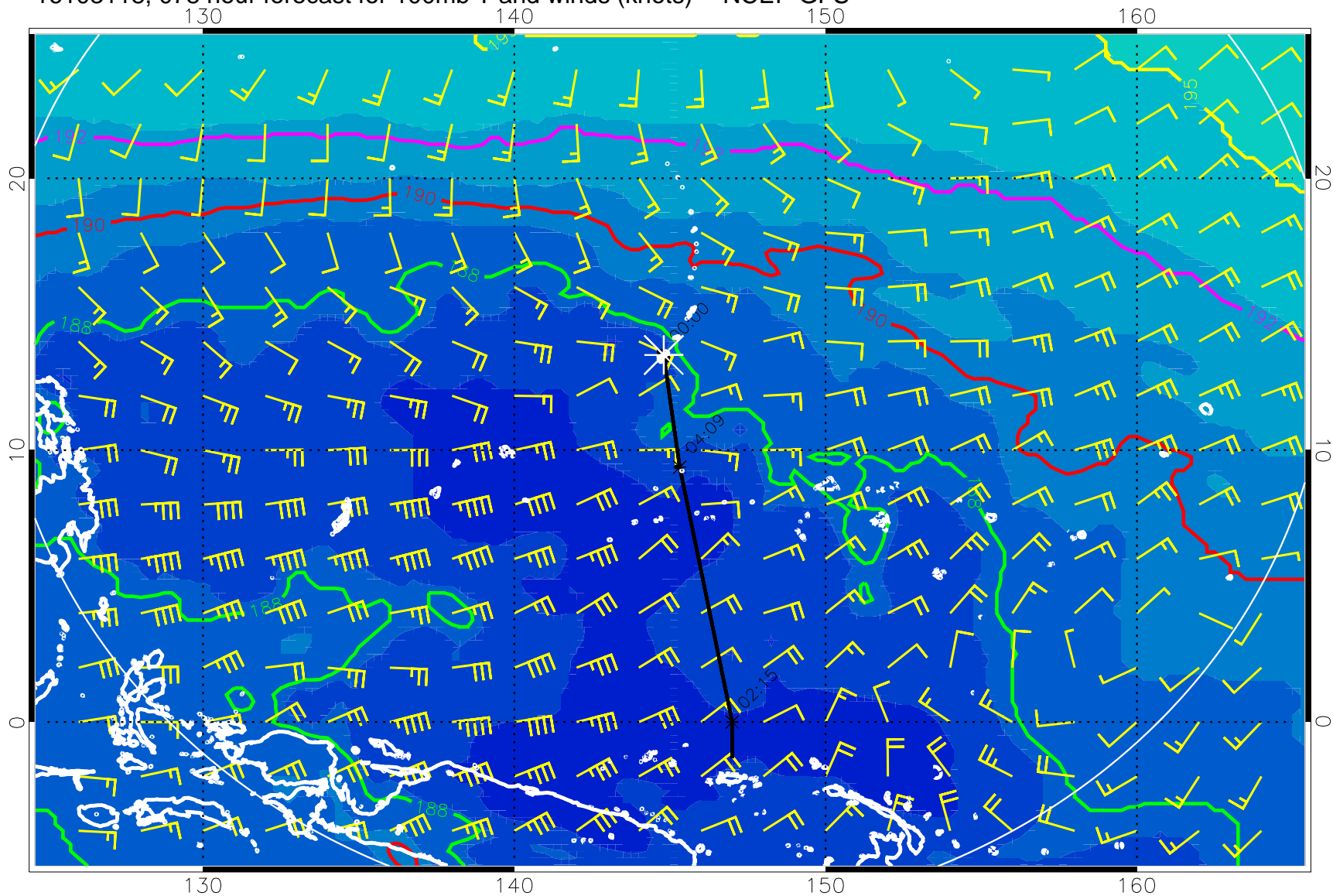
16103118, 078 hour forecast for 100mb T and winds (knots) -- NCEP GFS
