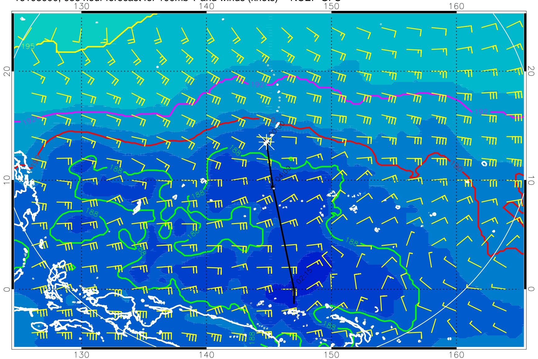
16103000, 036 hour forecast for 100mb T and winds (knots) -- NCEP GFS
