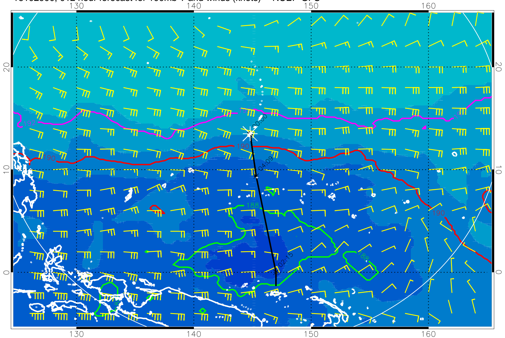
16102900, 012 hour forecast for 100mb T and winds (knots) -- NCEP GFS
