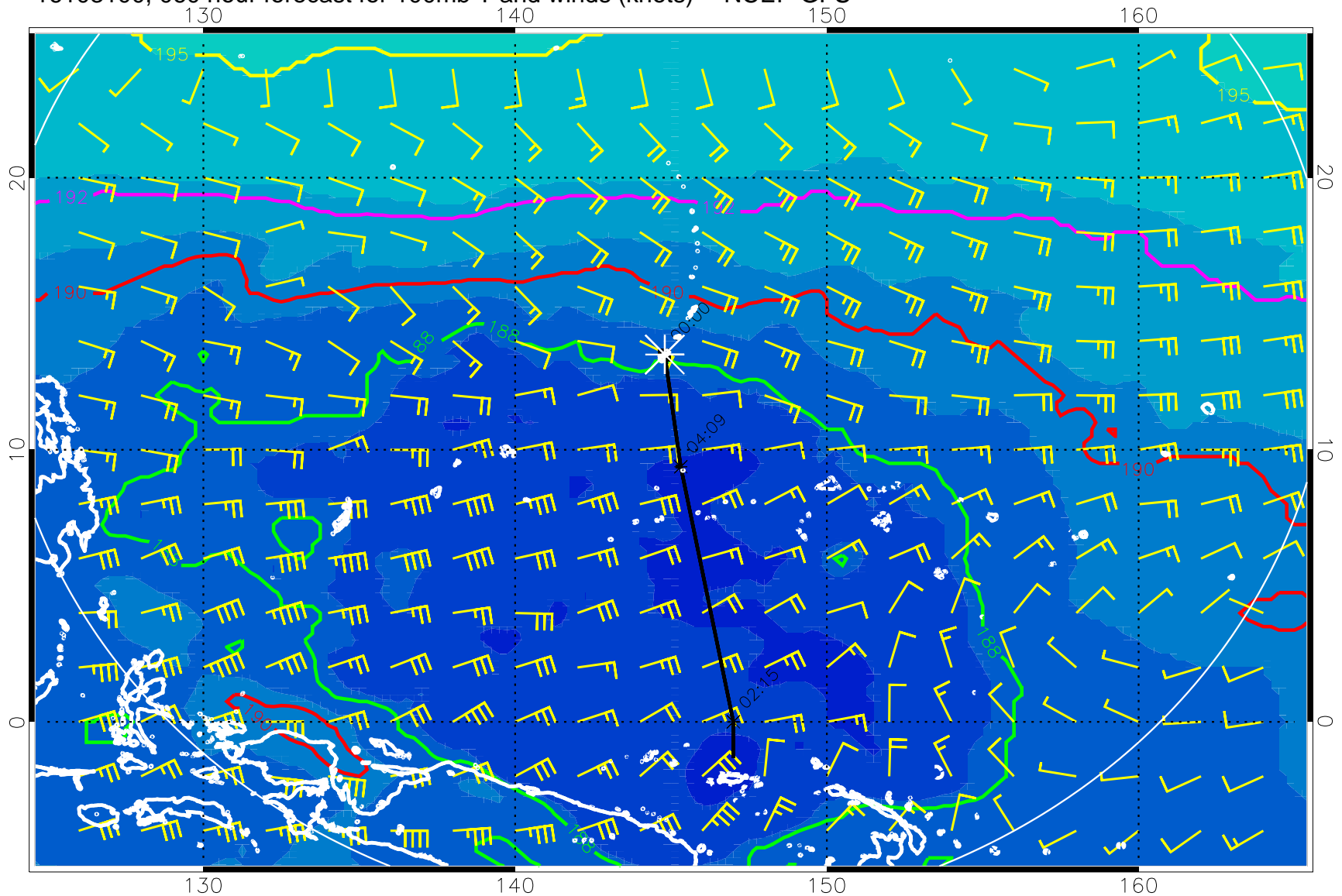
16103100, 060 hour forecast for 100mb T and winds (knots) -- NCEP GFS
