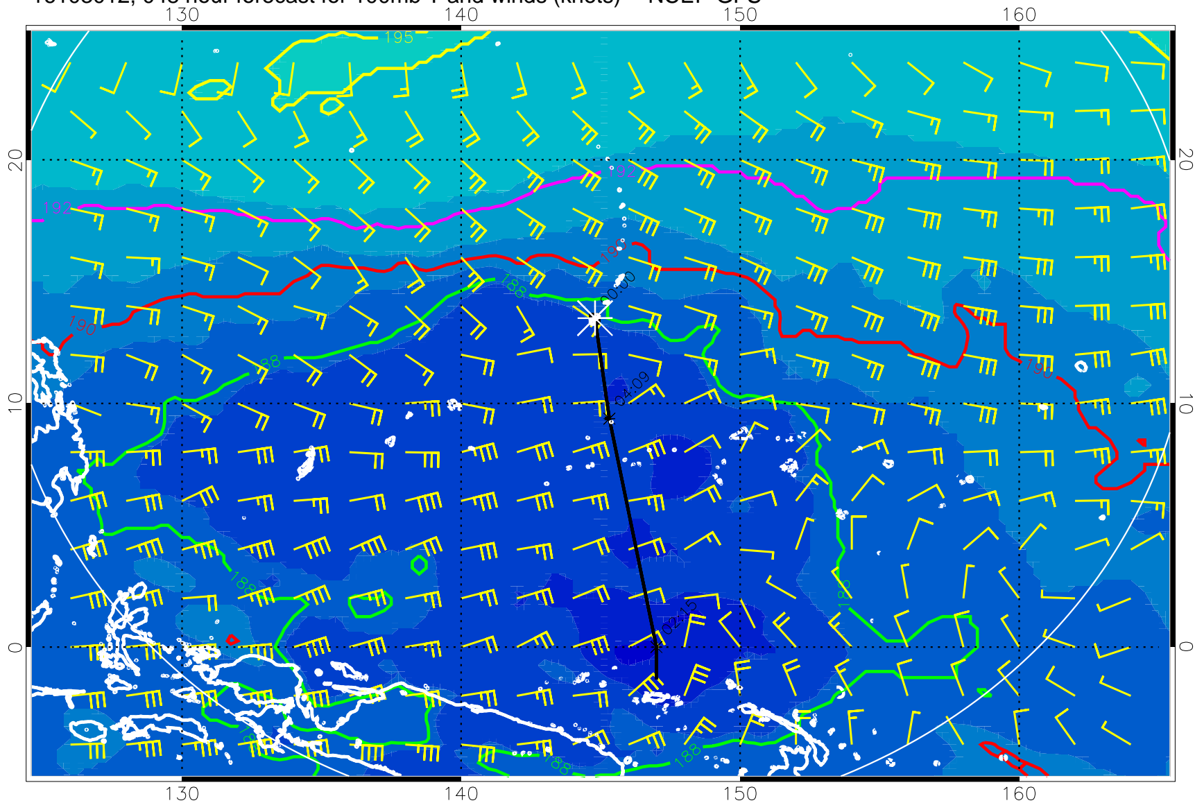
16103012, 048 hour forecast for 100mb T and winds (knots) -- NCEP GFS
