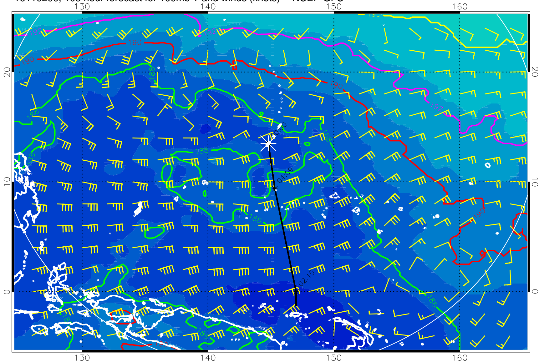
16110200, 108 hour forecast for 100mb T and winds (knots) -- NCEP GFS
