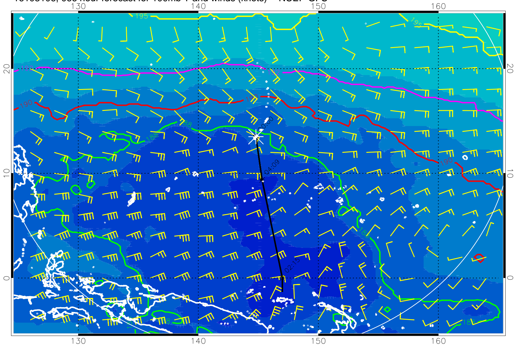
16103106, 066 hour forecast for 100mb T and winds (knots) -- NCEP GFS
