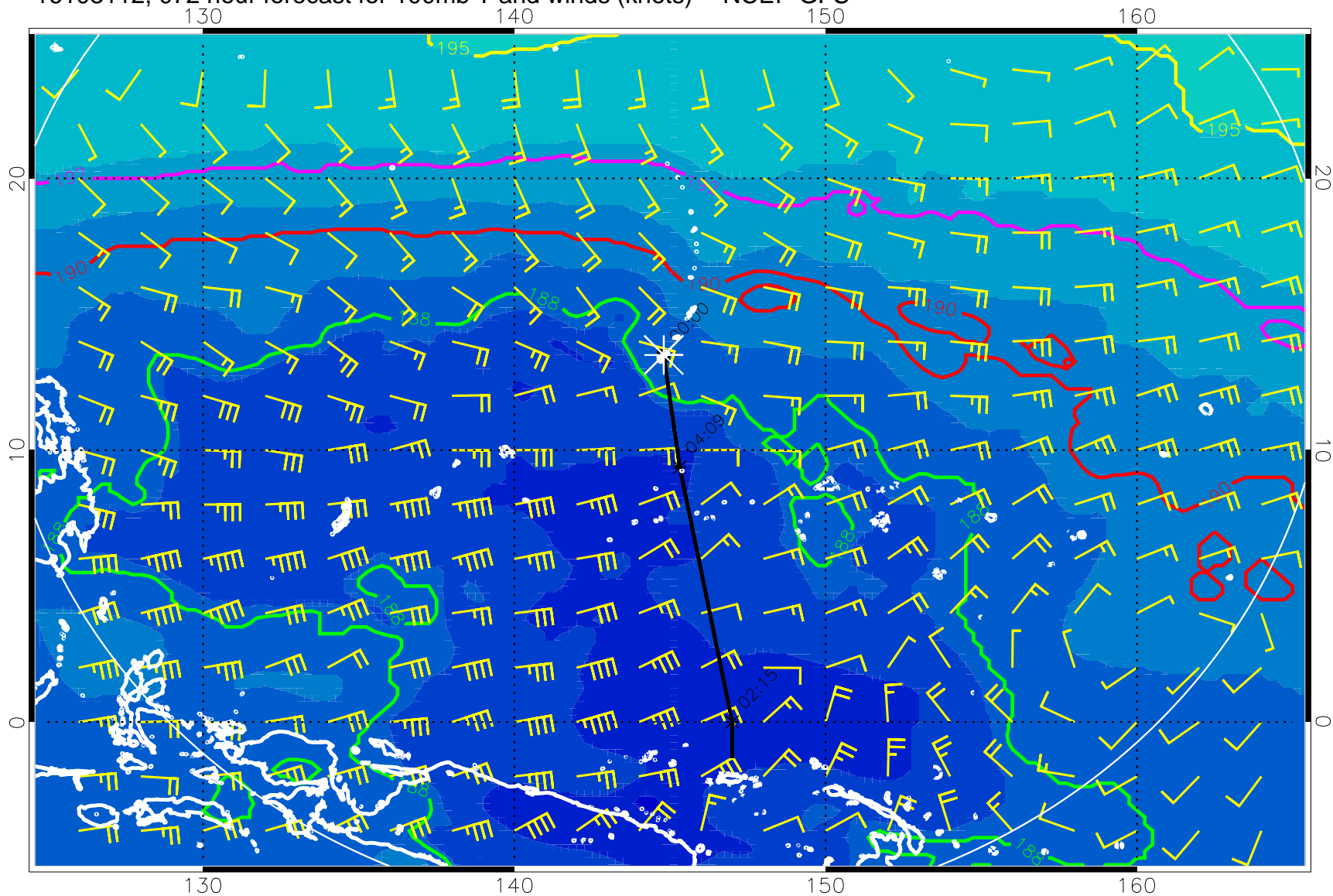
16103112, 072 hour forecast for 100mb T and winds (knots) -- NCEP GFS
