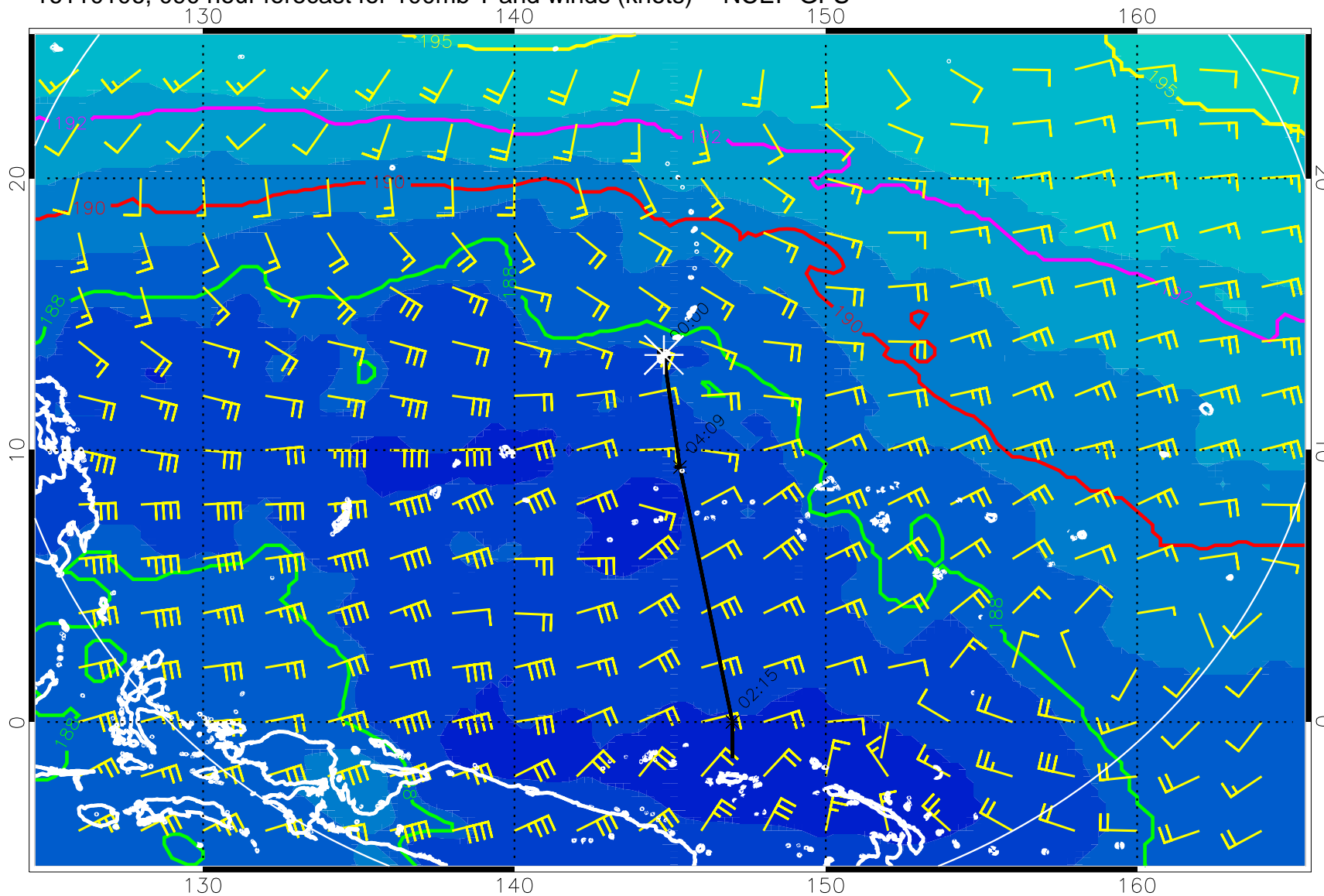
16110106, 090 hour forecast for 100mb T and winds (knots) -- NCEP GFS
