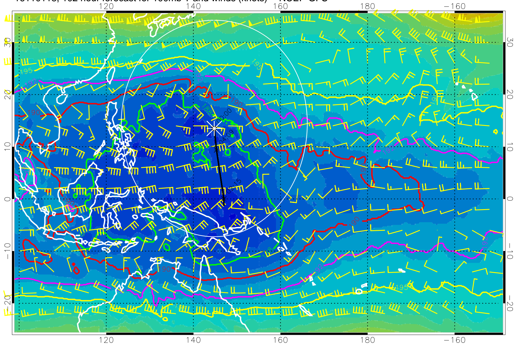
16110118, 102 hour forecast for 100mb T and winds (knots) -- NCEP GFS
