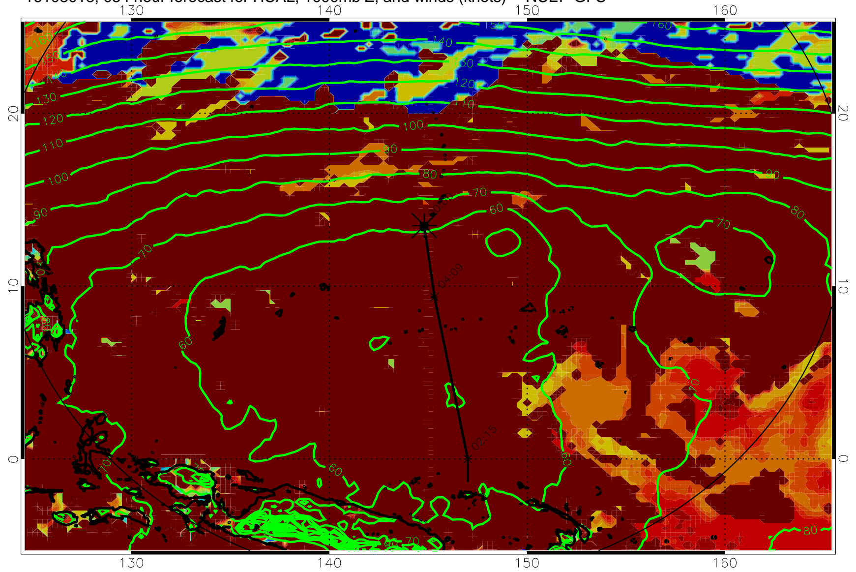
16103018, 054 hour forecast for HCAL, 1000mb Z, and winds (knots) -- NCEP GFS
