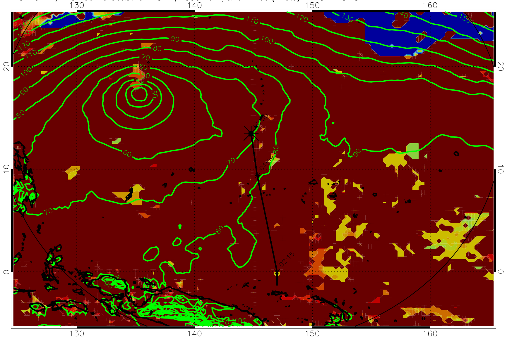
16110212, 120 hour forecast for HCAL, 1000mb Z, and winds (knots) -- NCEP GFS
