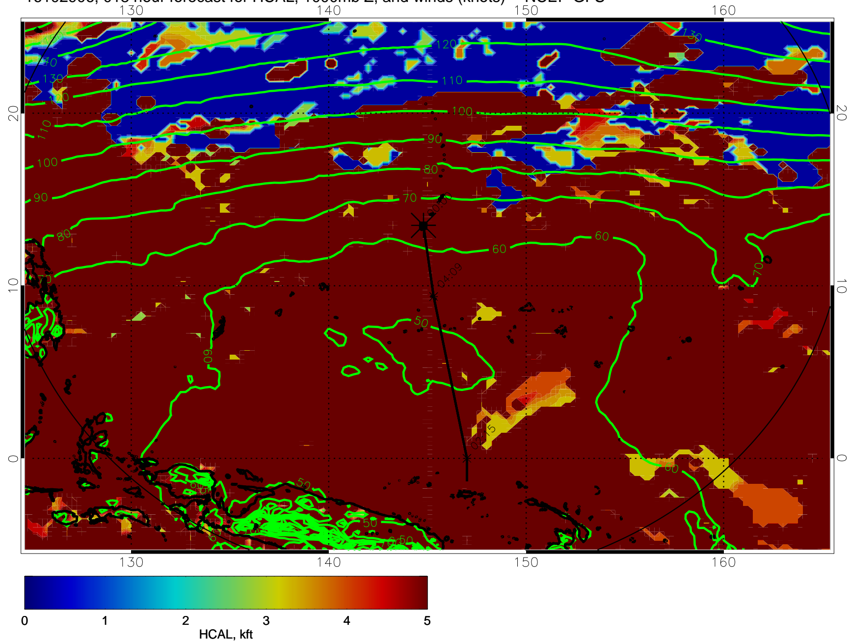
16102906, 018 hour forecast for HCAL, 1000mb Z, and winds (knots) -- NCEP GFS
