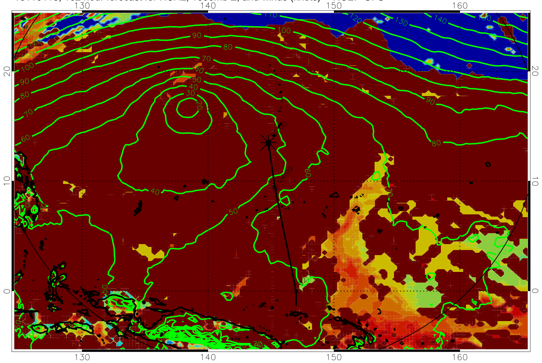
16110118, 102 hour forecast for HCAL, 1000mb Z, and winds (knots) -- NCEP GFS
