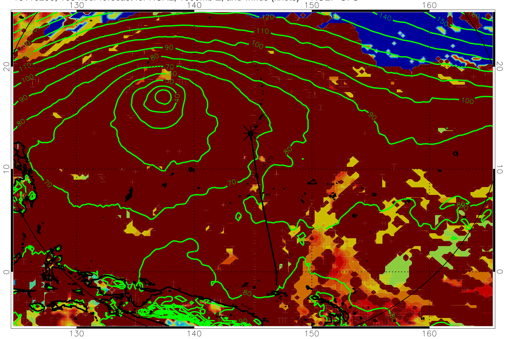
16110200, 108 hour forecast for HCAL, 1000mb Z, and winds (knots) -- NCEP GFS
