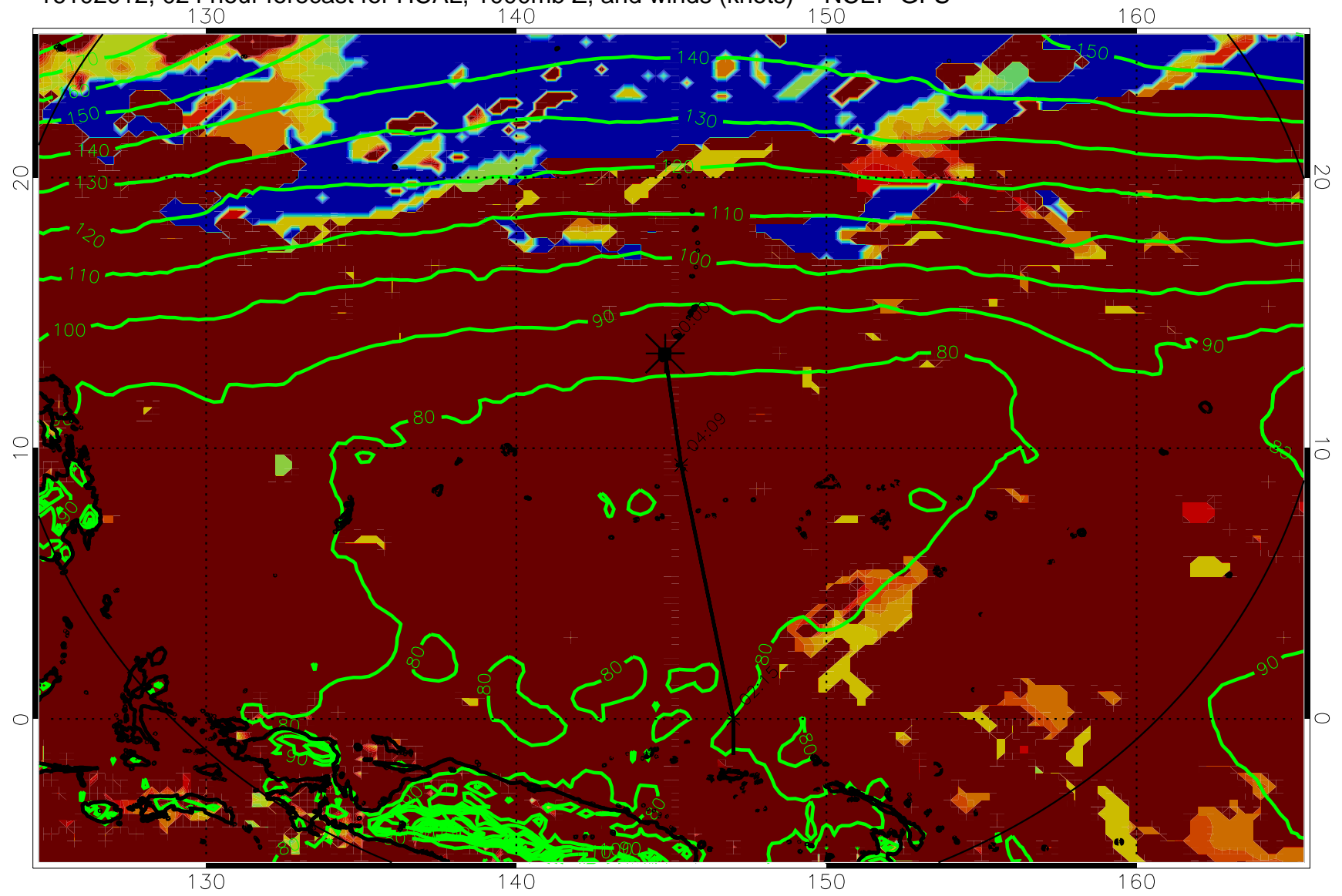
16102912, 024 hour forecast for HCAL, 1000mb Z, and winds (knots) -- NCEP GFS
