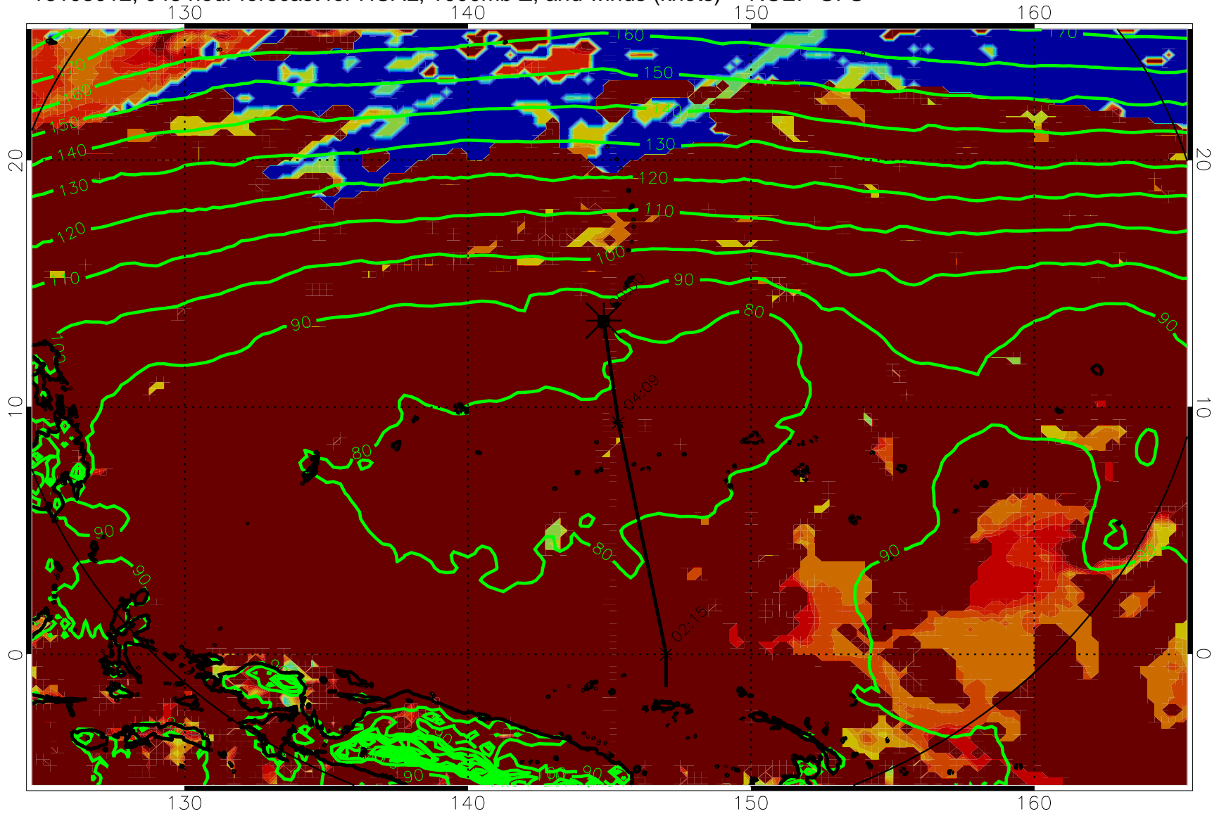
16103012, 048 hour forecast for HCAL, 1000mb Z, and winds (knots) -- NCEP GFS
