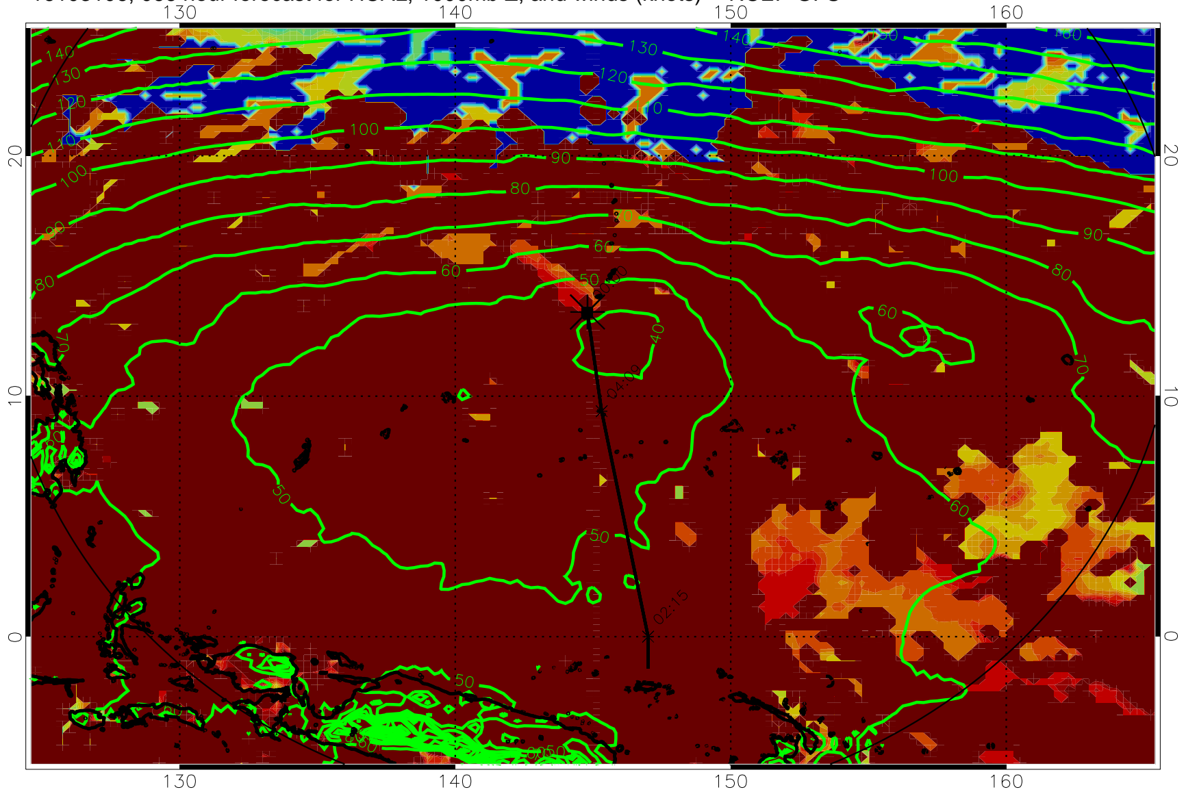
16103106, 066 hour forecast for HCAL, 1000mb Z, and winds (knots) -- NCEP GFS
