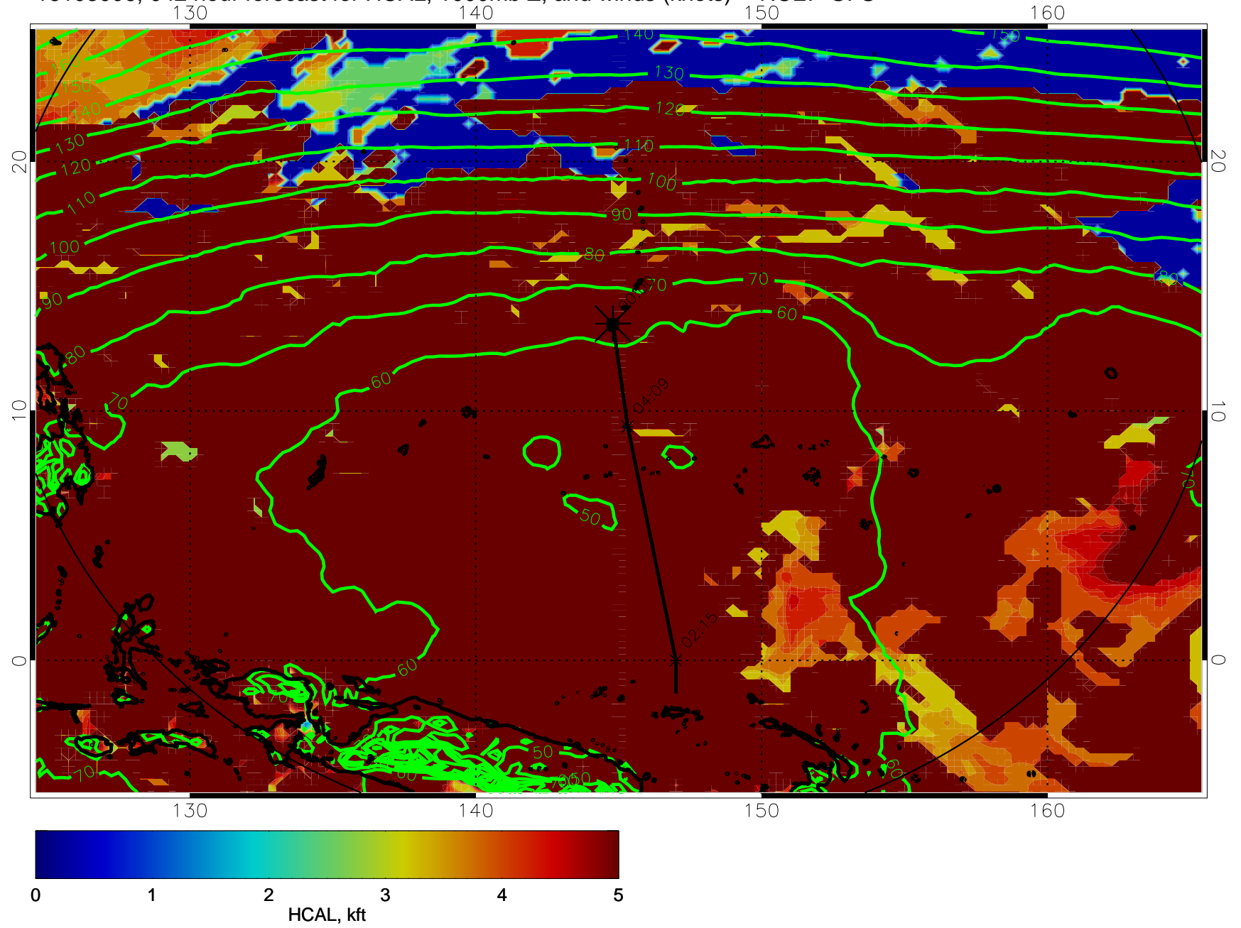
16103006, 042 hour forecast for HCAL, 1000mb Z, and winds (knots) -- NCEP GFS
