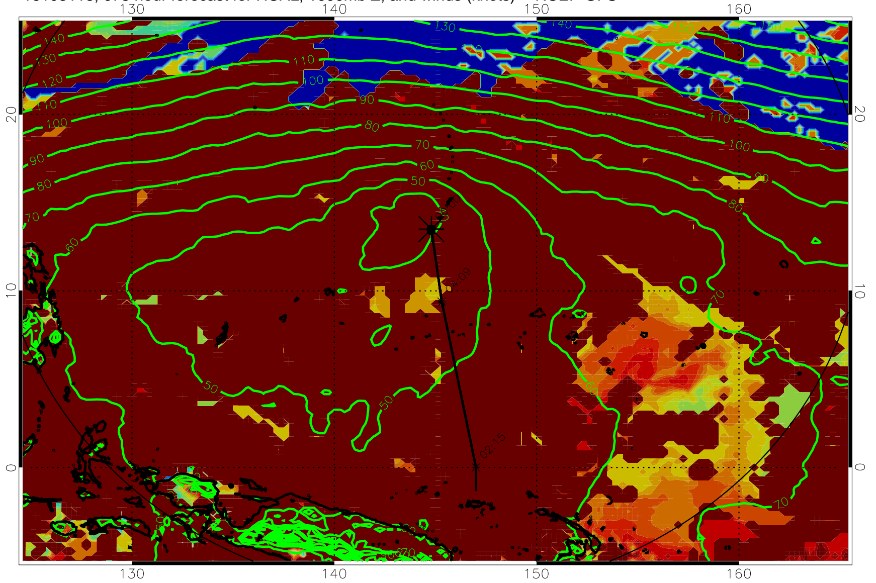
16103118, 078 hour forecast for HCAL, 1000mb Z, and winds (knots) -- NCEP GFS
