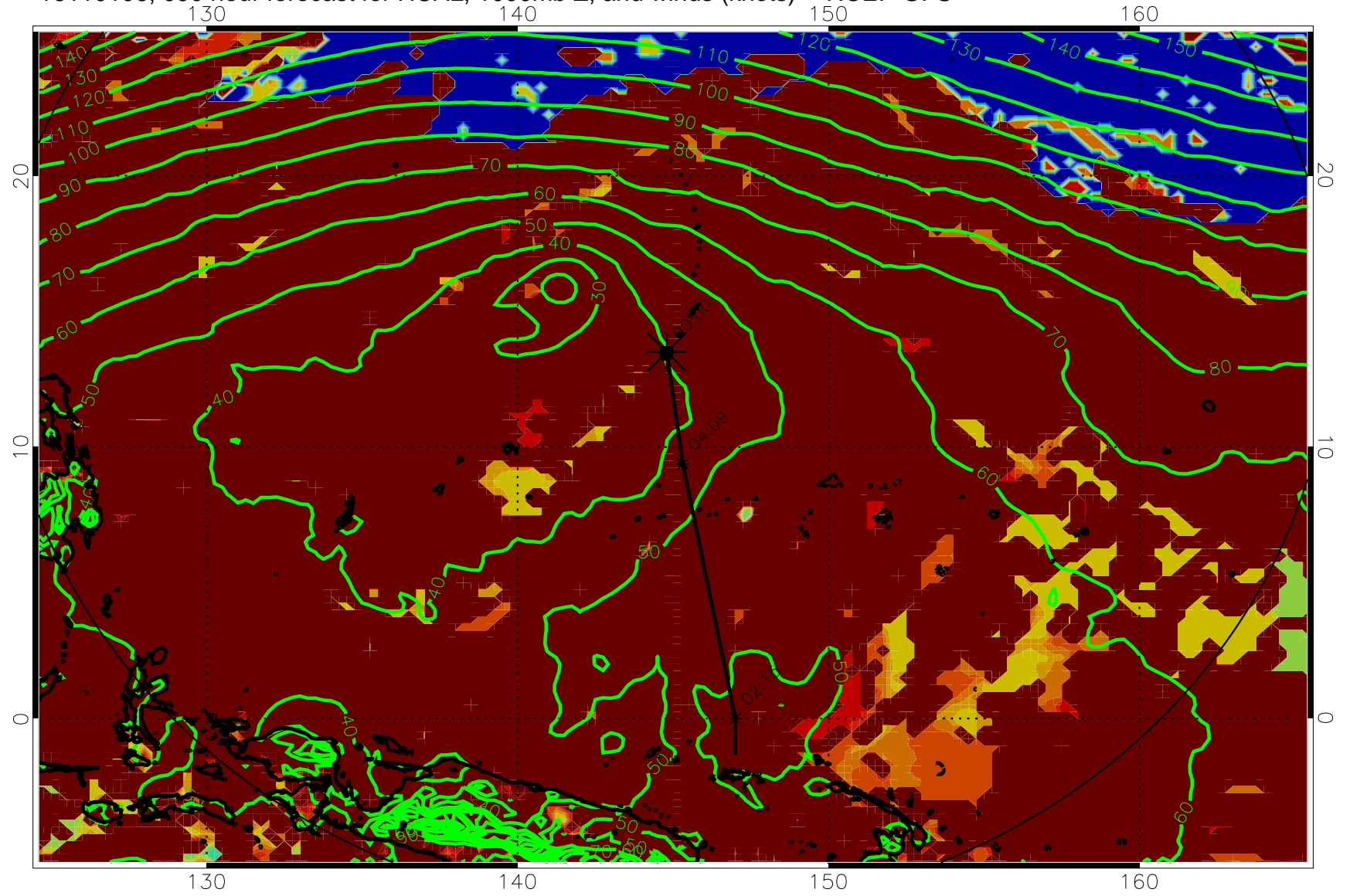
16110106, 090 hour forecast for HCAL, 1000mb Z, and winds (knots) -- NCEP GFS
