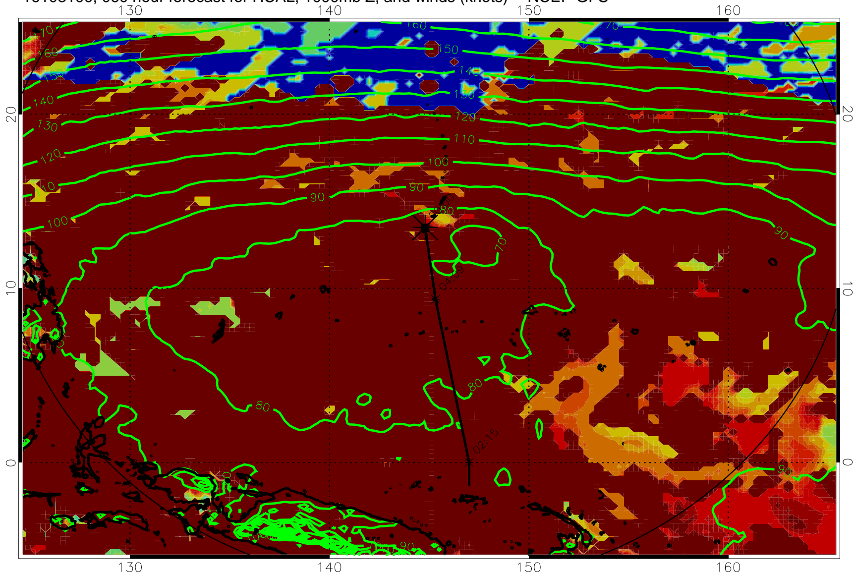
16103100, 060 hour forecast for HCAL, 1000mb Z, and winds (knots) -- NCEP GFS
