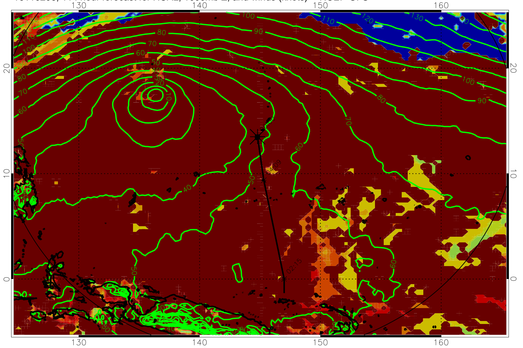
16110206, 114 hour forecast for HCAL, 1000mb Z, and winds (knots) -- NCEP GFS
