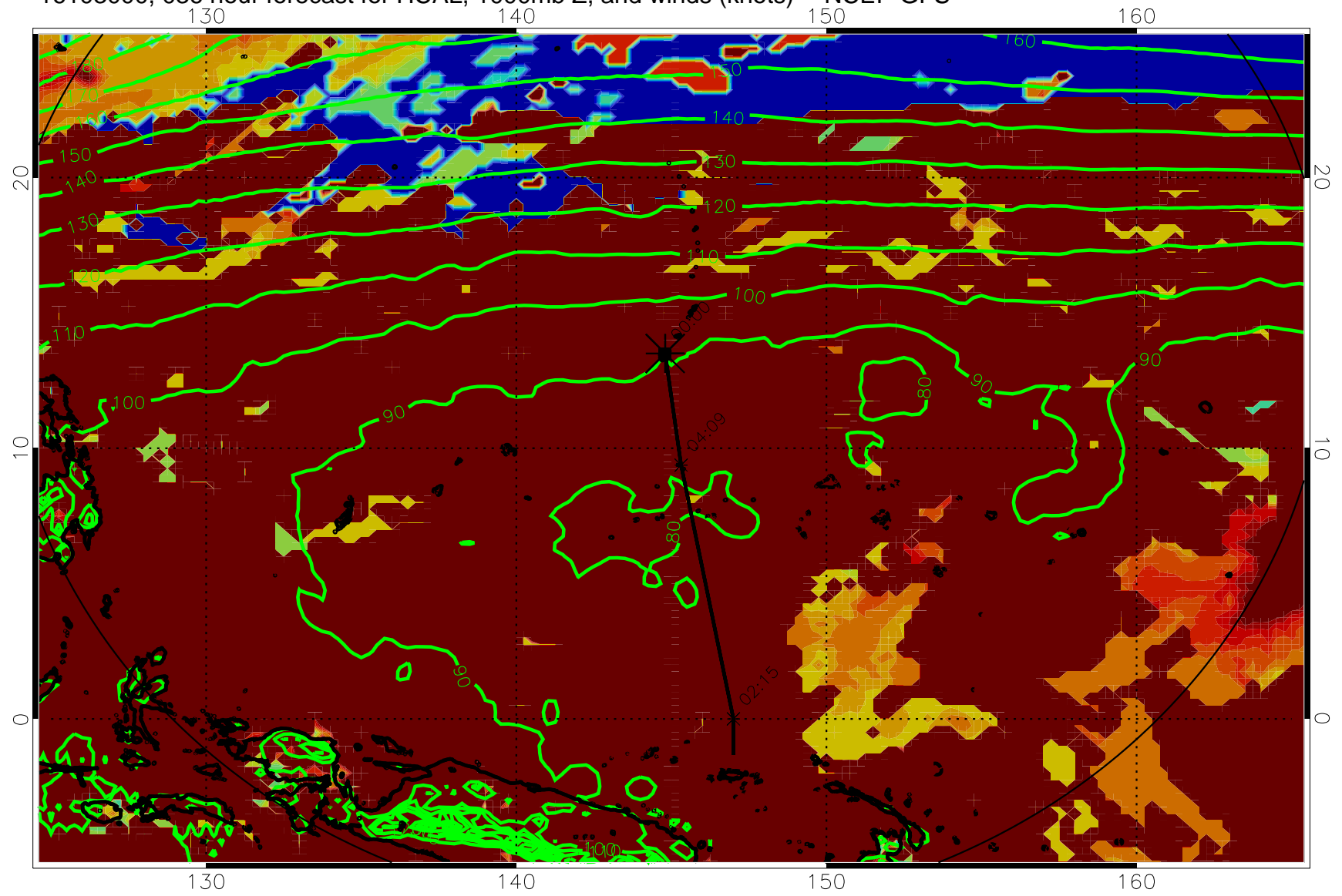
16103000, 036 hour forecast for HCAL, 1000mb Z, and winds (knots) -- NCEP GFS
