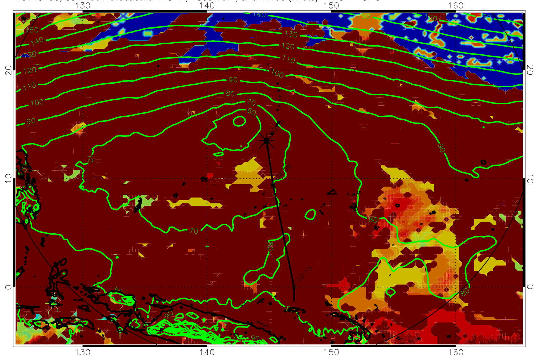
16110100, 084 hour forecast for HCAL, 1000mb Z, and winds (knots) -- NCEP GFS
