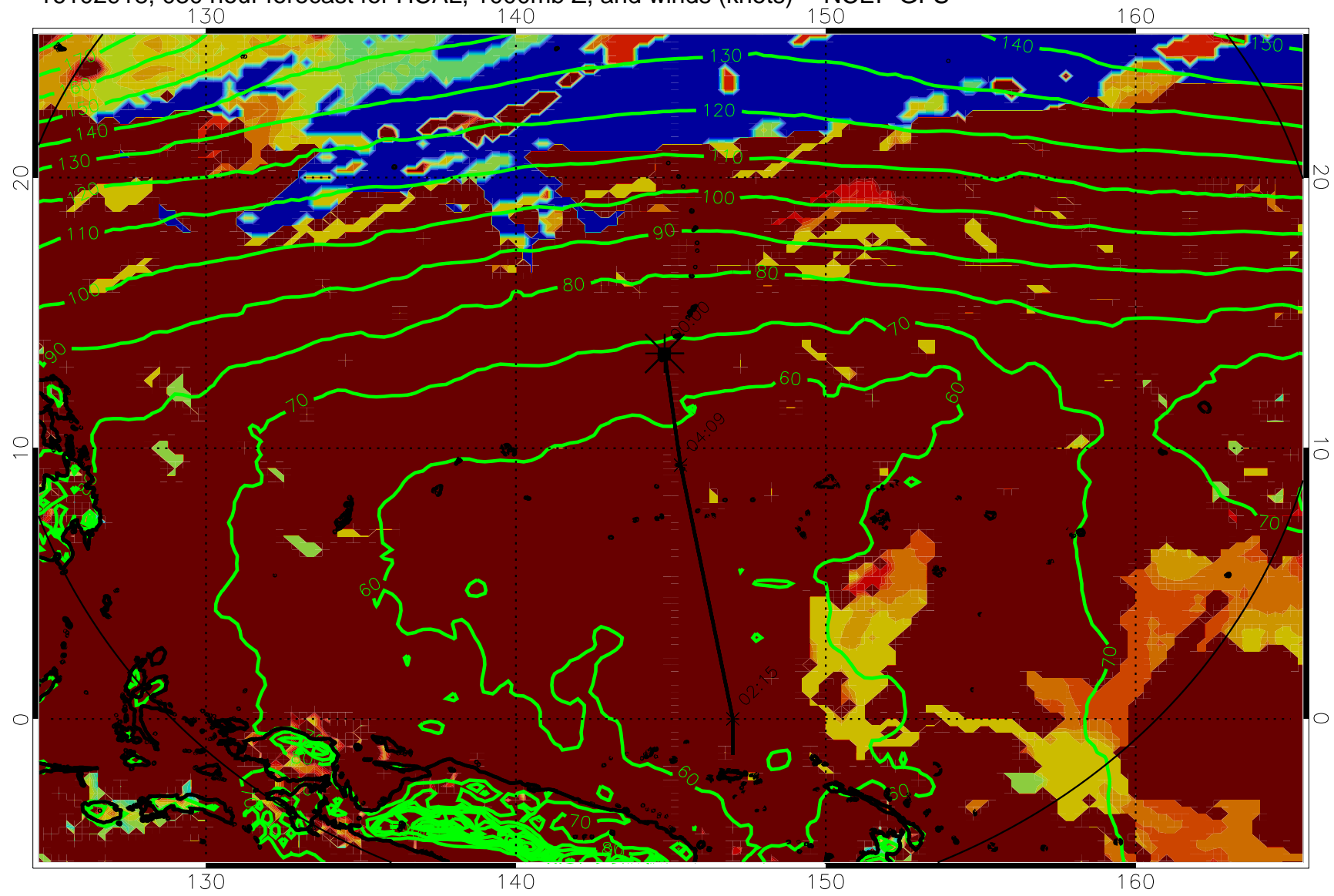
16102918, 030 hour forecast for HCAL, 1000mb Z, and winds (knots) -- NCEP GFS
