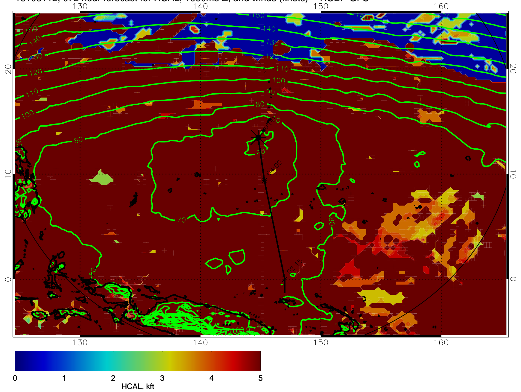
16103112, 072 hour forecast for HCAL, 1000mb Z, and winds (knots) -- NCEP GFS
