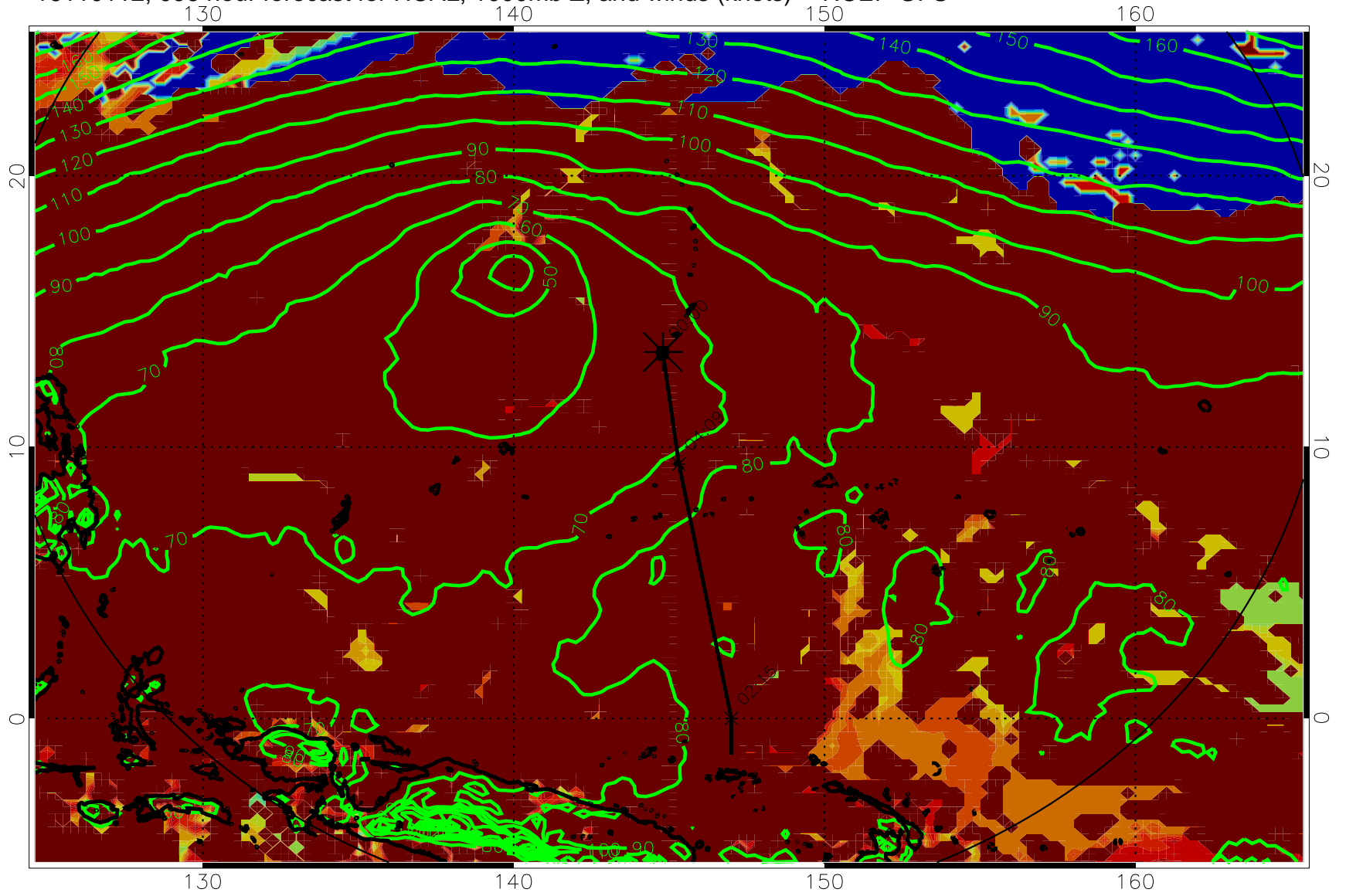
16110112, 096 hour forecast for HCAL, 1000mb Z, and winds (knots) -- NCEP GFS
