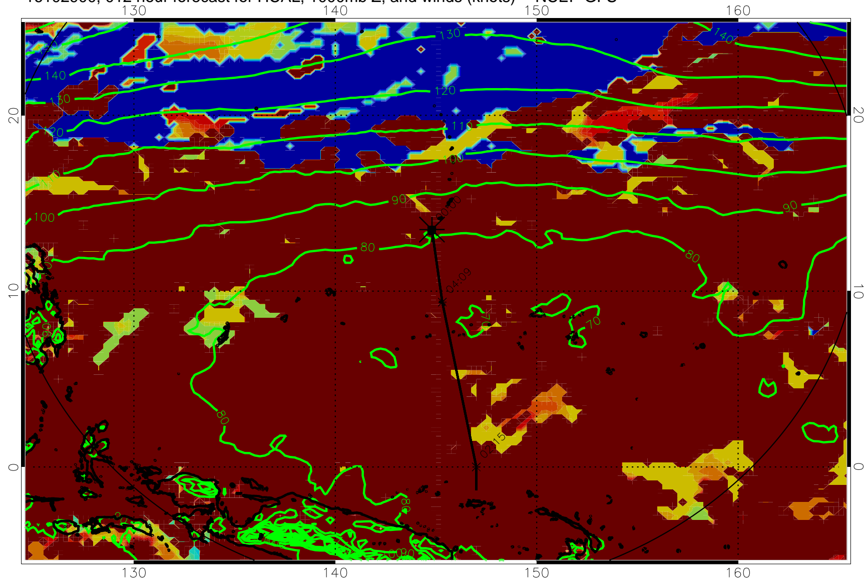
16102900, 012 hour forecast for HCAL, 1000mb Z, and winds (knots) -- NCEP GFS
