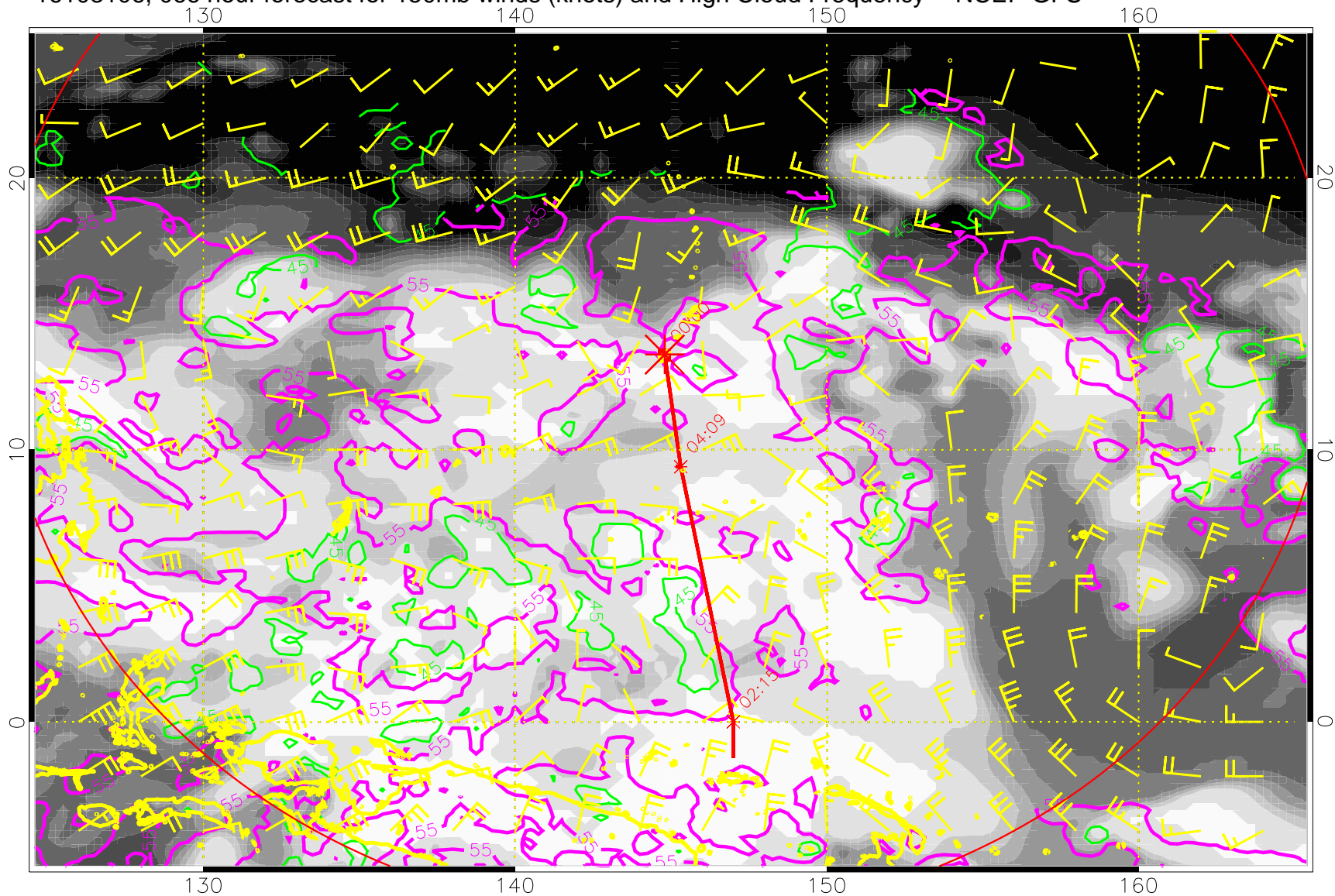
16103106, 066 hour forecast for 150mb winds (knots) and High Cloud Frequency -- NCEP GFS
