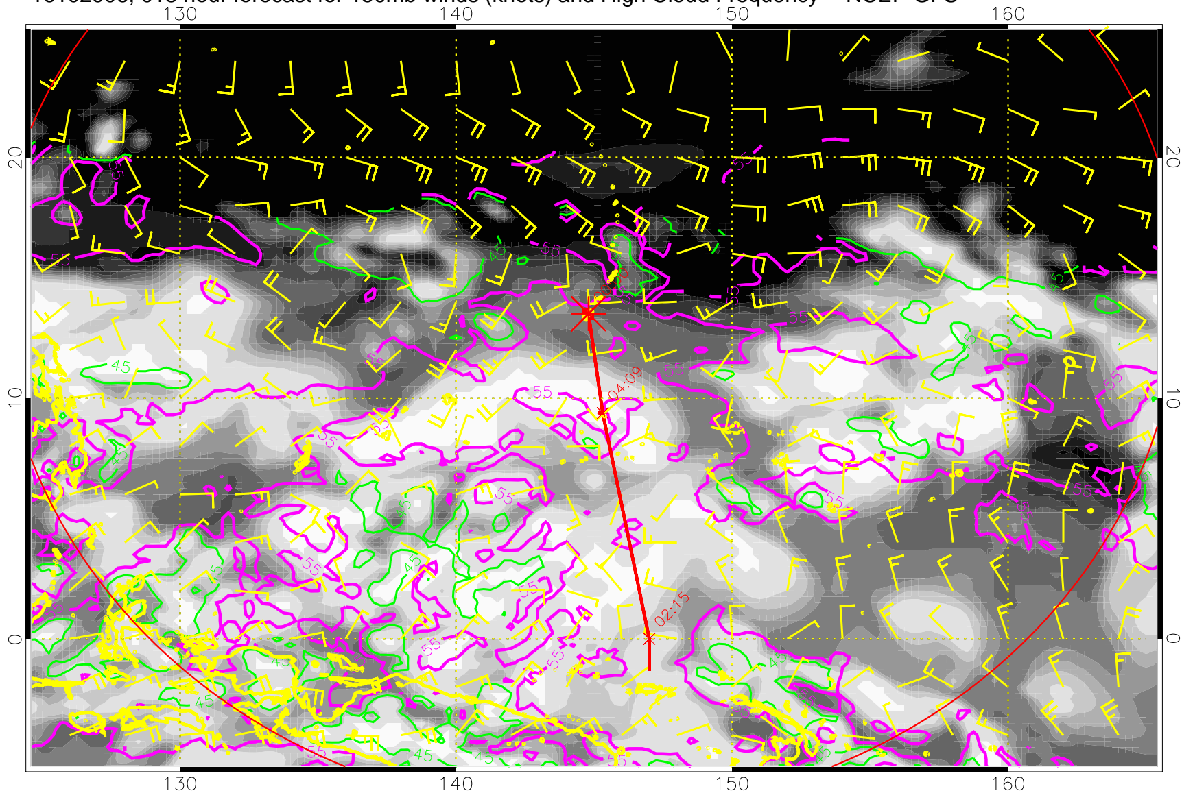
16102906, 018 hour forecast for 150mb winds (knots) and High Cloud Frequency -- NCEP GFS
