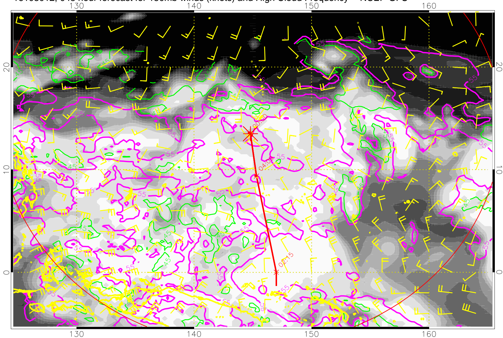
16103012, 048 hour forecast for 150mb winds (knots) and High Cloud Frequency -- NCEP GFS
