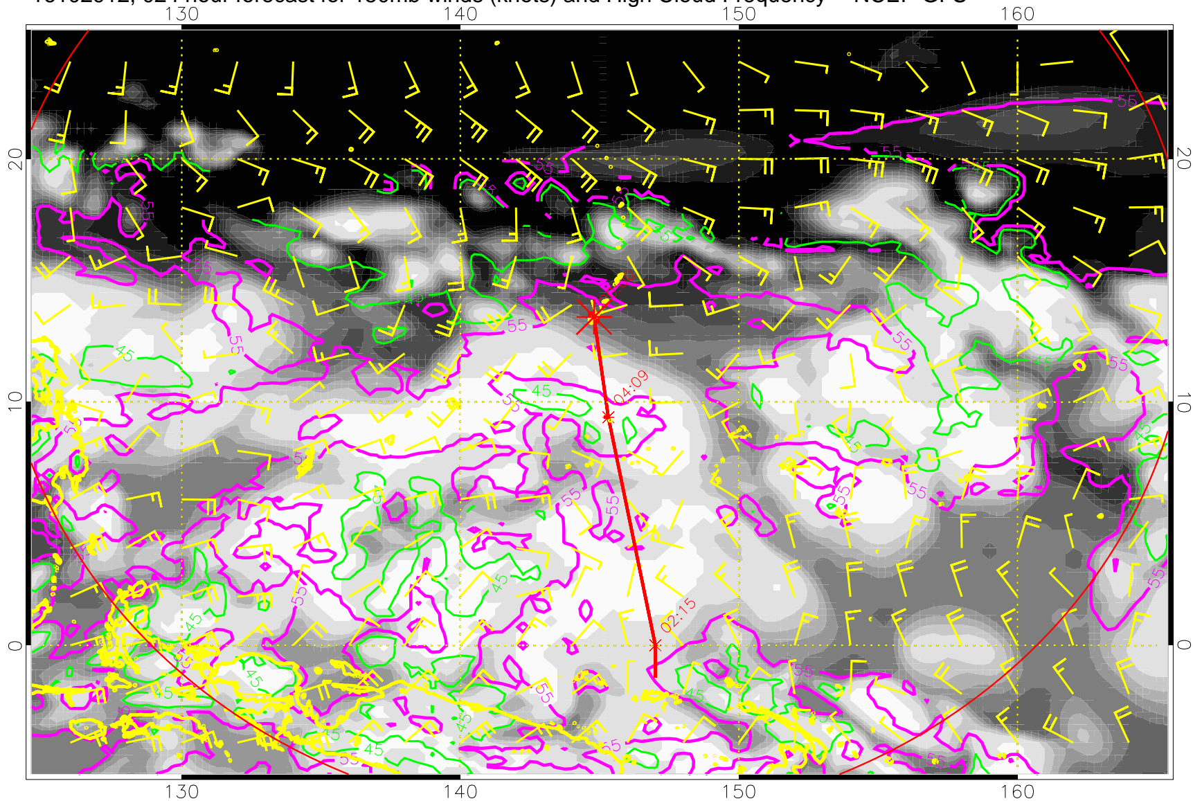
16102912, 024 hour forecast for 150mb winds (knots) and High Cloud Frequency -- NCEP GFS
