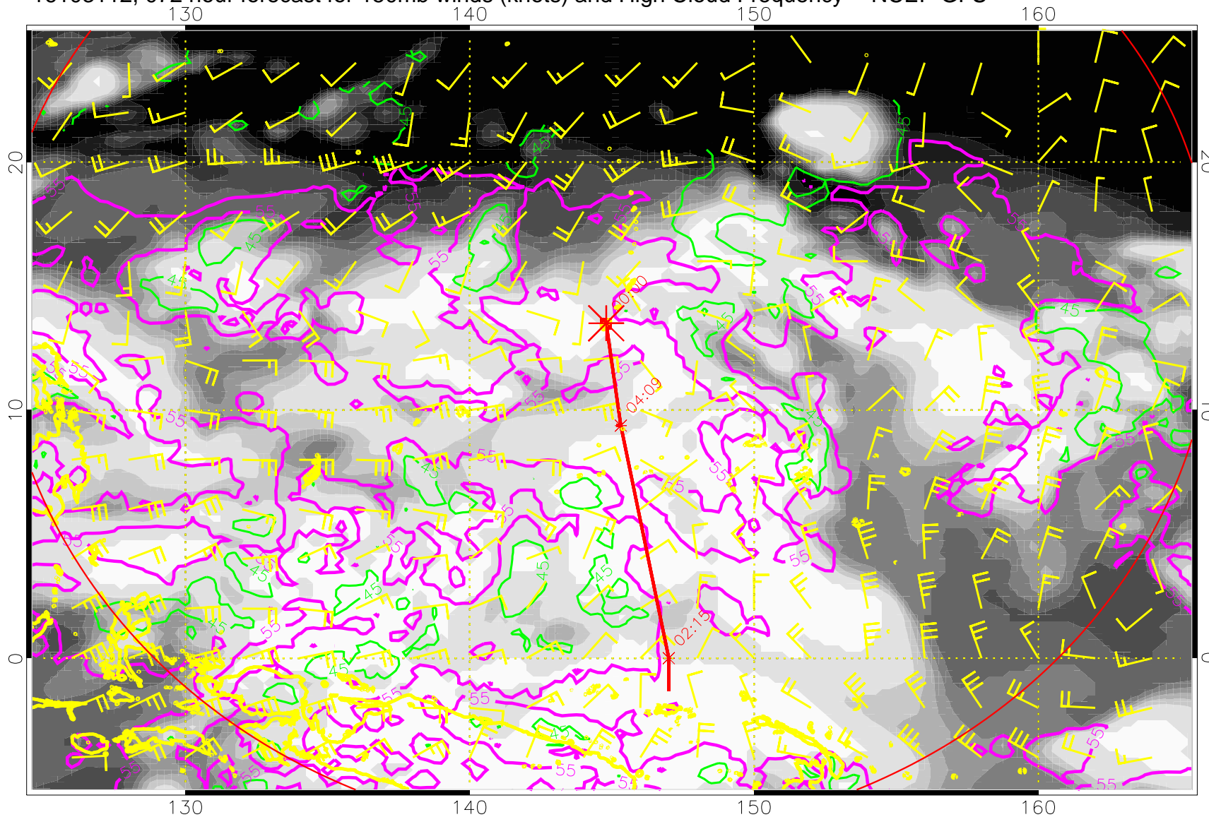
16103112, 072 hour forecast for 150mb winds (knots) and High Cloud Frequency -- NCEP GFS
