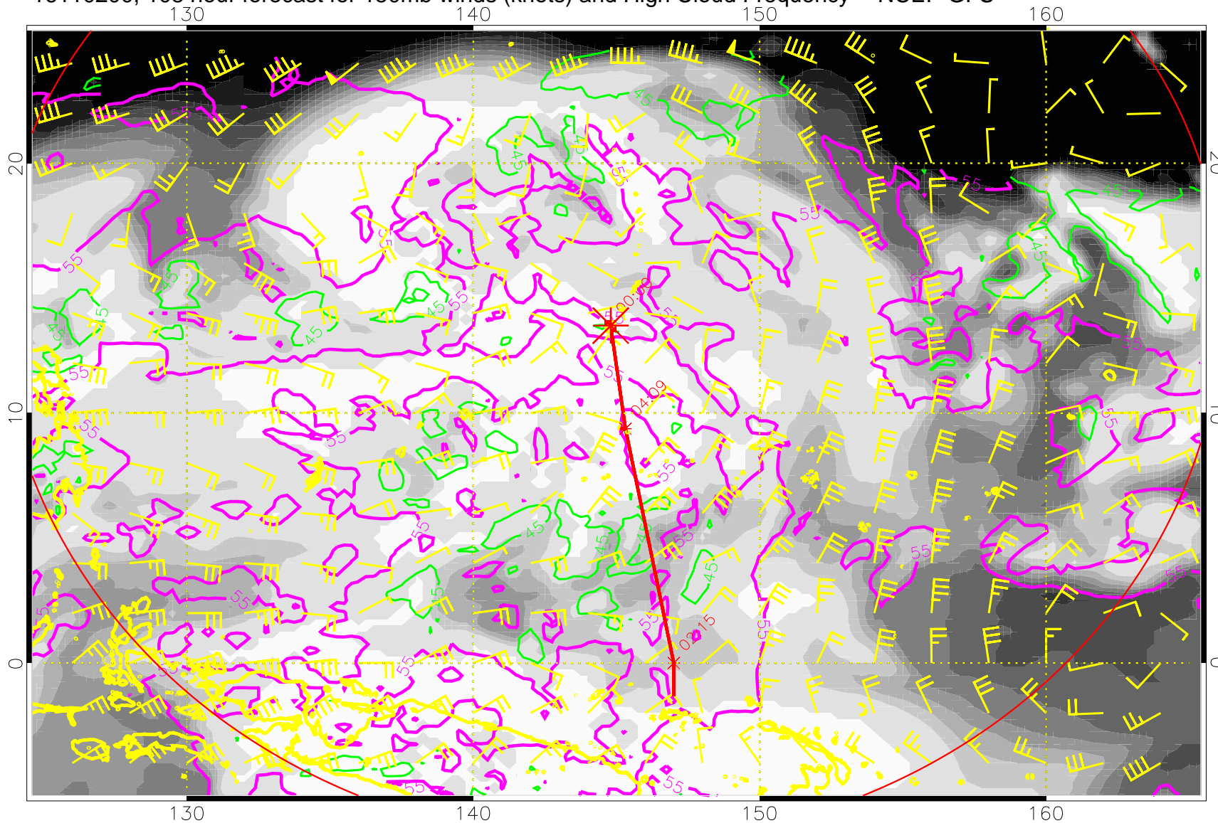
16110200, 108 hour forecast for 150mb winds (knots) and High Cloud Frequency -- NCEP GFS
