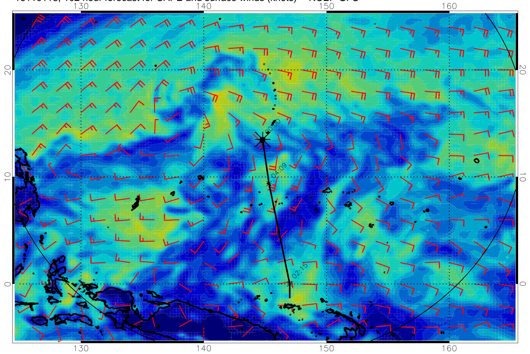
16110118, 102 hour forecast for CAPE and surface winds (knots) -- NCEP GFS
