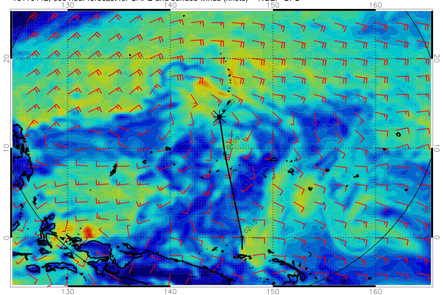
16110112, 096 hour forecast for CAPE and surface winds (knots) -- NCEP GFS
