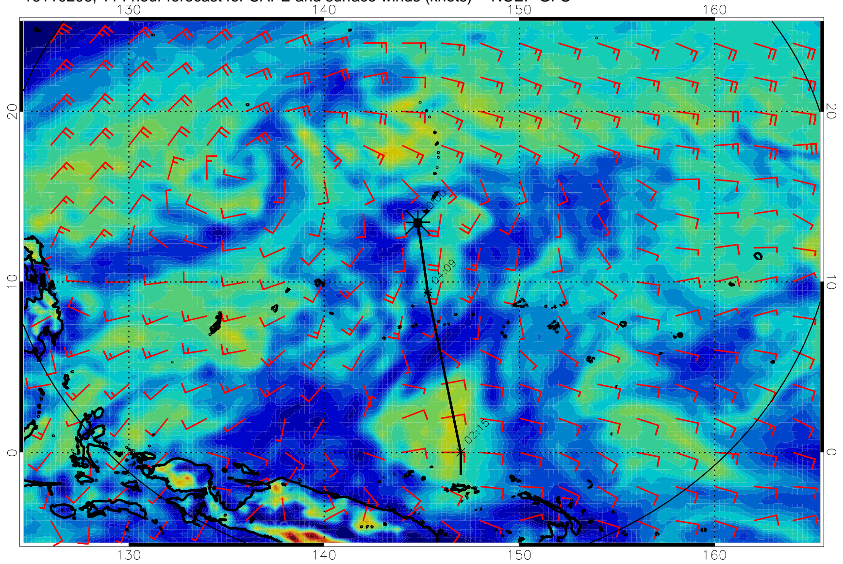
16110206, 114 hour forecast for CAPE and surface winds (knots) -- NCEP GFS
