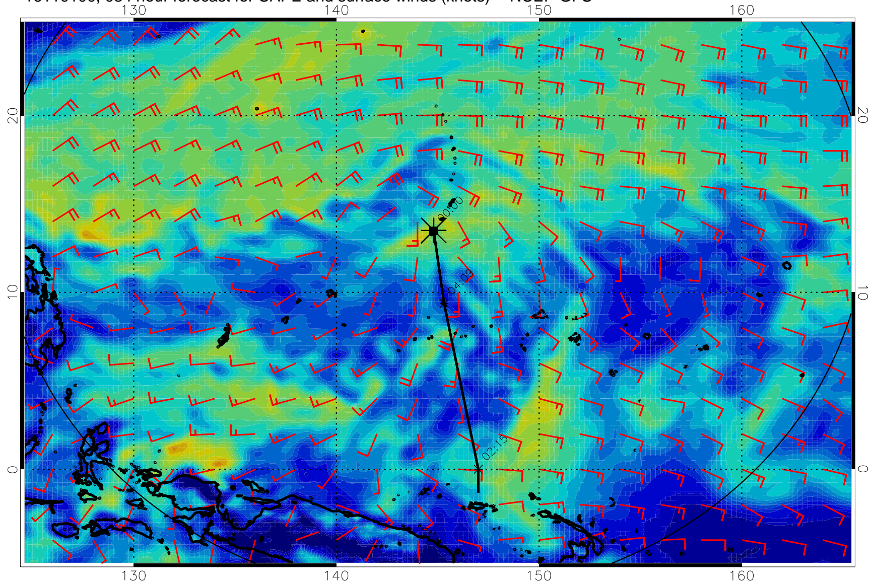
16110100, 084 hour forecast for CAPE and surface winds (knots) -- NCEP GFS
