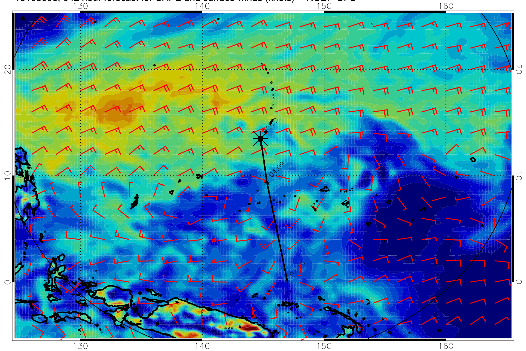
16103006, 042 hour forecast for CAPE and surface winds (knots) -- NCEP GFS
