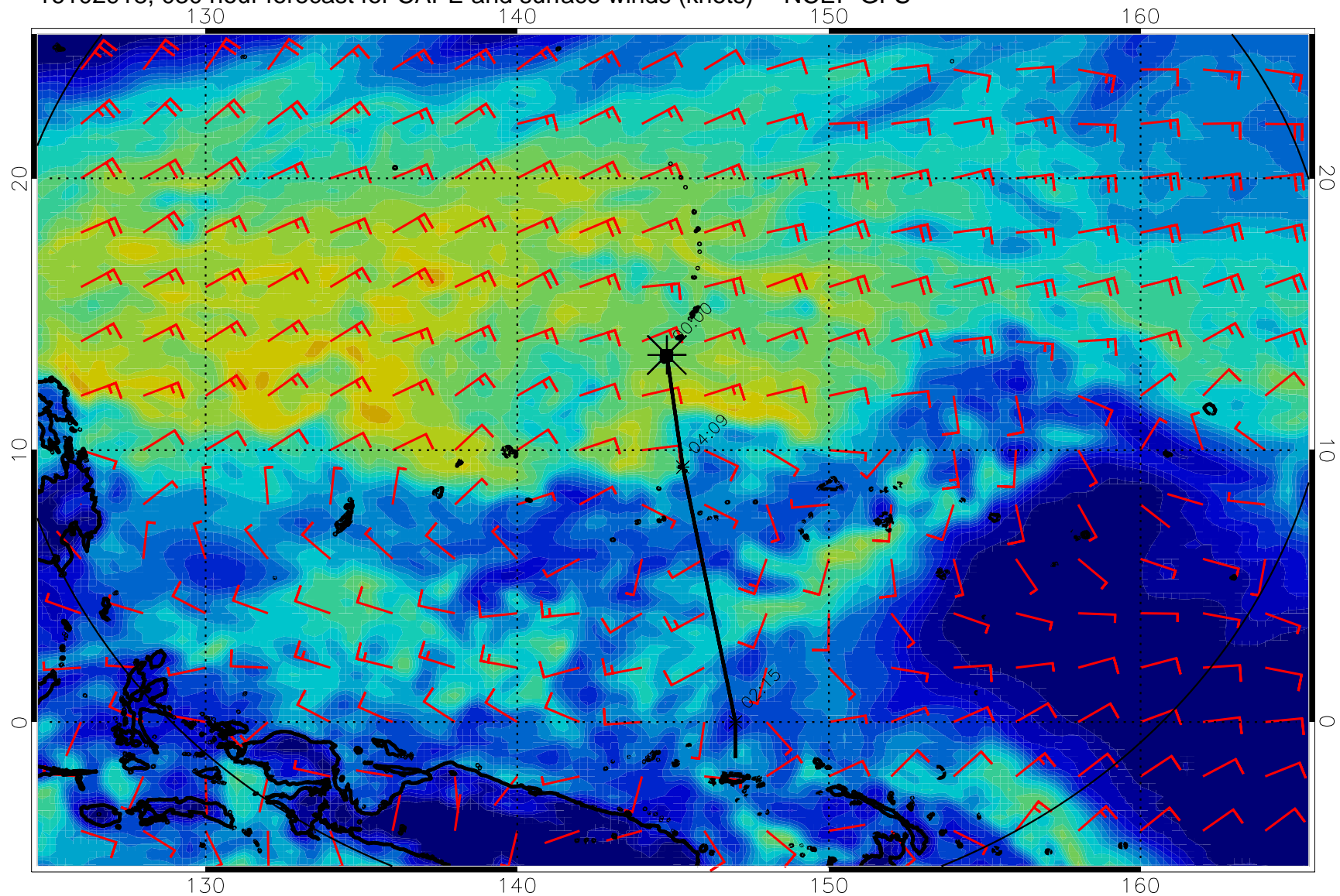
16102918, 030 hour forecast for CAPE and surface winds (knots) -- NCEP GFS
