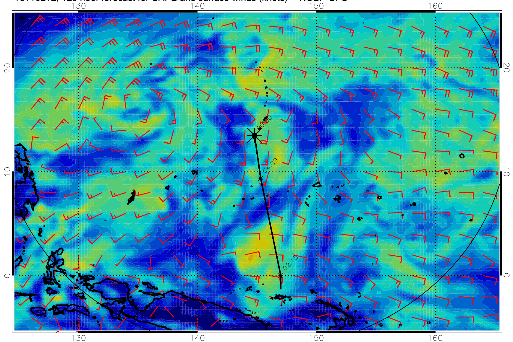
16110212, 120 hour forecast for CAPE and surface winds (knots) -- NCEP GFS
