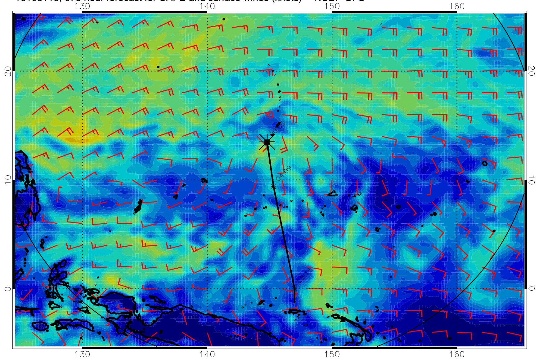
16103118, 078 hour forecast for CAPE and surface winds (knots) -- NCEP GFS
