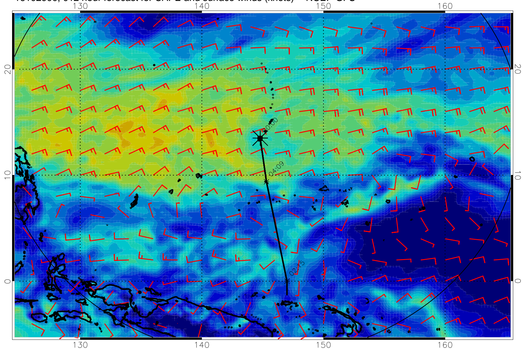
16102900, 012 hour forecast for CAPE and surface winds (knots) -- NCEP GFS
