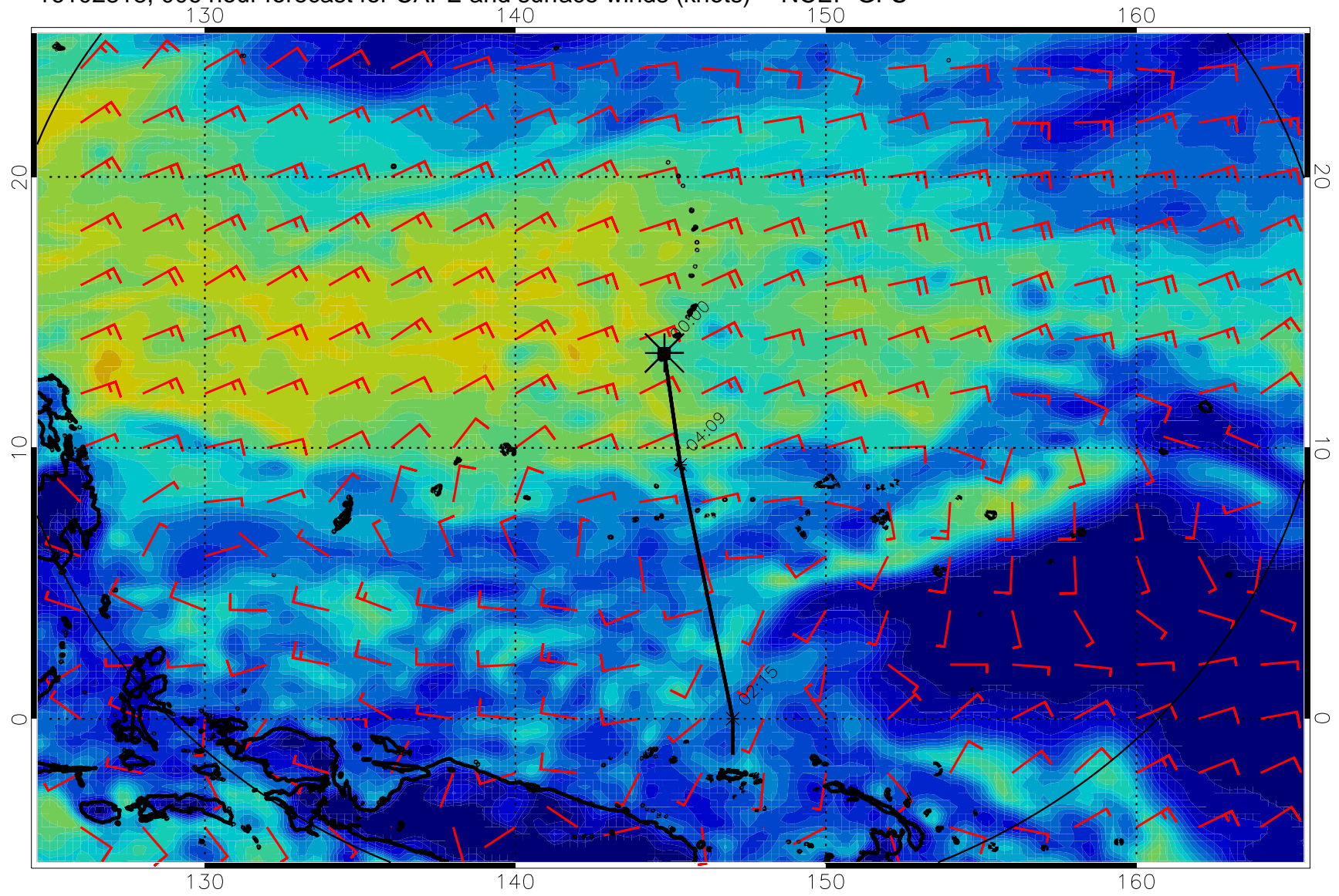
16102818, 006 hour forecast for CAPE and surface winds (knots) -- NCEP GFS
