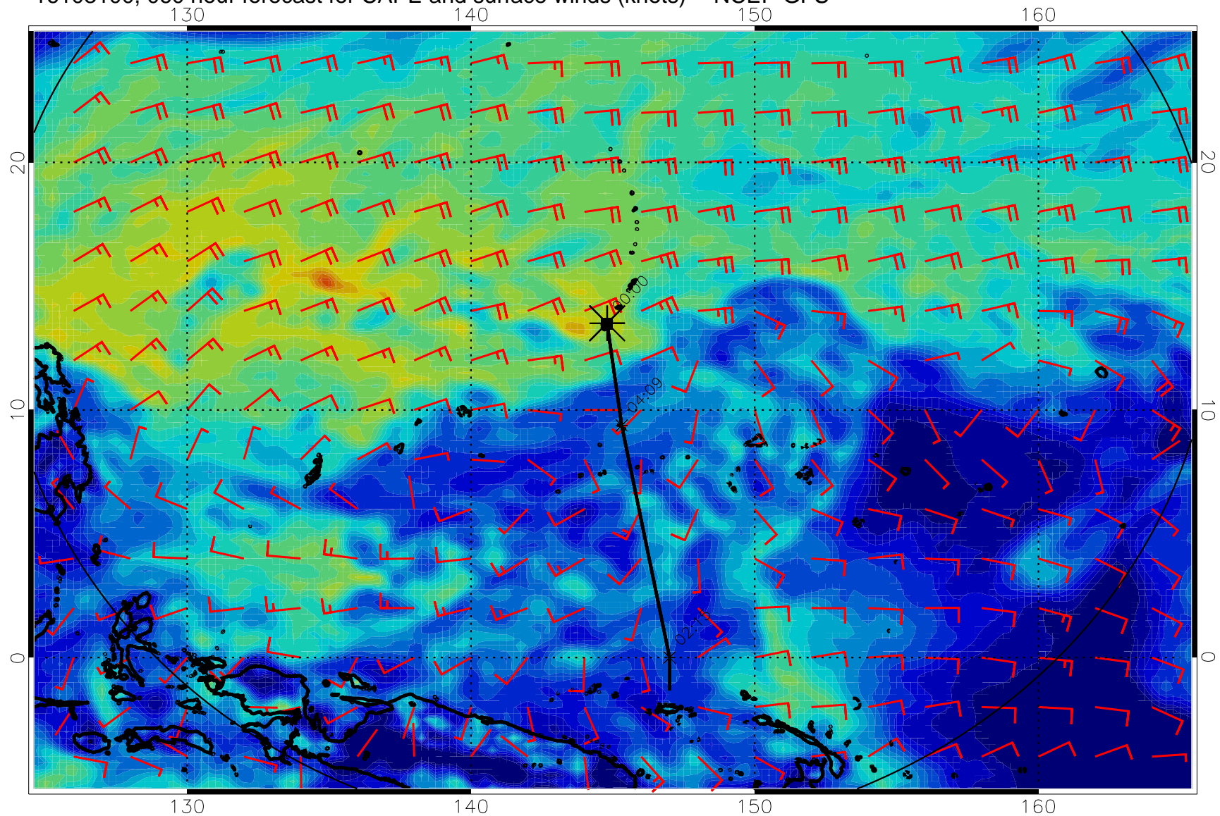
16103100, 060 hour forecast for CAPE and surface winds (knots) -- NCEP GFS
