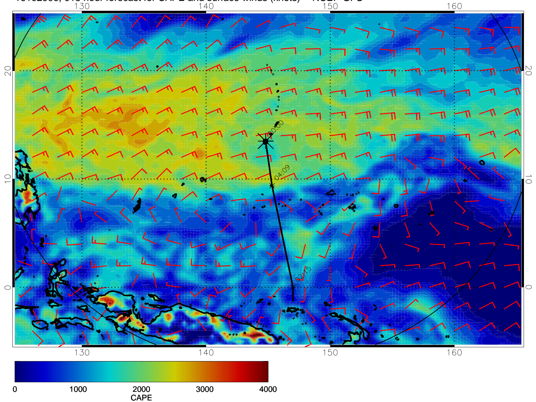
16102906, 018 hour forecast for CAPE and surface winds (knots) -- NCEP GFS
