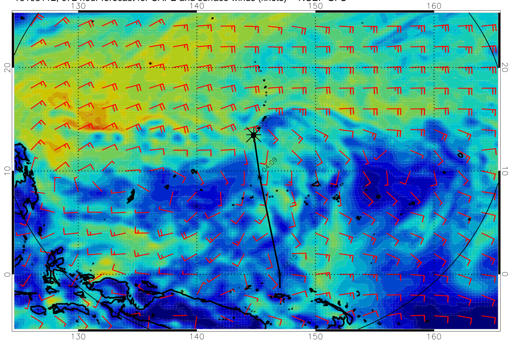
16103112, 072 hour forecast for CAPE and surface winds (knots) -- NCEP GFS
