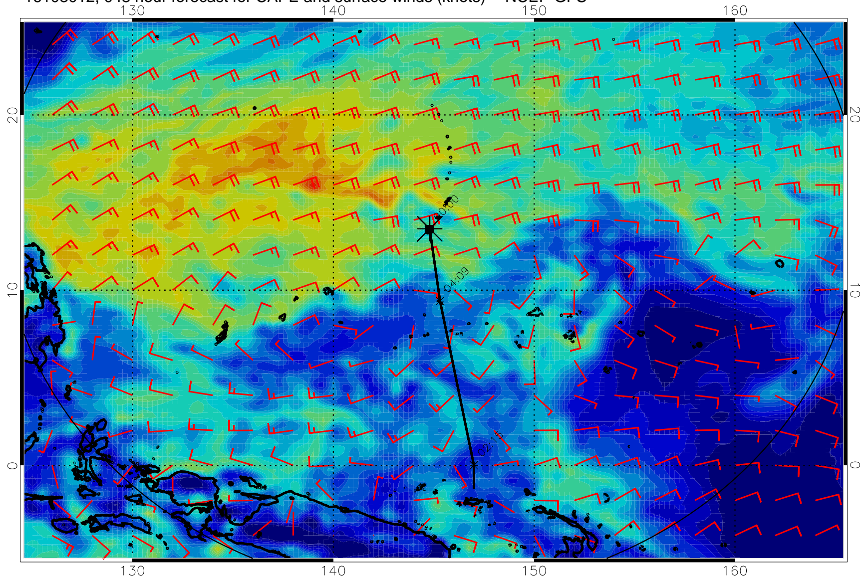
16103012, 048 hour forecast for CAPE and surface winds (knots) -- NCEP GFS
