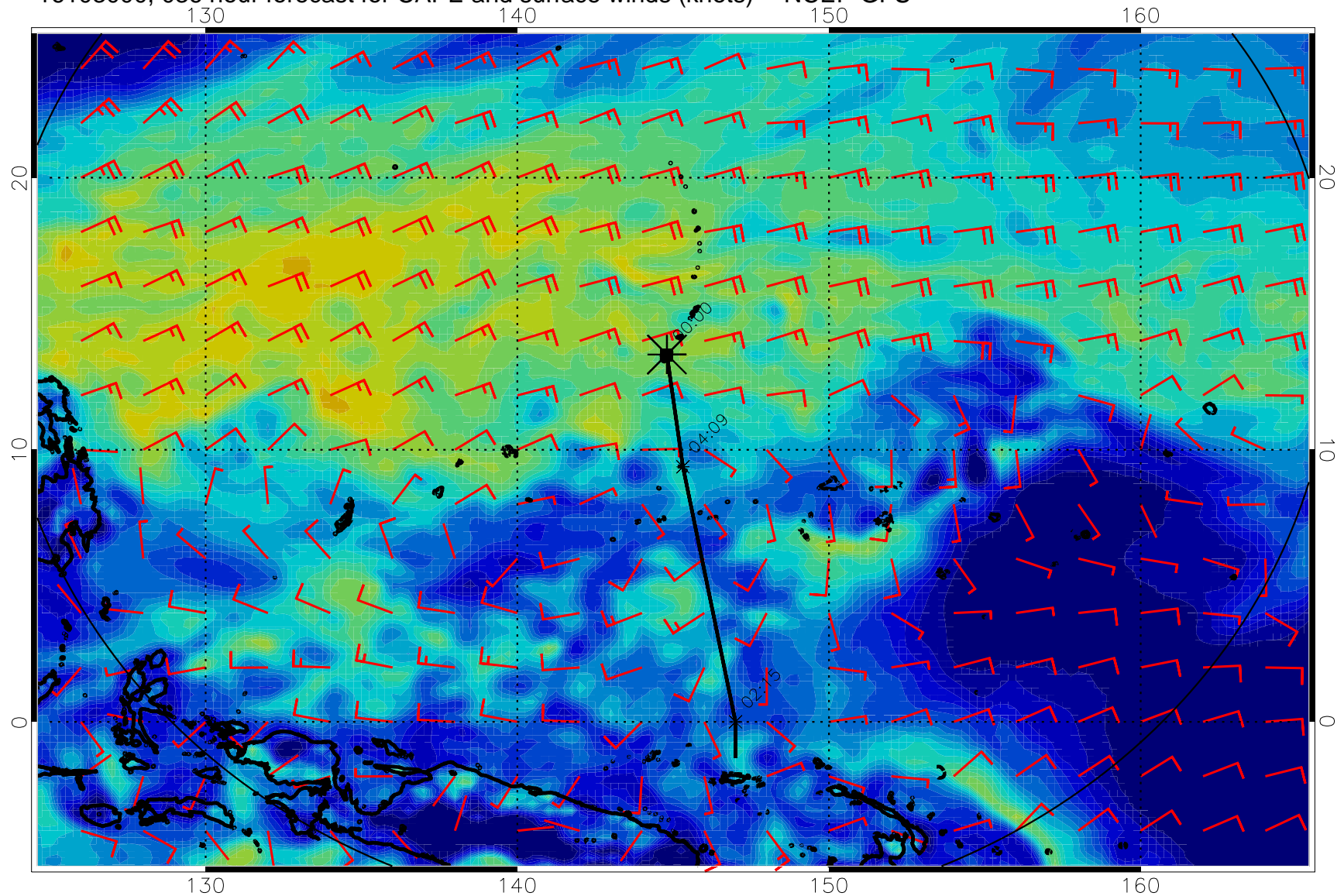
16103000, 036 hour forecast for CAPE and surface winds (knots) -- NCEP GFS
