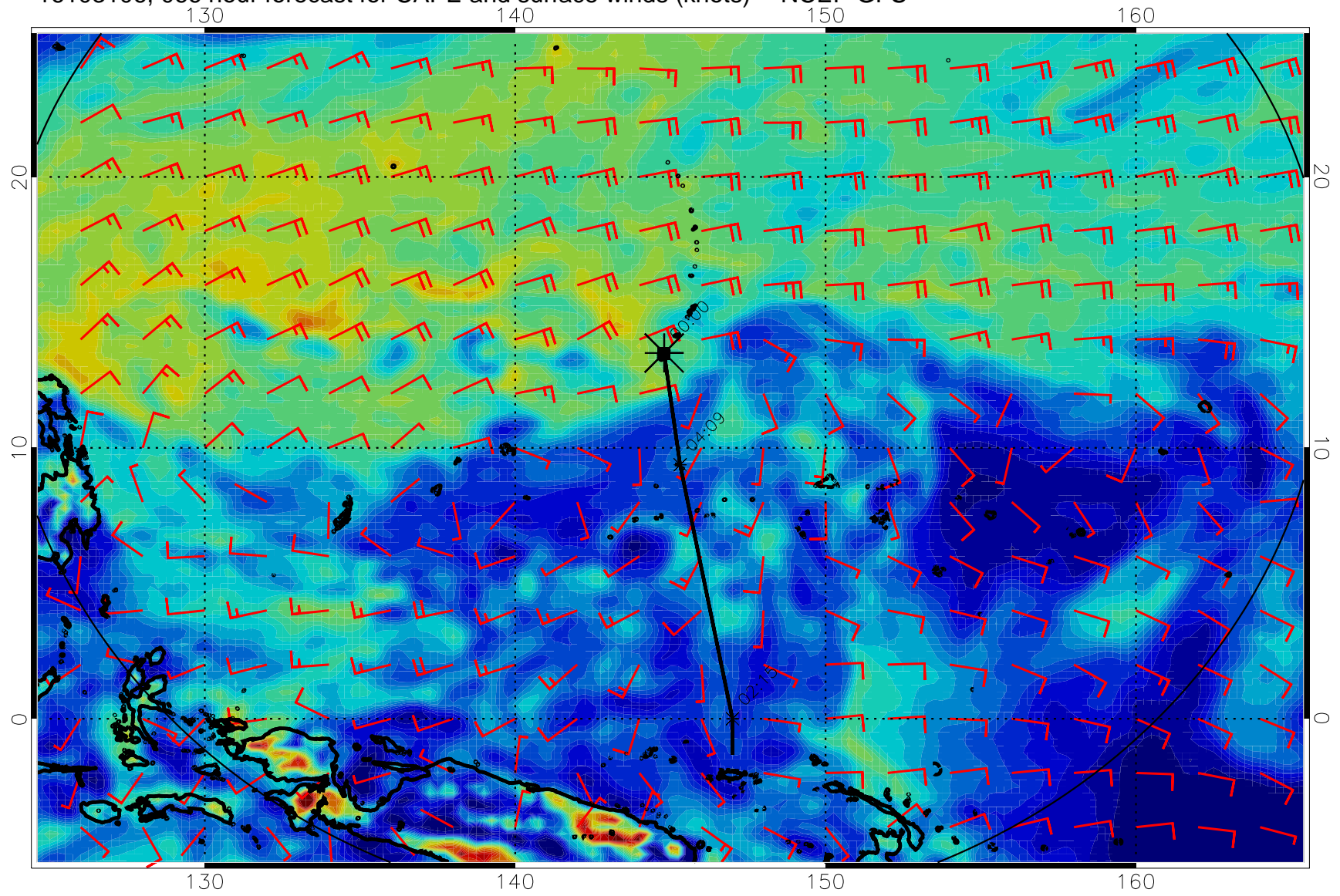
16103106, 066 hour forecast for CAPE and surface winds (knots) -- NCEP GFS
