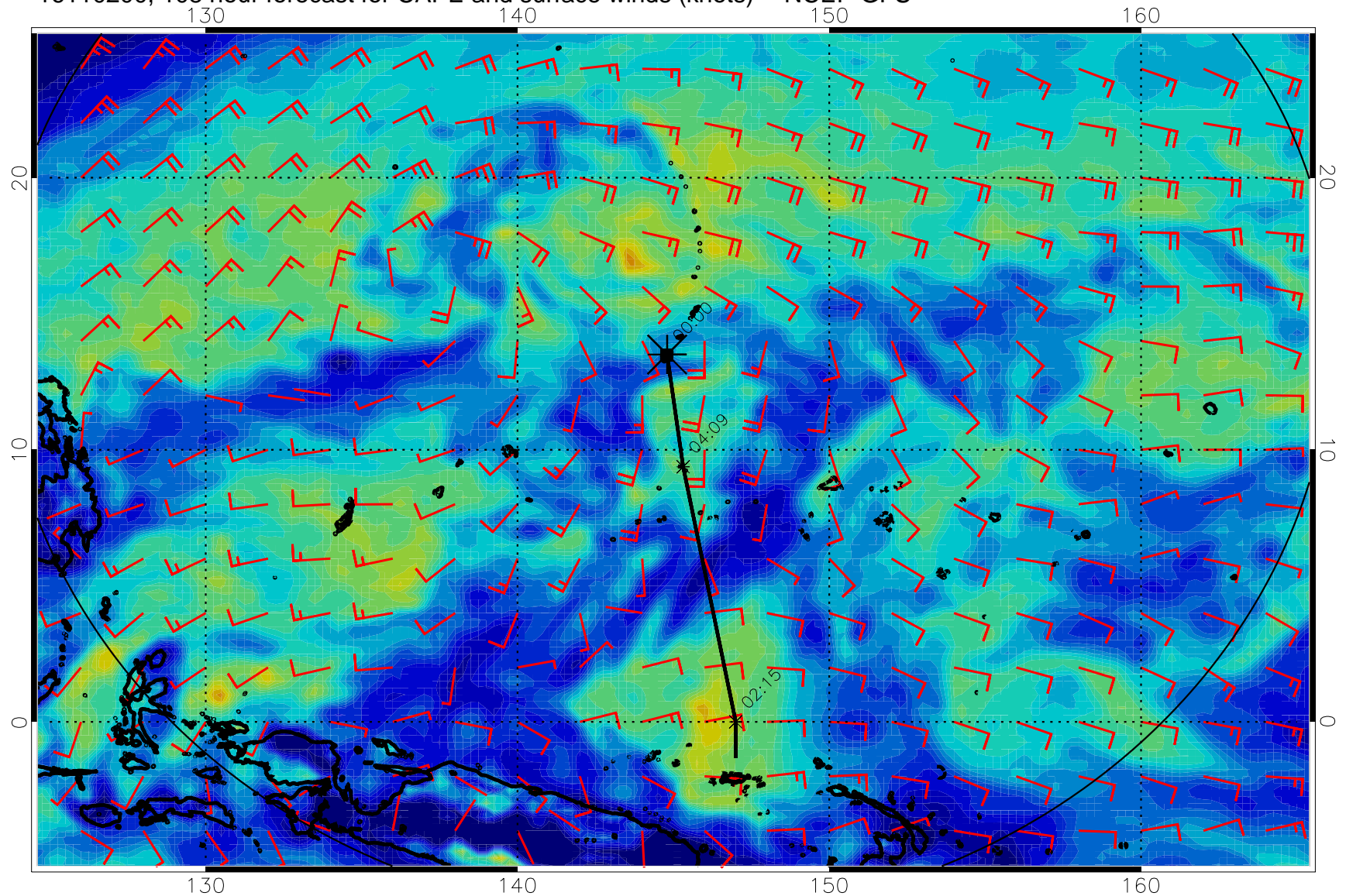
16110200, 108 hour forecast for CAPE and surface winds (knots) -- NCEP GFS
