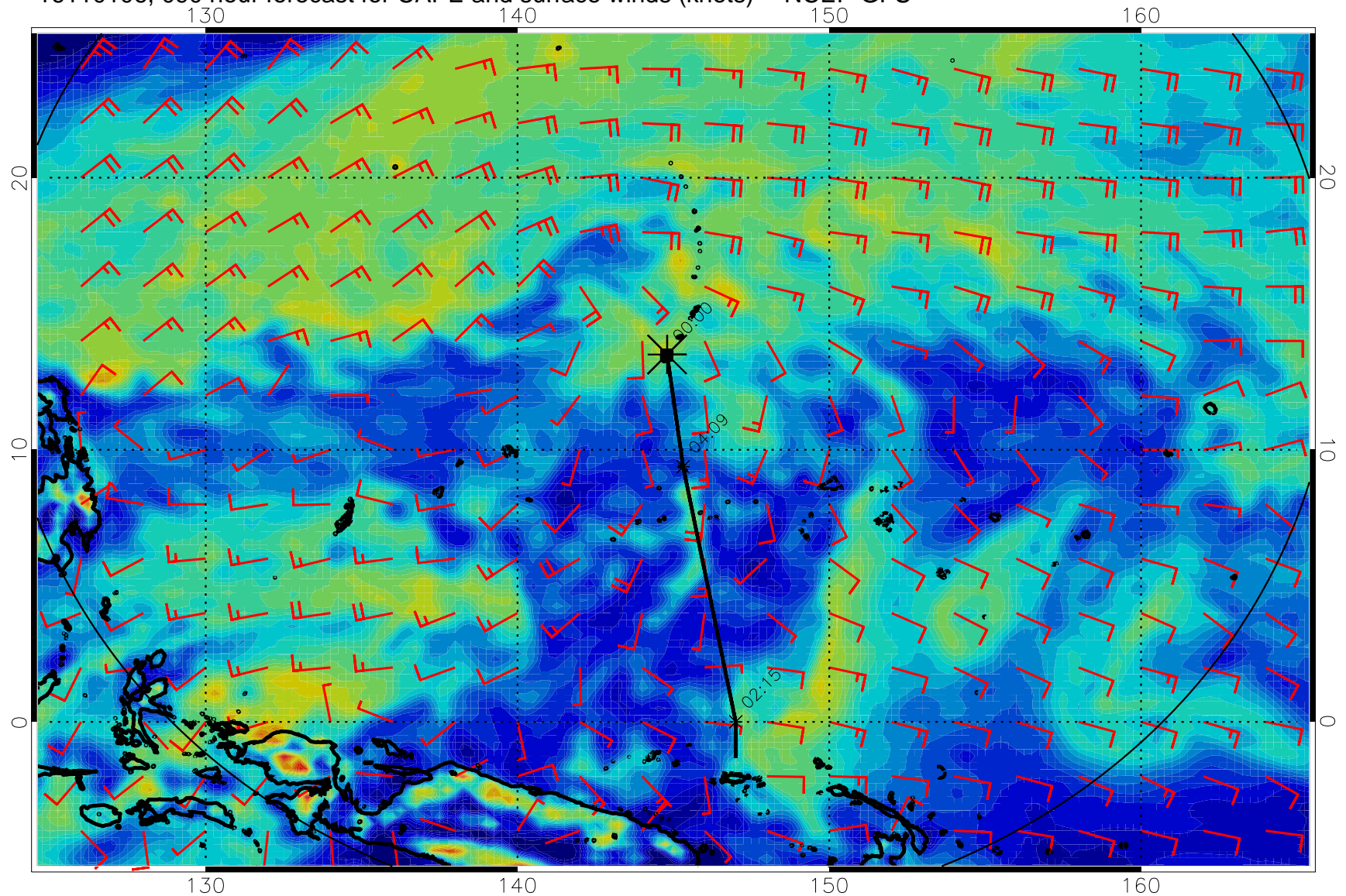
16110106, 090 hour forecast for CAPE and surface winds (knots) -- NCEP GFS
