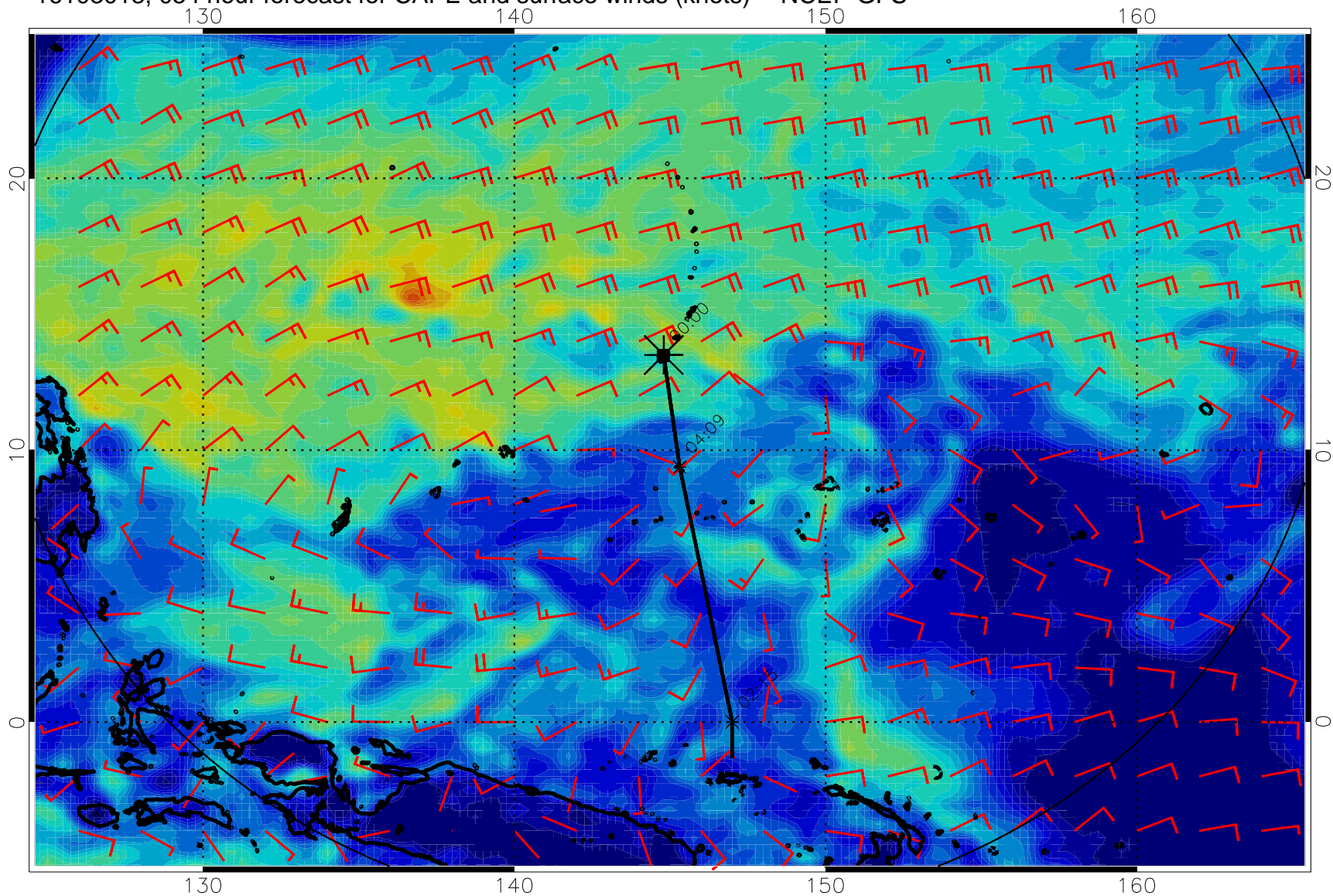
16103018, 054 hour forecast for CAPE and surface winds (knots) -- NCEP GFS
