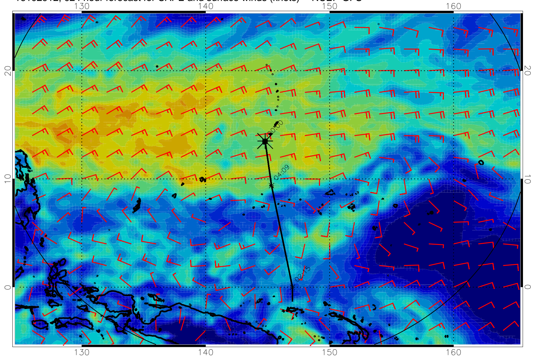
16102912, 024 hour forecast for CAPE and surface winds (knots) -- NCEP GFS
