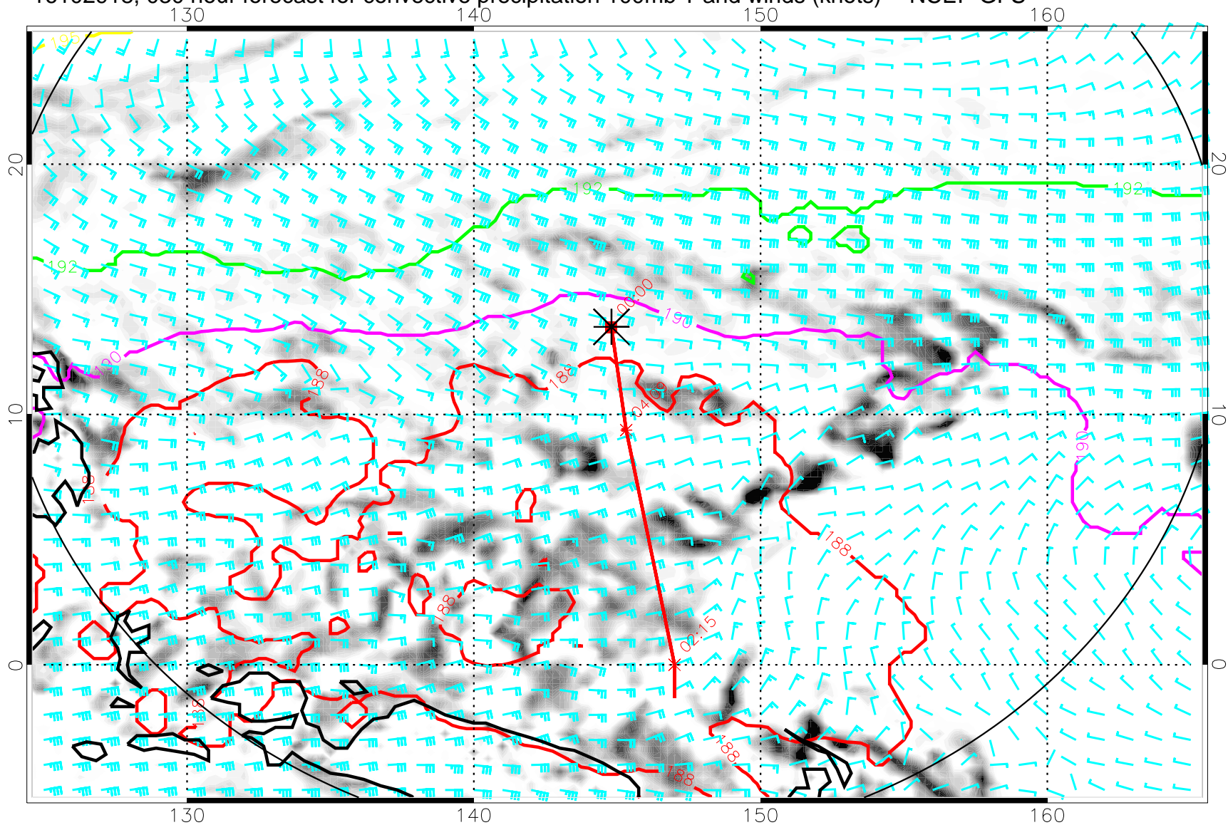
16102918, 030 hour forecast for convective precipitation 100mb T and winds (knots) -- NCEP GFS
