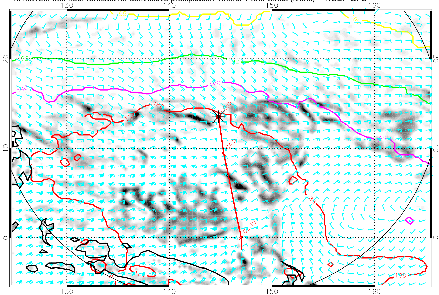
16103106, 066 hour forecast for convective precipitation 100mb T and winds (knots) -- NCEP GFS
