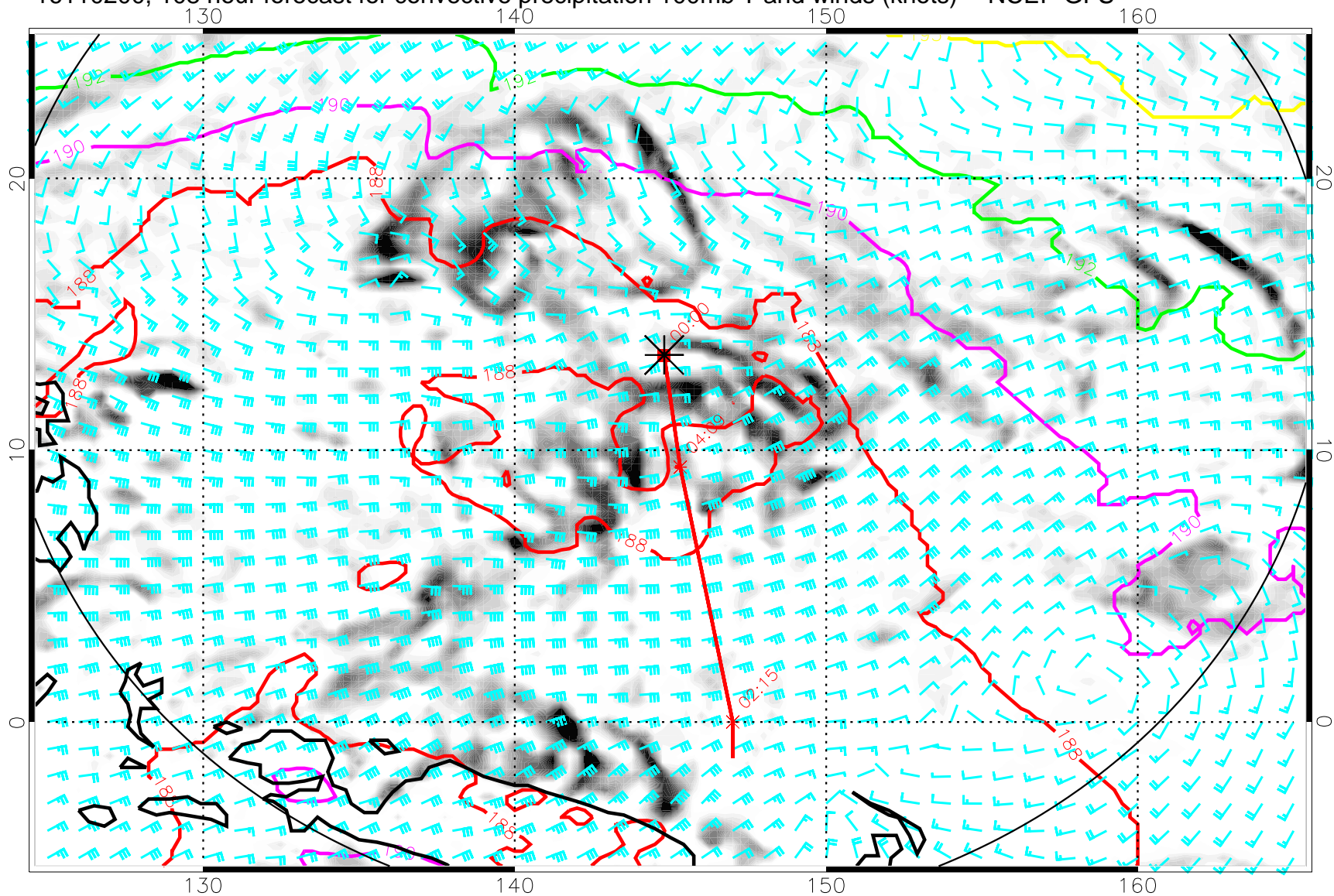
16110200, 108 hour forecast for convective precipitation 100mb T and winds (knots) -- NCEP GFS
