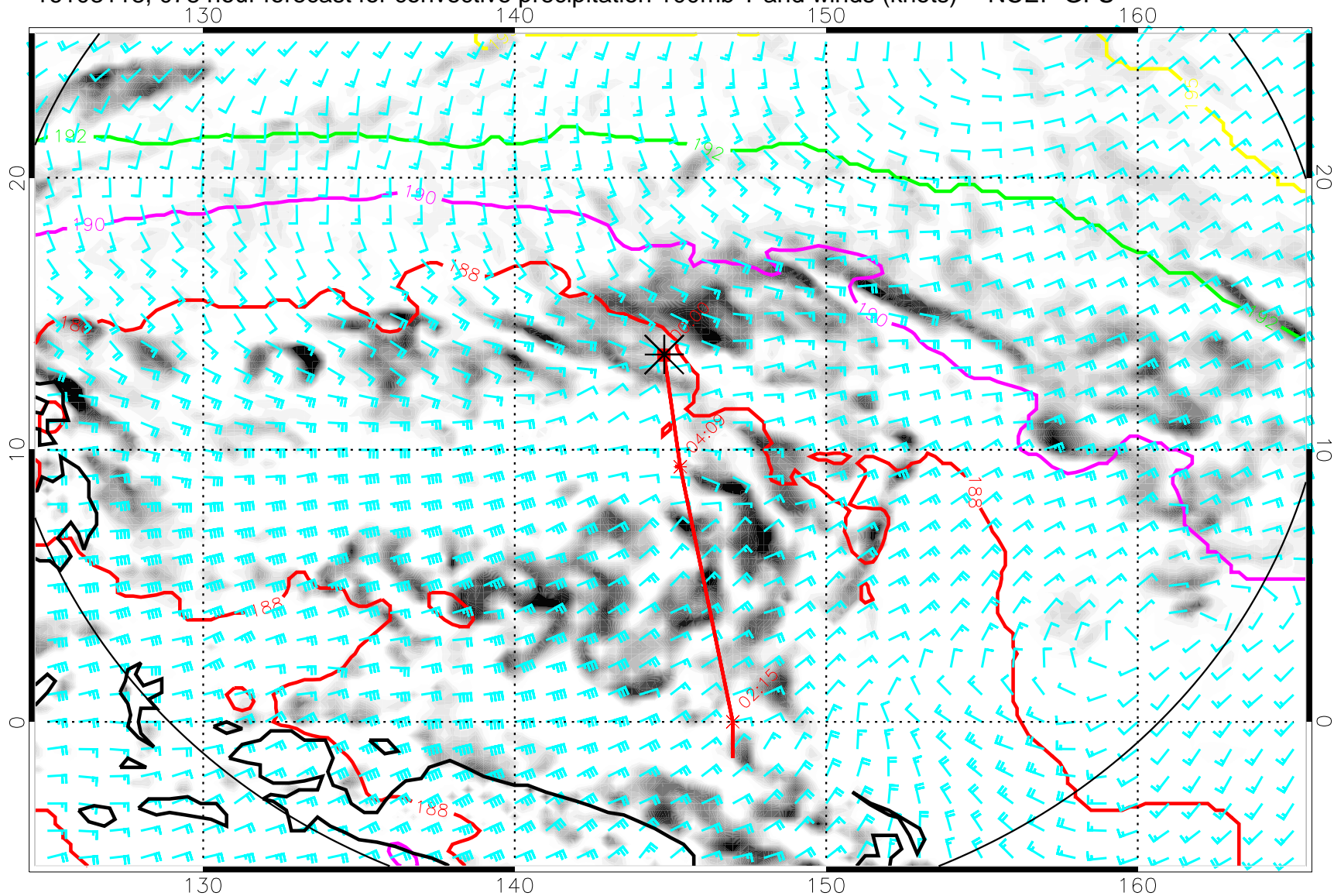
16103118, 078 hour forecast for convective precipitation 100mb T and winds (knots) -- NCEP GFS
