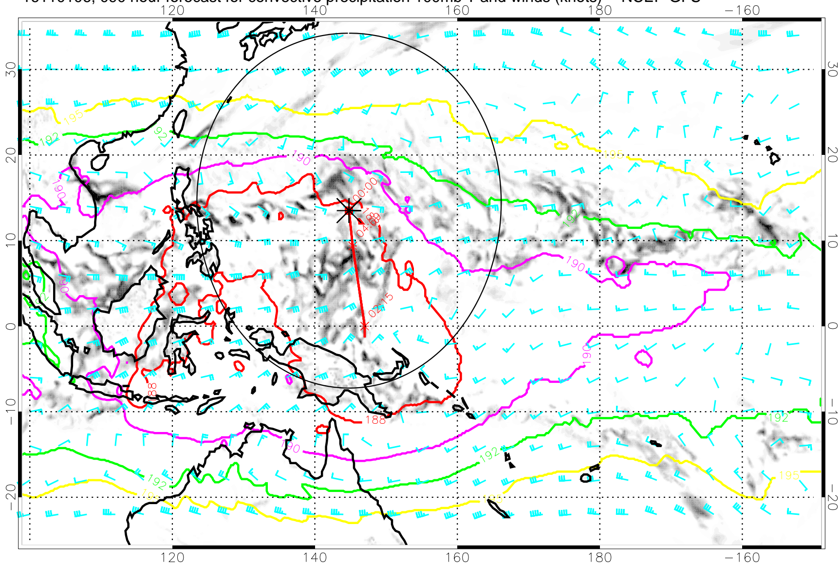
16110106, 090 hour forecast for convective precipitation 100mb T and winds (knots) -- NCEP GFS
