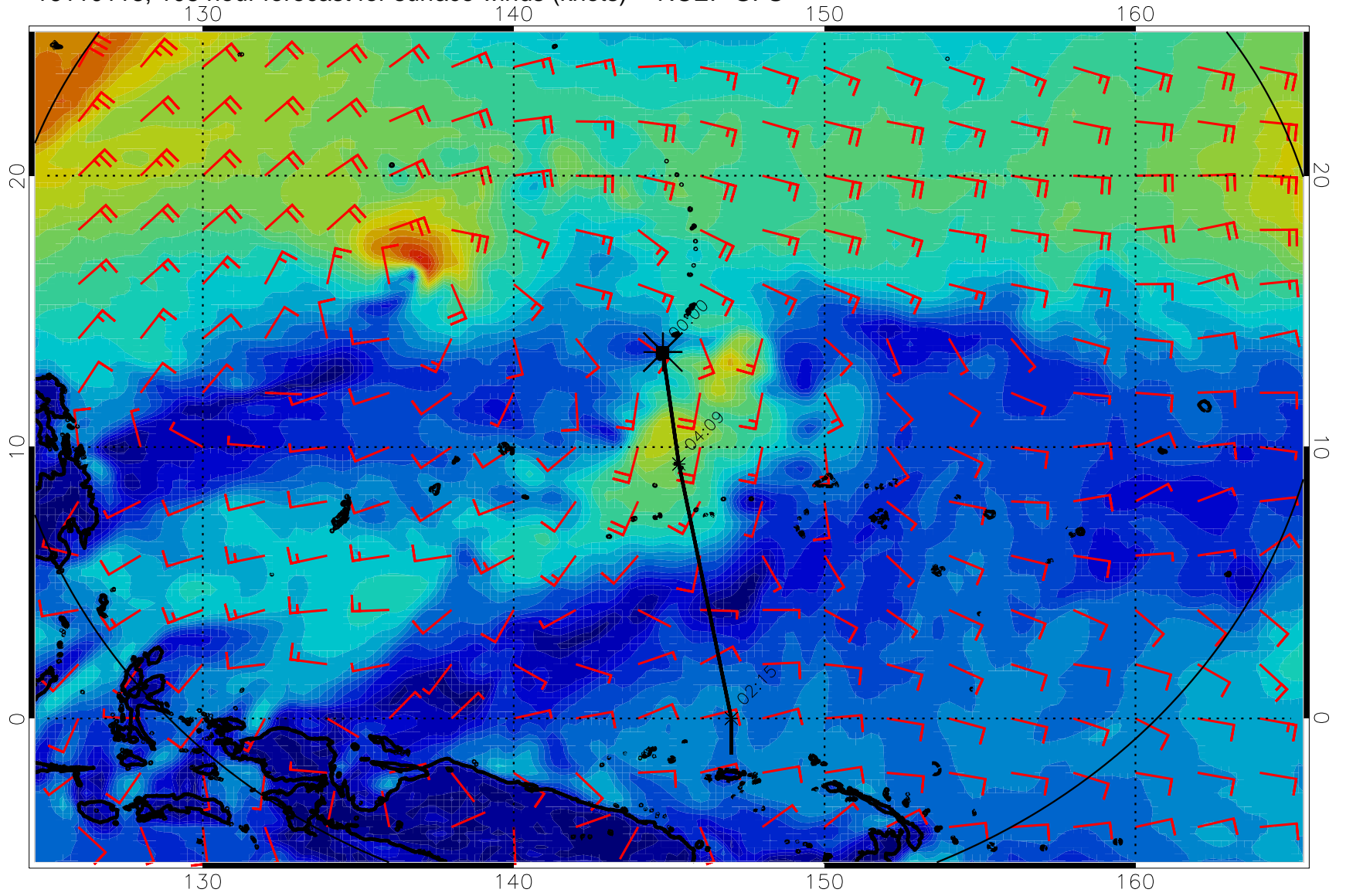
16110118, 108 hour forecast for surface winds (knots) -- NCEP GFS
