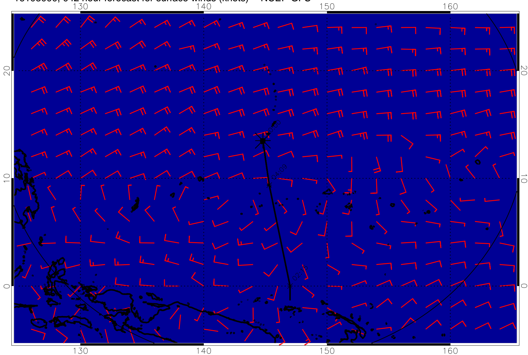
16103000, 042 hour forecast for surface winds (knots) -- NCEP GFS
