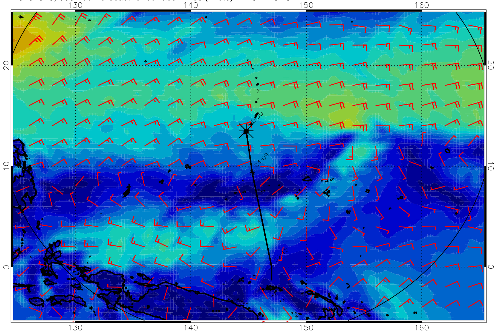
16102918, 036 hour forecast for surface winds (knots) -- NCEP GFS
