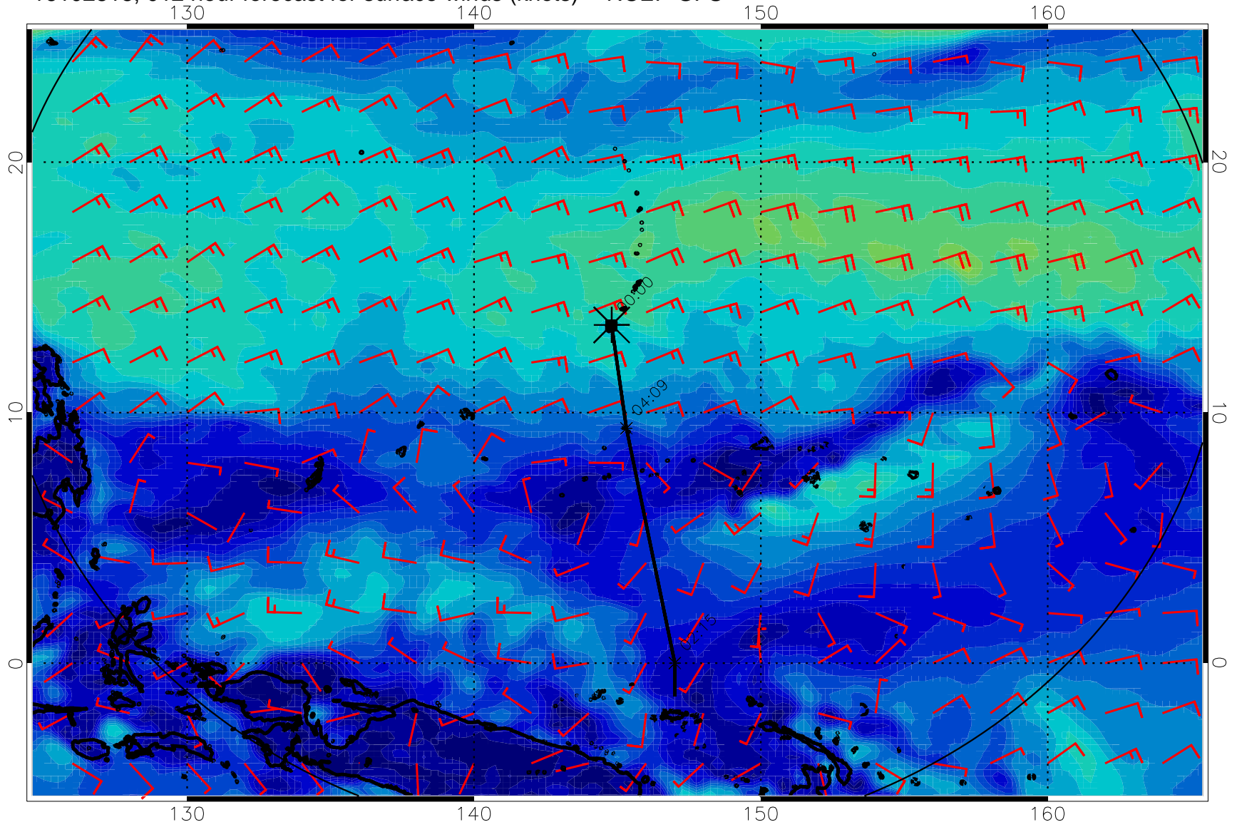
16102818, 012 hour forecast for surface winds (knots) -- NCEP GFS
