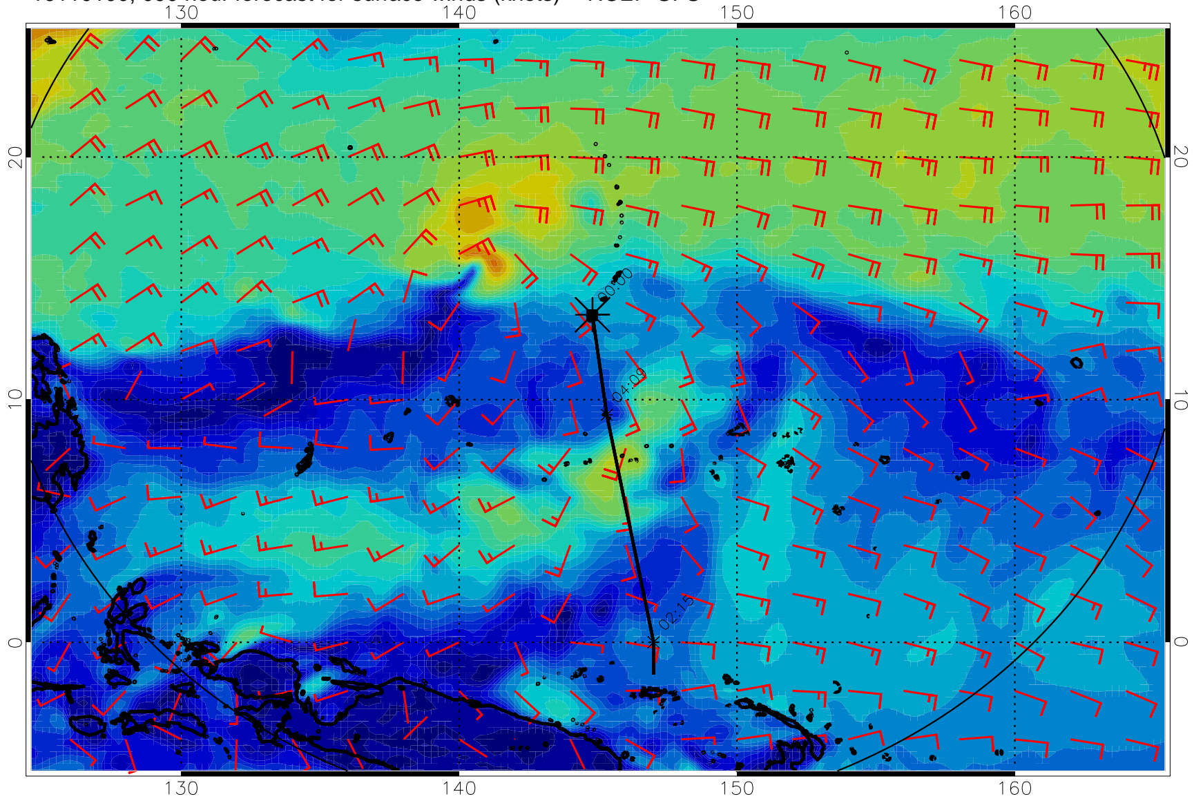
16110100, 090 hour forecast for surface winds (knots) -- NCEP GFS
