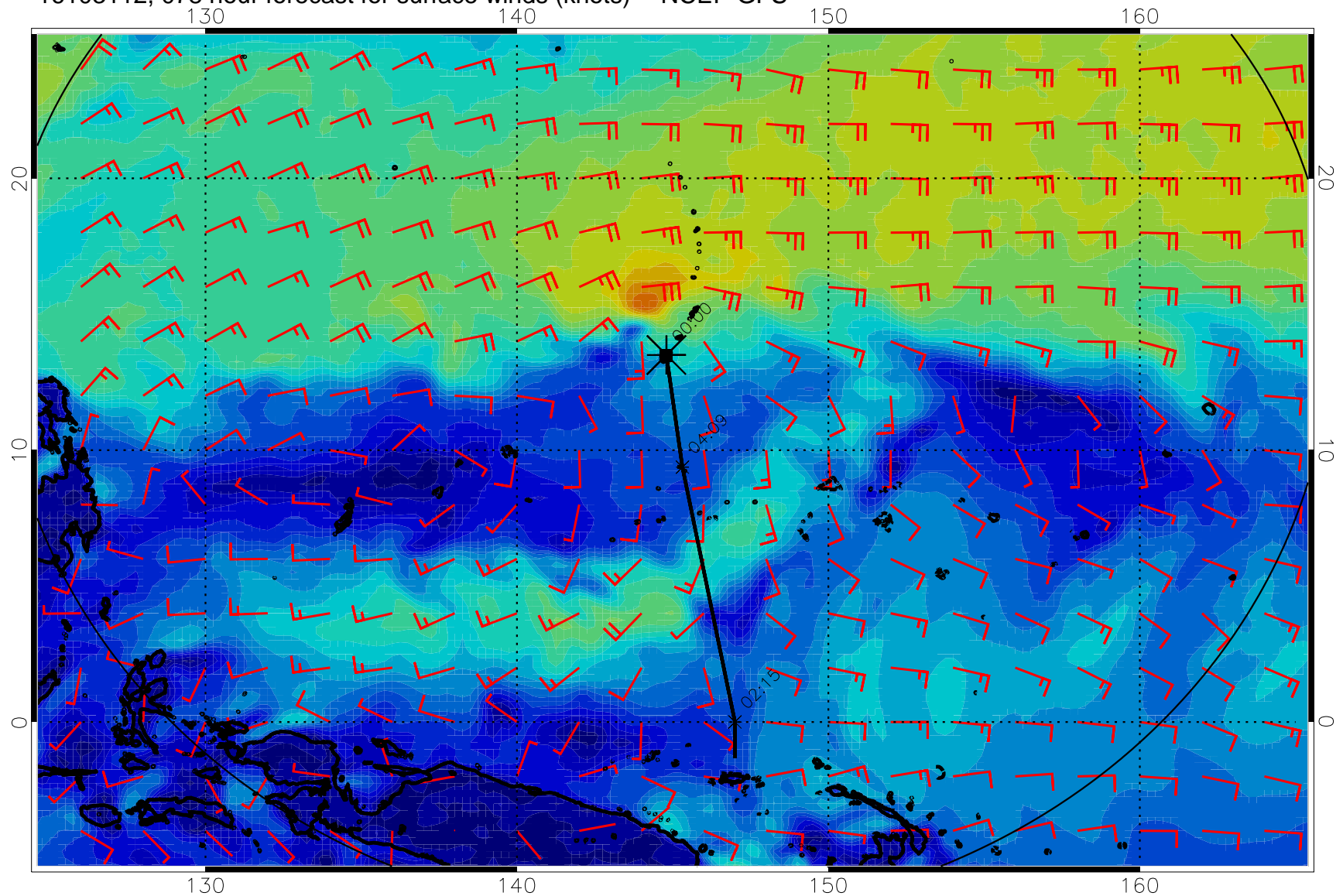
16103112, 078 hour forecast for surface winds (knots) -- NCEP GFS
