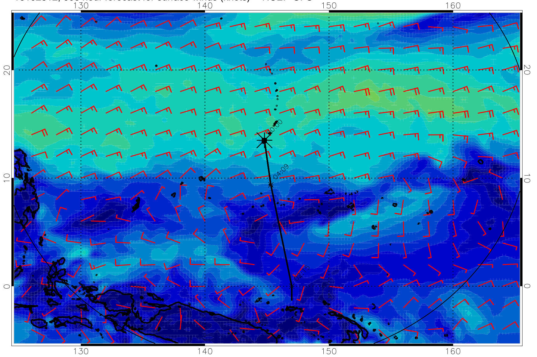
16102812, 006 hour forecast for surface winds (knots) -- NCEP GFS
