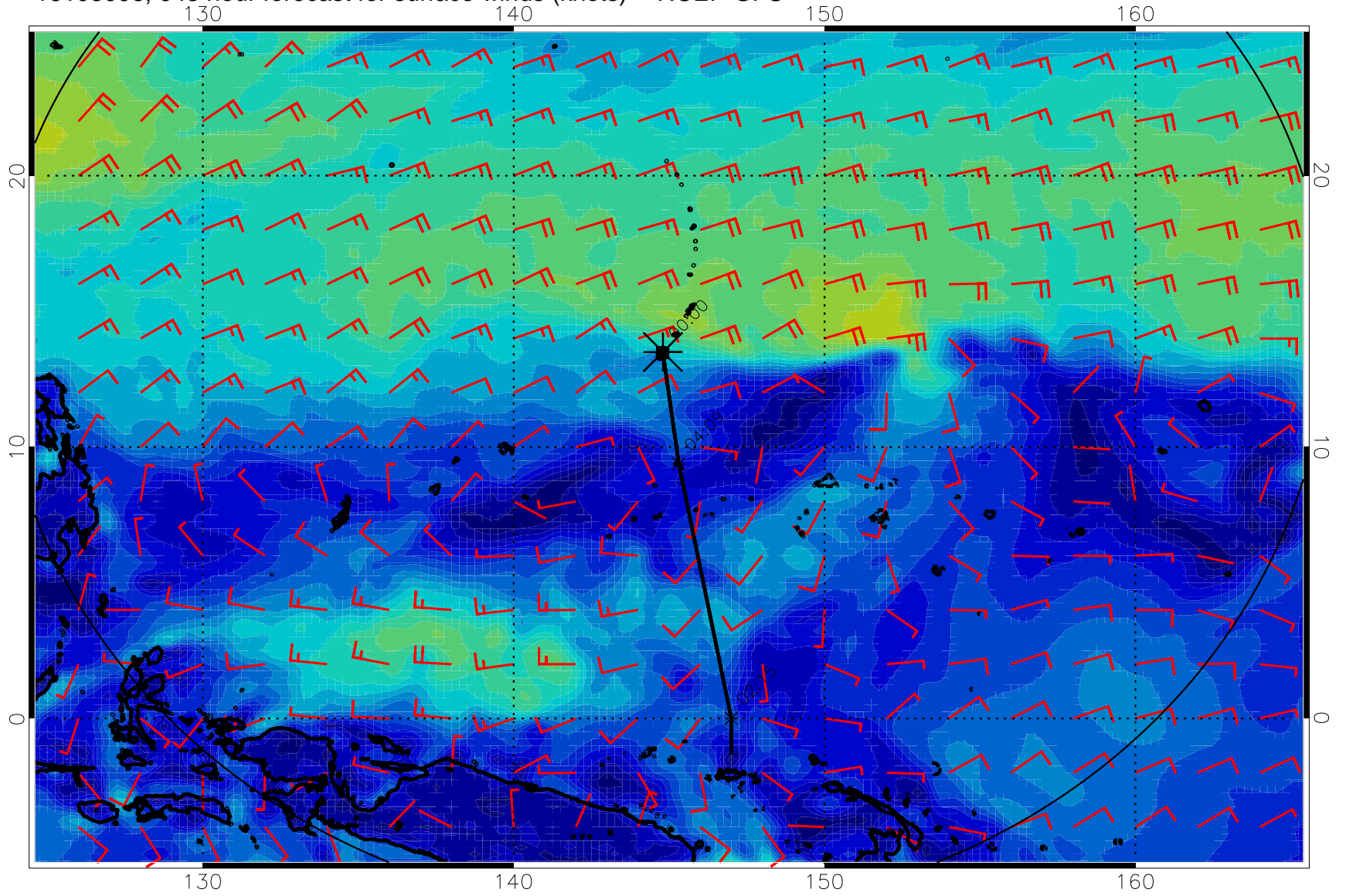
16103006, 048 hour forecast for surface winds (knots) -- NCEP GFS
