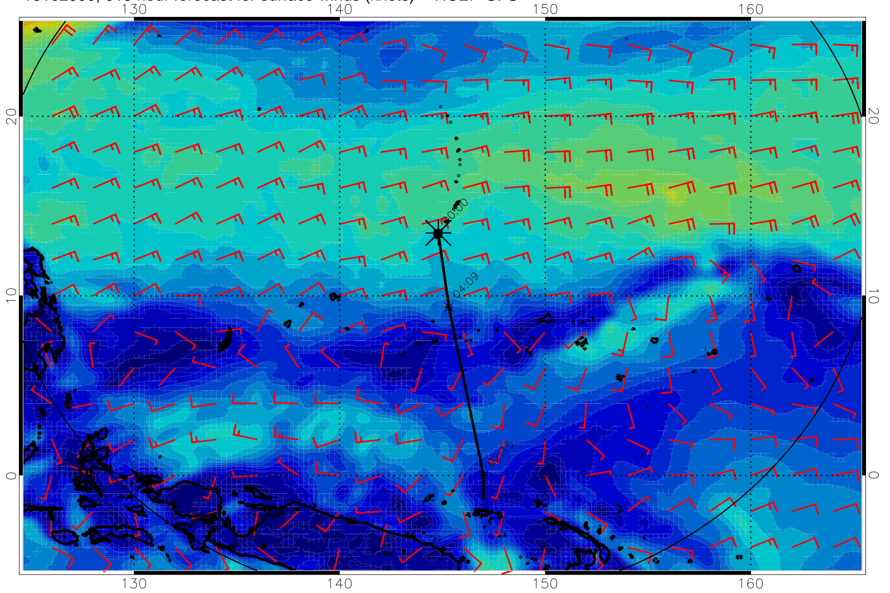
16102900, 018 hour forecast for surface winds (knots) -- NCEP GFS
