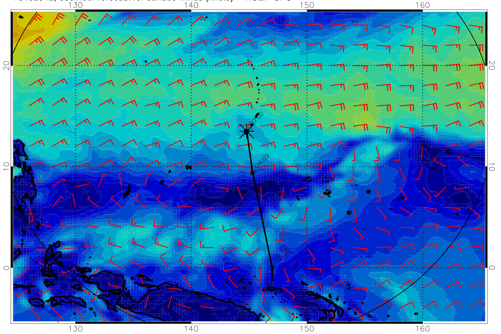
16102912, 030 hour forecast for surface winds (knots) -- NCEP GFS
