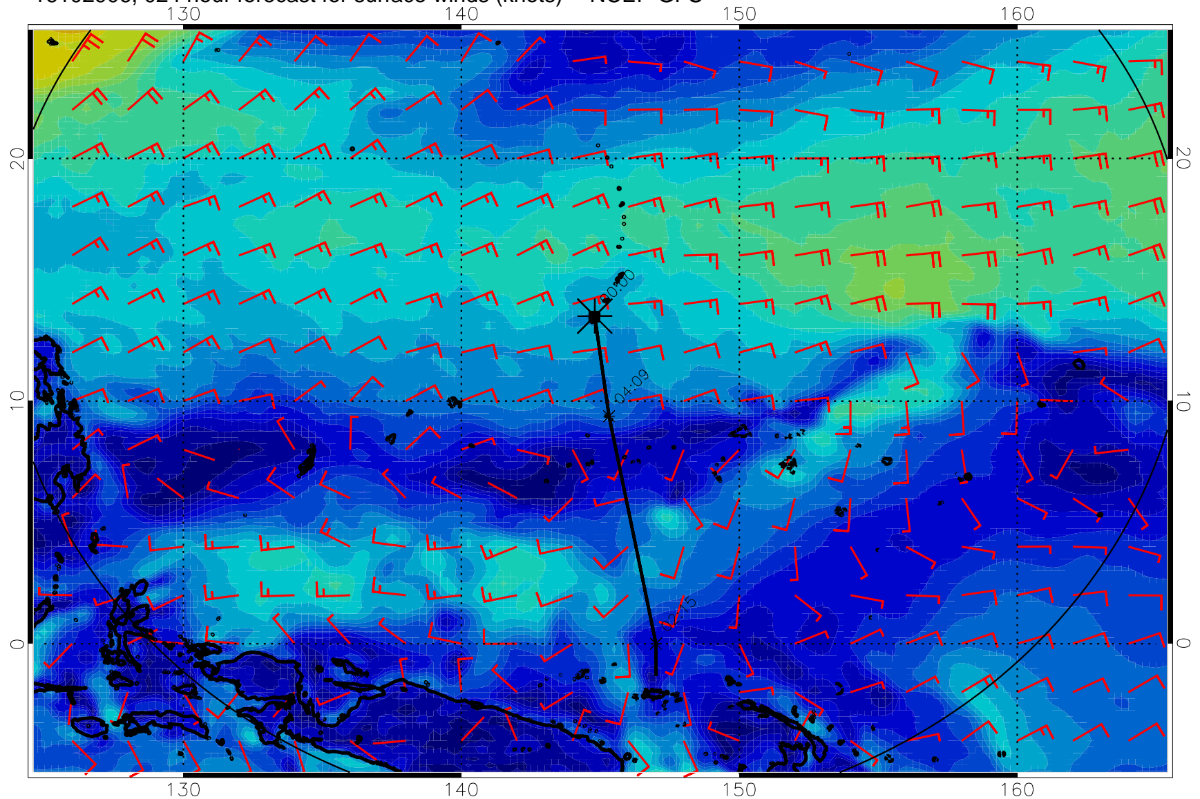
16102906, 024 hour forecast for surface winds (knots) -- NCEP GFS
