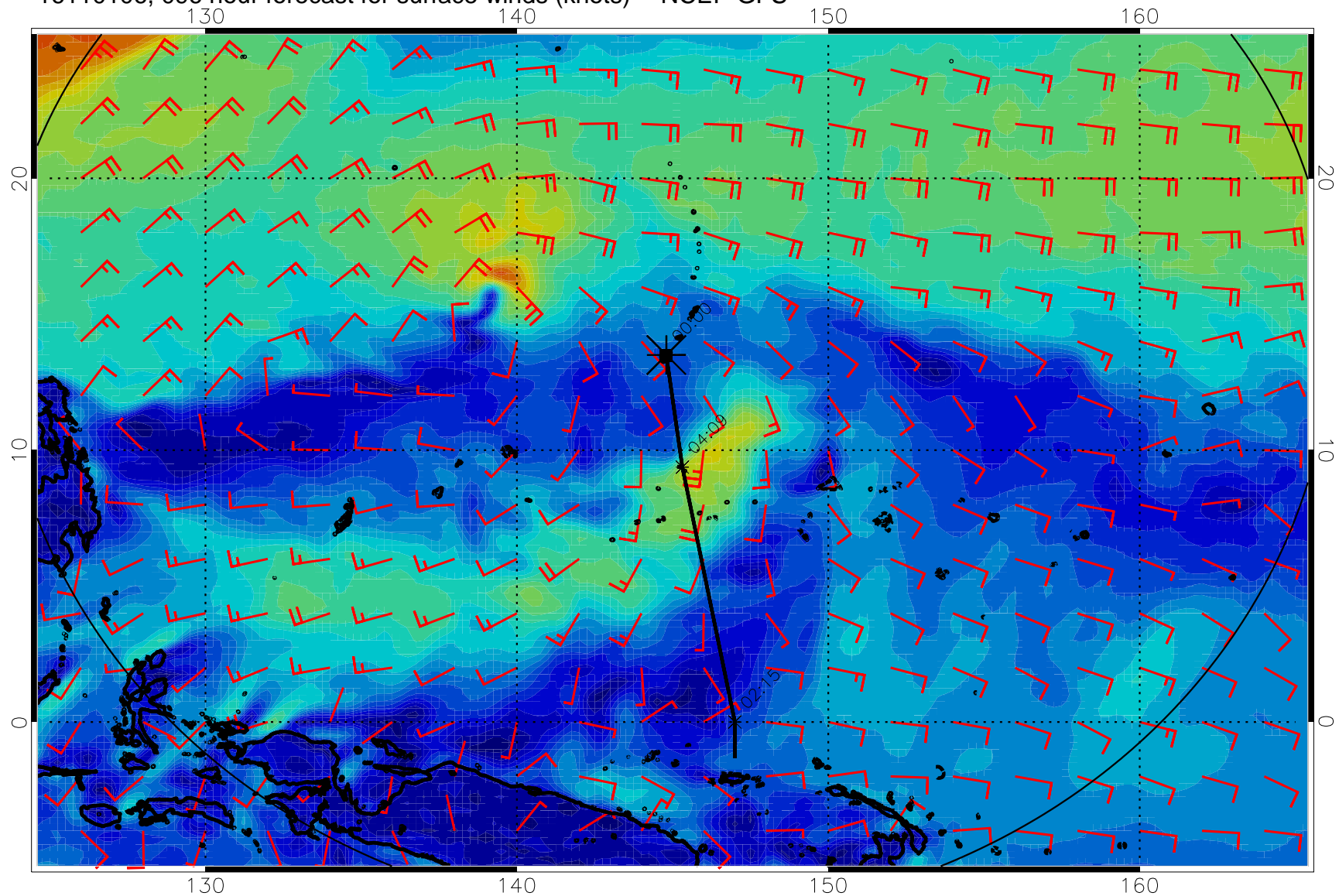
16110106, 096 hour forecast for surface winds (knots) -- NCEP GFS
