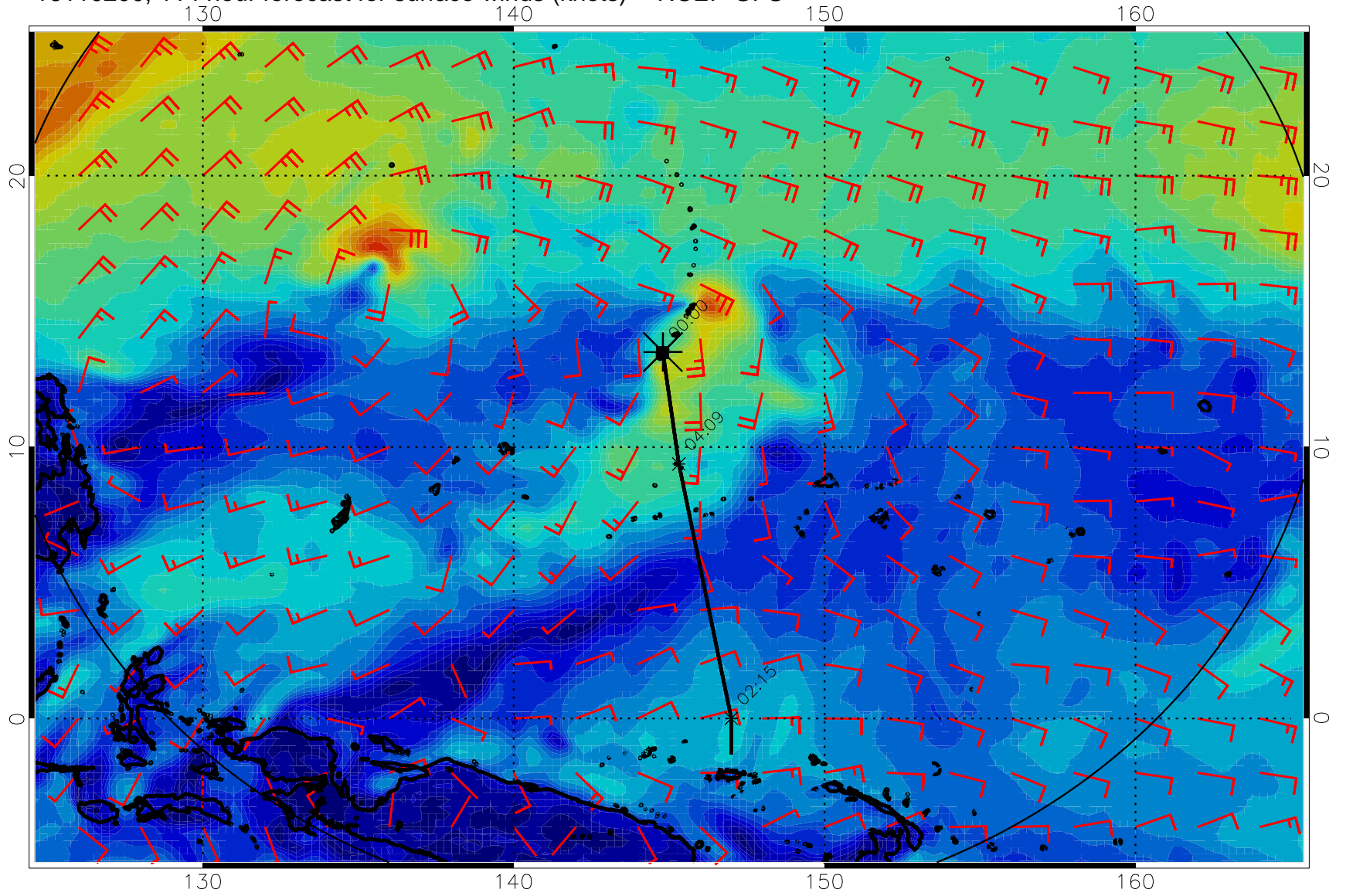
16110200, 114 hour forecast for surface winds (knots) -- NCEP GFS
