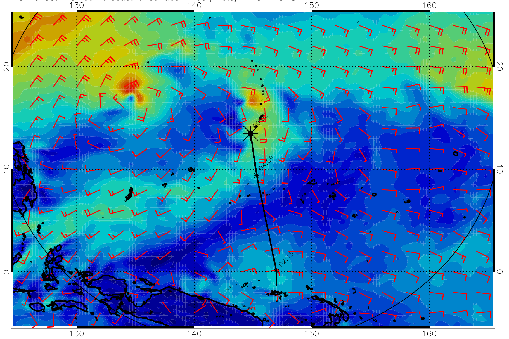
16110206, 120 hour forecast for surface winds (knots) -- NCEP GFS
