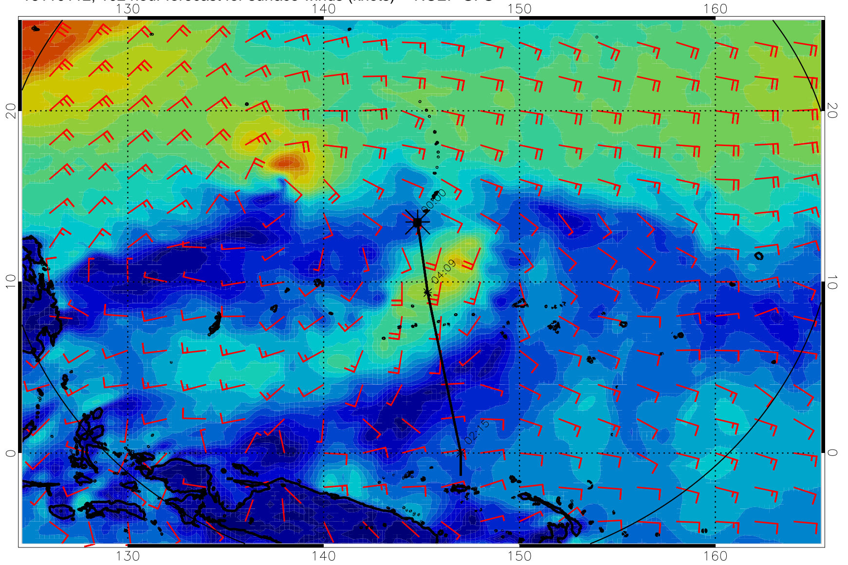
16110112, 102 hour forecast for surface winds (knots) -- NCEP GFS
