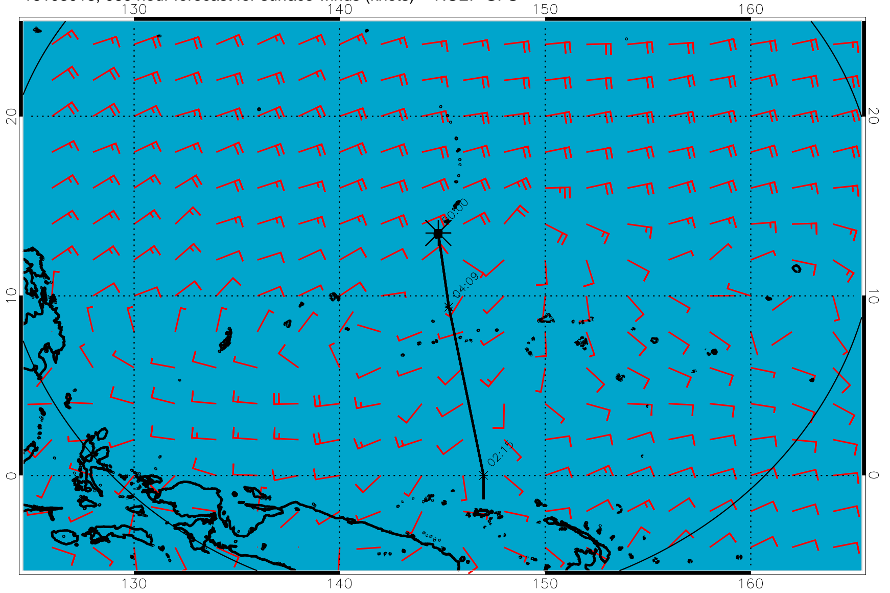
16103018, 060 hour forecast for surface winds (knots) -- NCEP GFS
