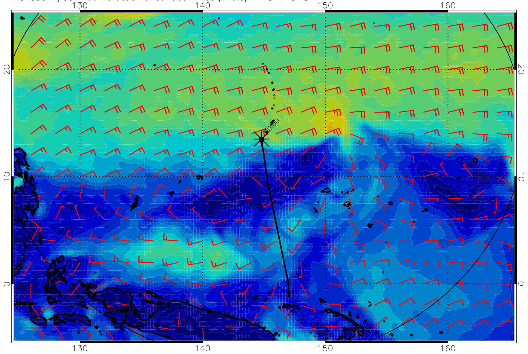
16103012, 054 hour forecast for surface winds (knots) -- NCEP GFS
