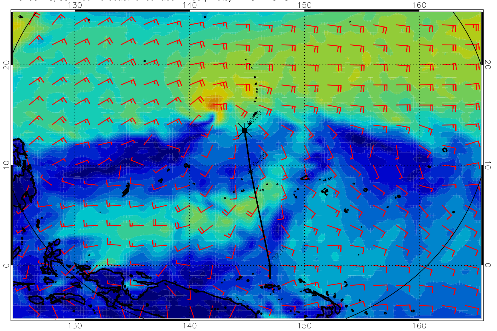
16103118, 084 hour forecast for surface winds (knots) -- NCEP GFS
