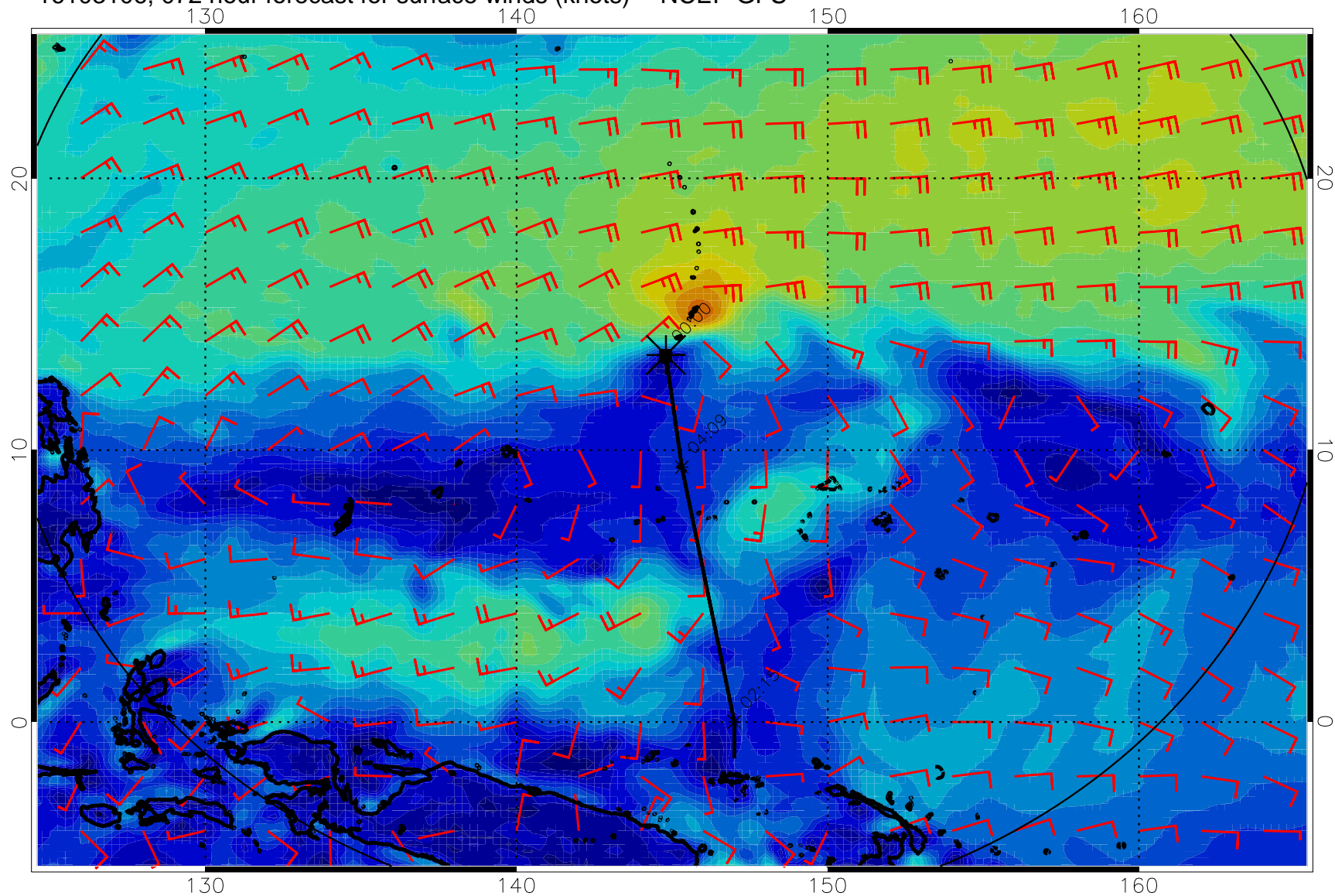
16103106, 072 hour forecast for surface winds (knots) -- NCEP GFS
