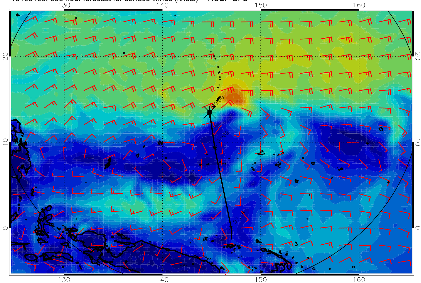
16103100, 066 hour forecast for surface winds (knots) -- NCEP GFS
