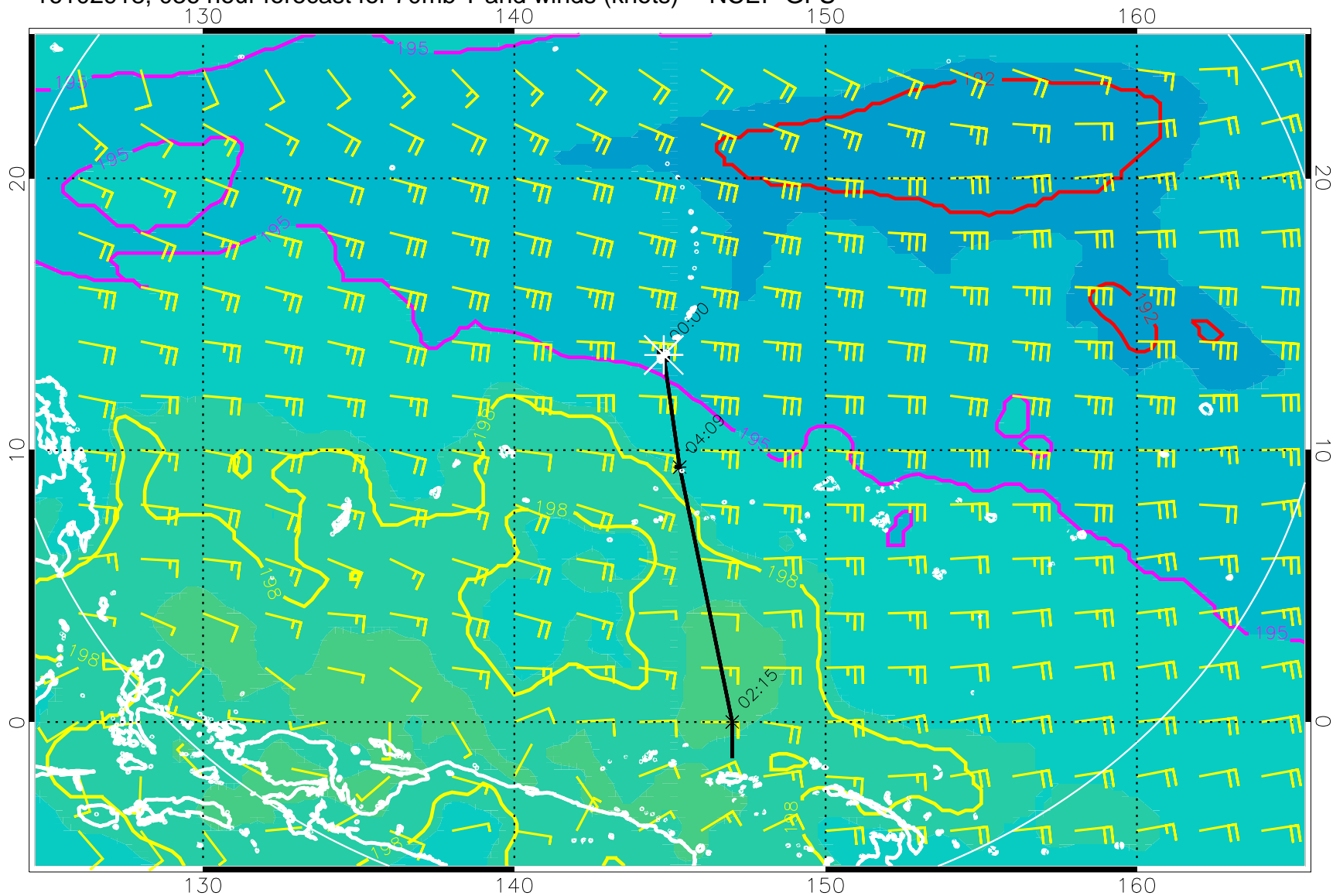
16102918, 036 hour forecast for 70mb T and winds (knots) -- NCEP GFS
