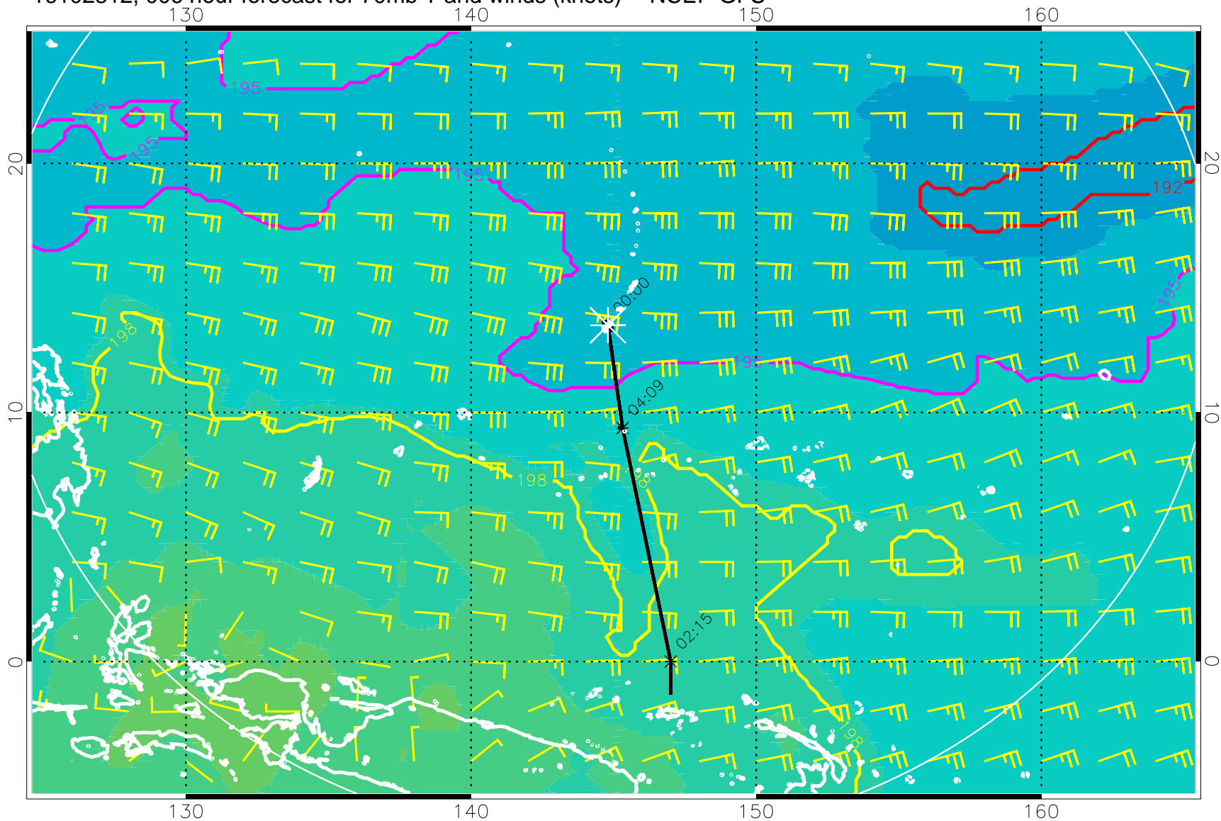
16102812, 006 hour forecast for 70mb T and winds (knots) -- NCEP GFS
