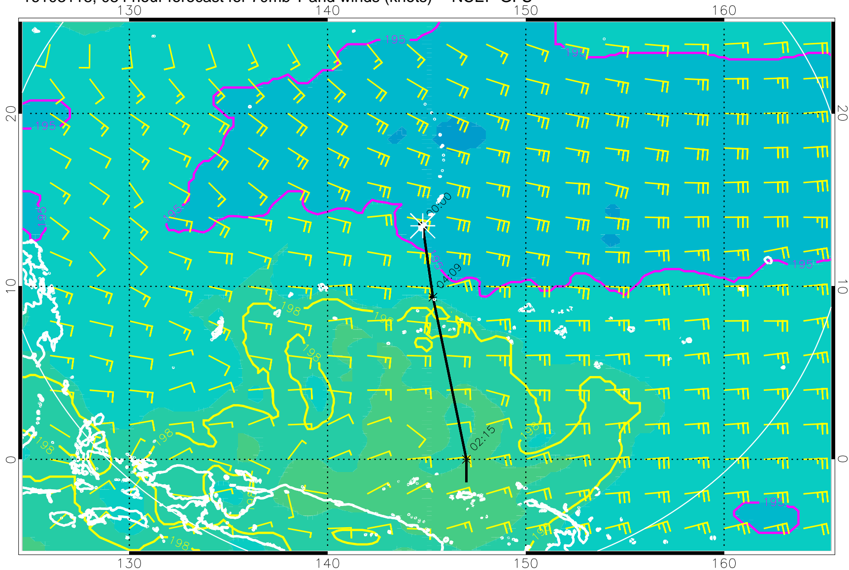
16103118, 084 hour forecast for 70mb T and winds (knots) -- NCEP GFS
