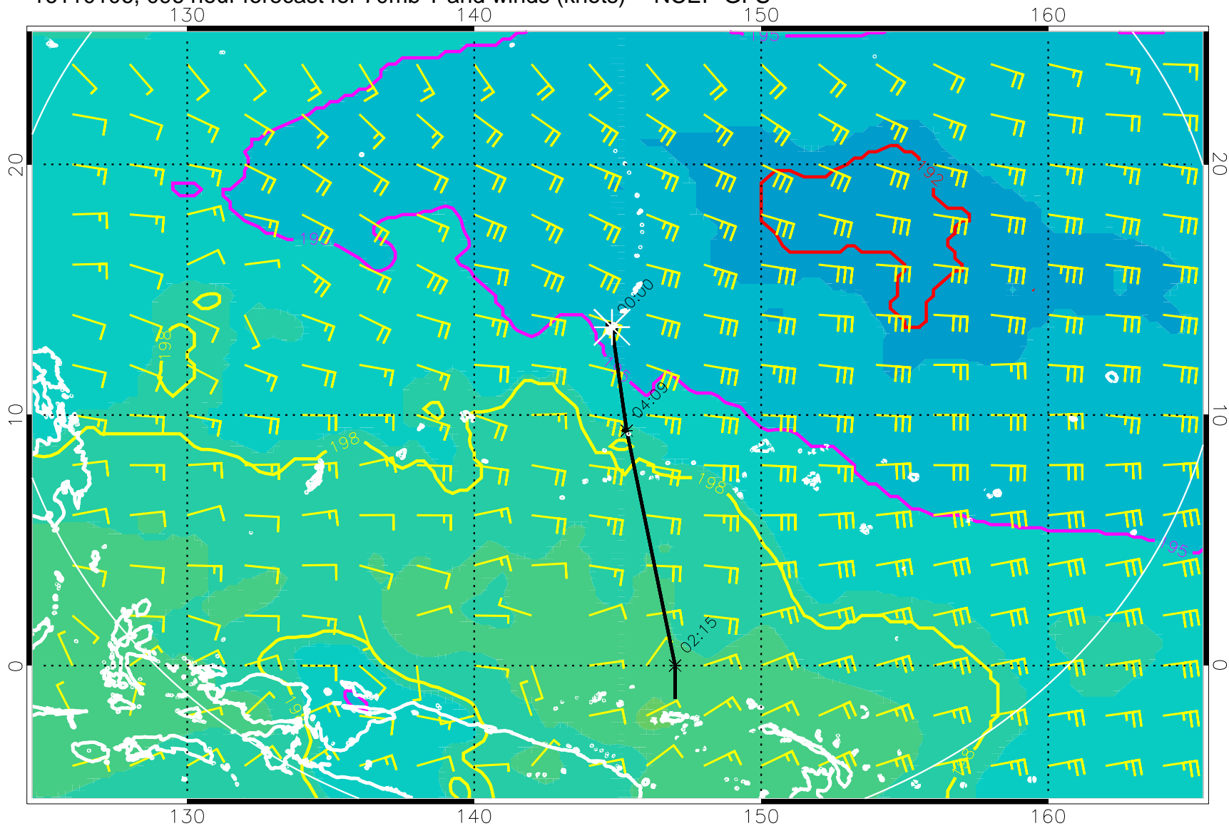
16110106, 096 hour forecast for 70mb T and winds (knots) -- NCEP GFS
