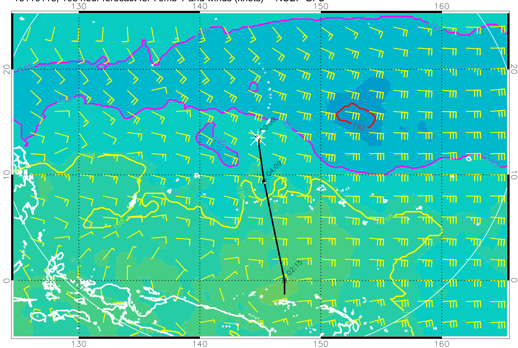
16110118, 108 hour forecast for 70mb T and winds (knots) -- NCEP GFS
