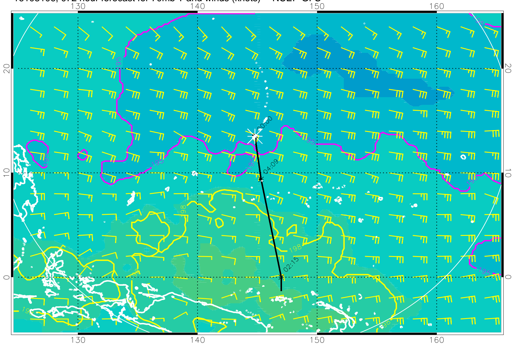
16103106, 072 hour forecast for 70mb T and winds (knots) -- NCEP GFS
