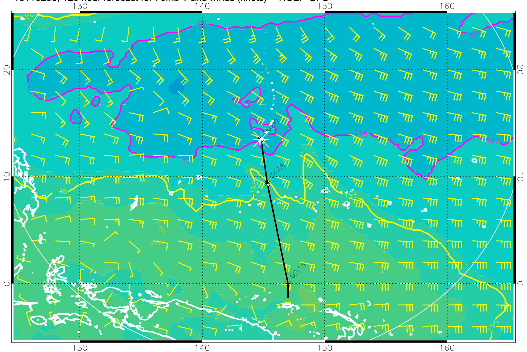
16110206, 120 hour forecast for 70mb T and winds (knots) -- NCEP GFS
