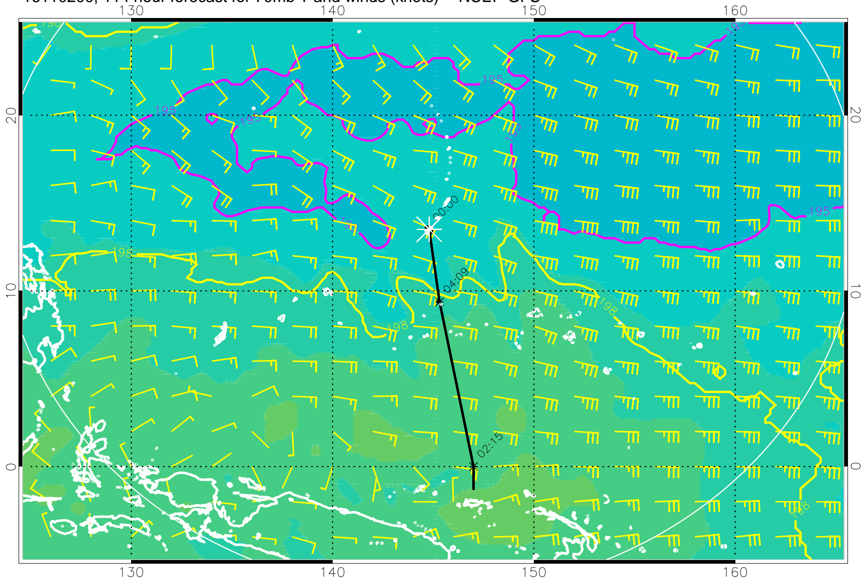
16110200, 114 hour forecast for 70mb T and winds (knots) -- NCEP GFS
