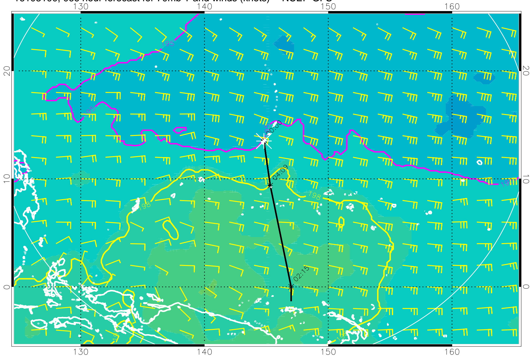
16103100, 066 hour forecast for 70mb T and winds (knots) -- NCEP GFS
