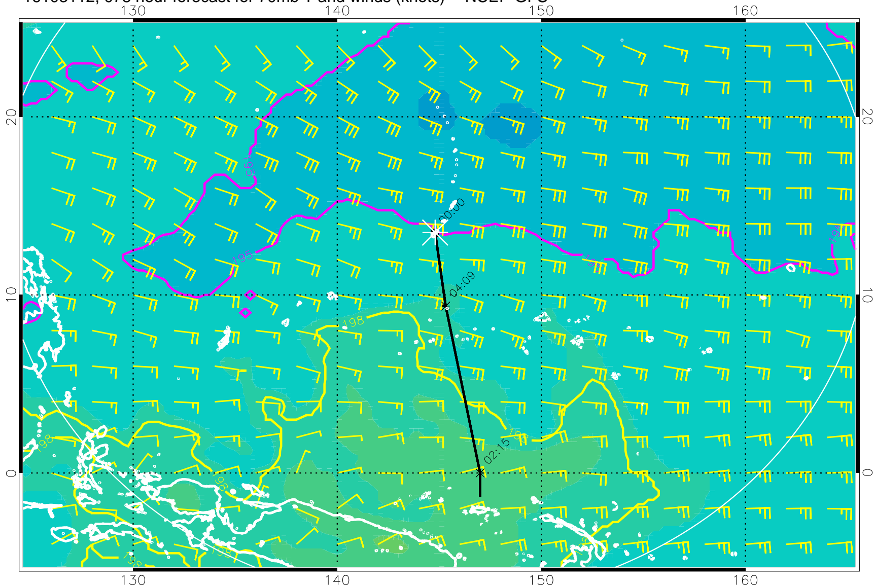
16103112, 078 hour forecast for 70mb T and winds (knots) -- NCEP GFS
