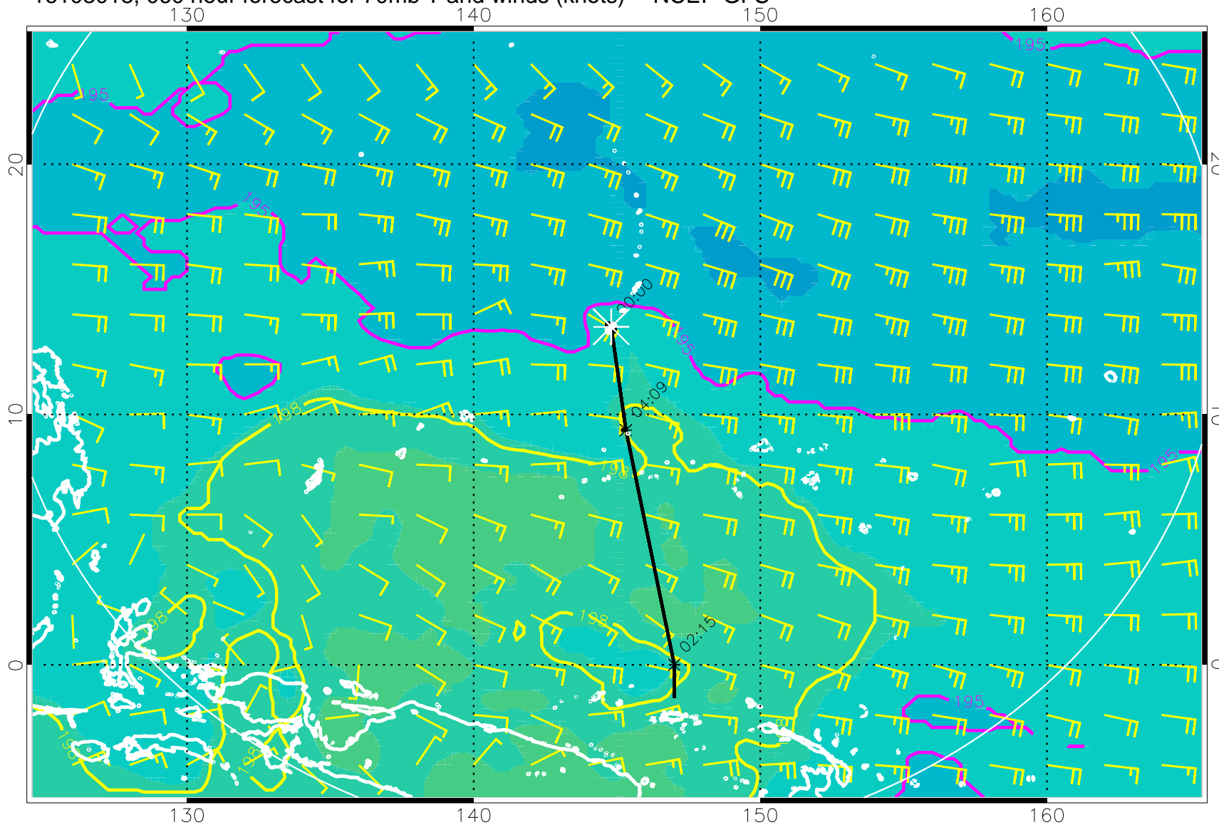
16103018, 060 hour forecast for 70mb T and winds (knots) -- NCEP GFS
