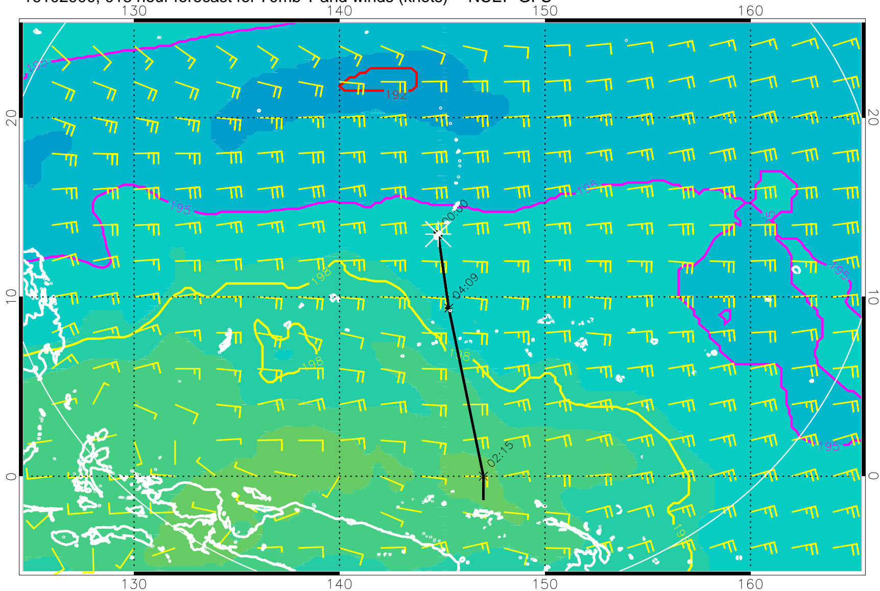
16102900, 018 hour forecast for 70mb T and winds (knots) -- NCEP GFS
