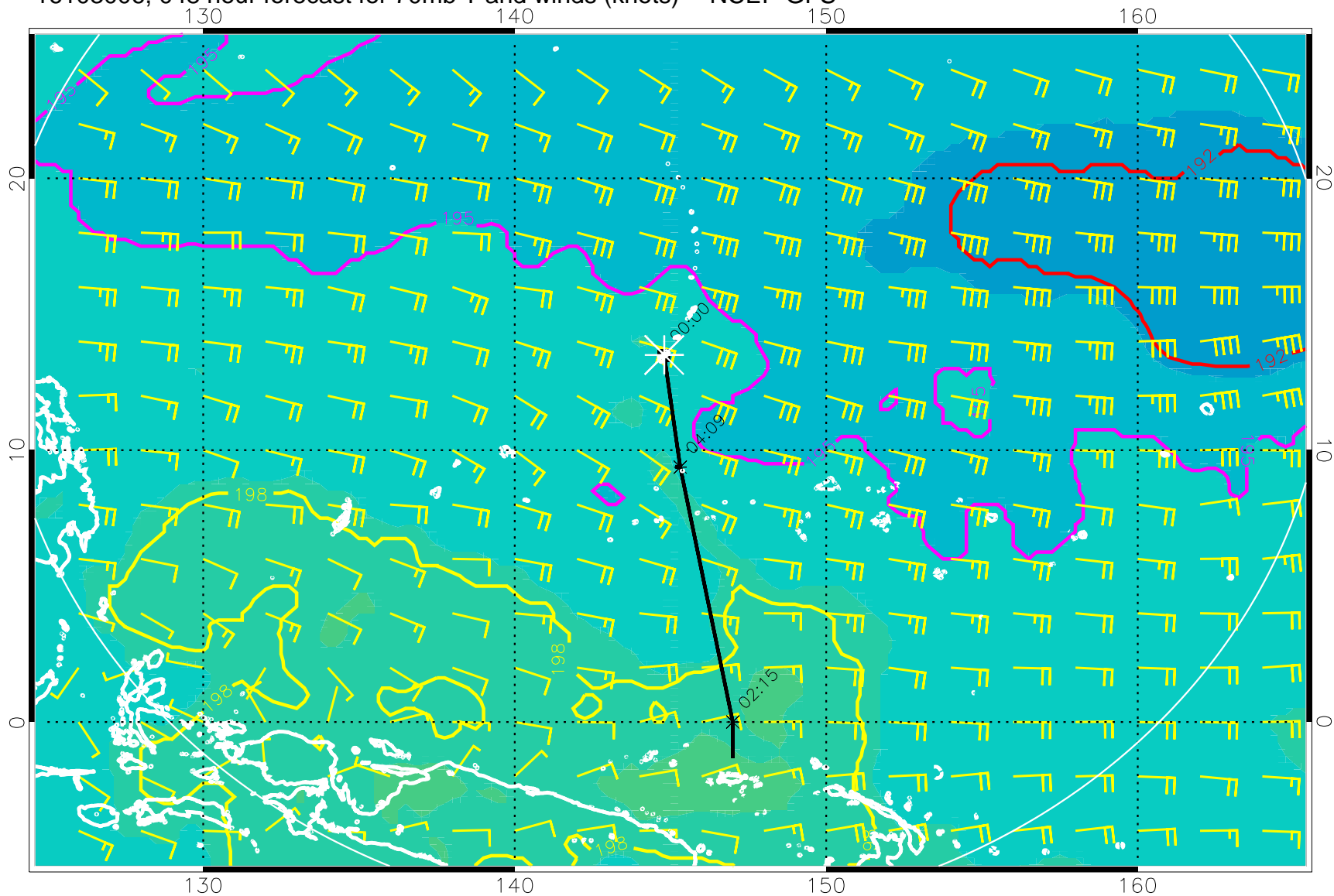
16103006, 048 hour forecast for 70mb T and winds (knots) -- NCEP GFS
