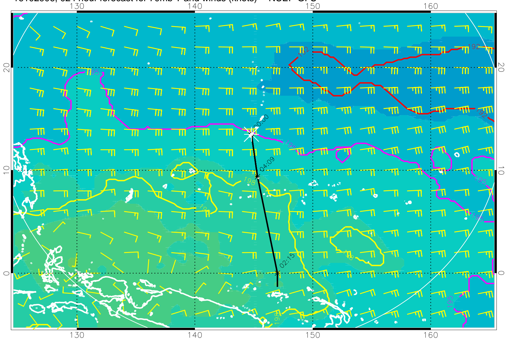
16102906, 024 hour forecast for 70mb T and winds (knots) -- NCEP GFS
