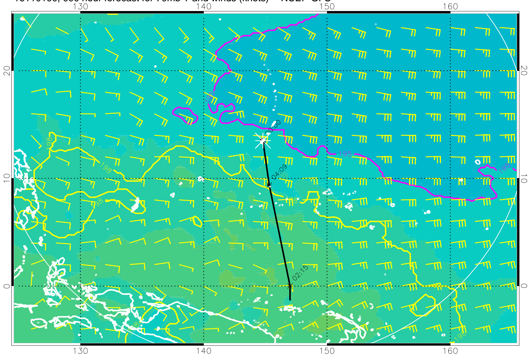
16110100, 090 hour forecast for 70mb T and winds (knots) -- NCEP GFS
