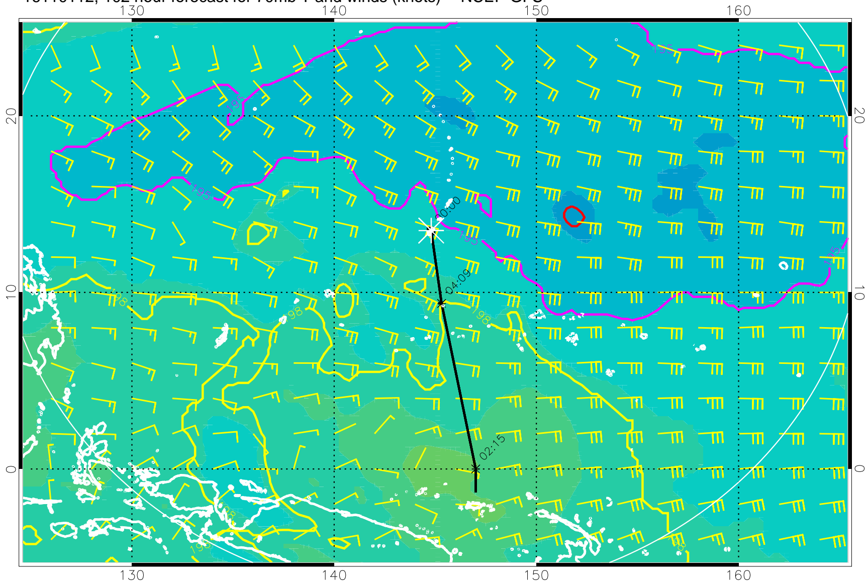
16110112, 102 hour forecast for 70mb T and winds (knots) -- NCEP GFS
