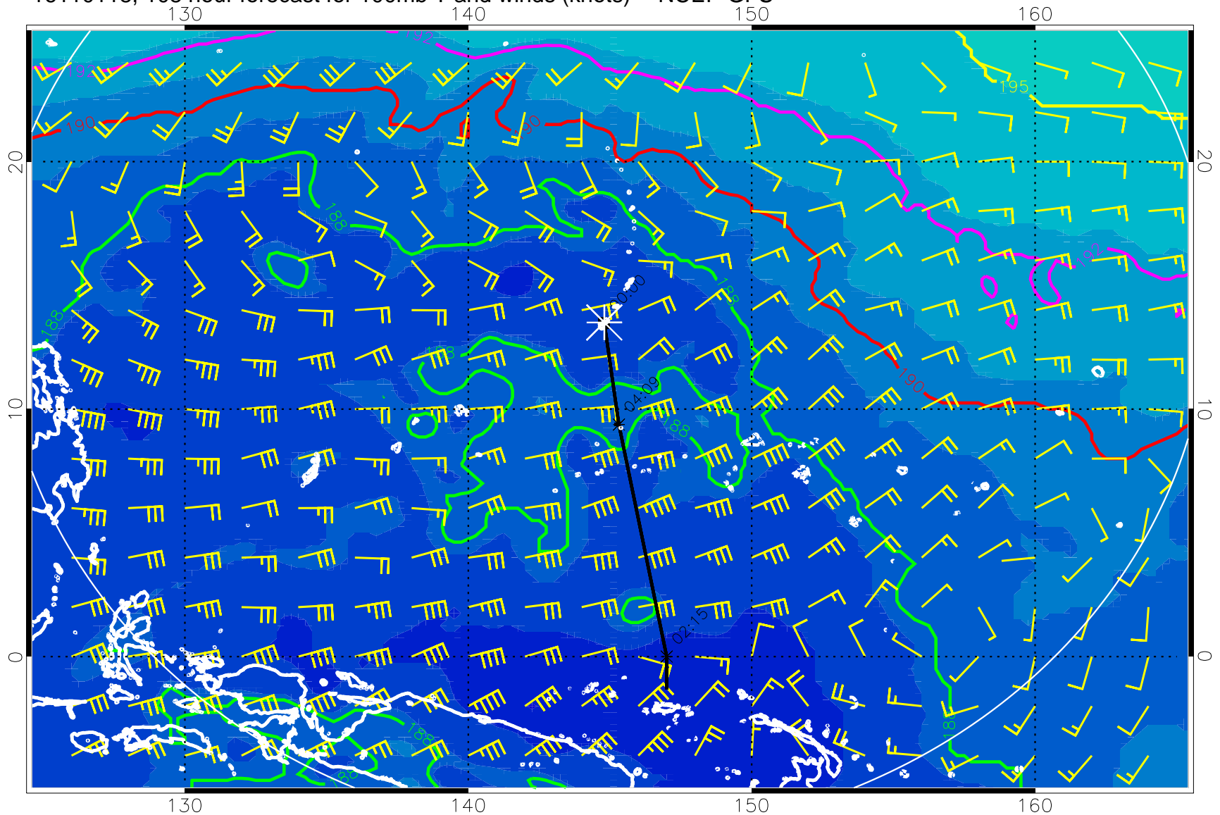
16110118, 108 hour forecast for 100mb T and winds (knots) -- NCEP GFS
