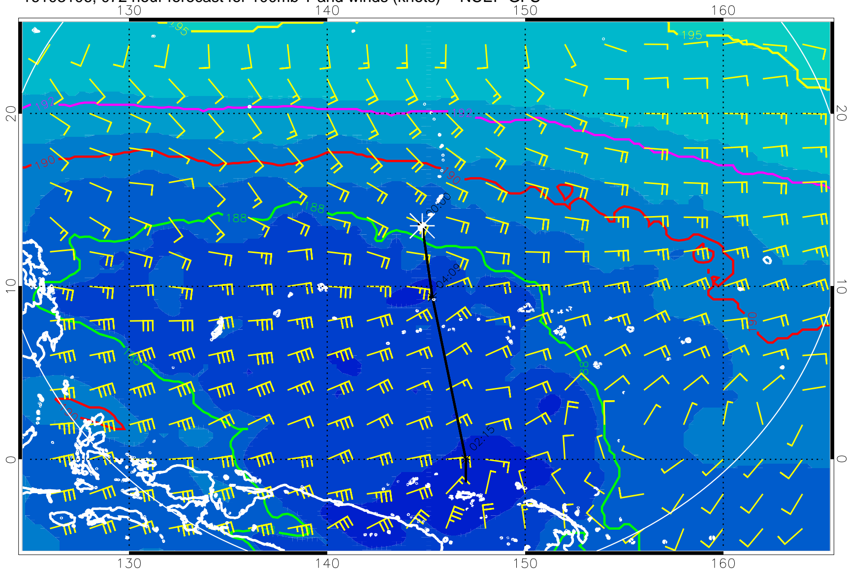
16103106, 072 hour forecast for 100mb T and winds (knots) -- NCEP GFS
