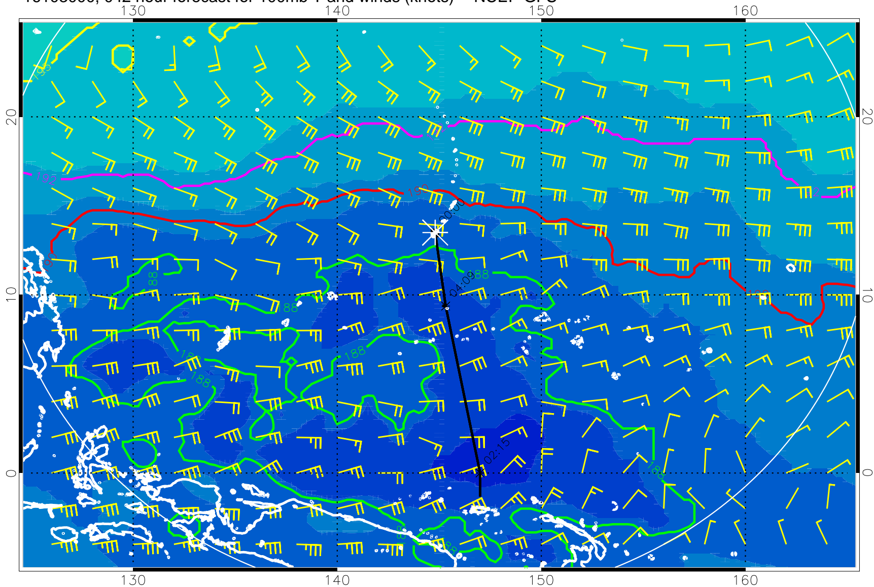
16103000, 042 hour forecast for 100mb T and winds (knots) -- NCEP GFS
