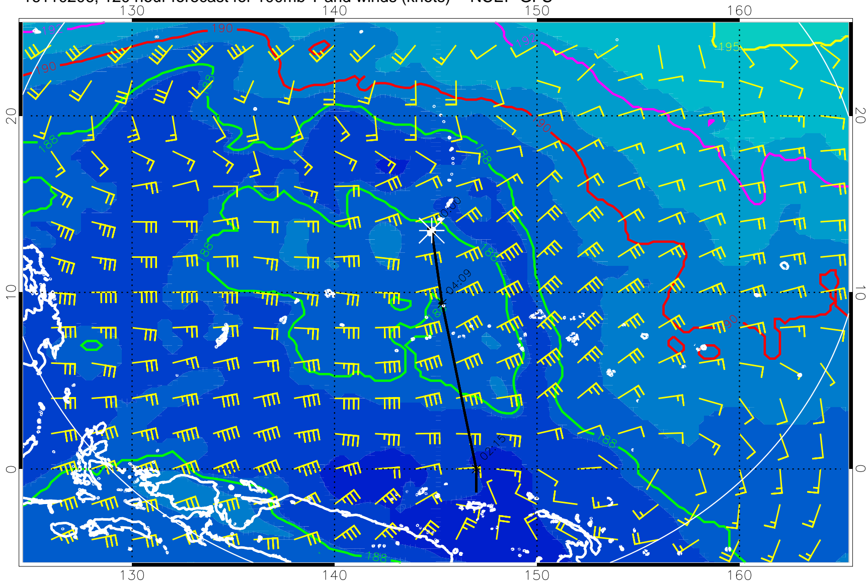
16110206, 120 hour forecast for 100mb T and winds (knots) -- NCEP GFS
