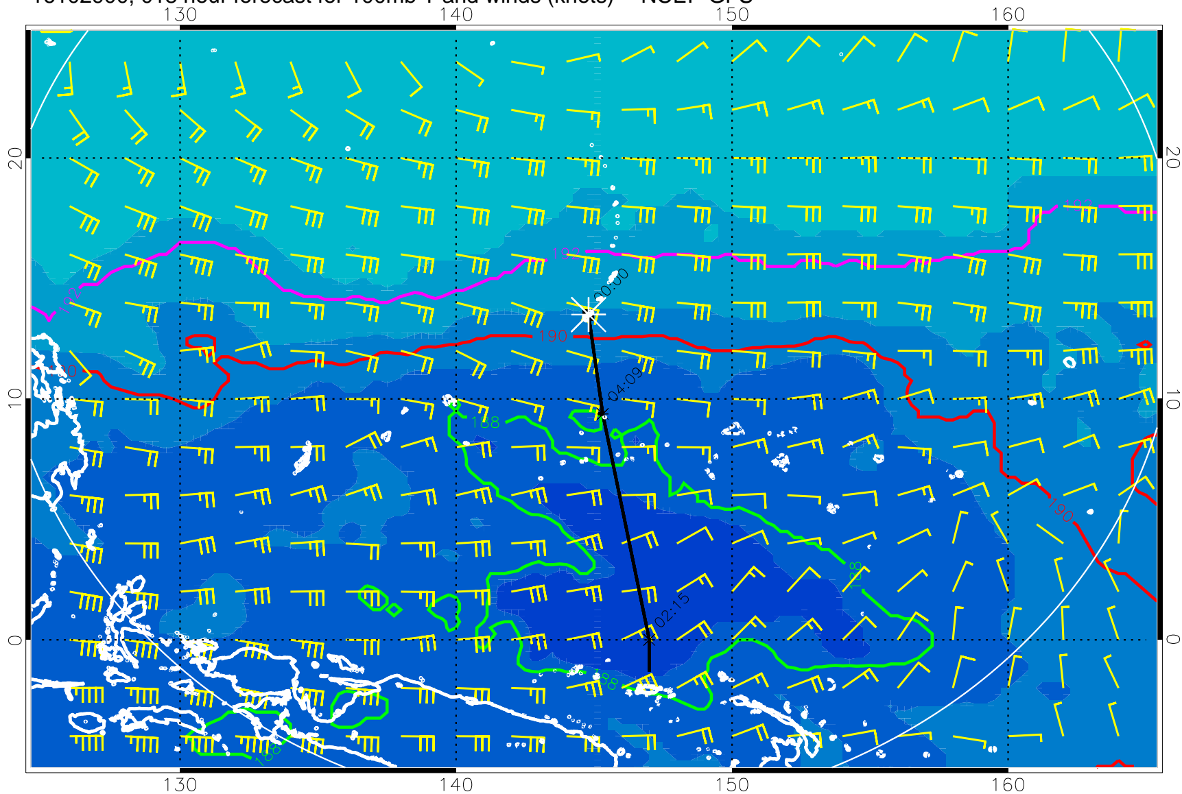
16102900, 018 hour forecast for 100mb T and winds (knots) -- NCEP GFS
