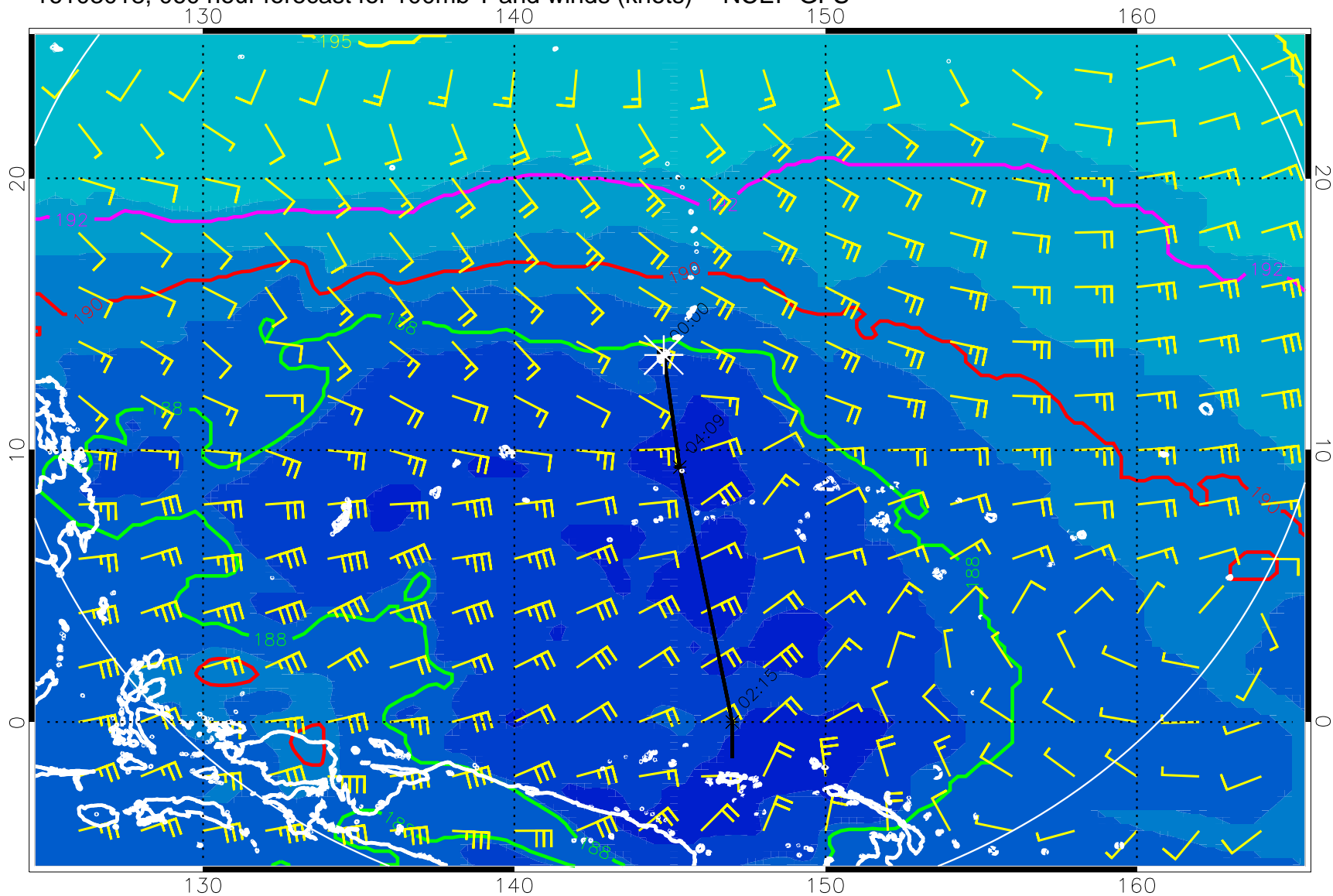
16103018, 060 hour forecast for 100mb T and winds (knots) -- NCEP GFS
