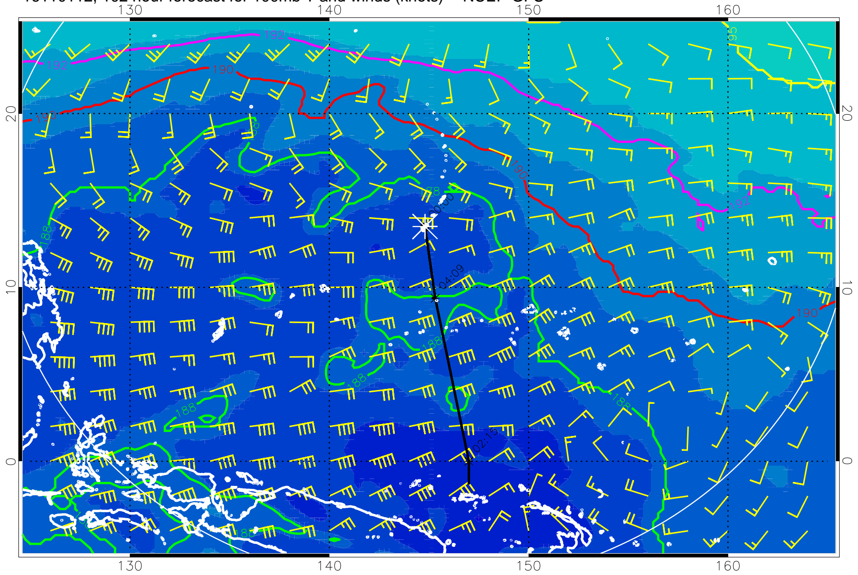
16110112, 102 hour forecast for 100mb T and winds (knots) -- NCEP GFS
