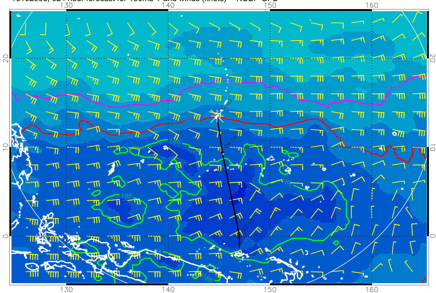
16102906, 024 hour forecast for 100mb T and winds (knots) -- NCEP GFS
