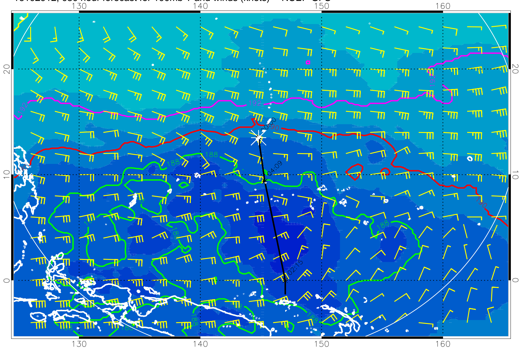
16102912, 030 hour forecast for 100mb T and winds (knots) -- NCEP GFS
