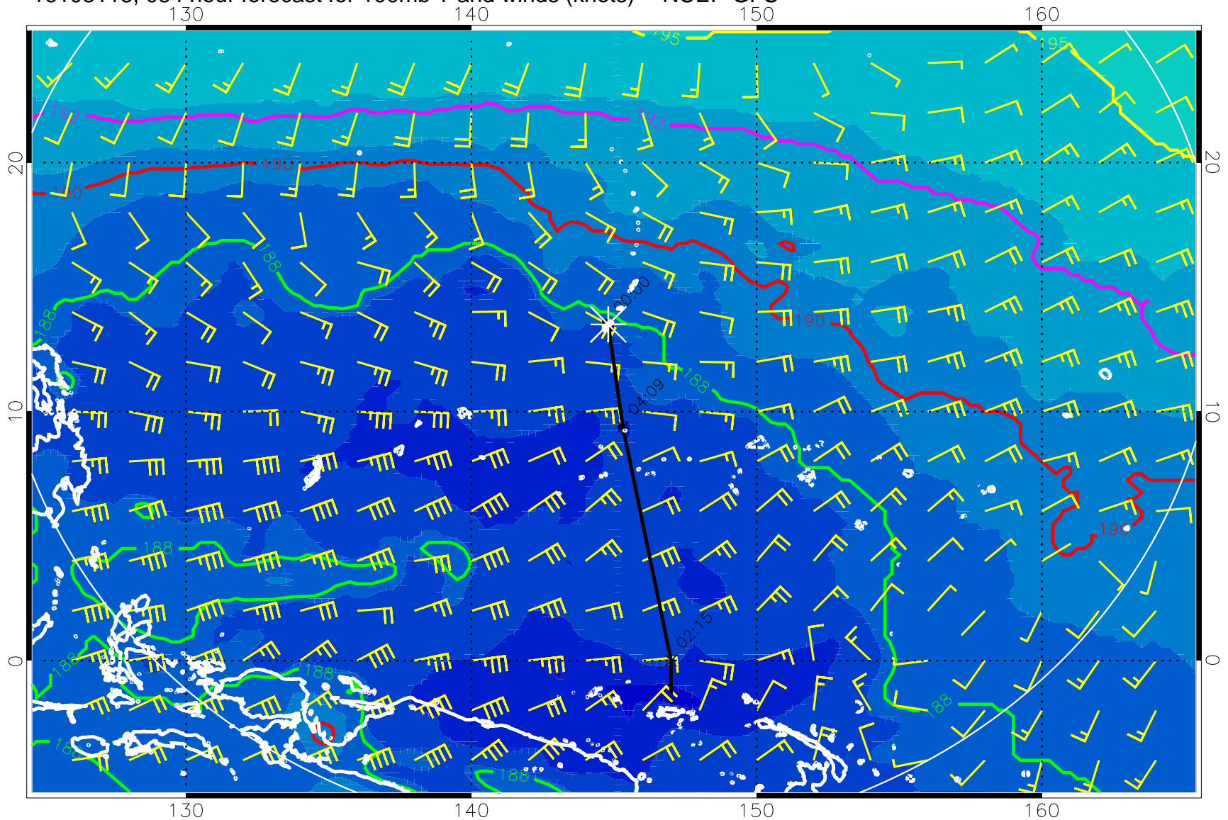
16103118, 084 hour forecast for 100mb T and winds (knots) -- NCEP GFS
