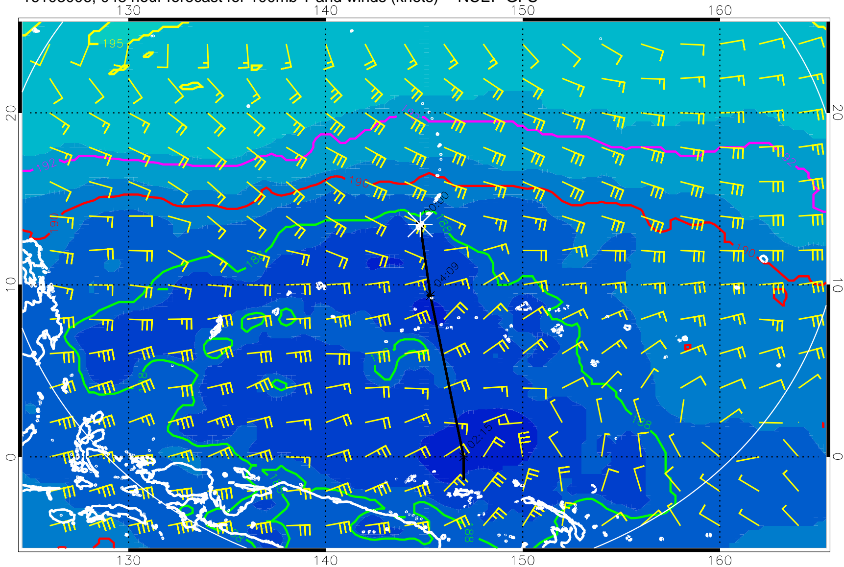
16103006, 048 hour forecast for 100mb T and winds (knots) -- NCEP GFS
