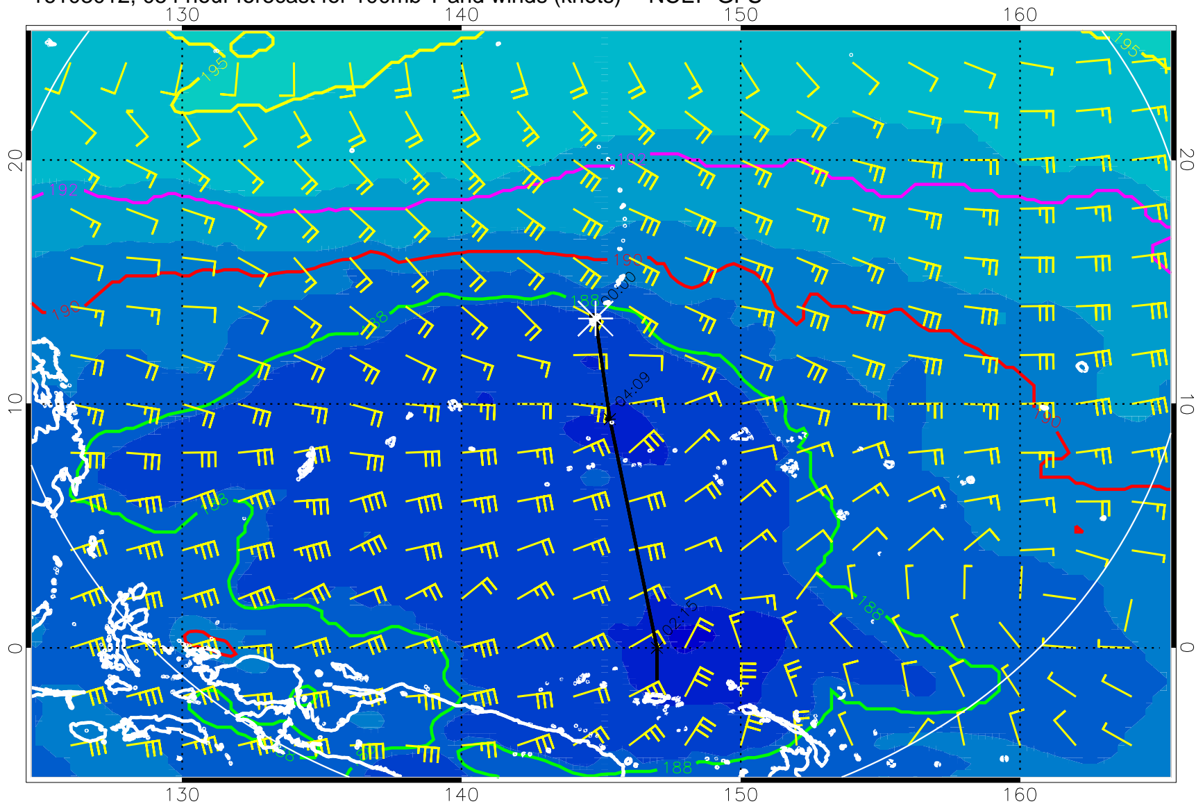
16103012, 054 hour forecast for 100mb T and winds (knots) -- NCEP GFS
