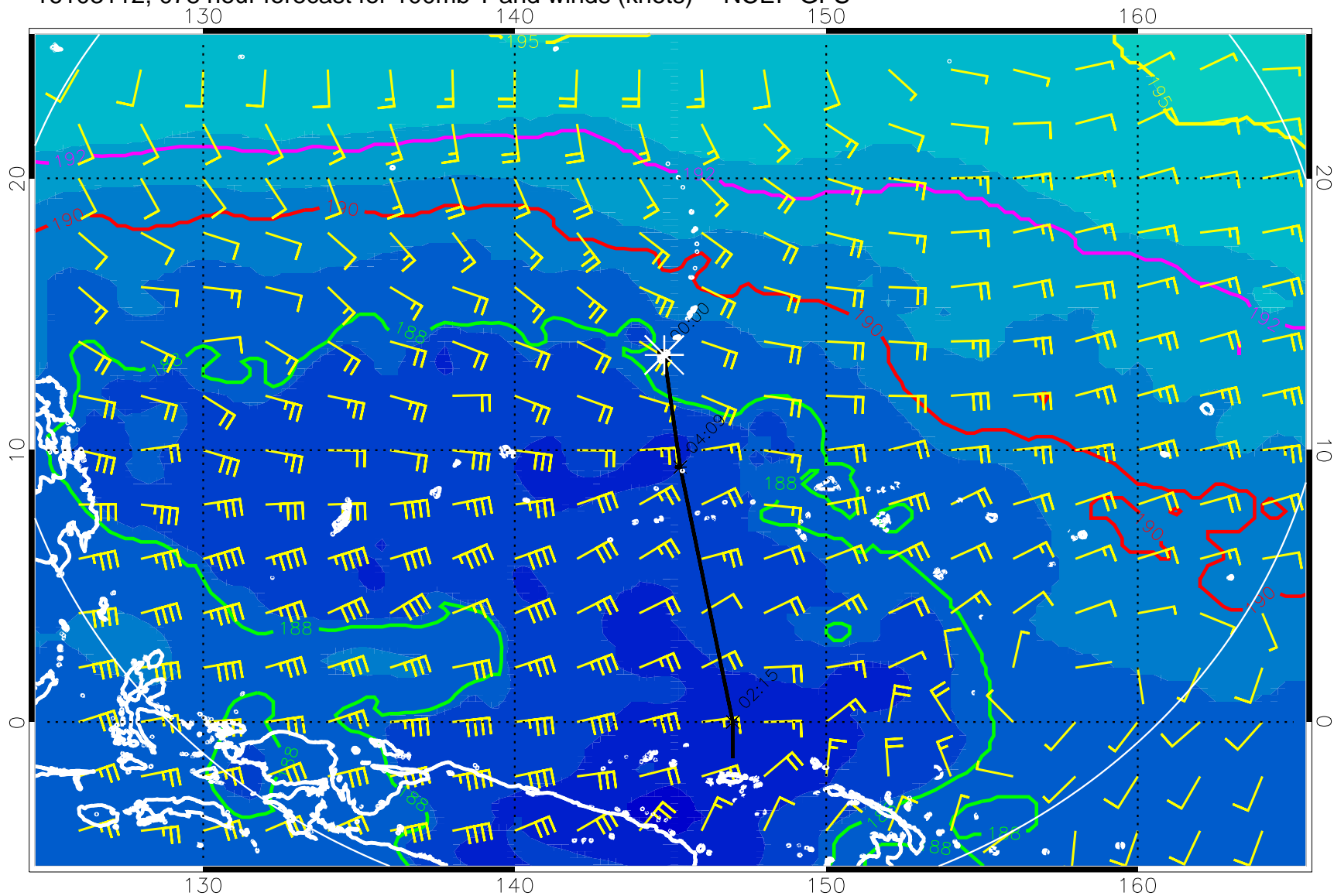
16103112, 078 hour forecast for 100mb T and winds (knots) -- NCEP GFS
