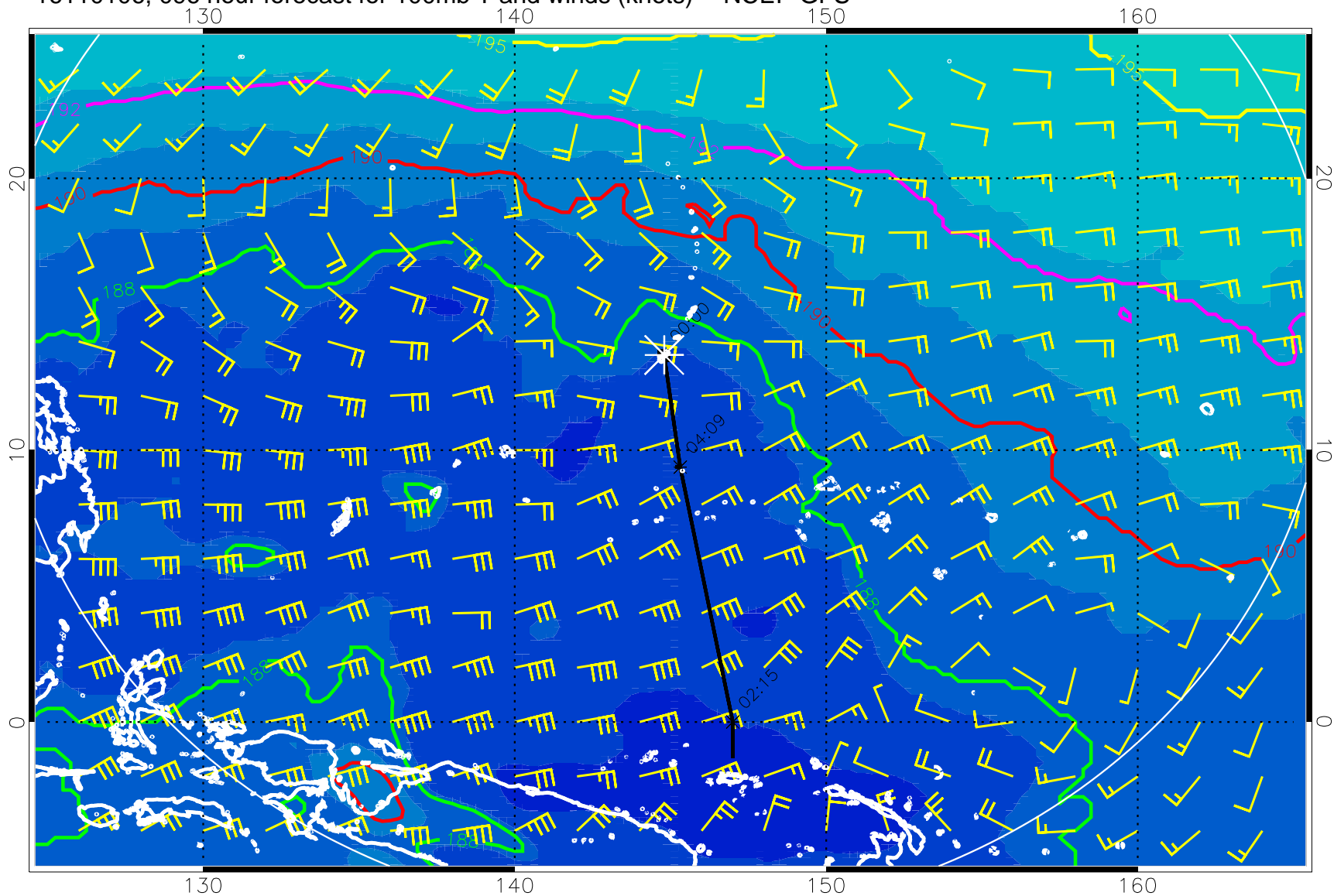
16110106, 096 hour forecast for 100mb T and winds (knots) -- NCEP GFS
