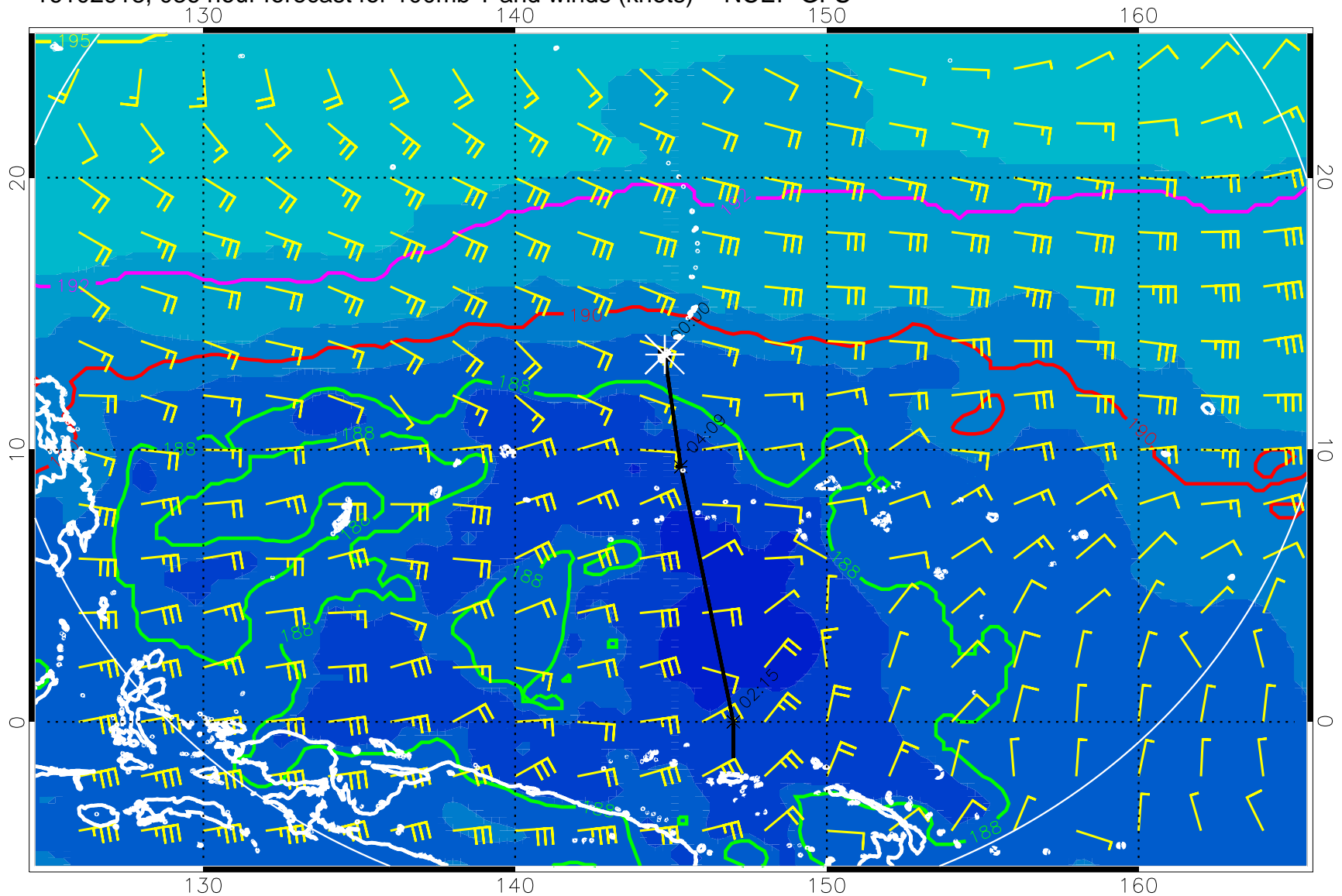
16102918, 036 hour forecast for 100mb T and winds (knots) -- NCEP GFS
