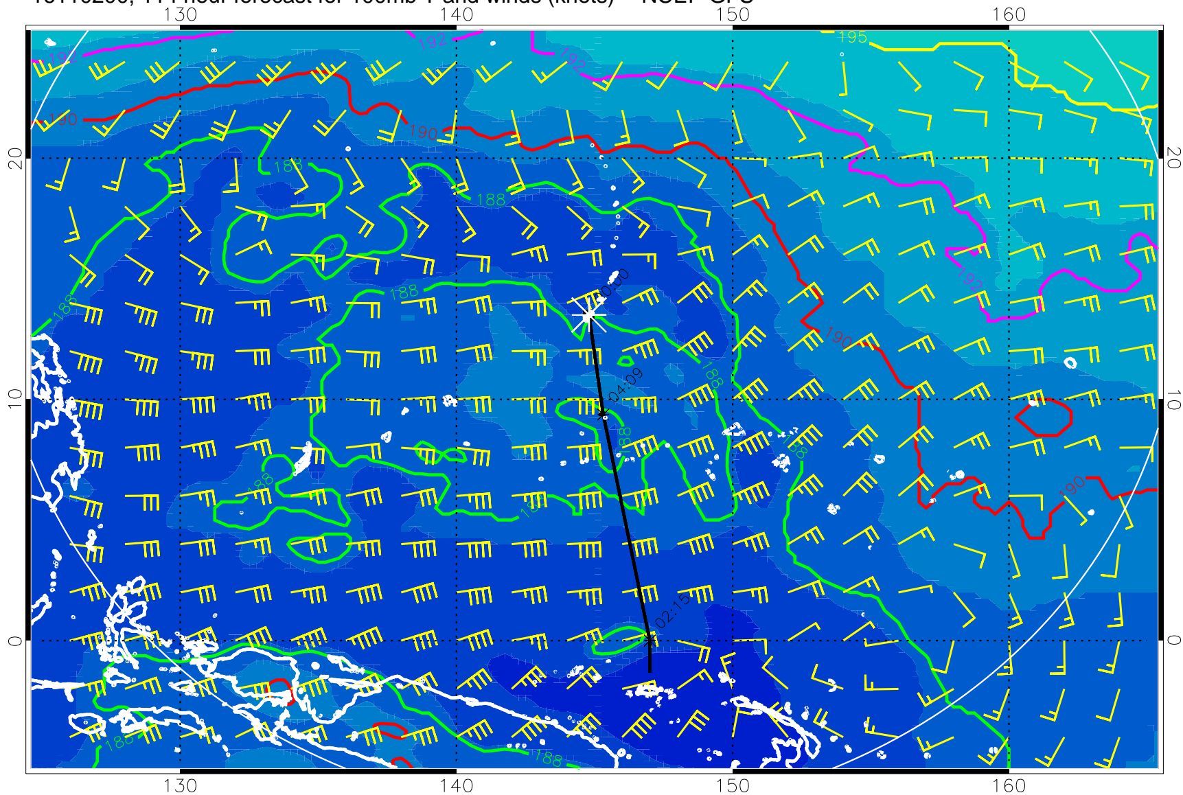
16110200, 114 hour forecast for 100mb T and winds (knots) -- NCEP GFS
