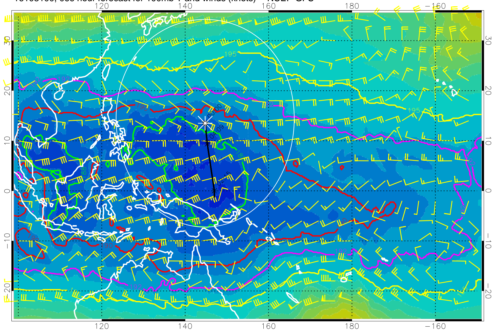
16103100, 066 hour forecast for 100mb T and winds (knots) -- NCEP GFS
