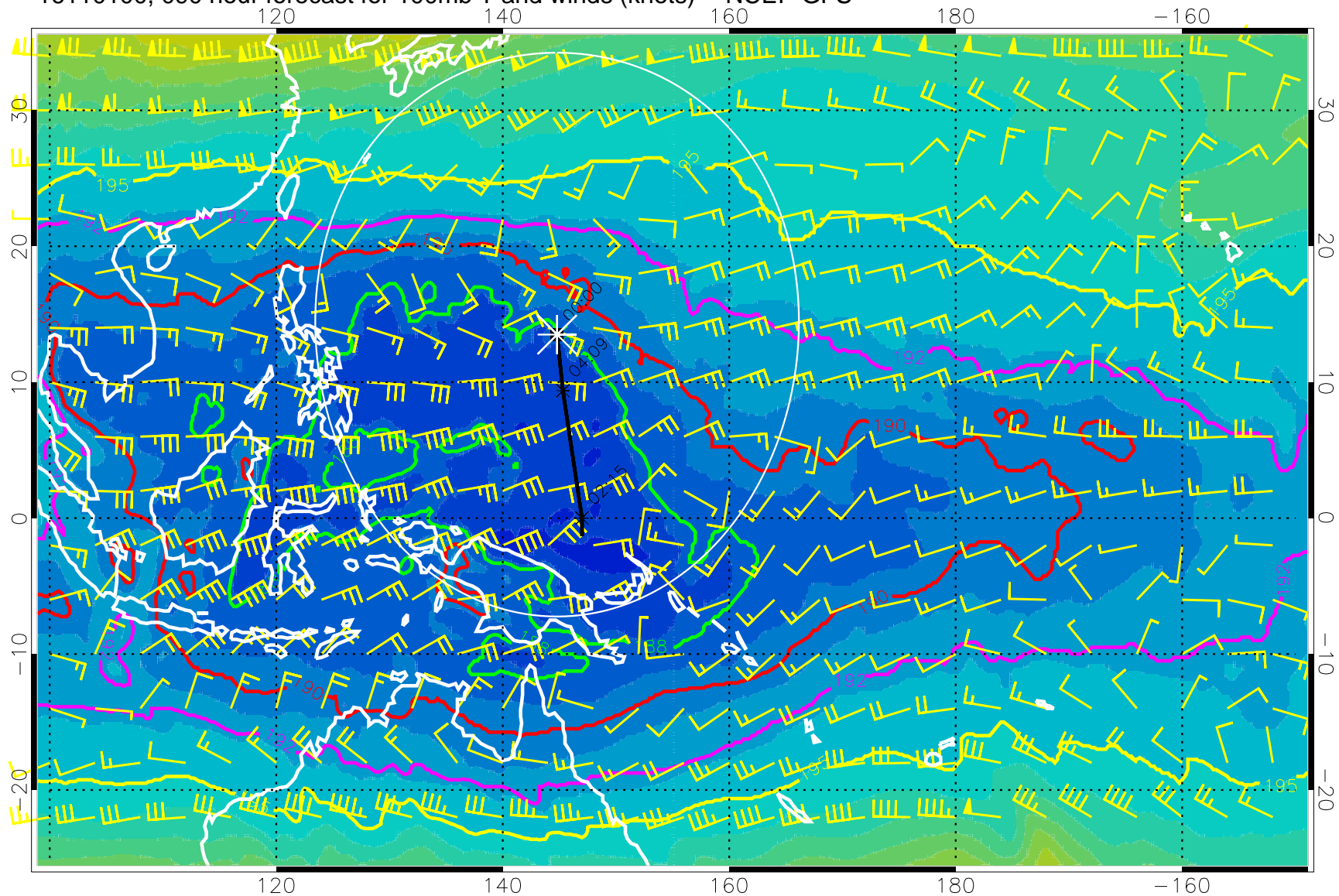
16110100, 090 hour forecast for 100mb T and winds (knots) -- NCEP GFS
