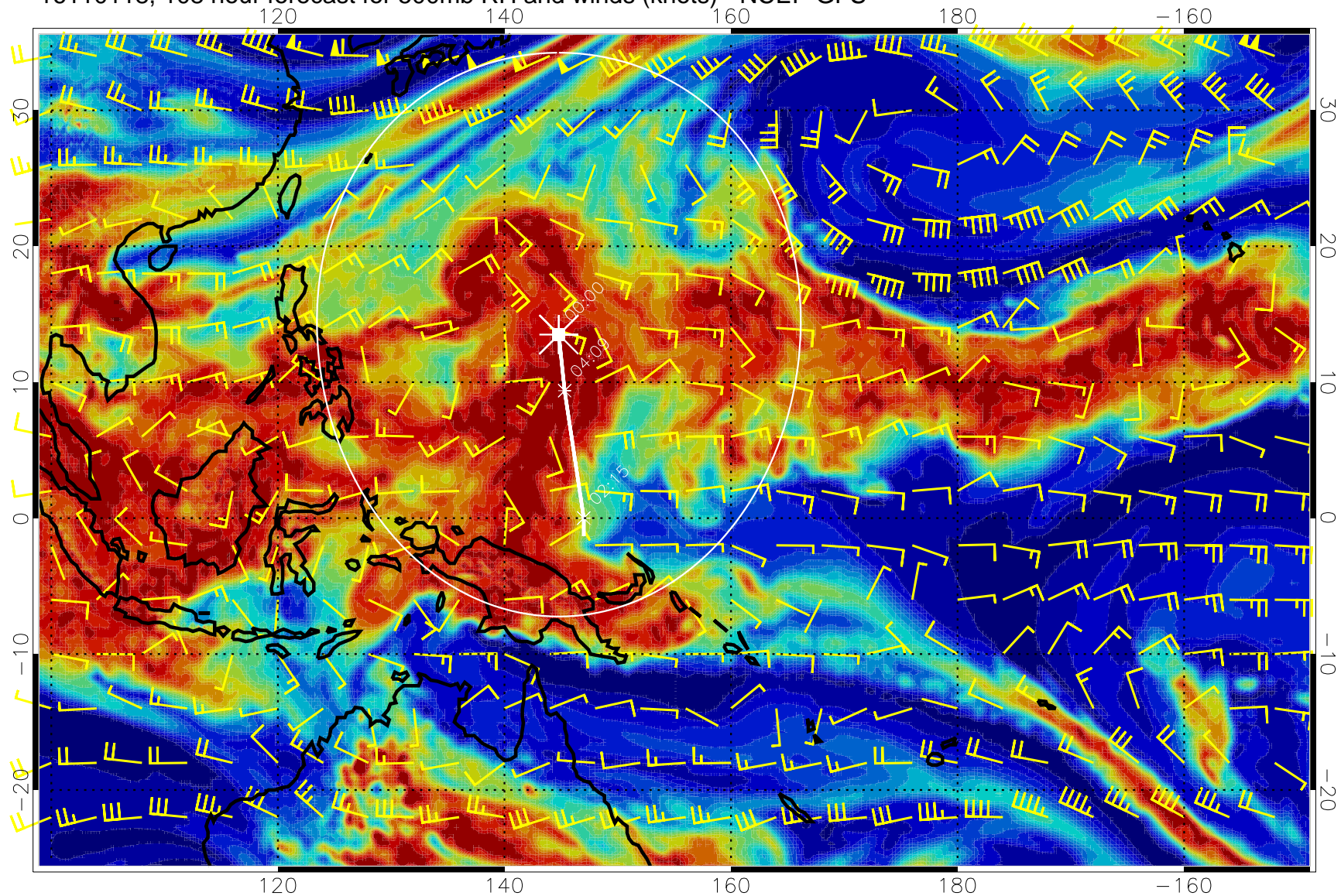
16110118, 108 hour forecast for 500mb RH and winds (knots) - NCEP GFS
