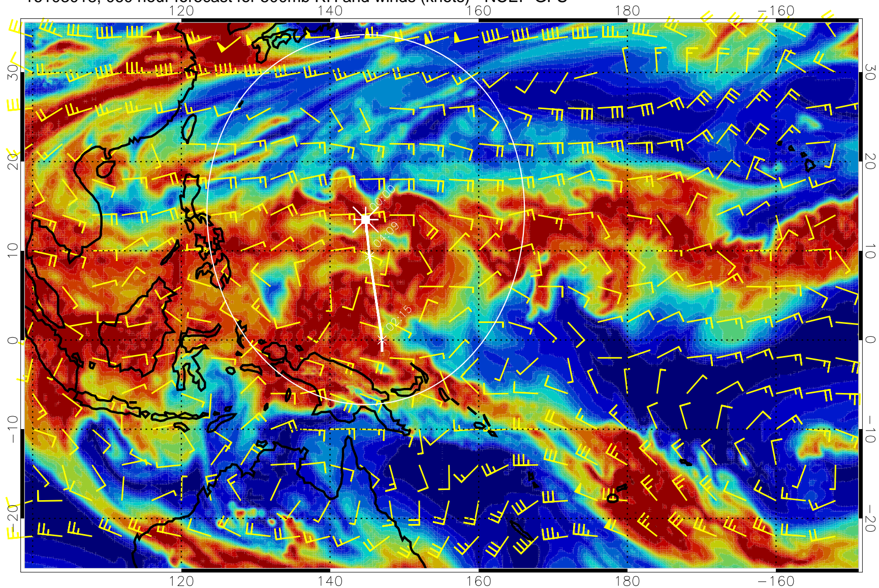
16103018, 060 hour forecast for 500mb RH and winds (knots) - NCEP GFS
