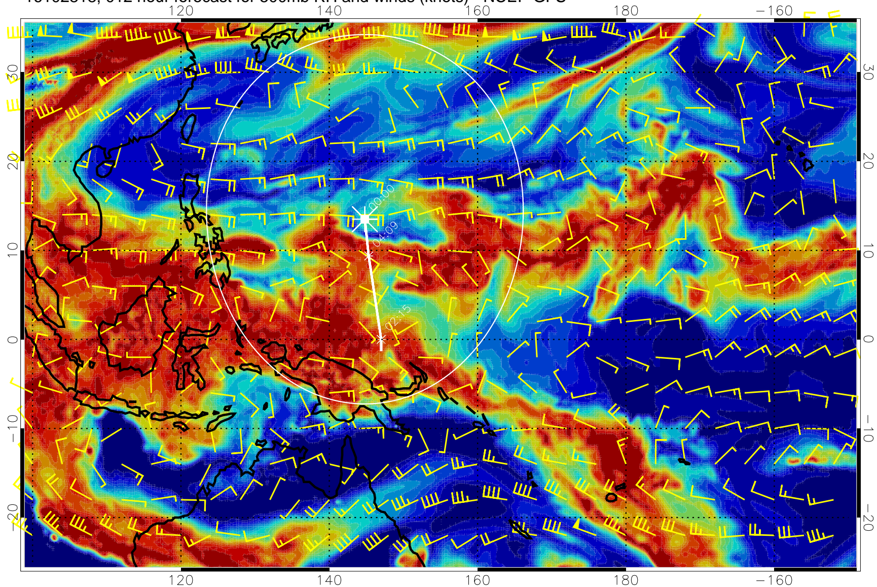
16102818, 012 hour forecast for 500mb RH and winds (knots) - NCEP GFS
