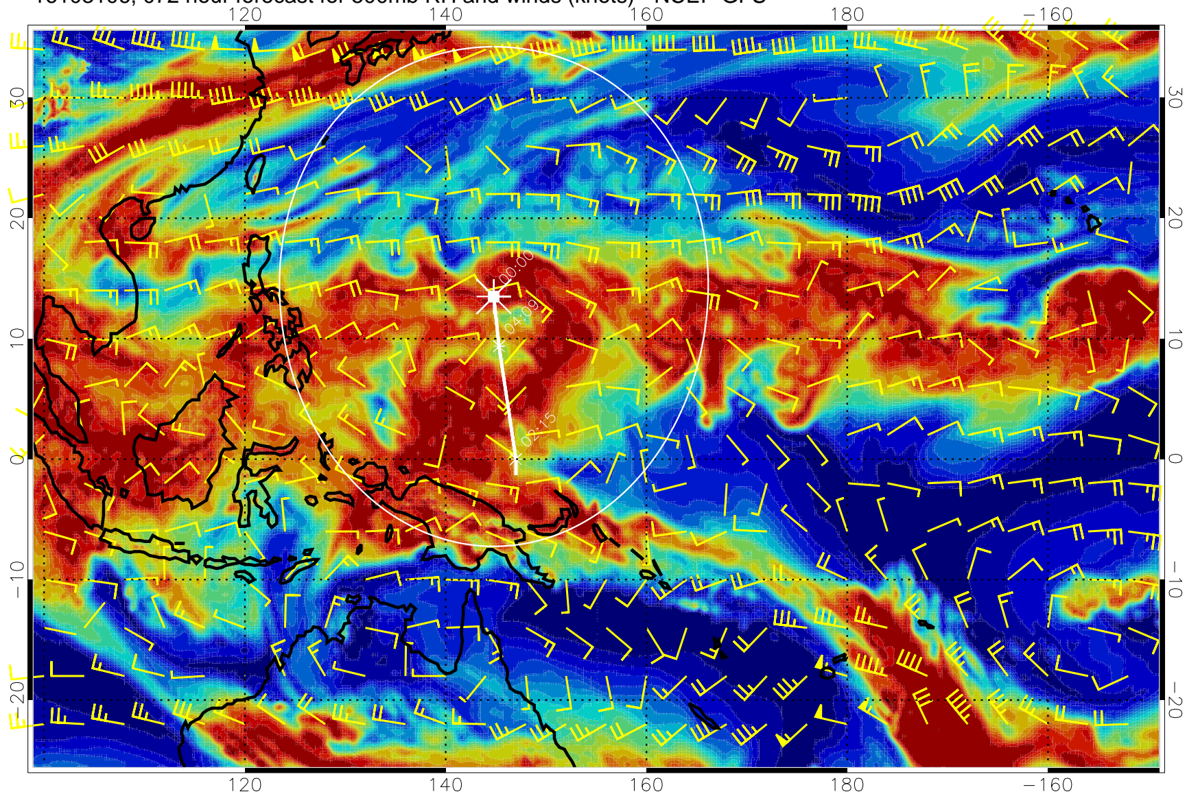
16103106, 072 hour forecast for 500mb RH and winds (knots) - NCEP GFS
