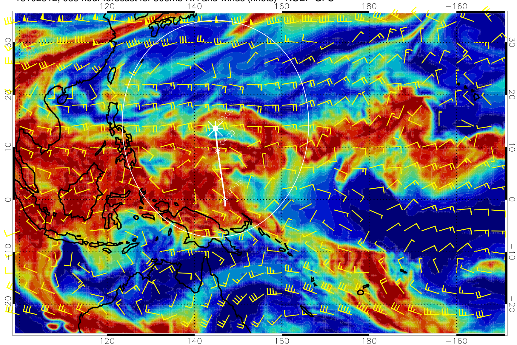
16102912, 030 hour forecast for 500mb RH and winds (knots) - NCEP GFS
