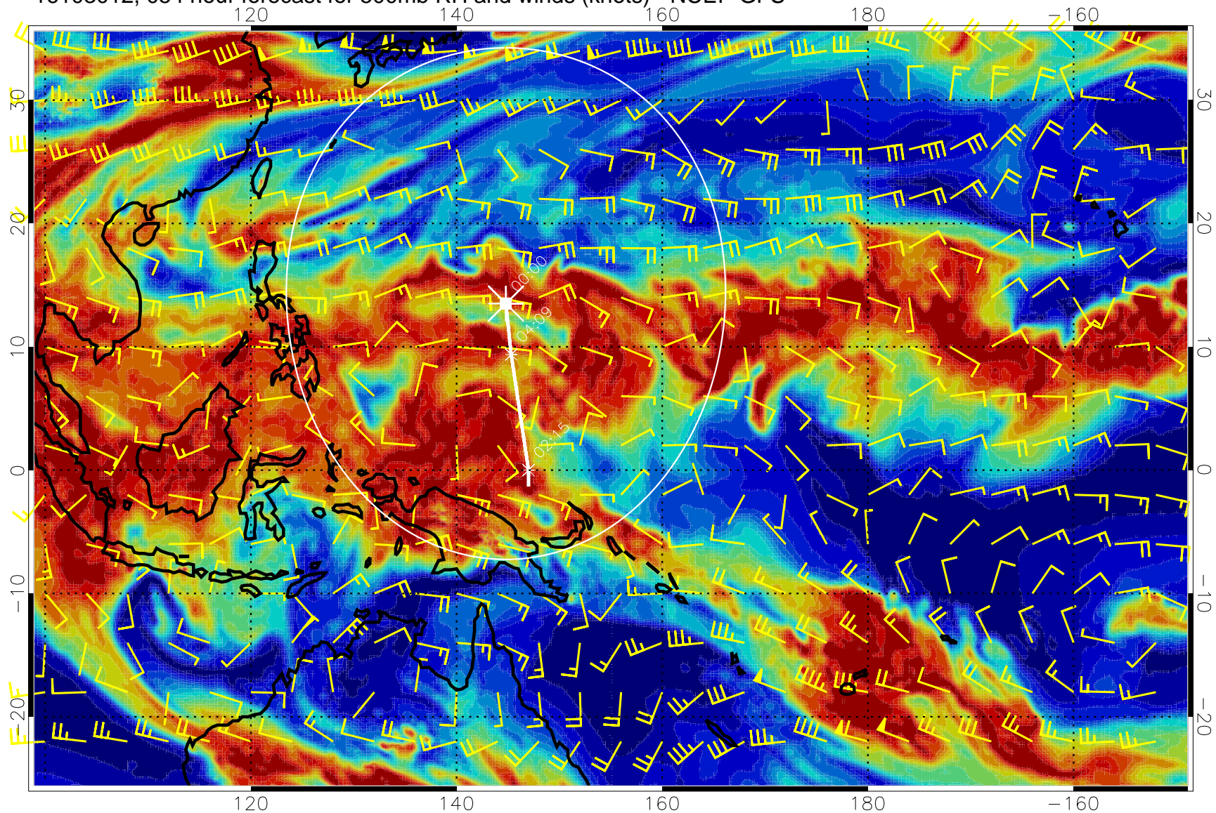
16103012, 054 hour forecast for 500mb RH and winds (knots) - NCEP GFS
