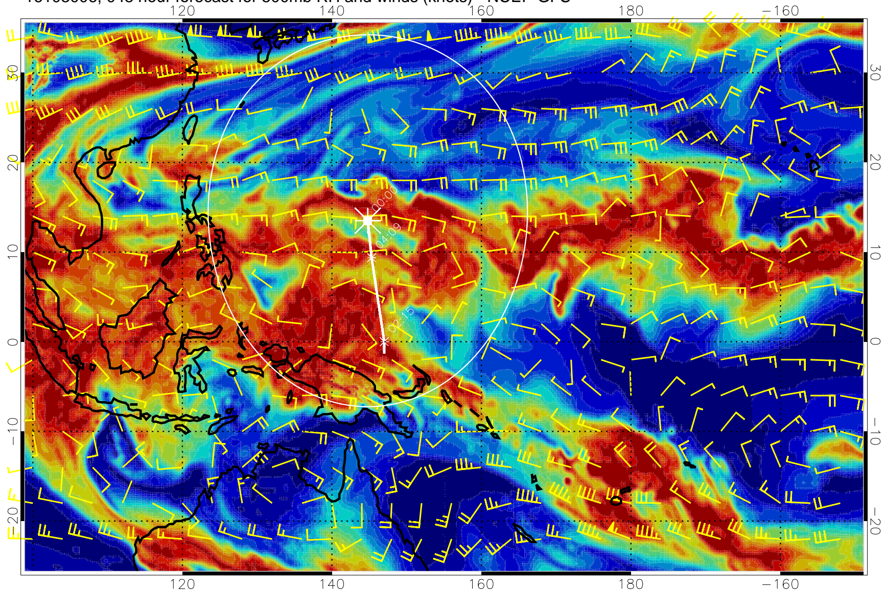
16103006, 048 hour forecast for 500mb RH and winds (knots) - NCEP GFS
