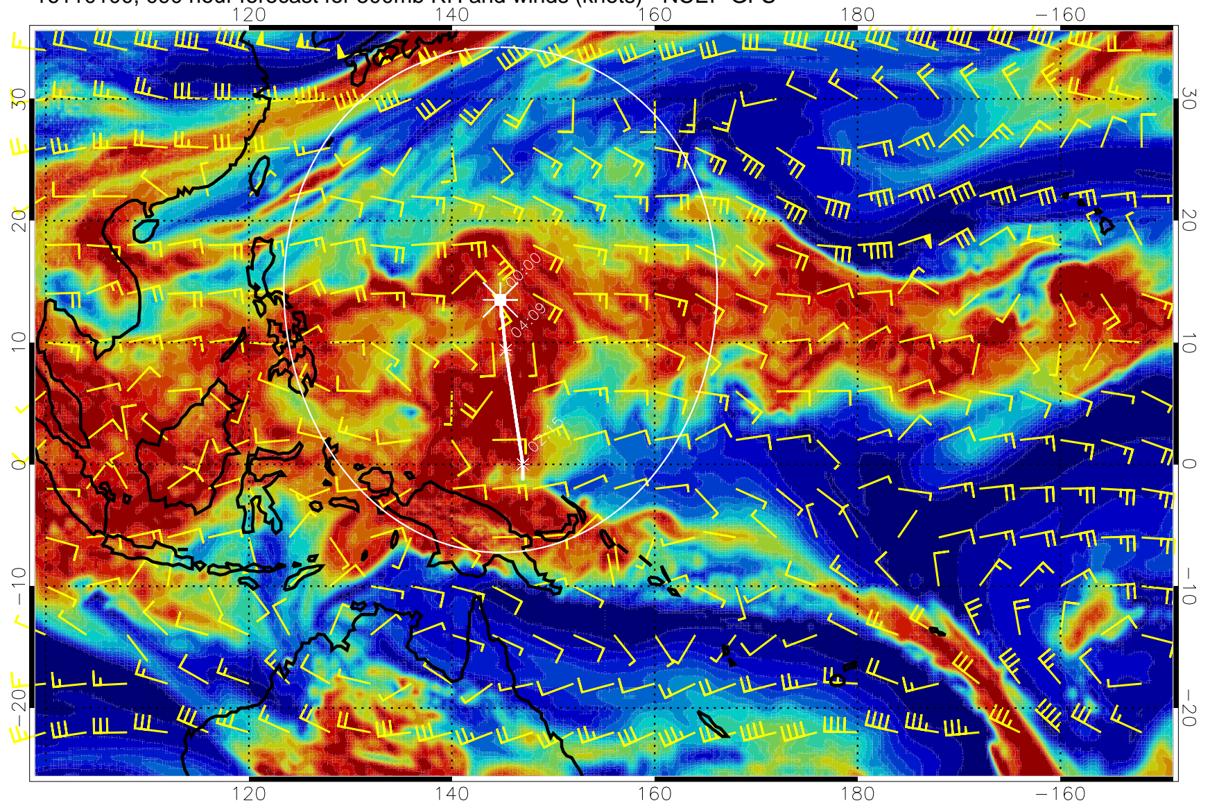
16110100, 090 hour forecast for 500mb RH and winds (knots) - NCEP GFS
