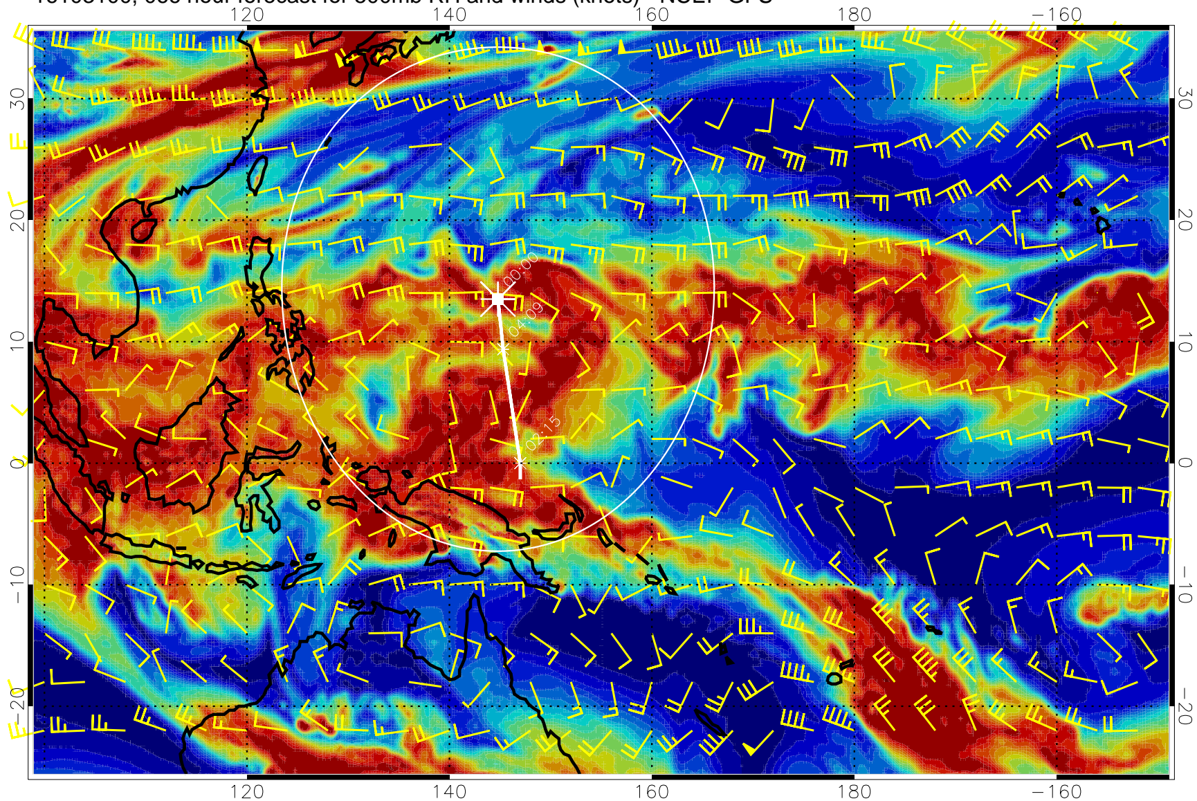
16103100, 066 hour forecast for 500mb RH and winds (knots) - NCEP GFS
