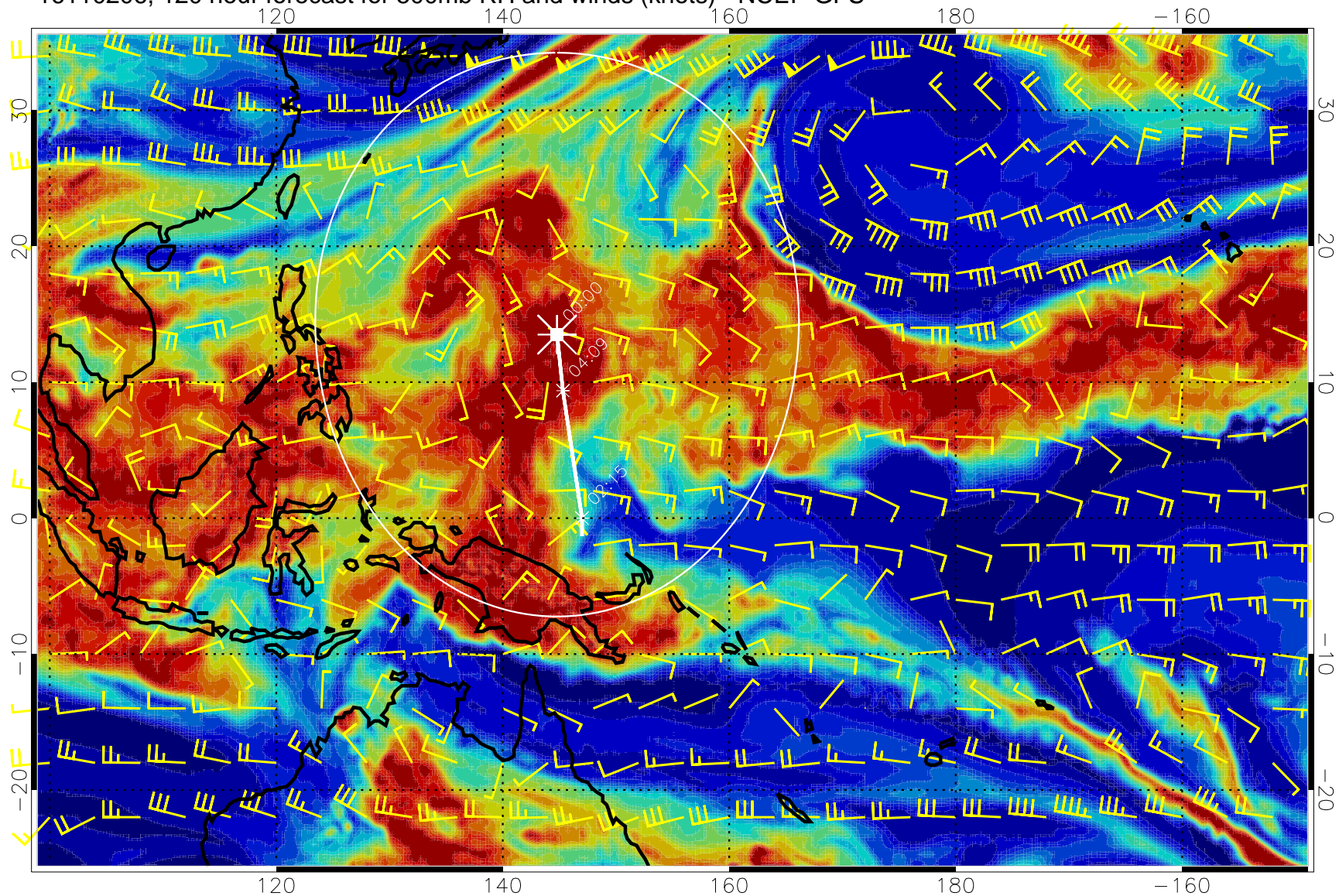
16110206, 120 hour forecast for 500mb RH and winds (knots) - NCEP GFS
