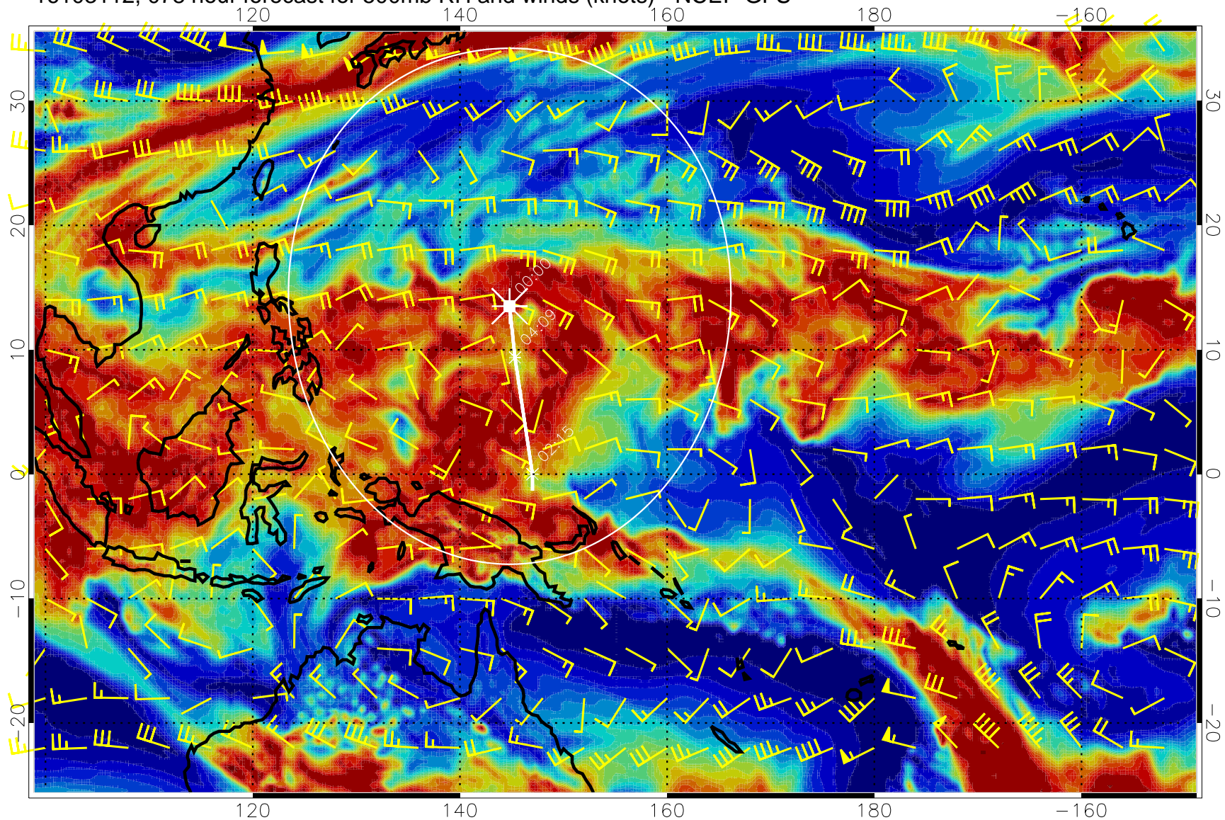
16103112, 078 hour forecast for 500mb RH and winds (knots) - NCEP GFS
