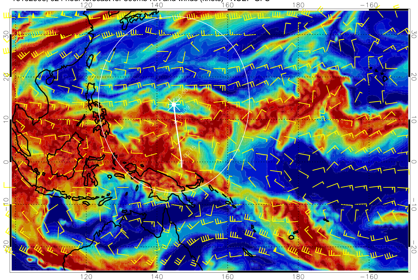
16102906, 024 hour forecast for 500mb RH and winds (knots) - NCEP GFS
