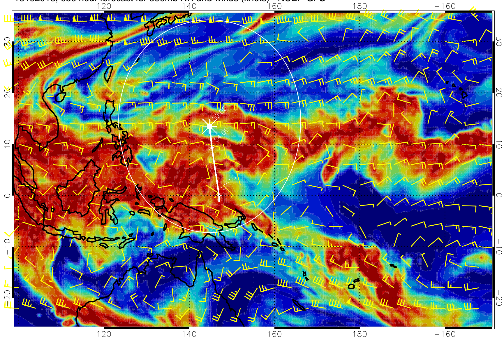
16102918, 036 hour forecast for 500mb RH and winds (knots) - NCEP GFS
