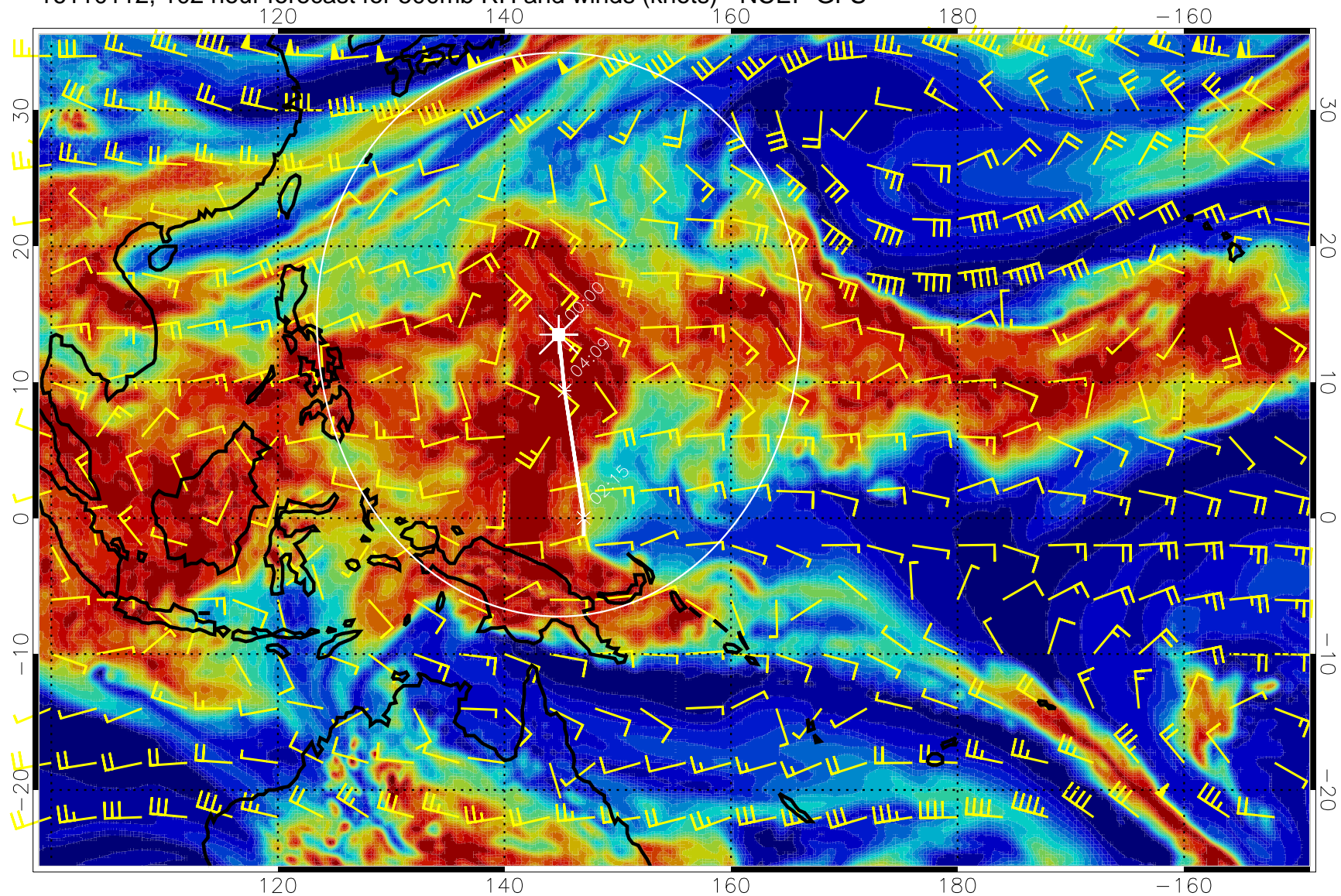
16110112, 102 hour forecast for 500mb RH and winds (knots) - NCEP GFS
