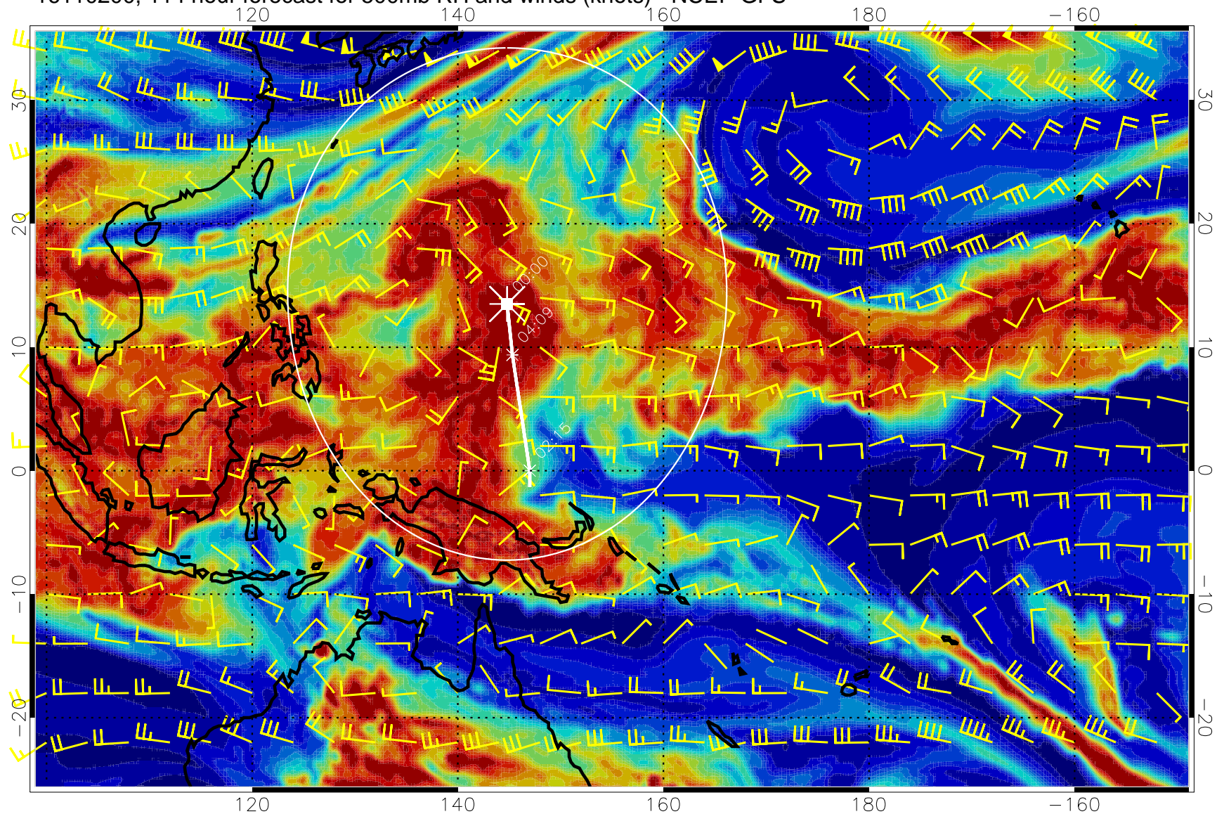
16110200, 114 hour forecast for 500mb RH and winds (knots) - NCEP GFS
