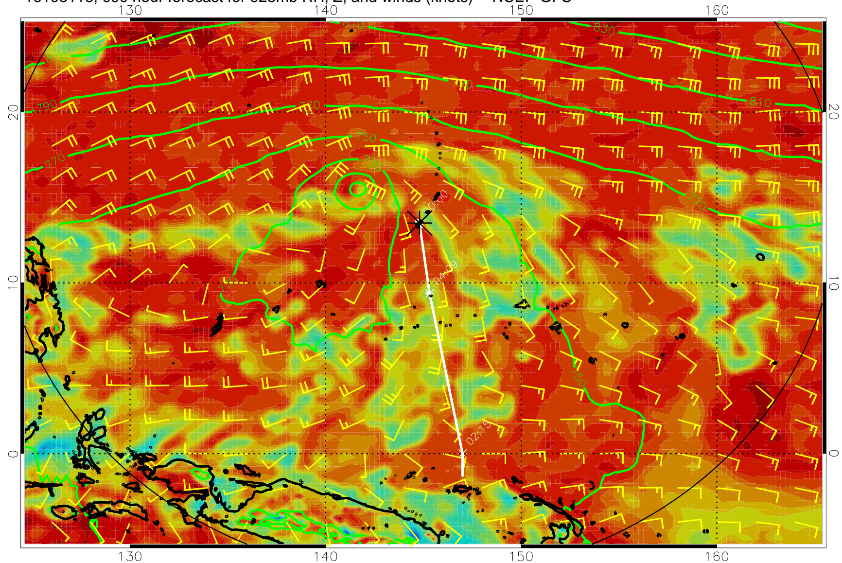
16103118, 090 hour forecast for 925mb RH, Z, and winds (knots) -- NCEP GFS
