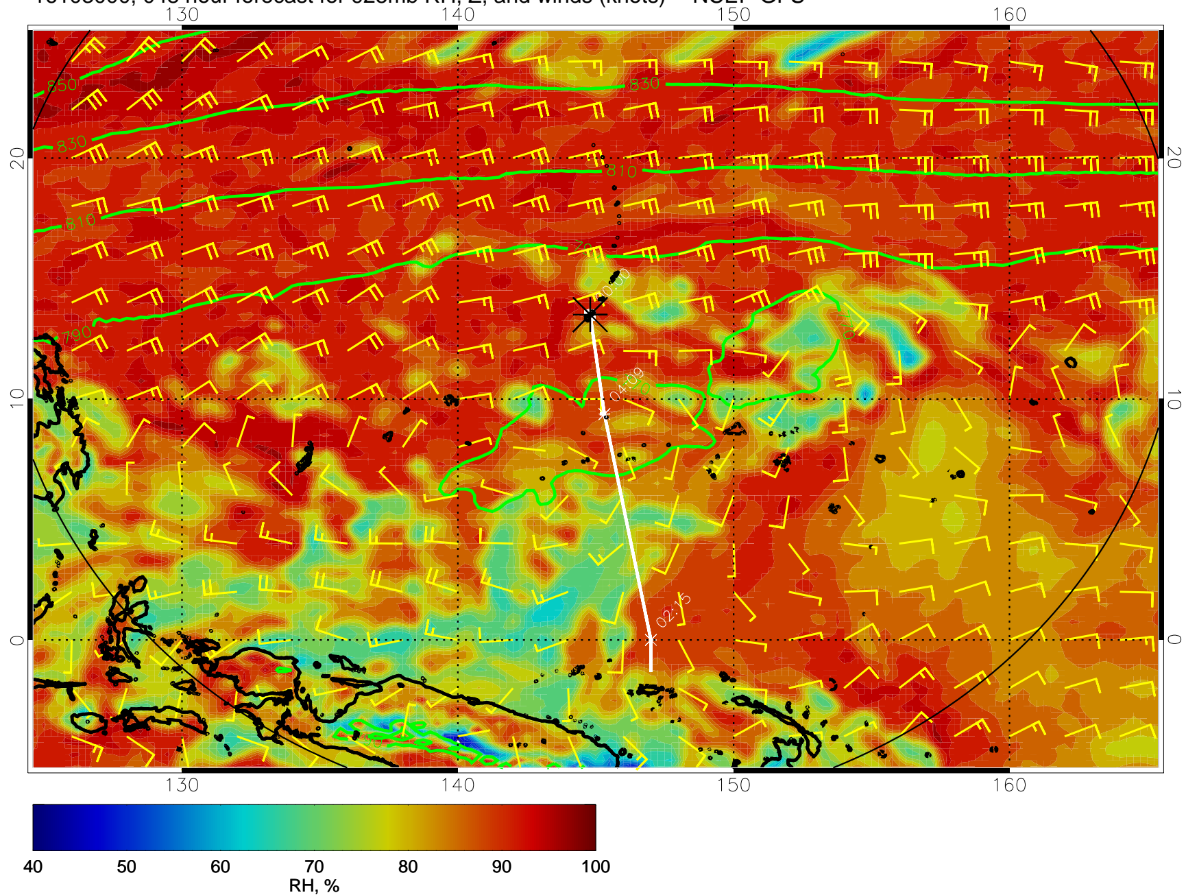
16103000, 048 hour forecast for 925mb RH, Z, and winds (knots) -- NCEP GFS
