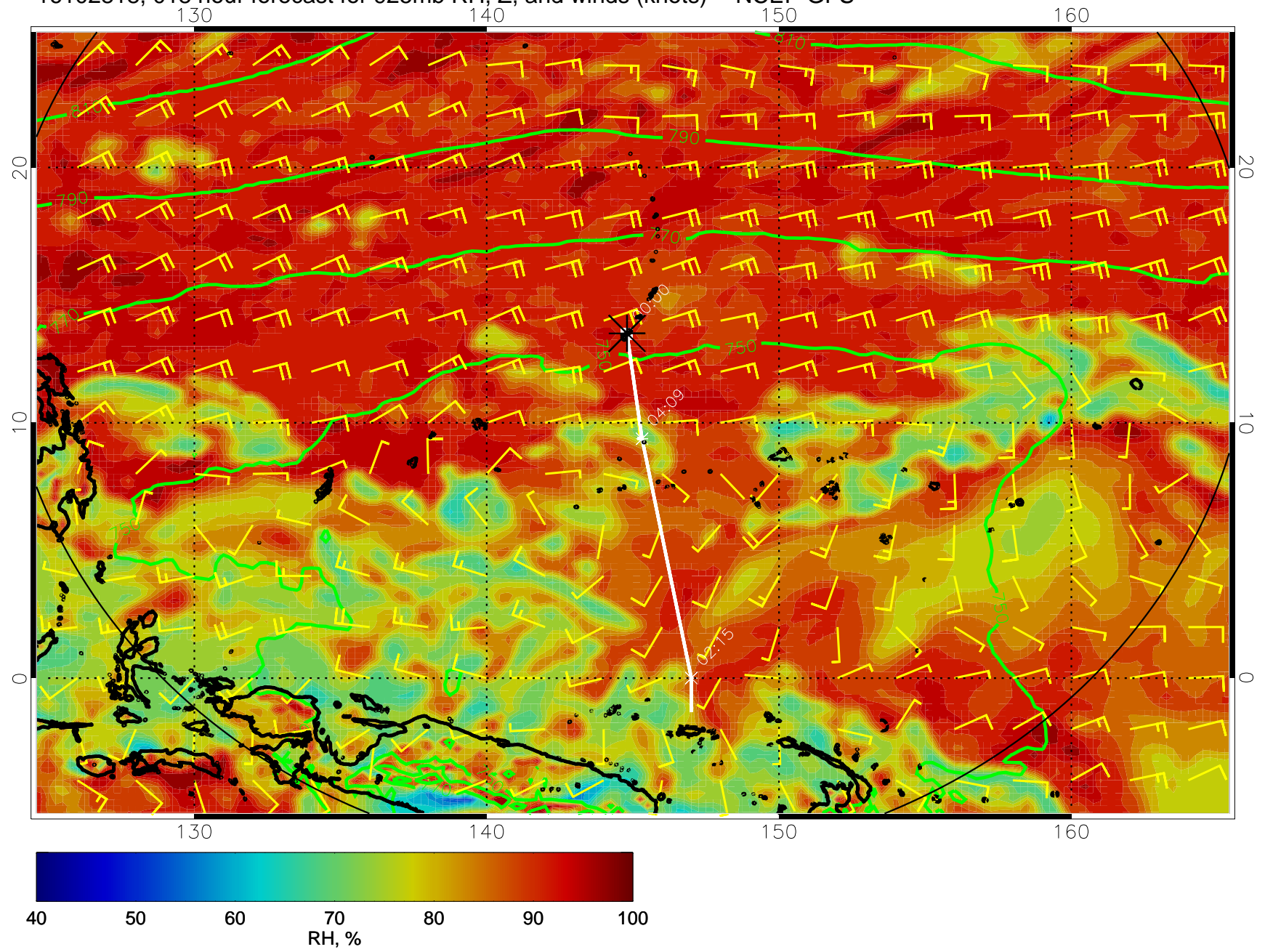
16102818, 018 hour forecast for 925mb RH, Z, and winds (knots) -- NCEP GFS
