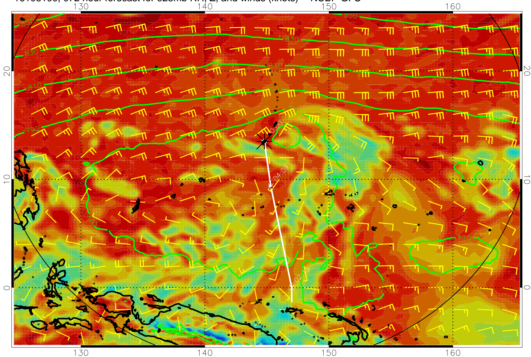
16103100, 072 hour forecast for 925mb RH, Z, and winds (knots) -- NCEP GFS
