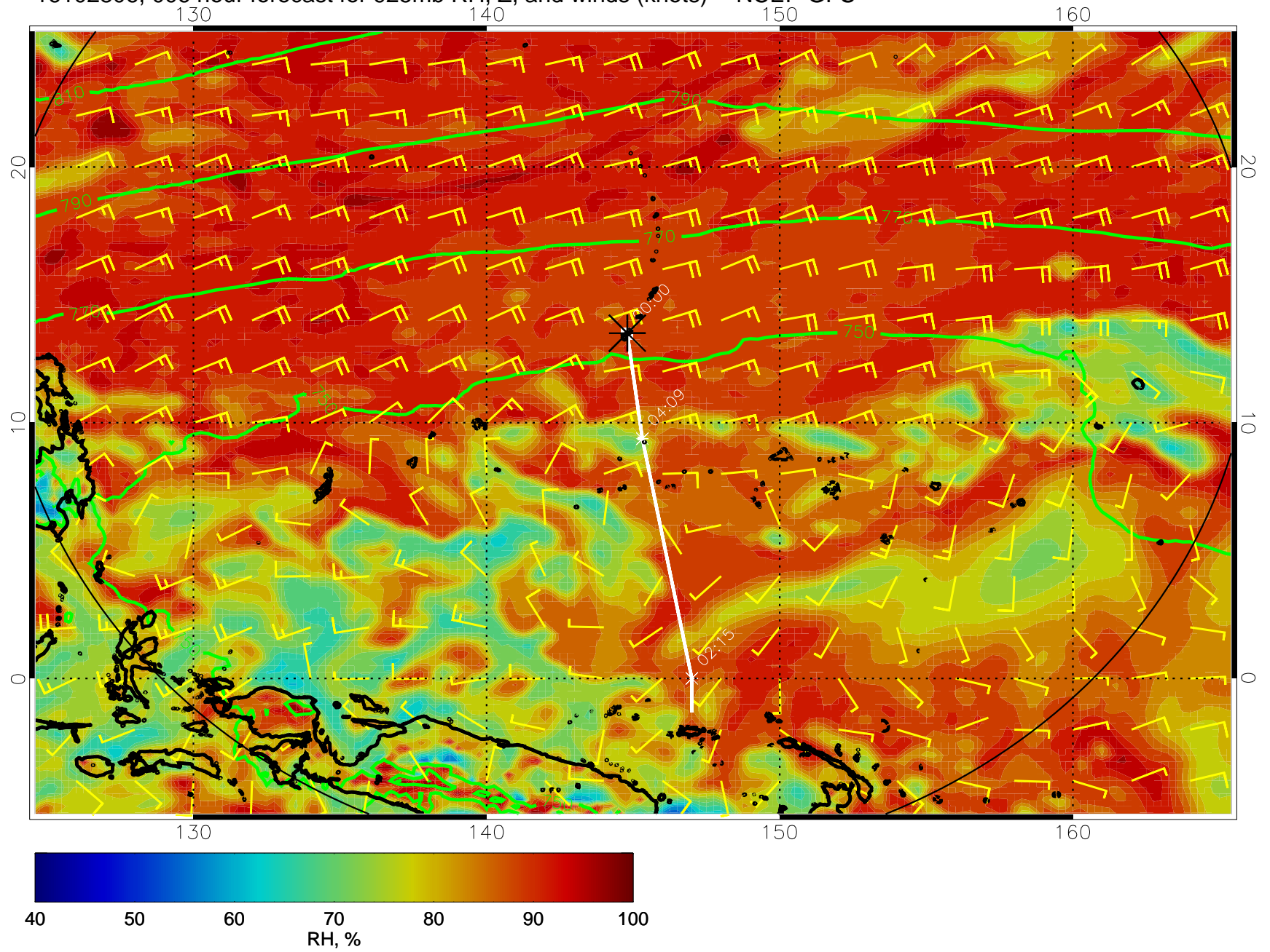
16102806, 006 hour forecast for 925mb RH, Z, and winds (knots) -- NCEP GFS
