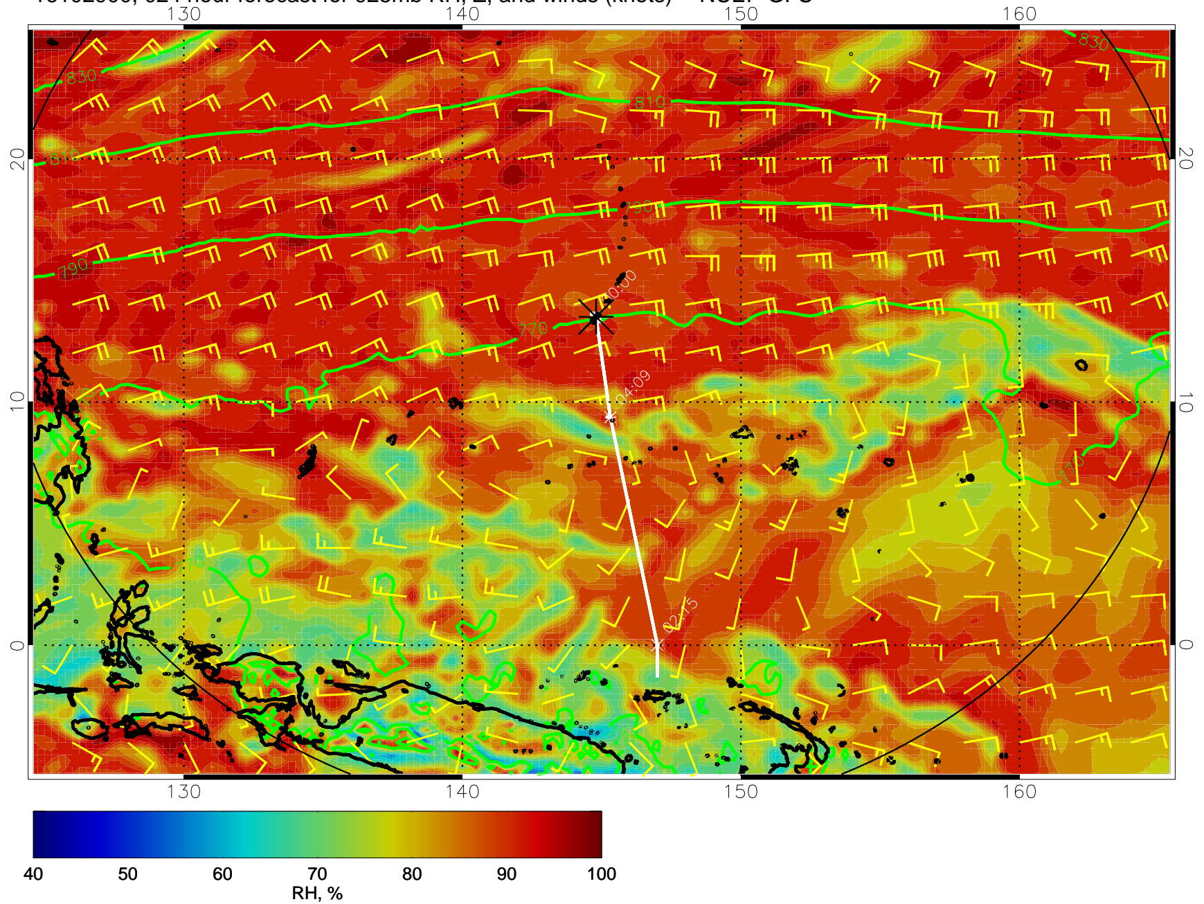
16102900, 024 hour forecast for 925mb RH, Z, and winds (knots) -- NCEP GFS
