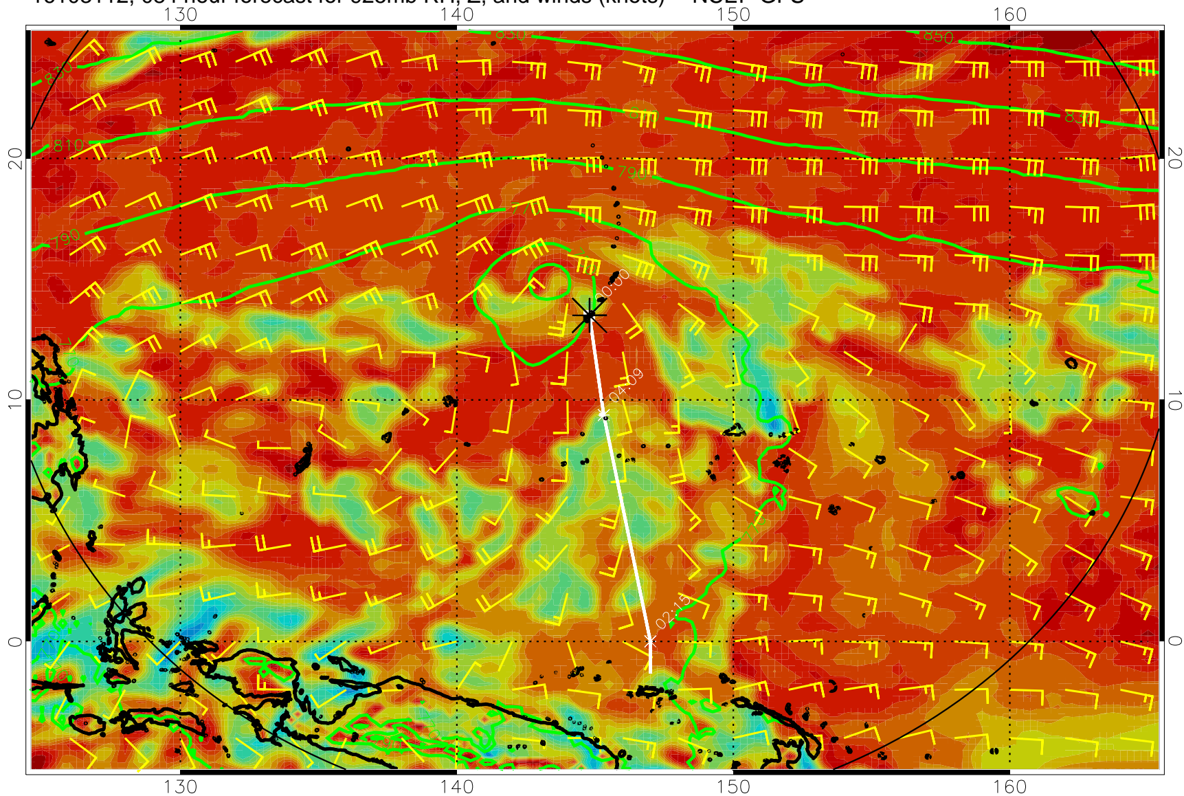
16103112, 084 hour forecast for 925mb RH, Z, and winds (knots) -- NCEP GFS
