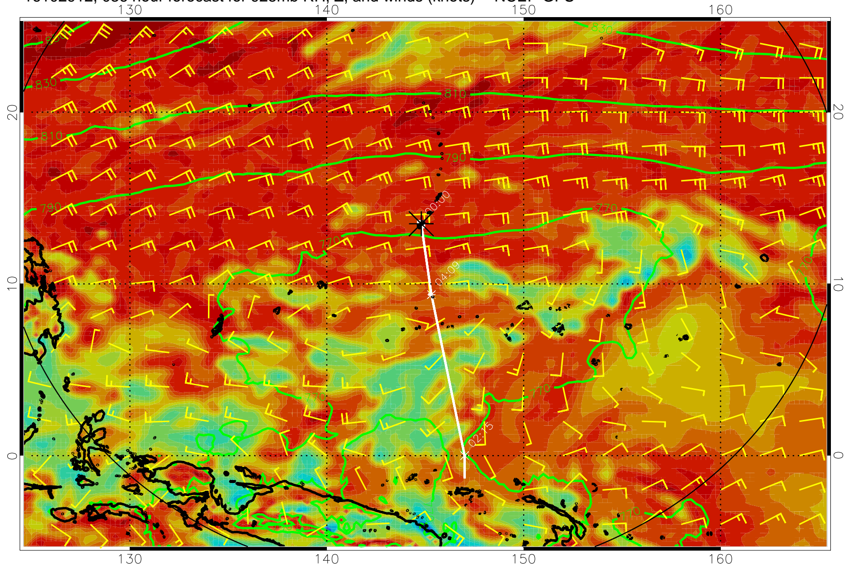
16102912, 036 hour forecast for 925mb RH, Z, and winds (knots) -- NCEP GFS
