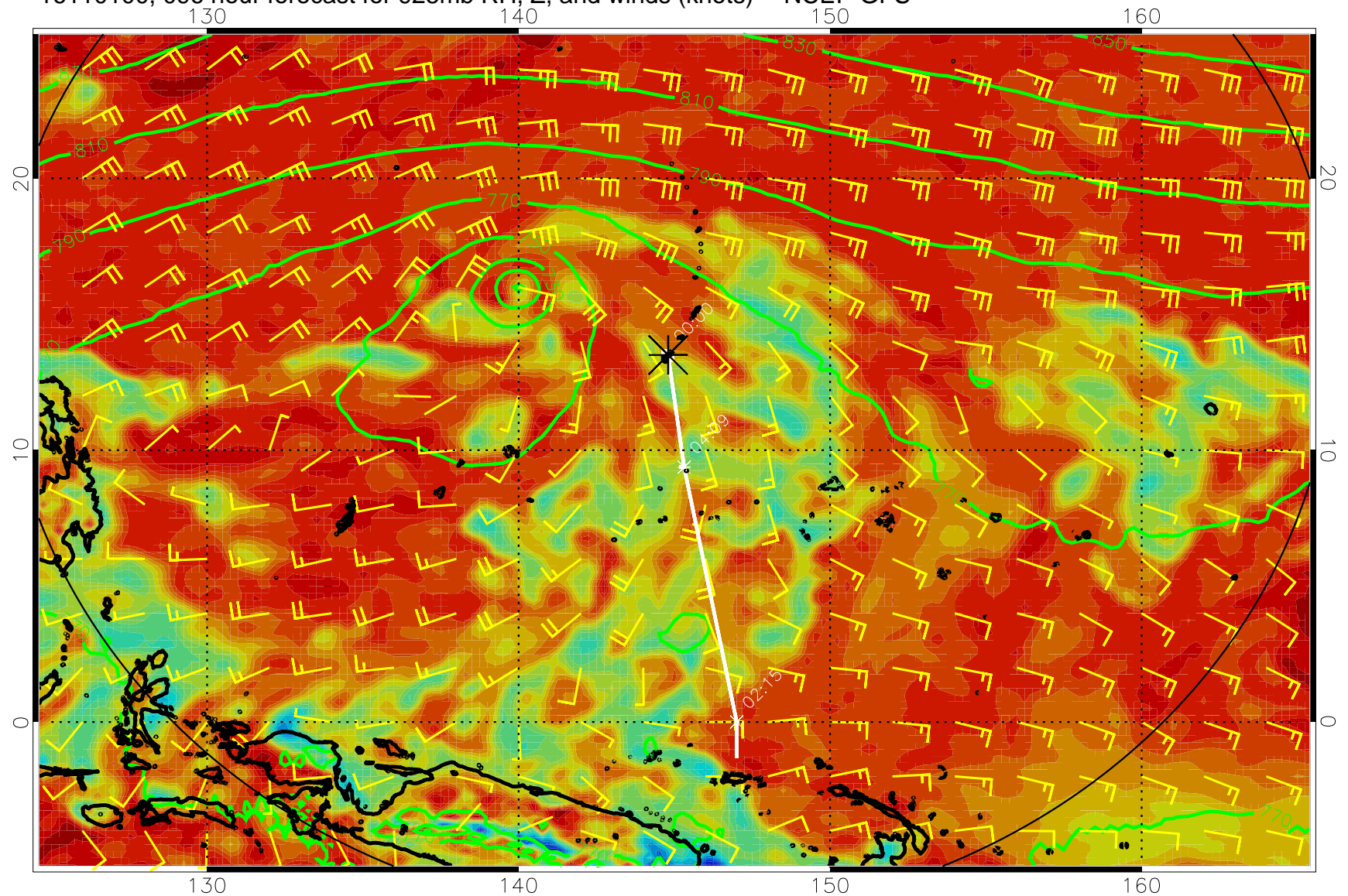
16110100, 096 hour forecast for 925mb RH, Z, and winds (knots) -- NCEP GFS
