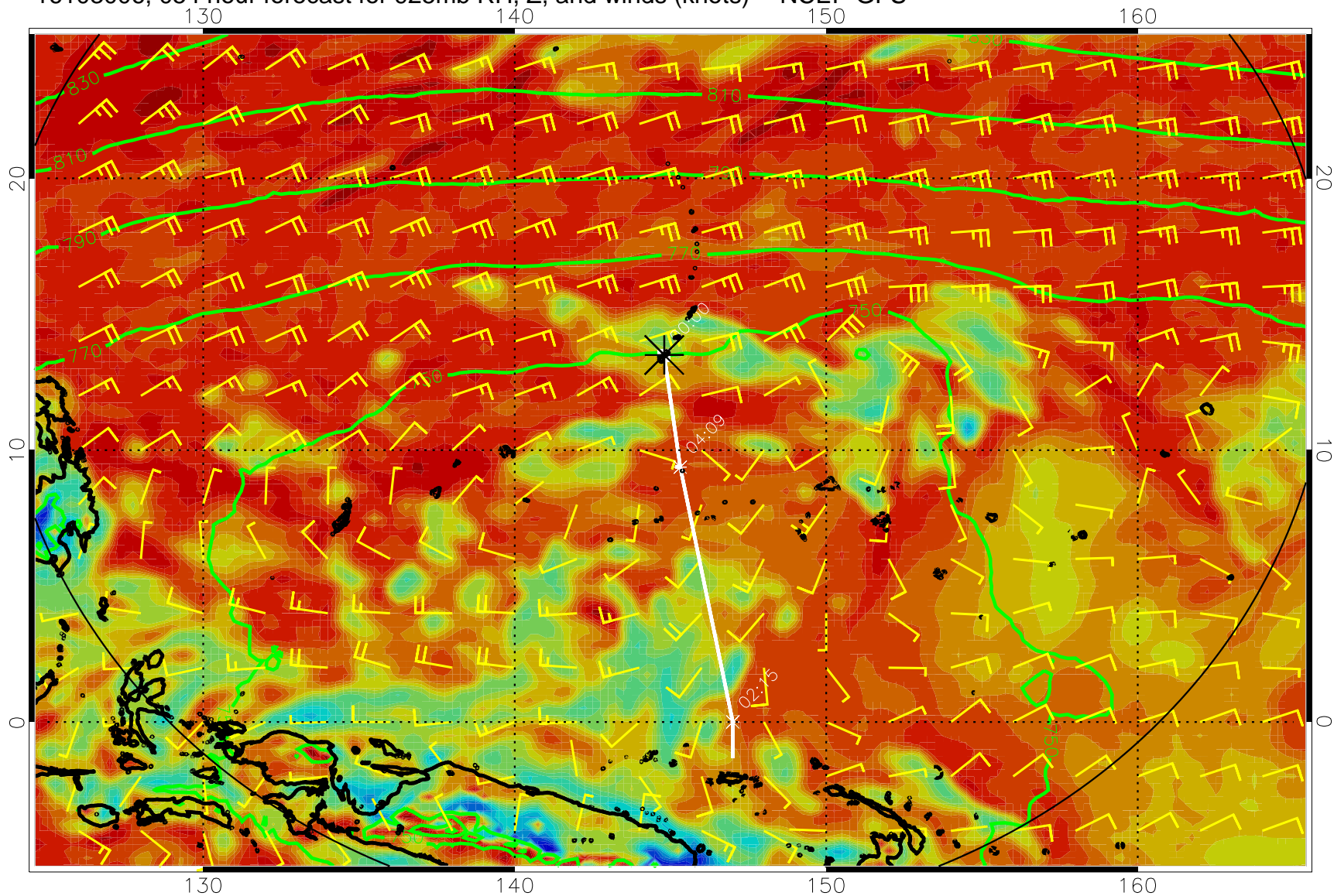
16103006, 054 hour forecast for 925mb RH, Z, and winds (knots) -- NCEP GFS
