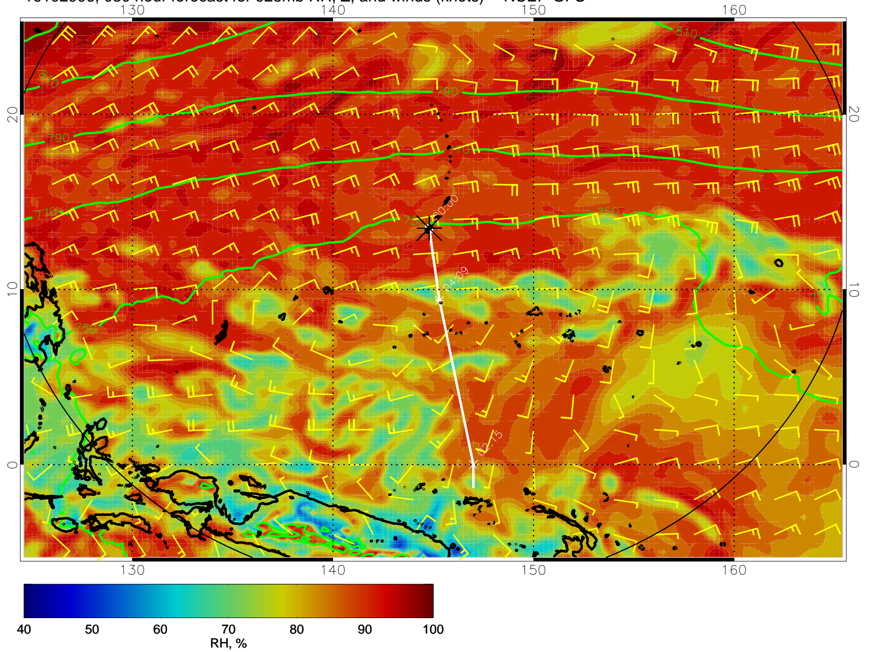
16102906, 030 hour forecast for 925mb RH, Z, and winds (knots) -- NCEP GFS
