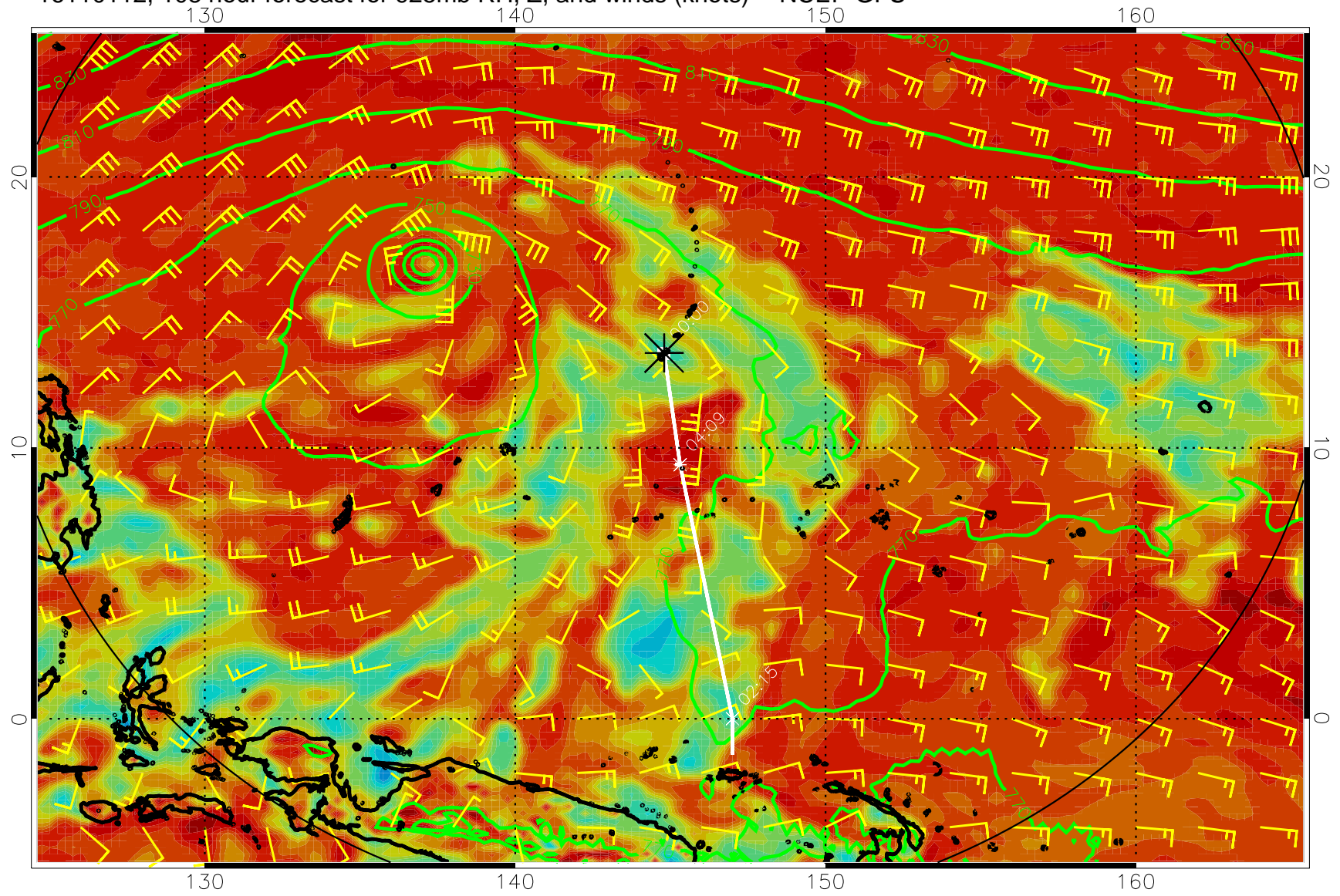
16110112, 108 hour forecast for 925mb RH, Z, and winds (knots) -- NCEP GFS
