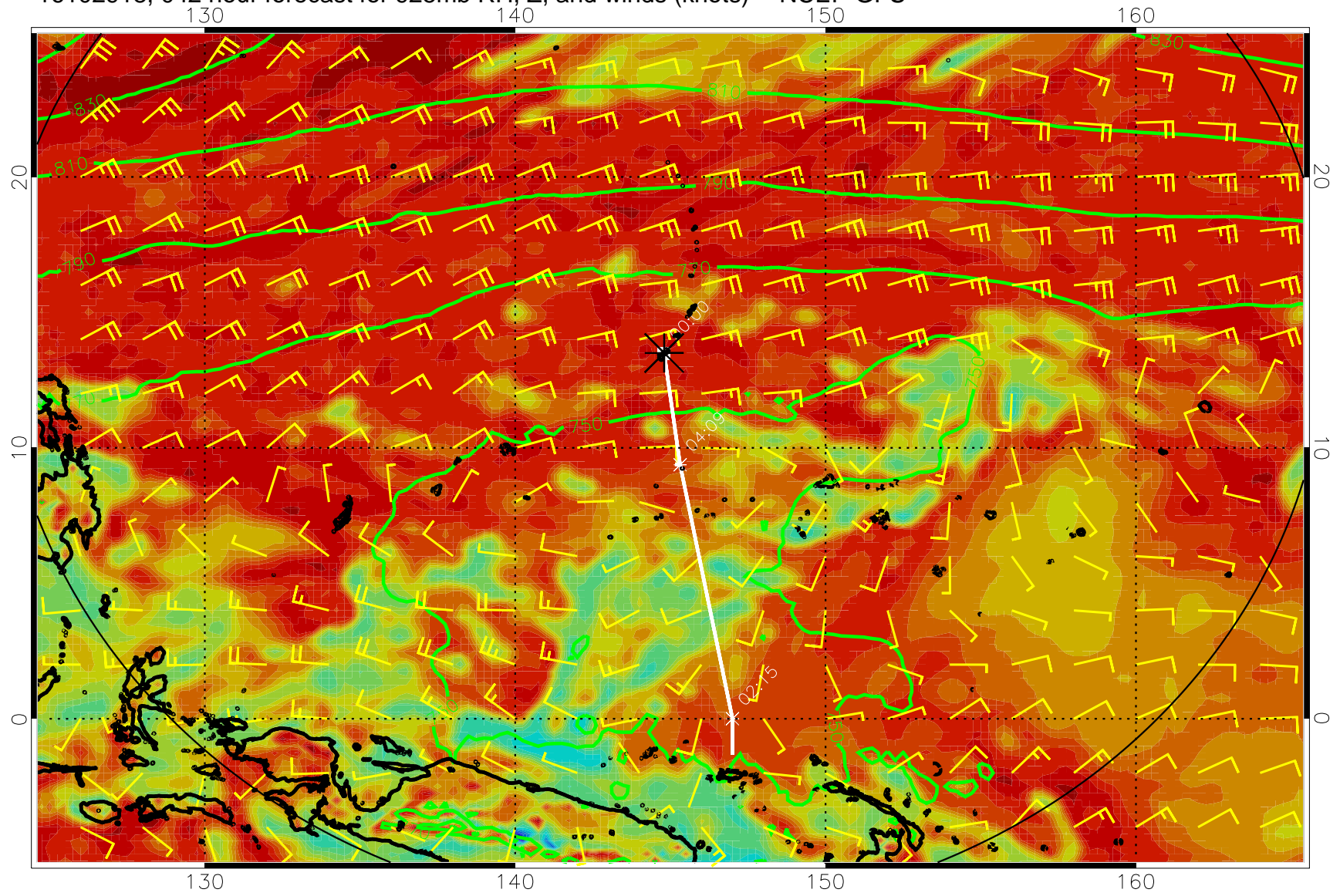
16102918, 042 hour forecast for 925mb RH, Z, and winds (knots) -- NCEP GFS
