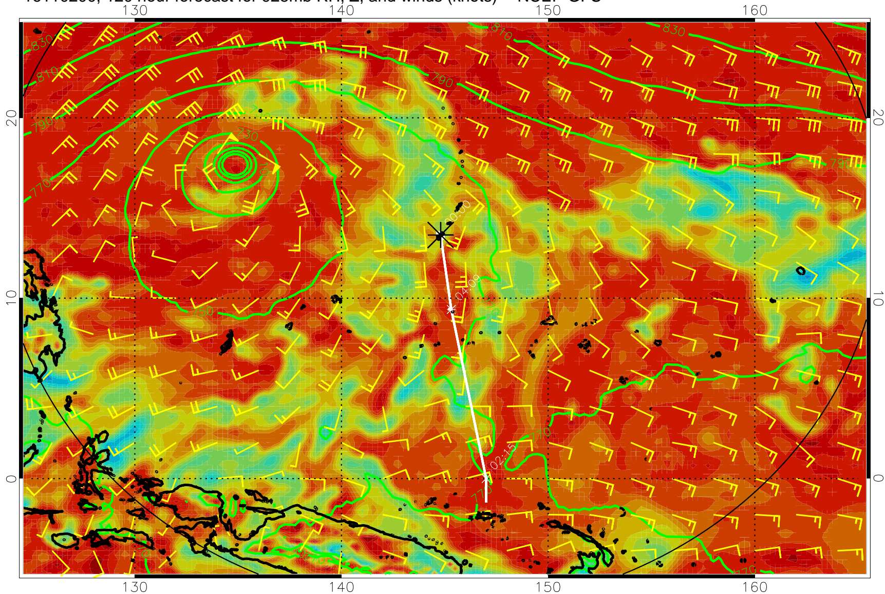
16110200, 120 hour forecast for 925mb RH, Z, and winds (knots) -- NCEP GFS
