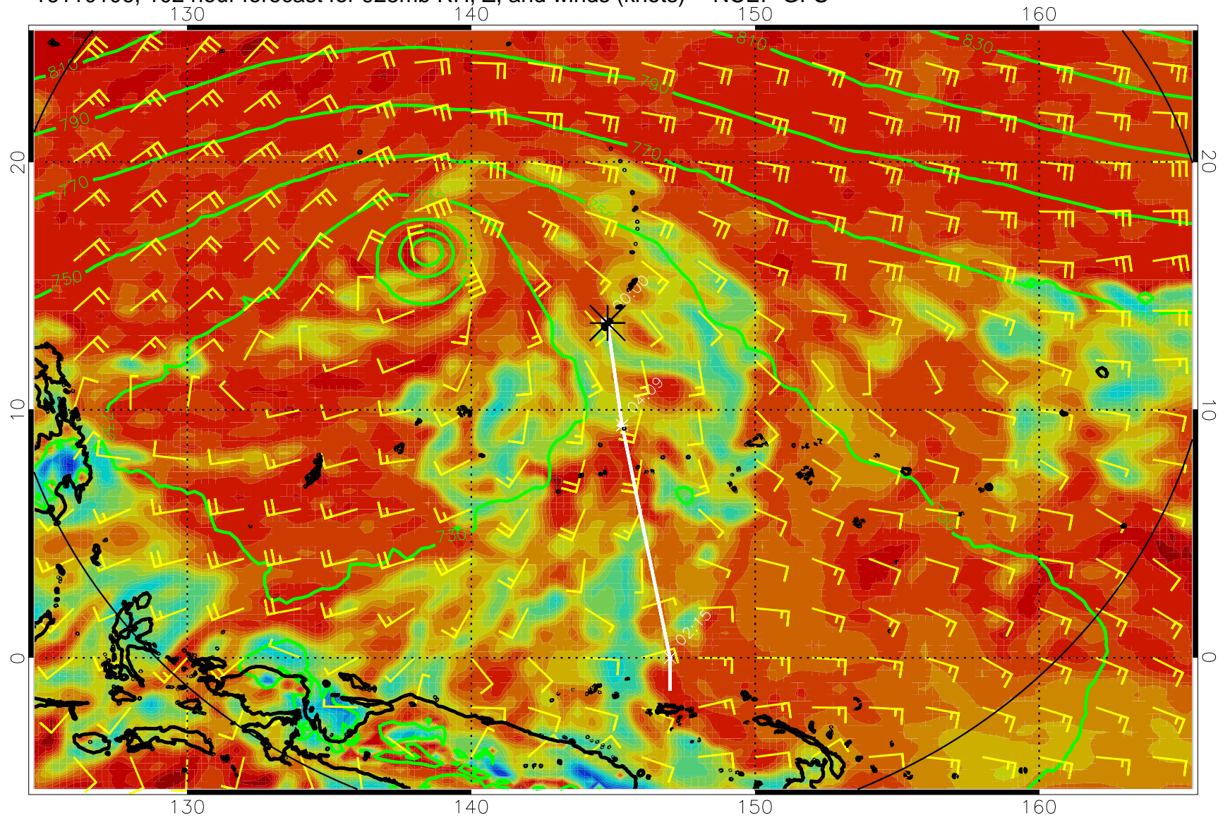
16110106, 102 hour forecast for 925mb RH, Z, and winds (knots) -- NCEP GFS
