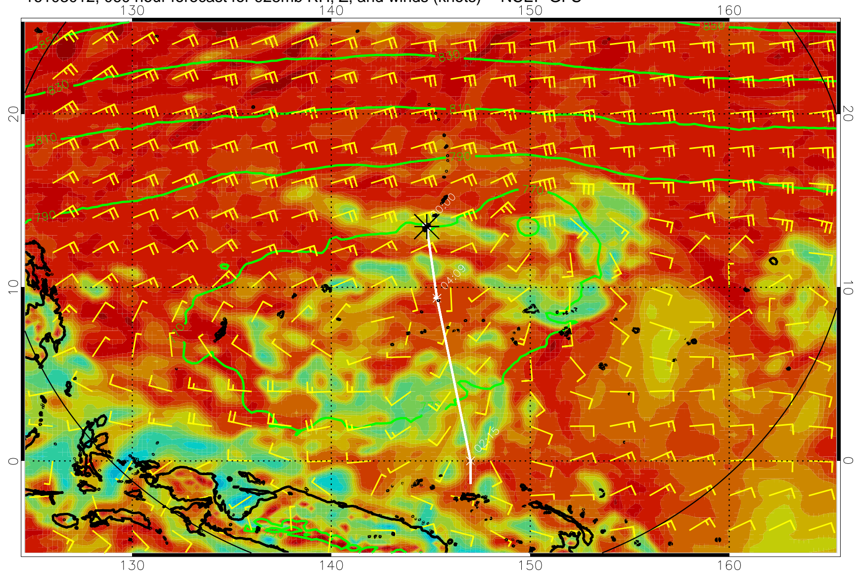
16103012, 060 hour forecast for 925mb RH, Z, and winds (knots) -- NCEP GFS
