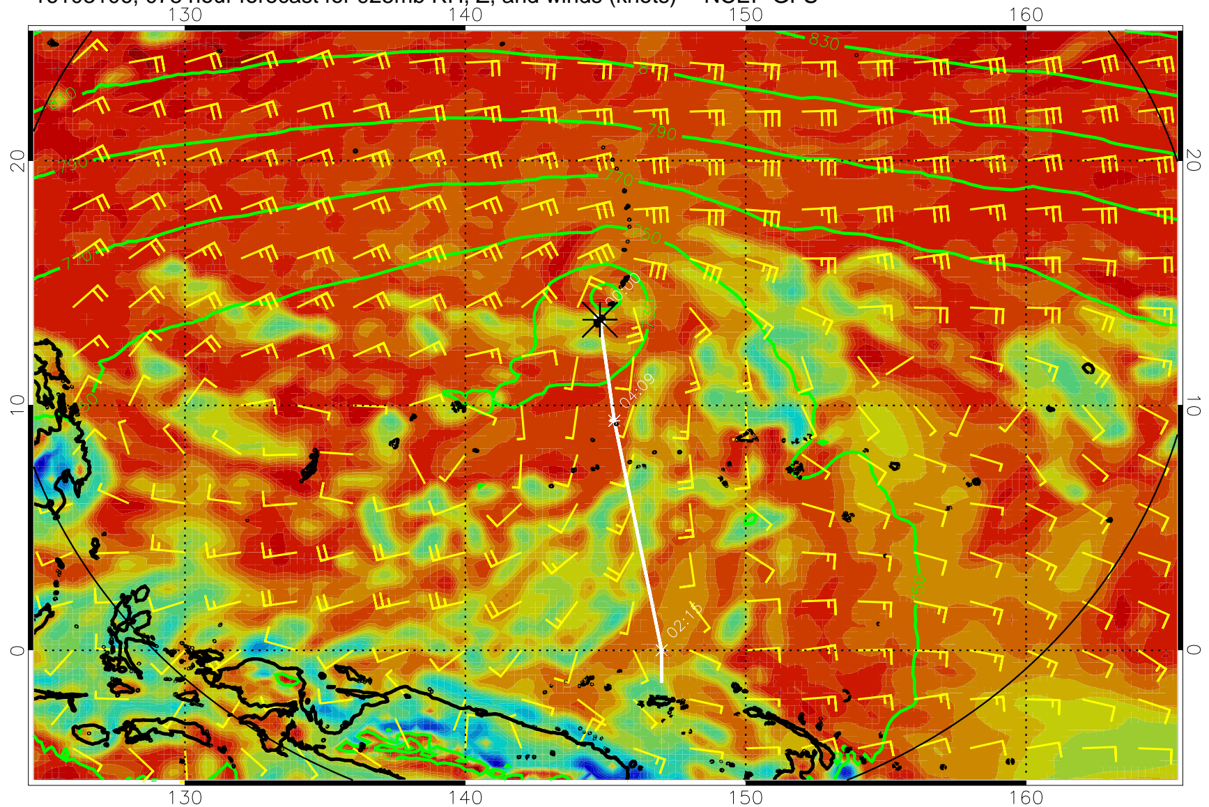
16103106, 078 hour forecast for 925mb RH, Z, and winds (knots) -- NCEP GFS
