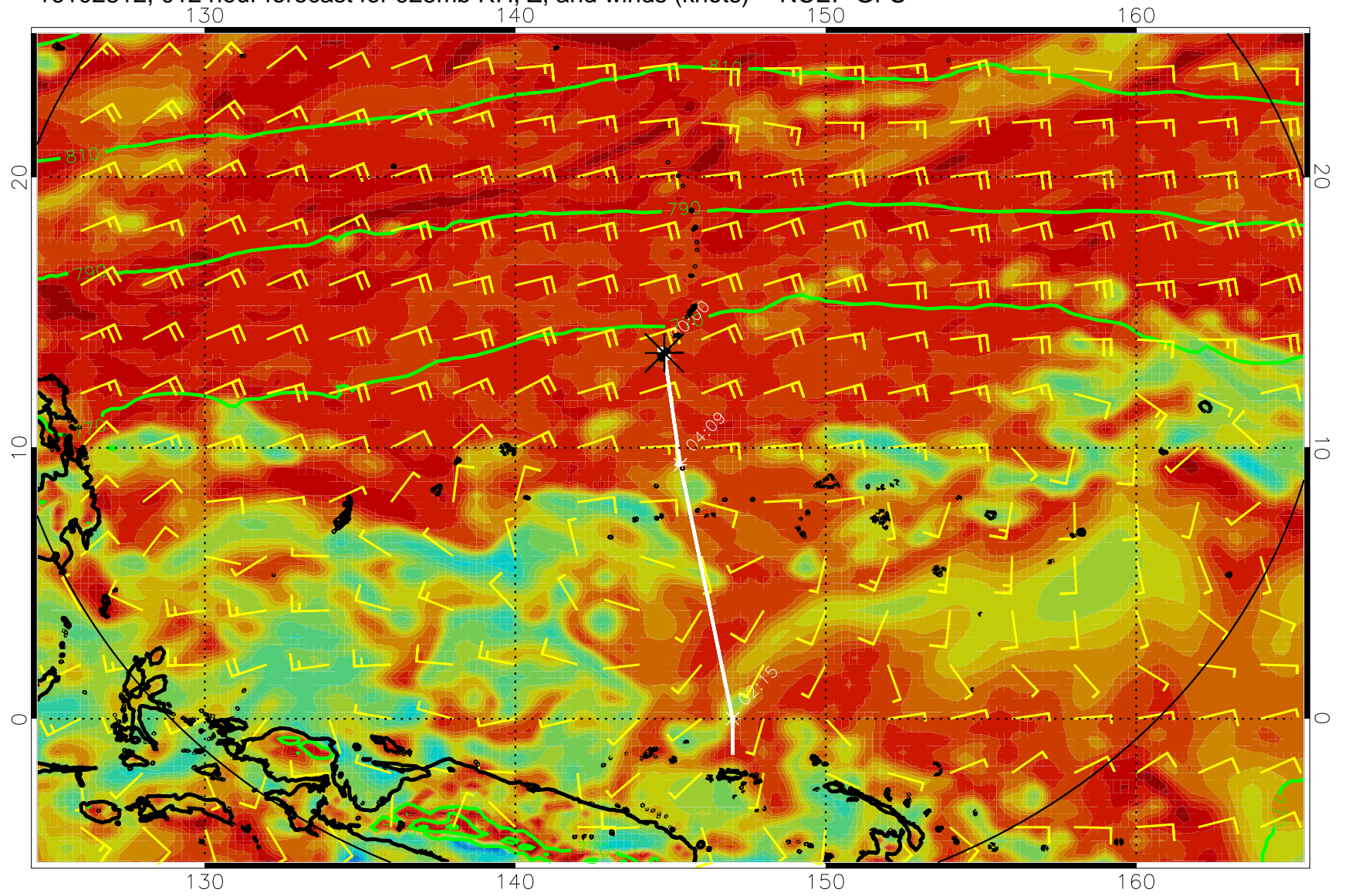
16102812, 012 hour forecast for 925mb RH, Z, and winds (knots) -- NCEP GFS
