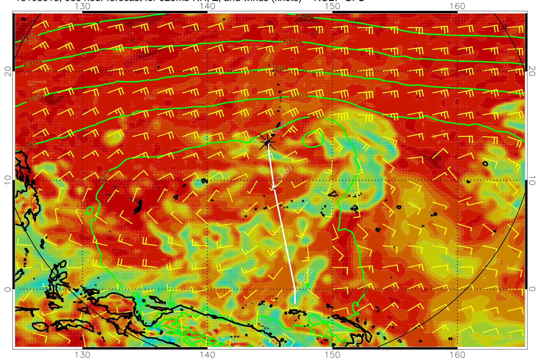
16103018, 066 hour forecast for 925mb RH, Z, and winds (knots) -- NCEP GFS
