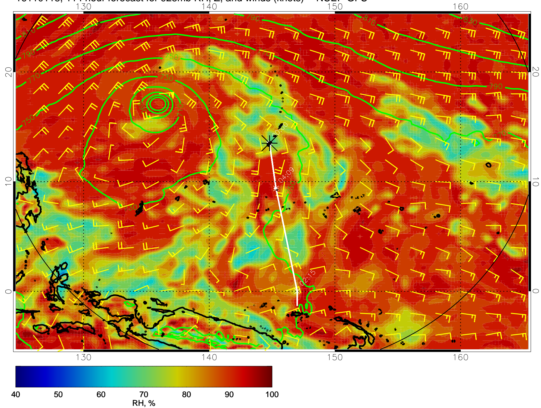
16110118, 114 hour forecast for 925mb RH, Z, and winds (knots) -- NCEP GFS
